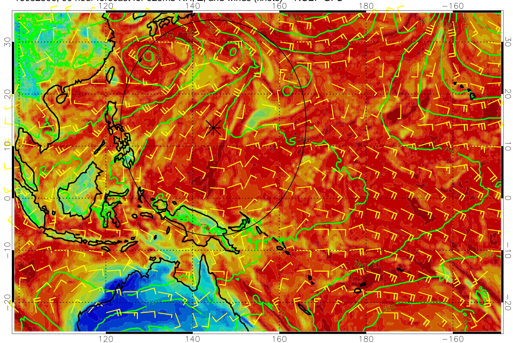
16082506, 90 hour forecast for 925mb RH, Z, and winds (knots) -- NCEP GFS
