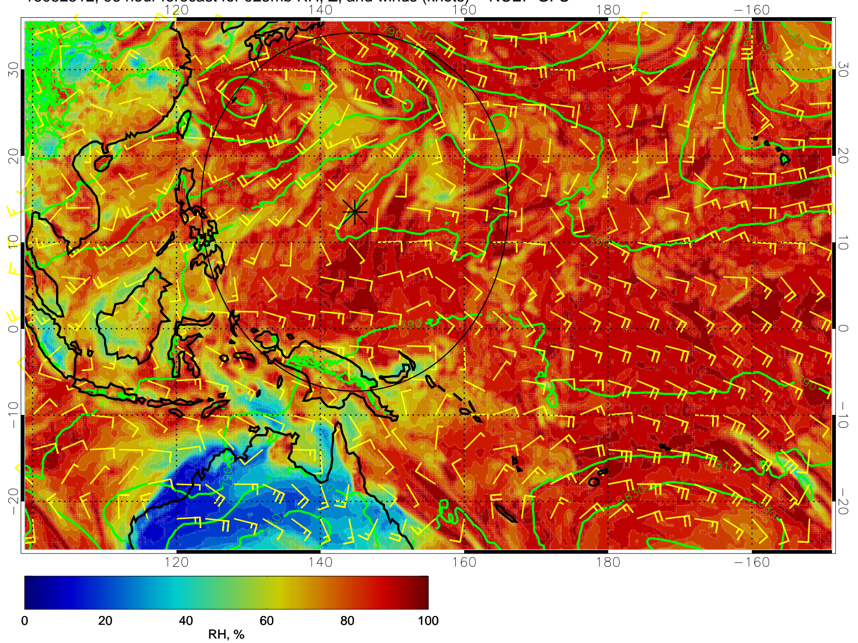
16082512, 96 hour forecast for 925mb RH, Z, and winds (knots) -- NCEP GFS
