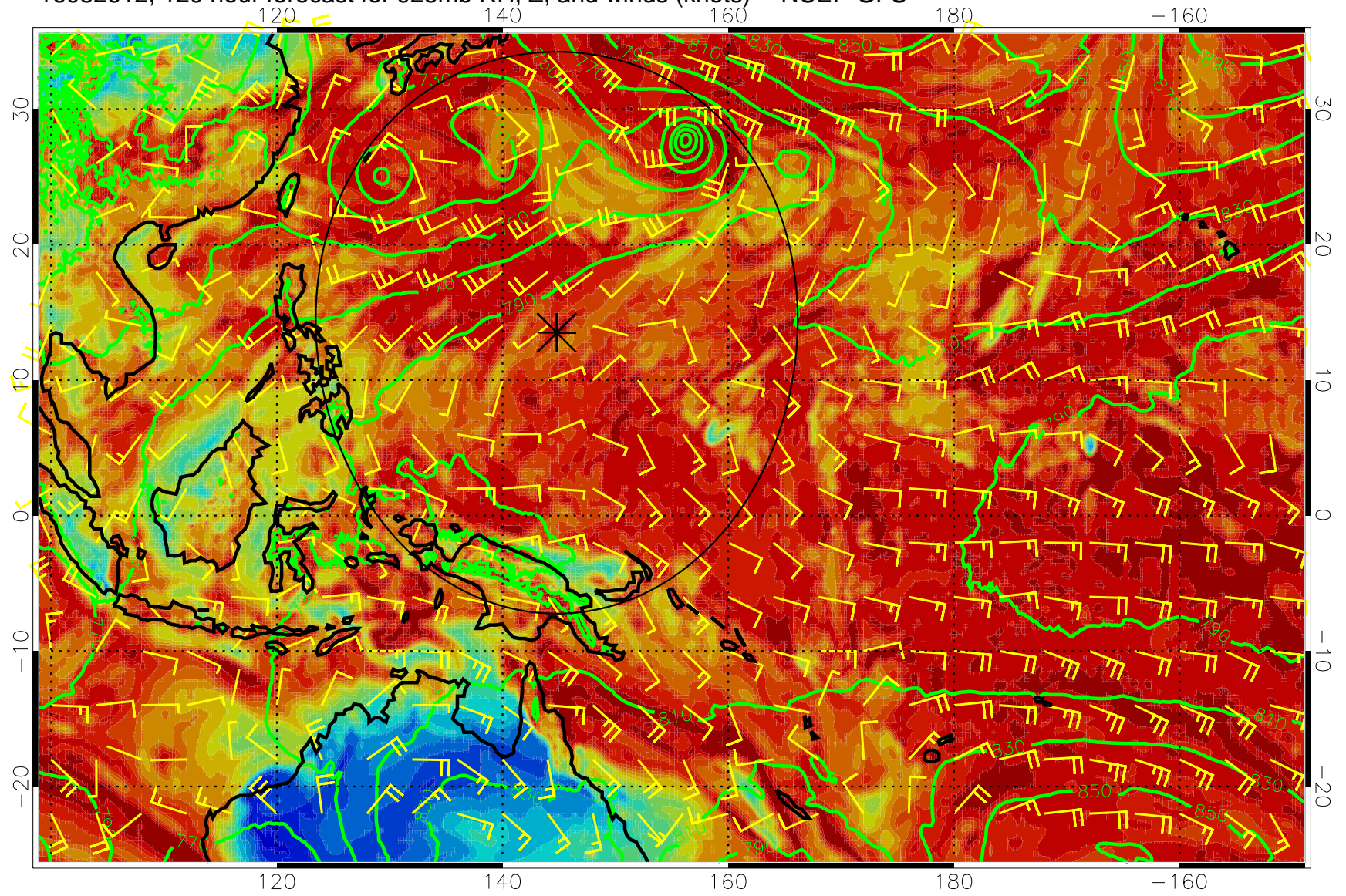
16082612, 120 hour forecast for 925mb RH, Z, and winds (knots) -- NCEP GFS
