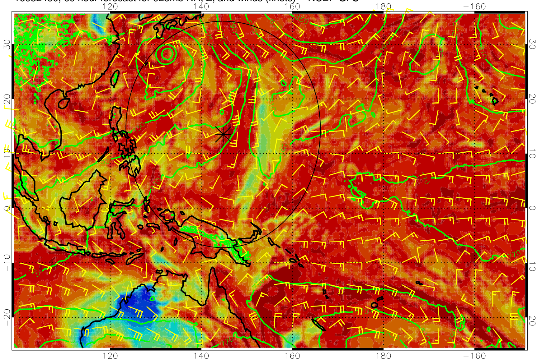
16082400, 60 hour forecast for 925mb RH, Z, and winds (knots) -- NCEP GFS
