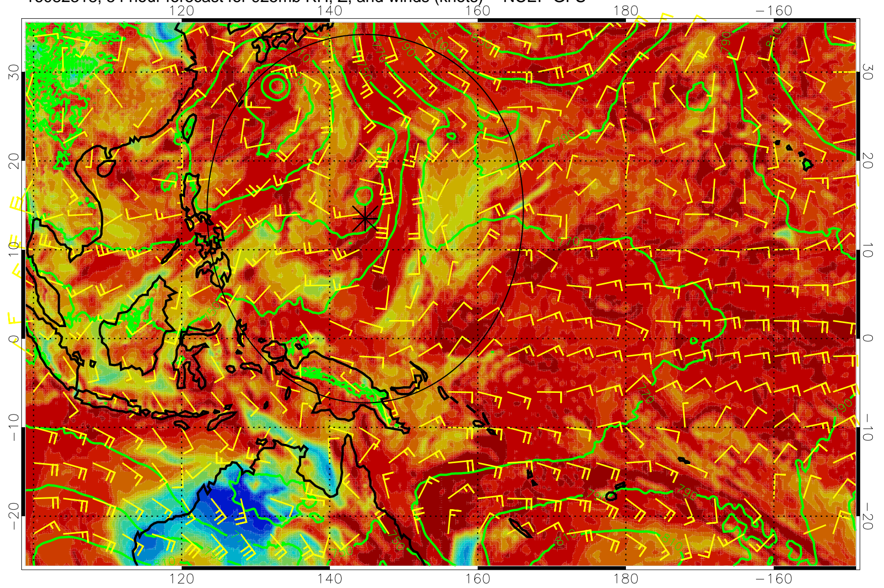
16082318, 54 hour forecast for 925mb RH, Z, and winds (knots) -- NCEP GFS
