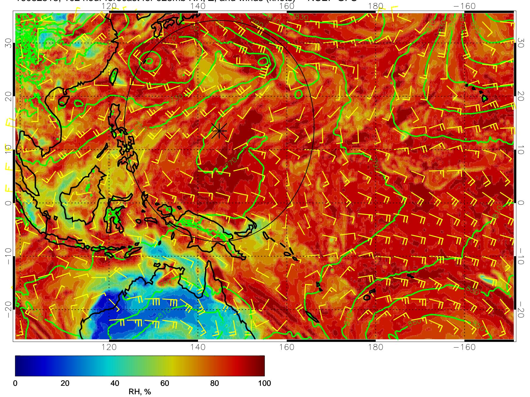
16082518, 102 hour forecast for 925mb RH, Z, and winds (knots) -- NCEP GFS
