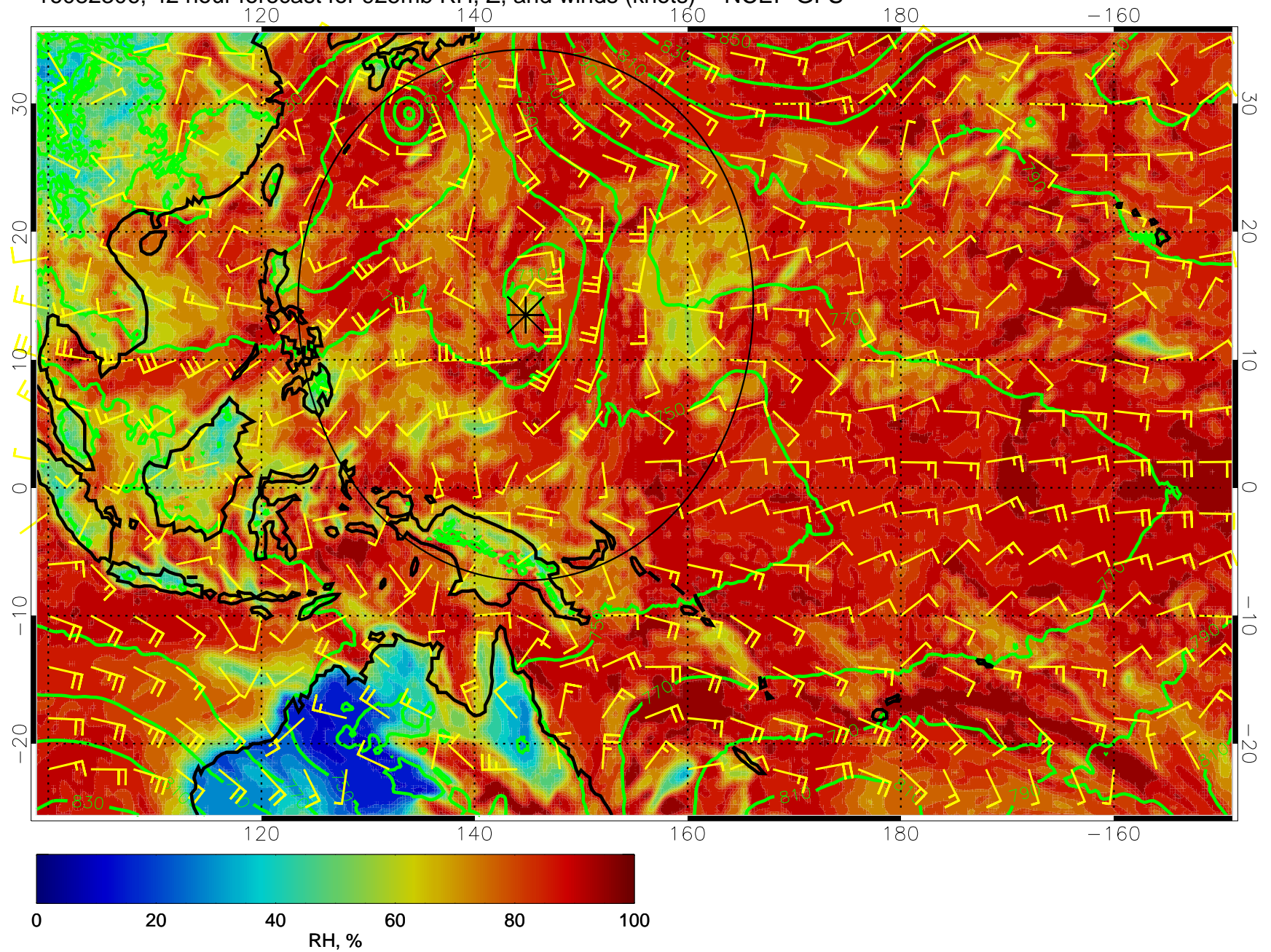
16082306, 42 hour forecast for 925mb RH, Z, and winds (knots) -- NCEP GFS
