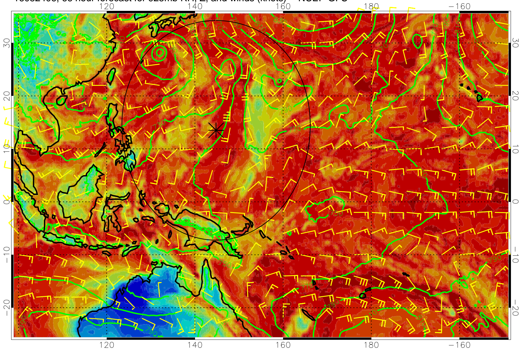
16082406, 66 hour forecast for 925mb RH, Z, and winds (knots) -- NCEP GFS
