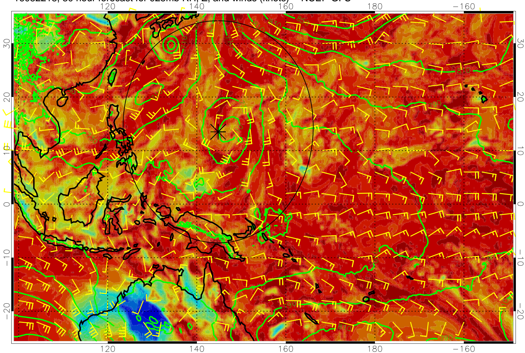
16082218, 30 hour forecast for 925mb RH, Z, and winds (knots) -- NCEP GFS
