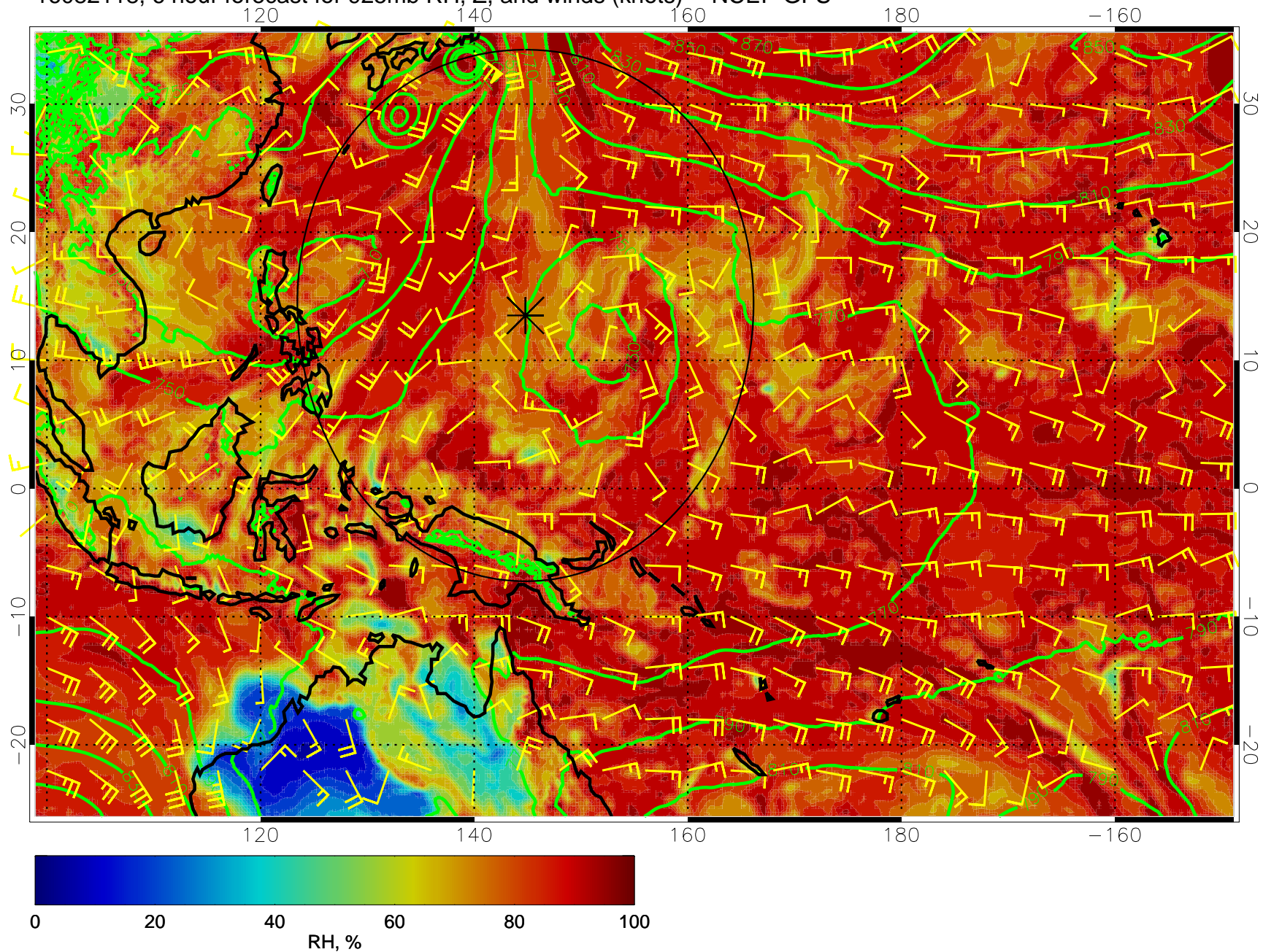
16082118, 6 hour forecast for 925mb RH, Z, and winds (knots) -- NCEP GFS
