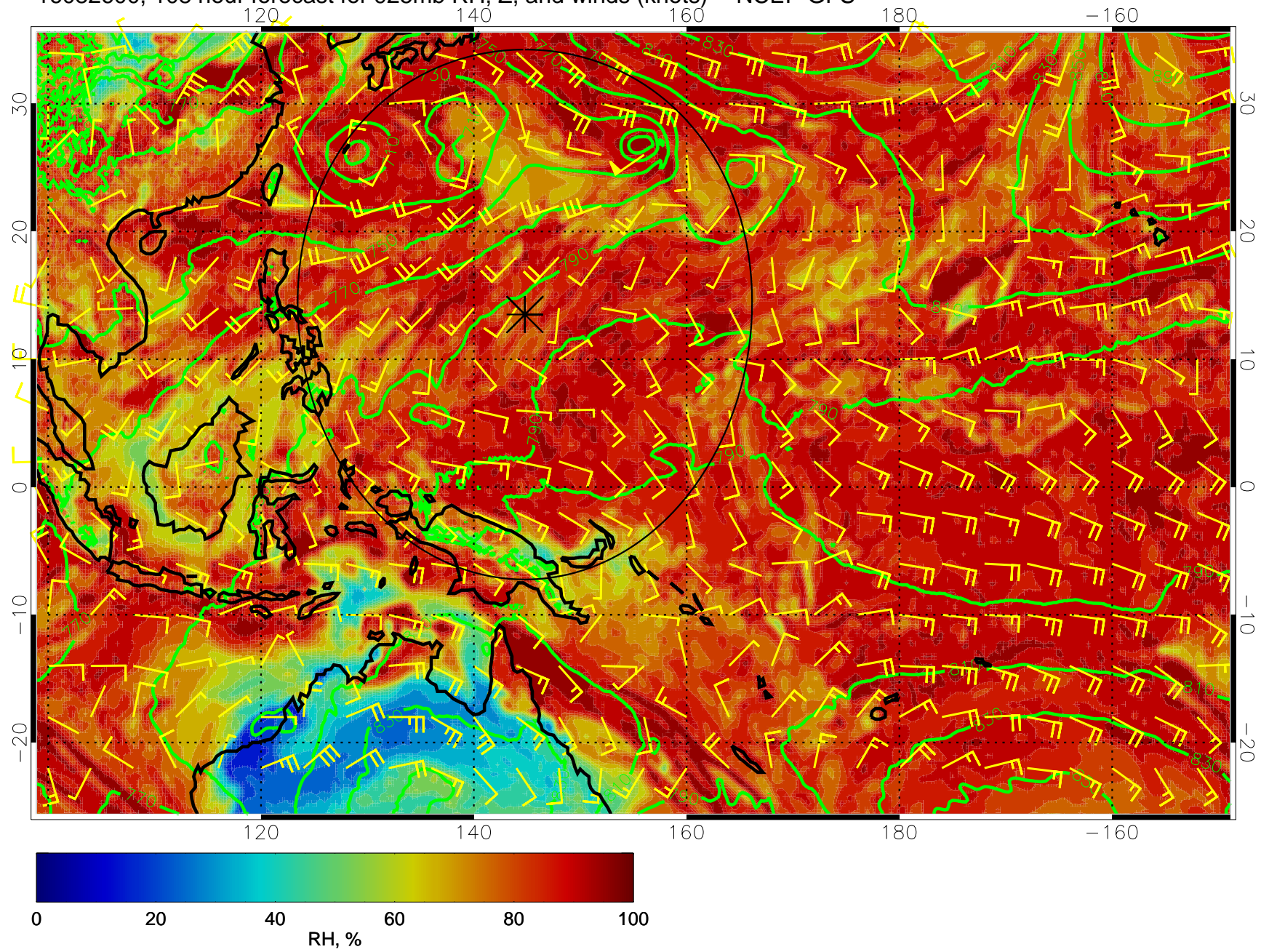
16082600, 108 hour forecast for 925mb RH, Z, and winds (knots) -- NCEP GFS
