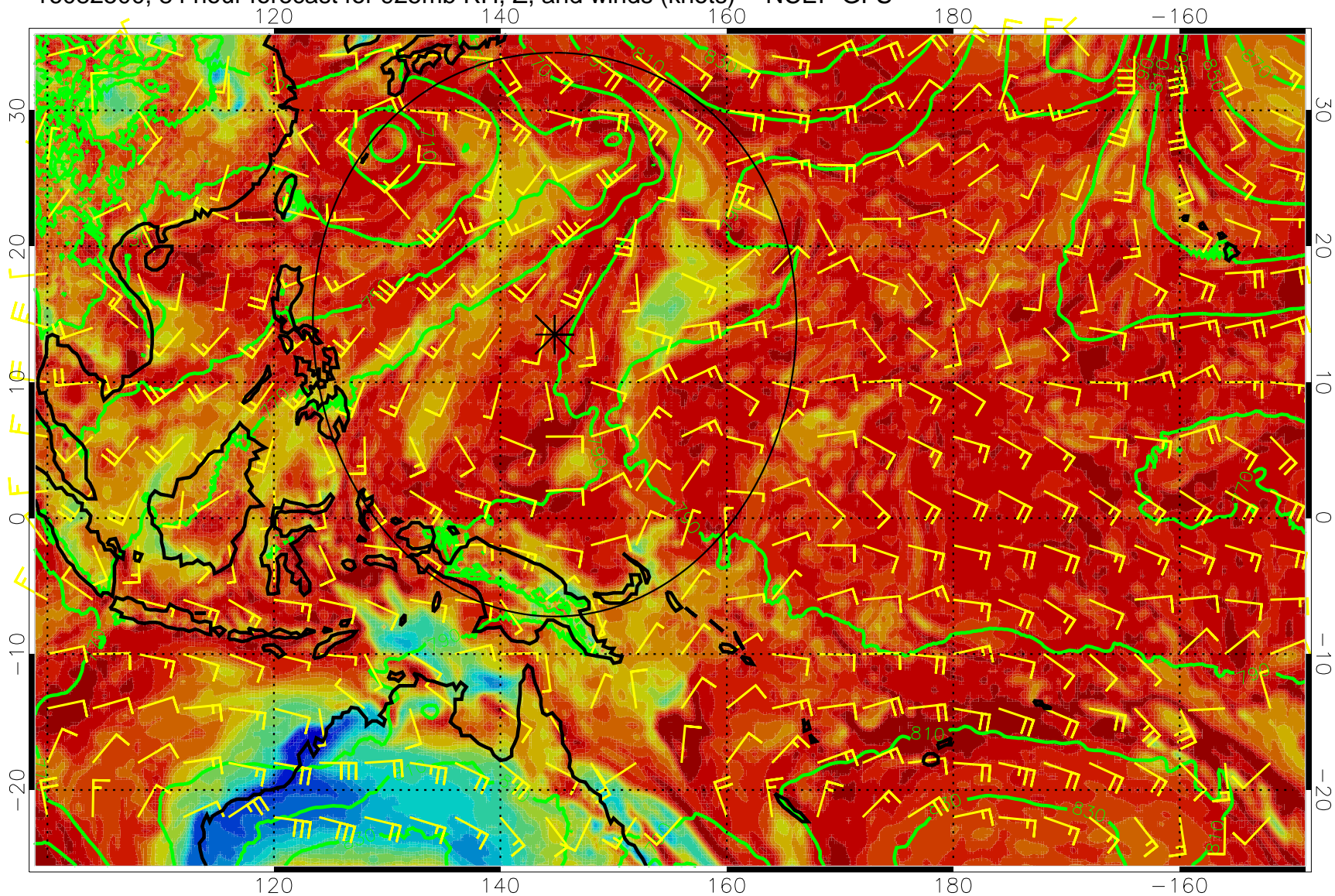
16082500, 84 hour forecast for 925mb RH, Z, and winds (knots) -- NCEP GFS
