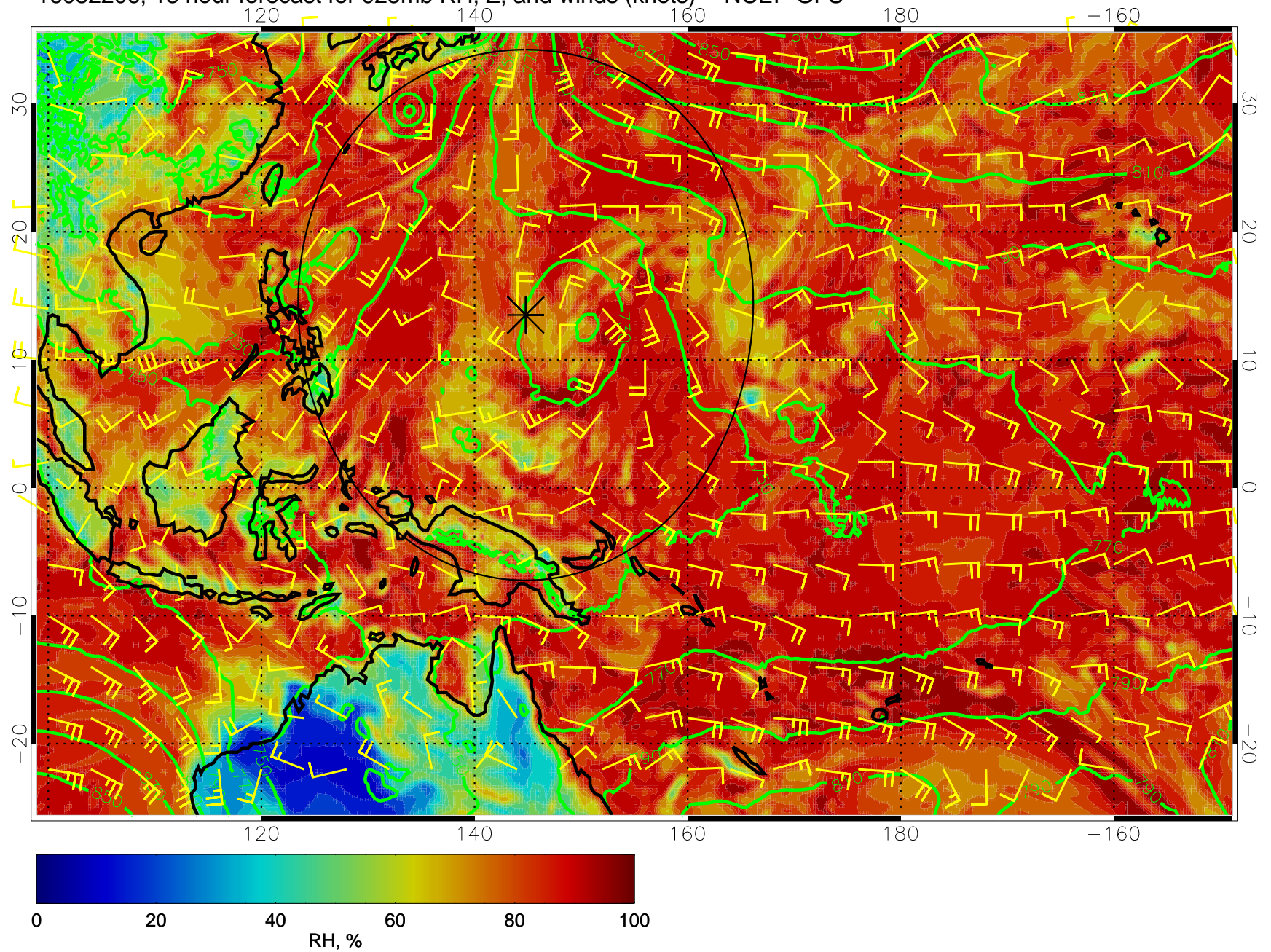
16082206, 18 hour forecast for 925mb RH, Z, and winds (knots) -- NCEP GFS
