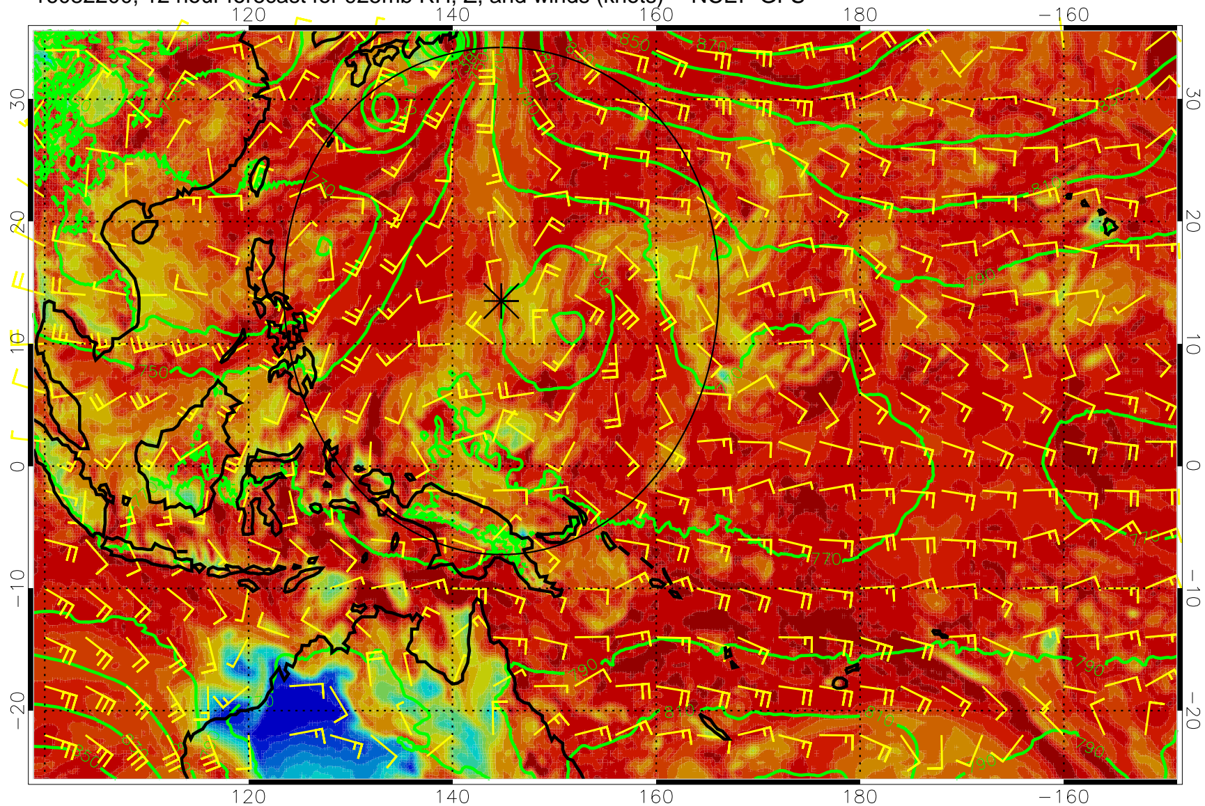
16082200, 12 hour forecast for 925mb RH, Z, and winds (knots) -- NCEP GFS
