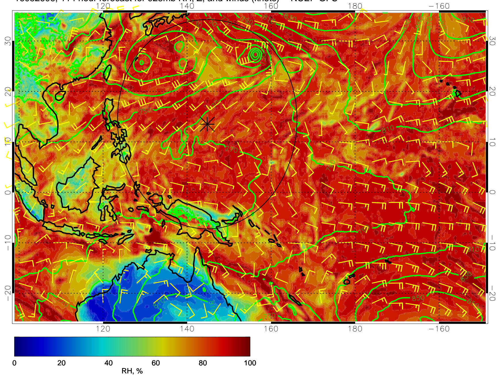
16082606, 114 hour forecast for 925mb RH, Z, and winds (knots) -- NCEP GFS
