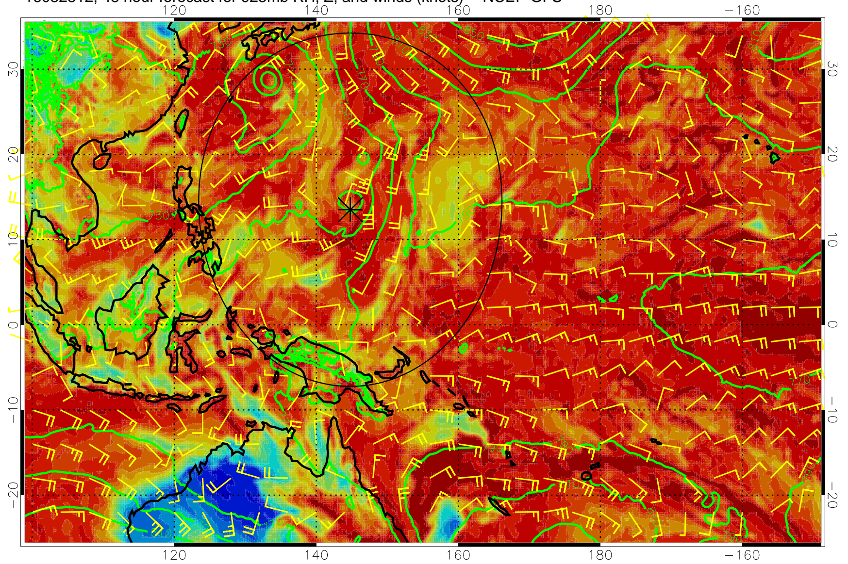
16082312, 48 hour forecast for 925mb RH, Z, and winds (knots) -- NCEP GFS
