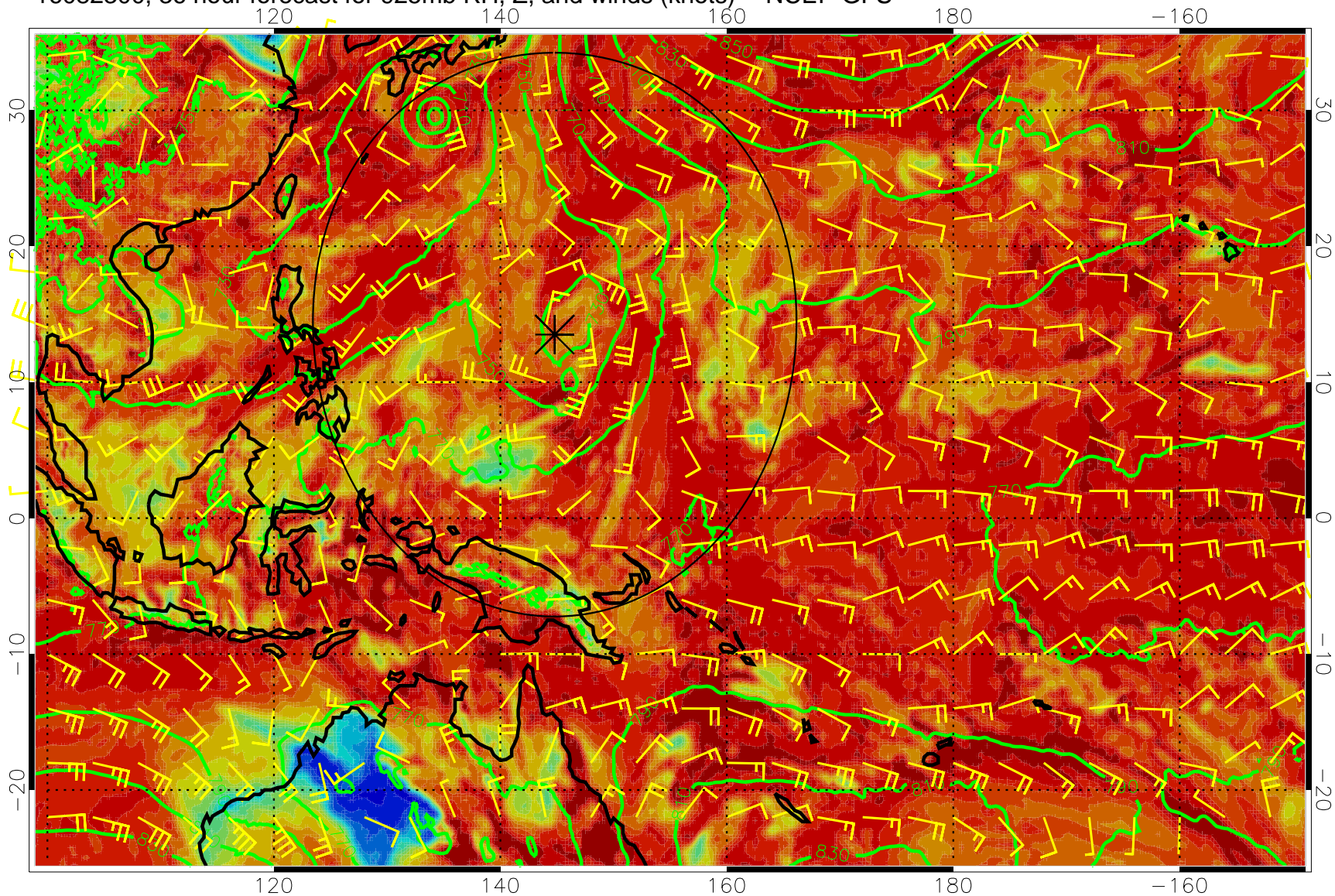
16082300, 36 hour forecast for 925mb RH, Z, and winds (knots) -- NCEP GFS
