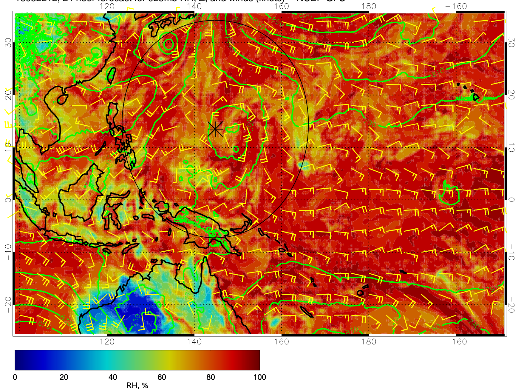
16082212, 24 hour forecast for 925mb RH, Z, and winds (knots) -- NCEP GFS
