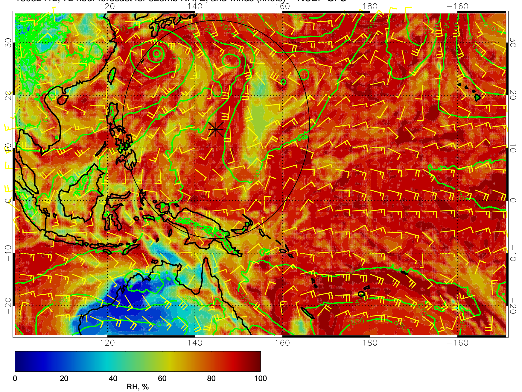
16082412, 72 hour forecast for 925mb RH, Z, and winds (knots) -- NCEP GFS
