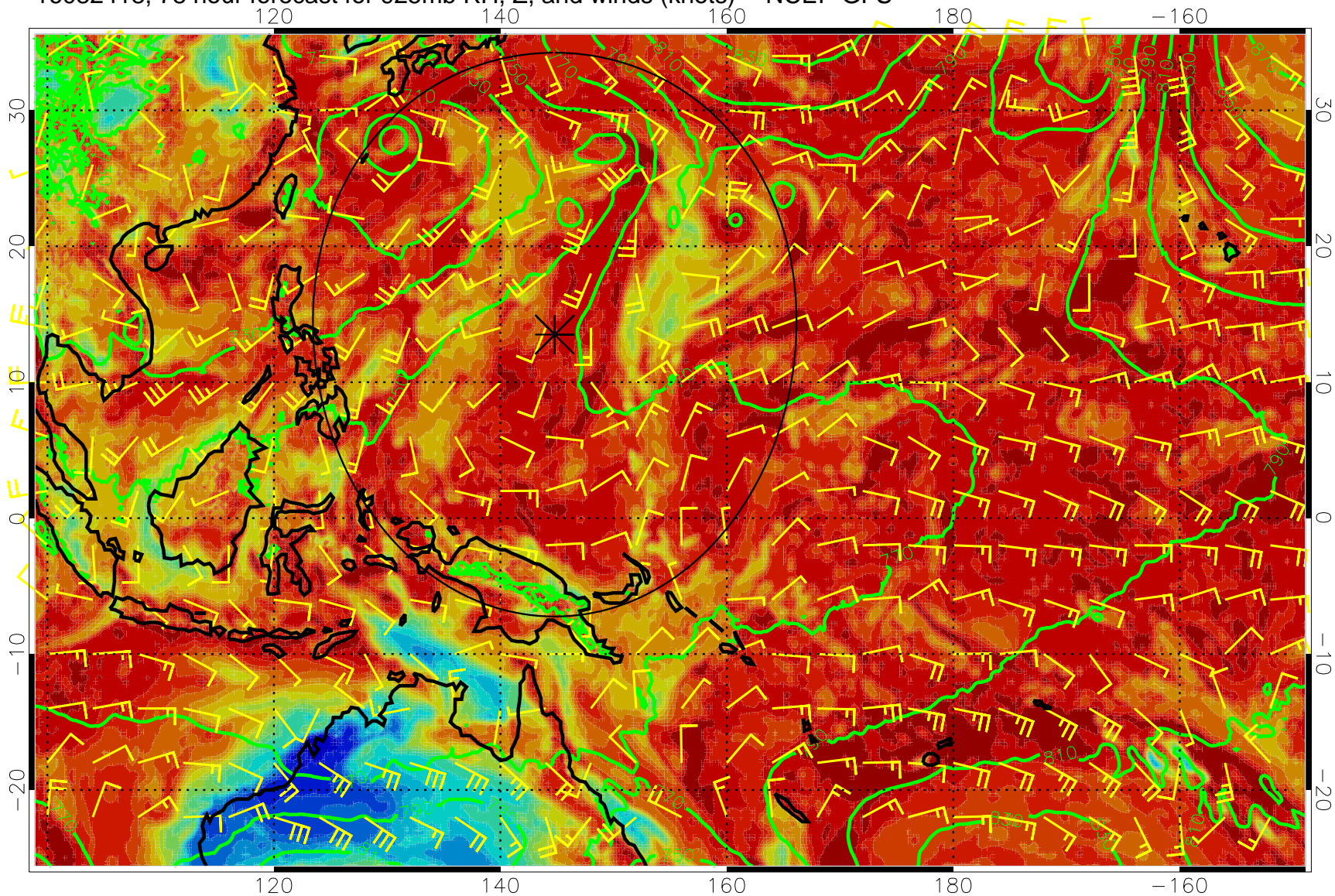
16082418, 78 hour forecast for 925mb RH, Z, and winds (knots) -- NCEP GFS
