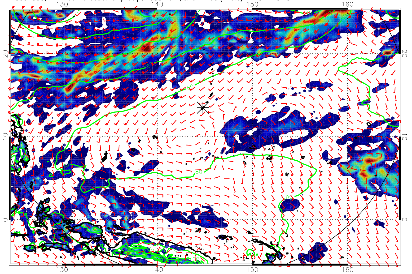
16082606, 114 hour forecast for precip, 1000mb Z, and winds (knots) -- NCEP GFS
