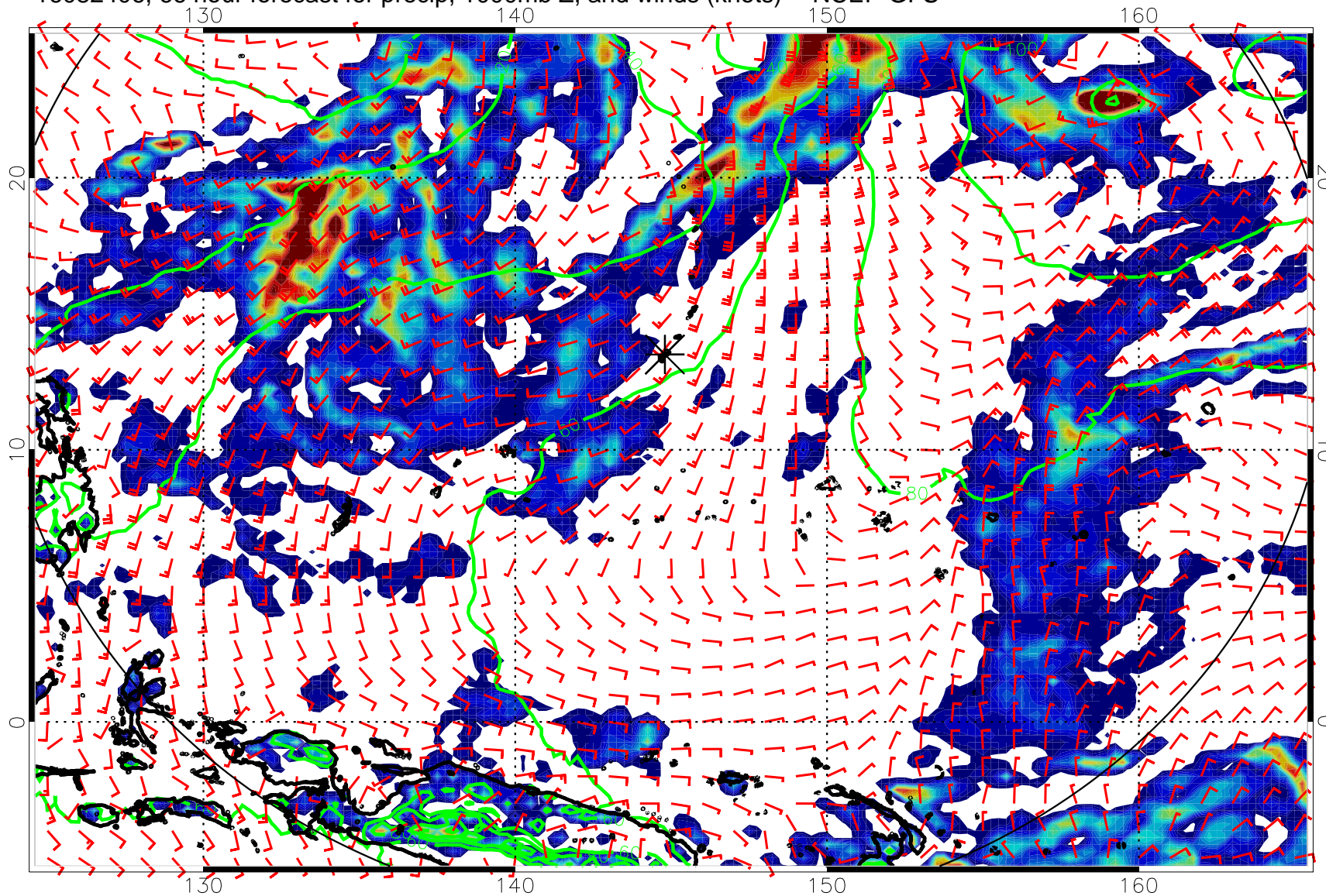
16082406, 66 hour forecast for precip, 1000mb Z, and winds (knots) -- NCEP GFS
