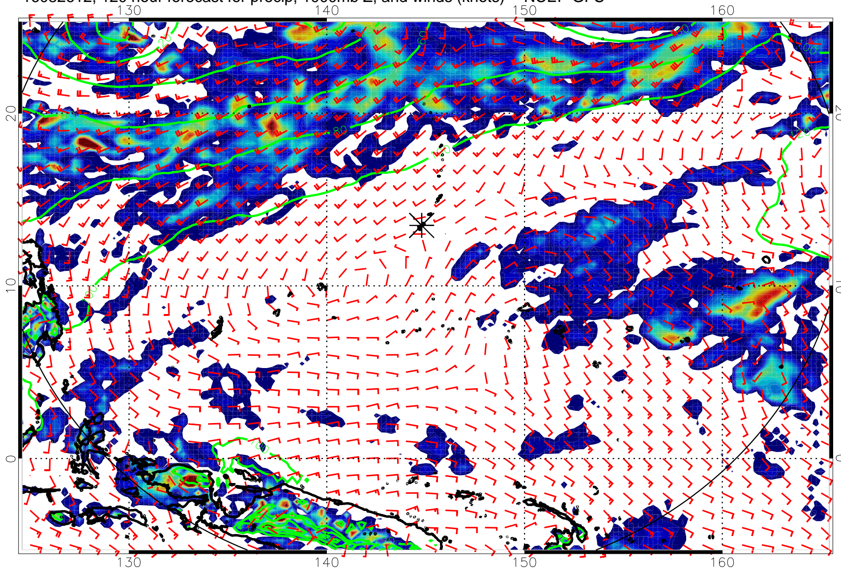
16082612, 120 hour forecast for precip, 1000mb Z, and winds (knots) -- NCEP GFS
