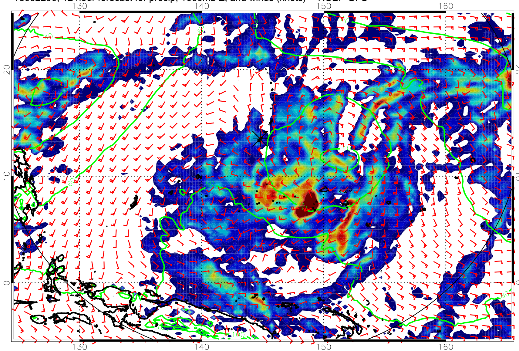
16082200, 12 hour forecast for precip, 1000mb Z, and winds (knots) -- NCEP GFS
