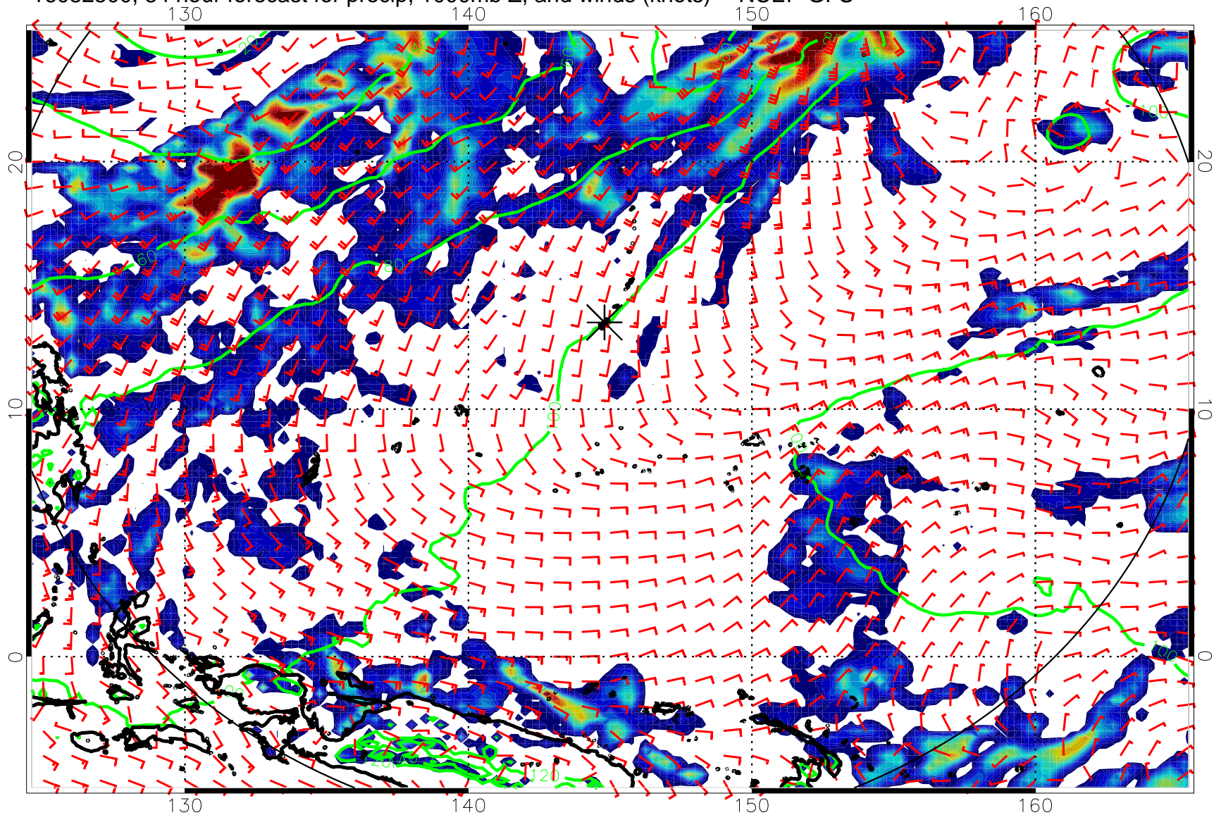
16082500, 84 hour forecast for precip, 1000mb Z, and winds (knots) -- NCEP GFS
