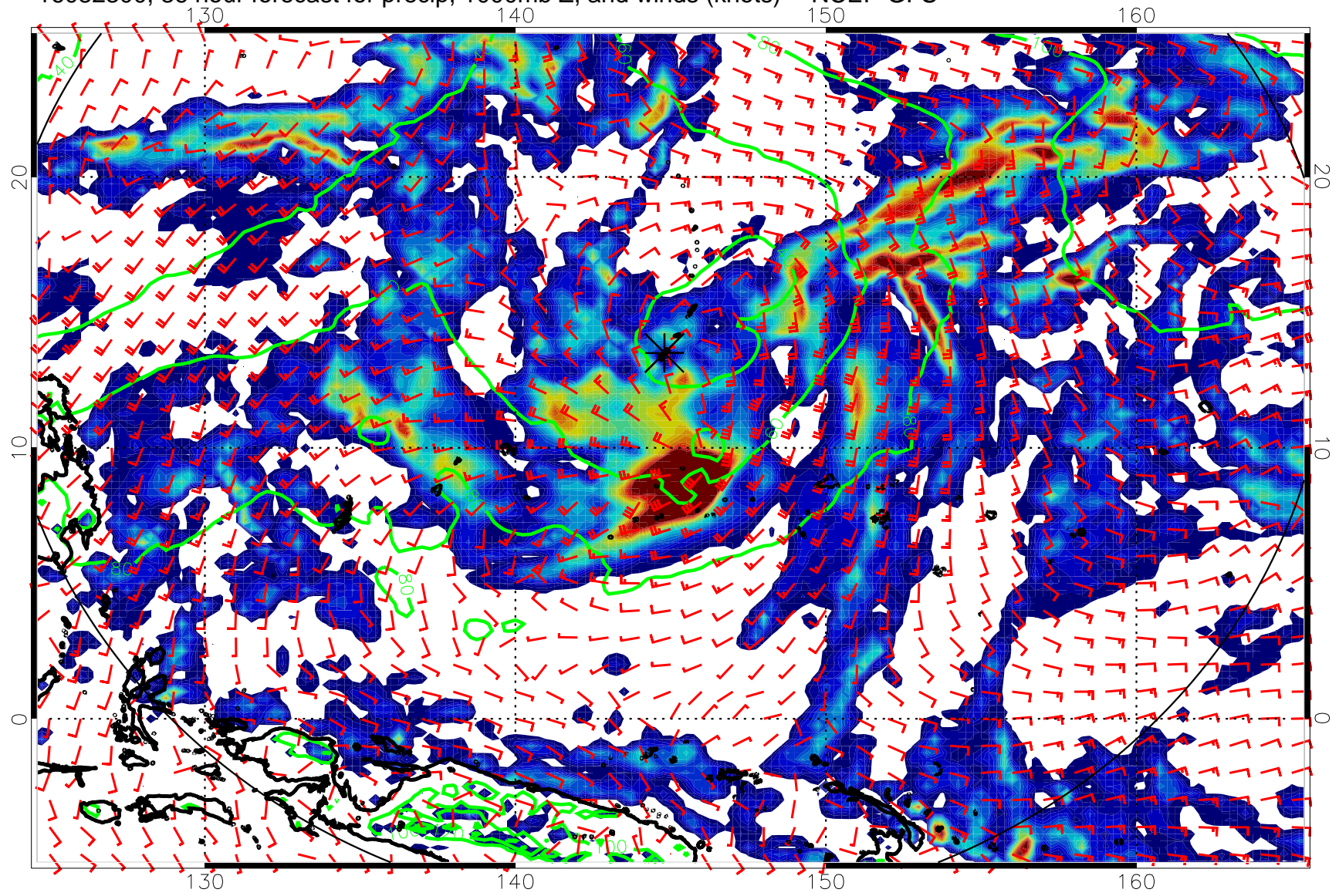
16082300, 36 hour forecast for precip, 1000mb Z, and winds (knots) -- NCEP GFS
