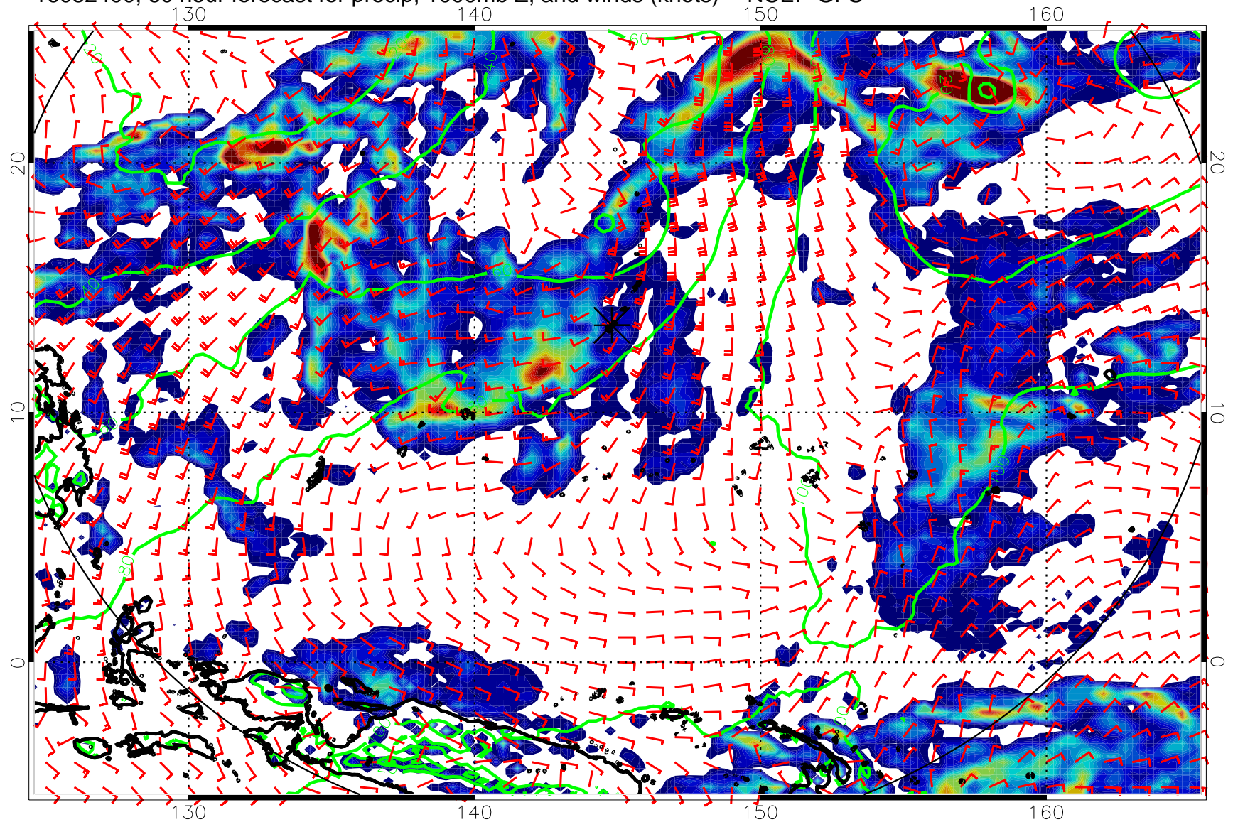
16082400, 60 hour forecast for precip, 1000mb Z, and winds (knots) -- NCEP GFS
