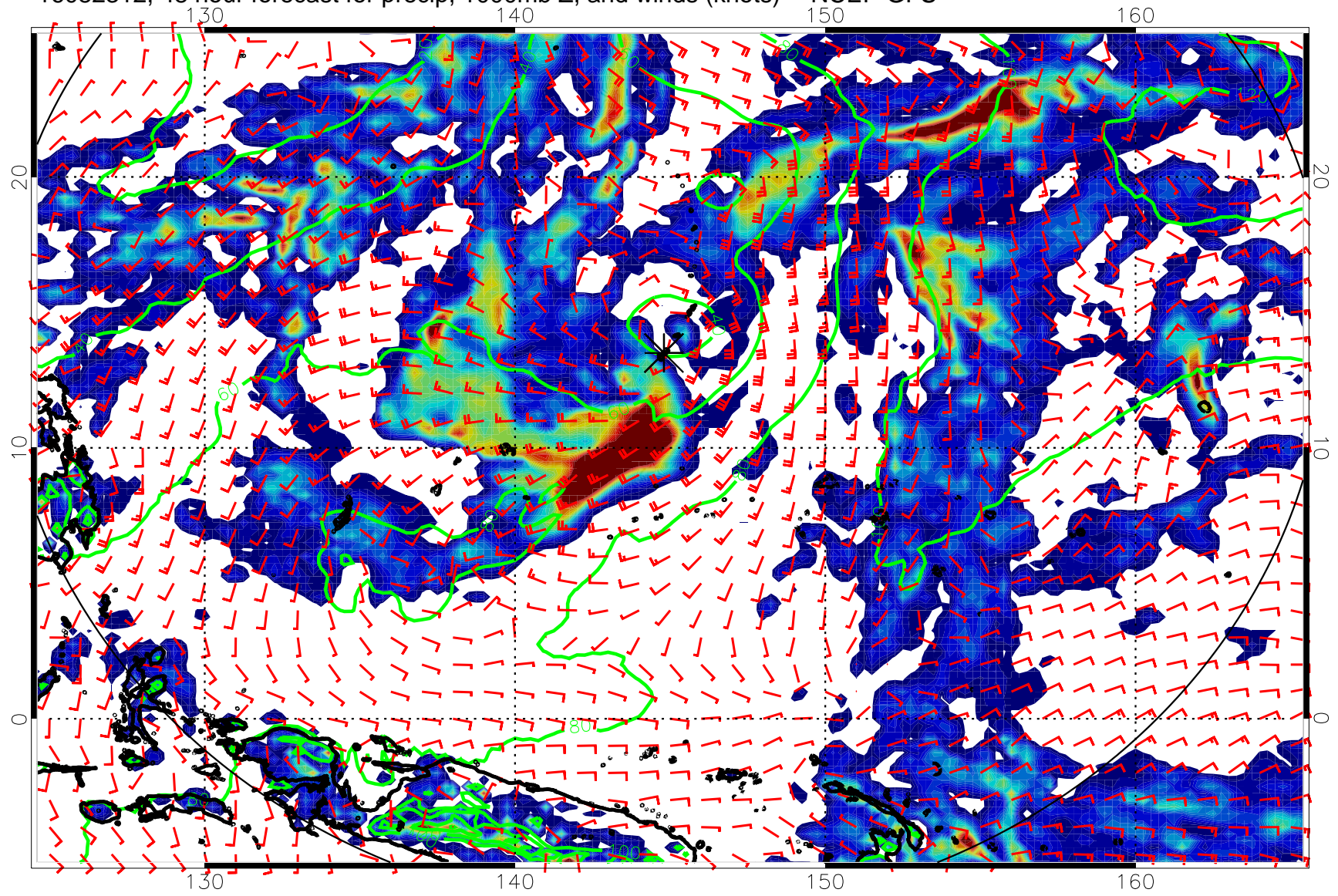
16082312, 48 hour forecast for precip, 1000mb Z, and winds (knots) -- NCEP GFS
