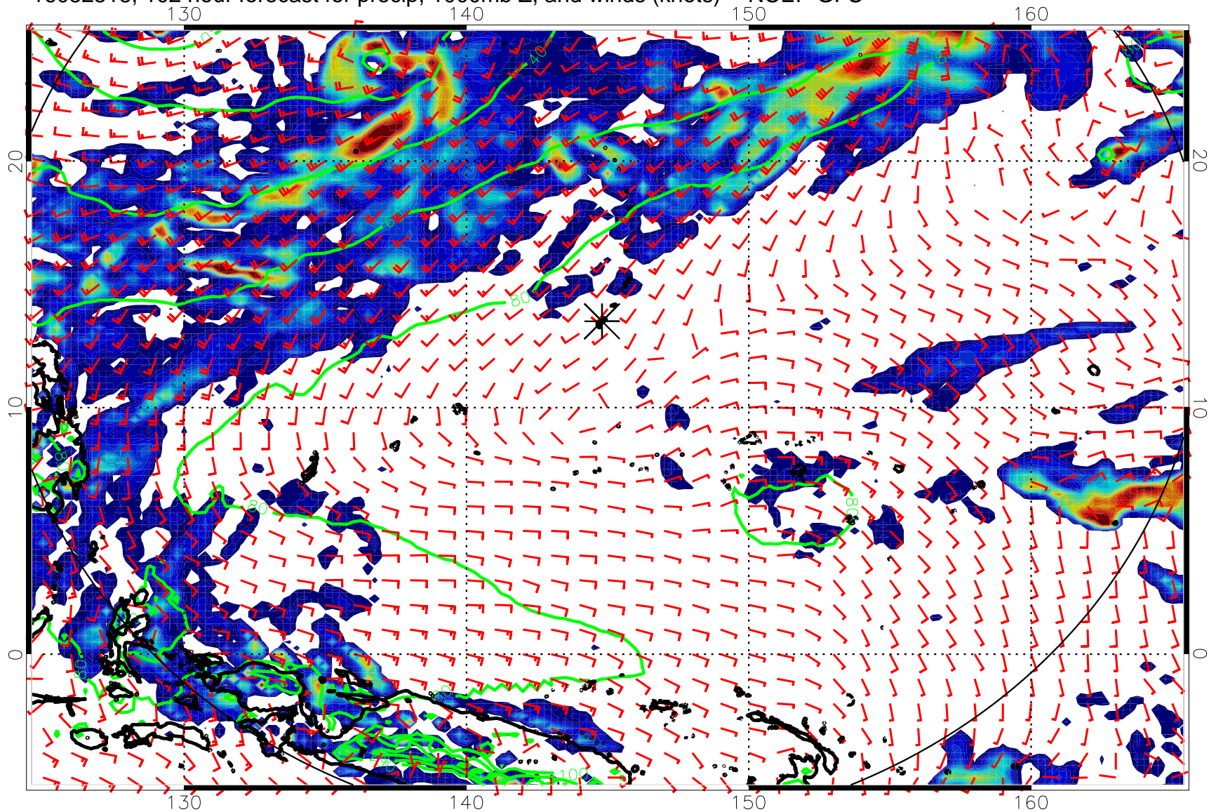
16082518, 102 hour forecast for precip, 1000mb Z, and winds (knots) -- NCEP GFS
