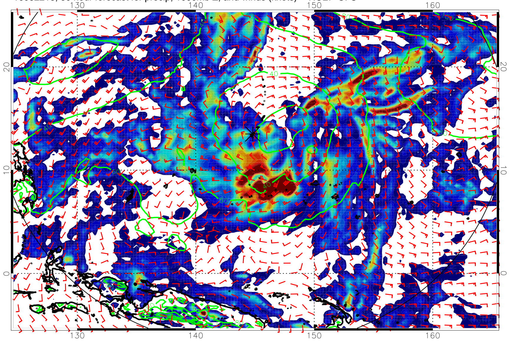
16082218, 30 hour forecast for precip, 1000mb Z, and winds (knots) -- NCEP GFS
