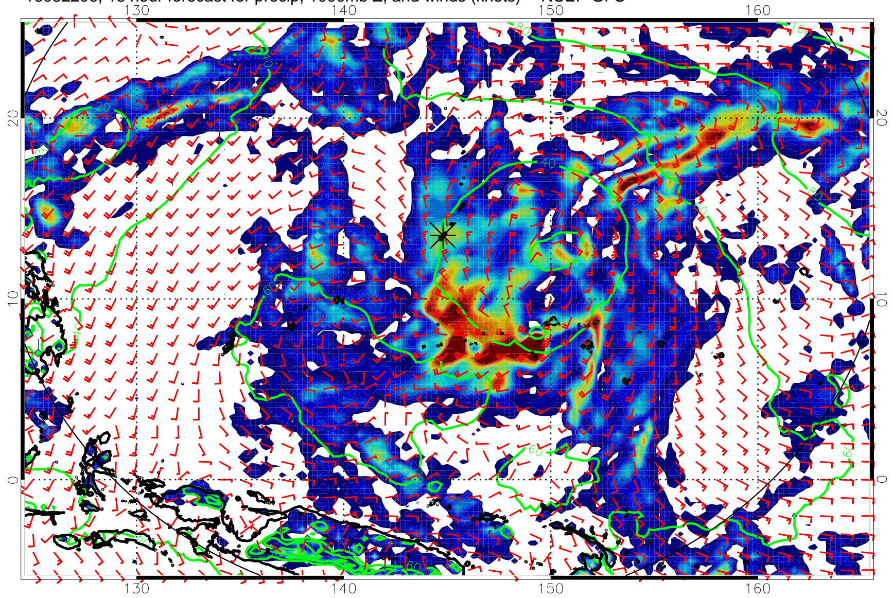
16082206, 18 hour forecast for precip, 1000mb Z, and winds (knots) -- NCEP GFS
