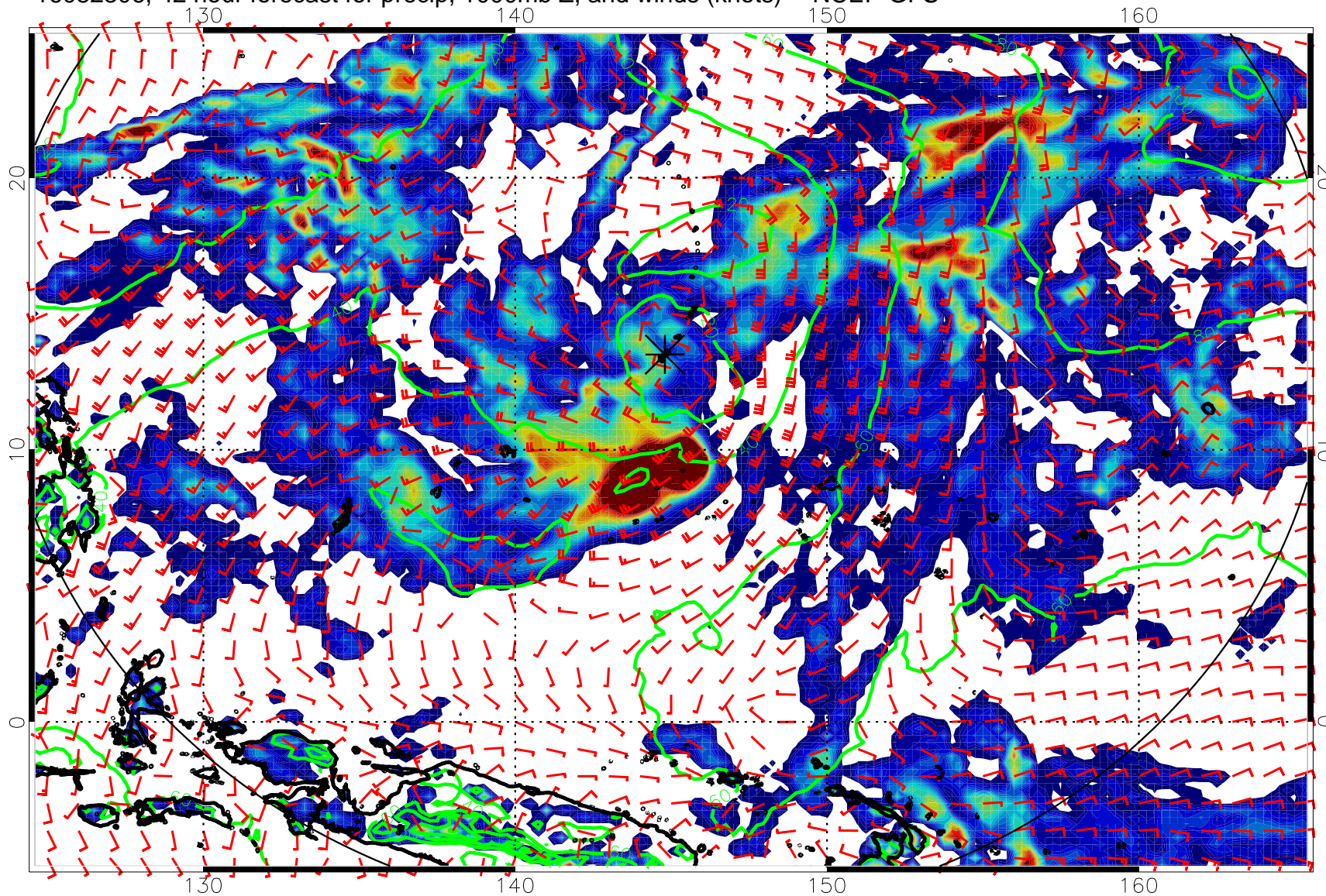
16082306, 42 hour forecast for precip, 1000mb Z, and winds (knots) -- NCEP GFS
