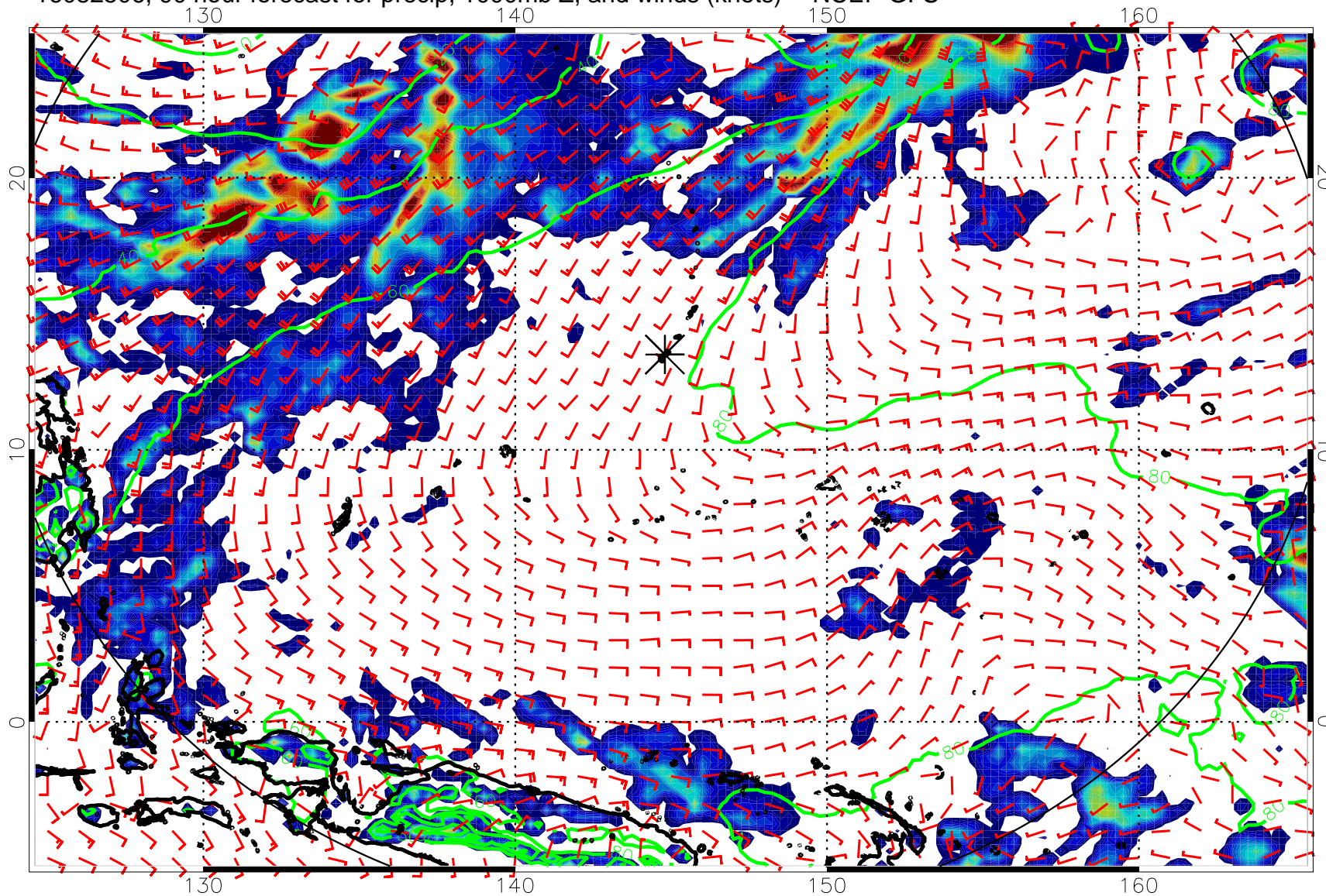
16082506, 90 hour forecast for precip, 1000mb Z, and winds (knots) -- NCEP GFS
