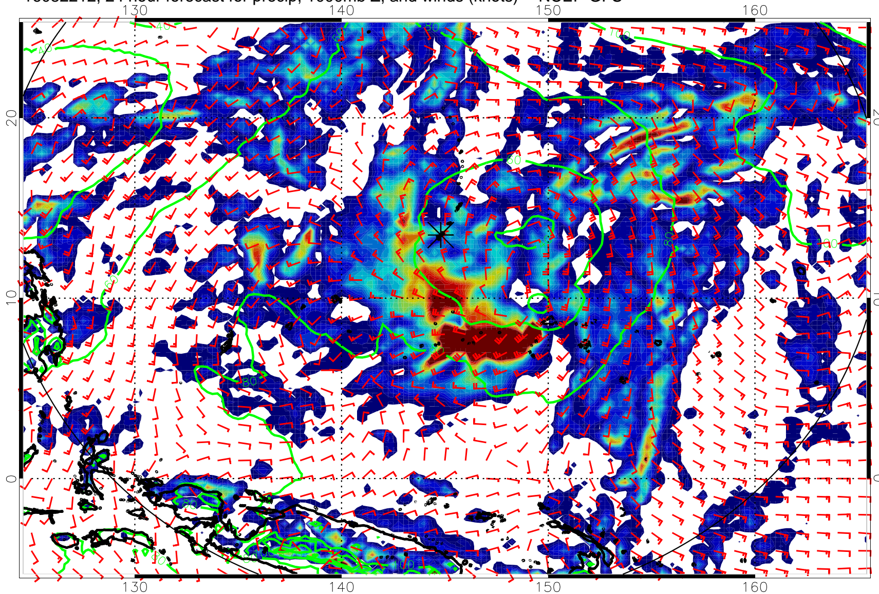
16082212, 24 hour forecast for precip, 1000mb Z, and winds (knots) -- NCEP GFS
