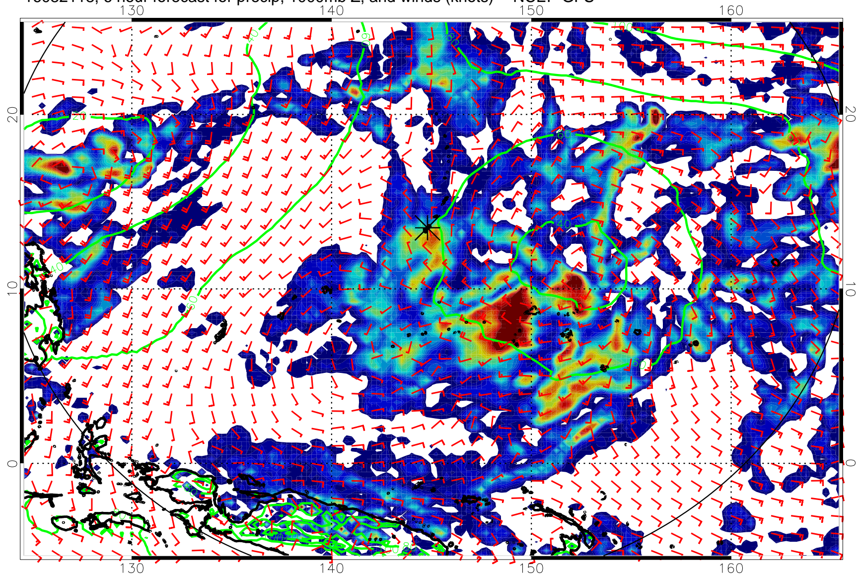
16082118, 6 hour forecast for precip, 1000mb Z, and winds (knots) -- NCEP GFS
