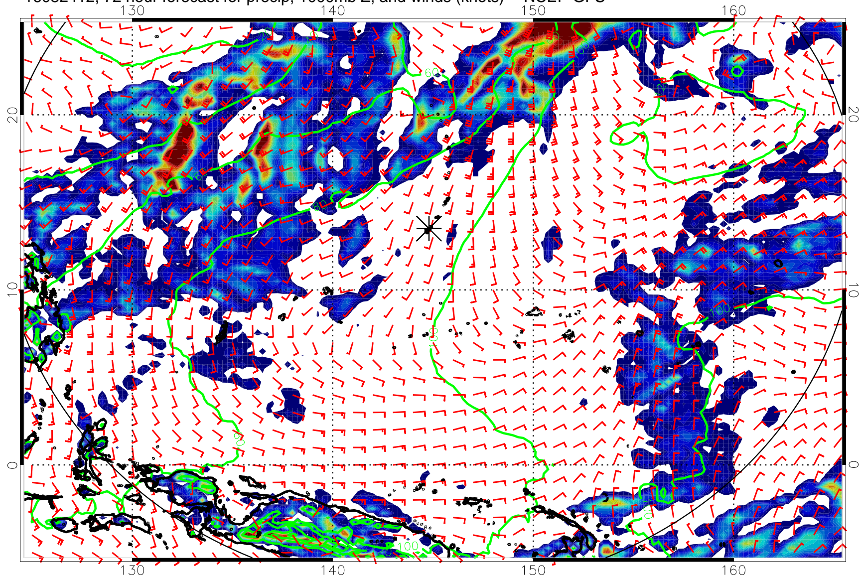
16082412, 72 hour forecast for precip, 1000mb Z, and winds (knots) -- NCEP GFS
