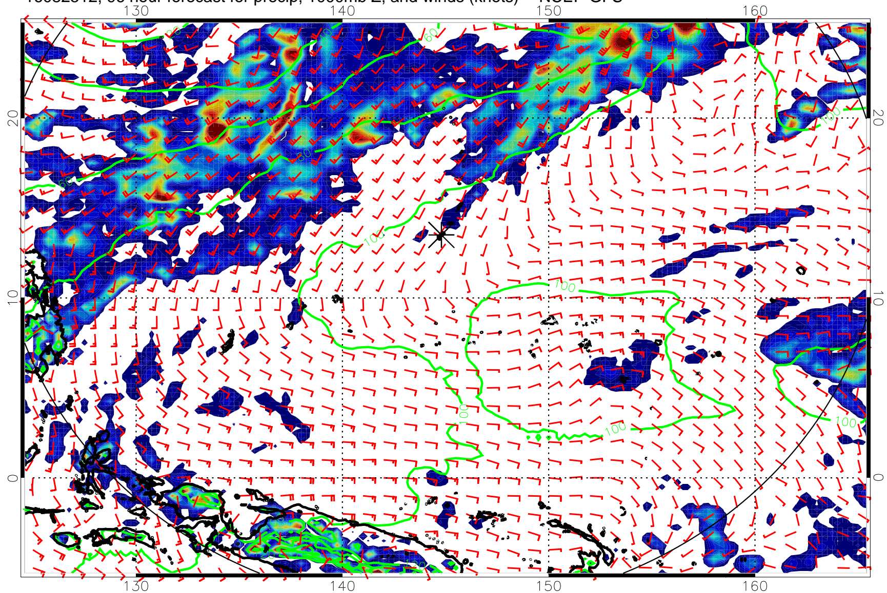
16082512, 96 hour forecast for precip, 1000mb Z, and winds (knots) -- NCEP GFS
