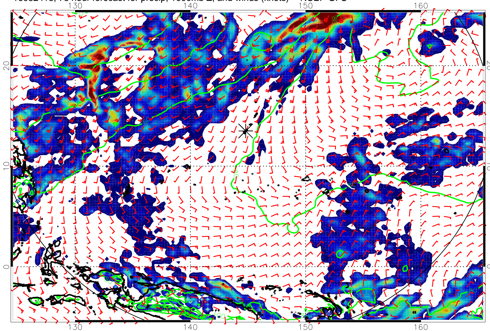
16082418, 78 hour forecast for precip, 1000mb Z, and winds (knots) -- NCEP GFS
