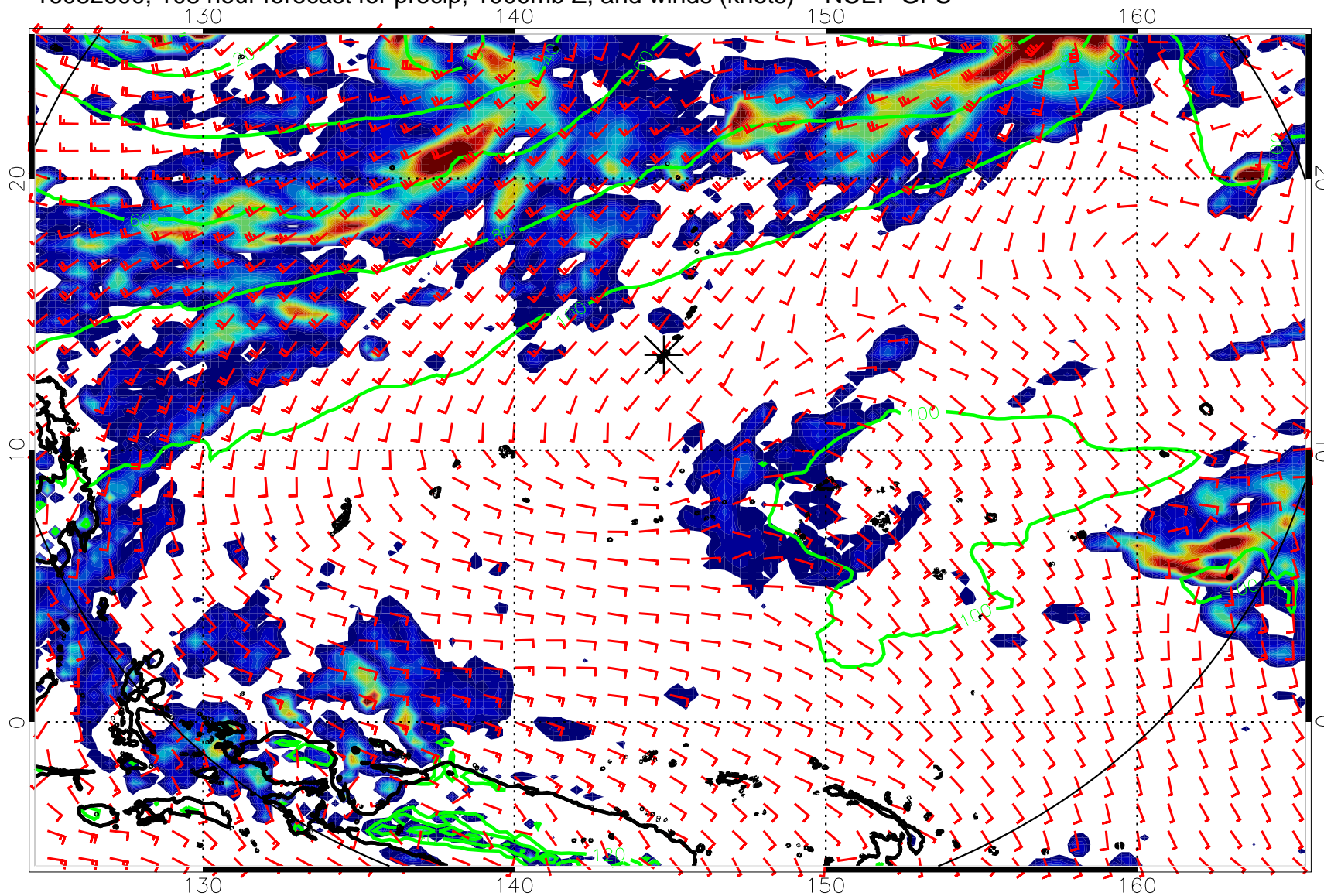
16082600, 108 hour forecast for precip, 1000mb Z, and winds (knots) -- NCEP GFS
