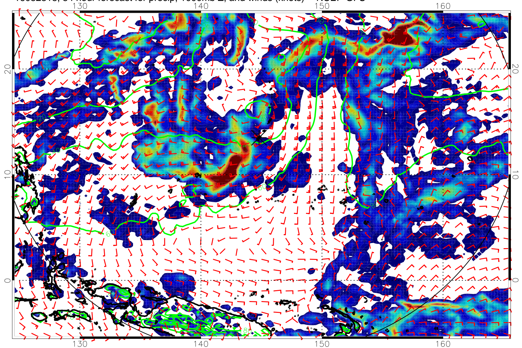
16082318, 54 hour forecast for precip, 1000mb Z, and winds (knots) -- NCEP GFS
