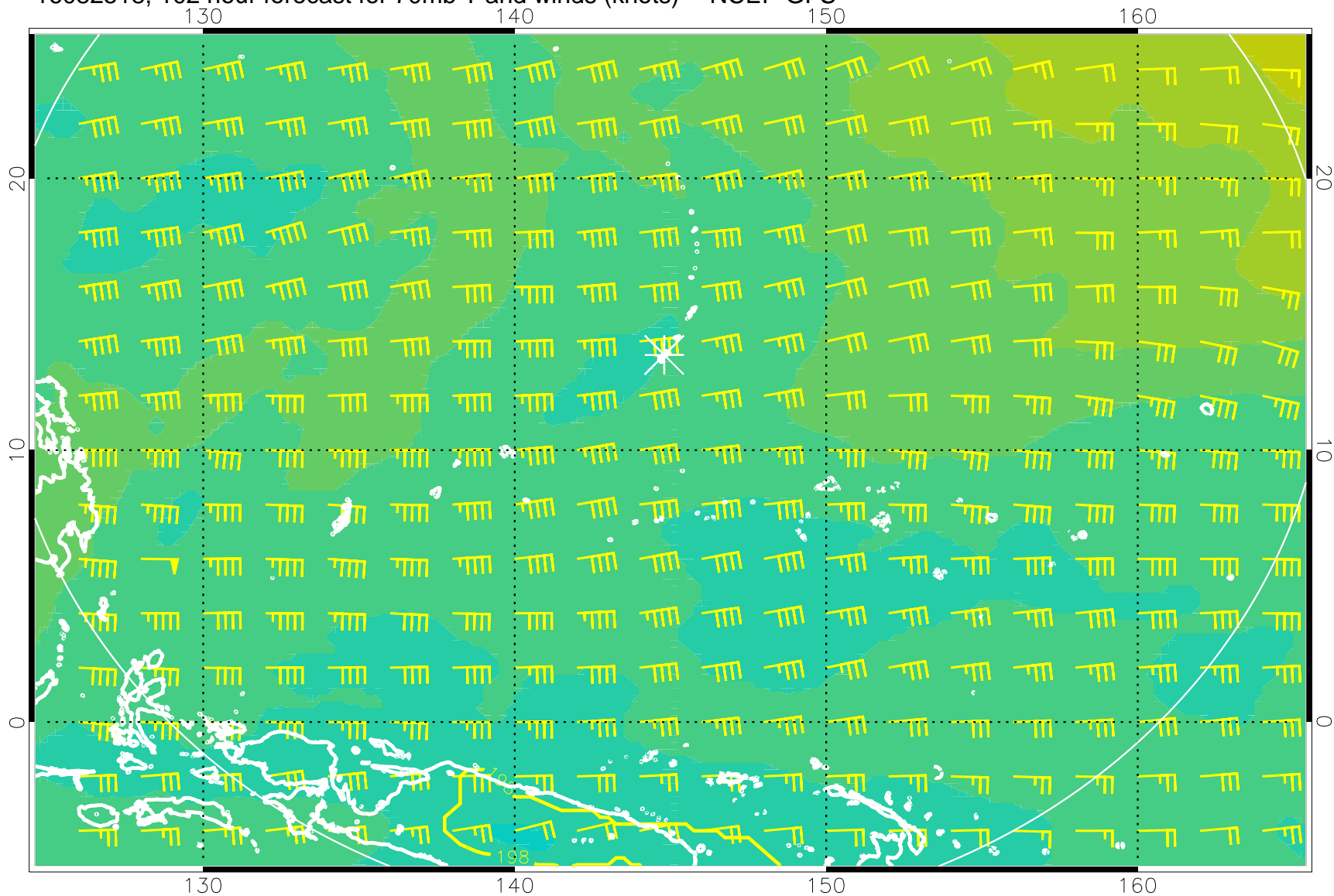
16082518, 102 hour forecast for 70mb T and winds (knots) -- NCEP GFS
