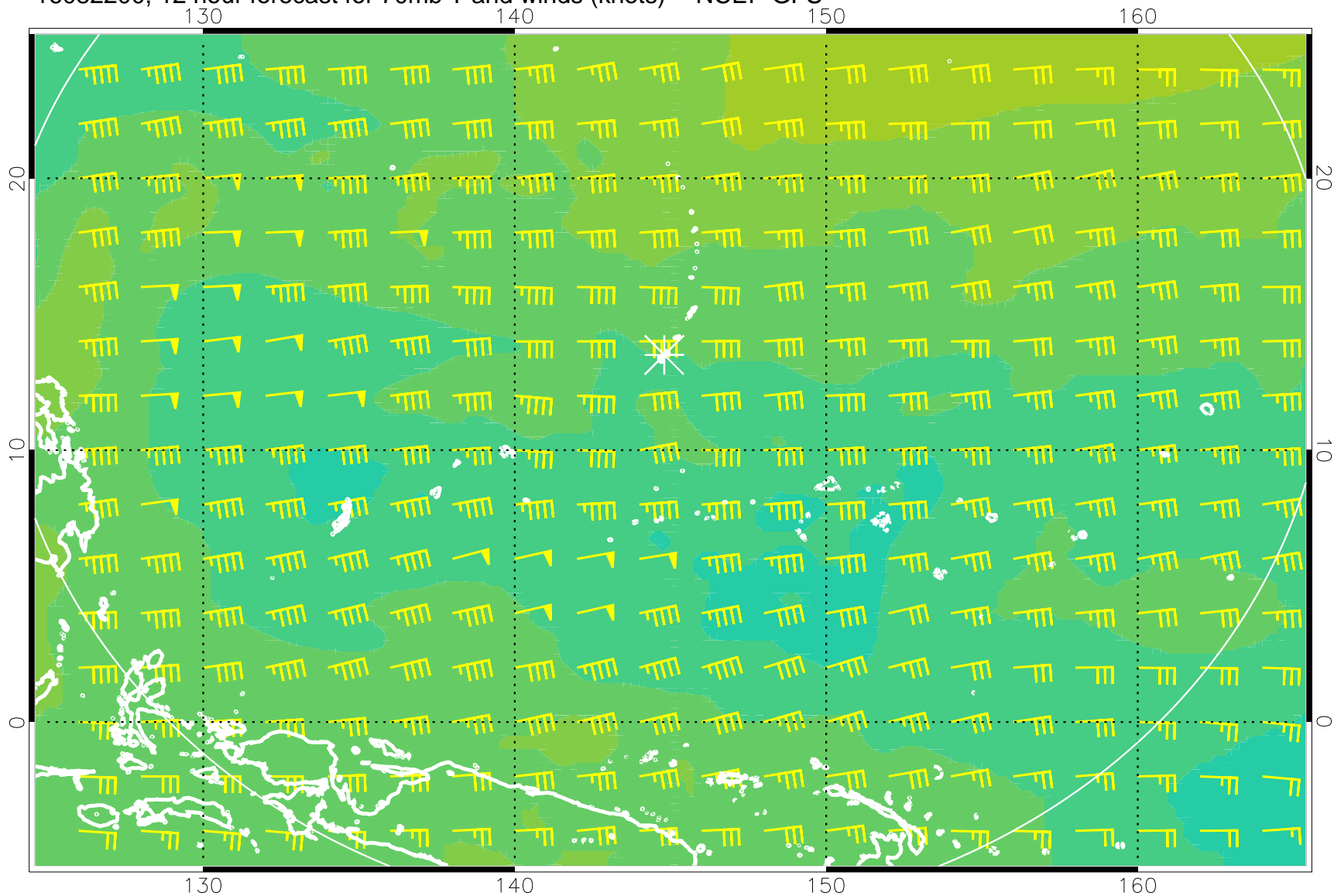
16082200, 12 hour forecast for 70mb T and winds (knots) -- NCEP GFS
