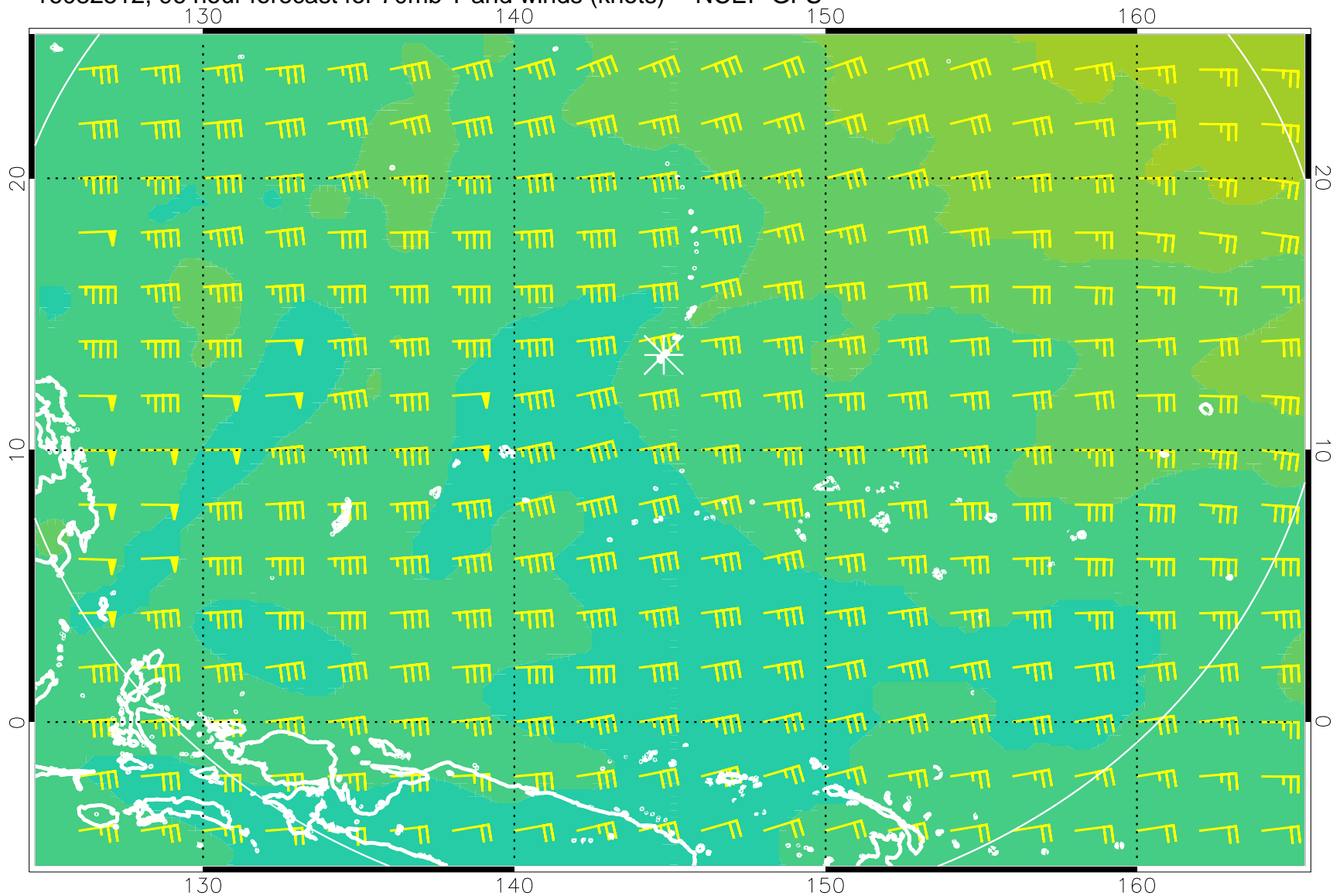
16082512, 96 hour forecast for 70mb T and winds (knots) -- NCEP GFS
