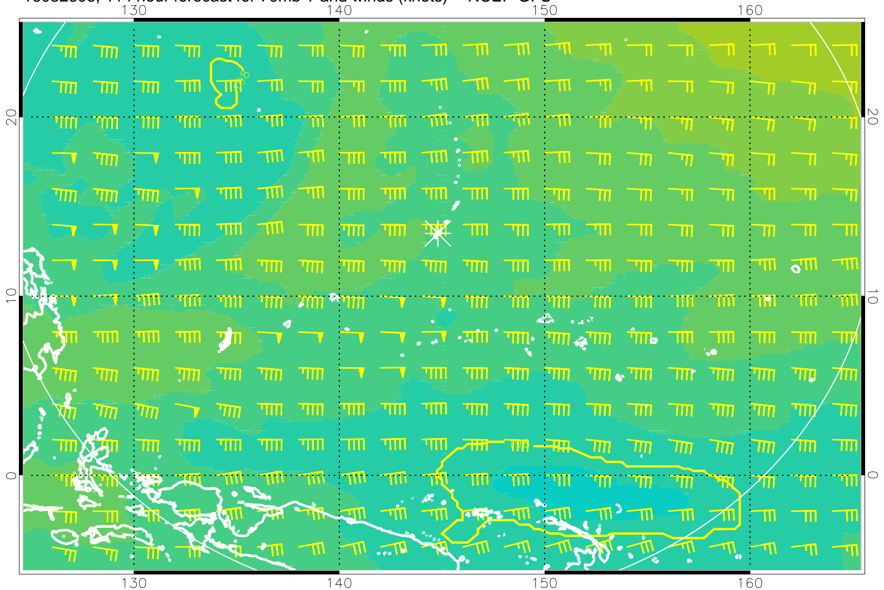
16082606, 114 hour forecast for 70mb T and winds (knots) -- NCEP GFS
