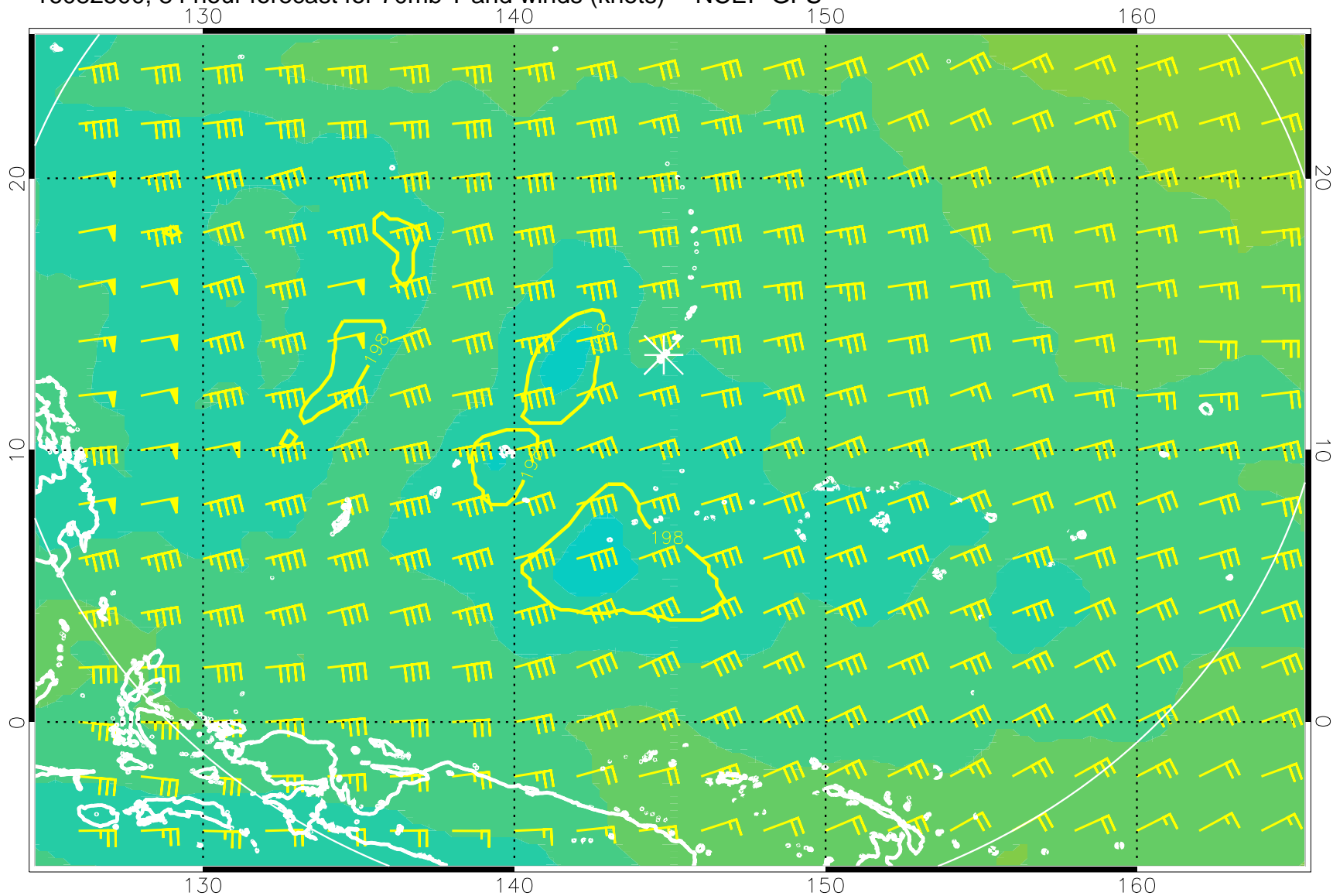
16082500, 84 hour forecast for 70mb T and winds (knots) -- NCEP GFS
