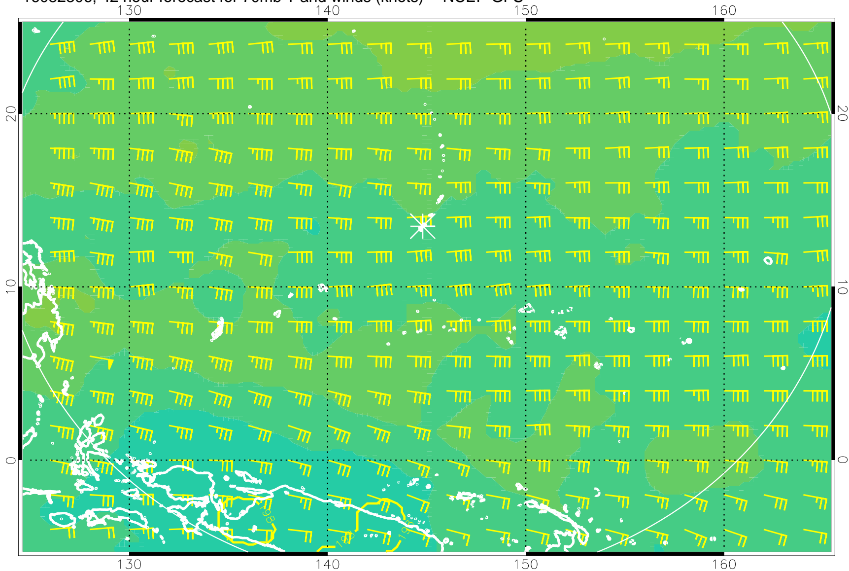
16082306, 42 hour forecast for 70mb T and winds (knots) -- NCEP GFS
