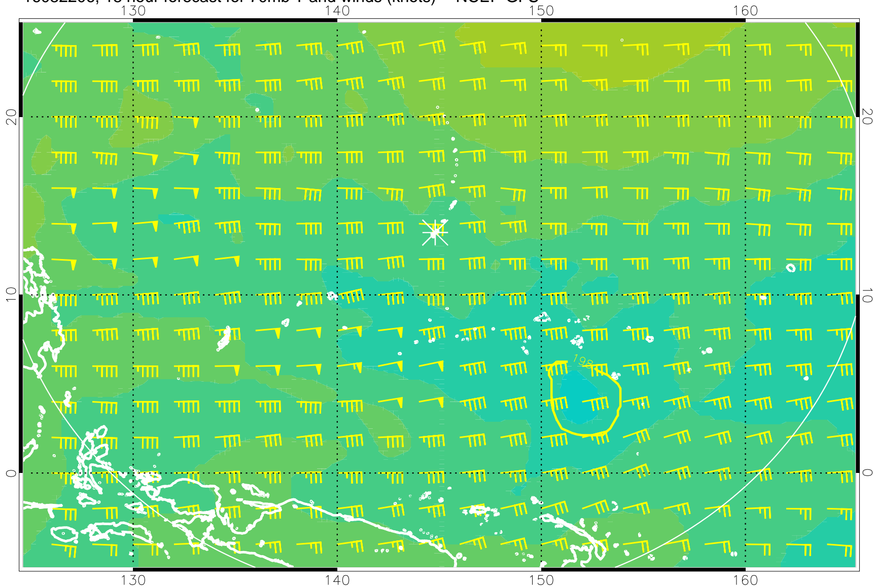
16082206, 18 hour forecast for 70mb T and winds (knots) -- NCEP GFS
