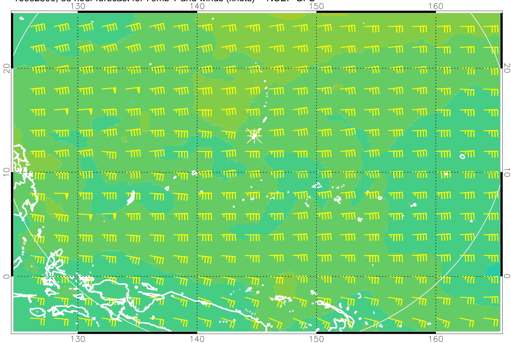
16082300, 36 hour forecast for 70mb T and winds (knots) -- NCEP GFS
