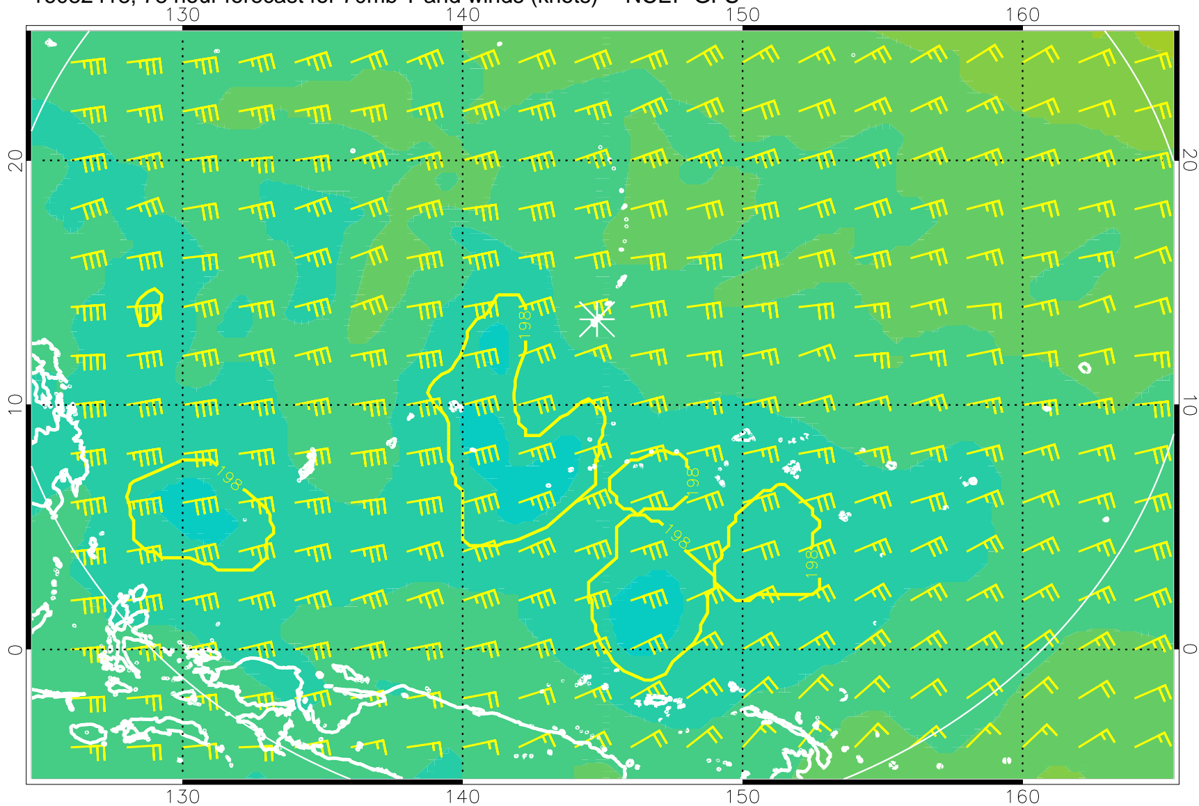
16082418, 78 hour forecast for 70mb T and winds (knots) -- NCEP GFS
