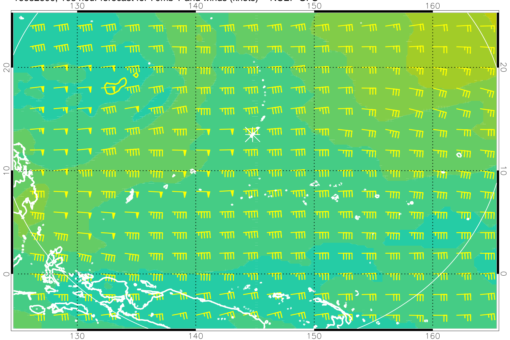
16082600, 108 hour forecast for 70mb T and winds (knots) -- NCEP GFS
