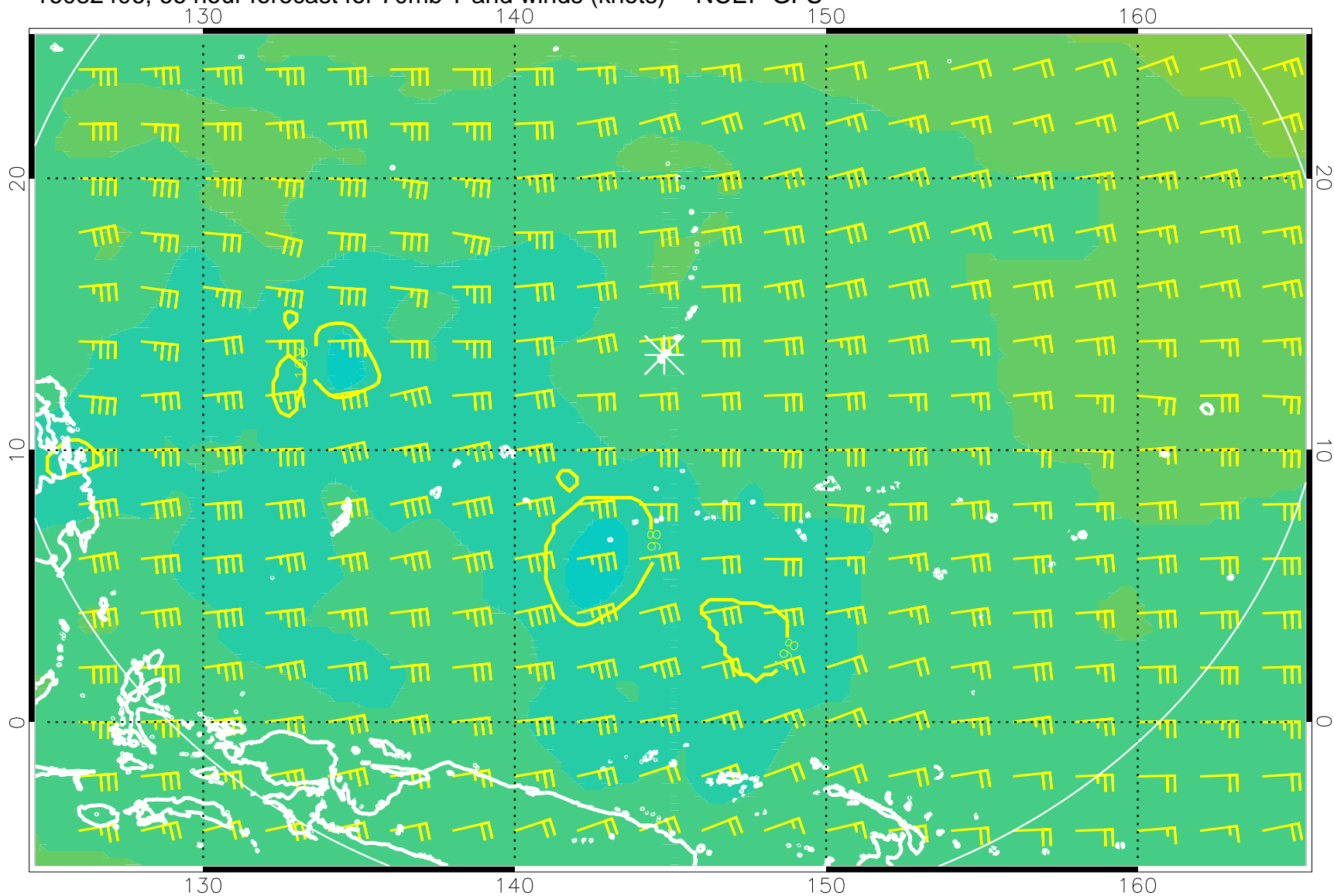
16082406, 66 hour forecast for 70mb T and winds (knots) -- NCEP GFS
