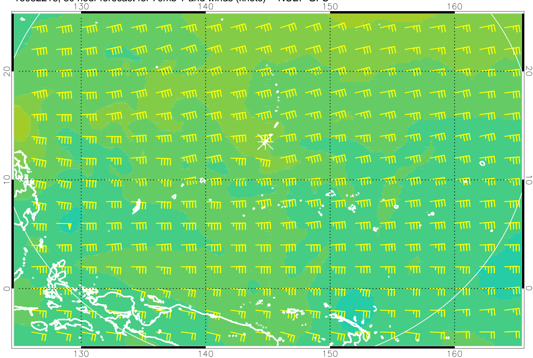
16082218, 30 hour forecast for 70mb T and winds (knots) -- NCEP GFS
