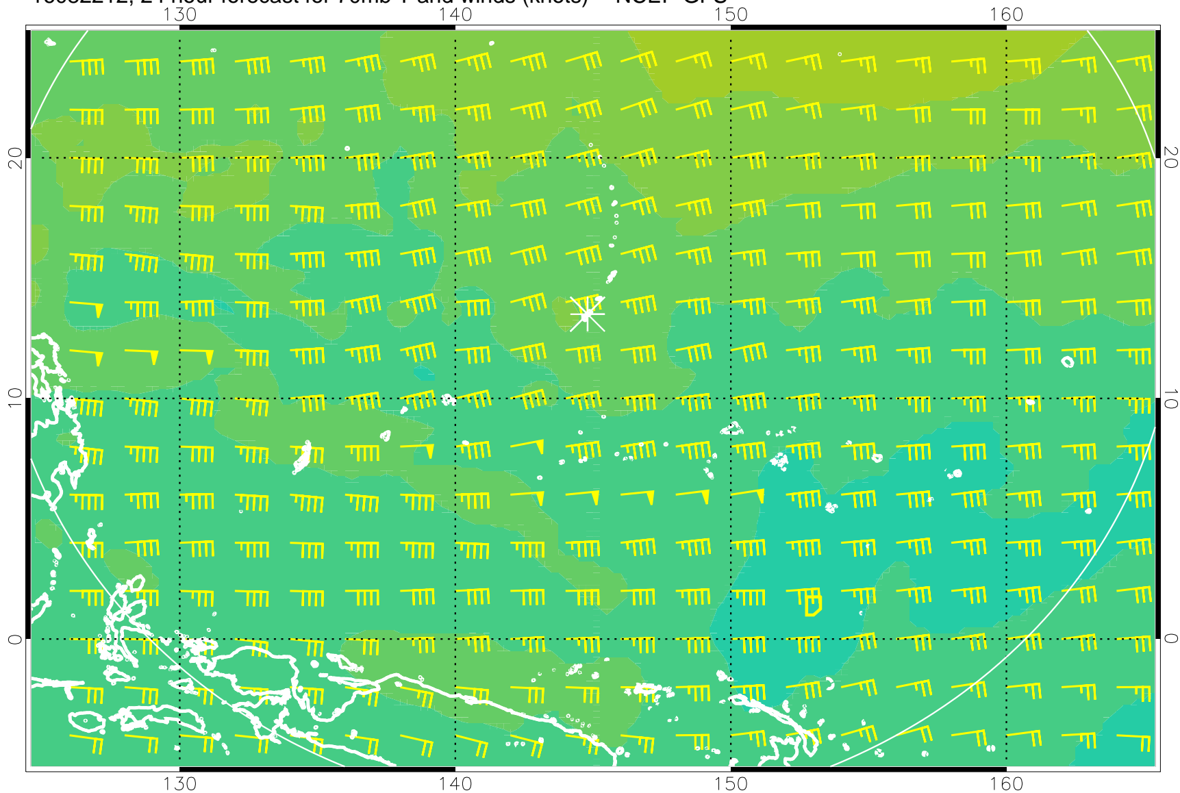
16082212, 24 hour forecast for 70mb T and winds (knots) -- NCEP GFS
