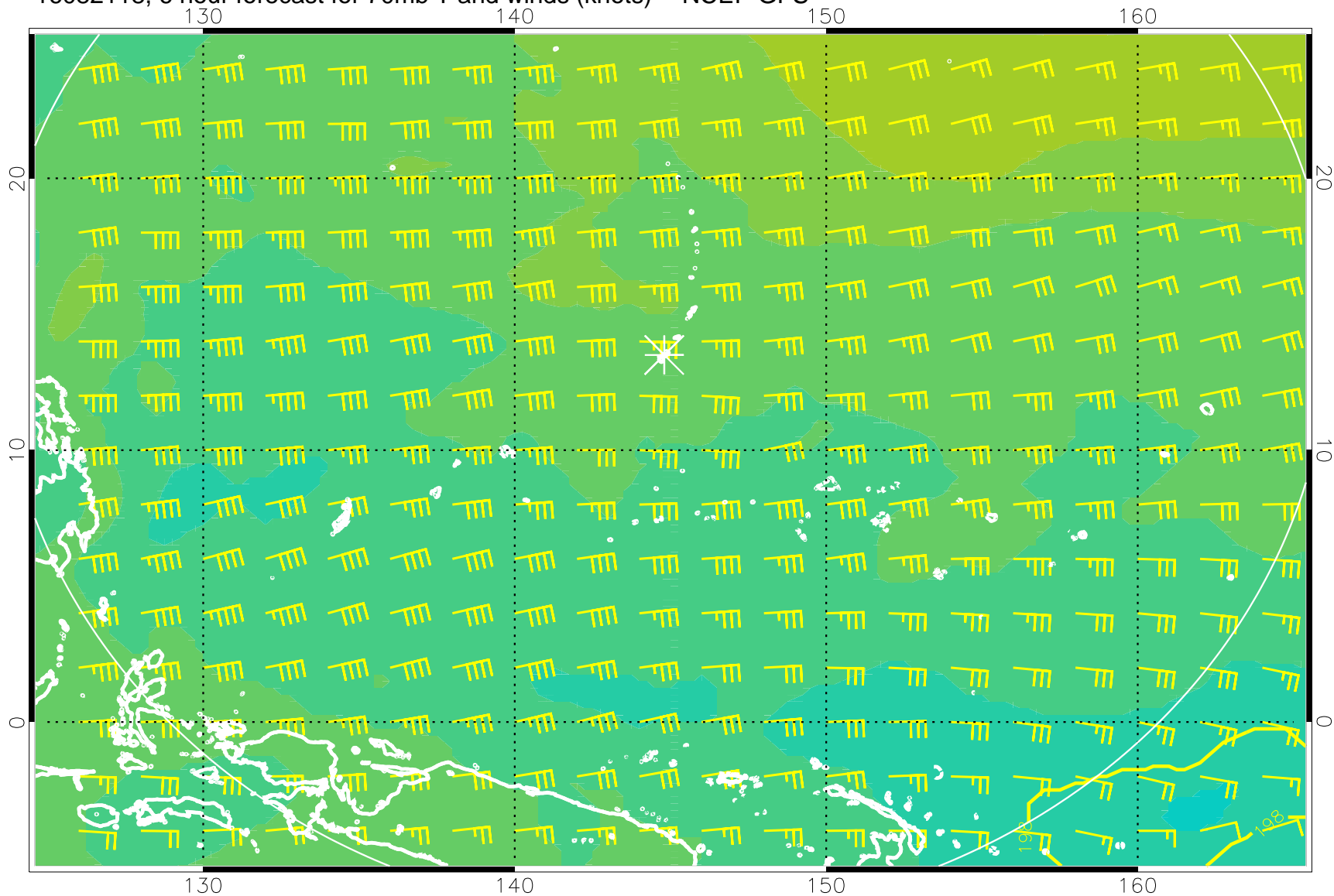
16082118, 6 hour forecast for 70mb T and winds (knots) -- NCEP GFS
