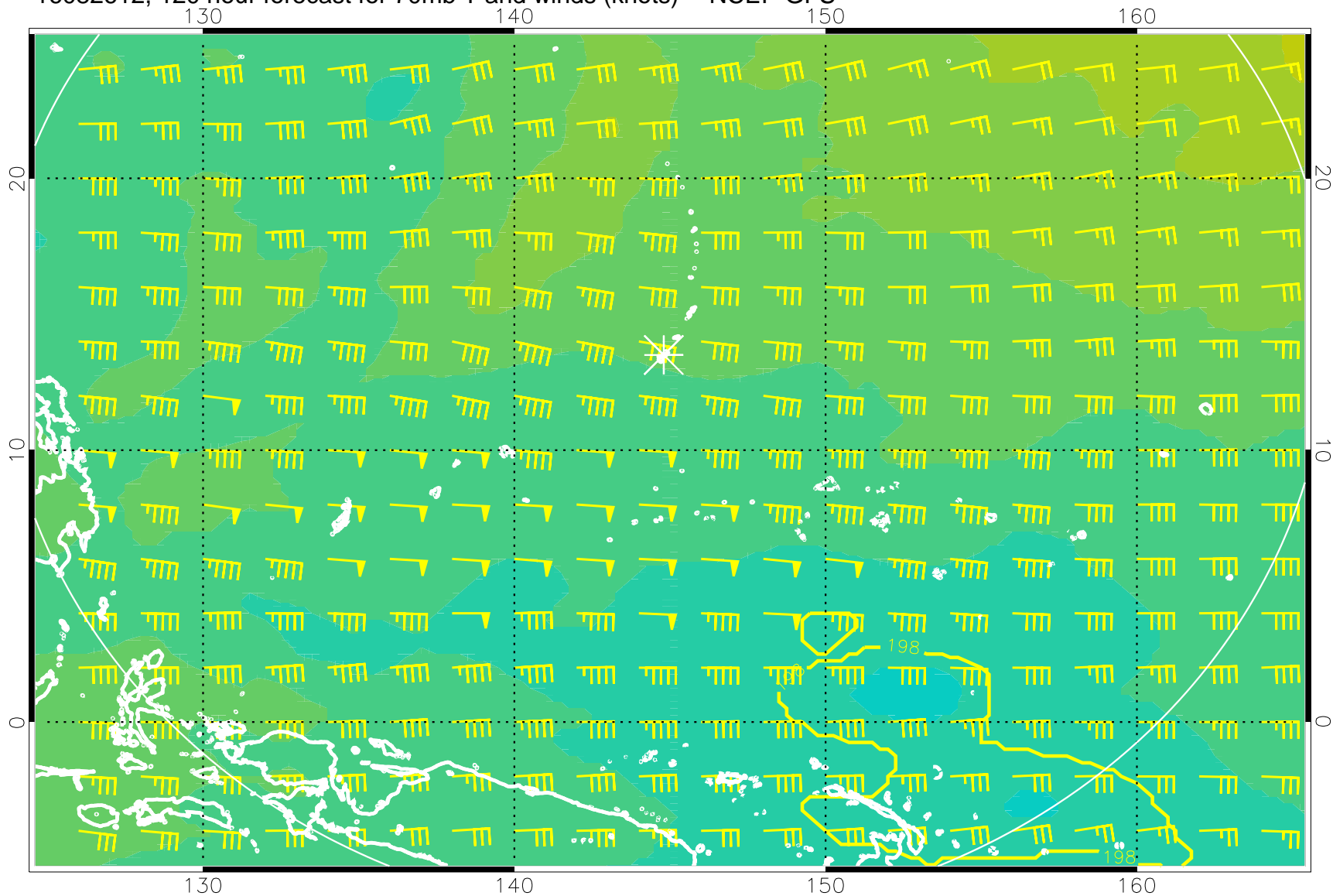
16082612, 120 hour forecast for 70mb T and winds (knots) -- NCEP GFS
