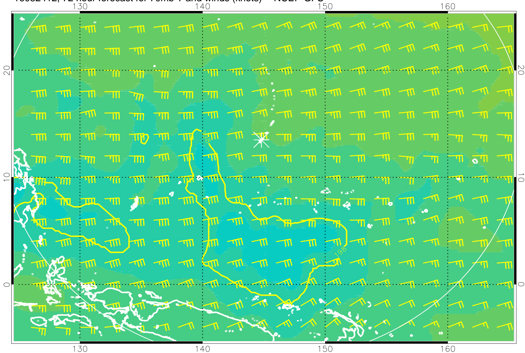
16082412, 72 hour forecast for 70mb T and winds (knots) -- NCEP GFS
