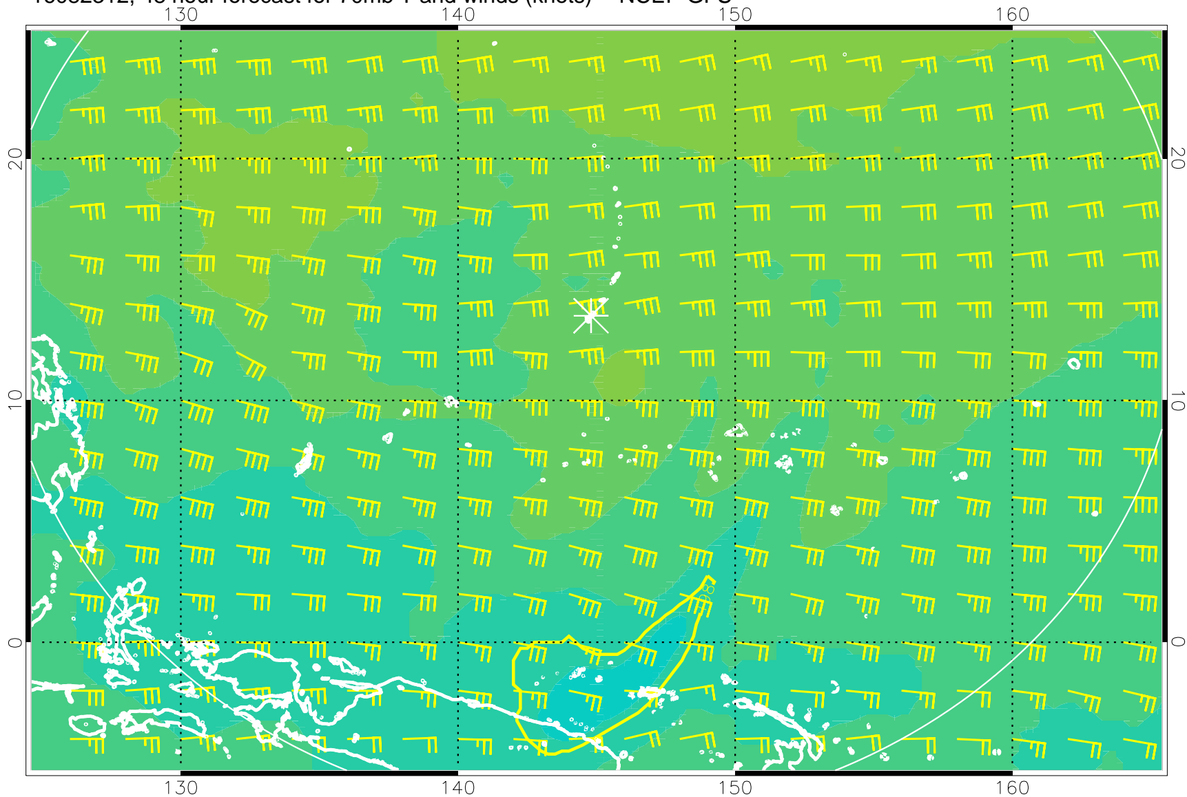
16082312, 48 hour forecast for 70mb T and winds (knots) -- NCEP GFS
