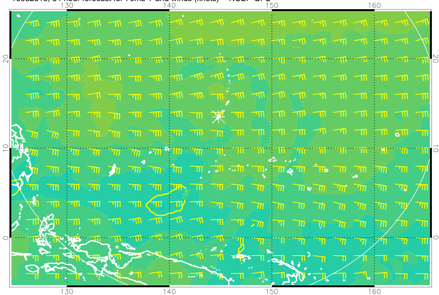
16082318, 54 hour forecast for 70mb T and winds (knots) -- NCEP GFS
