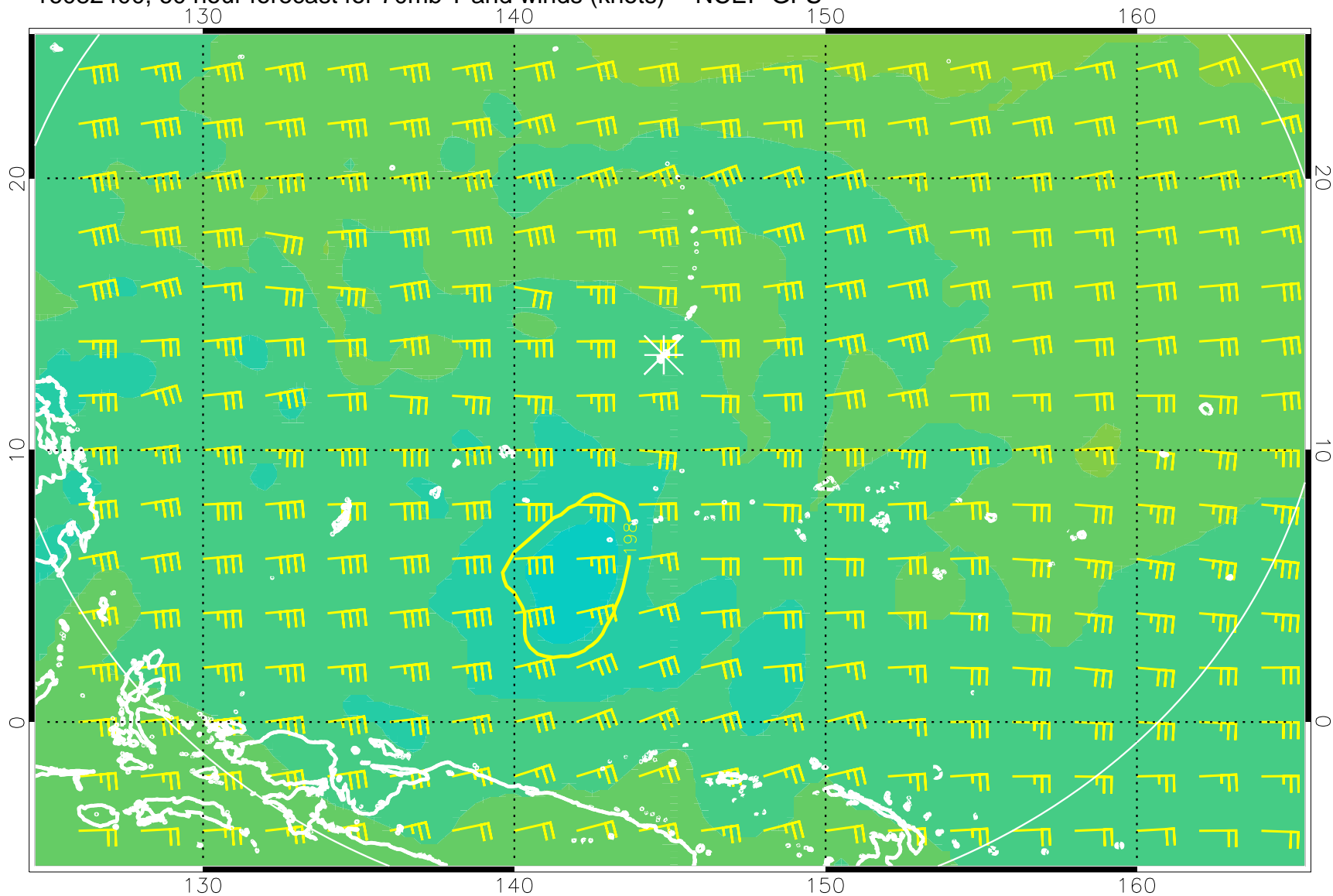
16082400, 60 hour forecast for 70mb T and winds (knots) -- NCEP GFS
