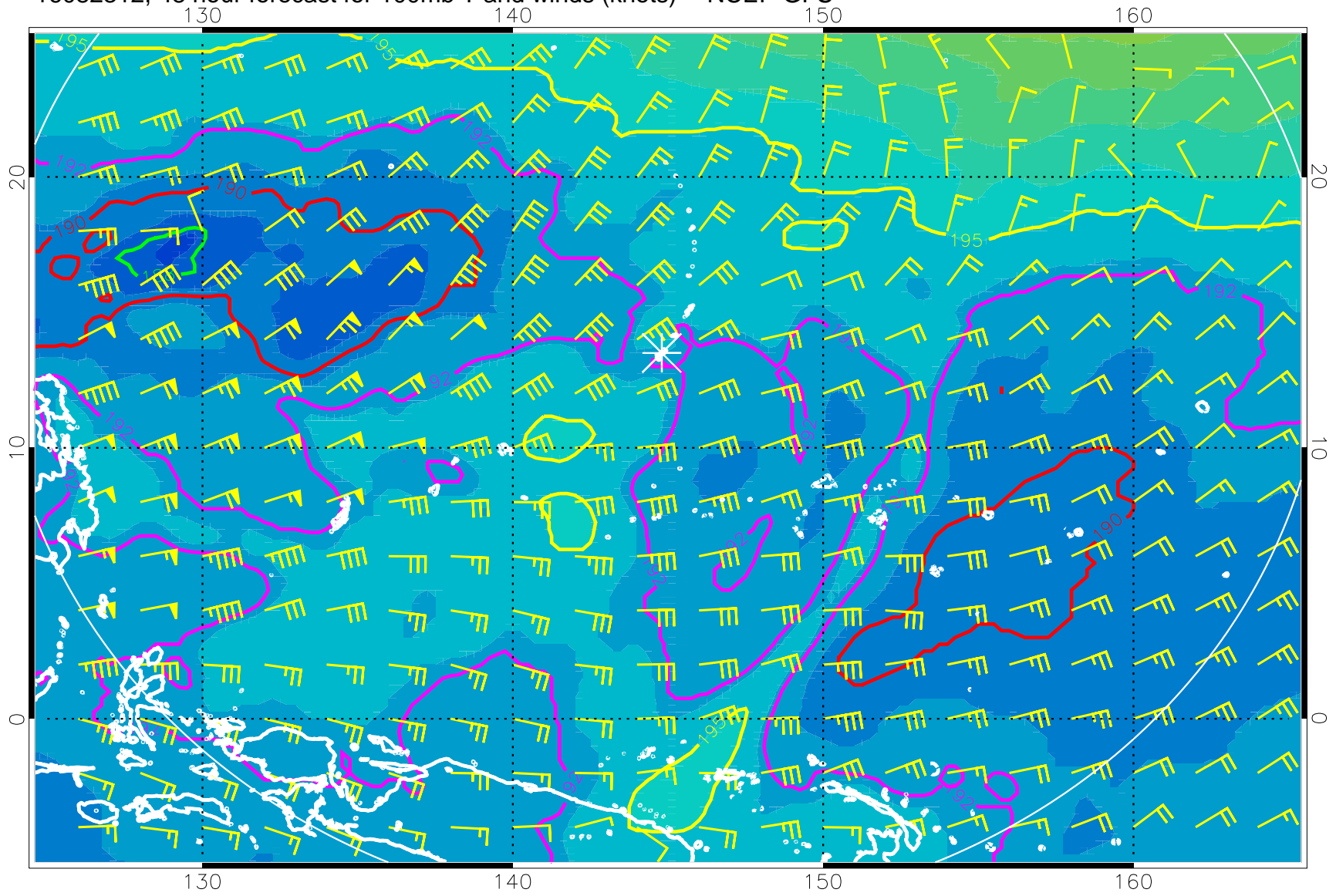
16082312, 48 hour forecast for 100mb T and winds (knots) -- NCEP GFS
