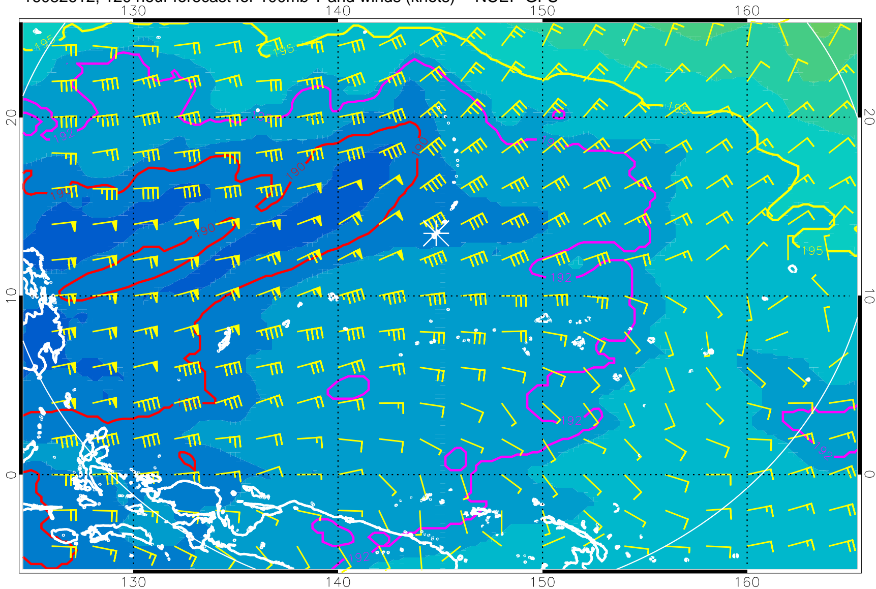
16082612, 120 hour forecast for 100mb T and winds (knots) -- NCEP GFS
