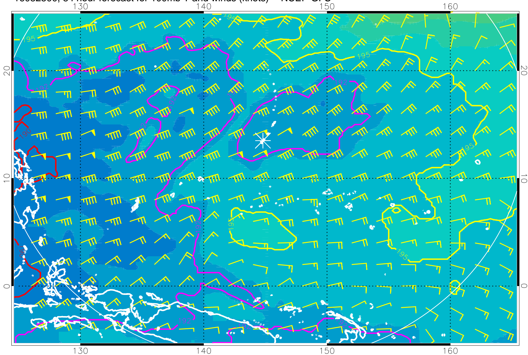
16082500, 84 hour forecast for 100mb T and winds (knots) -- NCEP GFS
