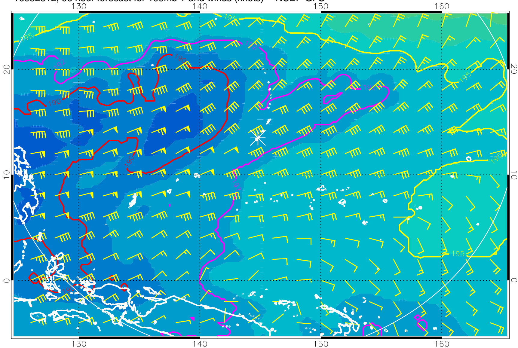
16082512, 96 hour forecast for 100mb T and winds (knots) -- NCEP GFS
