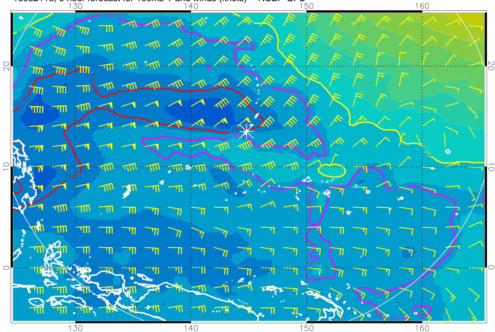
16082118, 6 hour forecast for 100mb T and winds (knots) -- NCEP GFS
