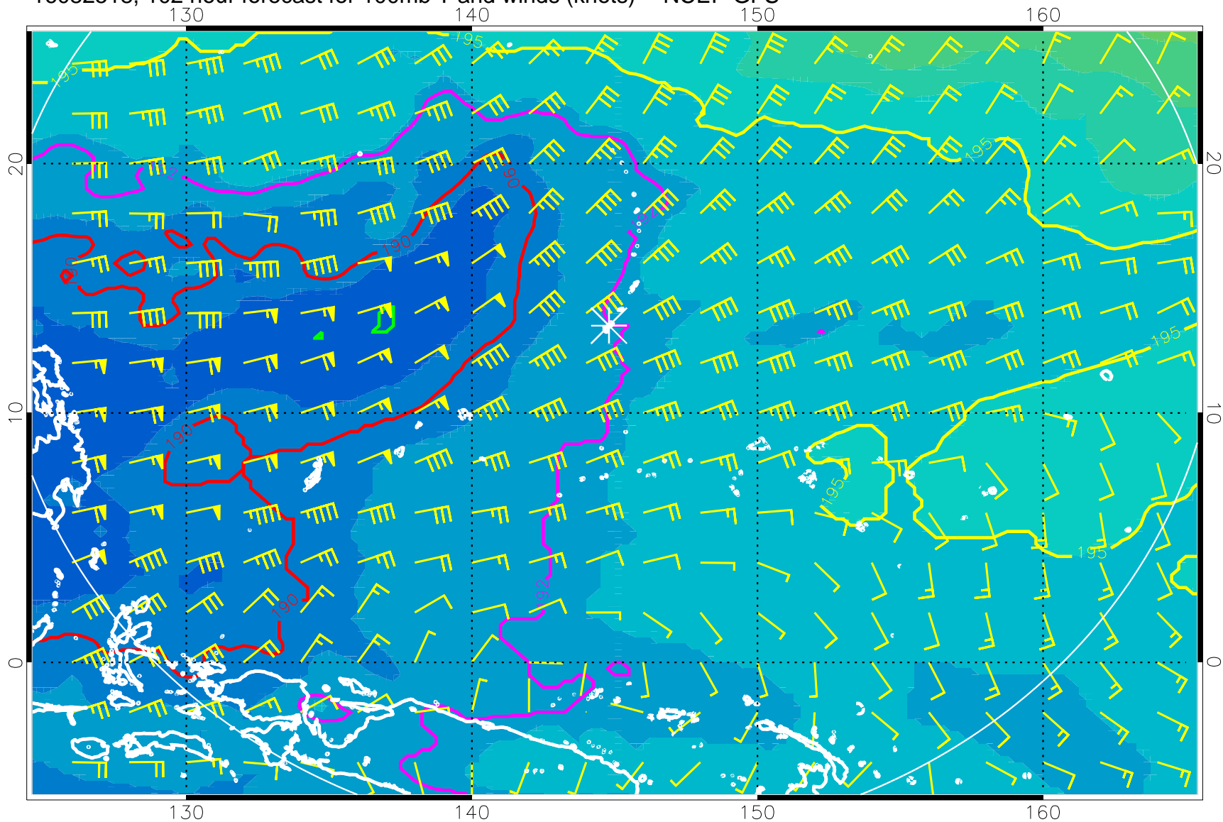
16082518, 102 hour forecast for 100mb T and winds (knots) -- NCEP GFS
