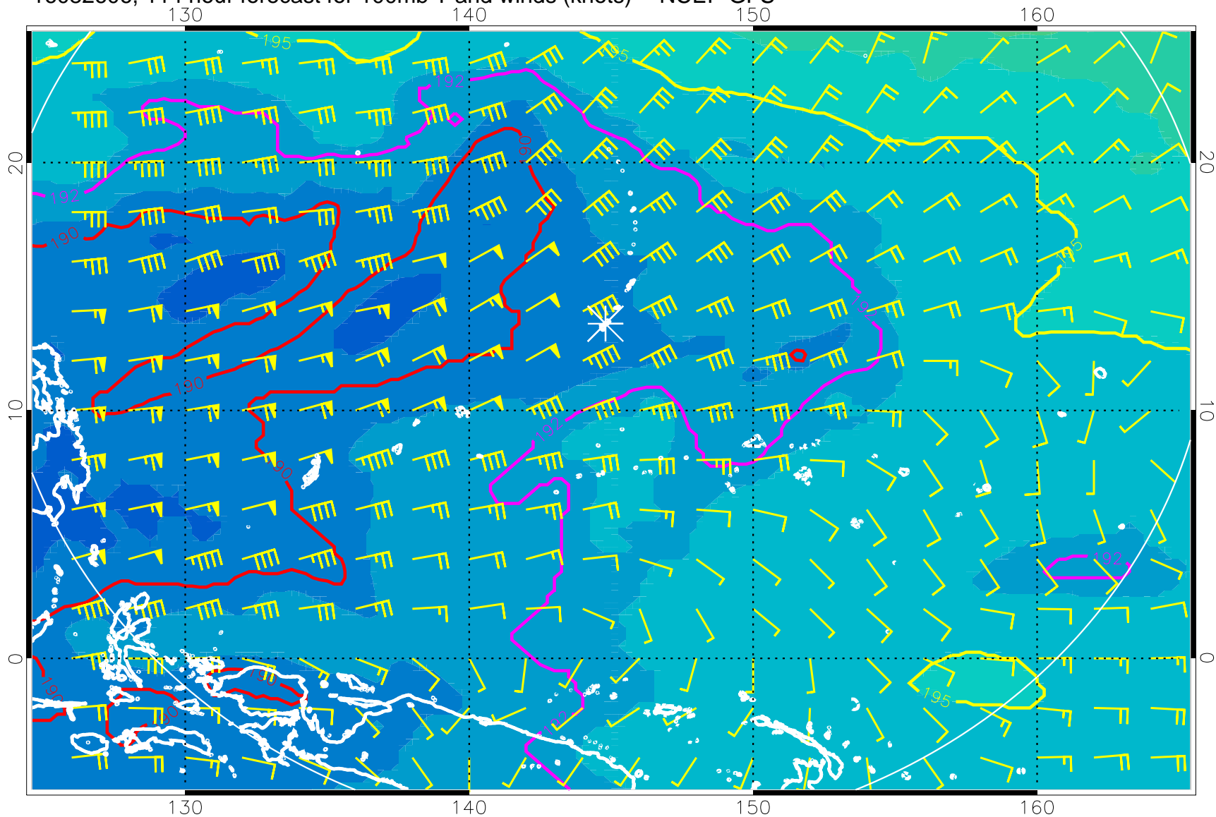
16082606, 114 hour forecast for 100mb T and winds (knots) -- NCEP GFS
