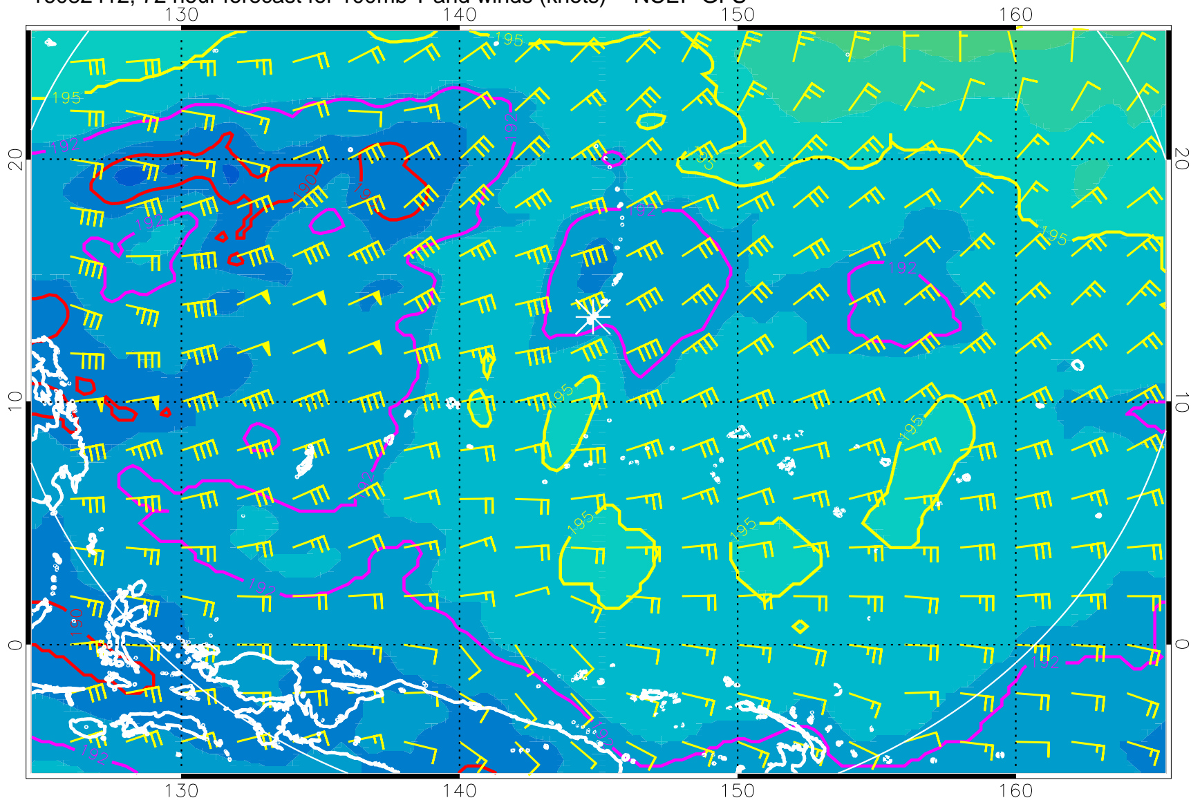
16082412, 72 hour forecast for 100mb T and winds (knots) -- NCEP GFS
