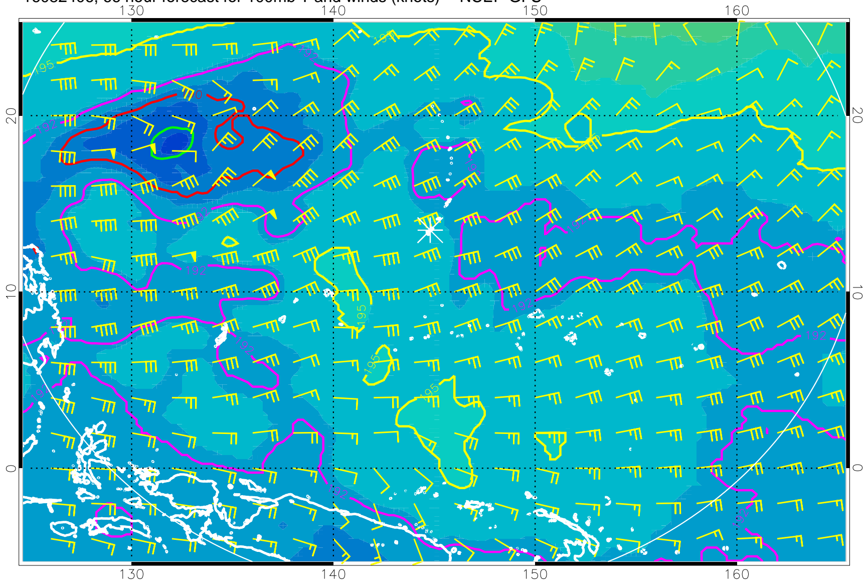
16082406, 66 hour forecast for 100mb T and winds (knots) -- NCEP GFS
