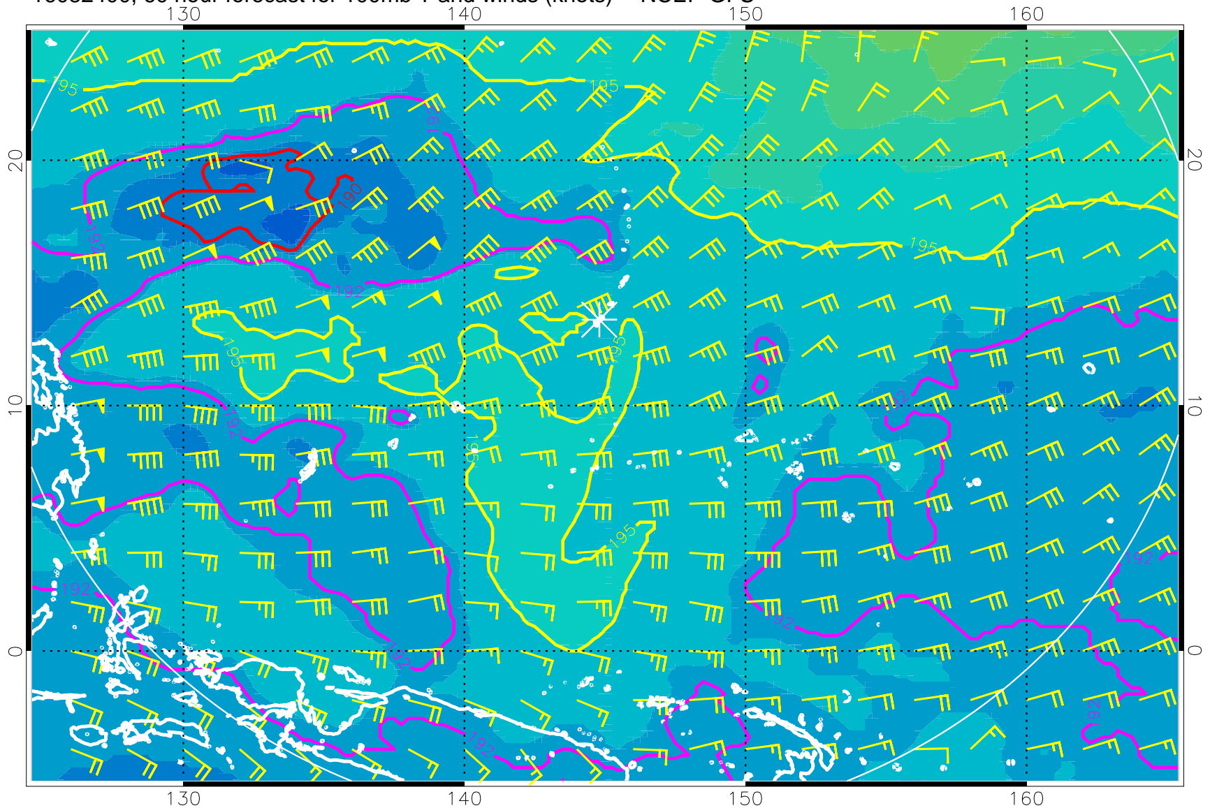
16082400, 60 hour forecast for 100mb T and winds (knots) -- NCEP GFS
