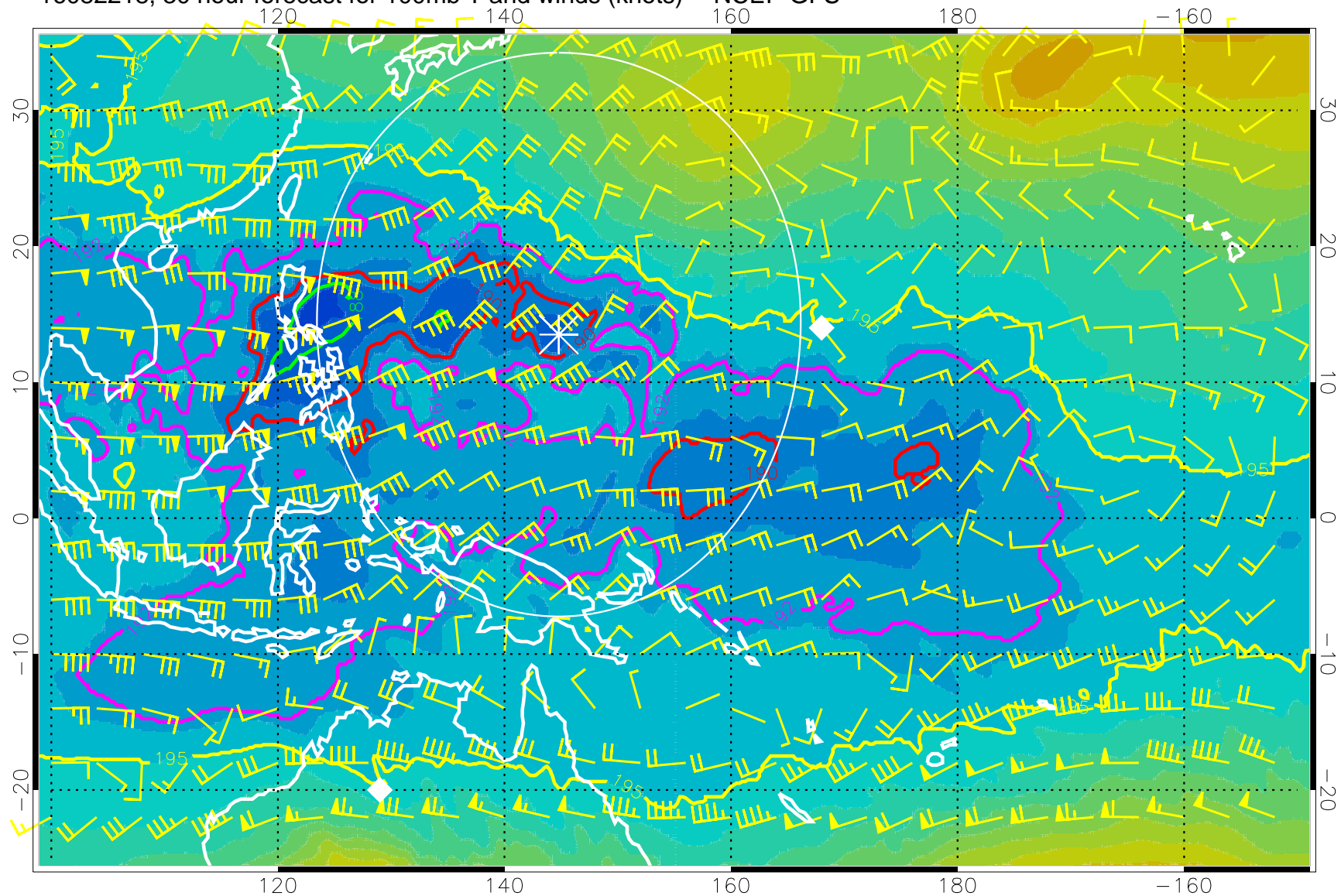
16082218, 30 hour forecast for 100mb T and winds (knots) -- NCEP GFS
