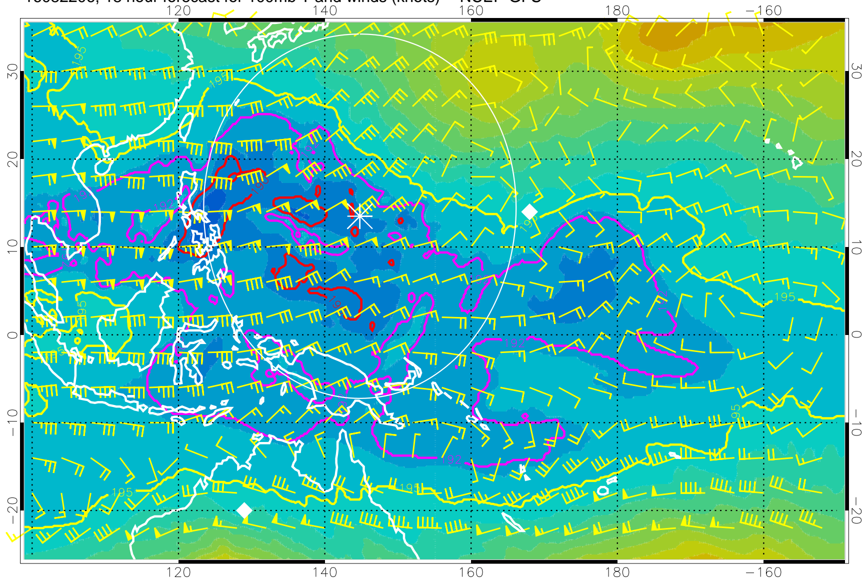
16082206, 18 hour forecast for 100mb T and winds (knots) -- NCEP GFS
