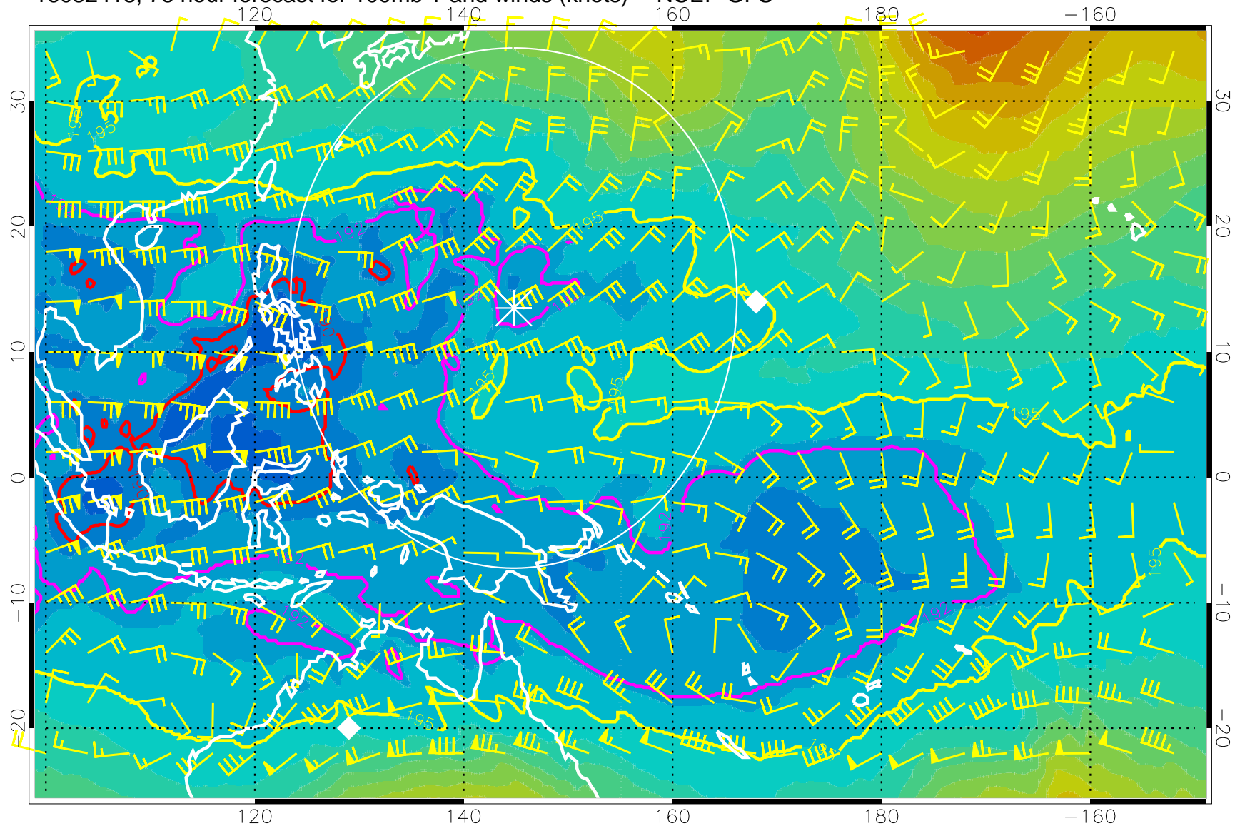
16082418, 78 hour forecast for 100mb T and winds (knots) -- NCEP GFS
