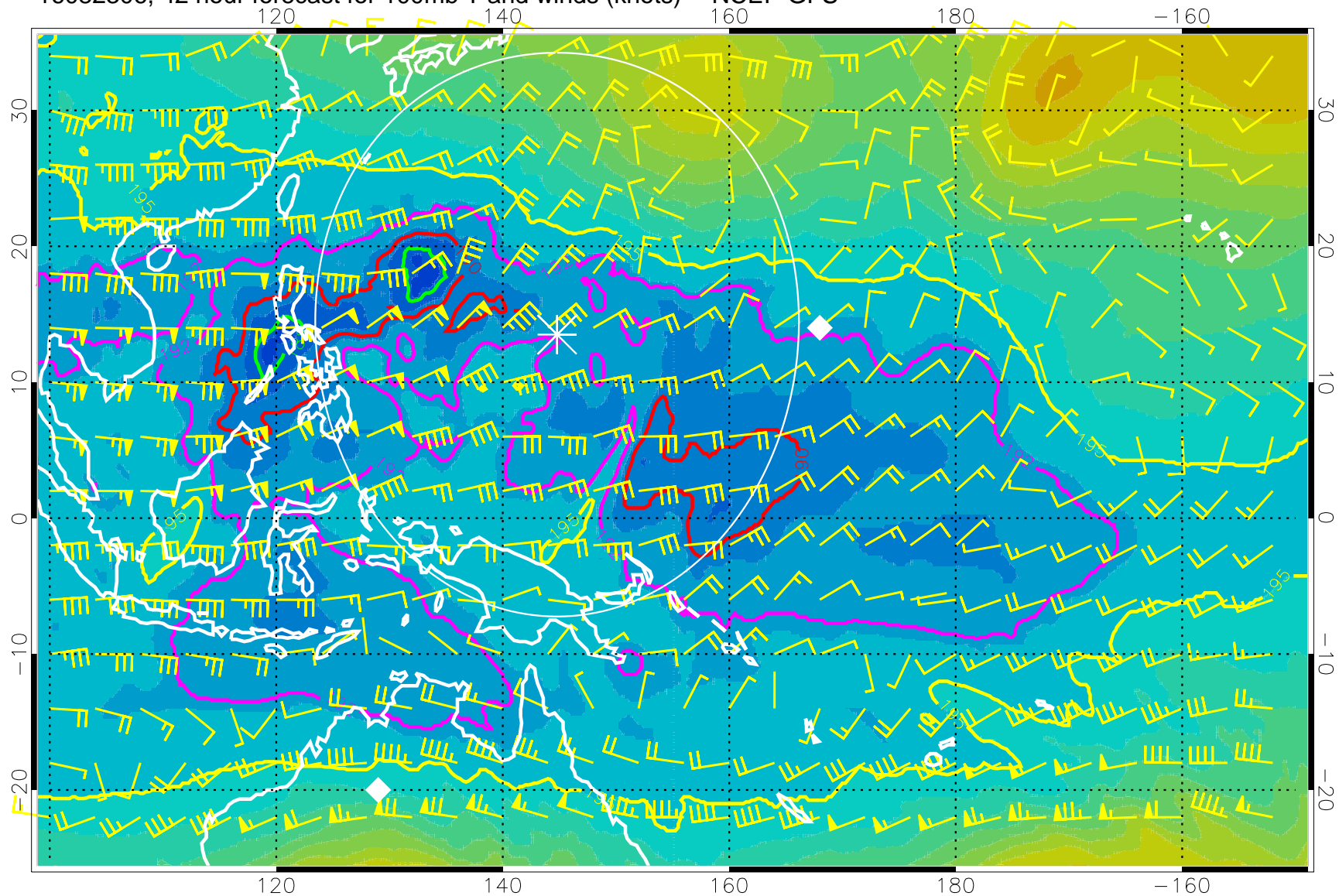
16082306, 42 hour forecast for 100mb T and winds (knots) -- NCEP GFS
