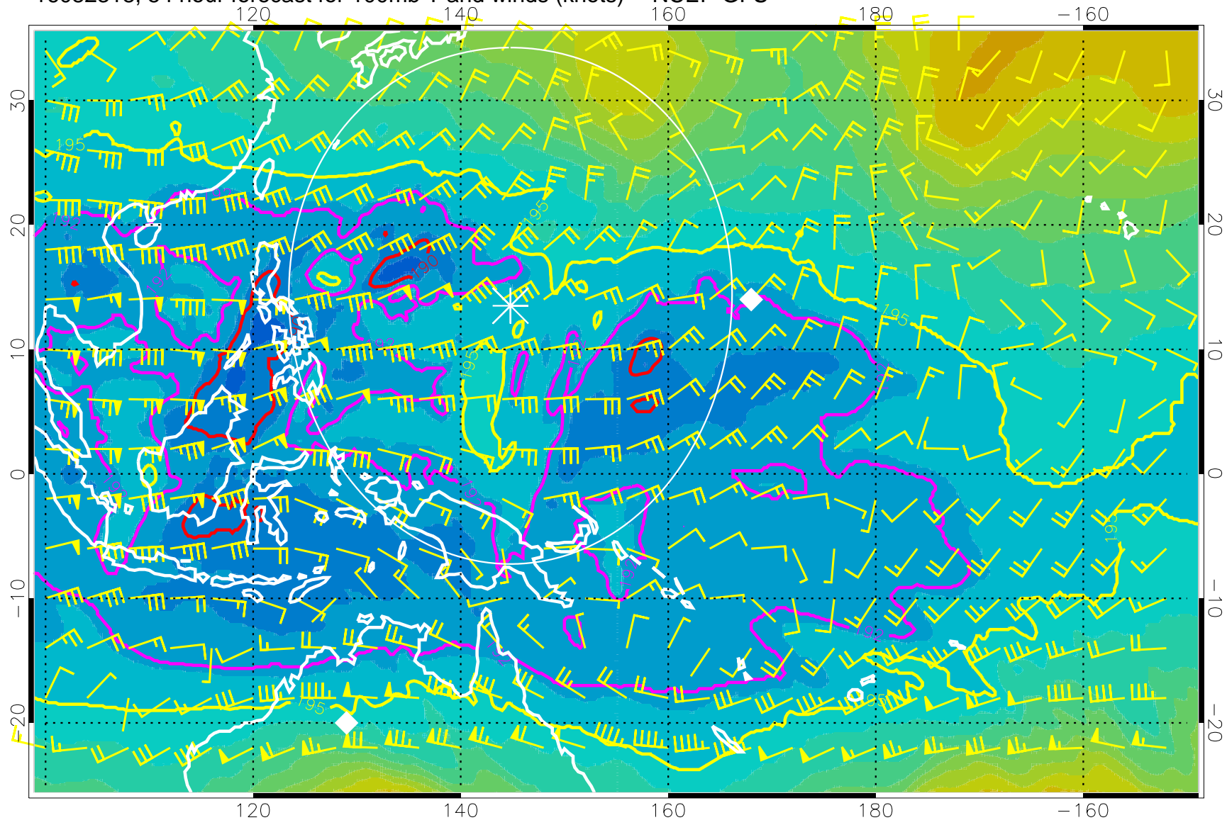
16082318, 54 hour forecast for 100mb T and winds (knots) -- NCEP GFS
