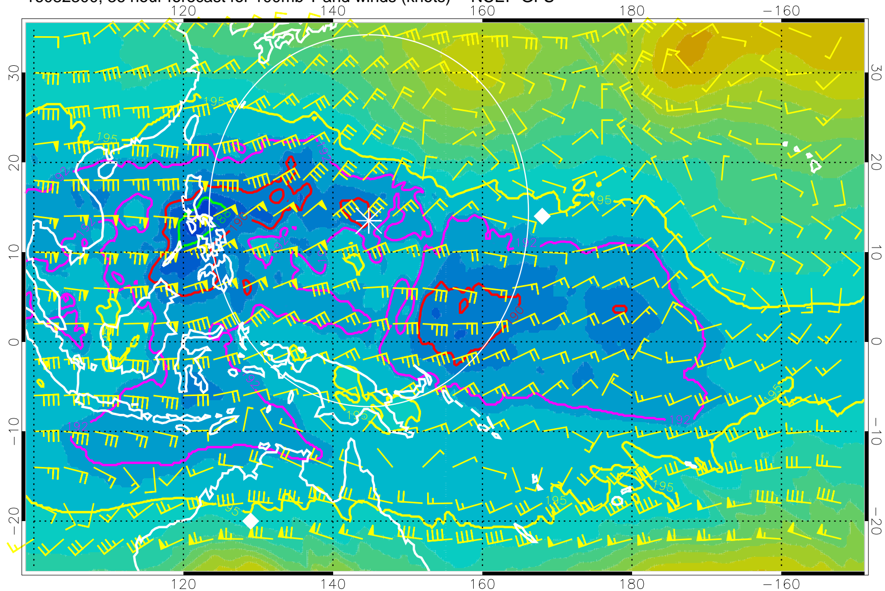
16082300, 36 hour forecast for 100mb T and winds (knots) -- NCEP GFS
