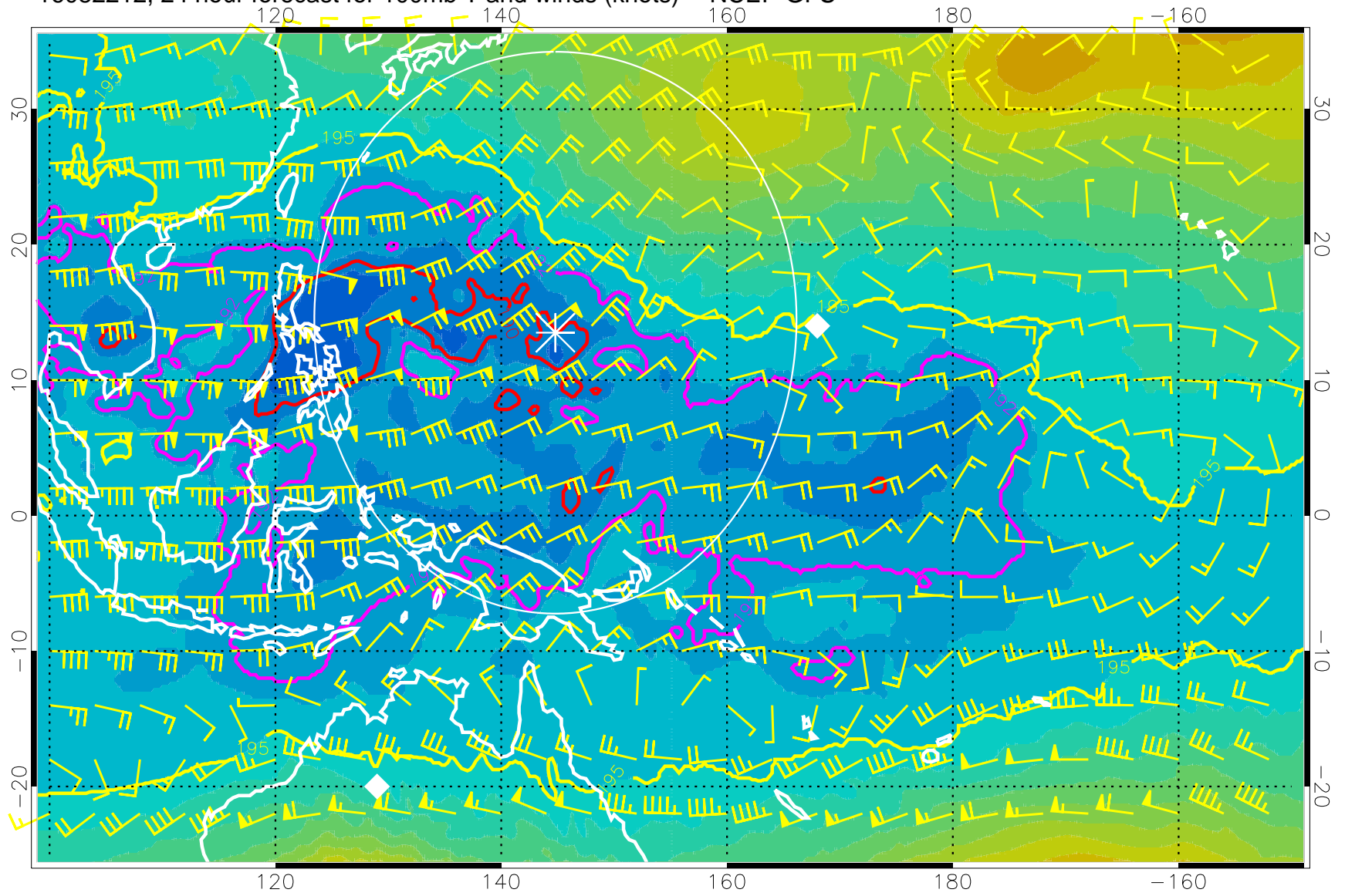
16082212, 24 hour forecast for 100mb T and winds (knots) -- NCEP GFS
