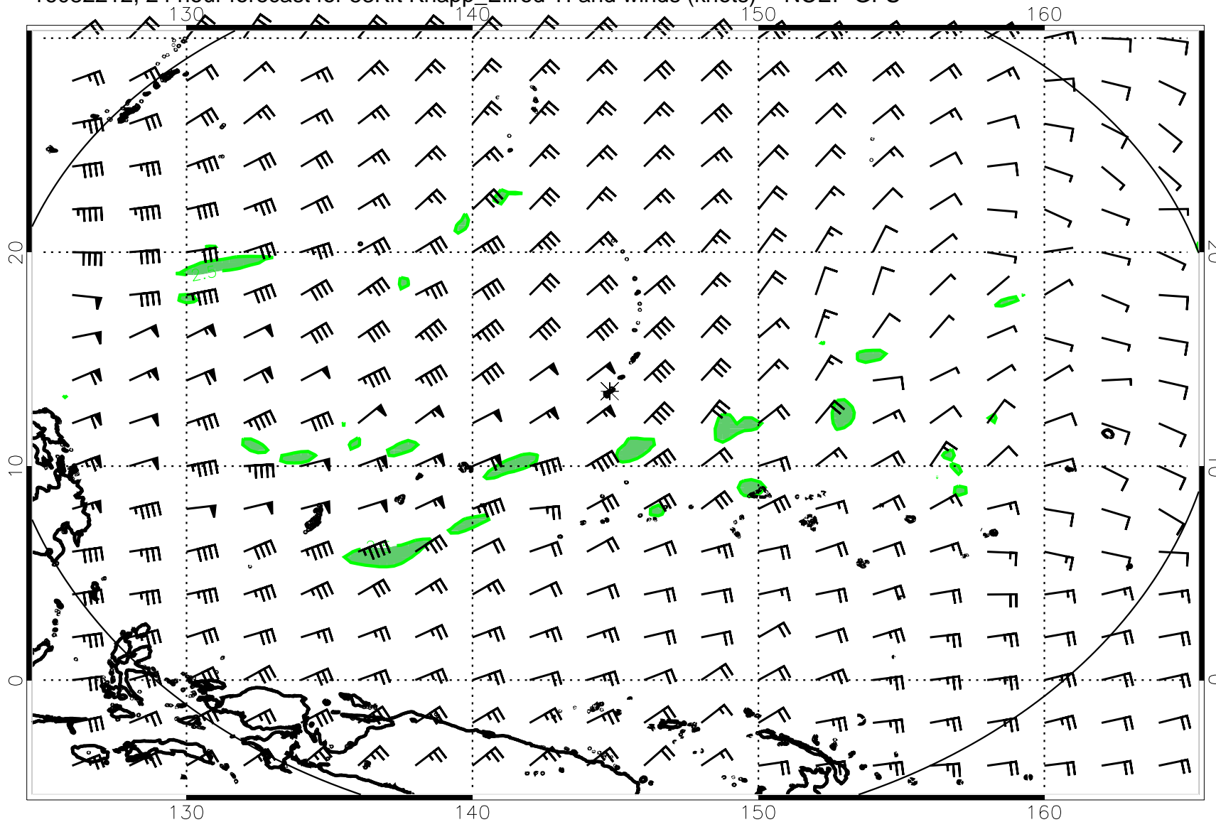
16082212, 24 hour forecast for 53Kft Knapp_Ellrod TI and winds (knots) -- NCEP GFS
