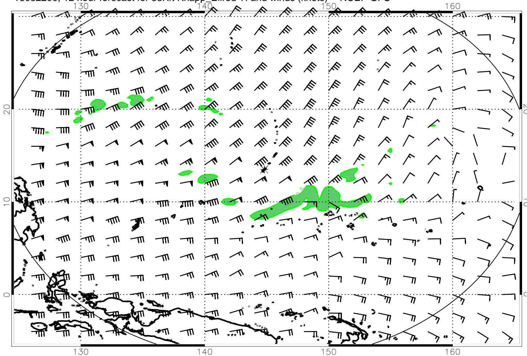
16082200, 12 hour forecast for 53Kft Knapp_Ellrod TI and winds (knots) -- NCEP GFS
