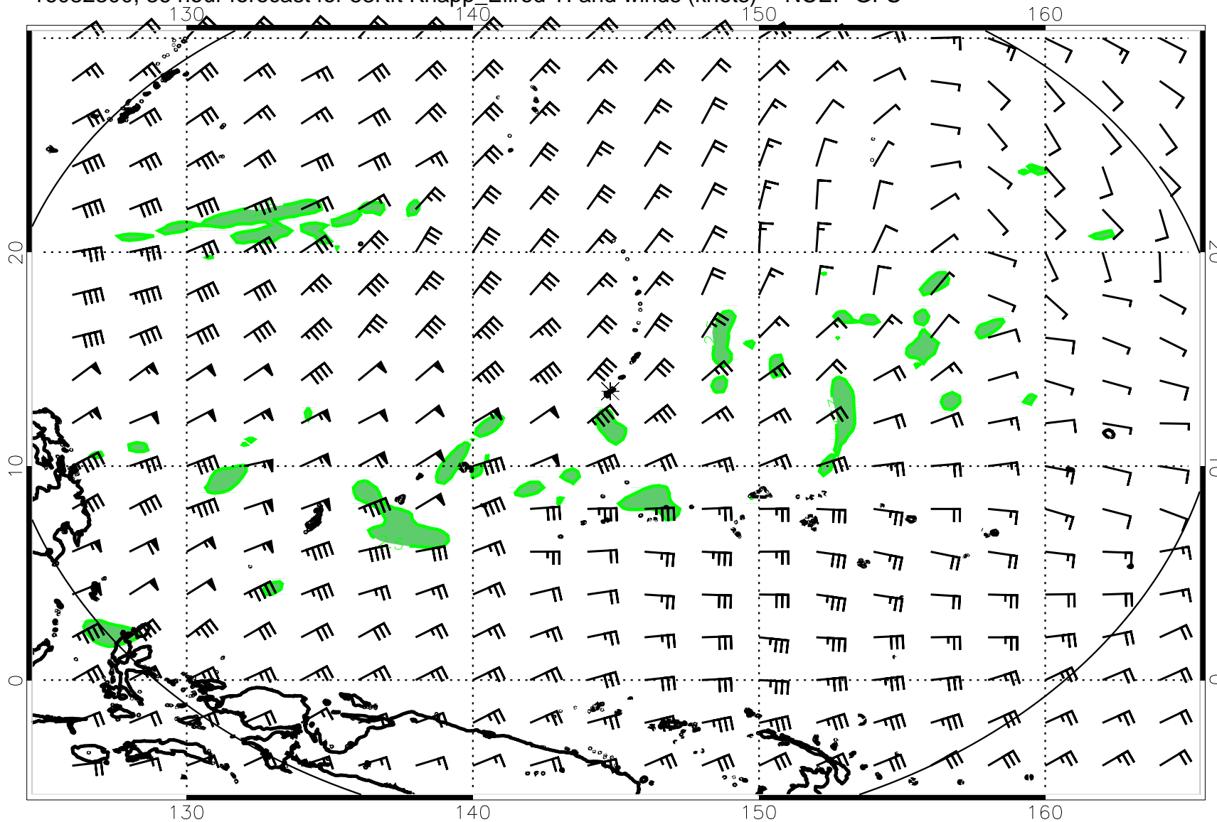
16082300, 36 hour forecast for 53Kft Knapp_Ellrod TI and winds (knots) -- NCEP GFS
