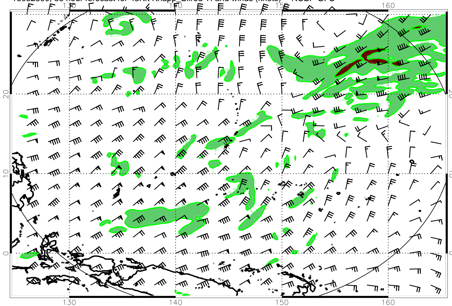
16082300, 36 hour forecast for 45Kft Knapp_Ellrod TI and winds (knots) -- NCEP GFS
