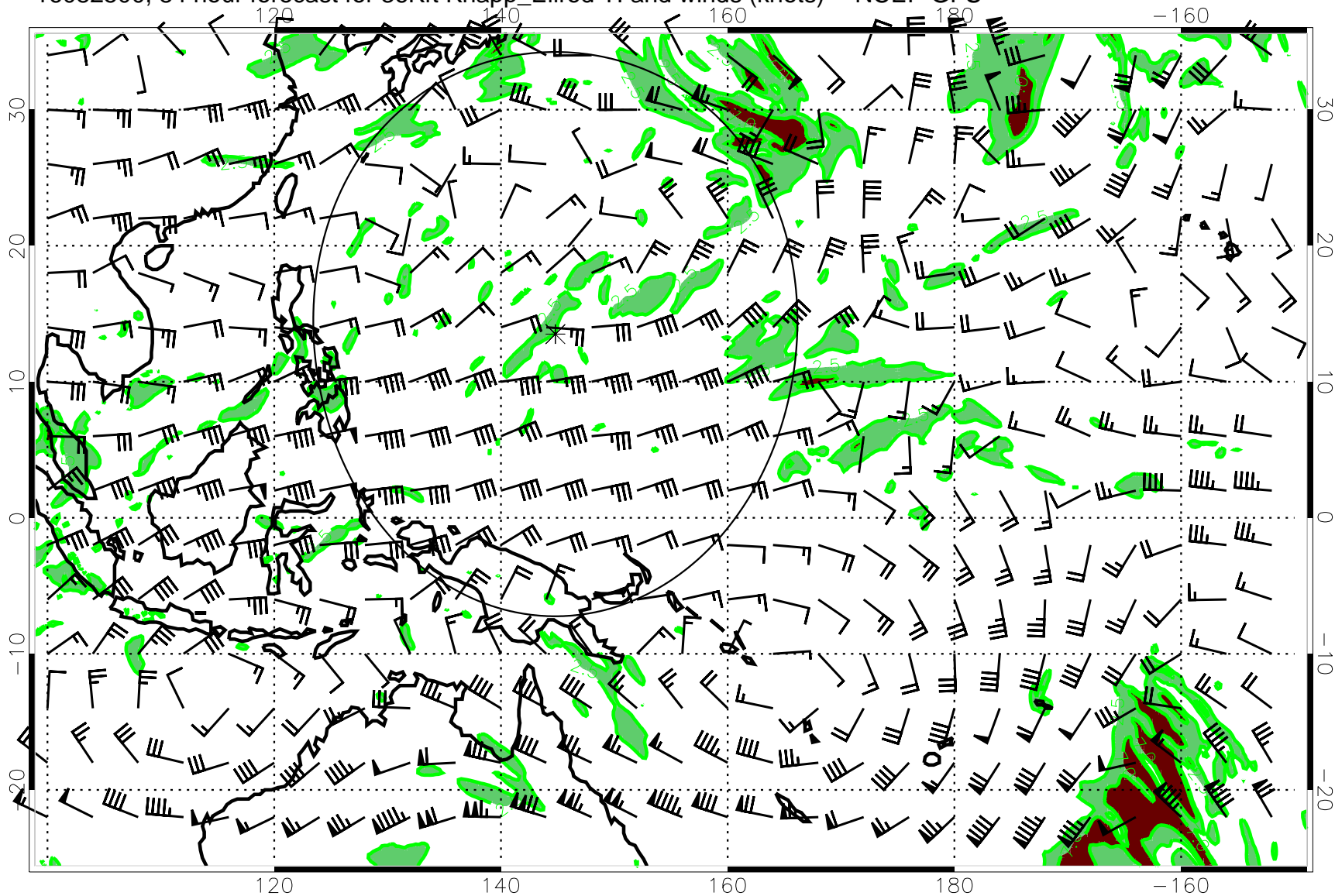
16082500, 84 hour forecast for 36Kft Knapp_Ellrod TI and winds (knots) -- NCEP GFS
