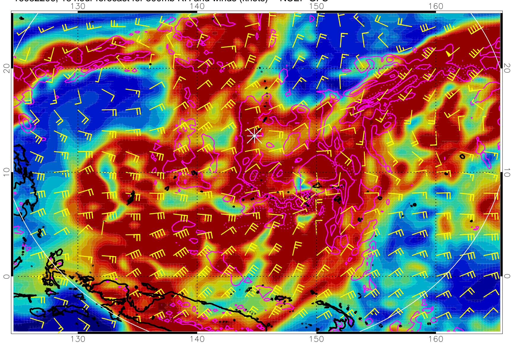
16082206, 18 hour forecast for 300mb RH and winds (knots) -- NCEP GFS
