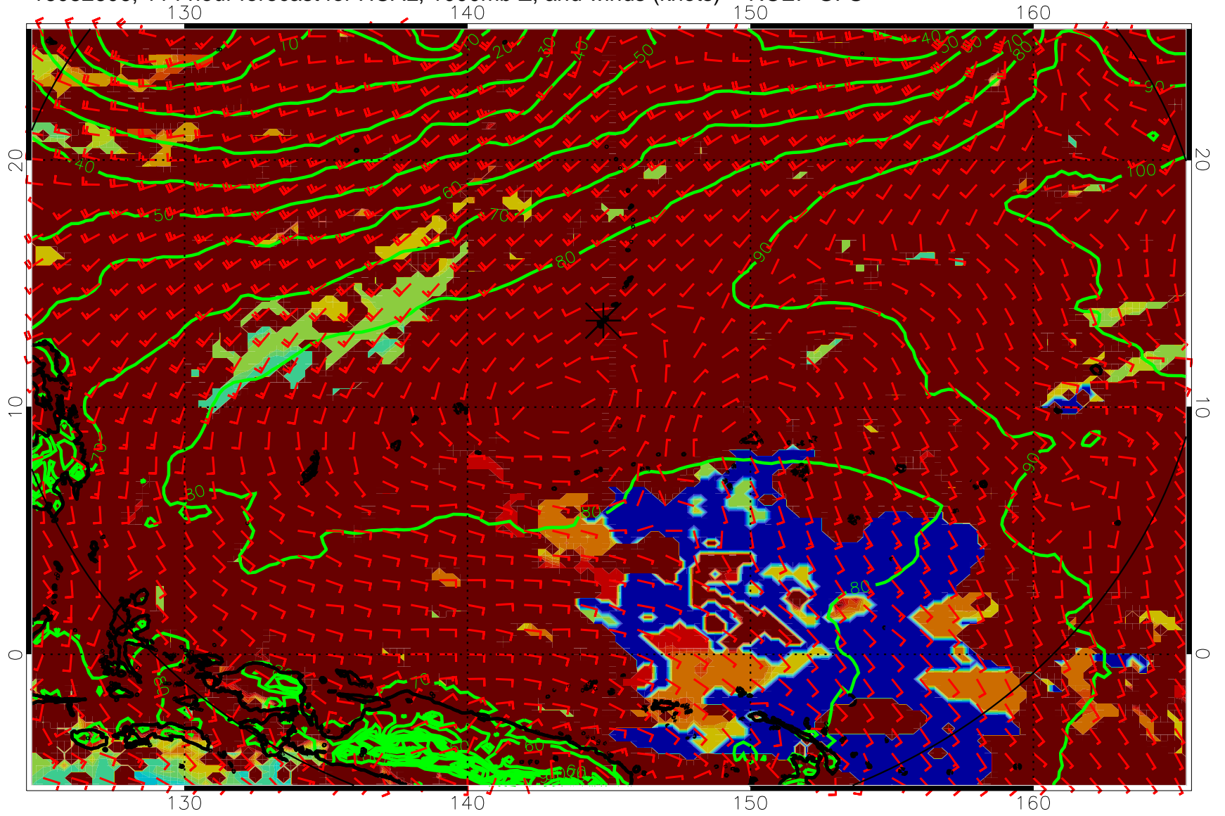
16082606, 114 hour forecast for HCAL, 1000mb Z, and winds (knots) -- NCEP GFS
