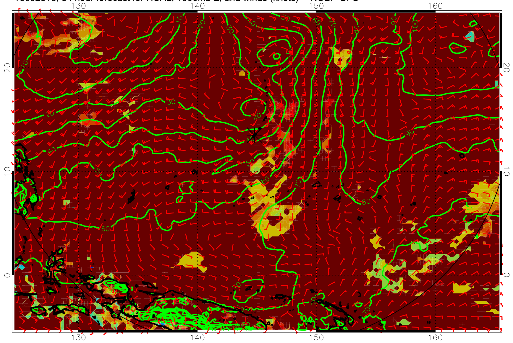
16082318, 54 hour forecast for HCAL, 1000mb Z, and winds (knots) -- NCEP GFS
