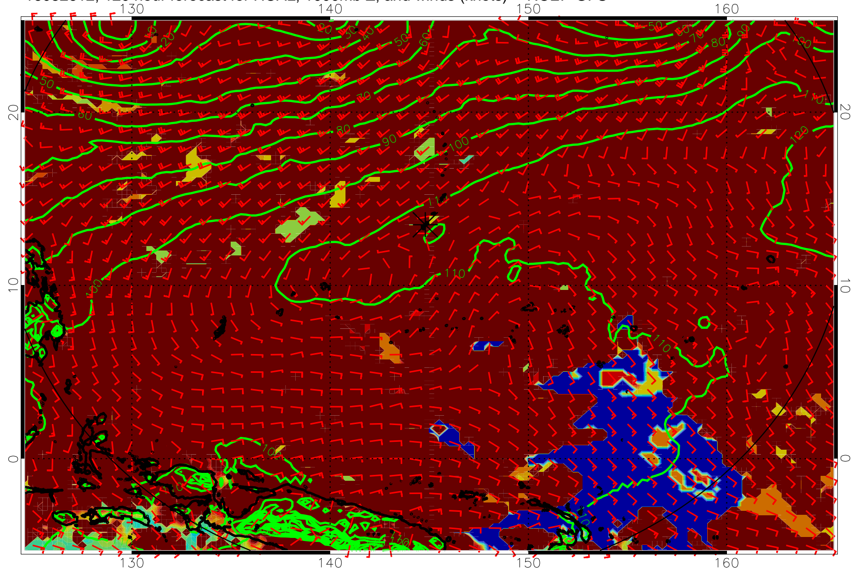
16082612, 120 hour forecast for HCAL, 1000mb Z, and winds (knots) -- NCEP GFS
