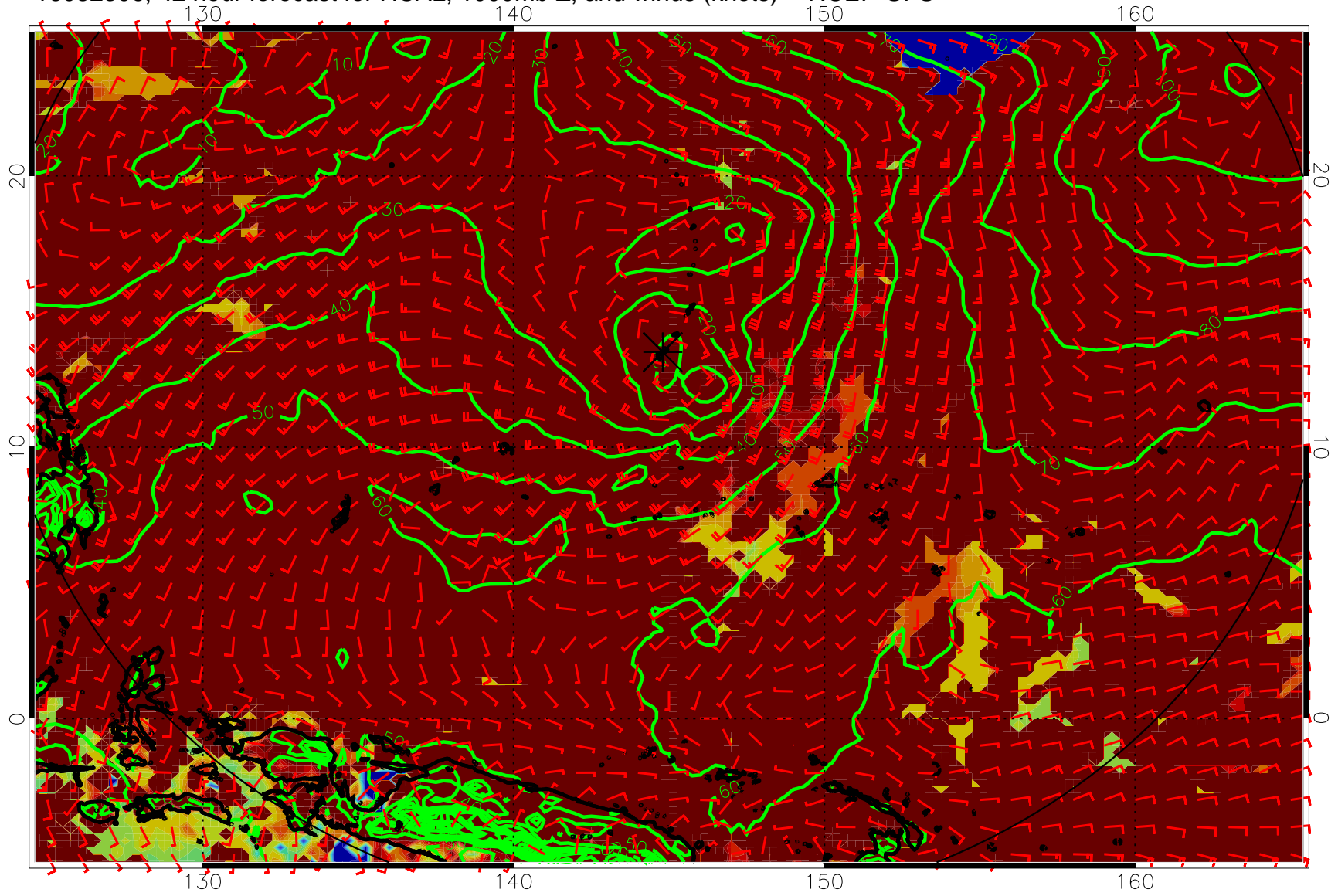
16082306, 42 hour forecast for HCAL, 1000mb Z, and winds (knots) -- NCEP GFS
