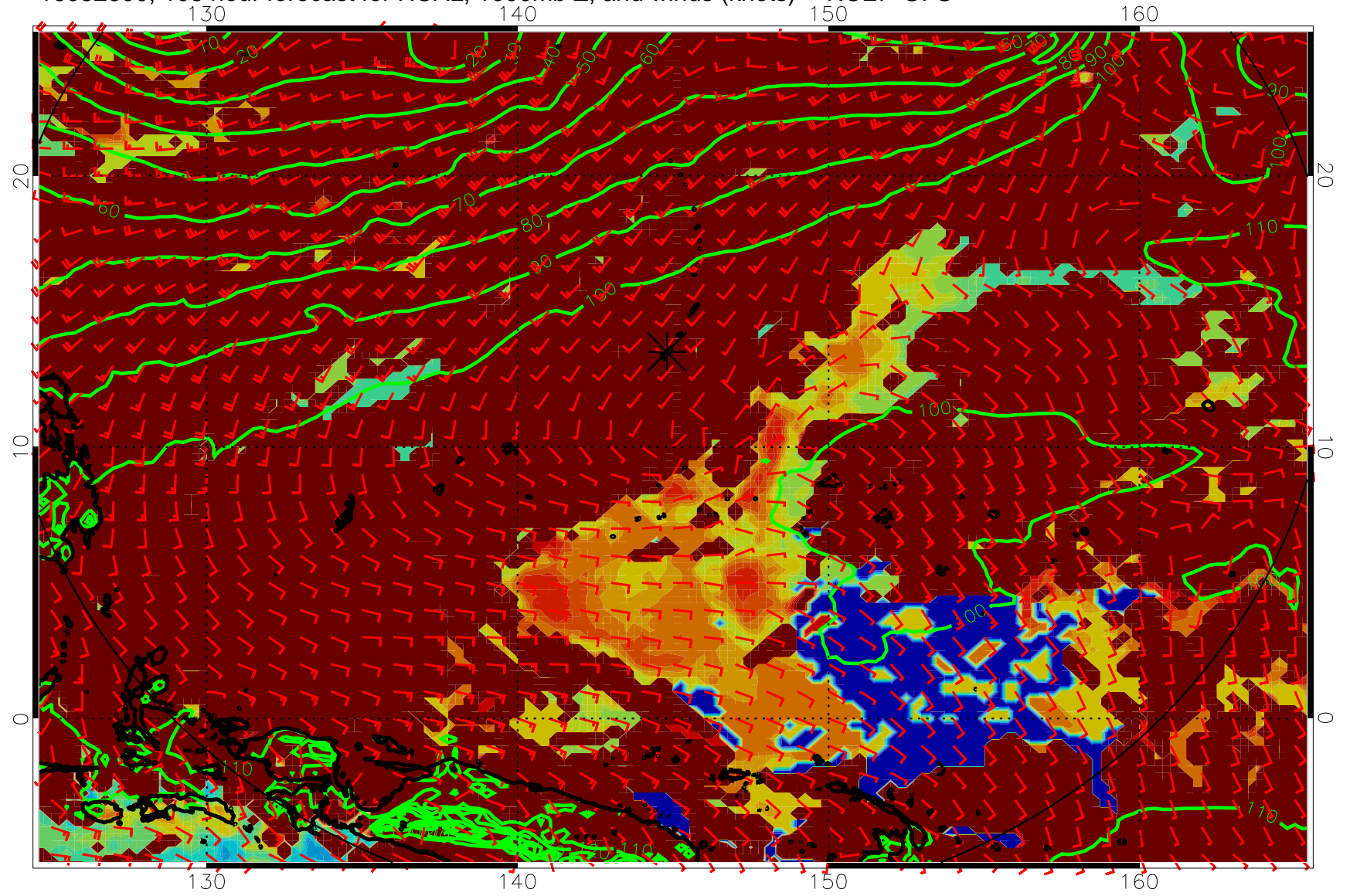
16082600, 108 hour forecast for HCAL, 1000mb Z, and winds (knots) -- NCEP GFS
