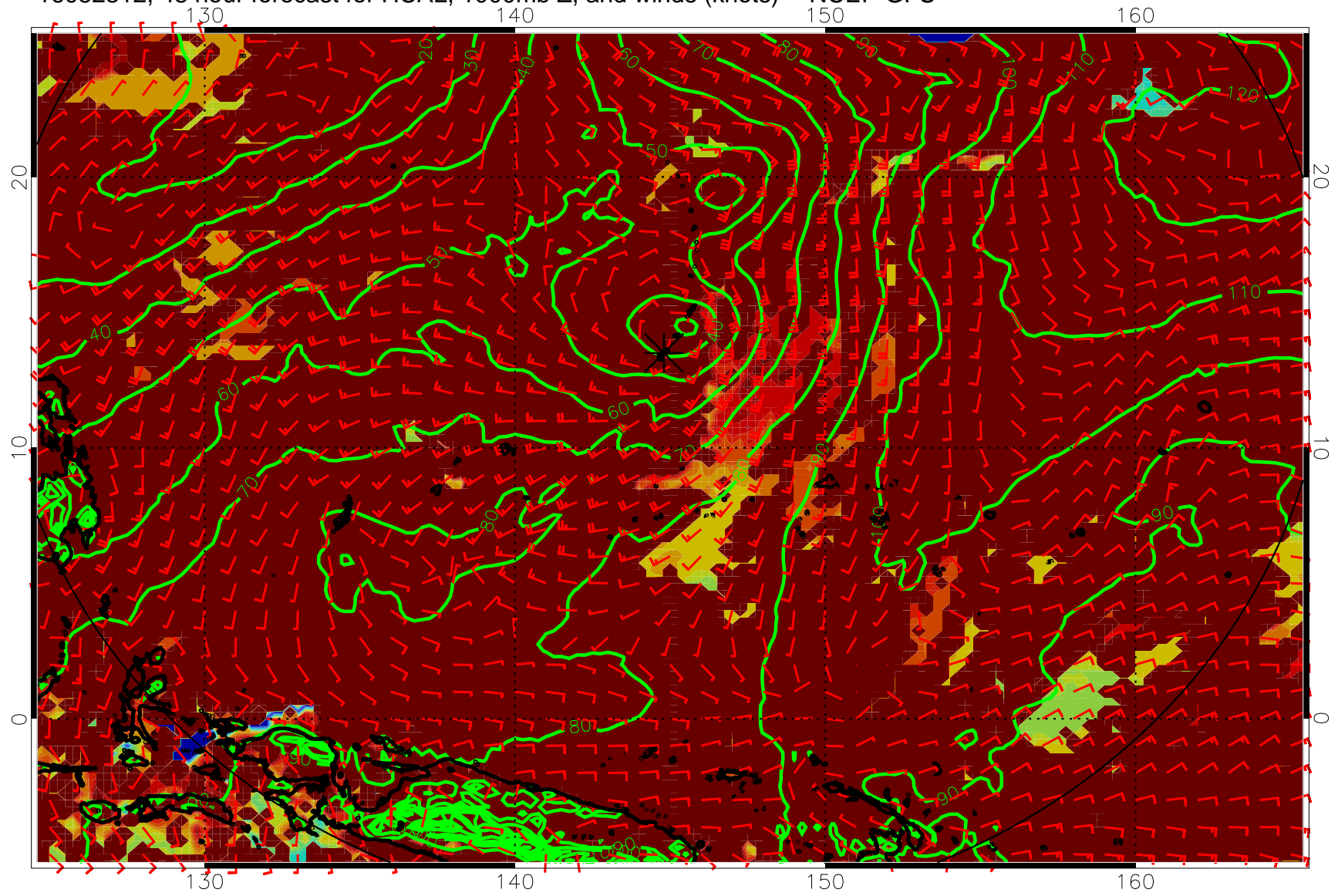
16082312, 48 hour forecast for HCAL, 1000mb Z, and winds (knots) -- NCEP GFS
