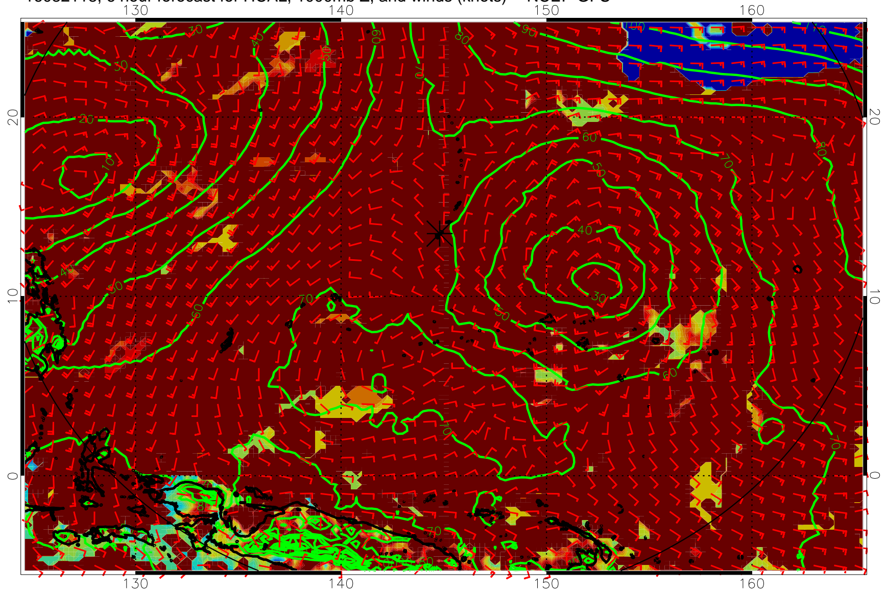
16082118, 6 hour forecast for HCAL, 1000mb Z, and winds (knots) -- NCEP GFS
