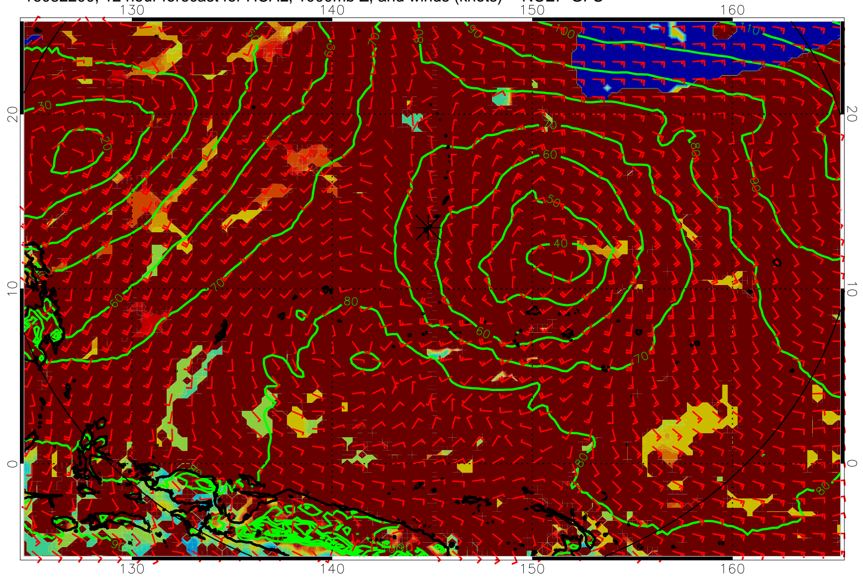
16082200, 12 hour forecast for HCAL, 1000mb Z, and winds (knots) -- NCEP GFS
