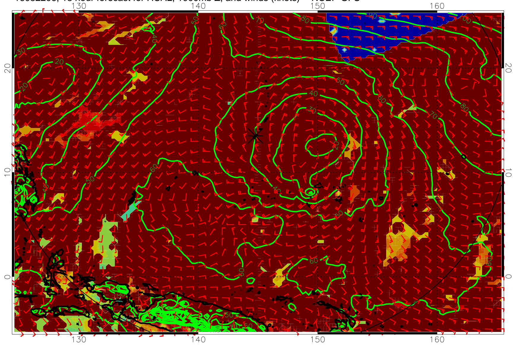
16082206, 18 hour forecast for HCAL, 1000mb Z, and winds (knots) -- NCEP GFS
