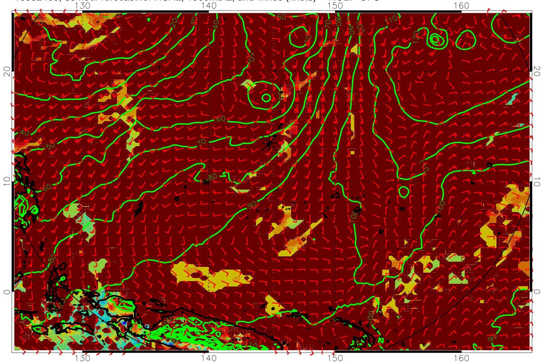
16082400, 60 hour forecast for HCAL, 1000mb Z, and winds (knots) -- NCEP GFS
