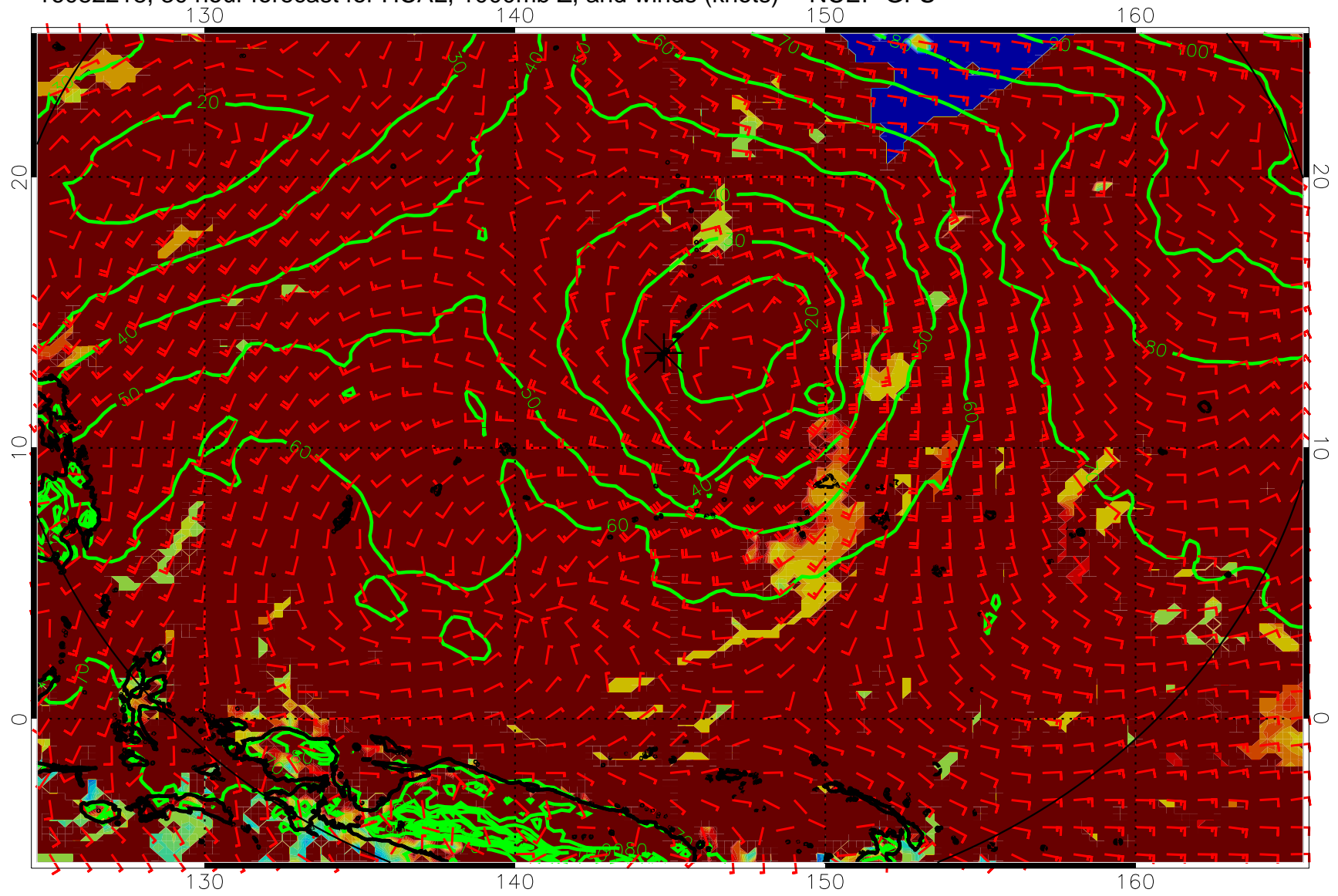
16082218, 30 hour forecast for HCAL, 1000mb Z, and winds (knots) -- NCEP GFS
