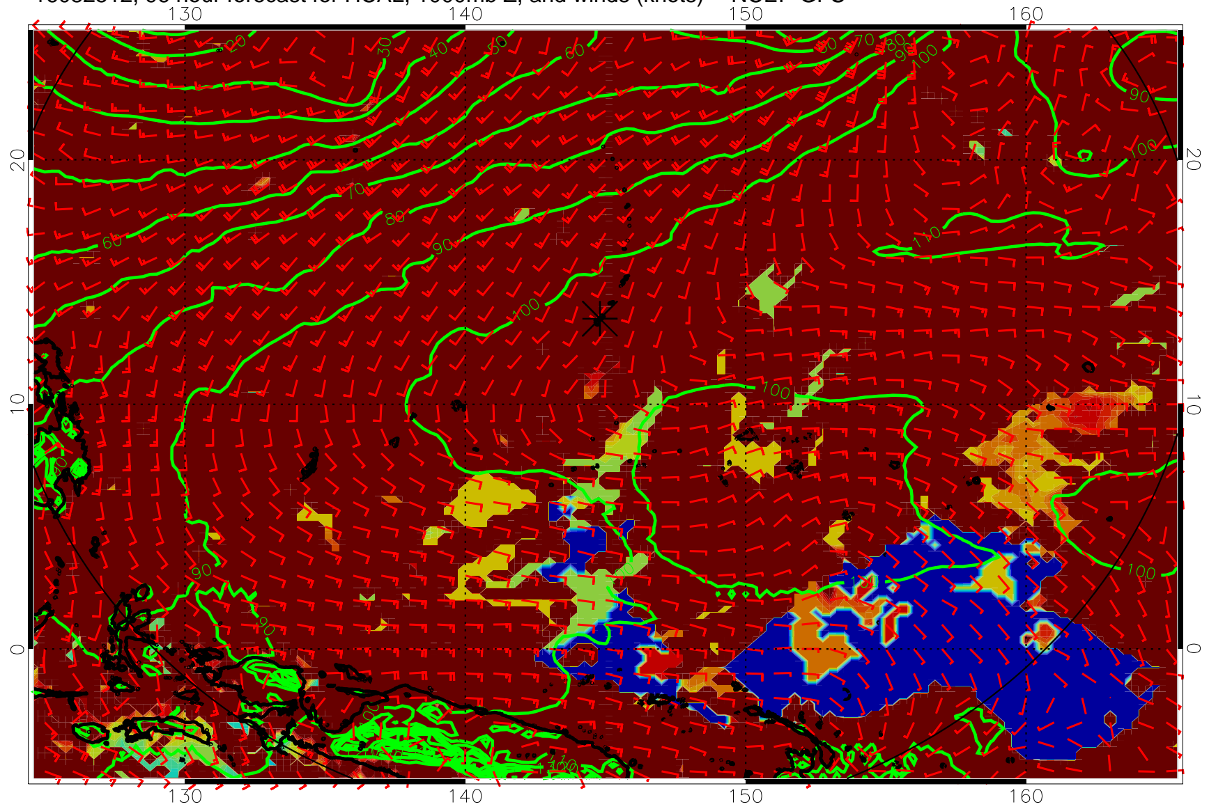
16082512, 96 hour forecast for HCAL, 1000mb Z, and winds (knots) -- NCEP GFS
