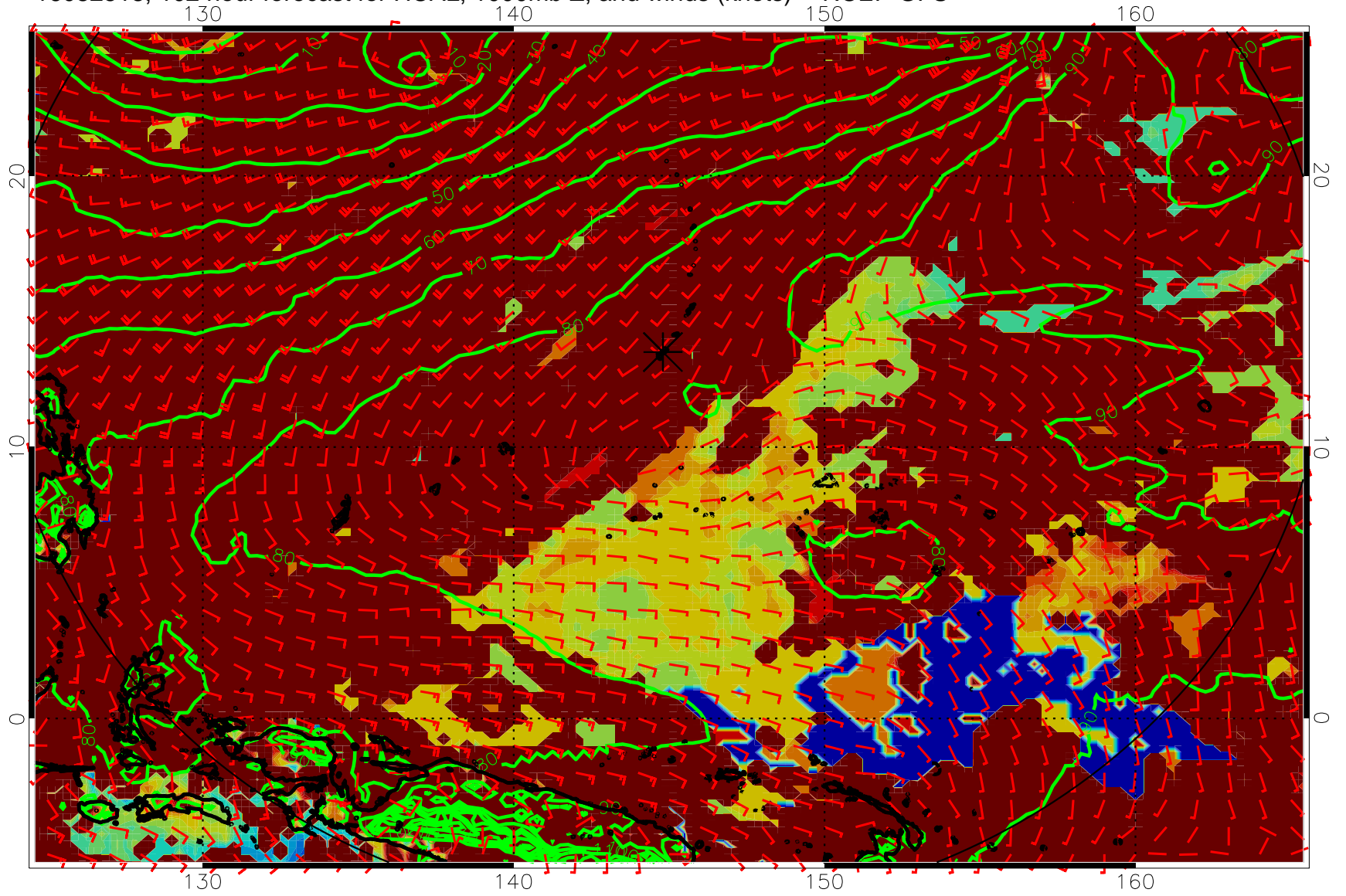
16082518, 102 hour forecast for HCAL, 1000mb Z, and winds (knots) -- NCEP GFS
