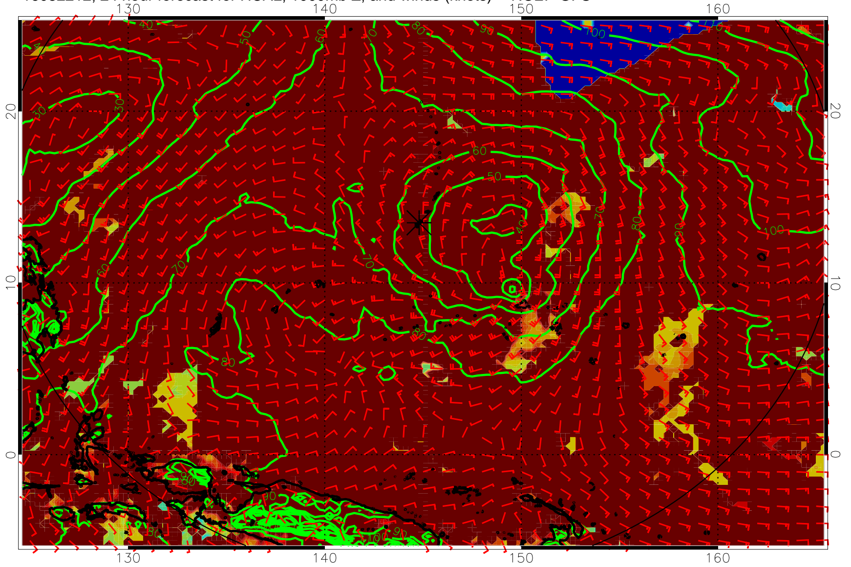
16082212, 24 hour forecast for HCAL, 1000mb Z, and winds (knots) -- NCEP GFS
