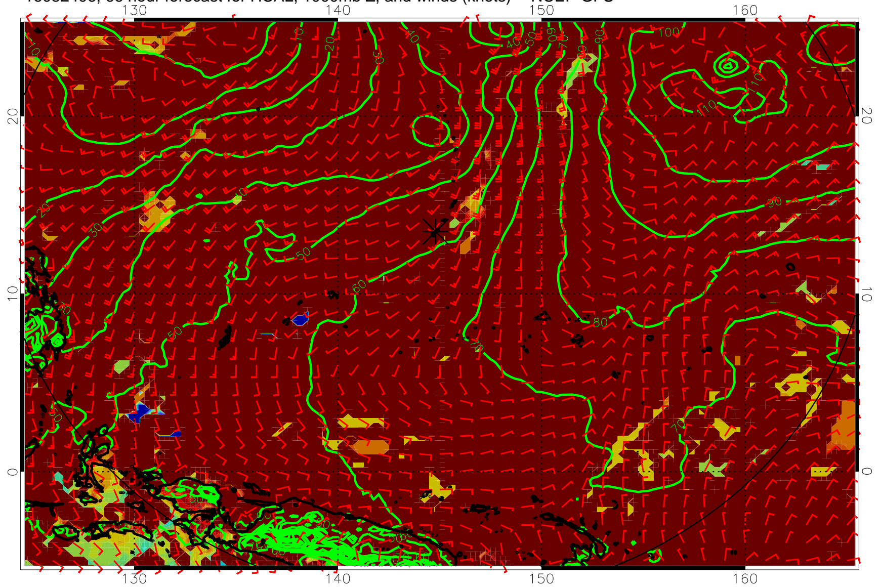
16082406, 66 hour forecast for HCAL, 1000mb Z, and winds (knots) -- NCEP GFS
