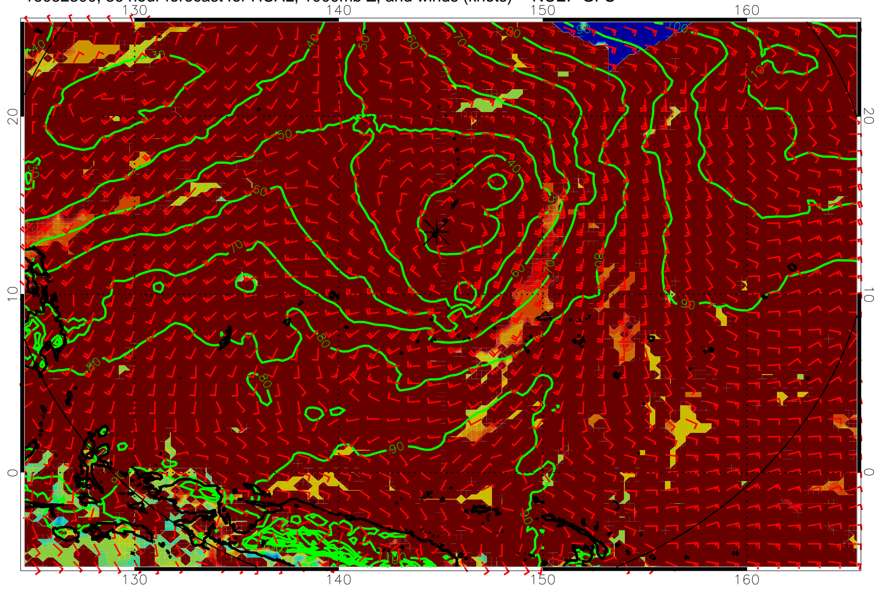
16082300, 36 hour forecast for HCAL, 1000mb Z, and winds (knots) -- NCEP GFS
