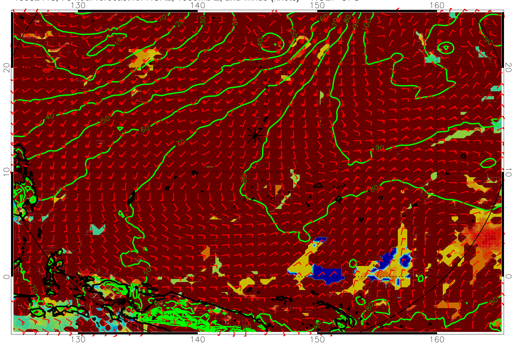
16082418, 78 hour forecast for HCAL, 1000mb Z, and winds (knots) -- NCEP GFS
