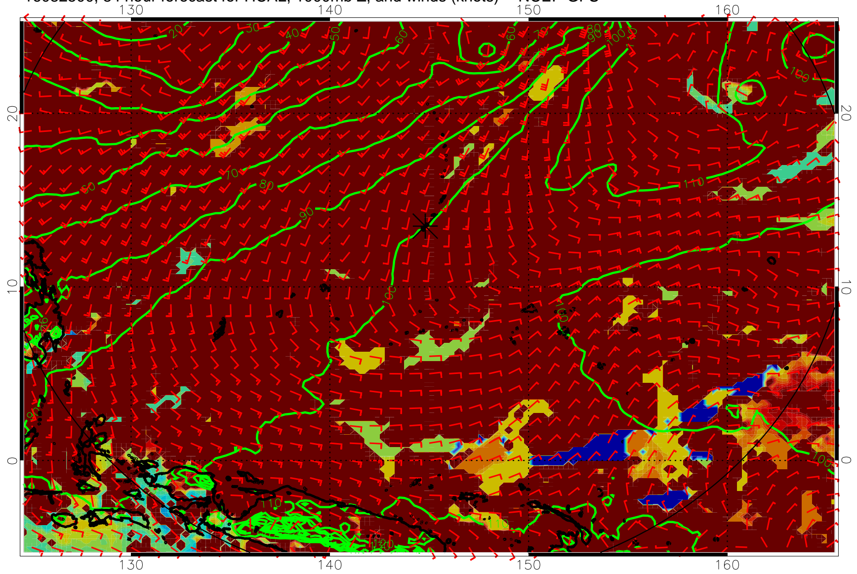
16082500, 84 hour forecast for HCAL, 1000mb Z, and winds (knots) -- NCEP GFS
