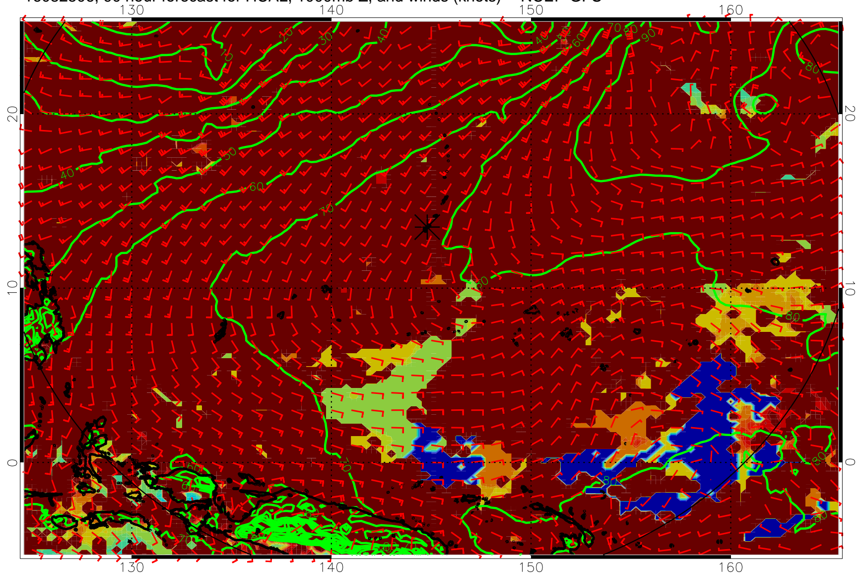
16082506, 90 hour forecast for HCAL, 1000mb Z, and winds (knots) -- NCEP GFS
