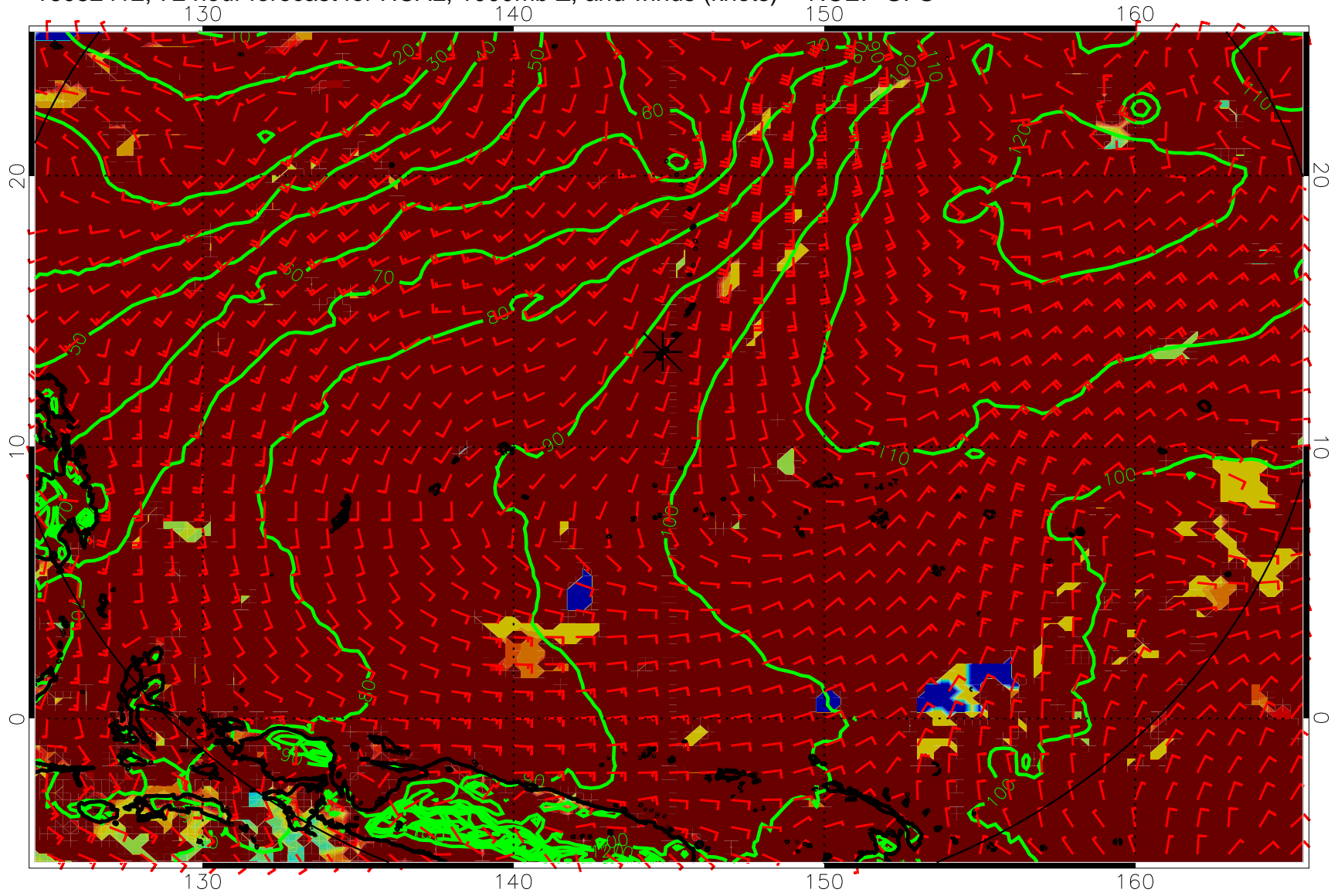
16082412, 72 hour forecast for HCAL, 1000mb Z, and winds (knots) -- NCEP GFS
