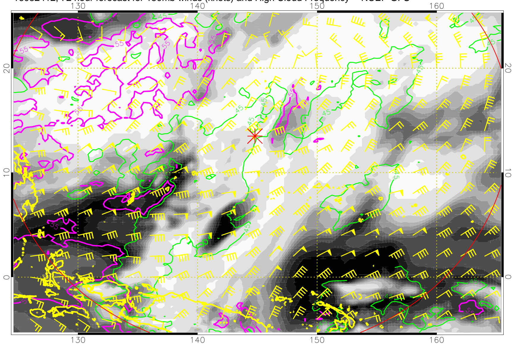
16082412, 72 hour forecast for 150mb winds (knots) and High Cloud Frequency -- NCEP GFS
