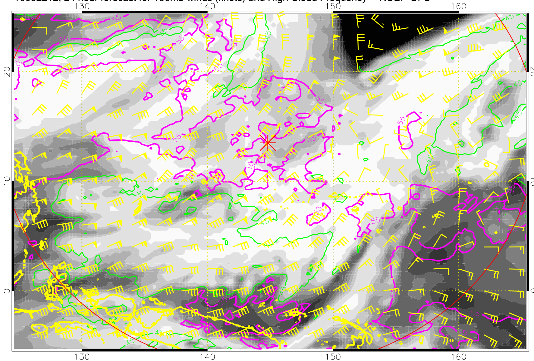
16082212, 24 hour forecast for 150mb winds (knots) and High Cloud Frequency -- NCEP GFS
