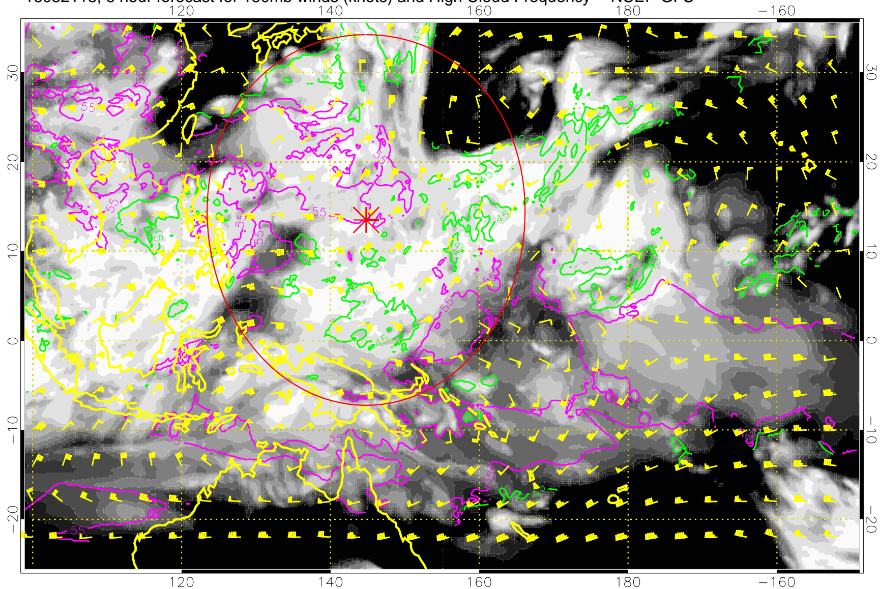
16082118, 6 hour forecast for 150mb winds (knots) and High Cloud Frequency -- NCEP GFS
