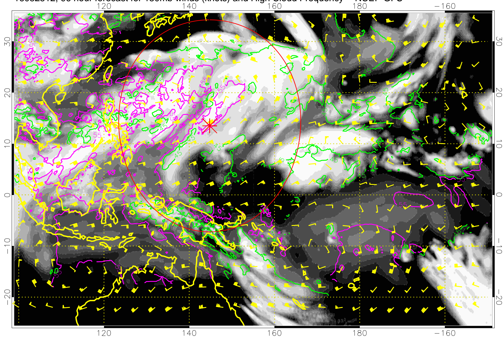
16082512, 96 hour forecast for 150mb winds (knots) and High Cloud Frequency -- NCEP GFS
