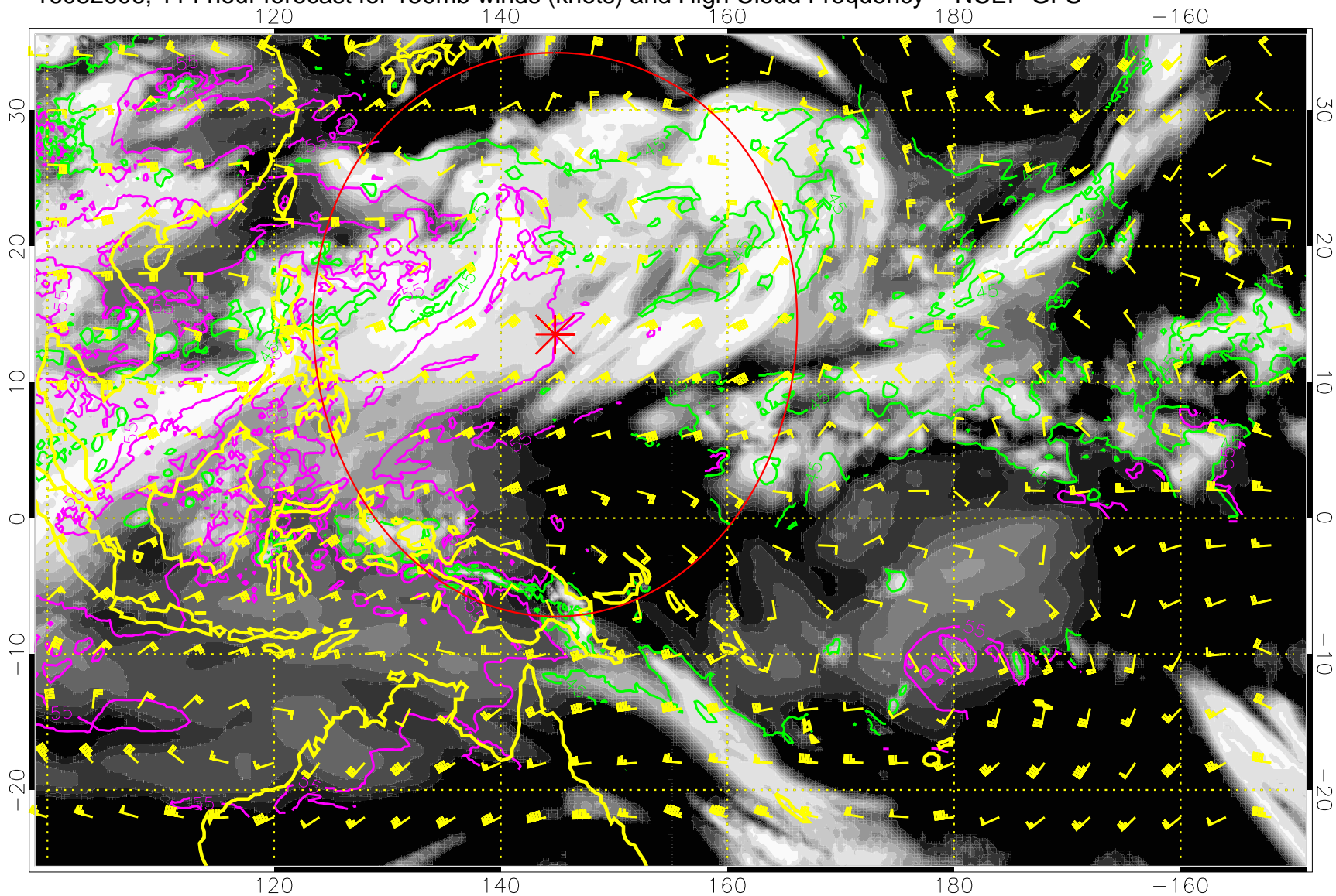
16082606, 114 hour forecast for 150mb winds (knots) and High Cloud Frequency -- NCEP GFS
