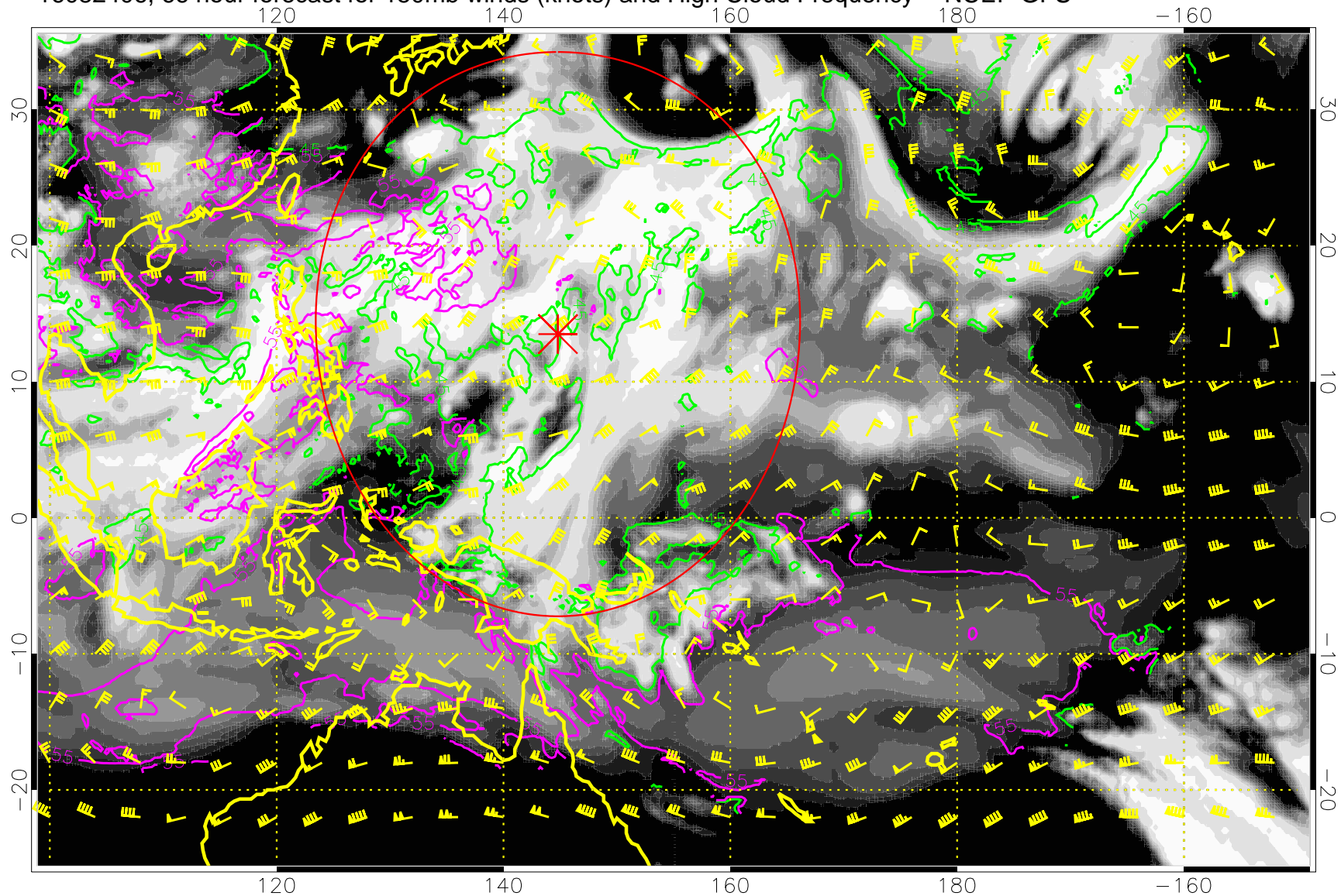
16082406, 66 hour forecast for 150mb winds (knots) and High Cloud Frequency -- NCEP GFS
