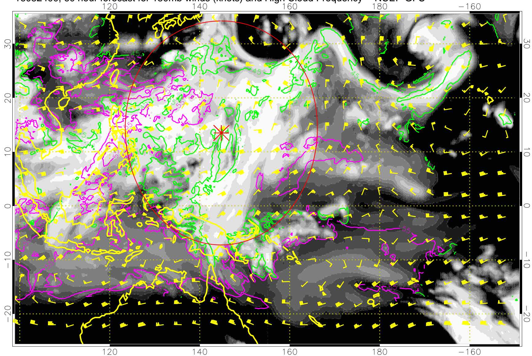
16082400, 60 hour forecast for 150mb winds (knots) and High Cloud Frequency -- NCEP GFS
