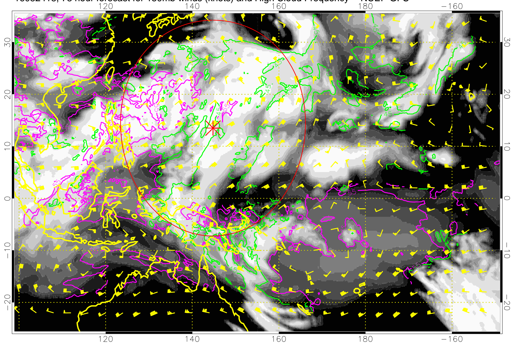
16082418, 78 hour forecast for 150mb winds (knots) and High Cloud Frequency -- NCEP GFS
