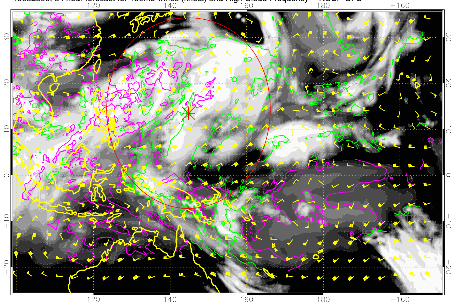
16082500, 84 hour forecast for 150mb winds (knots) and High Cloud Frequency -- NCEP GFS
