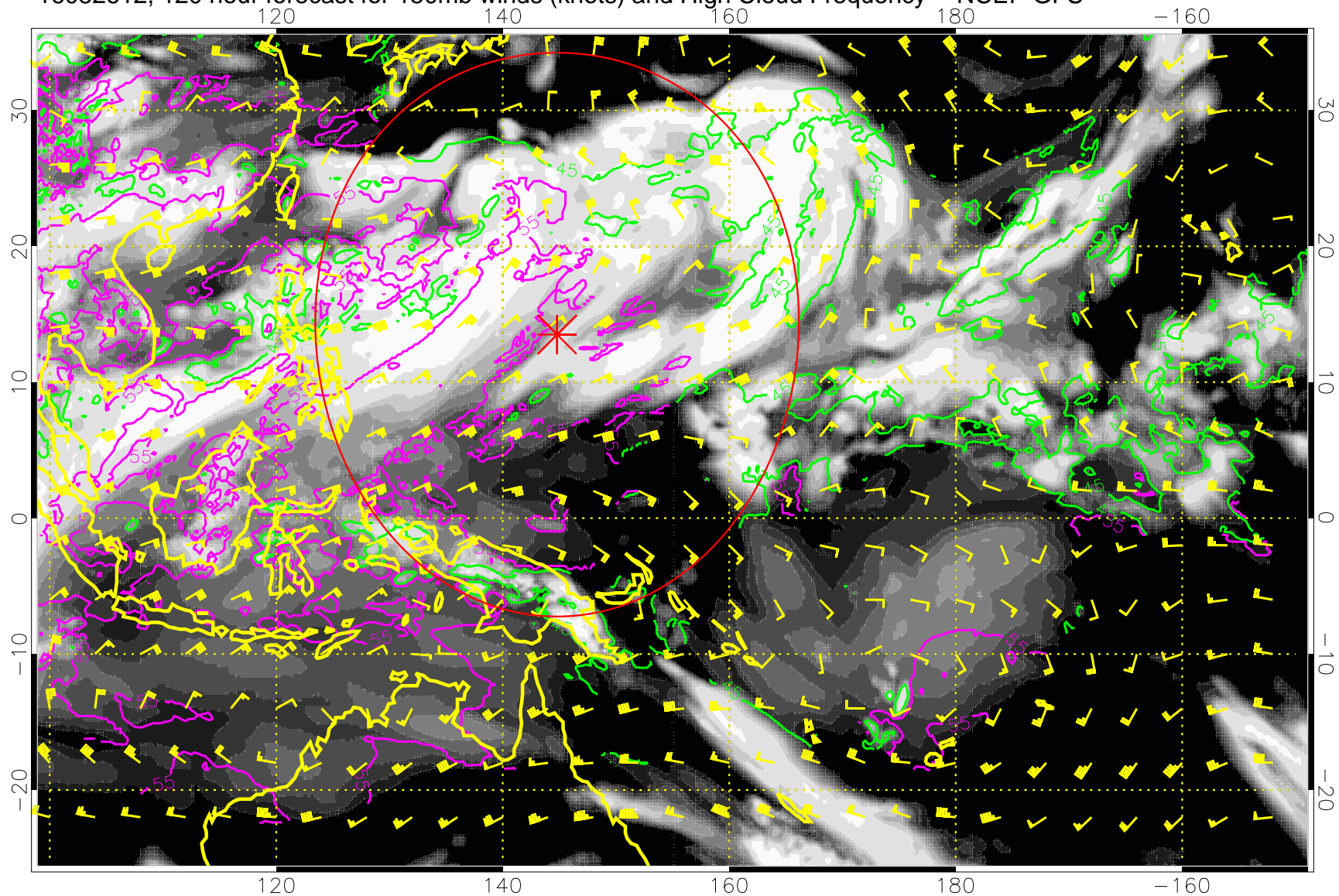
16082612, 120 hour forecast for 150mb winds (knots) and High Cloud Frequency -- NCEP GFS
