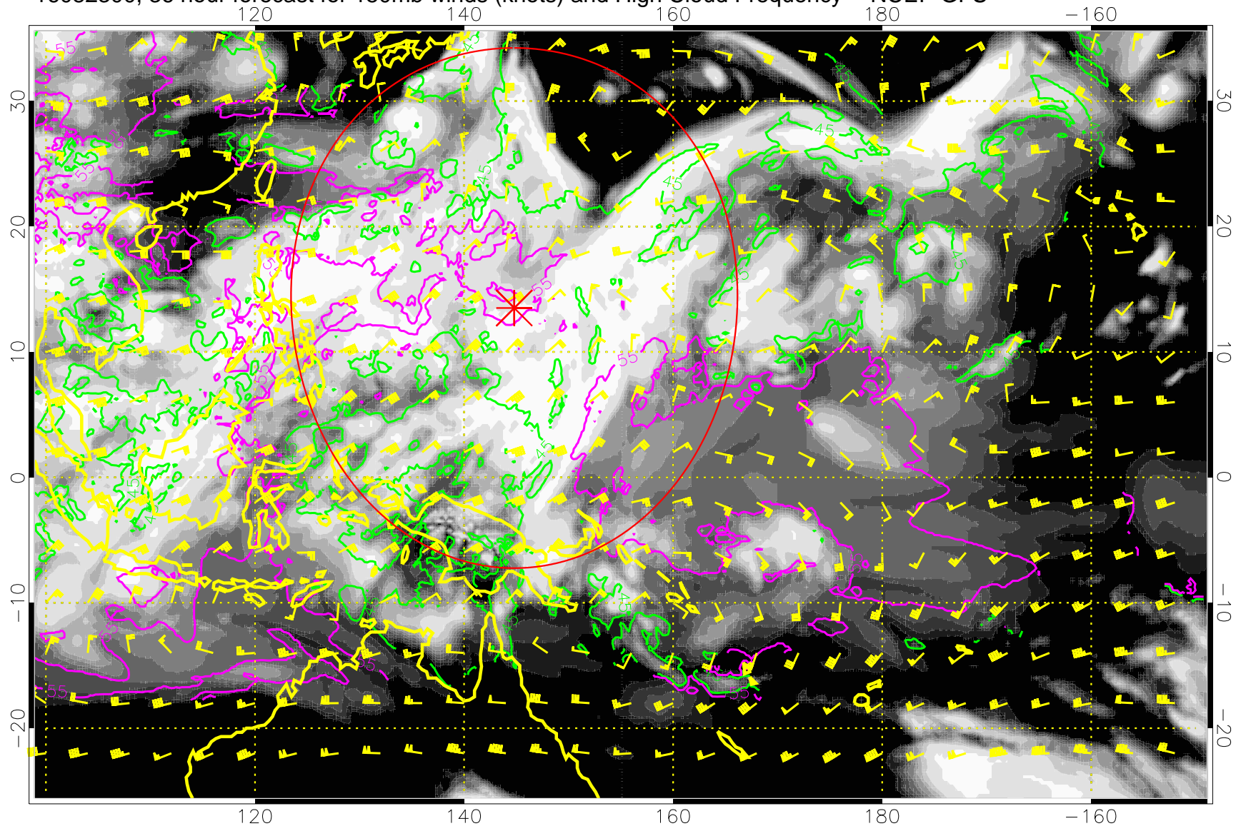
16082300, 36 hour forecast for 150mb winds (knots) and High Cloud Frequency -- NCEP GFS
