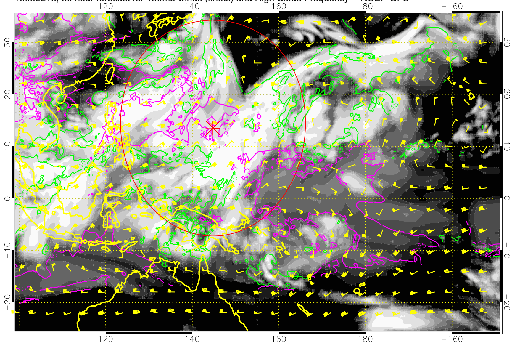
16082218, 30 hour forecast for 150mb winds (knots) and High Cloud Frequency -- NCEP GFS
