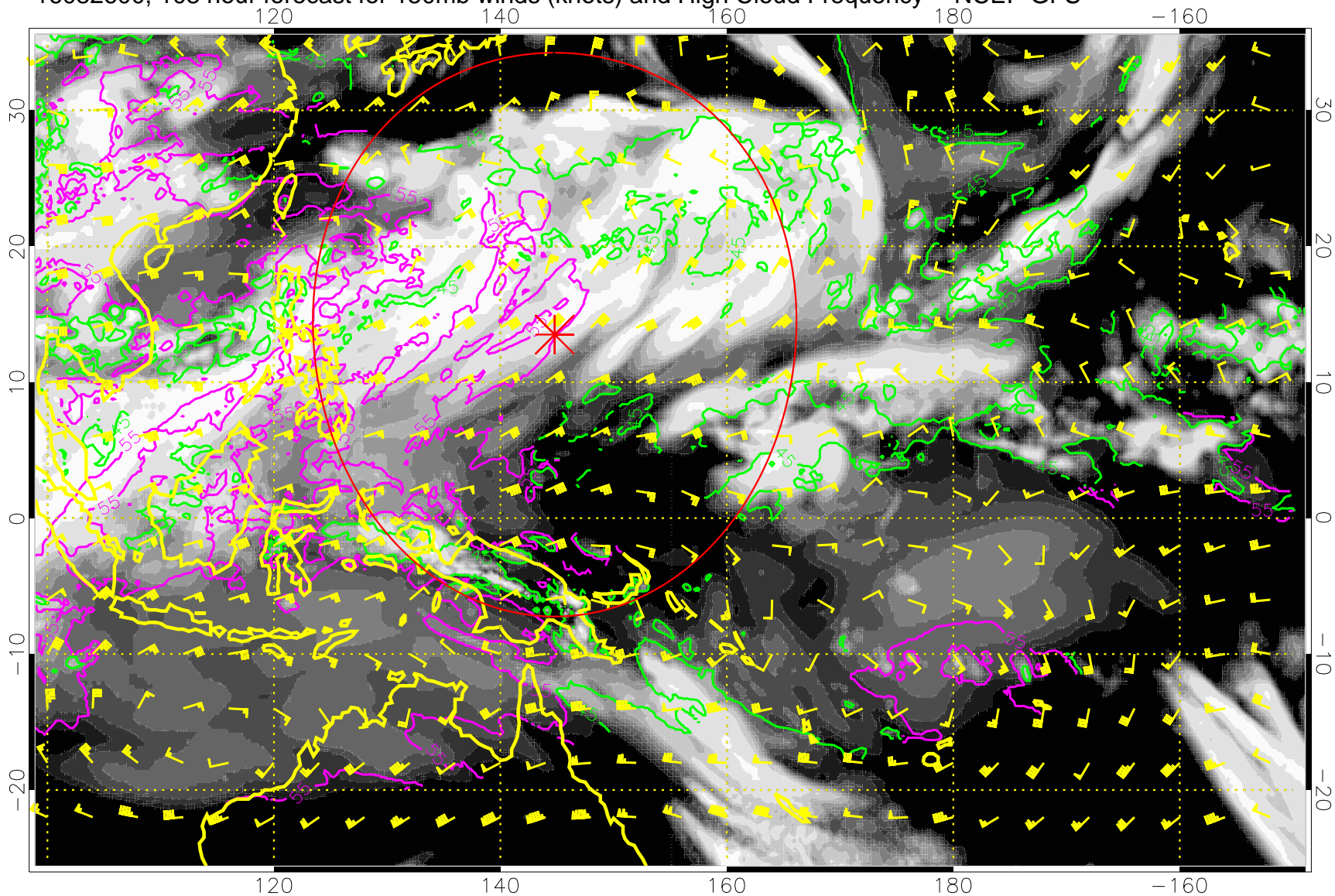
16082600, 108 hour forecast for 150mb winds (knots) and High Cloud Frequency -- NCEP GFS
