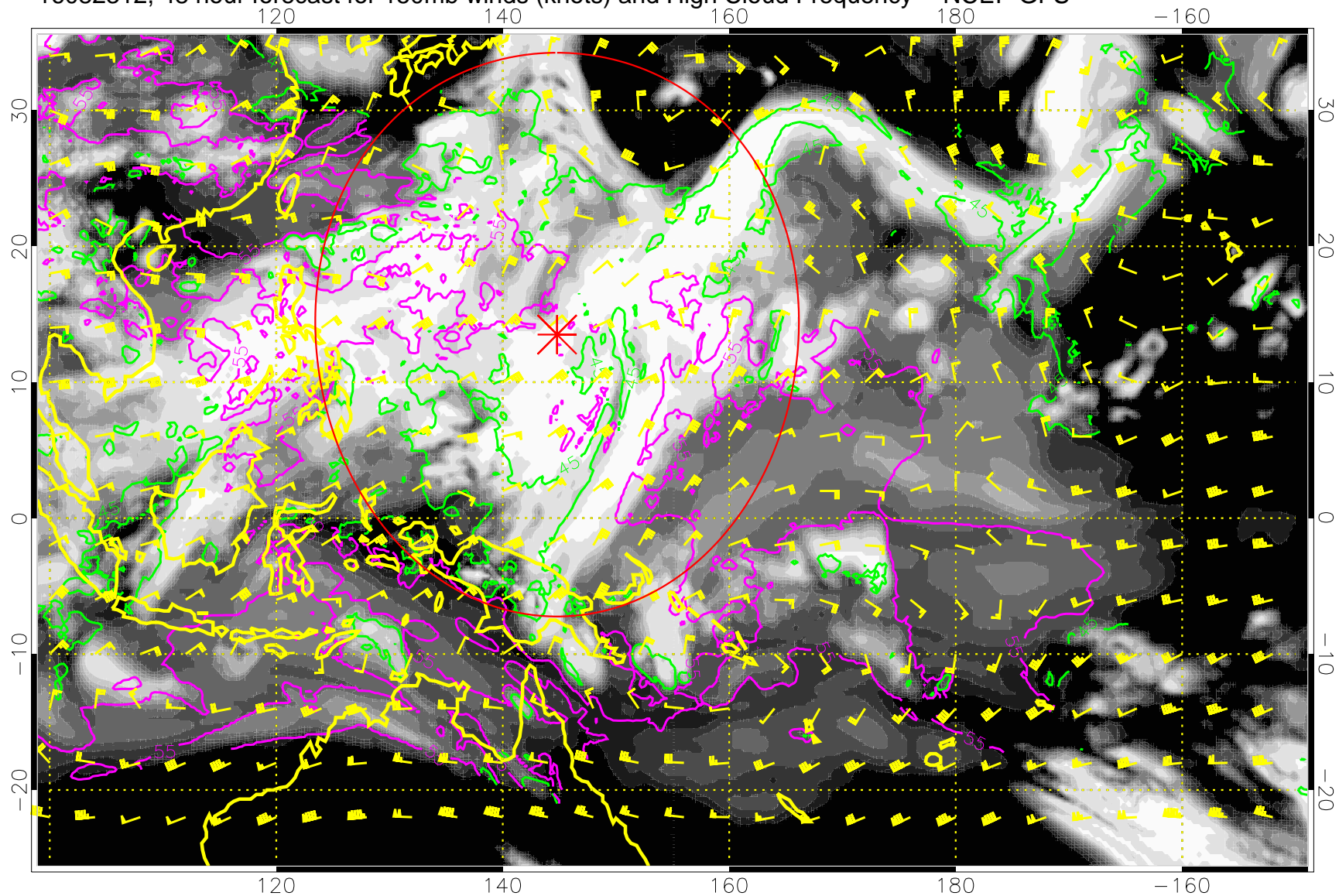
16082312, 48 hour forecast for 150mb winds (knots) and High Cloud Frequency -- NCEP GFS
