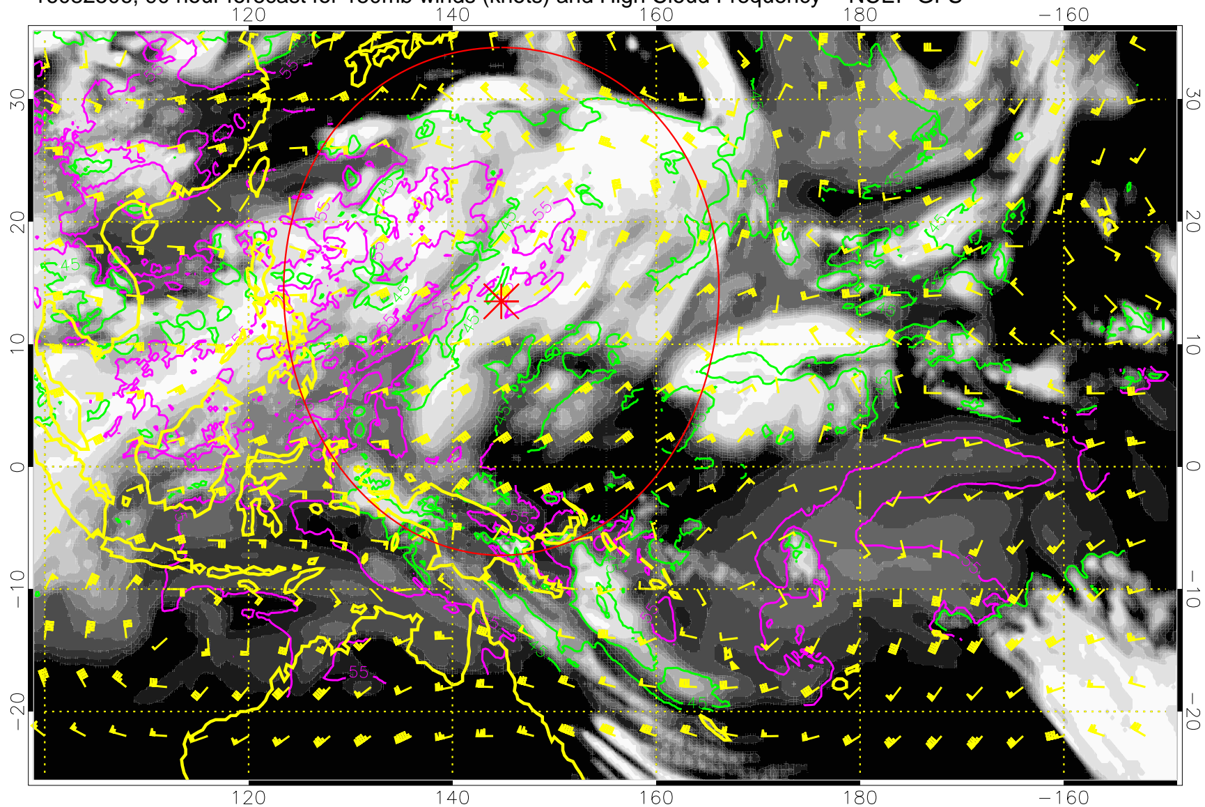
16082506, 90 hour forecast for 150mb winds (knots) and High Cloud Frequency -- NCEP GFS
