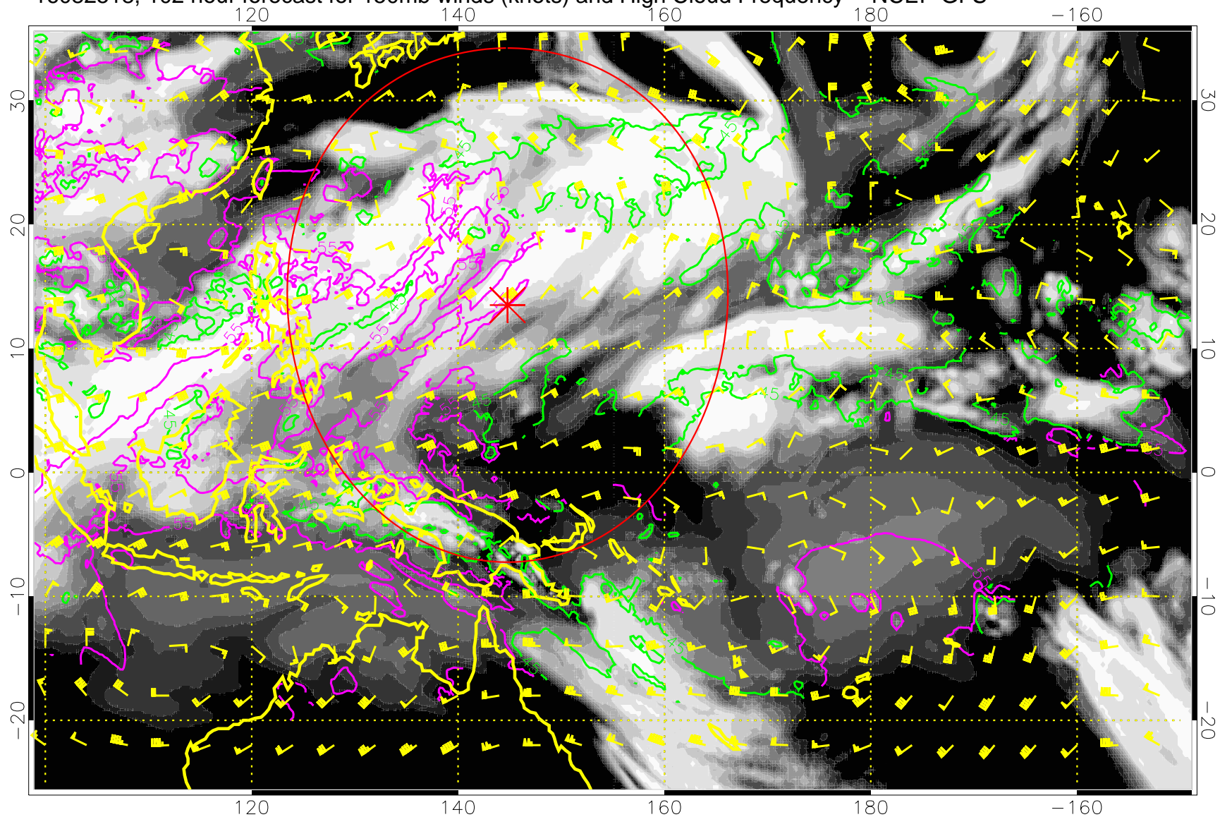
16082518, 102 hour forecast for 150mb winds (knots) and High Cloud Frequency -- NCEP GFS
