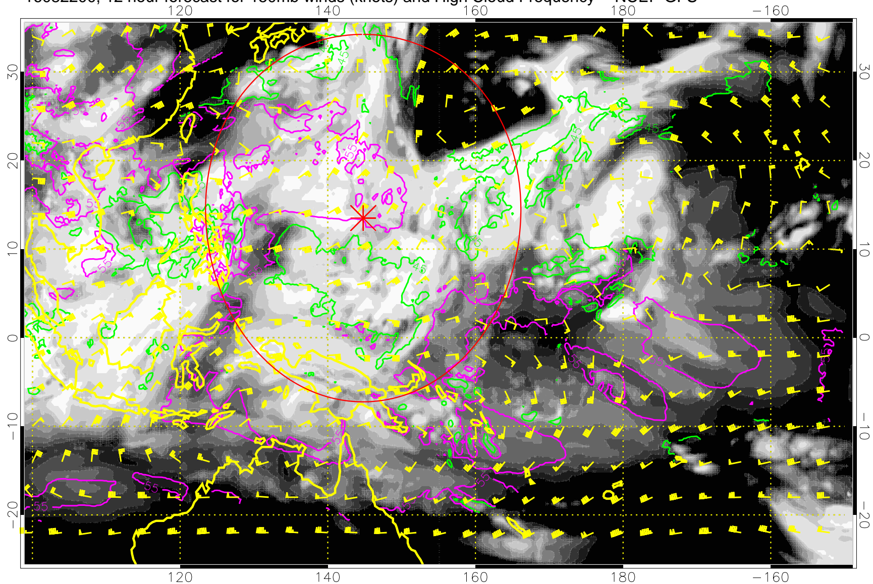
16082200, 12 hour forecast for 150mb winds (knots) and High Cloud Frequency -- NCEP GFS
