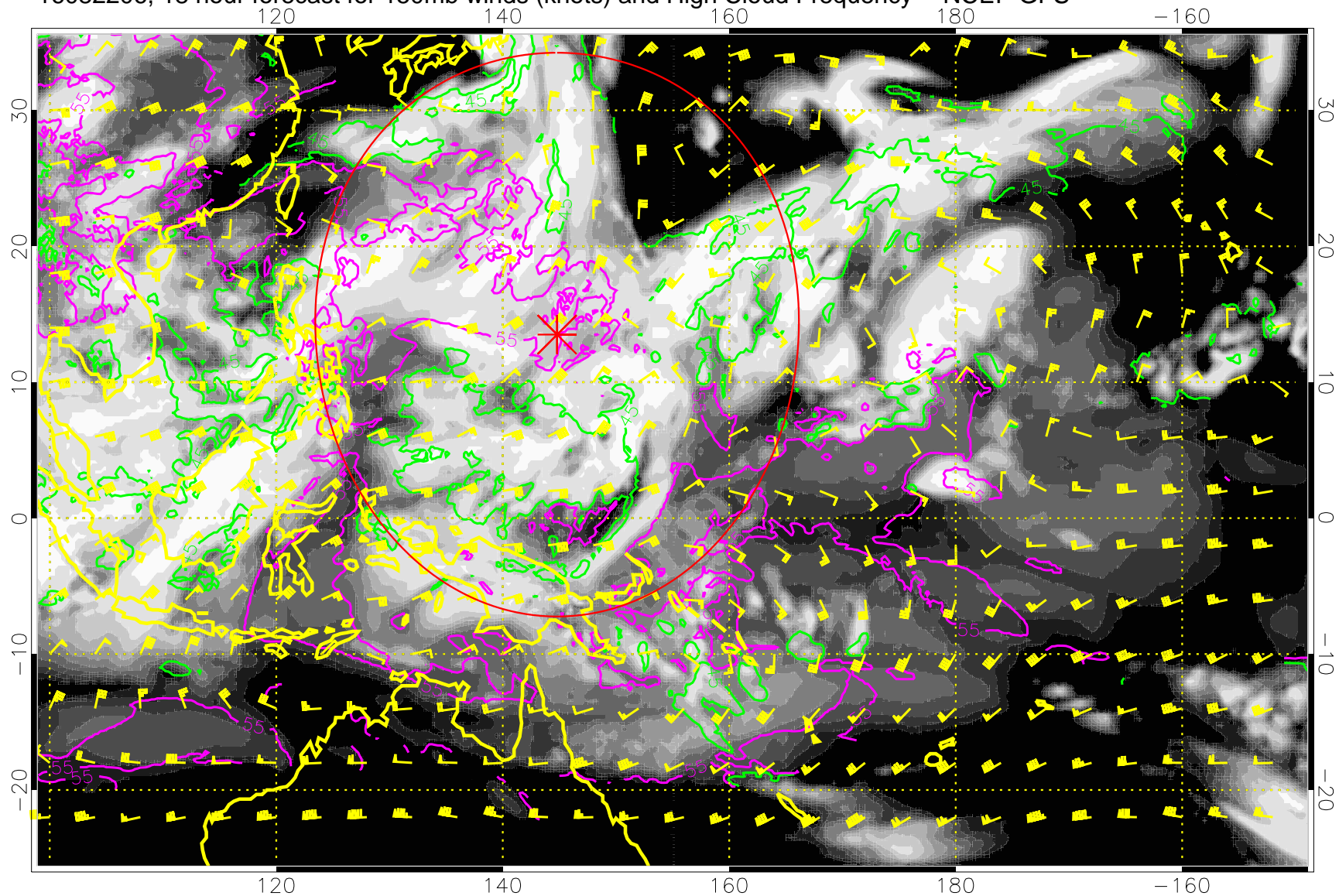
16082206, 18 hour forecast for 150mb winds (knots) and High Cloud Frequency -- NCEP GFS
