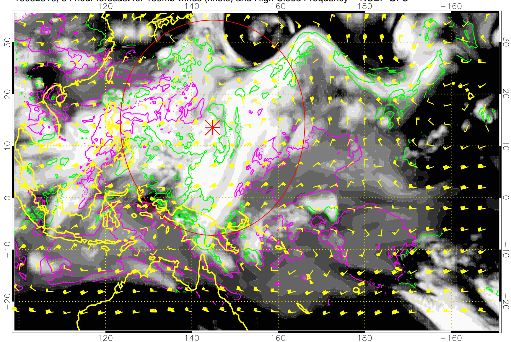
16082318, 54 hour forecast for 150mb winds (knots) and High Cloud Frequency -- NCEP GFS
