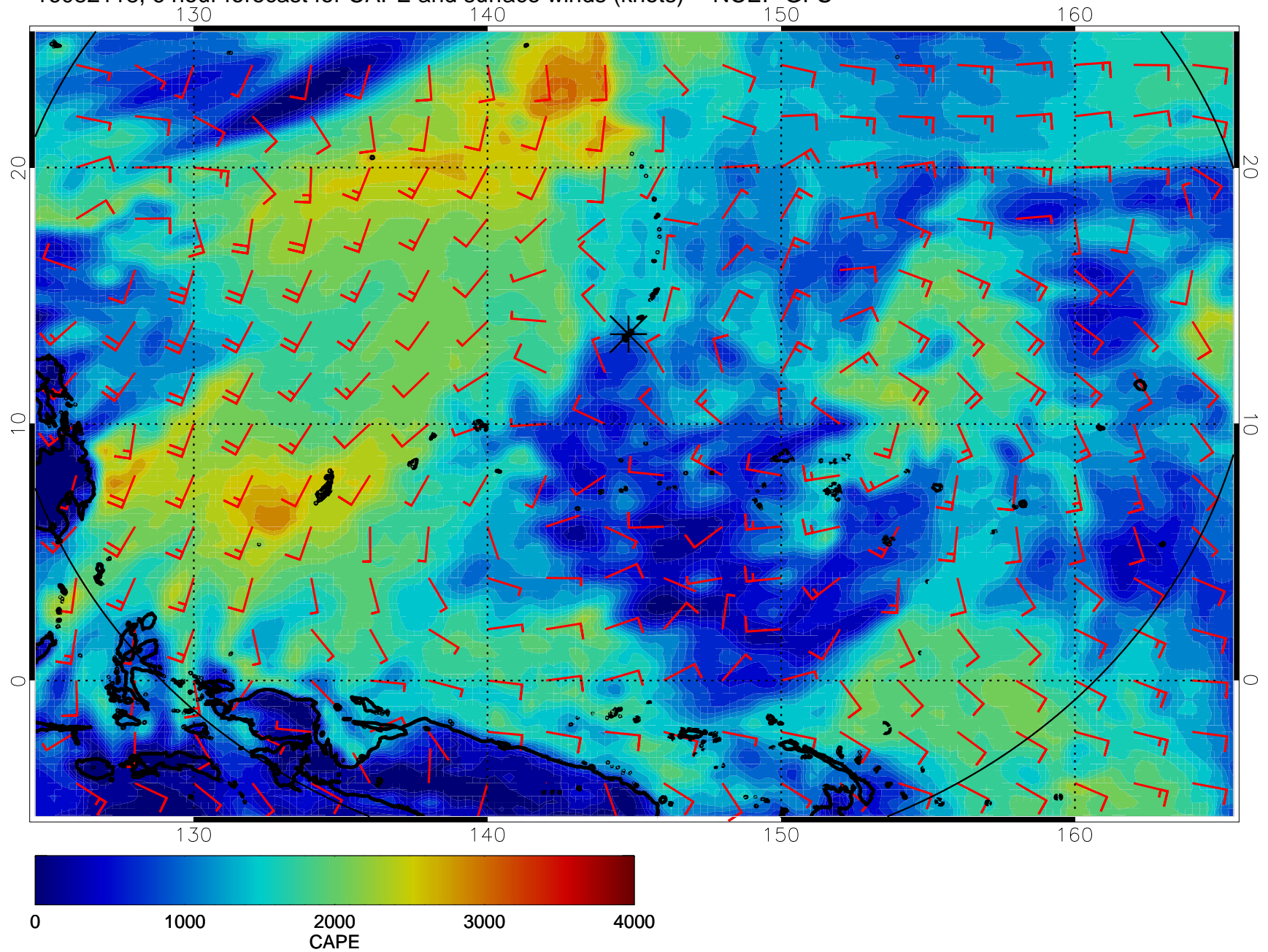
16082118, 6 hour forecast for CAPE and surface winds (knots) -- NCEP GFS
