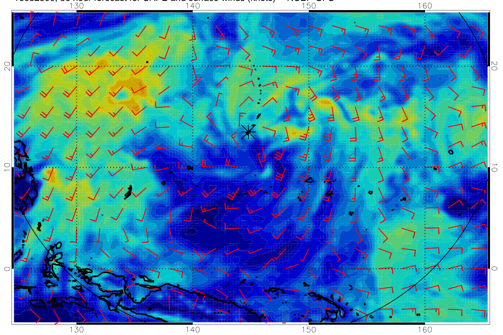
16082300, 36 hour forecast for CAPE and surface winds (knots) -- NCEP GFS
