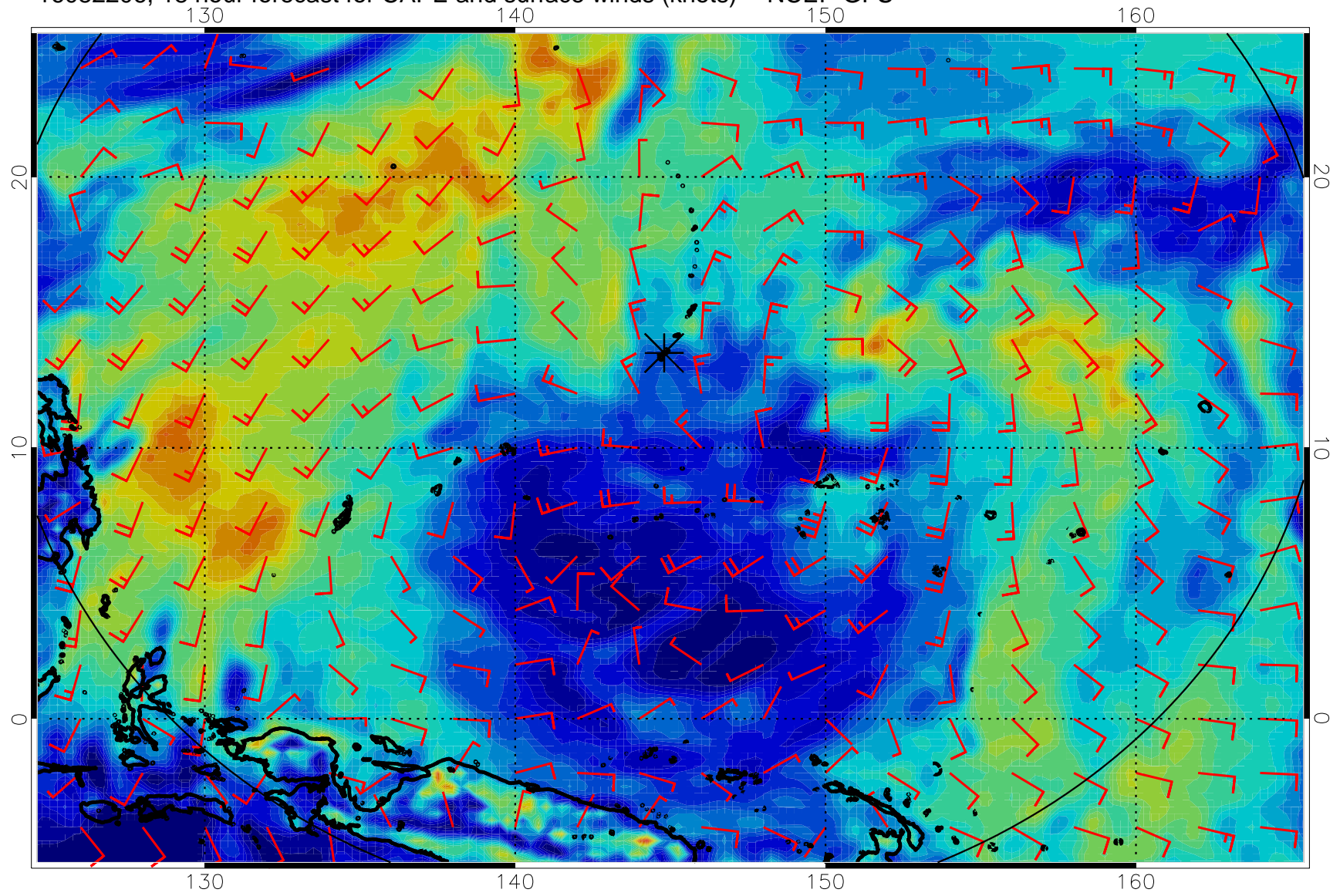
16082206, 18 hour forecast for CAPE and surface winds (knots) -- NCEP GFS
