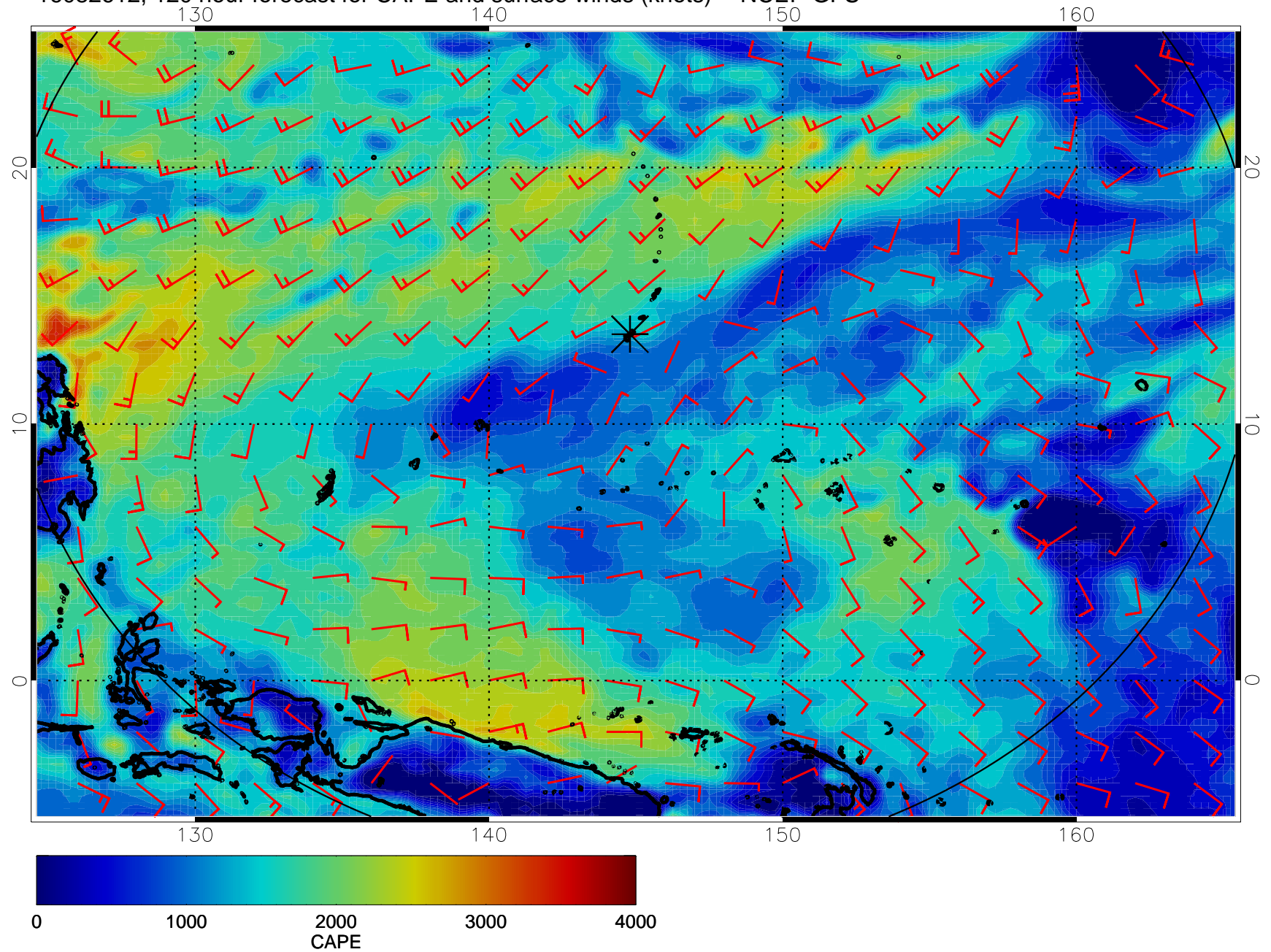
16082612, 120 hour forecast for CAPE and surface winds (knots) -- NCEP GFS
