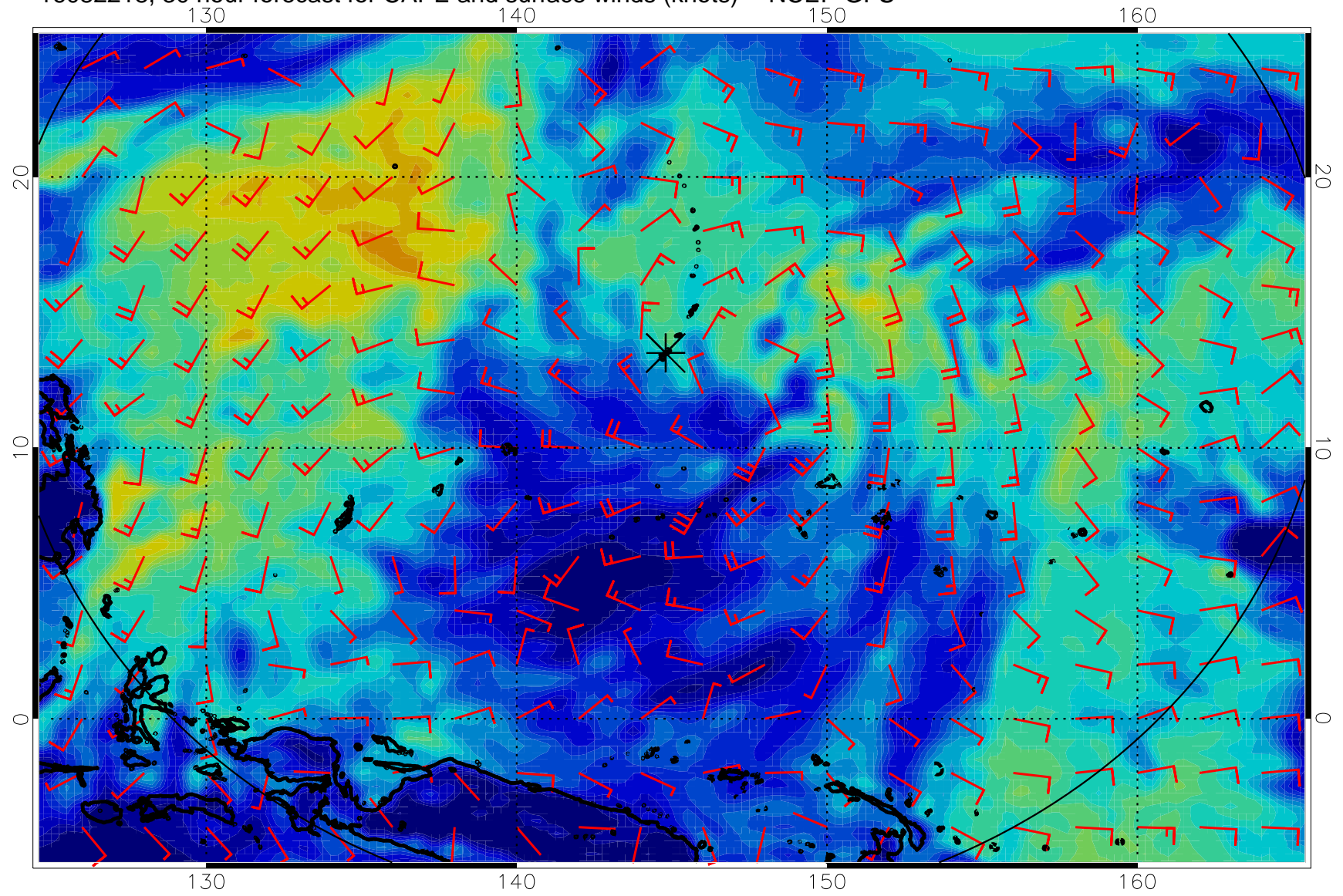
16082218, 30 hour forecast for CAPE and surface winds (knots) -- NCEP GFS
