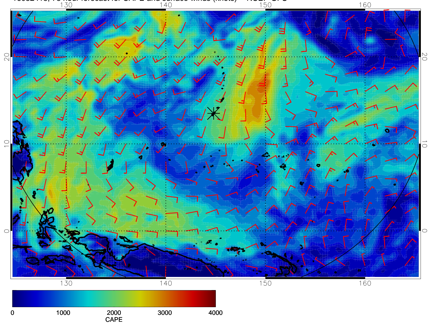
16082418, 78 hour forecast for CAPE and surface winds (knots) -- NCEP GFS
