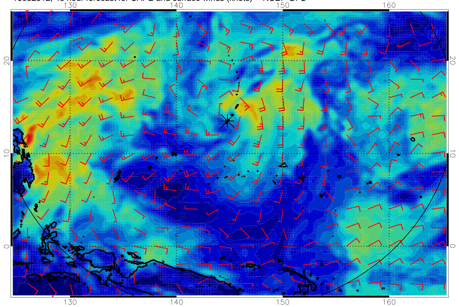
16082312, 48 hour forecast for CAPE and surface winds (knots) -- NCEP GFS
