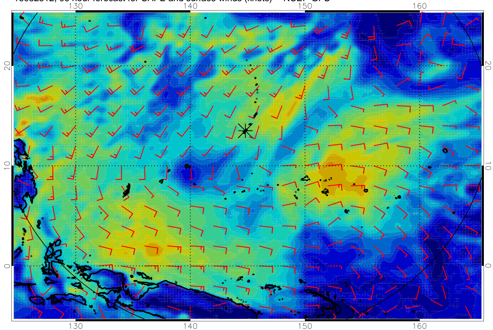
16082512, 96 hour forecast for CAPE and surface winds (knots) -- NCEP GFS
