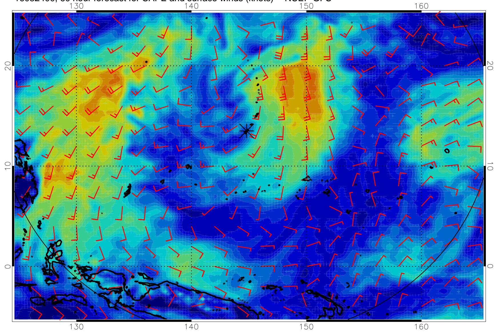
16082400, 60 hour forecast for CAPE and surface winds (knots) -- NCEP GFS
