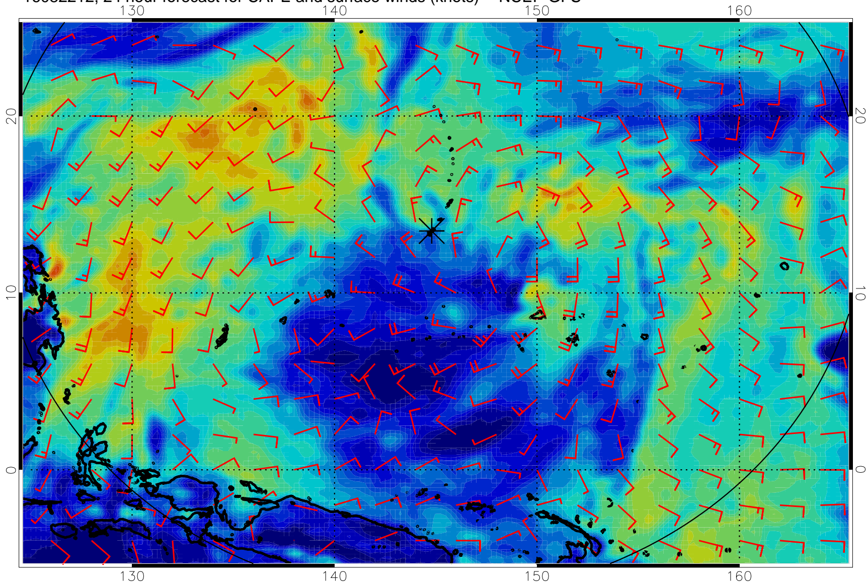
16082212, 24 hour forecast for CAPE and surface winds (knots) -- NCEP GFS
