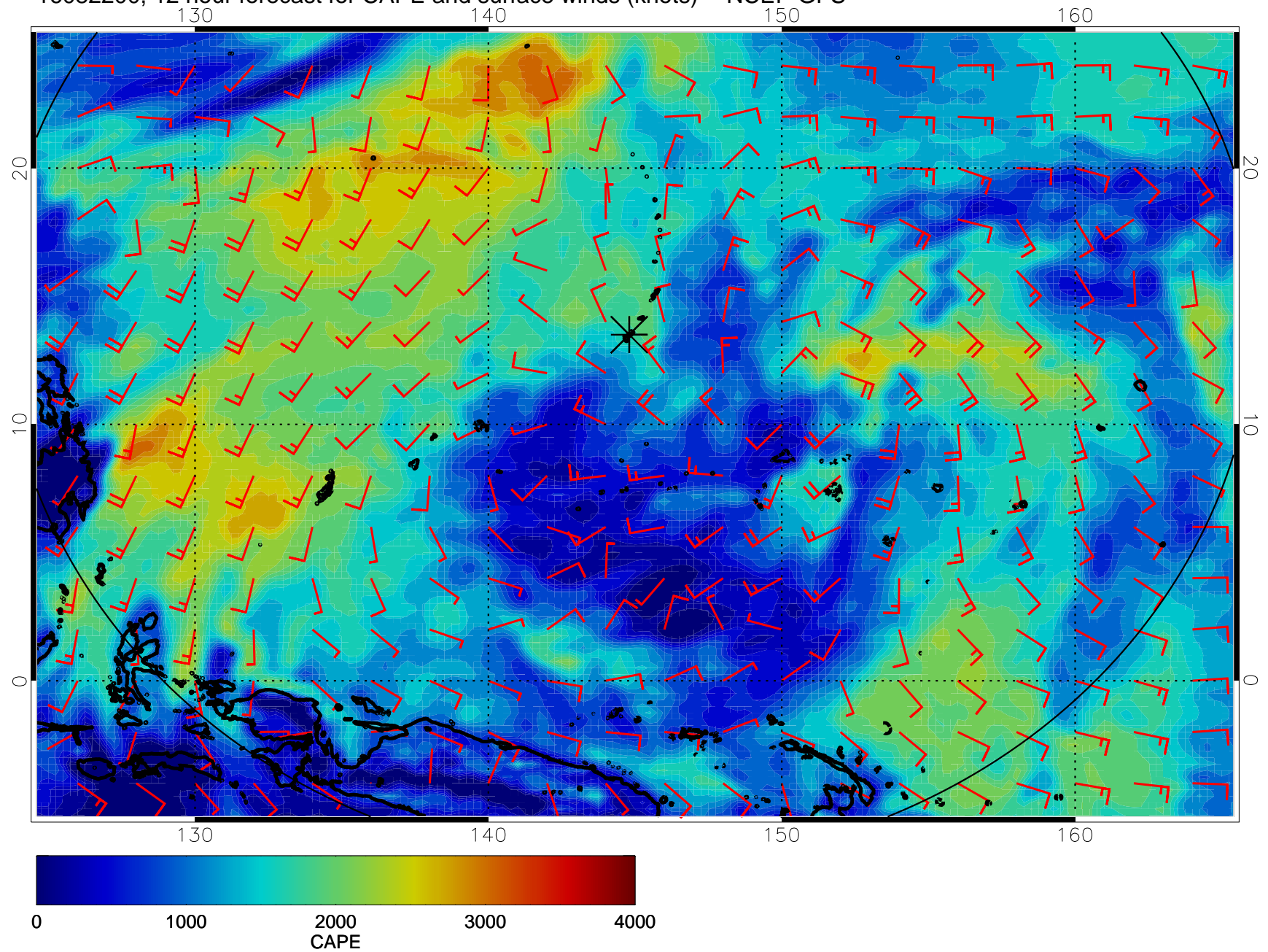
16082200, 12 hour forecast for CAPE and surface winds (knots) -- NCEP GFS
