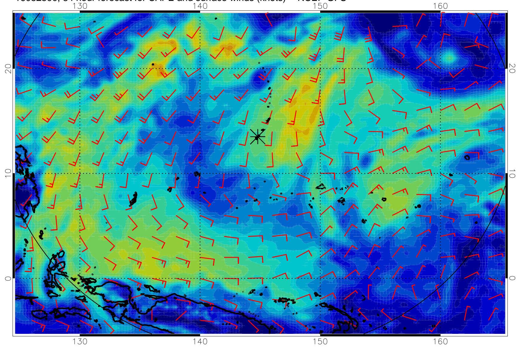
16082500, 84 hour forecast for CAPE and surface winds (knots) -- NCEP GFS
