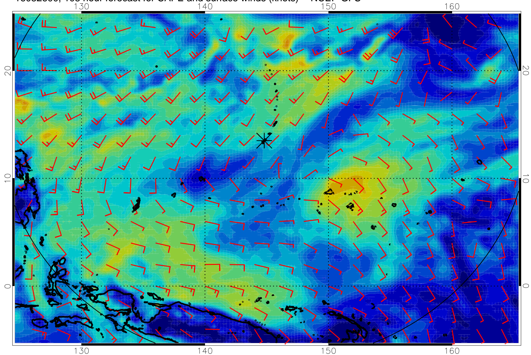
16082600, 108 hour forecast for CAPE and surface winds (knots) -- NCEP GFS
