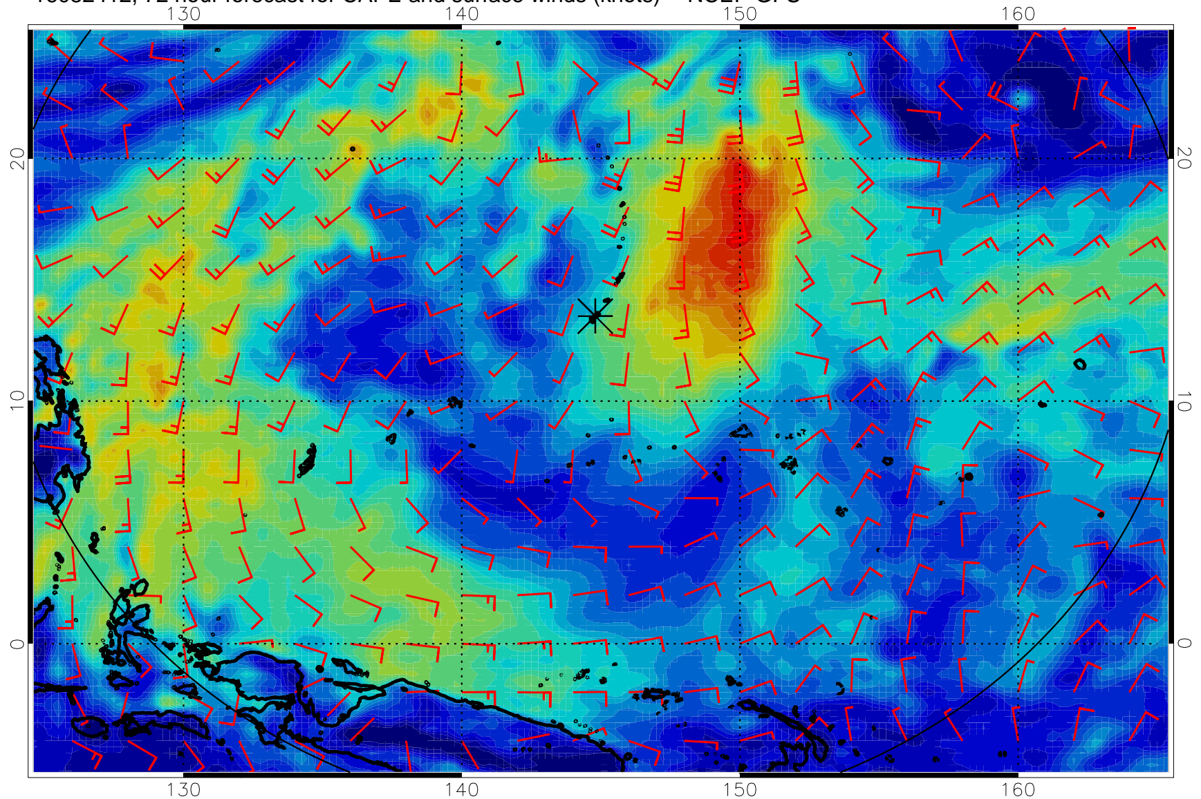
16082412, 72 hour forecast for CAPE and surface winds (knots) -- NCEP GFS
