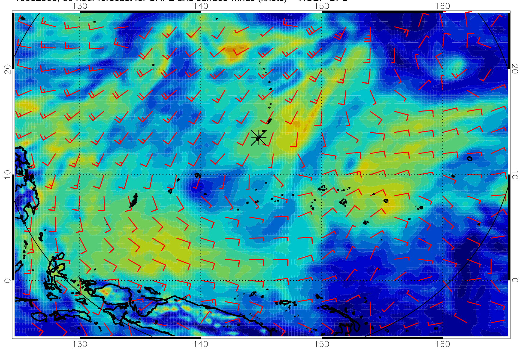
16082506, 90 hour forecast for CAPE and surface winds (knots) -- NCEP GFS
