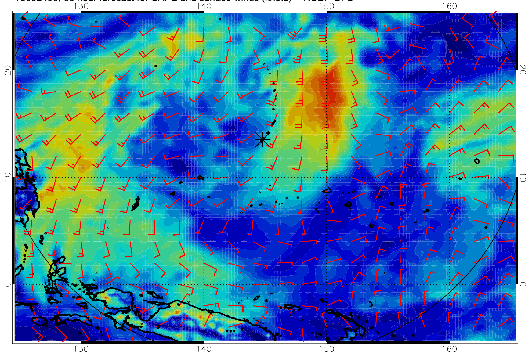
16082406, 66 hour forecast for CAPE and surface winds (knots) -- NCEP GFS
