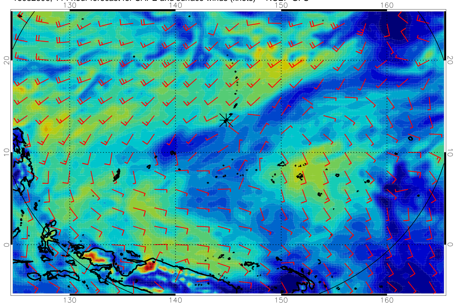
16082606, 114 hour forecast for CAPE and surface winds (knots) -- NCEP GFS
