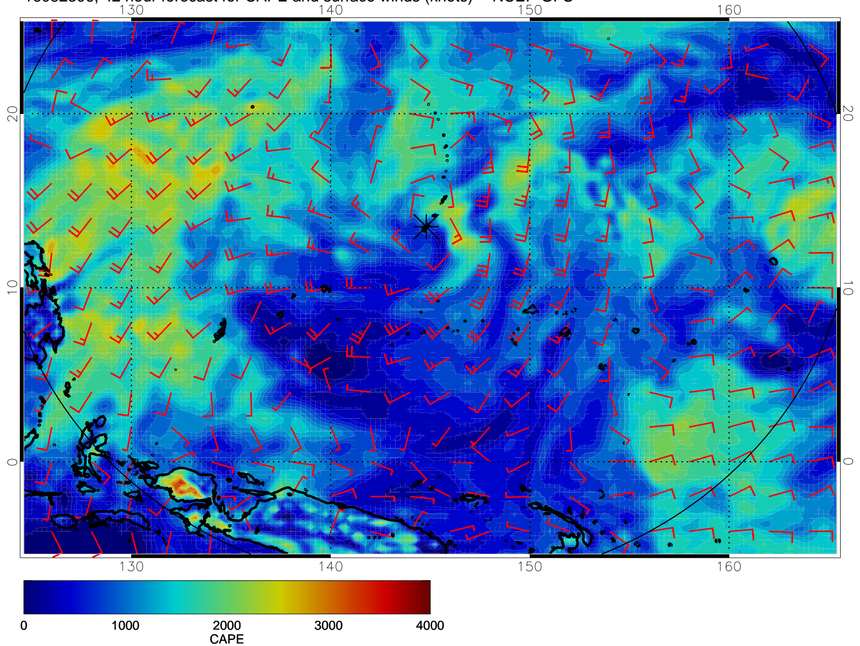
16082306, 42 hour forecast for CAPE and surface winds (knots) -- NCEP GFS
