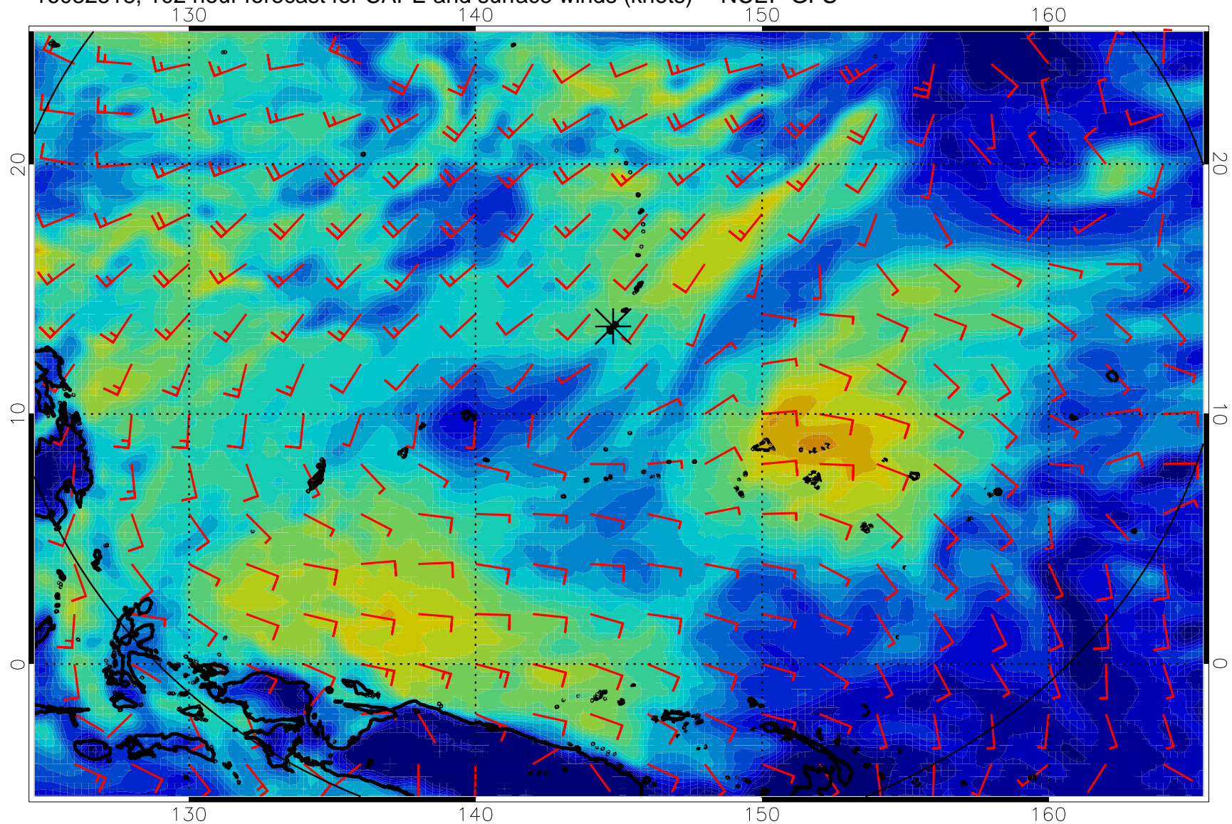
16082518, 102 hour forecast for CAPE and surface winds (knots) -- NCEP GFS
