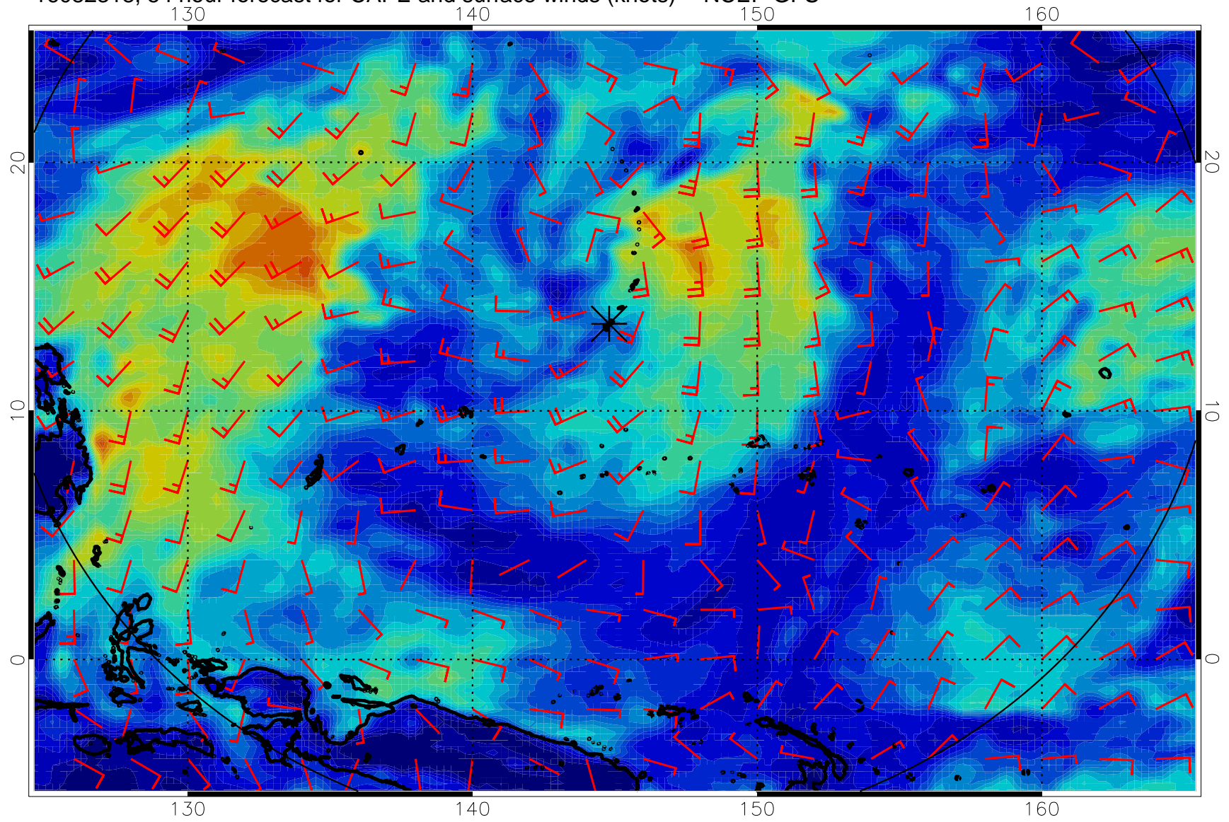
16082318, 54 hour forecast for CAPE and surface winds (knots) -- NCEP GFS
