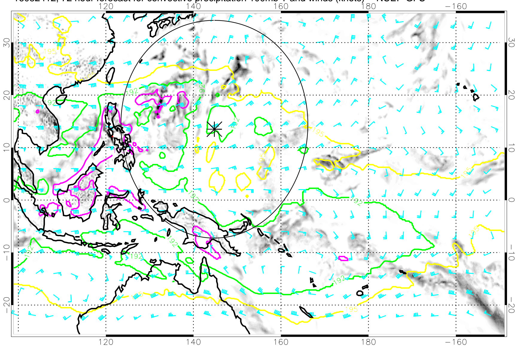
16082412, 72 hour forecast for convective precipitation 100mb T and winds (knots) -- NCEP GFS
