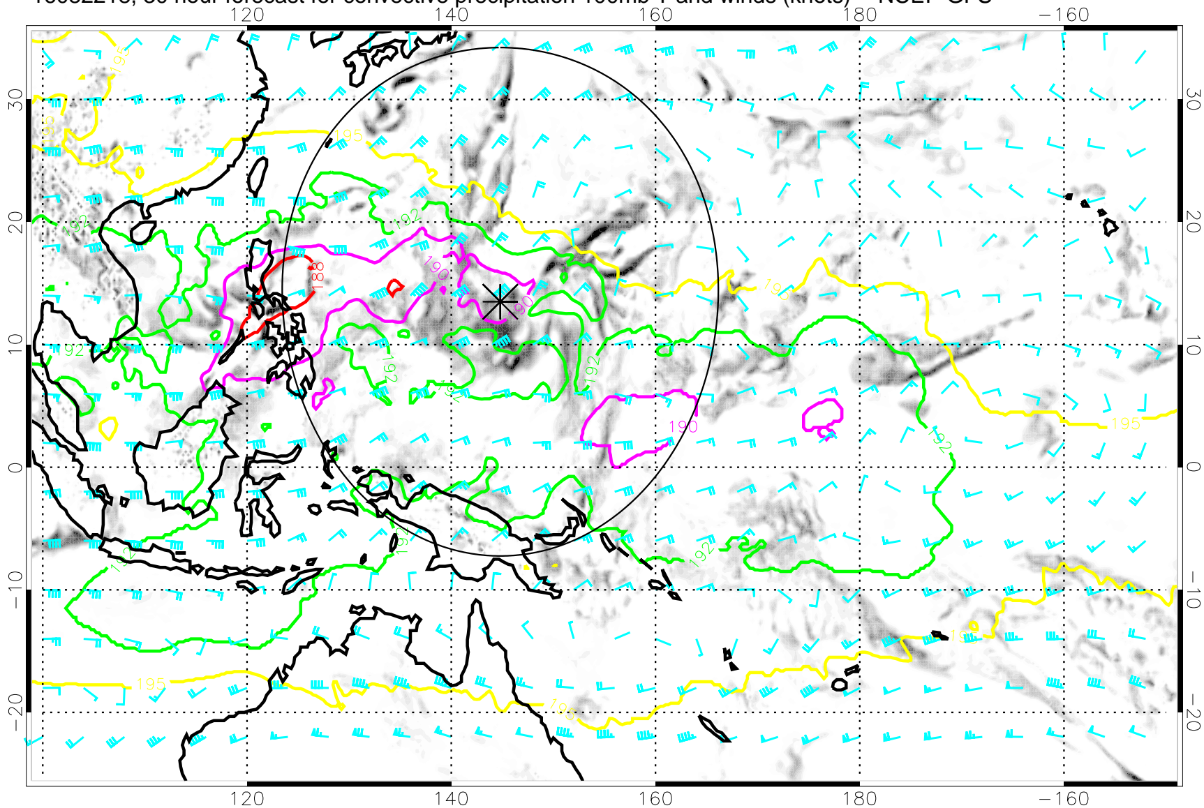
16082218, 30 hour forecast for convective precipitation 100mb T and winds (knots) -- NCEP GFS
