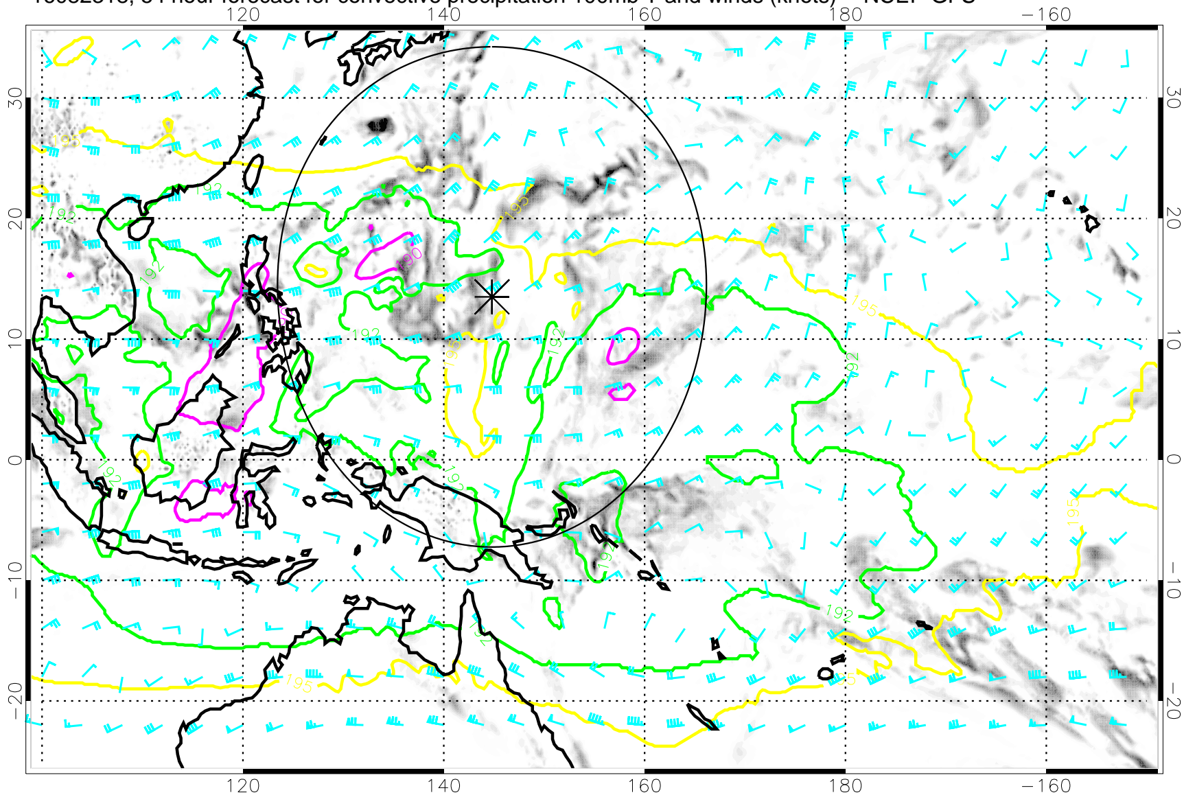
16082318, 54 hour forecast for convective precipitation 100mb T and winds (knots) -- NCEP GFS
