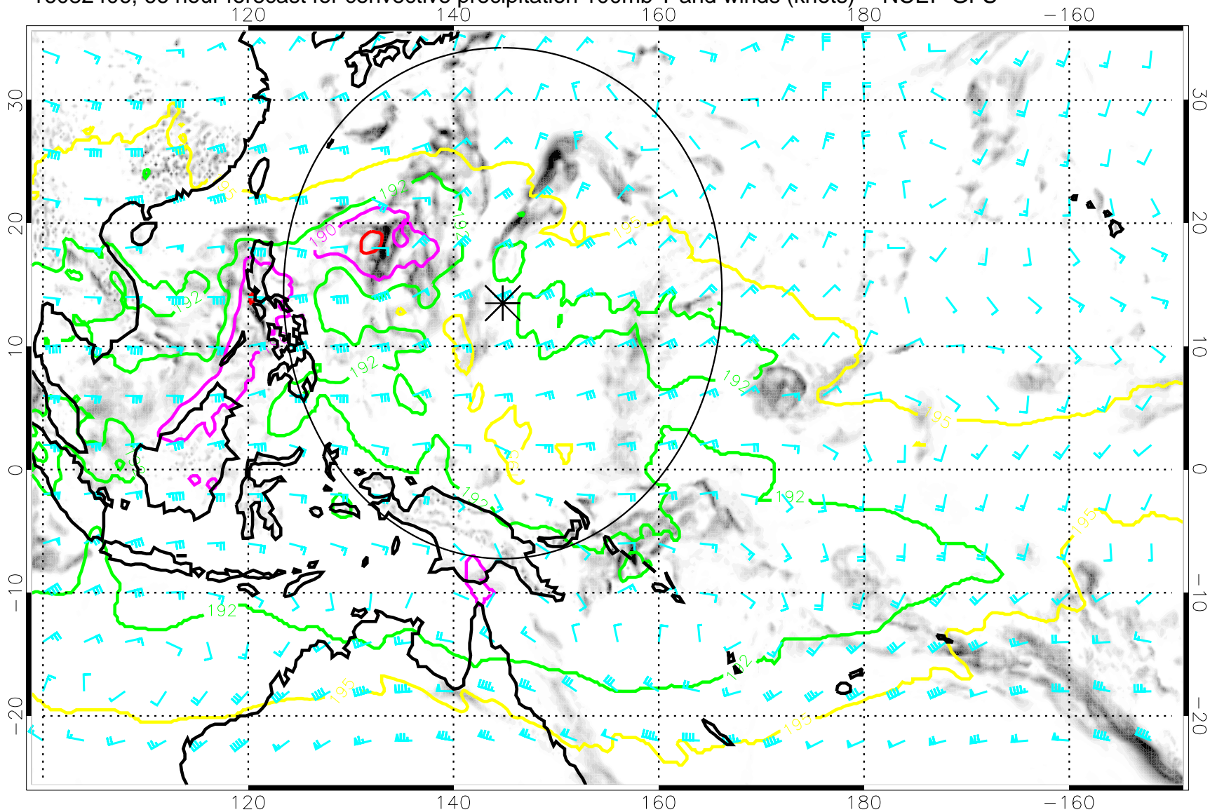
16082406, 66 hour forecast for convective precipitation 100mb T and winds (knots) -- NCEP GFS
