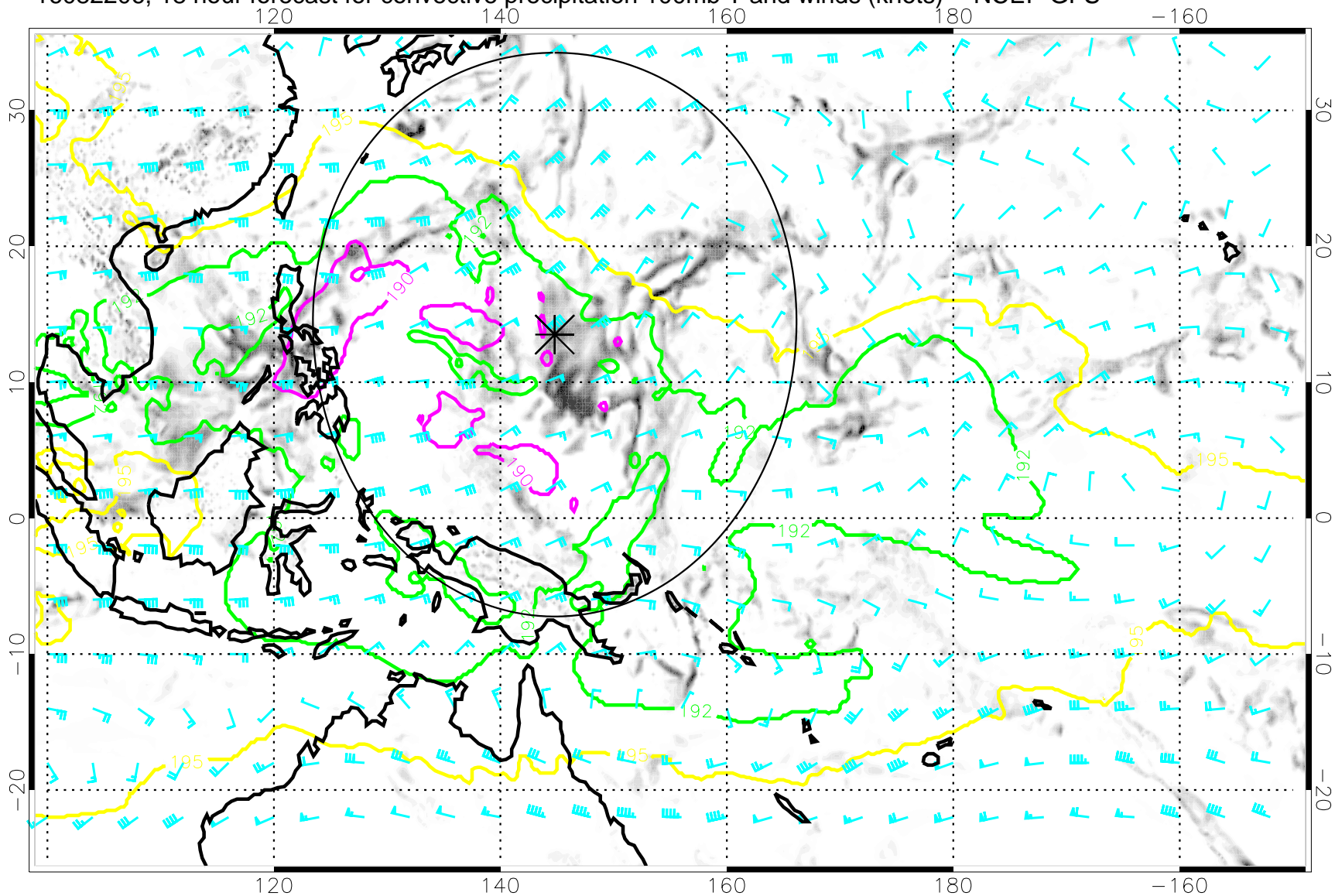
16082206, 18 hour forecast for convective precipitation 100mb T and winds (knots) -- NCEP GFS
