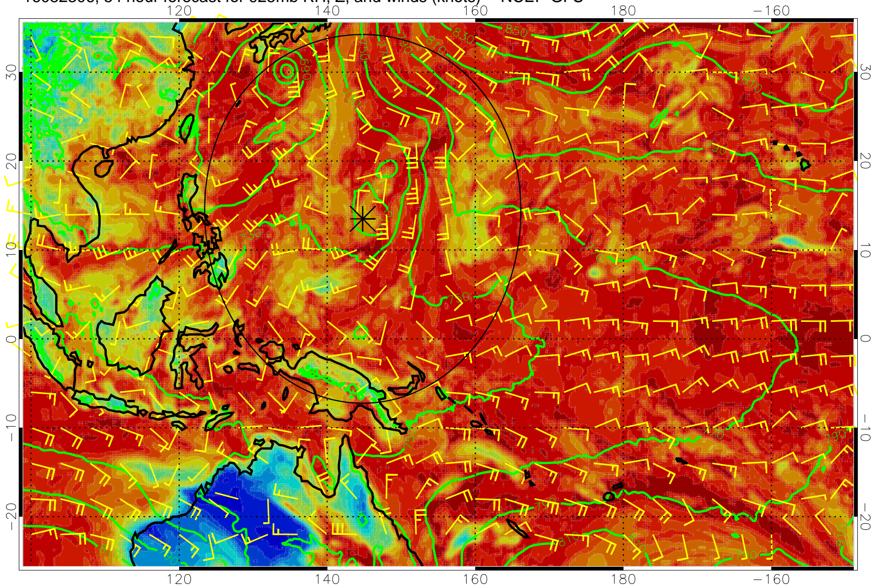
16082306, 54 hour forecast for 925mb RH, Z, and winds (knots) -- NCEP GFS
