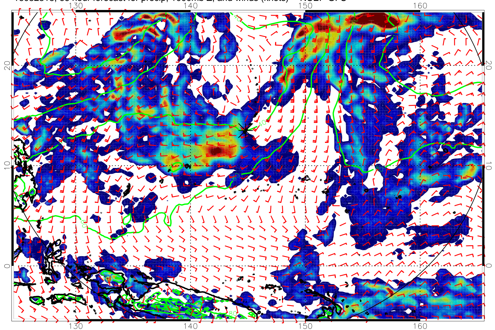
16082318, 66 hour forecast for precip, 1000mb Z, and winds (knots) -- NCEP GFS
