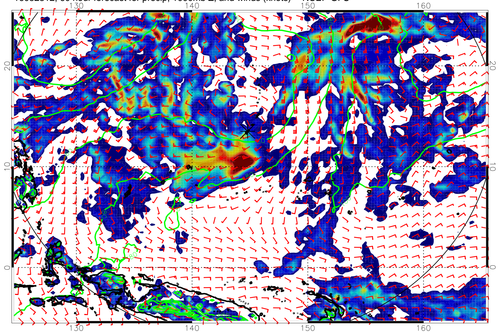
16082312, 60 hour forecast for precip, 1000mb Z, and winds (knots) -- NCEP GFS
