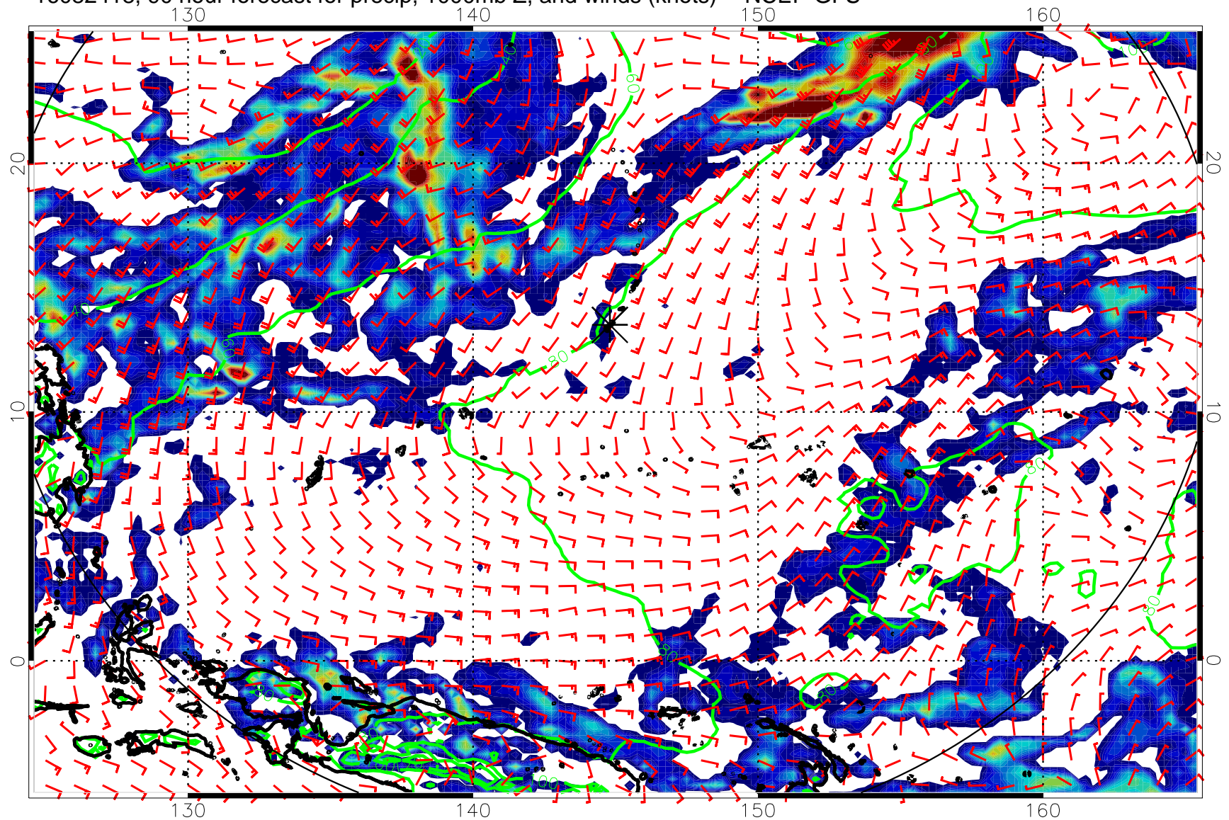
16082418, 90 hour forecast for precip, 1000mb Z, and winds (knots) -- NCEP GFS
