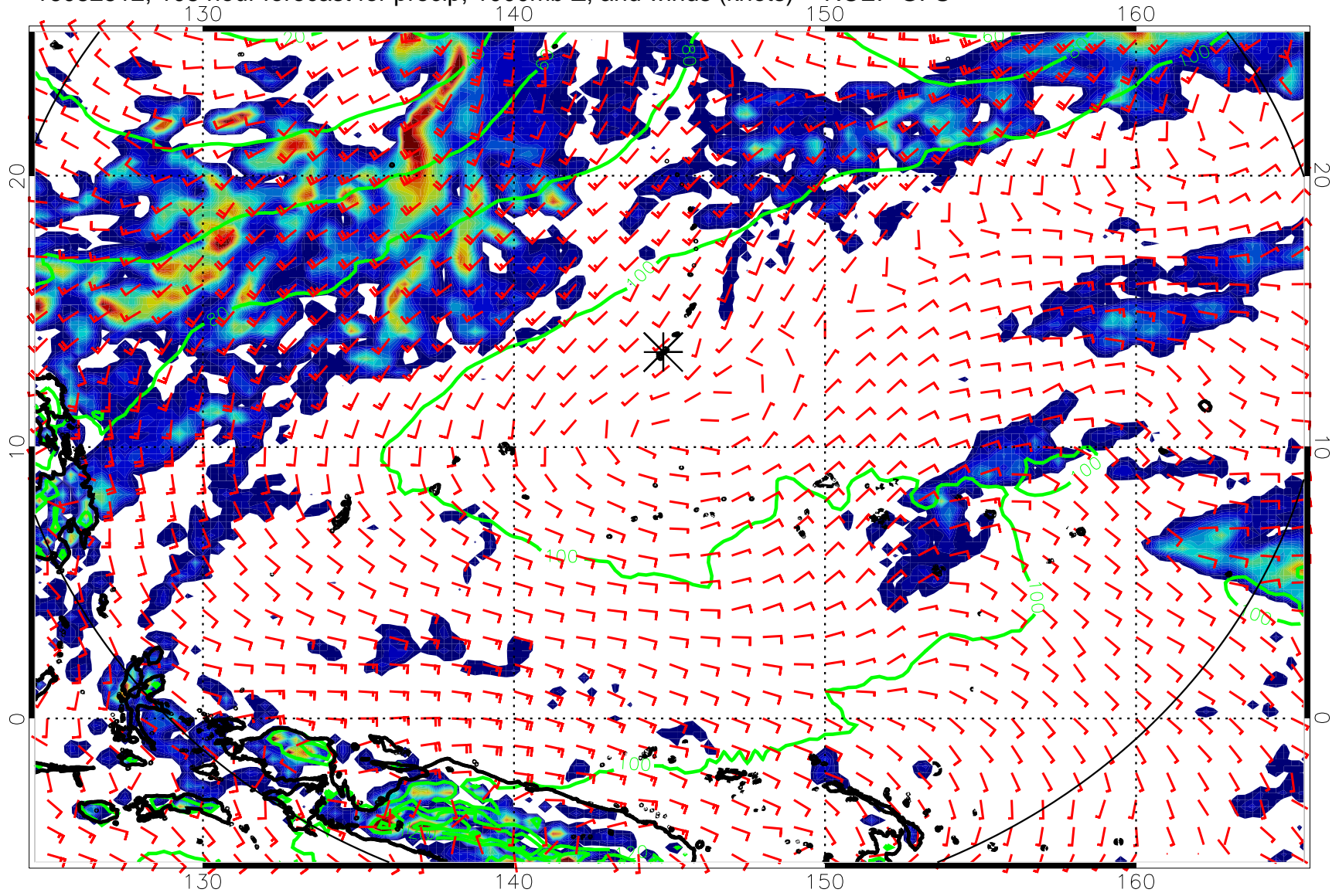
16082512, 108 hour forecast for precip, 1000mb Z, and winds (knots) -- NCEP GFS
