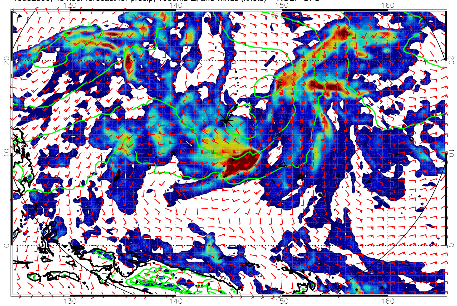
16082300, 48 hour forecast for precip, 1000mb Z, and winds (knots) -- NCEP GFS
