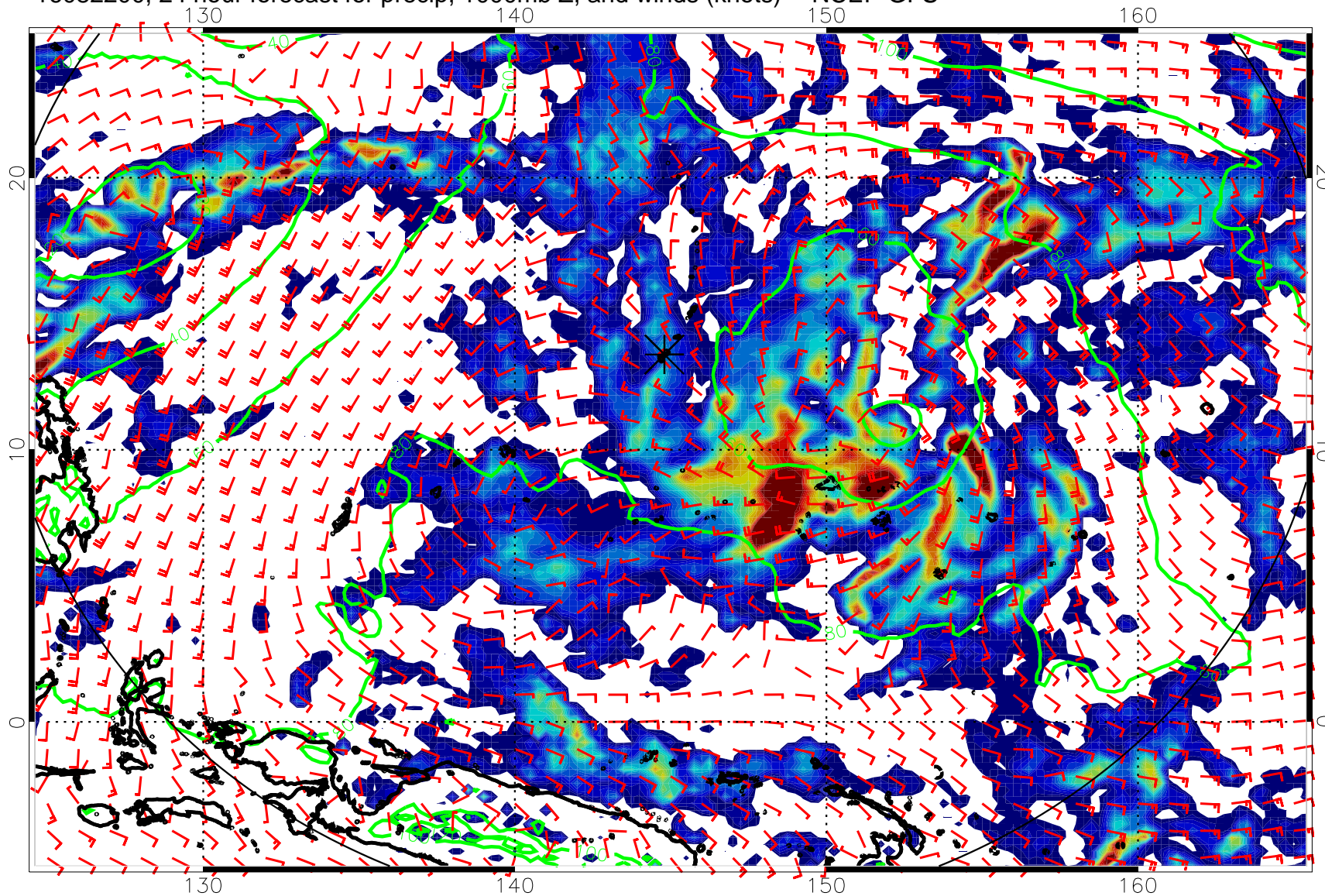
16082200, 24 hour forecast for precip, 1000mb Z, and winds (knots) -- NCEP GFS
