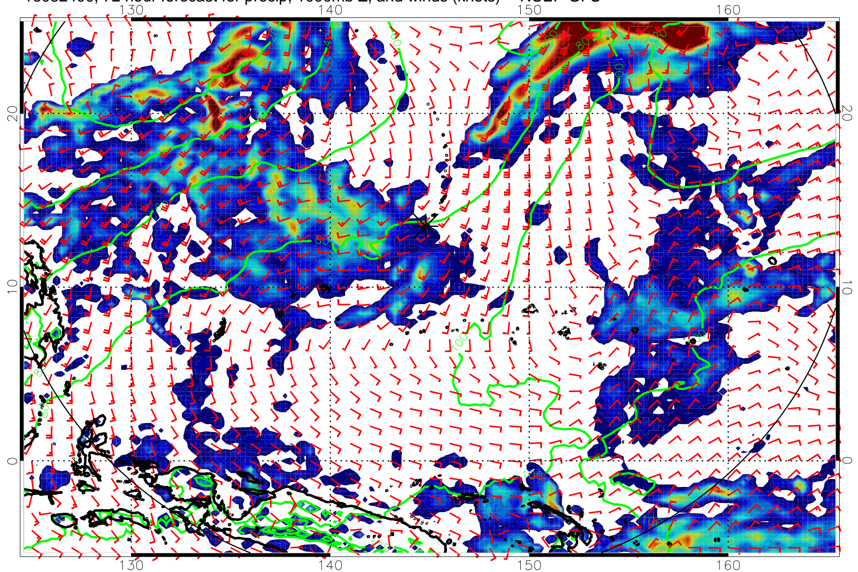
16082400, 72 hour forecast for precip, 1000mb Z, and winds (knots) -- NCEP GFS
