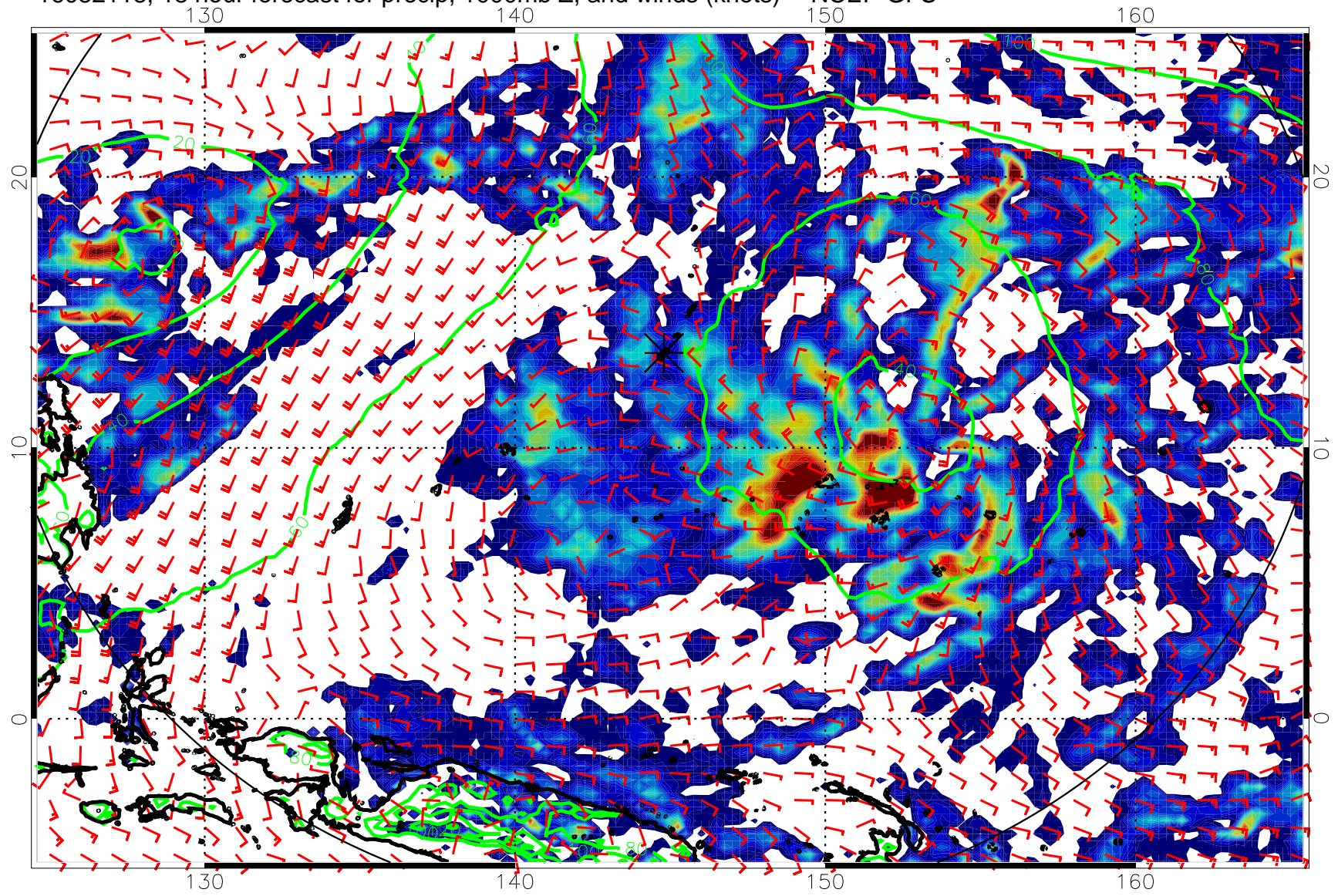
16082118, 18 hour forecast for precip, 1000mb Z, and winds (knots) -- NCEP GFS
