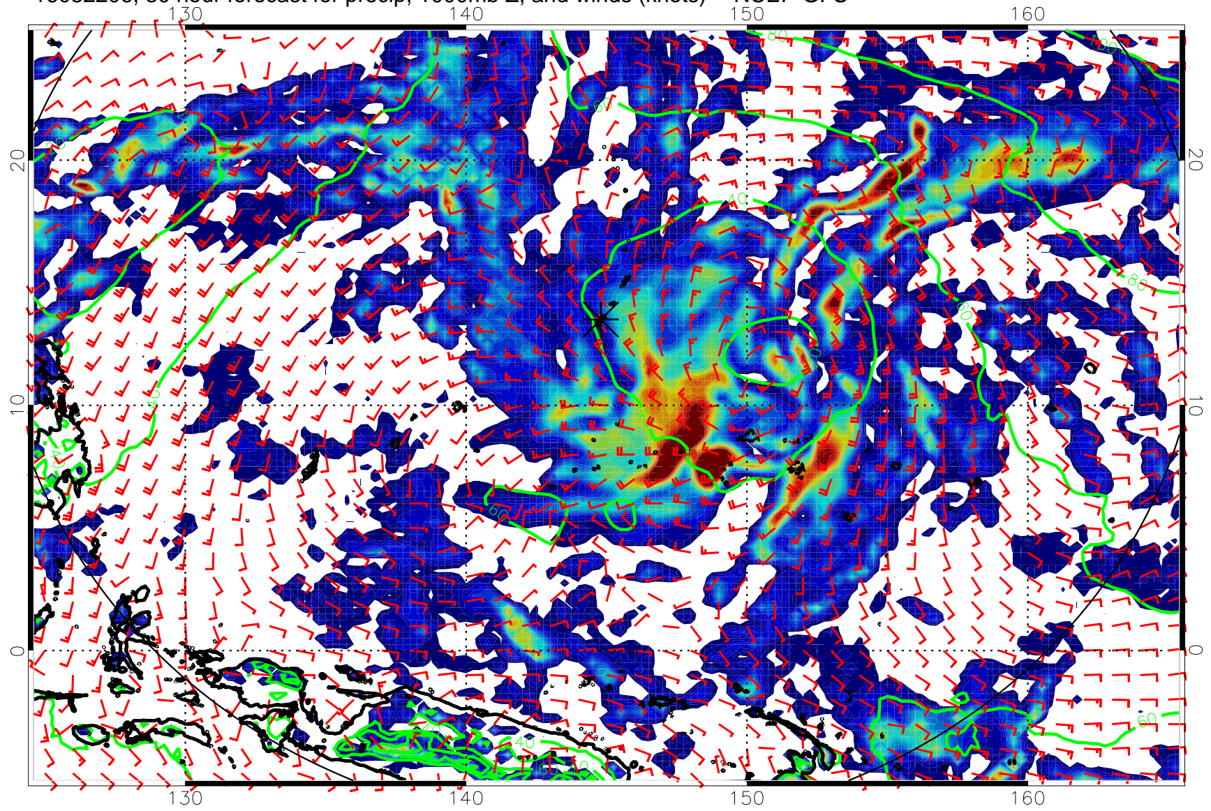
16082206, 30 hour forecast for precip, 1000mb Z, and winds (knots) -- NCEP GFS
