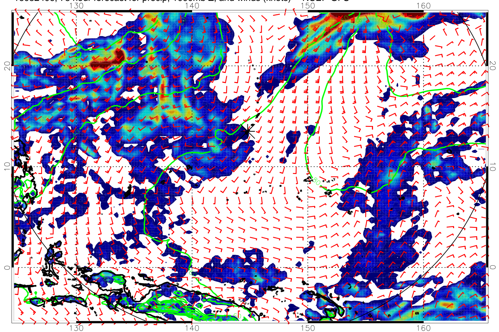
16082406, 78 hour forecast for precip, 1000mb Z, and winds (knots) -- NCEP GFS
