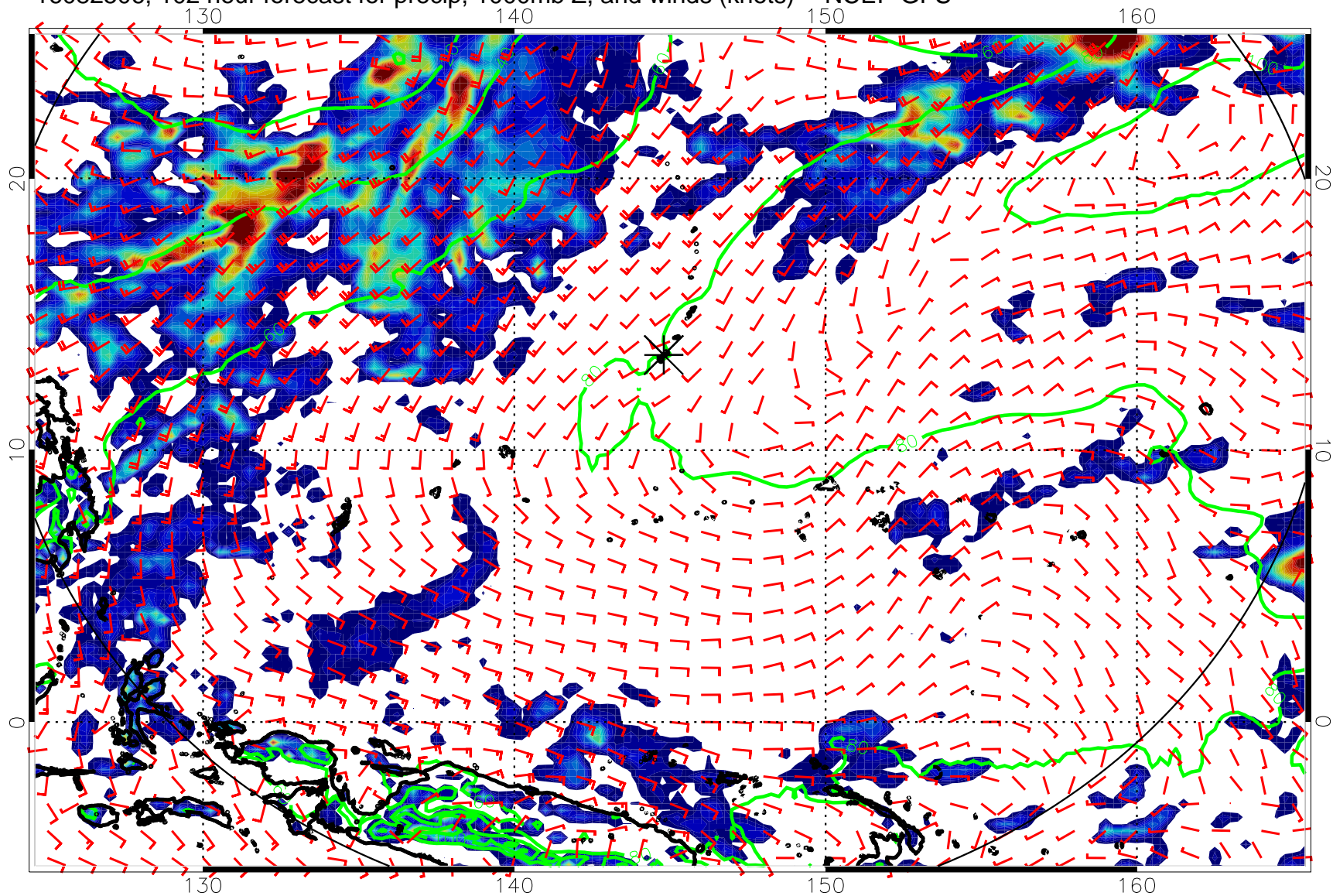
16082506, 102 hour forecast for precip, 1000mb Z, and winds (knots) -- NCEP GFS
