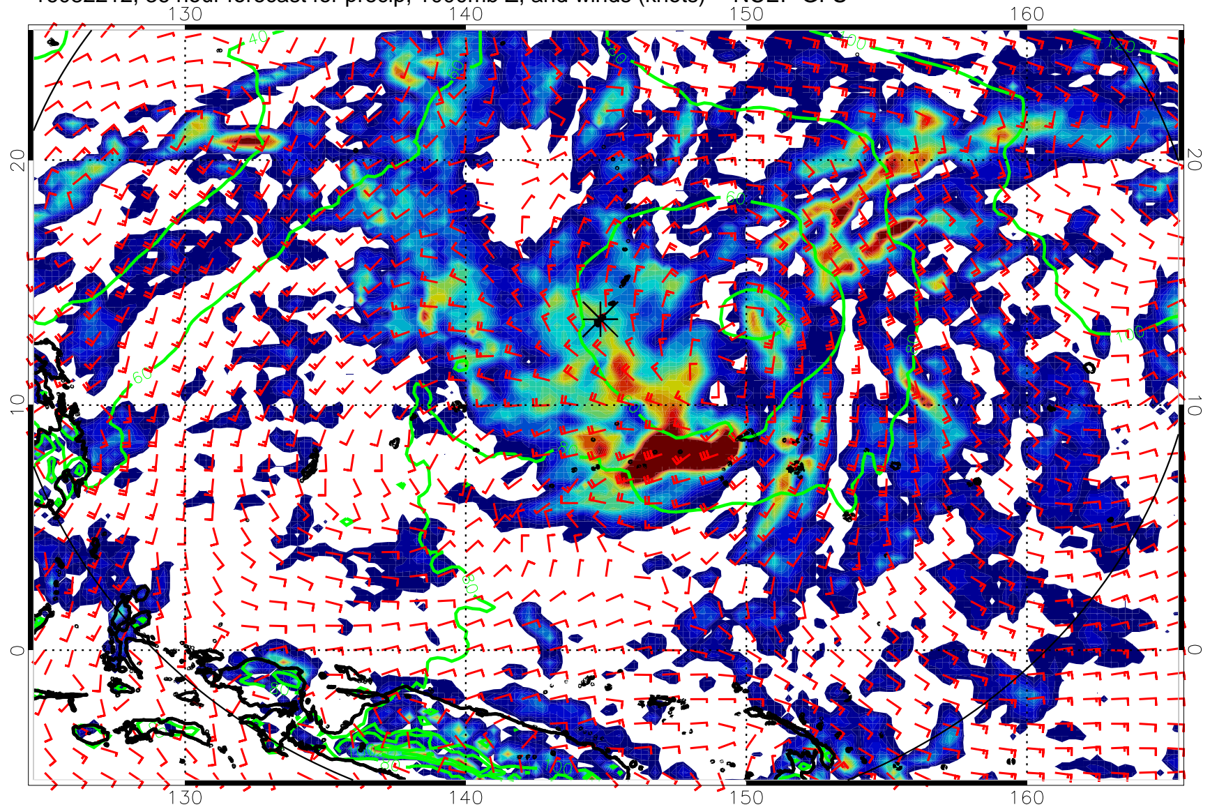
16082212, 36 hour forecast for precip, 1000mb Z, and winds (knots) -- NCEP GFS
