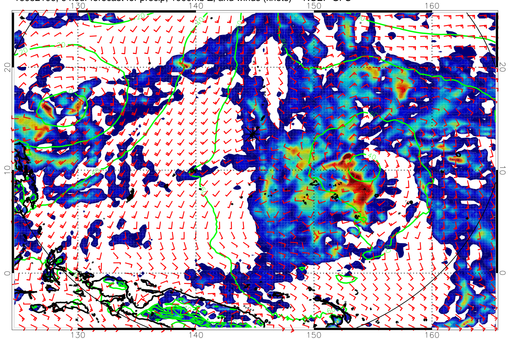
16082106, 6 hour forecast for precip, 1000mb Z, and winds (knots) -- NCEP GFS
