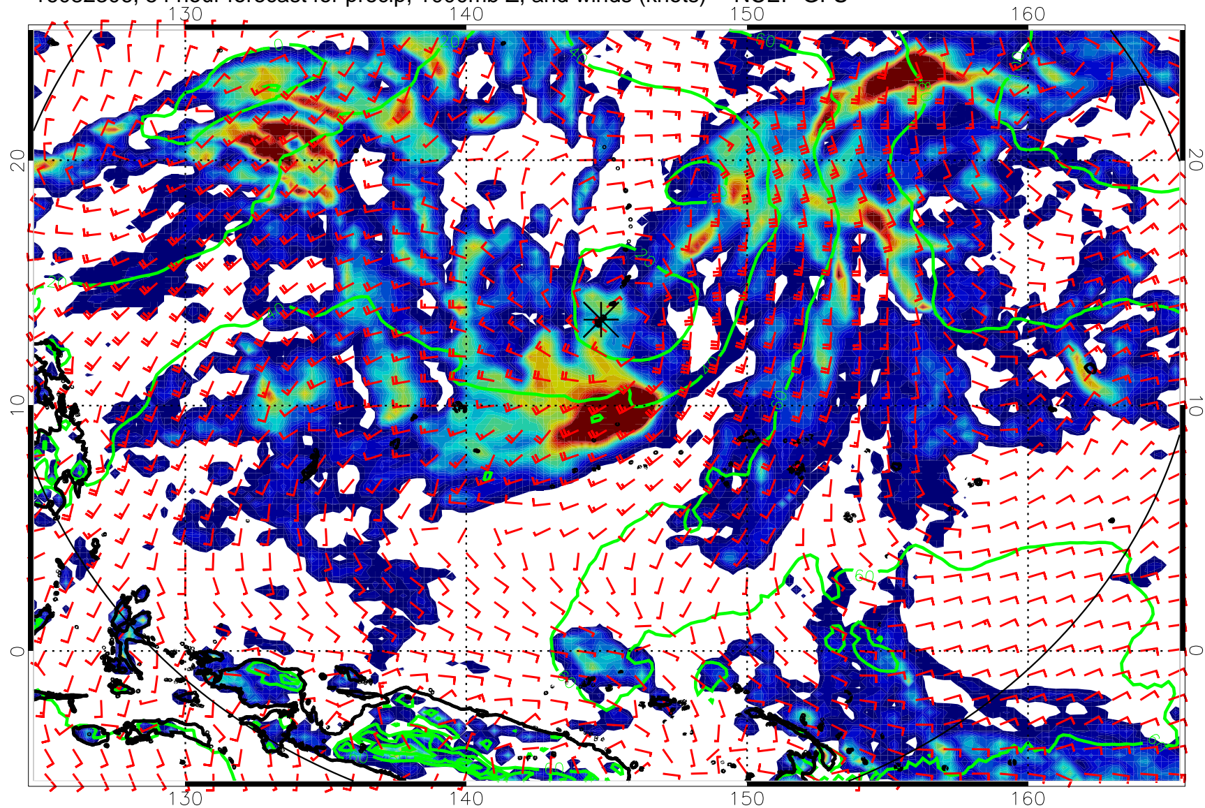
16082306, 54 hour forecast for precip, 1000mb Z, and winds (knots) -- NCEP GFS
