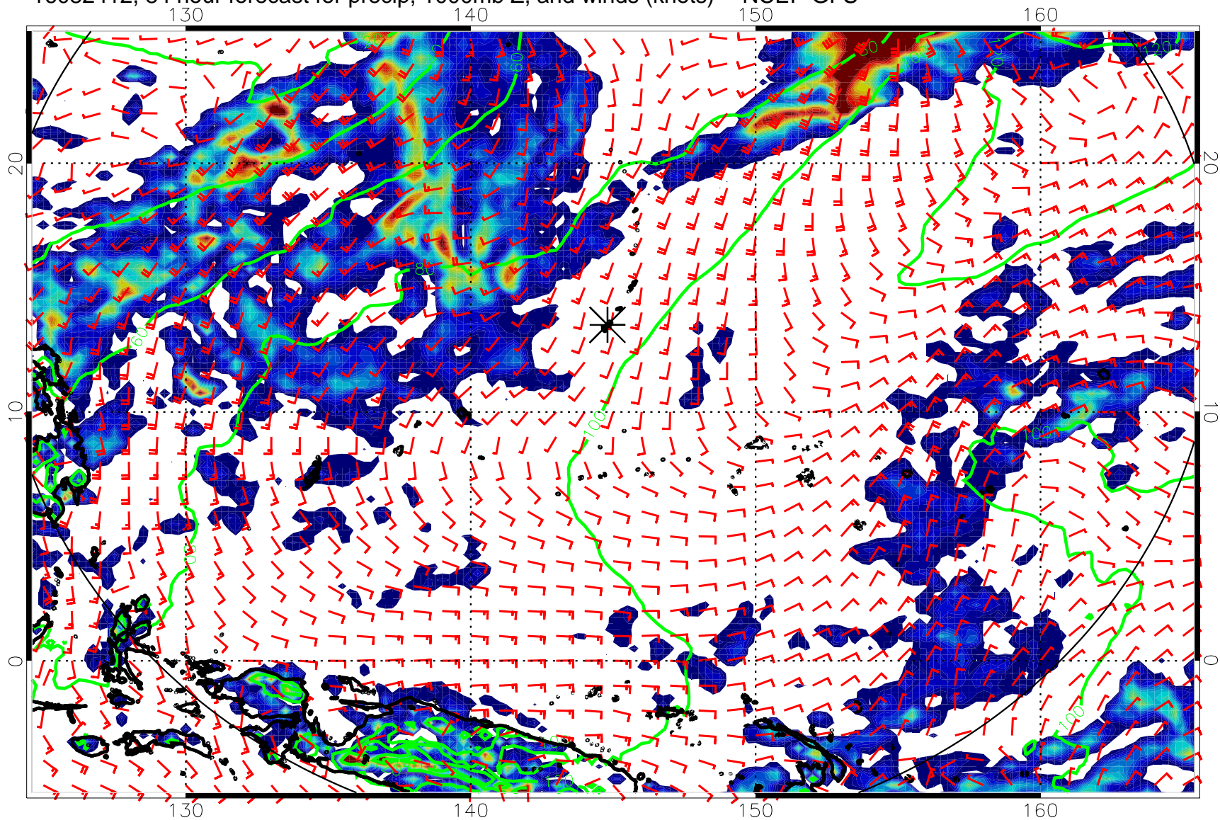
16082412, 84 hour forecast for precip, 1000mb Z, and winds (knots) -- NCEP GFS
