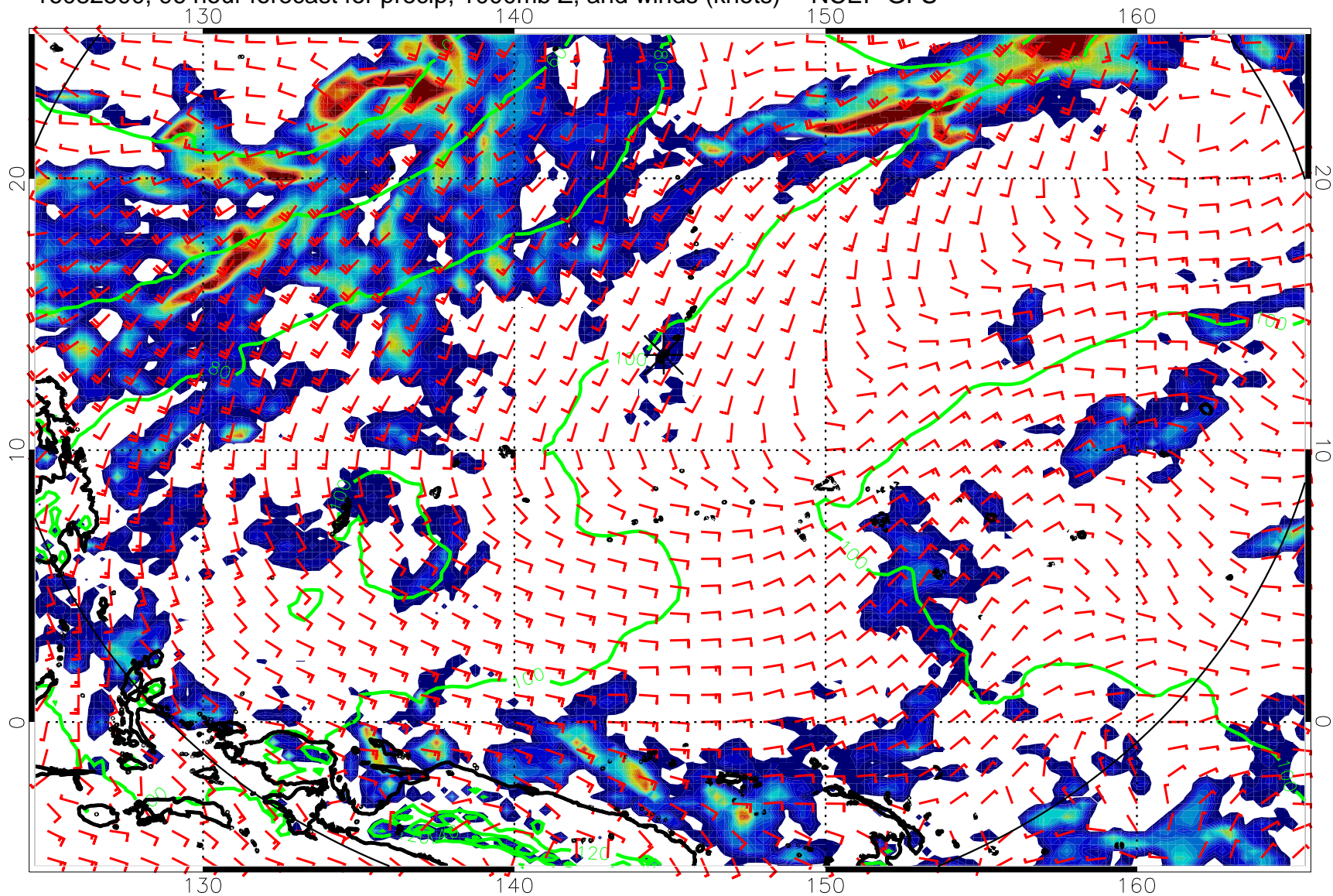
16082500, 96 hour forecast for precip, 1000mb Z, and winds (knots) -- NCEP GFS
