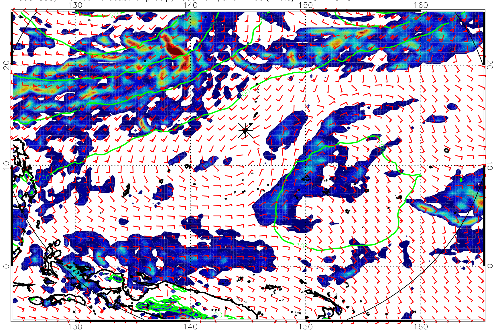
16082600, 120 hour forecast for precip, 1000mb Z, and winds (knots) -- NCEP GFS
