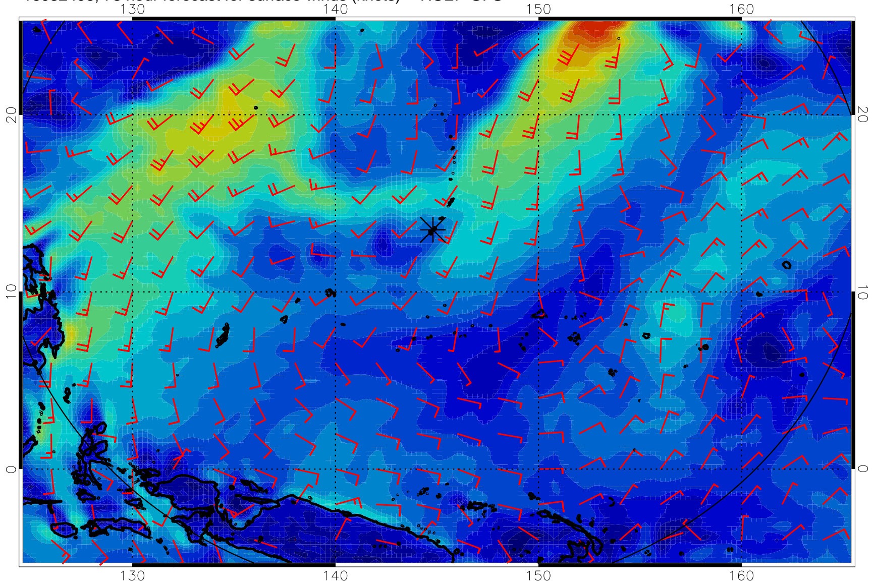
16082406, 78 hour forecast for surface winds (knots) -- NCEP GFS
