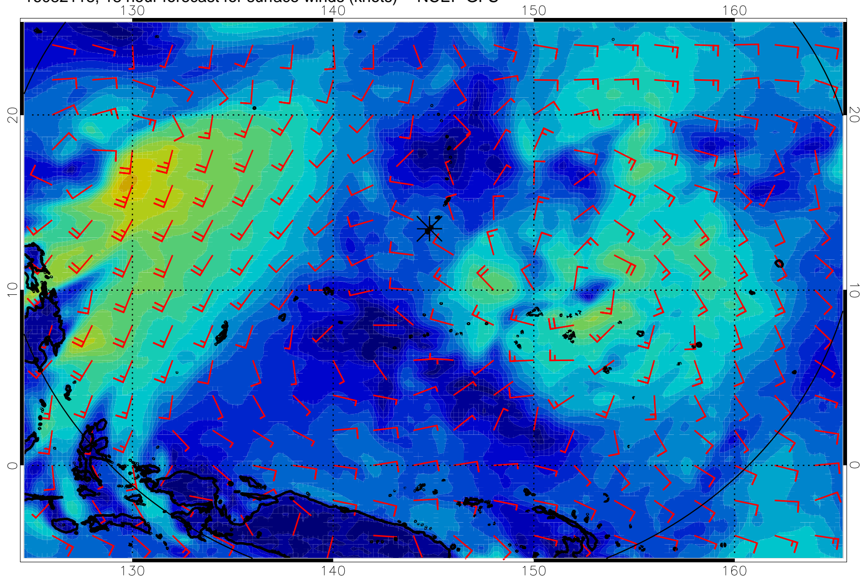
16082118, 18 hour forecast for surface winds (knots) -- NCEP GFS
