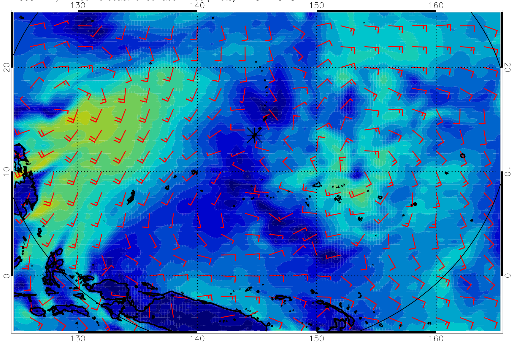
16082112, 12 hour forecast for surface winds (knots) -- NCEP GFS
