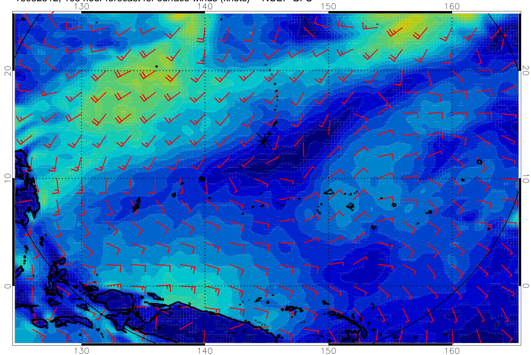
16082512, 108 hour forecast for surface winds (knots) -- NCEP GFS
