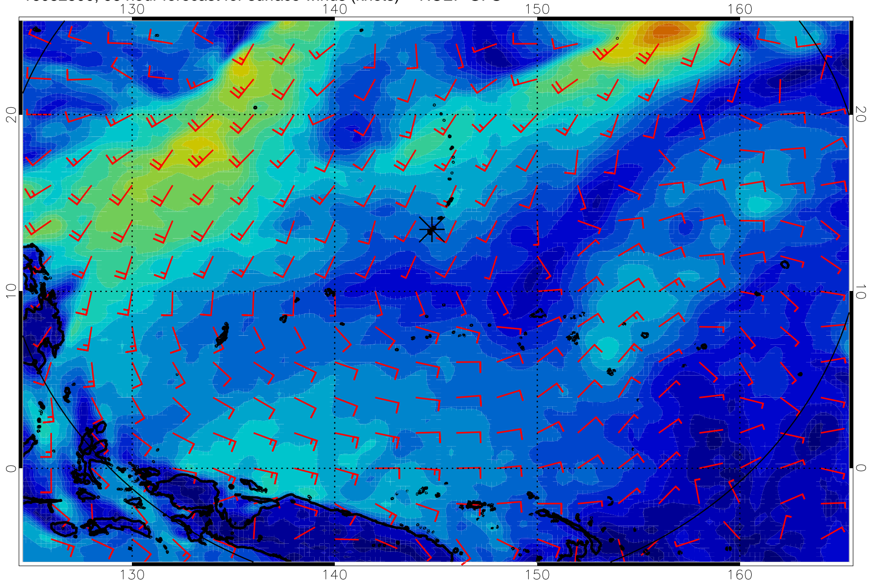
16082500, 96 hour forecast for surface winds (knots) -- NCEP GFS
