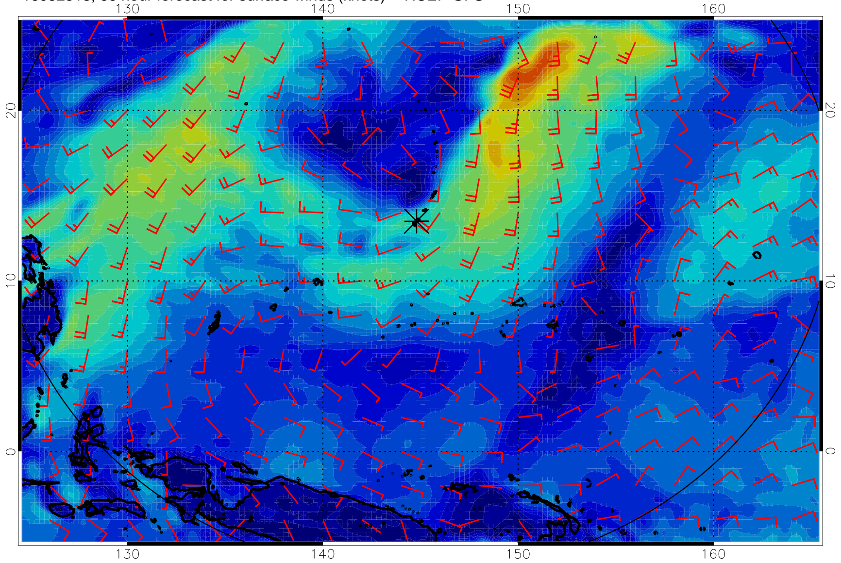
16082318, 66 hour forecast for surface winds (knots) -- NCEP GFS
