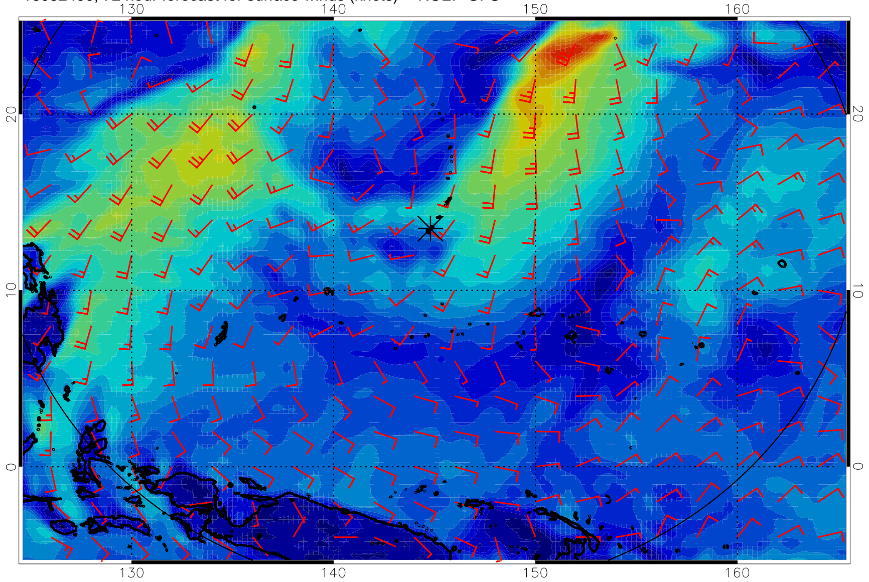
16082400, 72 hour forecast for surface winds (knots) -- NCEP GFS
