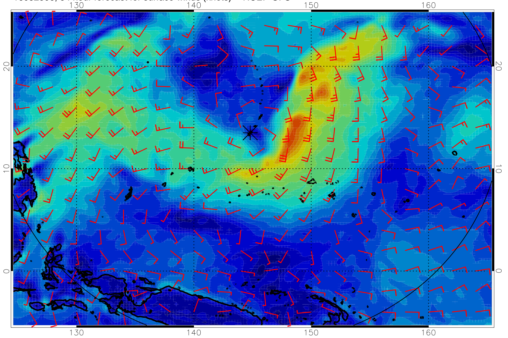
16082306, 54 hour forecast for surface winds (knots) -- NCEP GFS
