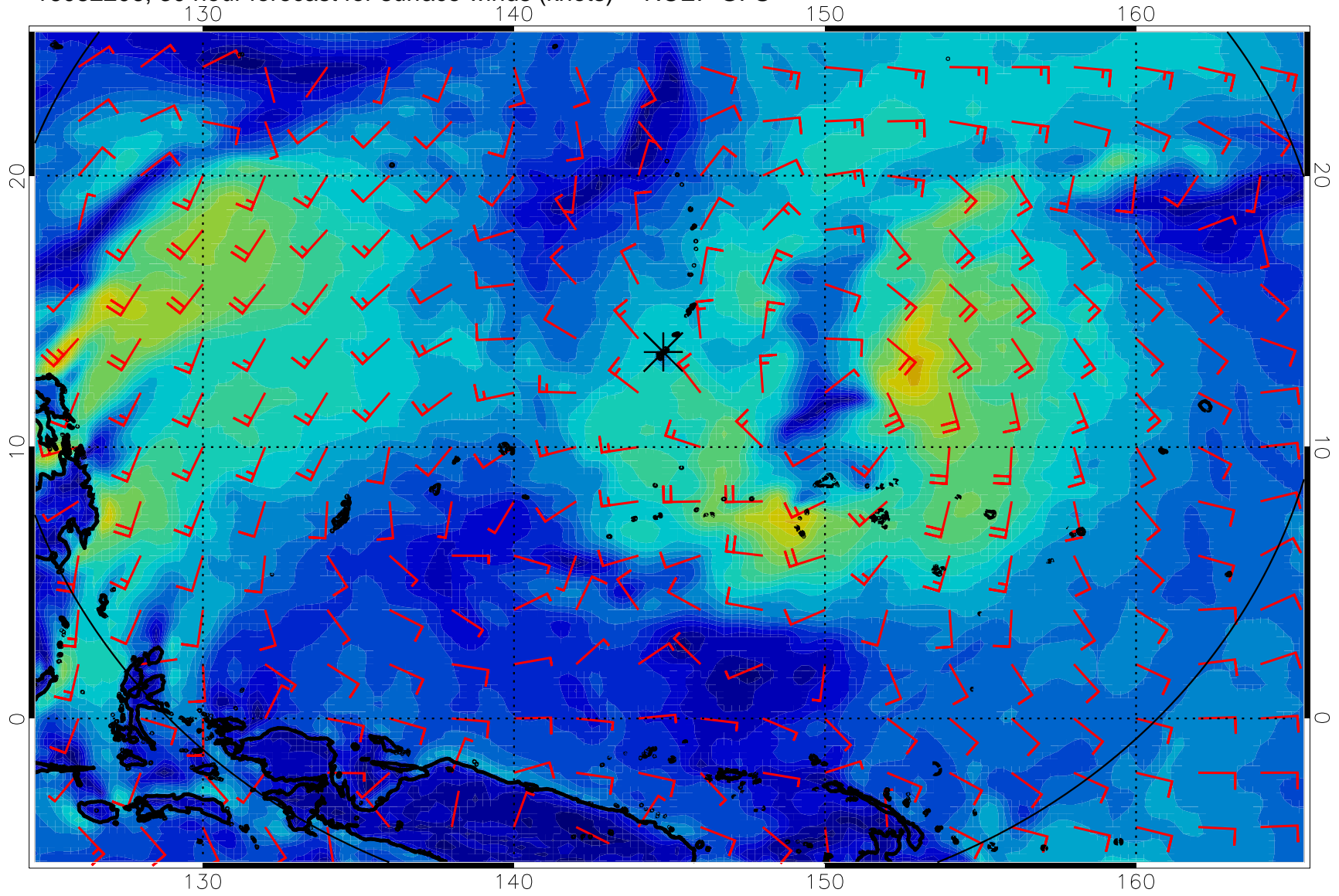
16082206, 30 hour forecast for surface winds (knots) -- NCEP GFS
