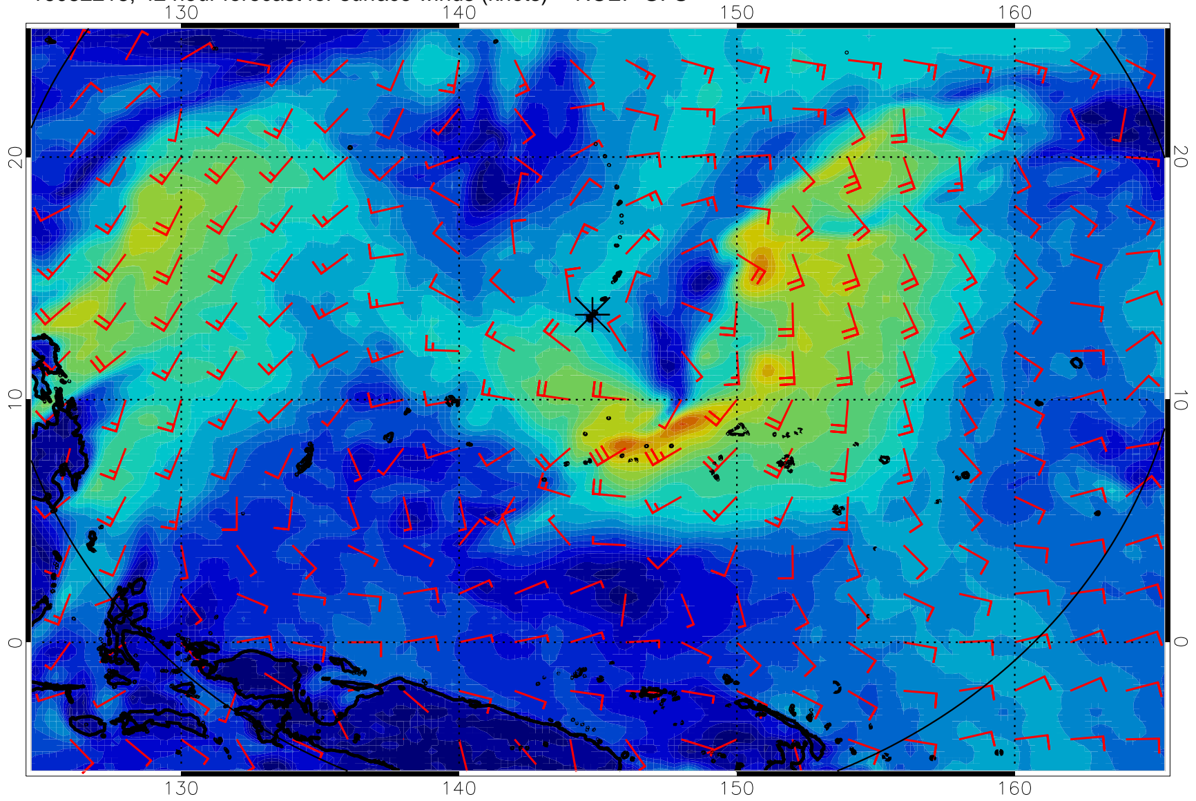
16082218, 42 hour forecast for surface winds (knots) -- NCEP GFS
