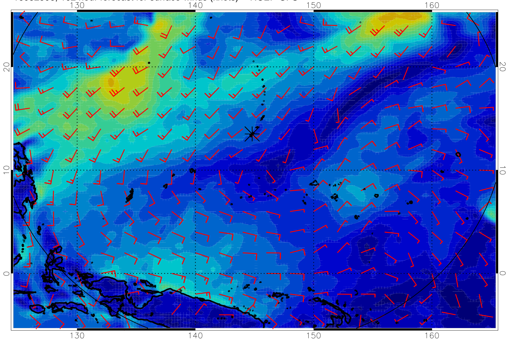
16082506, 102 hour forecast for surface winds (knots) -- NCEP GFS
