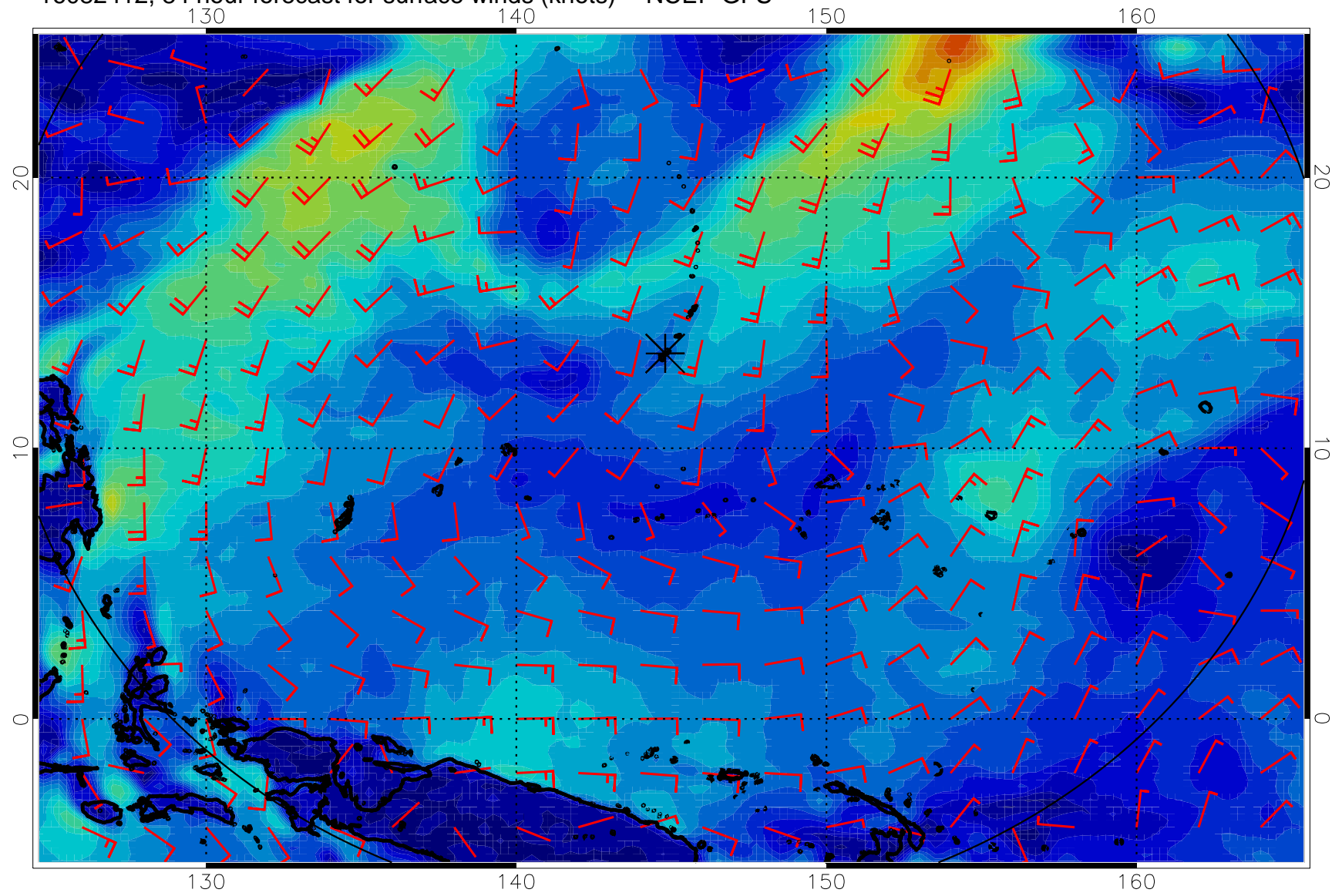
16082412, 84 hour forecast for surface winds (knots) -- NCEP GFS
