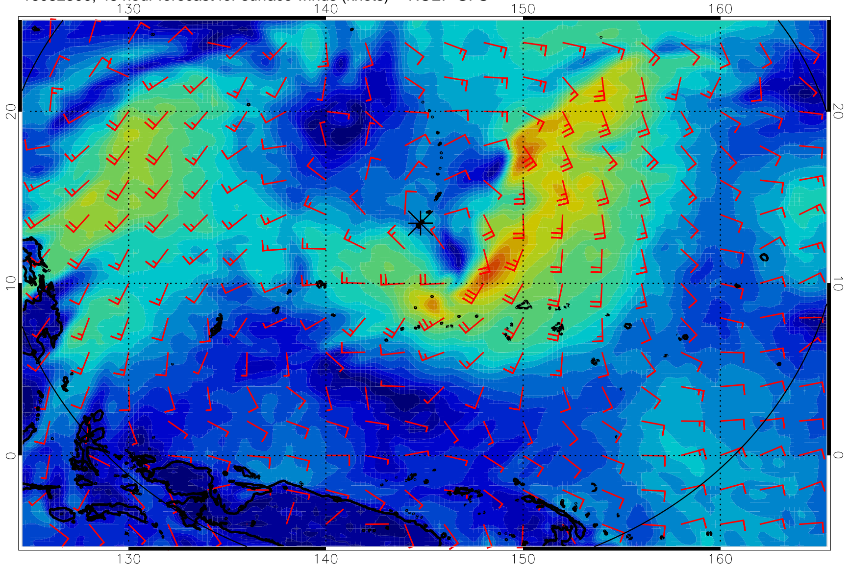
16082300, 48 hour forecast for surface winds (knots) -- NCEP GFS
