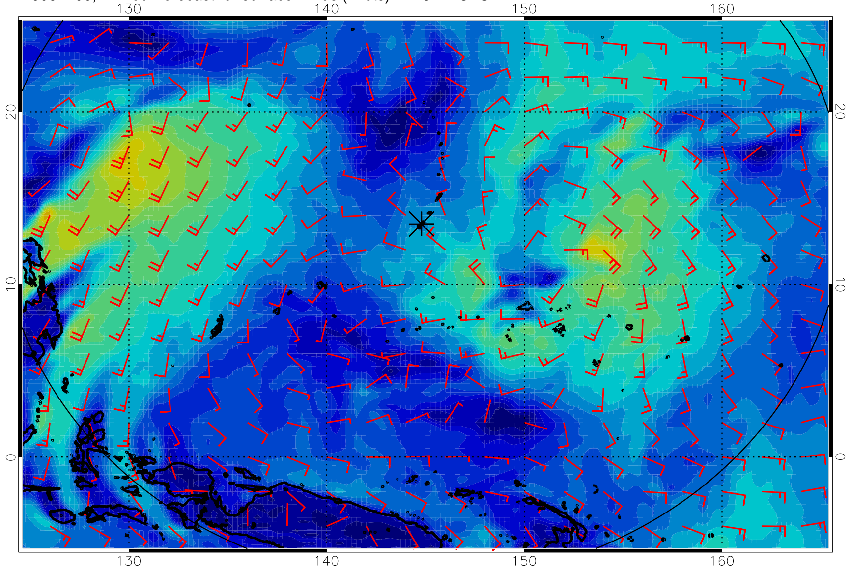
16082200, 24 hour forecast for surface winds (knots) -- NCEP GFS
