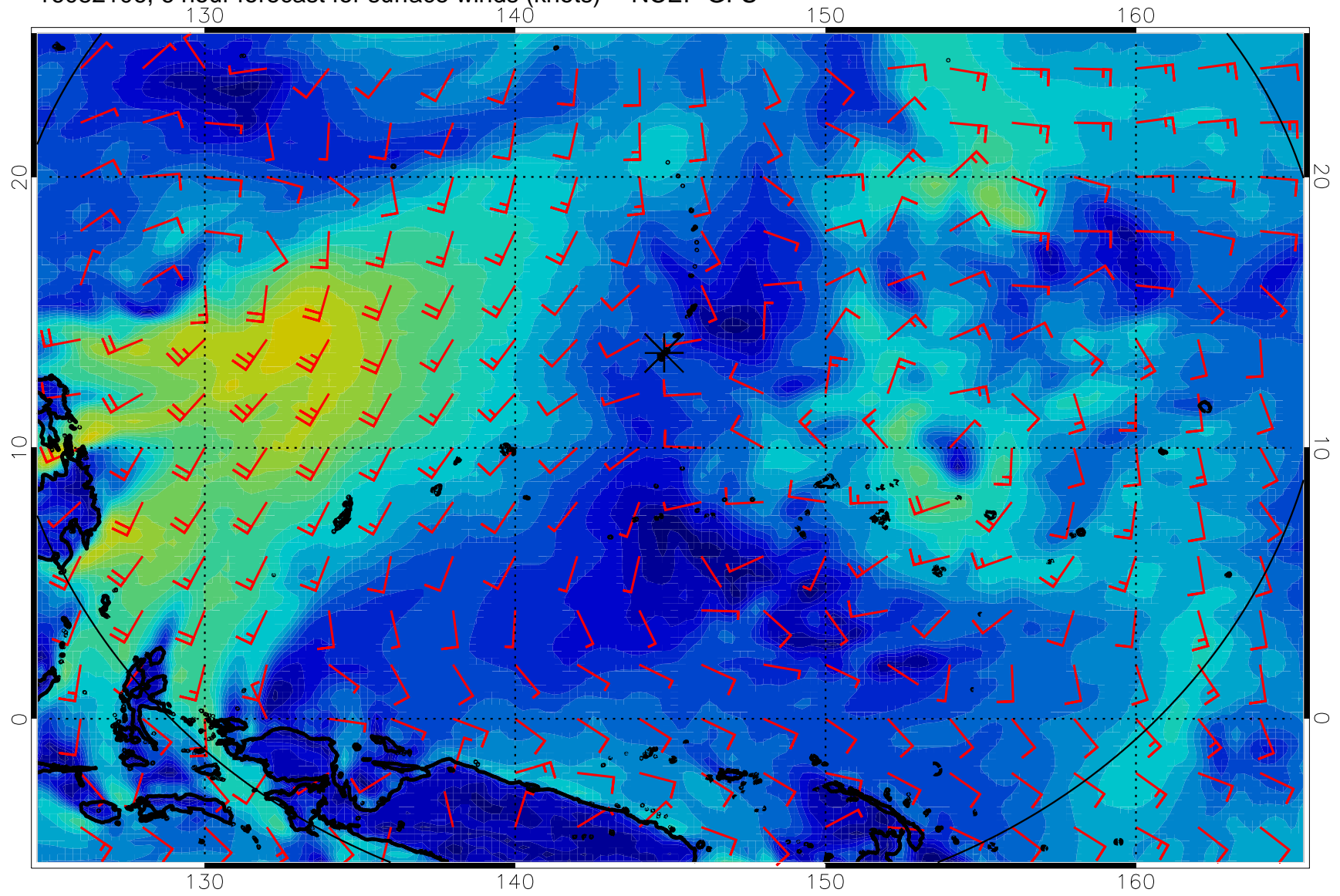
16082106, 6 hour forecast for surface winds (knots) -- NCEP GFS
