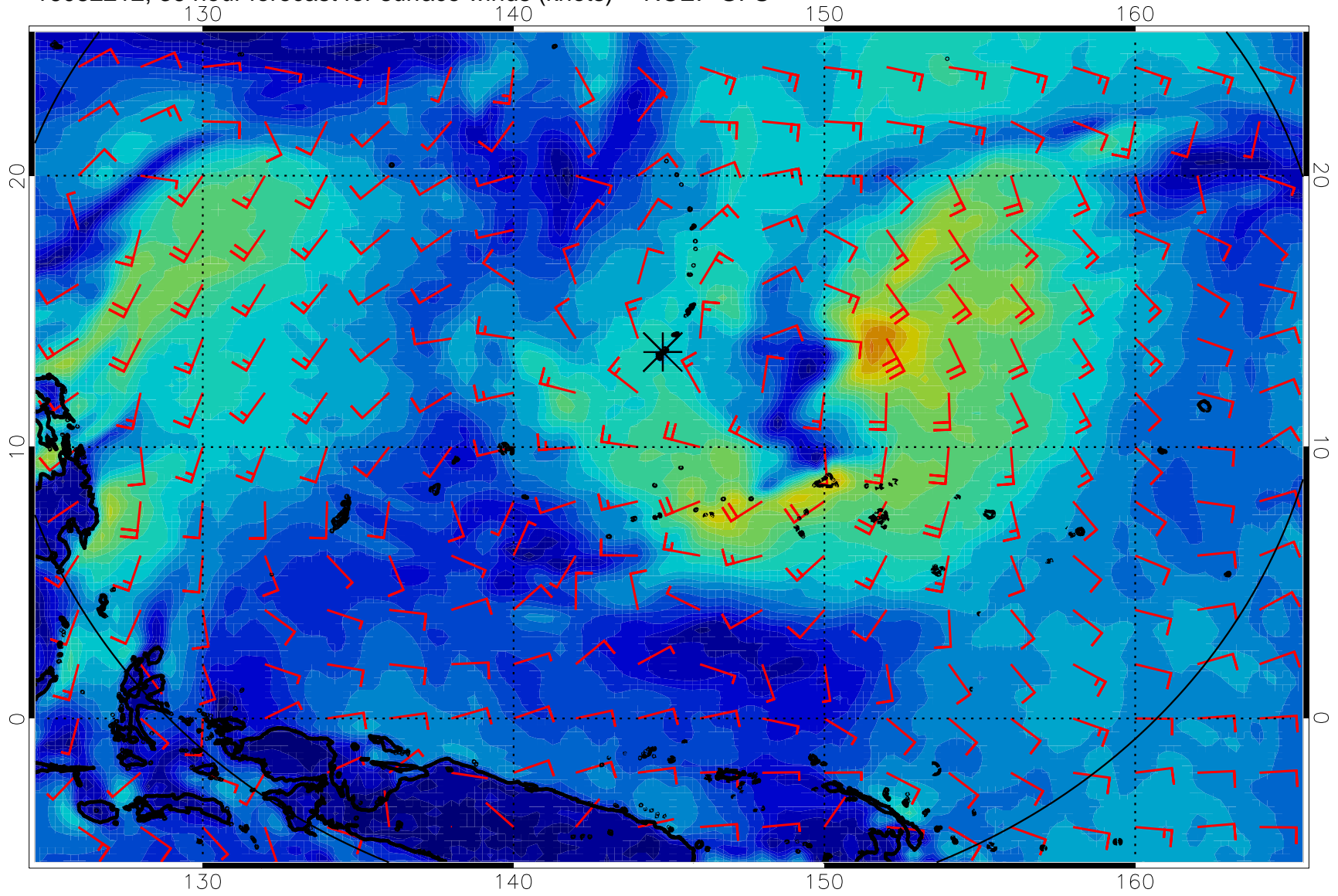
16082212, 36 hour forecast for surface winds (knots) -- NCEP GFS
