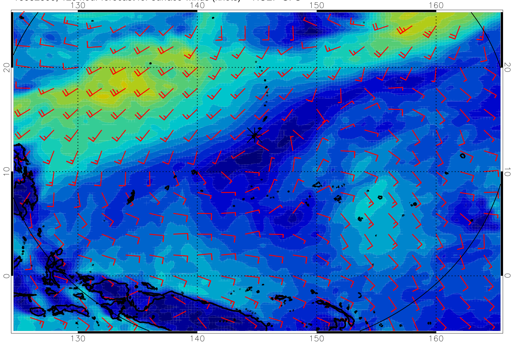
16082600, 120 hour forecast for surface winds (knots) -- NCEP GFS
