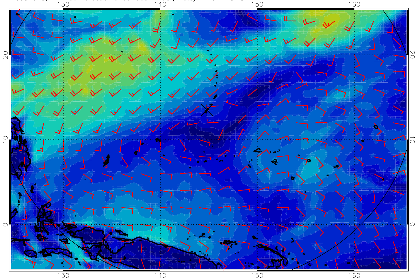
16082518, 114 hour forecast for surface winds (knots) -- NCEP GFS
