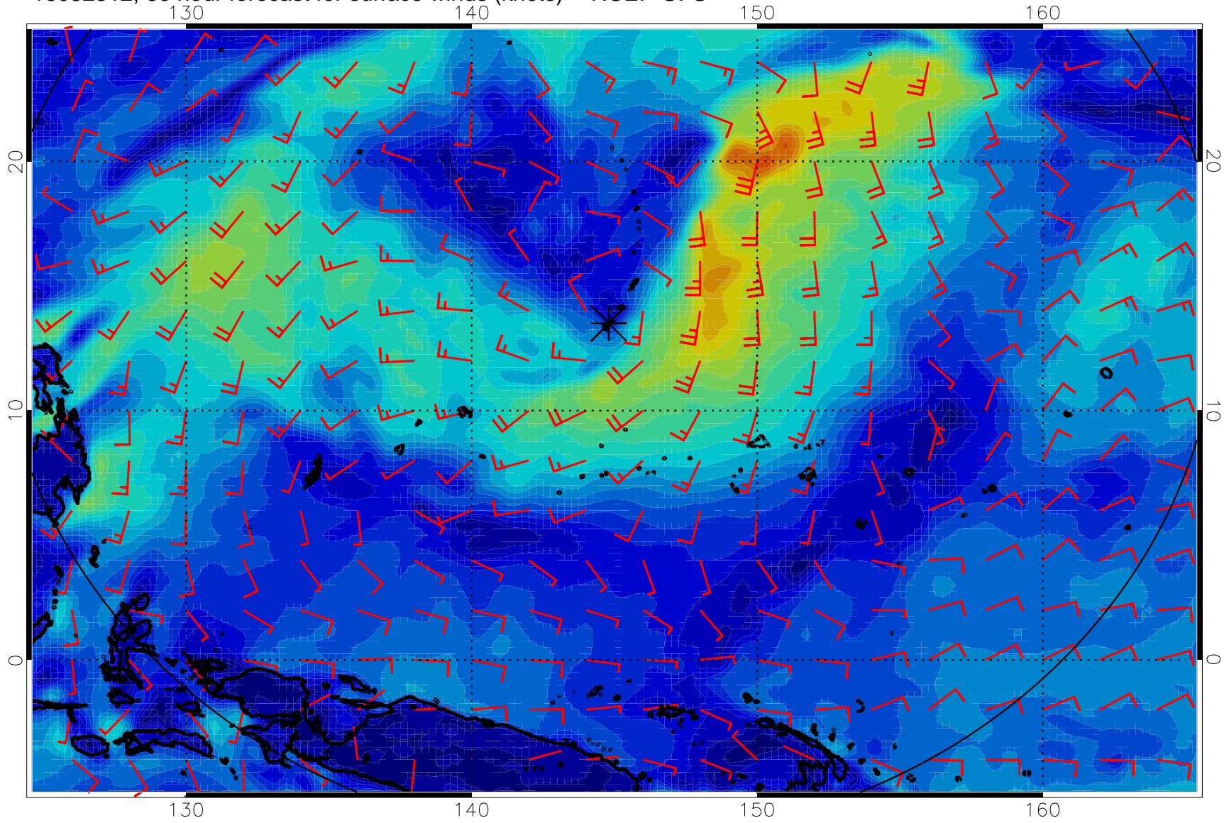
16082312, 60 hour forecast for surface winds (knots) -- NCEP GFS
