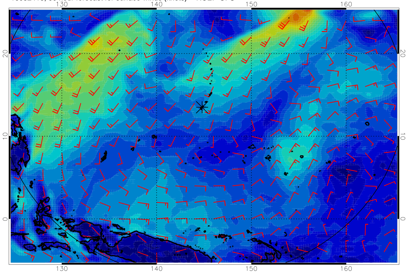
16082418, 90 hour forecast for surface winds (knots) -- NCEP GFS
