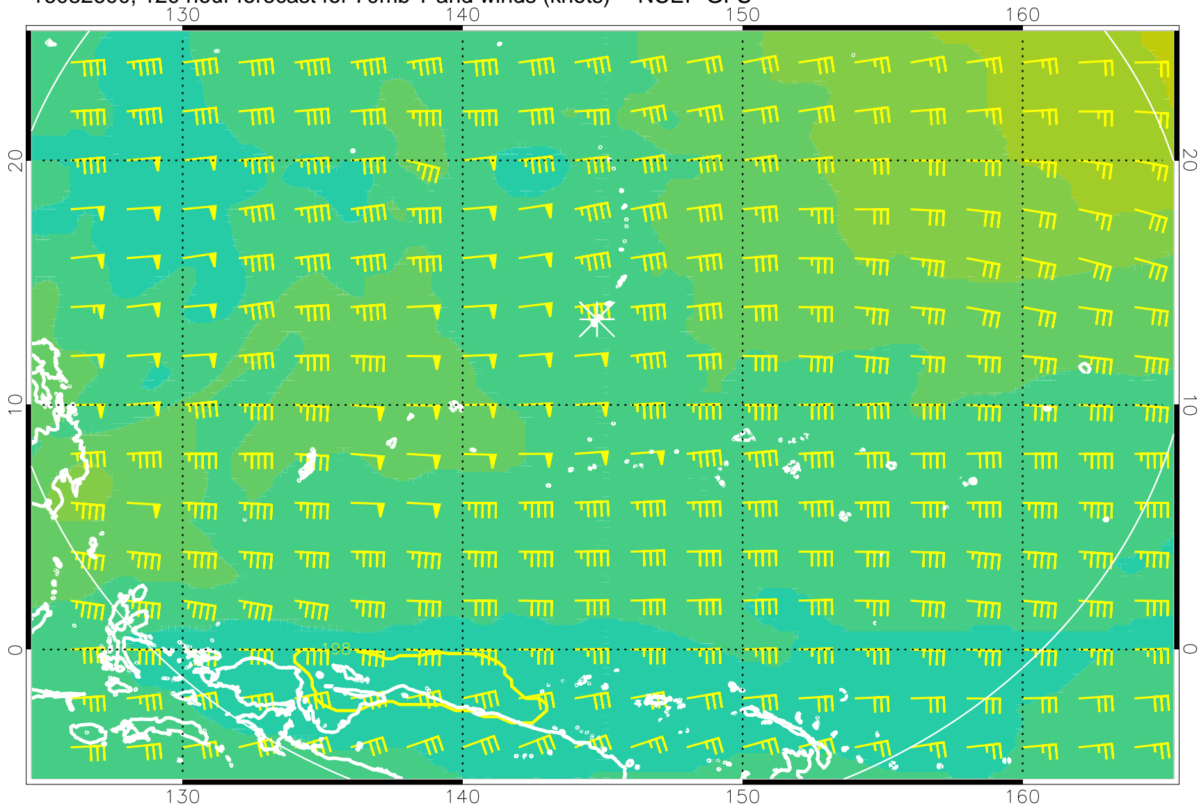
16082600, 120 hour forecast for 70mb T and winds (knots) -- NCEP GFS
