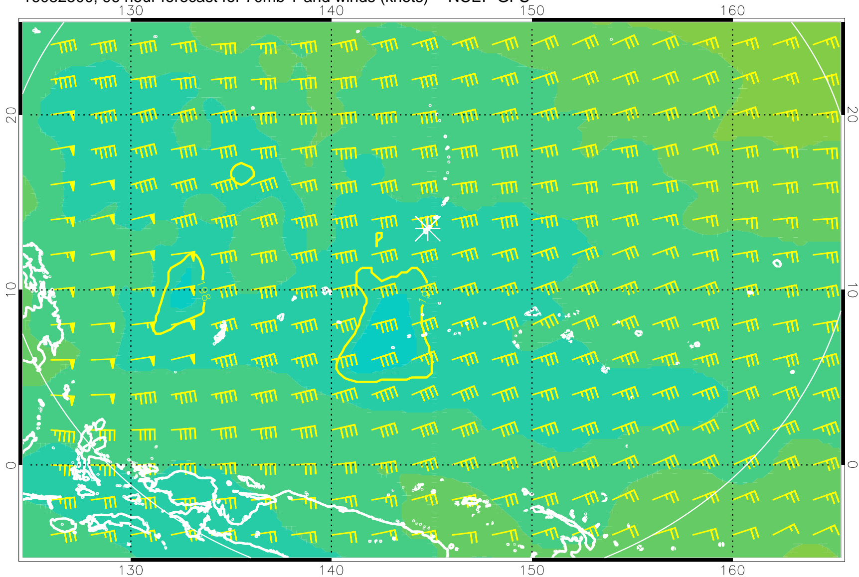
16082500, 96 hour forecast for 70mb T and winds (knots) -- NCEP GFS
