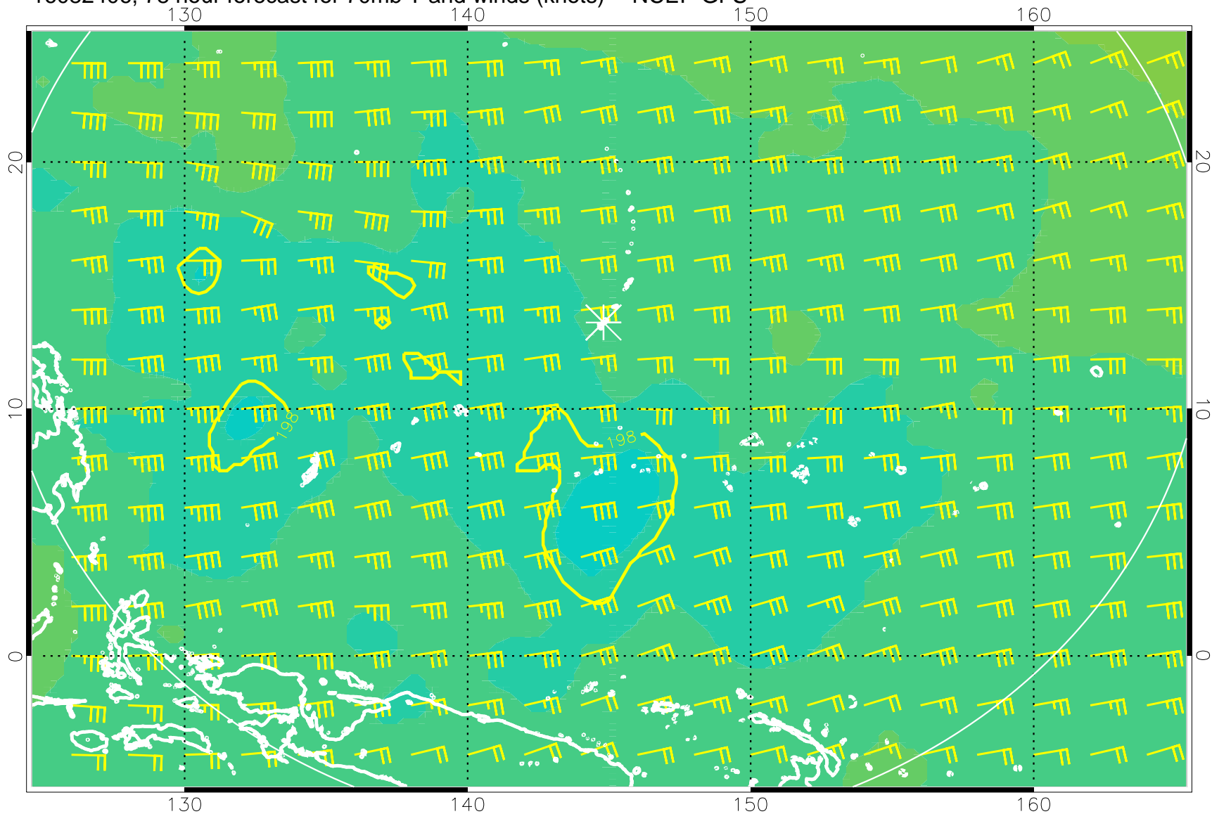
16082406, 78 hour forecast for 70mb T and winds (knots) -- NCEP GFS
