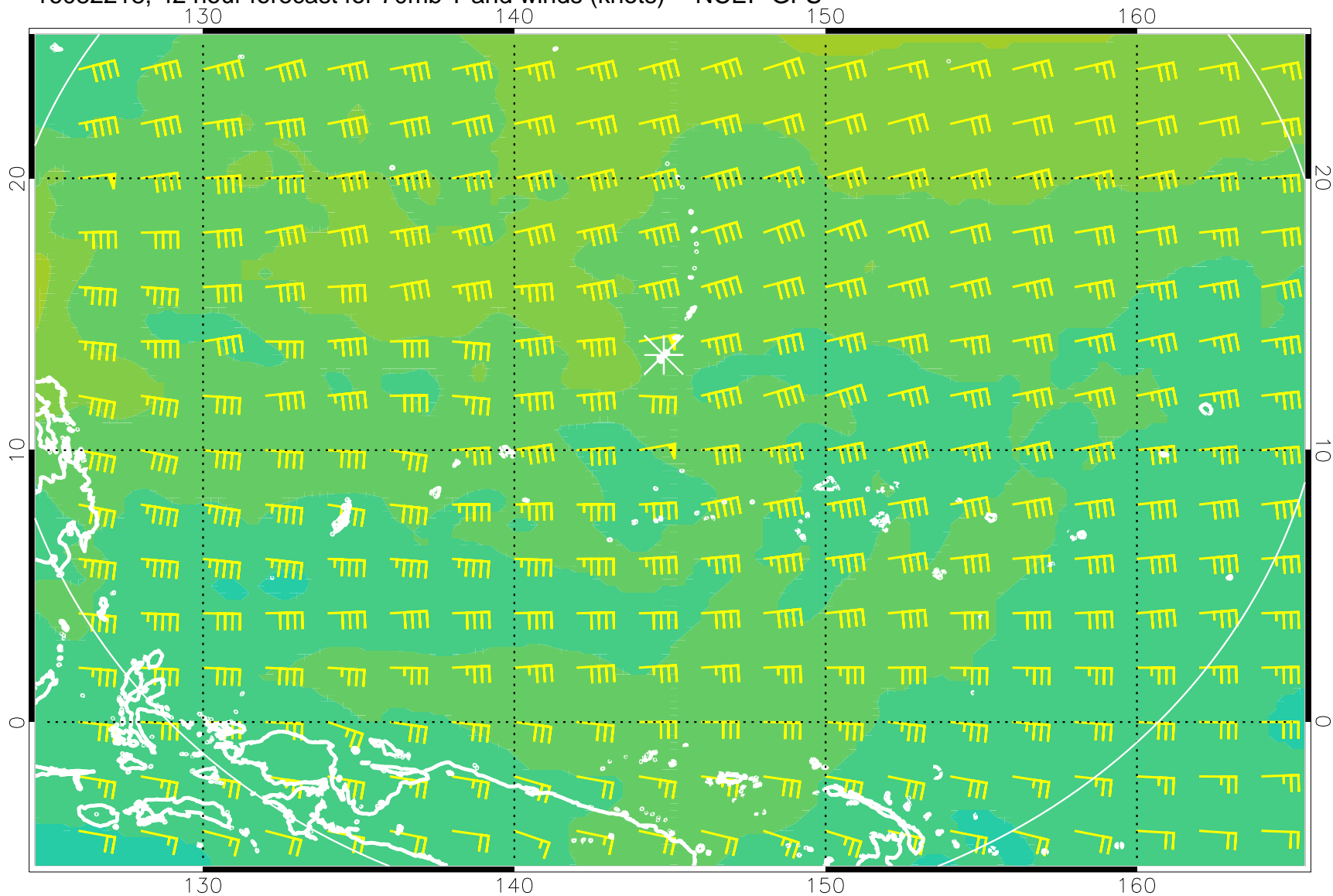
16082218, 42 hour forecast for 70mb T and winds (knots) -- NCEP GFS
