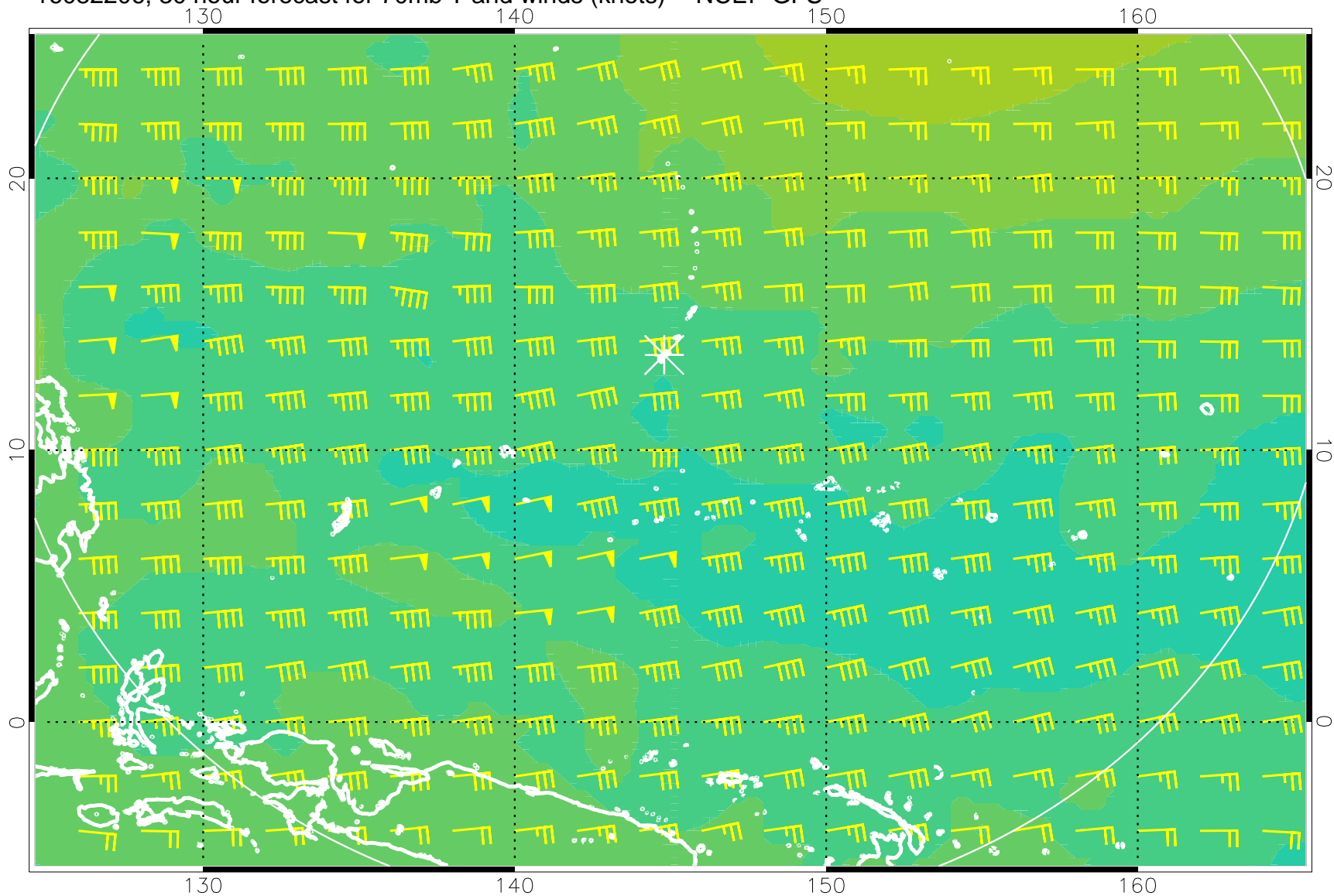
16082206, 30 hour forecast for 70mb T and winds (knots) -- NCEP GFS
