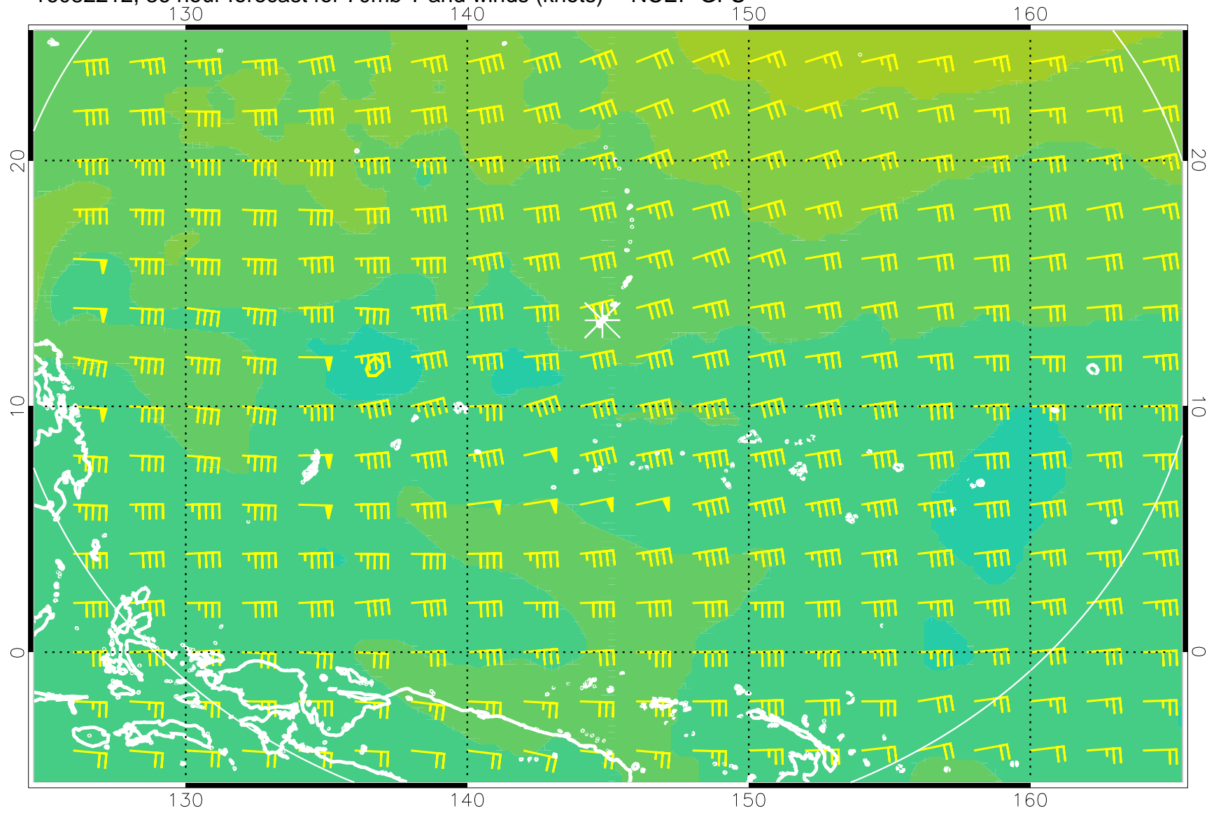
16082212, 36 hour forecast for 70mb T and winds (knots) -- NCEP GFS
