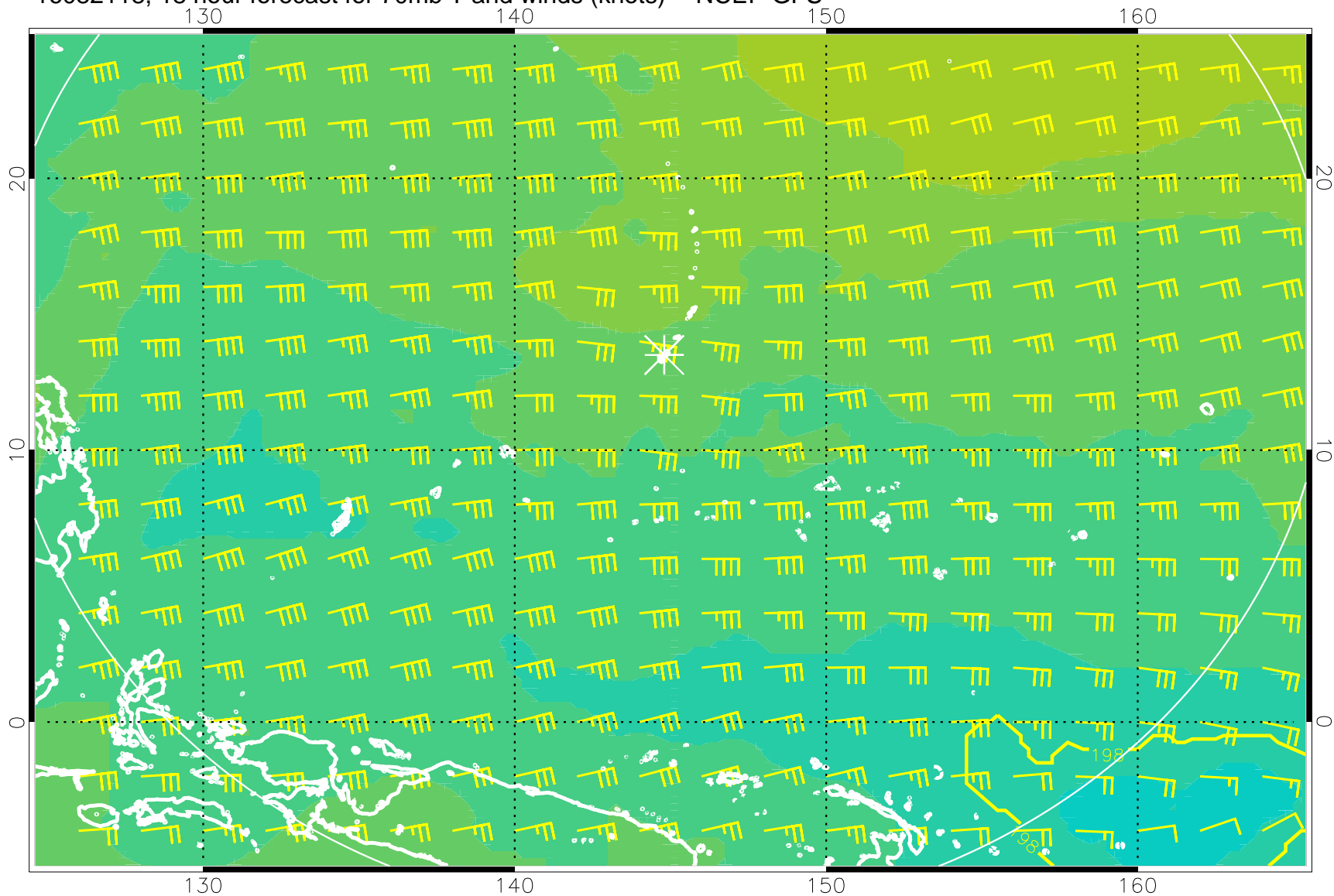
16082118, 18 hour forecast for 70mb T and winds (knots) -- NCEP GFS
