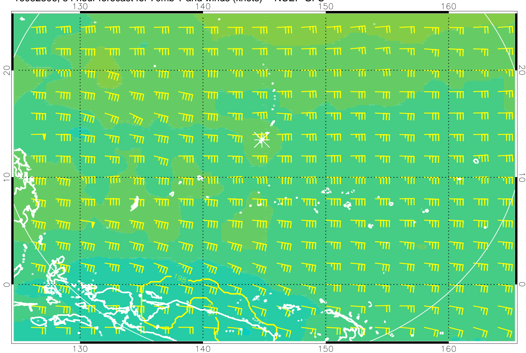
16082306, 54 hour forecast for 70mb T and winds (knots) -- NCEP GFS
