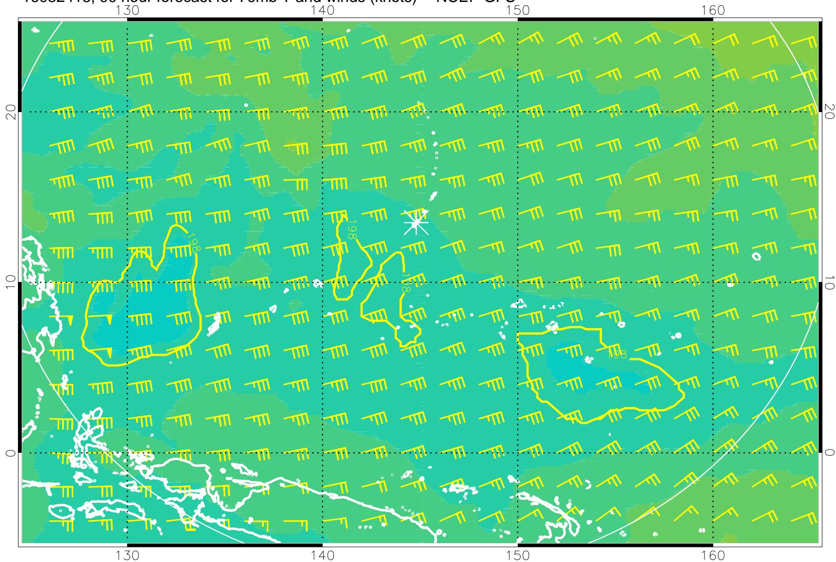
16082418, 90 hour forecast for 70mb T and winds (knots) -- NCEP GFS
