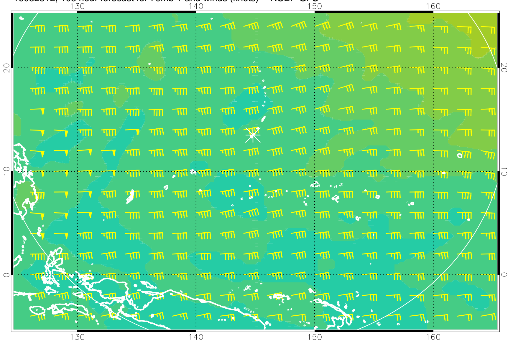
16082512, 108 hour forecast for 70mb T and winds (knots) -- NCEP GFS
