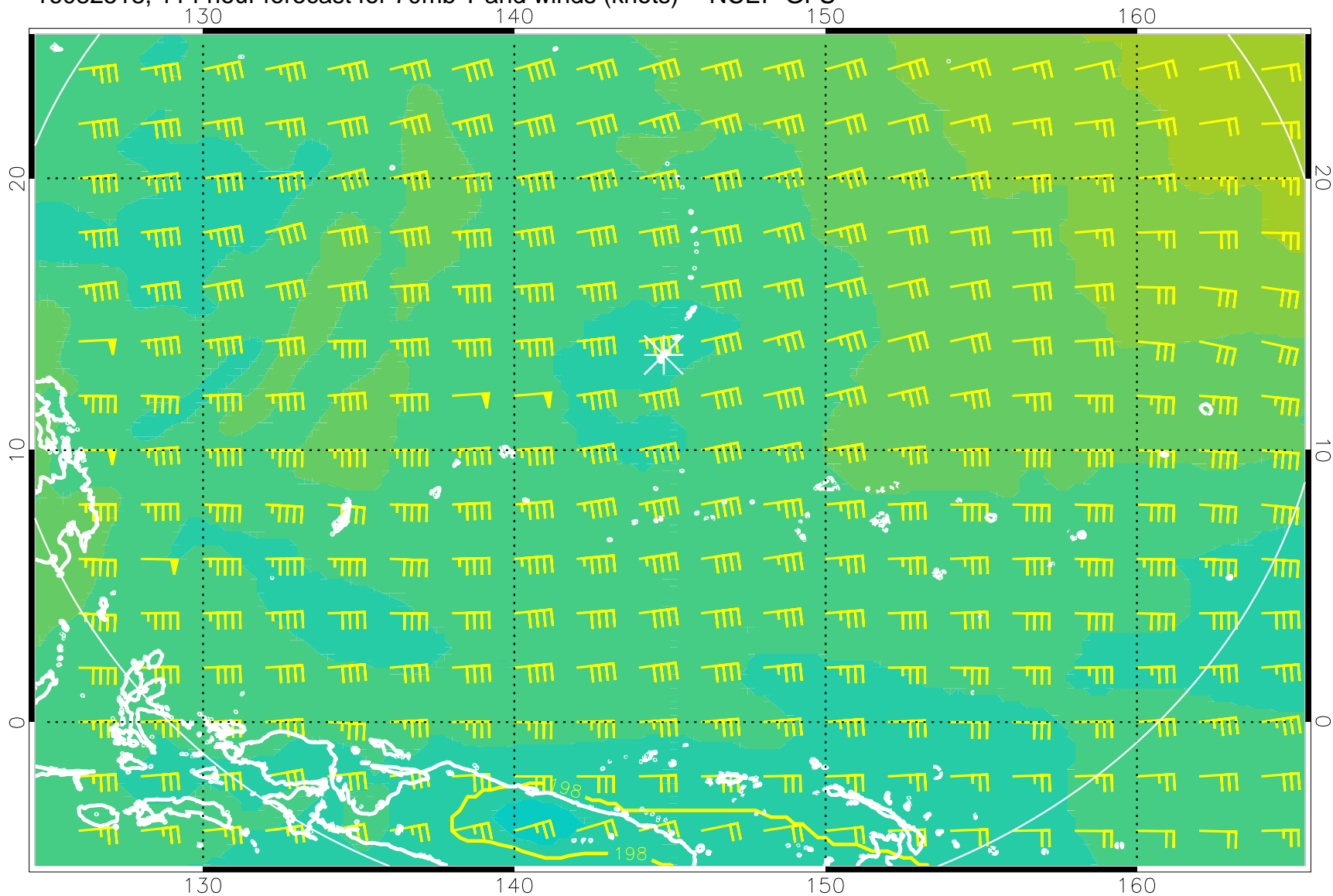
16082518, 114 hour forecast for 70mb T and winds (knots) -- NCEP GFS
