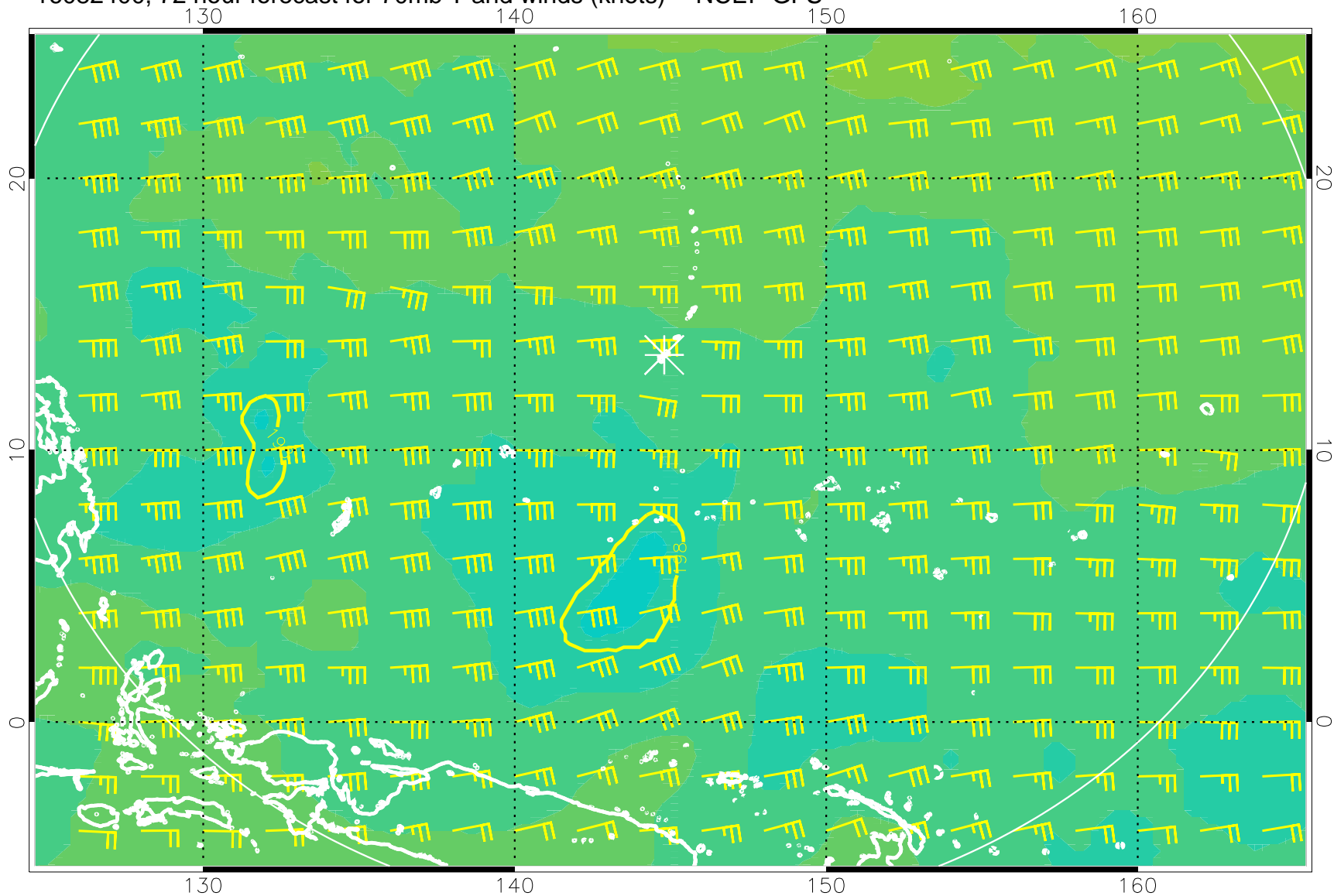
16082400, 72 hour forecast for 70mb T and winds (knots) -- NCEP GFS
