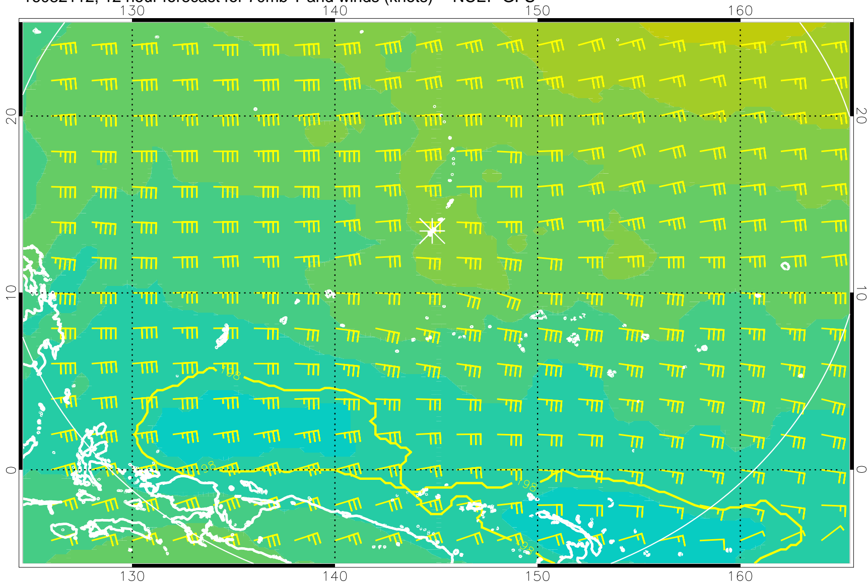
16082112, 12 hour forecast for 70mb T and winds (knots) -- NCEP GFS
