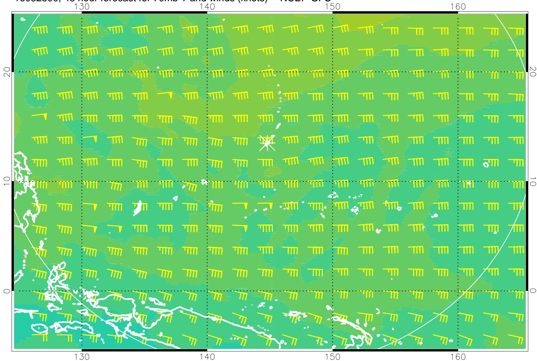
16082300, 48 hour forecast for 70mb T and winds (knots) -- NCEP GFS
