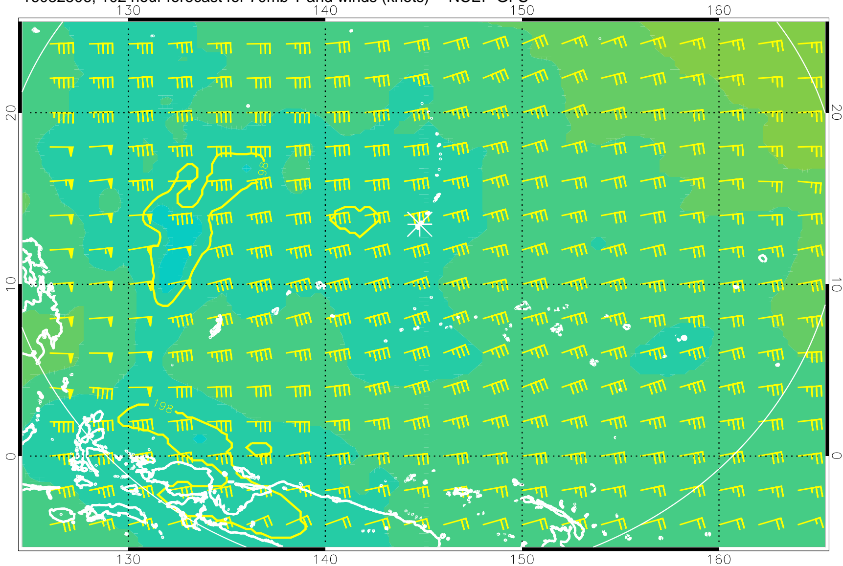
16082506, 102 hour forecast for 70mb T and winds (knots) -- NCEP GFS
