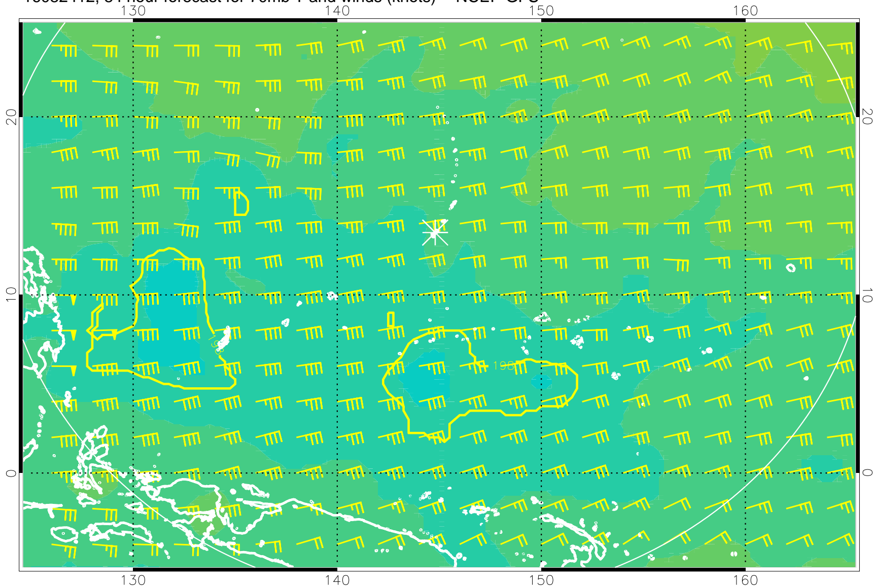
16082412, 84 hour forecast for 70mb T and winds (knots) -- NCEP GFS
