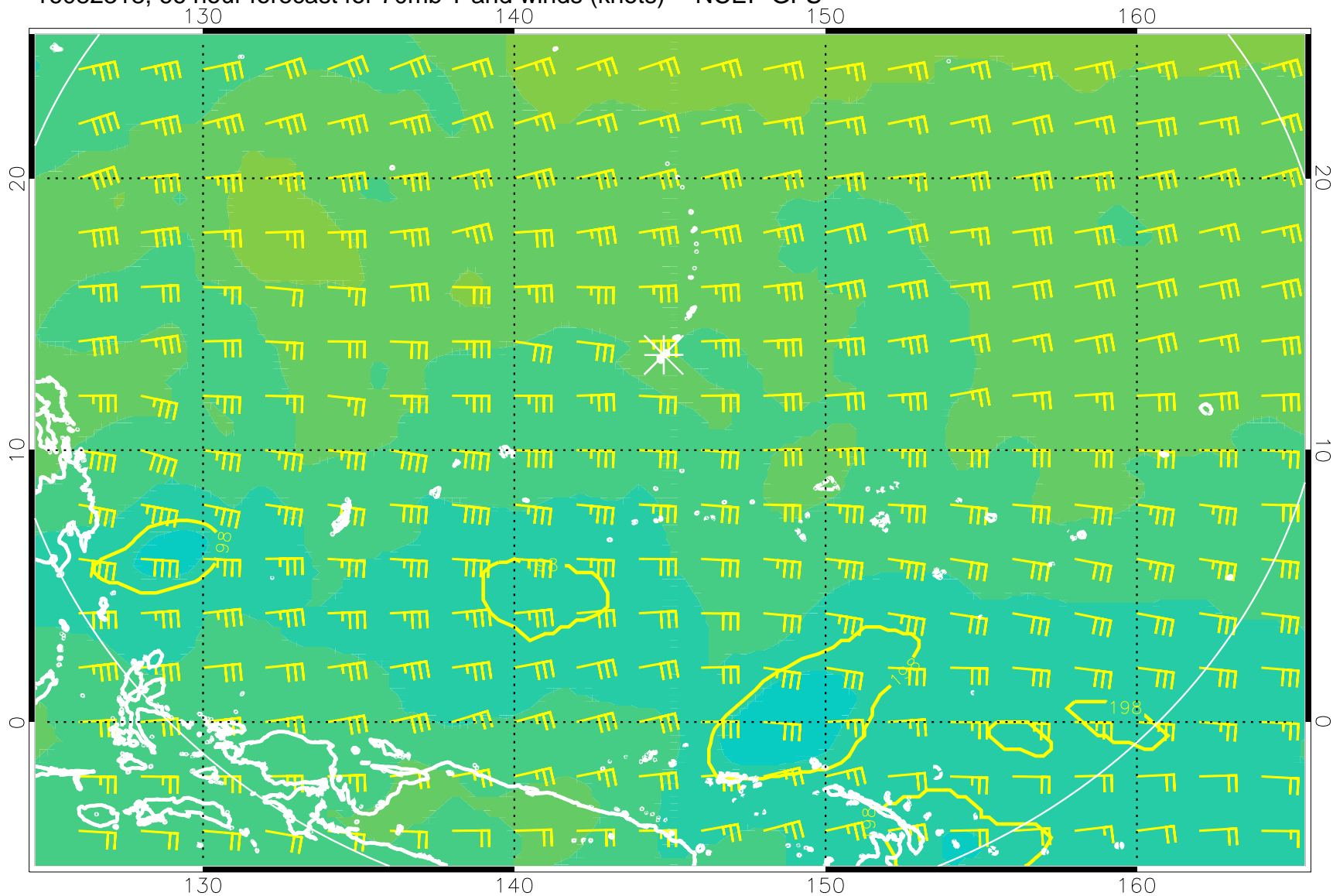
16082318, 66 hour forecast for 70mb T and winds (knots) -- NCEP GFS
