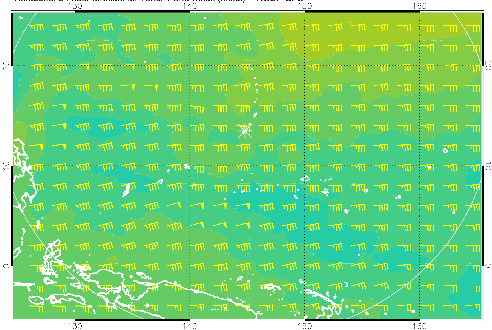
16082200, 24 hour forecast for 70mb T and winds (knots) -- NCEP GFS
