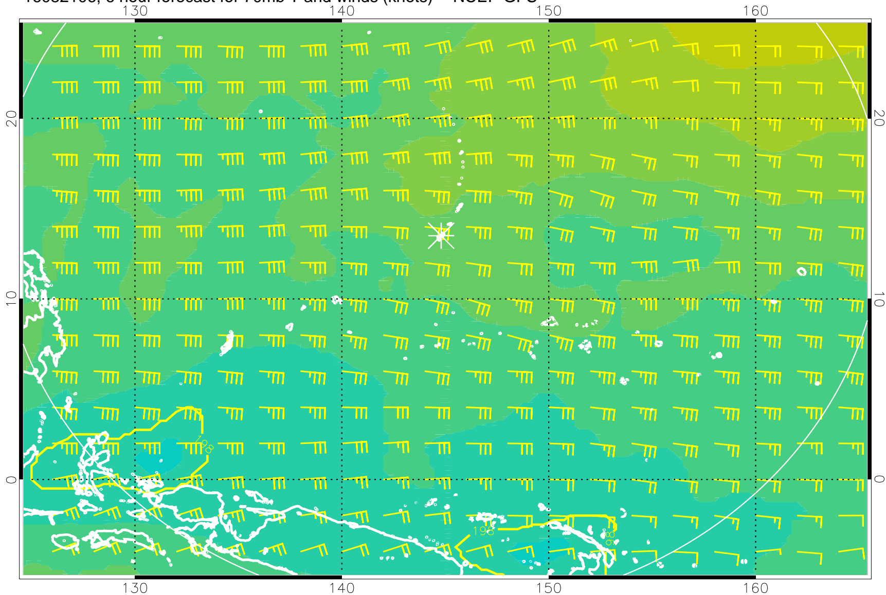
16082106, 6 hour forecast for 70mb T and winds (knots) -- NCEP GFS
