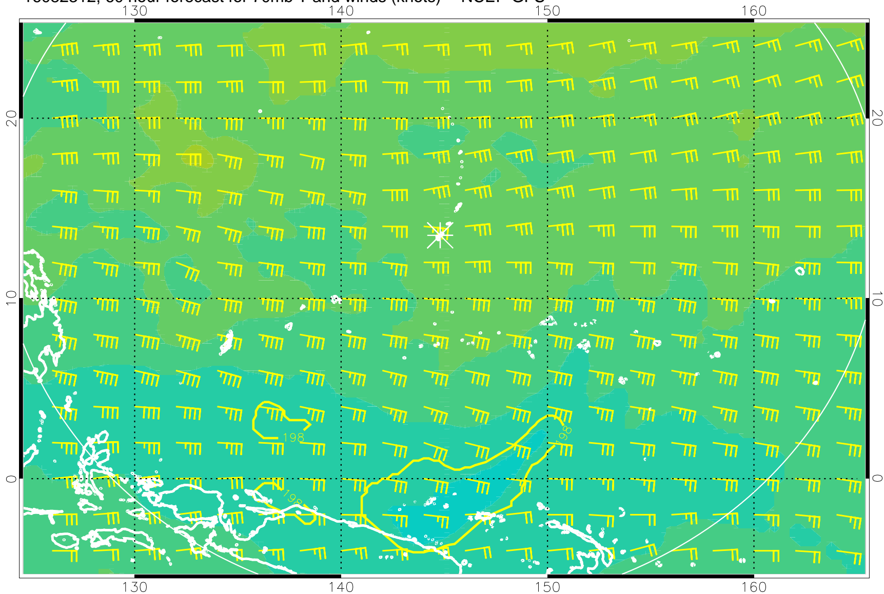
16082312, 60 hour forecast for 70mb T and winds (knots) -- NCEP GFS
