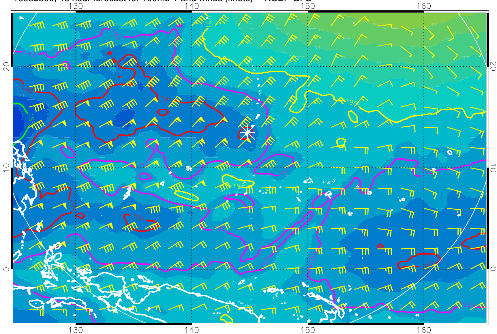
16082300, 48 hour forecast for 100mb T and winds (knots) -- NCEP GFS
