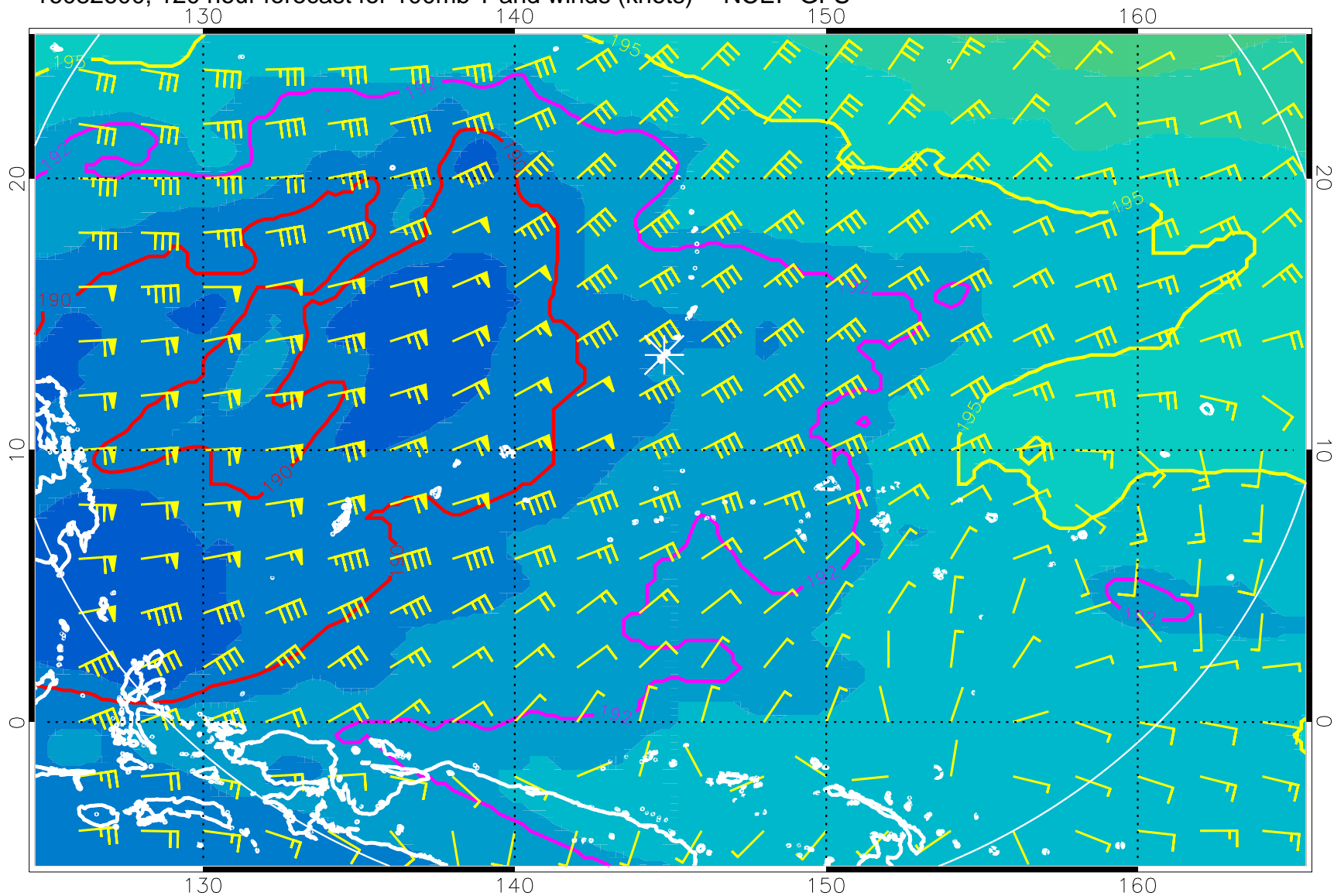
16082600, 120 hour forecast for 100mb T and winds (knots) -- NCEP GFS
