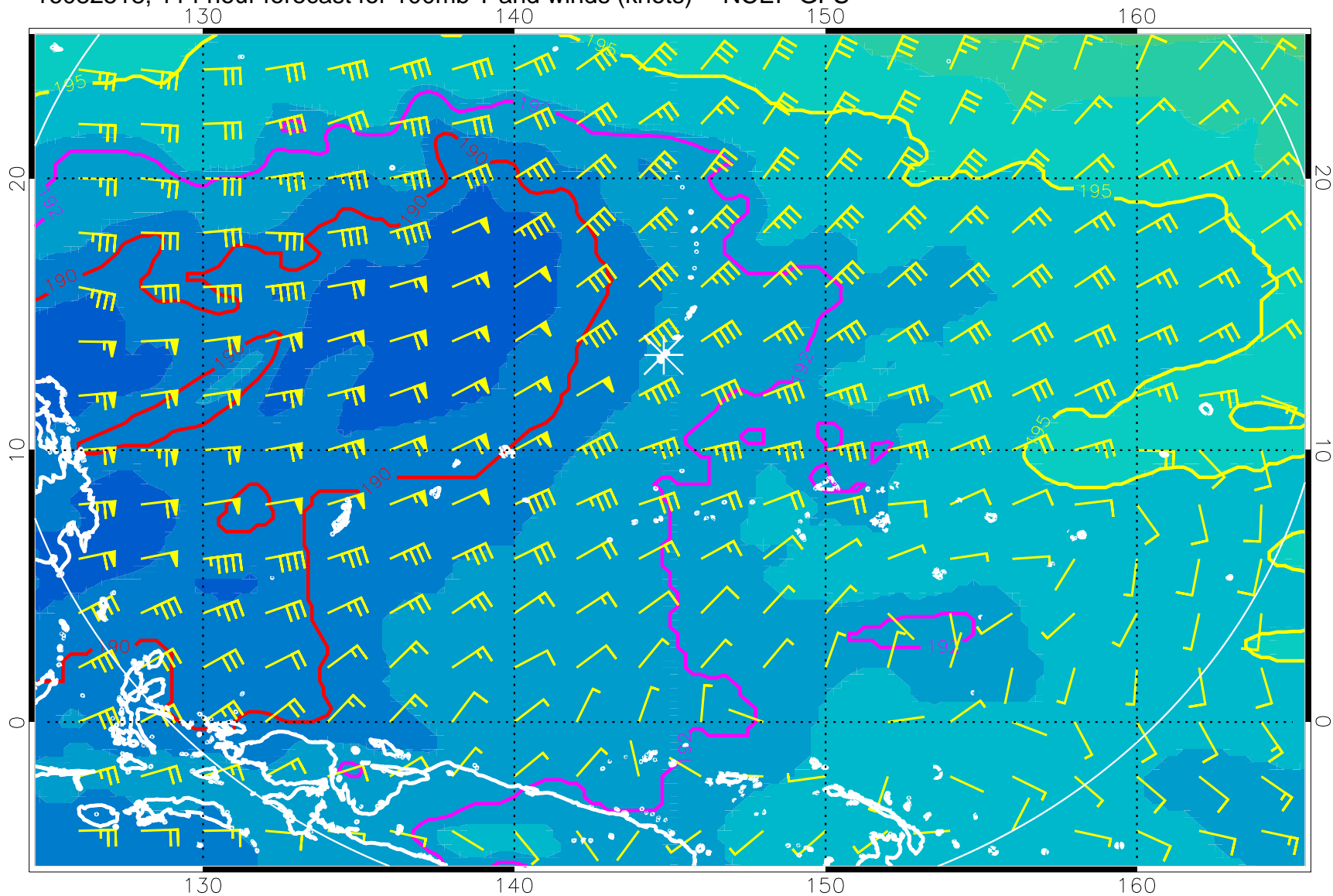
16082518, 114 hour forecast for 100mb T and winds (knots) -- NCEP GFS
