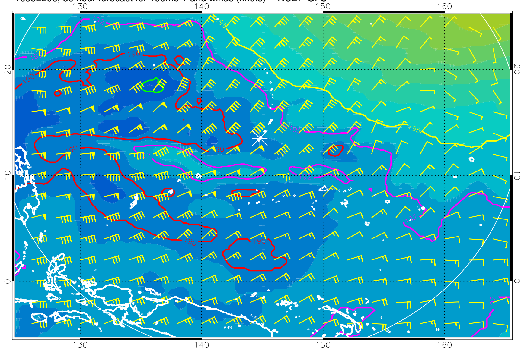
16082206, 30 hour forecast for 100mb T and winds (knots) -- NCEP GFS
