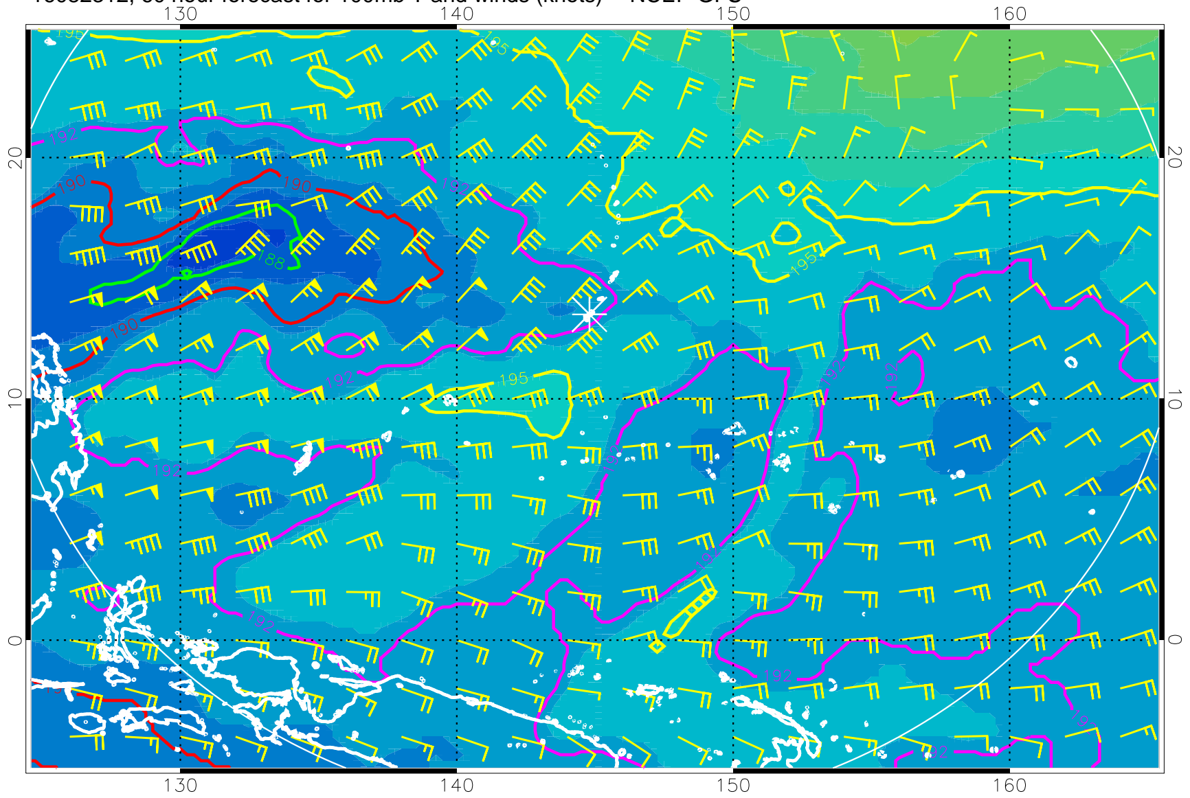
16082312, 60 hour forecast for 100mb T and winds (knots) -- NCEP GFS
