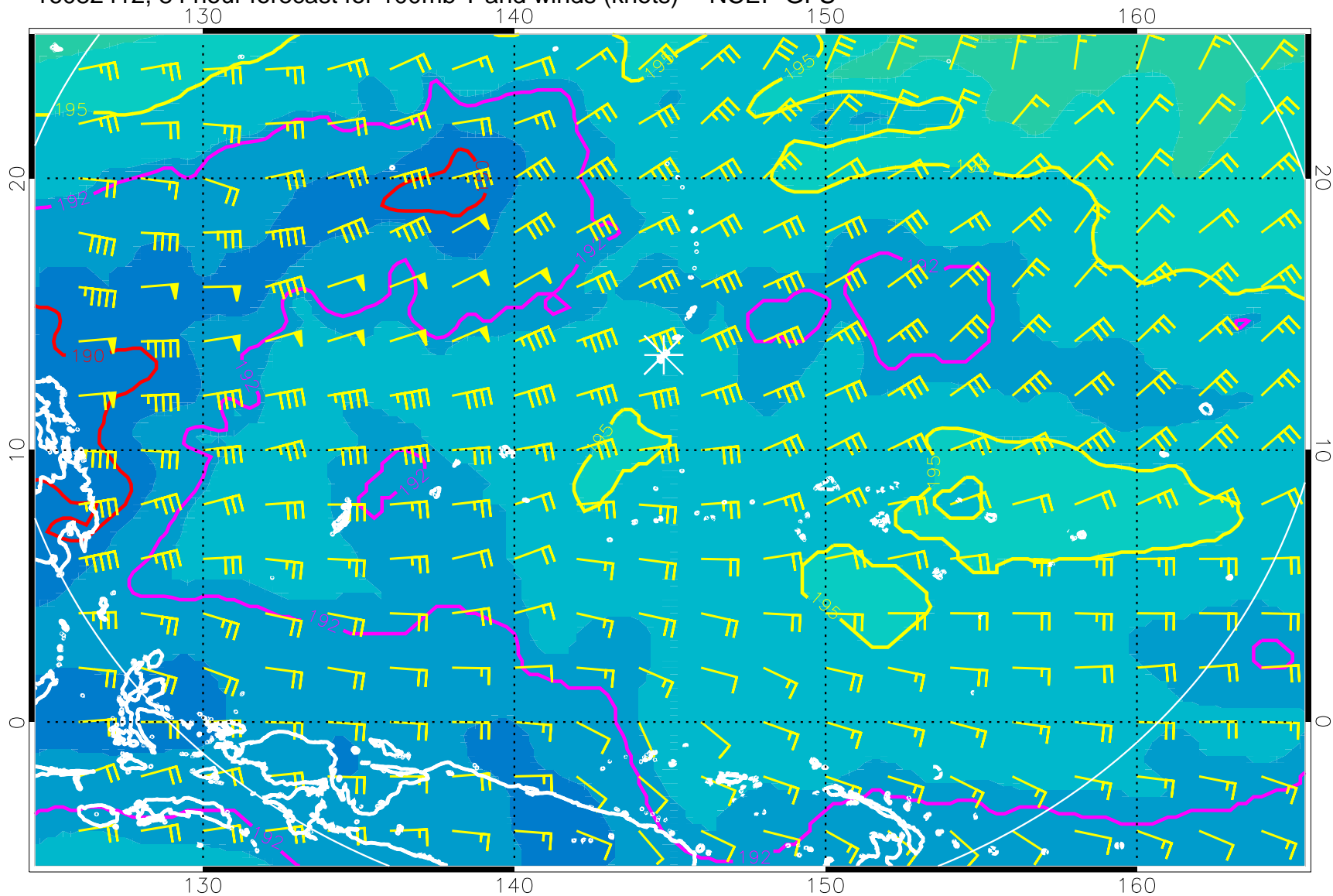
16082412, 84 hour forecast for 100mb T and winds (knots) -- NCEP GFS
