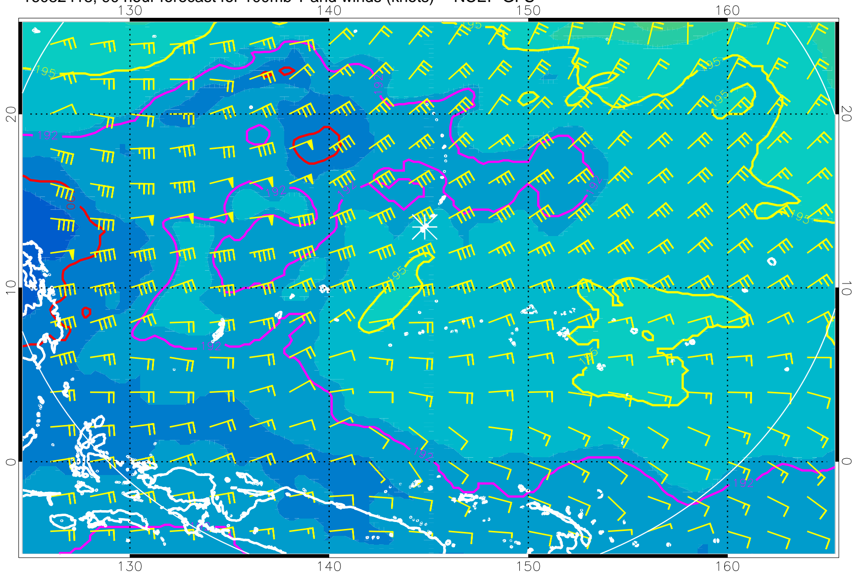
16082418, 90 hour forecast for 100mb T and winds (knots) -- NCEP GFS
