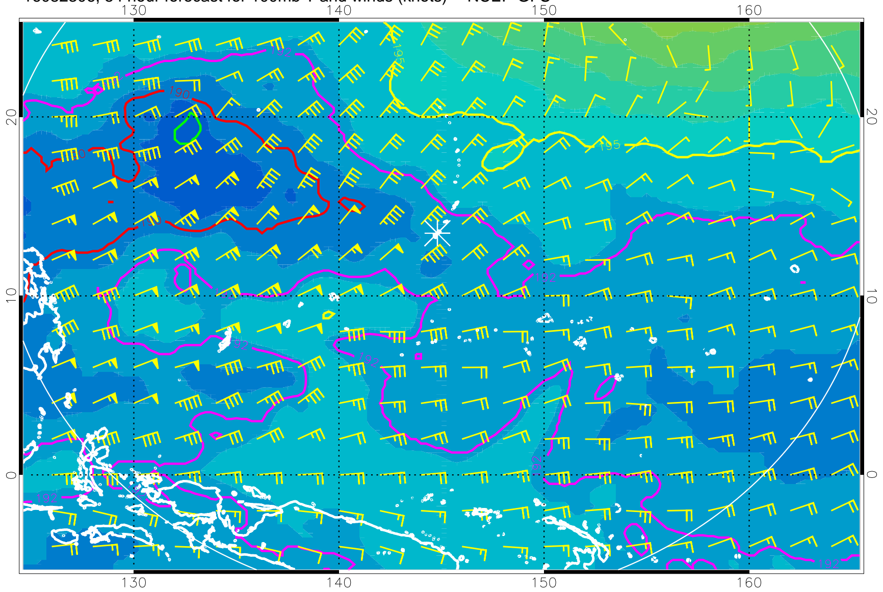
16082306, 54 hour forecast for 100mb T and winds (knots) -- NCEP GFS
