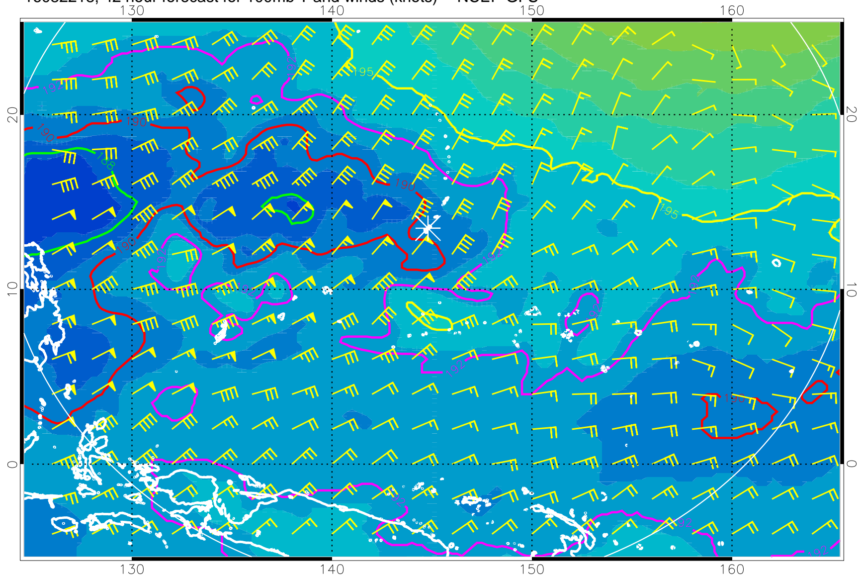
16082218, 42 hour forecast for 100mb T and winds (knots) -- NCEP GFS
