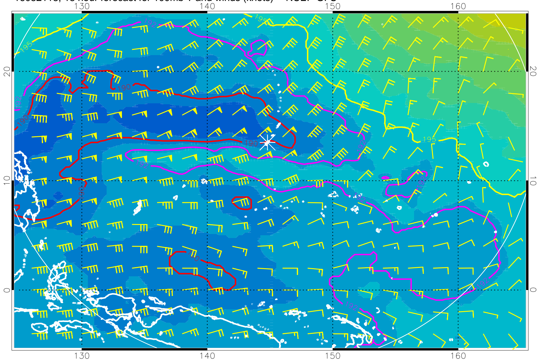
16082118, 18 hour forecast for 100mb T and winds (knots) -- NCEP GFS
