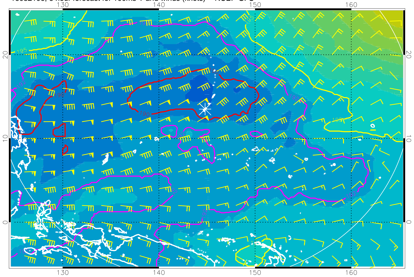
16082106, 6 hour forecast for 100mb T and winds (knots) -- NCEP GFS
