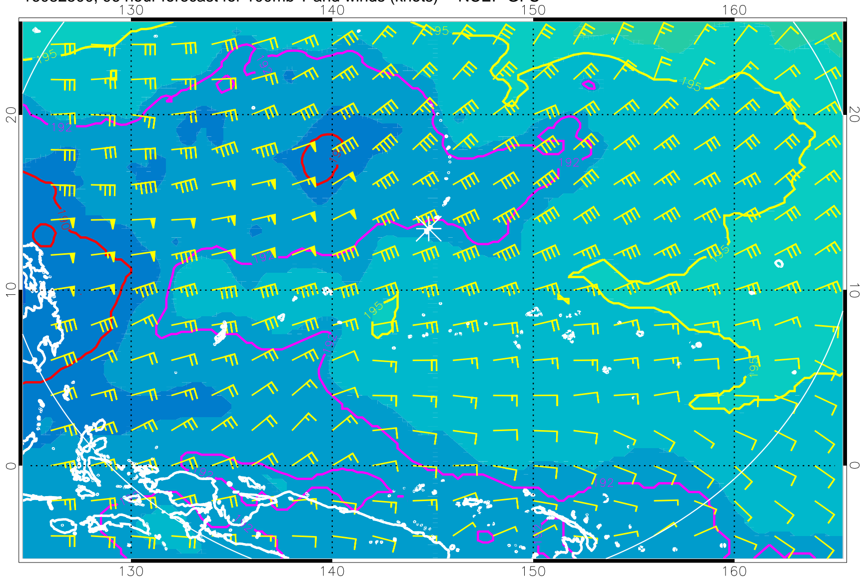
16082500, 96 hour forecast for 100mb T and winds (knots) -- NCEP GFS
