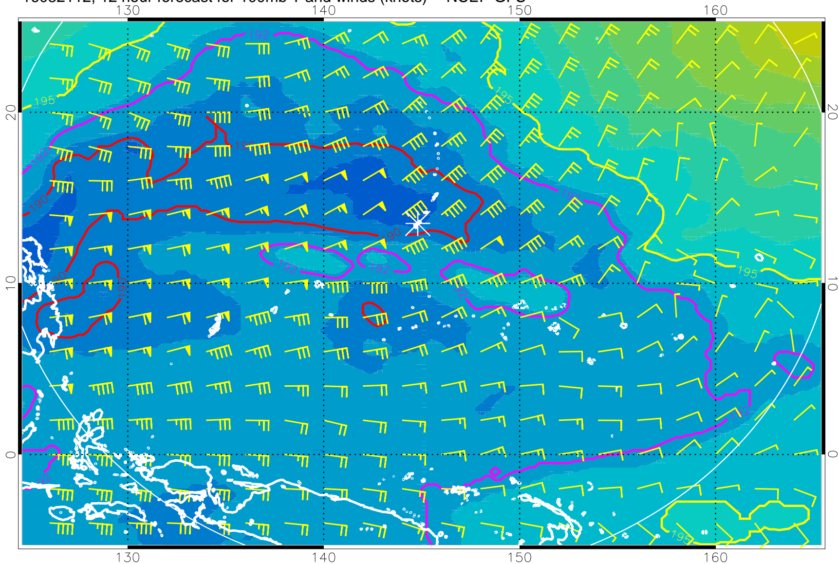
16082112, 12 hour forecast for 100mb T and winds (knots) -- NCEP GFS
