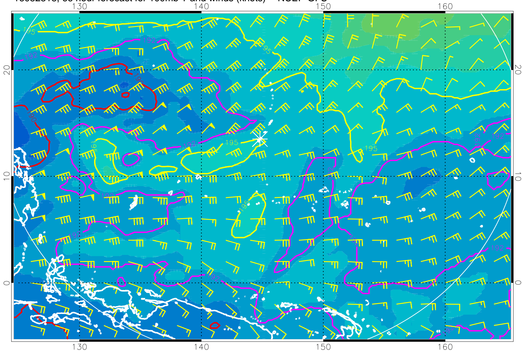
16082318, 66 hour forecast for 100mb T and winds (knots) -- NCEP GFS
