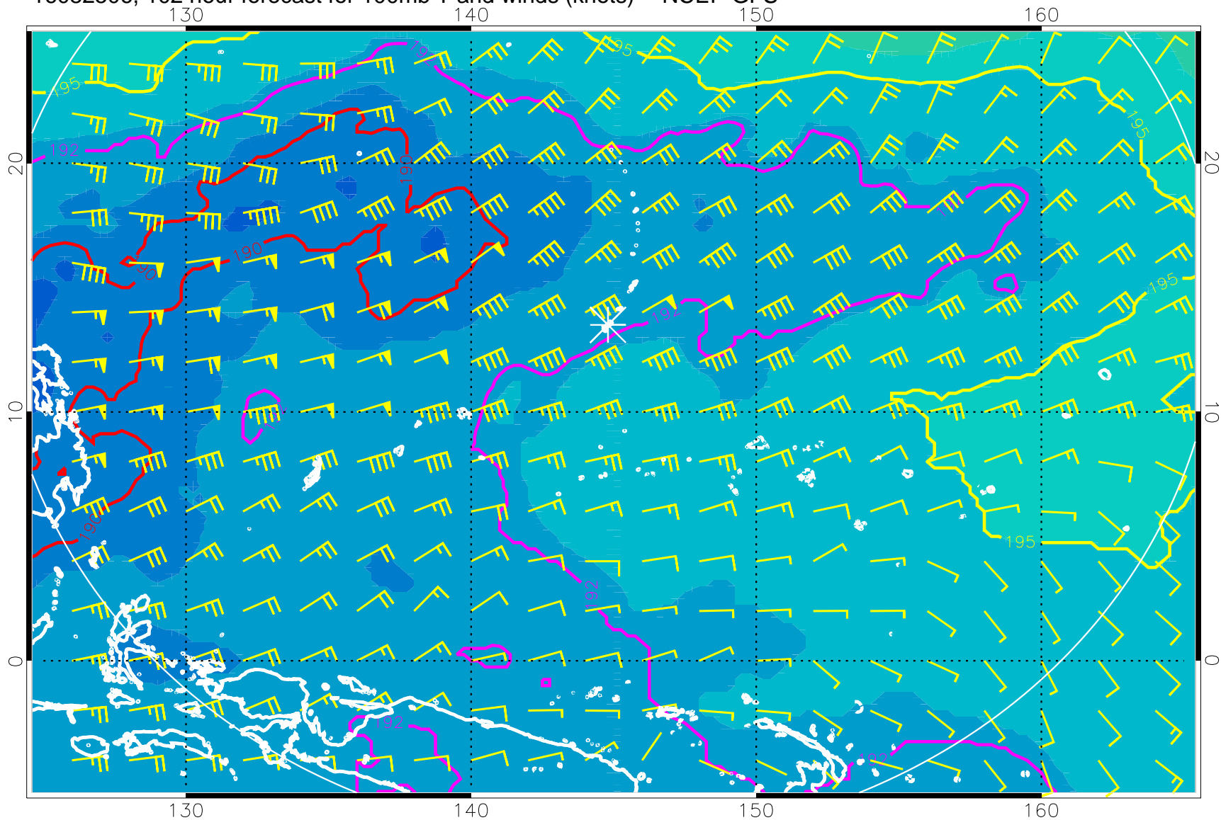
16082506, 102 hour forecast for 100mb T and winds (knots) -- NCEP GFS
