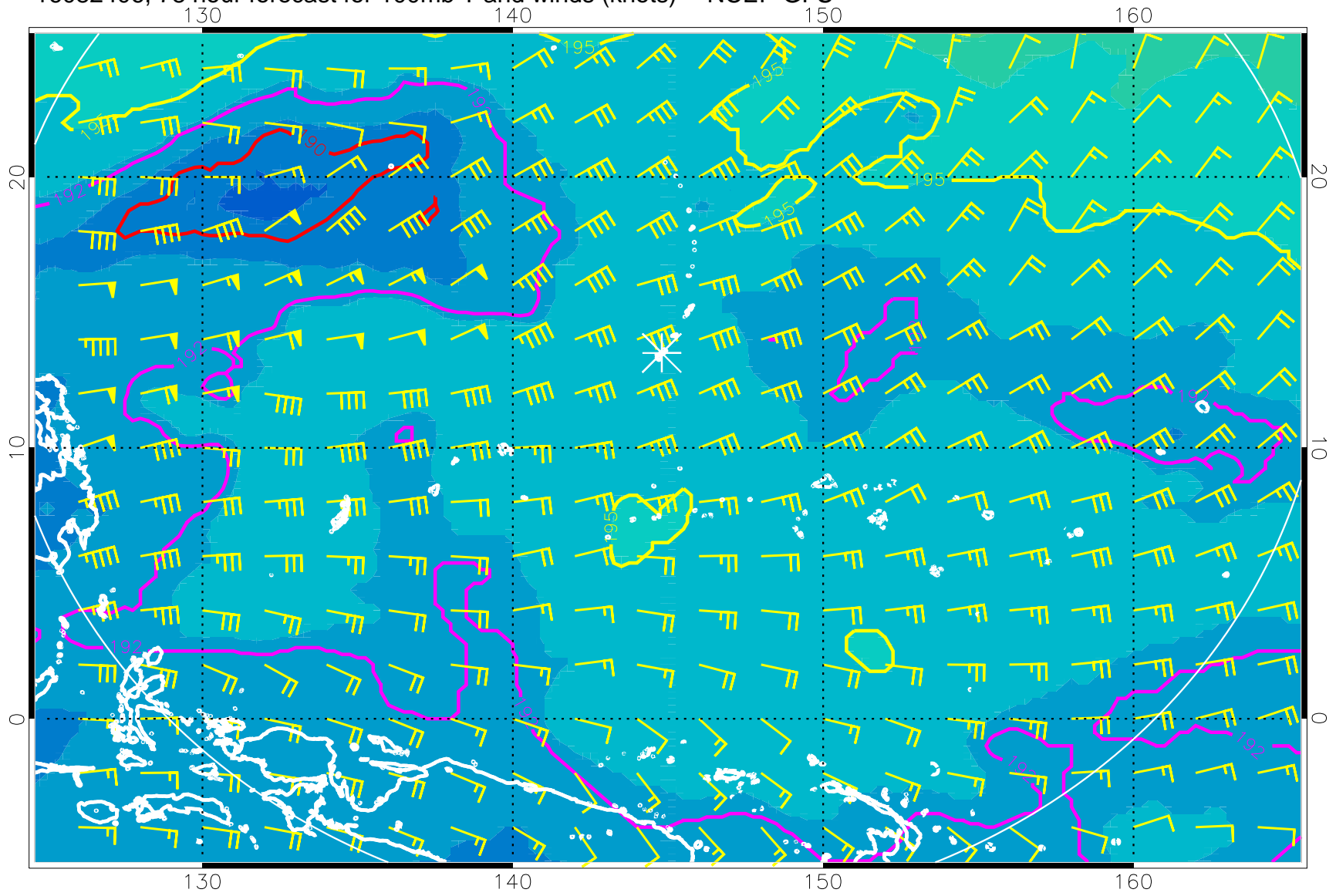
16082406, 78 hour forecast for 100mb T and winds (knots) -- NCEP GFS
