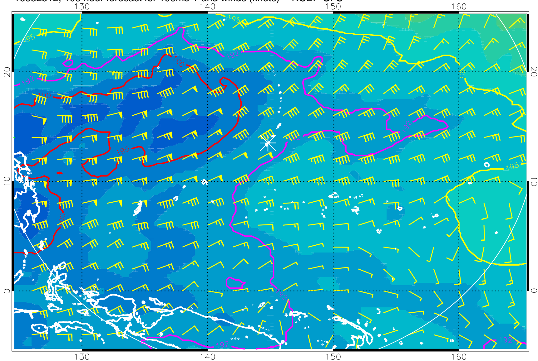
16082512, 108 hour forecast for 100mb T and winds (knots) -- NCEP GFS
