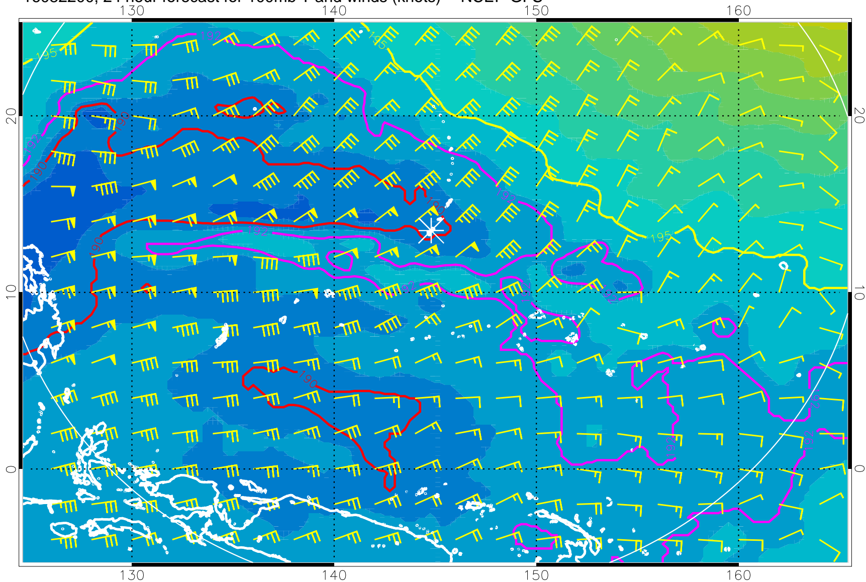
16082200, 24 hour forecast for 100mb T and winds (knots) -- NCEP GFS
