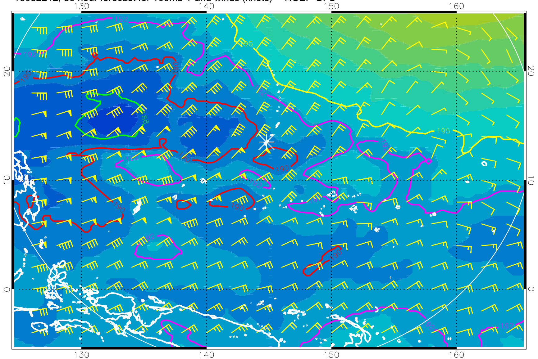
16082212, 36 hour forecast for 100mb T and winds (knots) -- NCEP GFS
