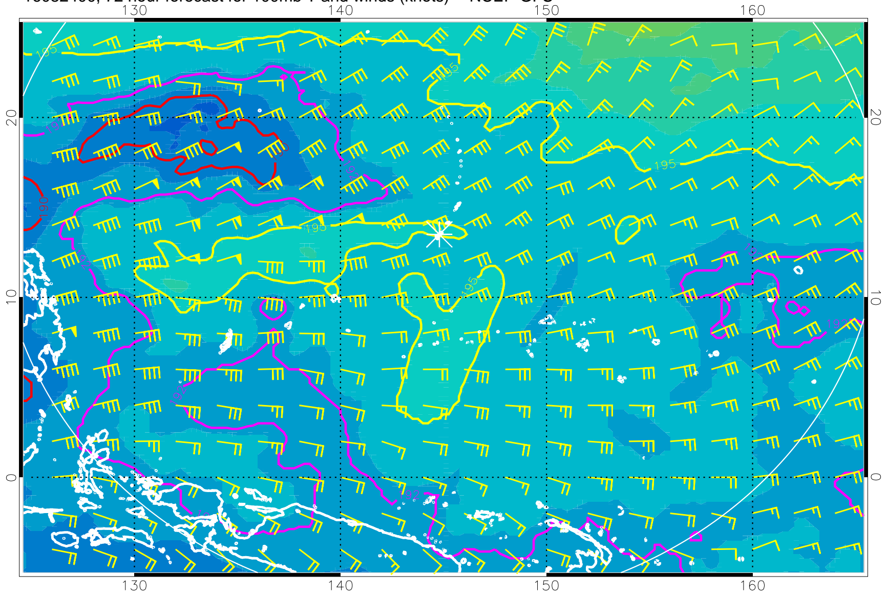
16082400, 72 hour forecast for 100mb T and winds (knots) -- NCEP GFS
