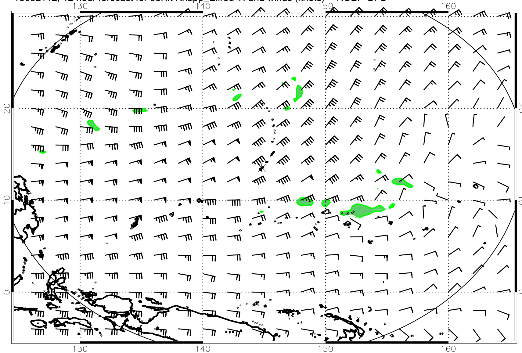
16082112, 12 hour forecast for 53Kft Knapp_Ellrod TI and winds (knots) -- NCEP GFS
