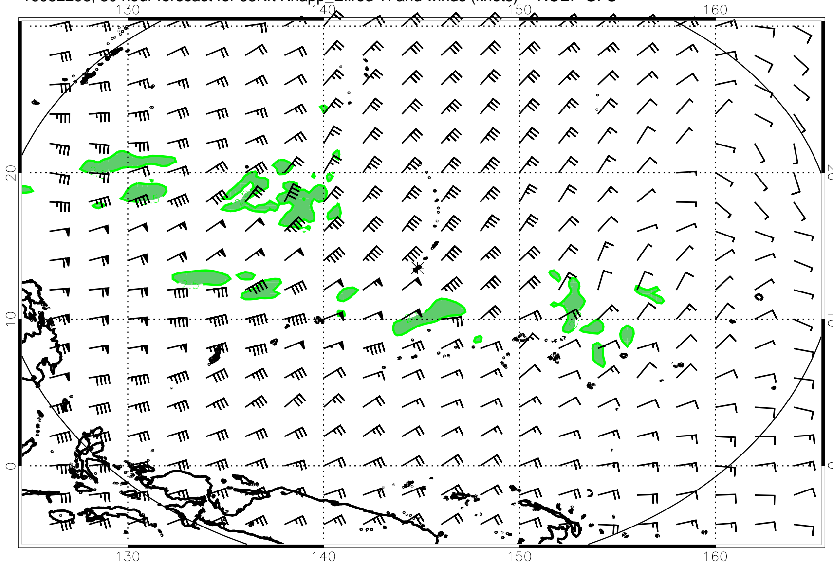
16082206, 30 hour forecast for 53Kft Knapp_Ellrod TI and winds (knots) -- NCEP GFS
