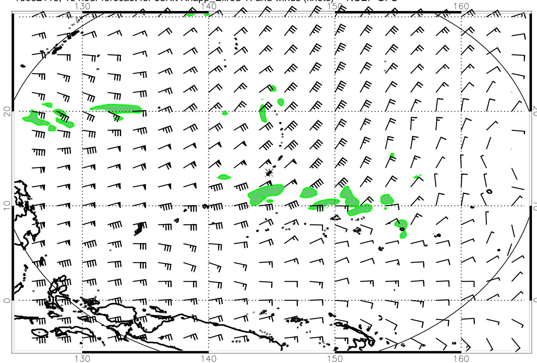
16082118, 18 hour forecast for 53Kft Knapp_Ellrod TI and winds (knots) -- NCEP GFS
