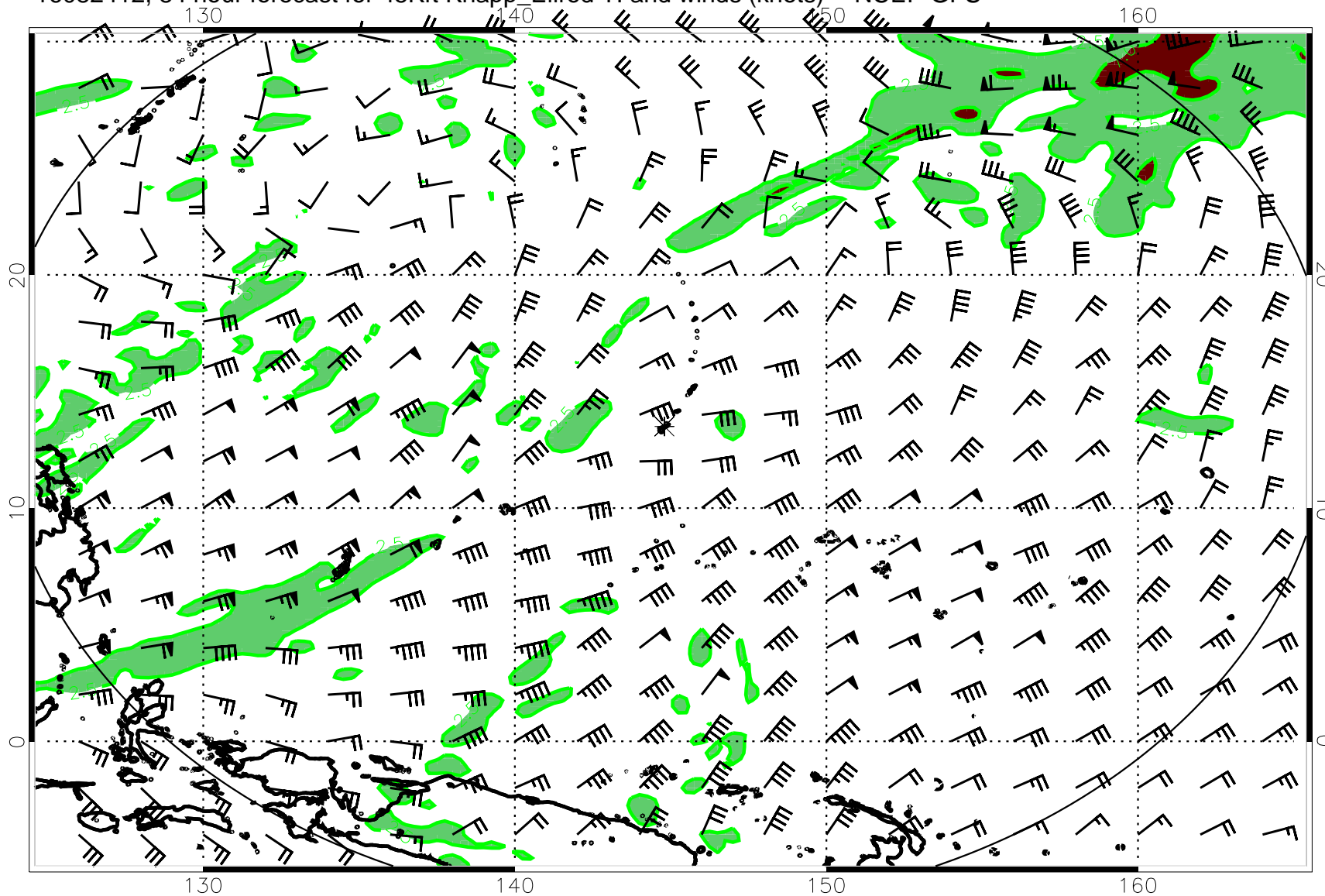
16082412, 84 hour forecast for 45Kft Knapp_Ellrod TI and winds (knots) -- NCEP GFS
