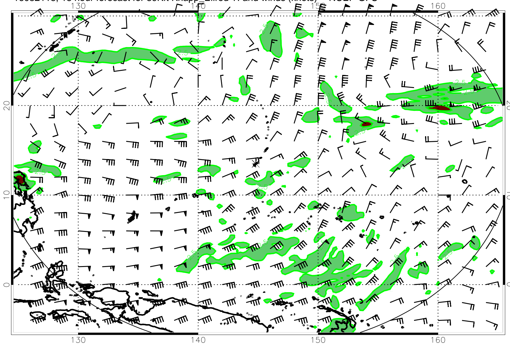
16082118, 18 hour forecast for 39Kft Knapp_Ellrod TI and winds (knots) -- NCEP GFS
