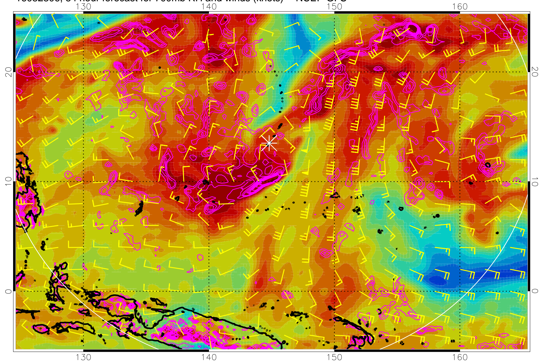
16082306, 54 hour forecast for 700mb RH and winds (knots) -- NCEP GFS
