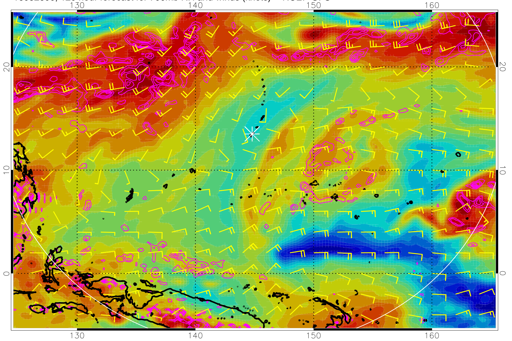
16082600, 120 hour forecast for 700mb RH and winds (knots) -- NCEP GFS
