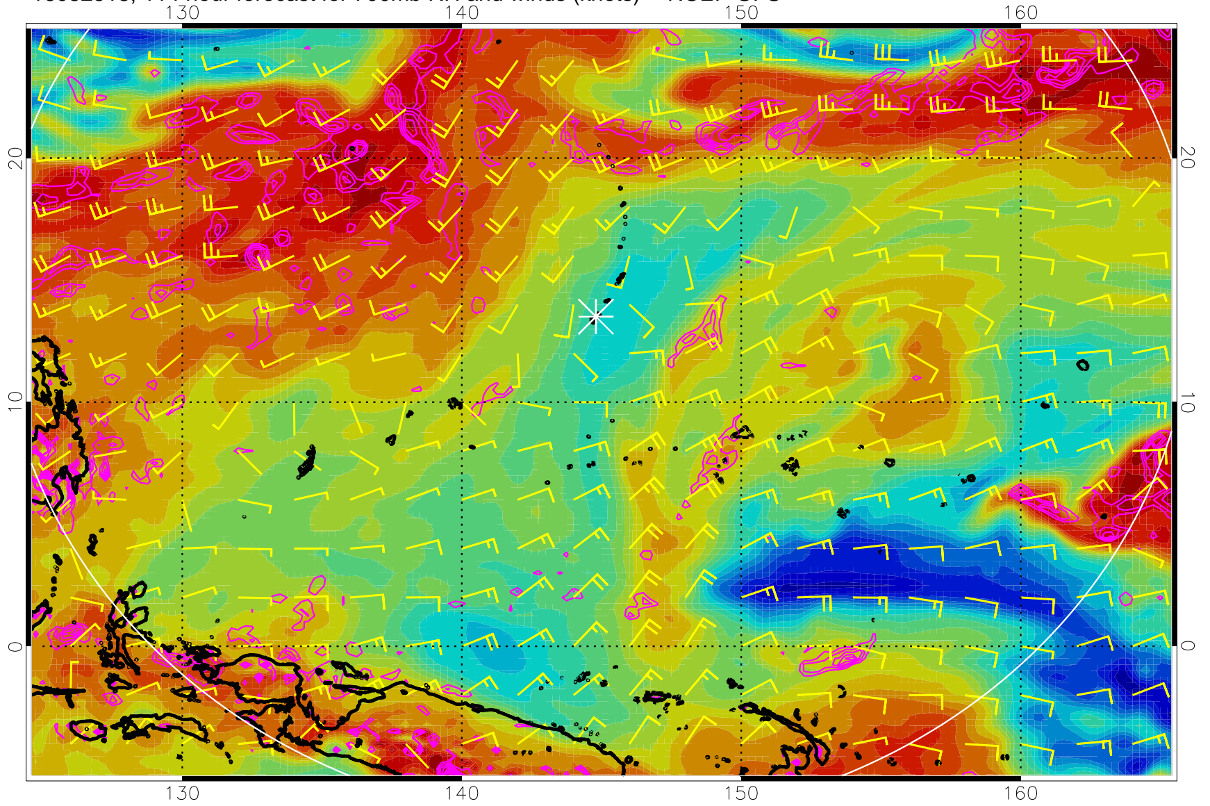
16082518, 114 hour forecast for 700mb RH and winds (knots) -- NCEP GFS
