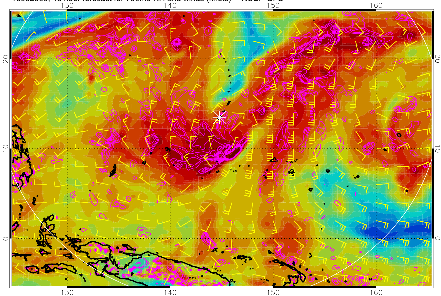
16082300, 48 hour forecast for 700mb RH and winds (knots) -- NCEP GFS
