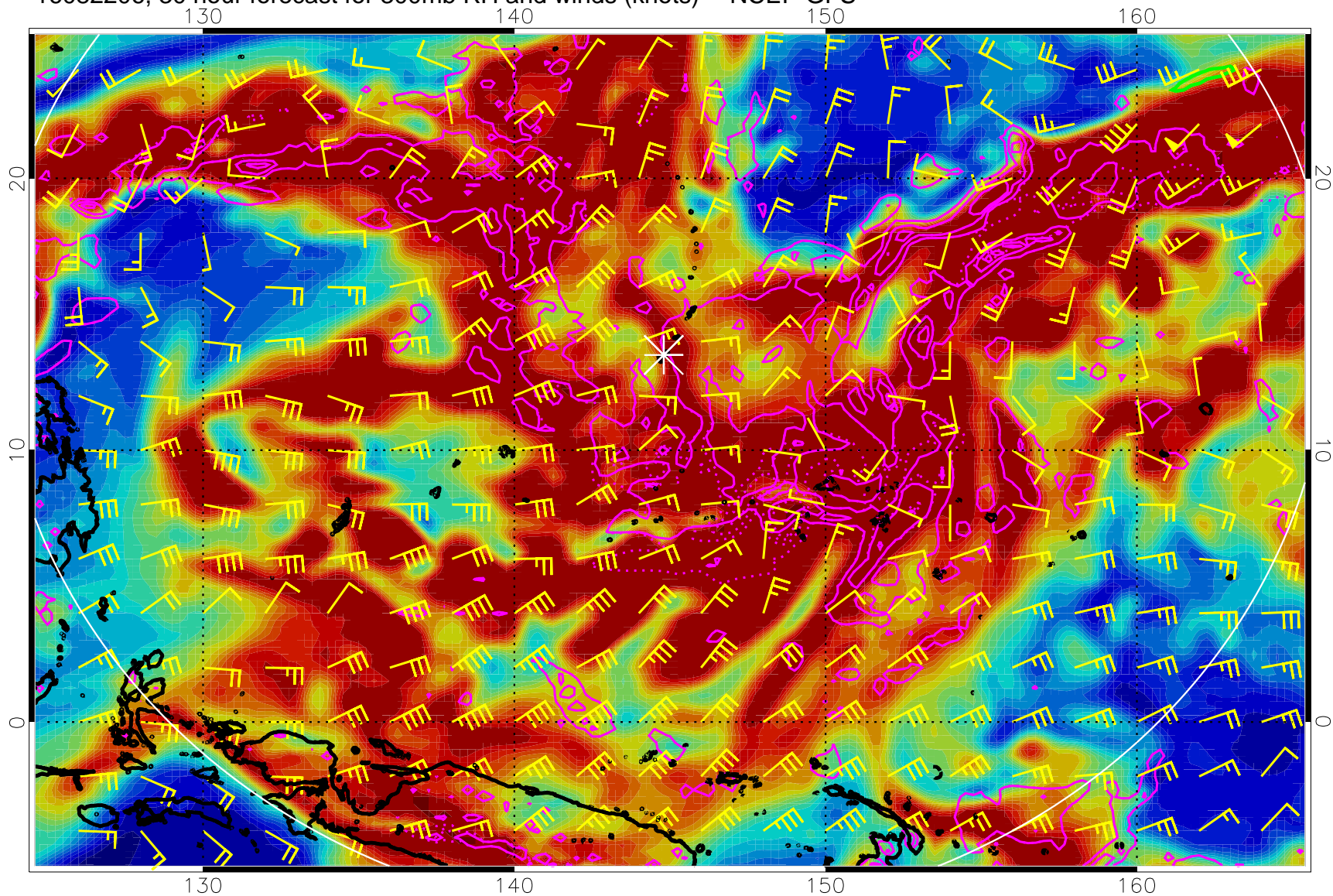
16082206, 30 hour forecast for 300mb RH and winds (knots) -- NCEP GFS
