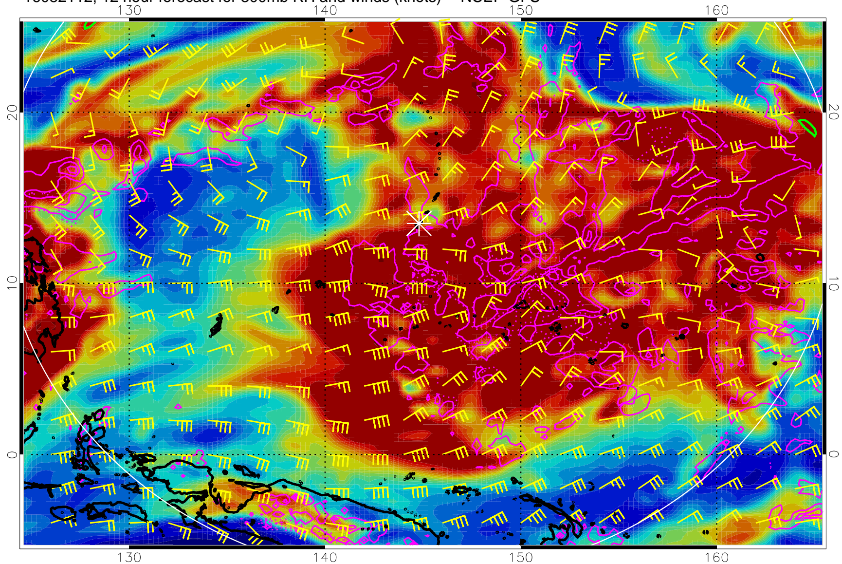
16082112, 12 hour forecast for 300mb RH and winds (knots) -- NCEP GFS
