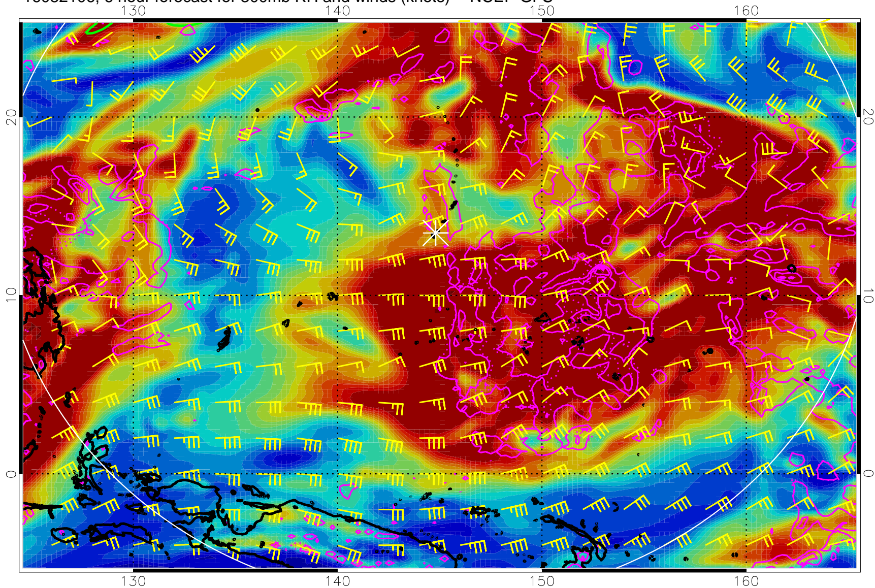
16082106, 6 hour forecast for 300mb RH and winds (knots) -- NCEP GFS
