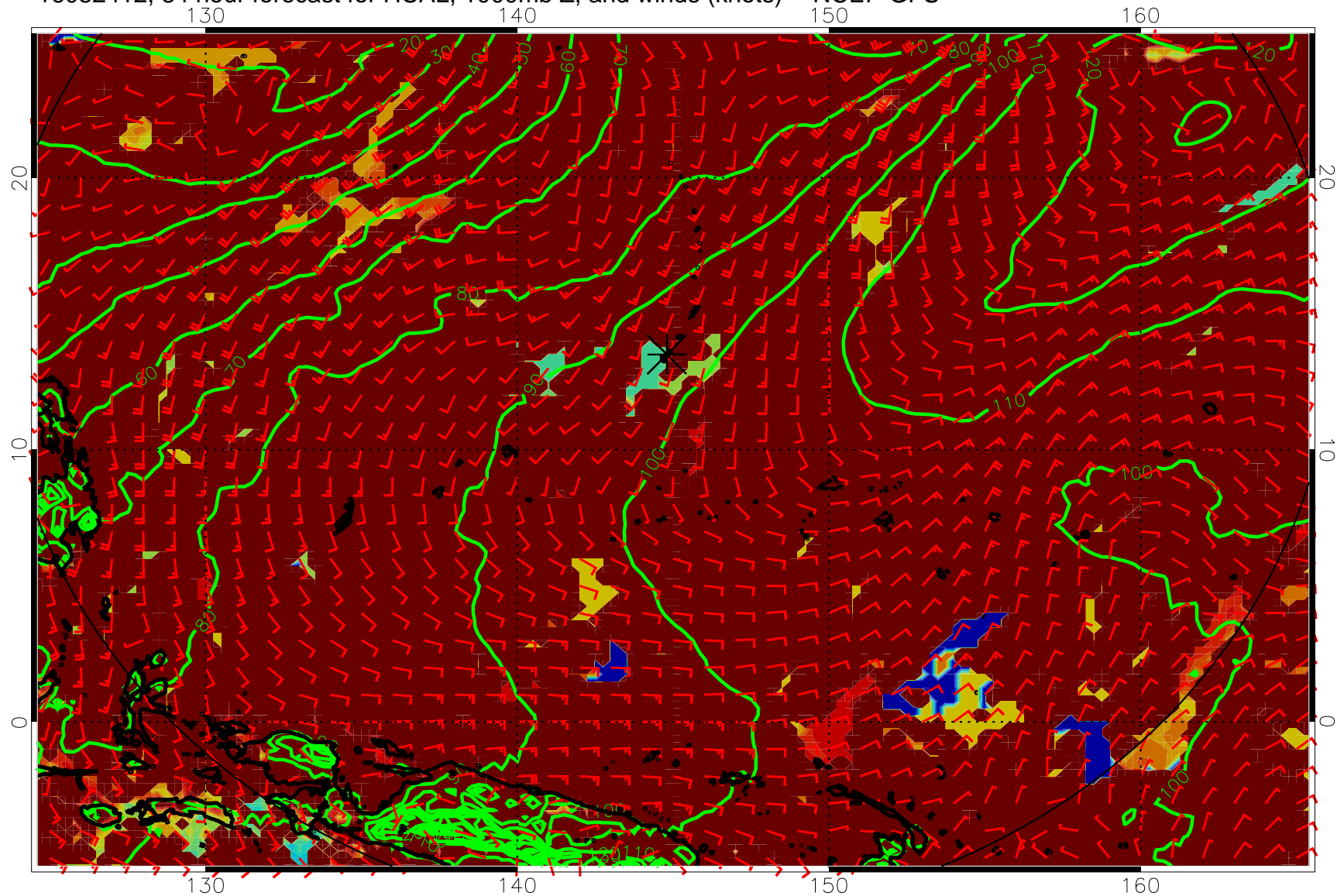
16082412, 84 hour forecast for HCAL, 1000mb Z, and winds (knots) -- NCEP GFS
