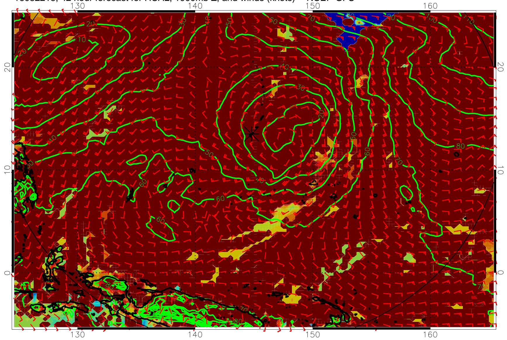
16082218, 42 hour forecast for HCAL, 1000mb Z, and winds (knots) -- NCEP GFS
