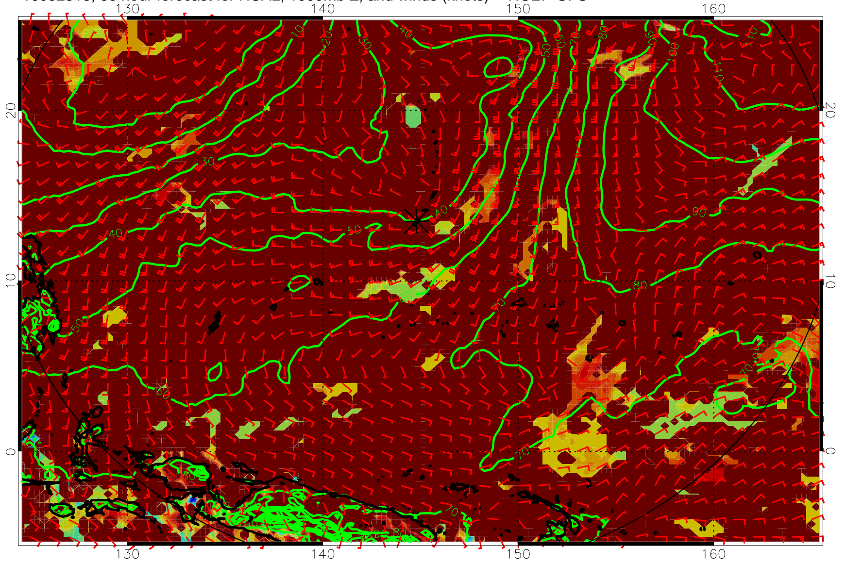
16082318, 66 hour forecast for HCAL, 1000mb Z, and winds (knots) -- NCEP GFS
