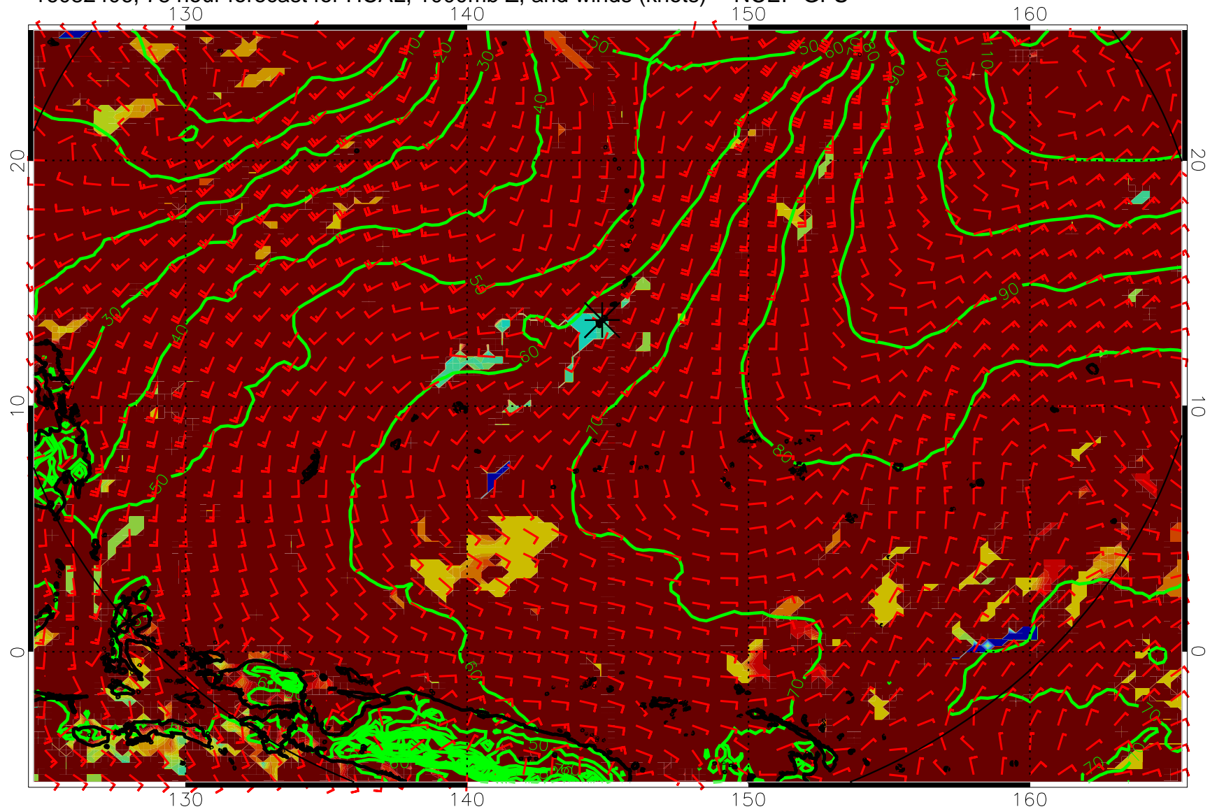
16082406, 78 hour forecast for HCAL, 1000mb Z, and winds (knots) -- NCEP GFS
