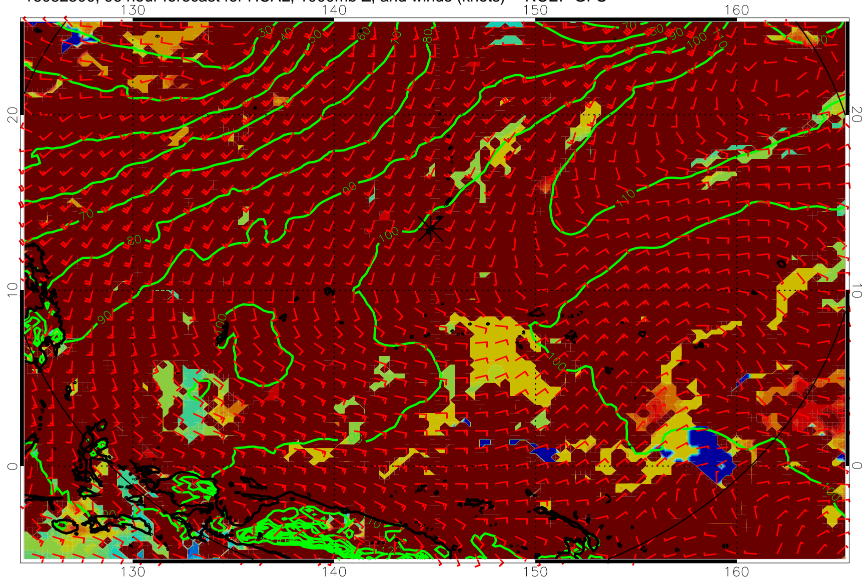
16082500, 96 hour forecast for HCAL, 1000mb Z, and winds (knots) -- NCEP GFS
