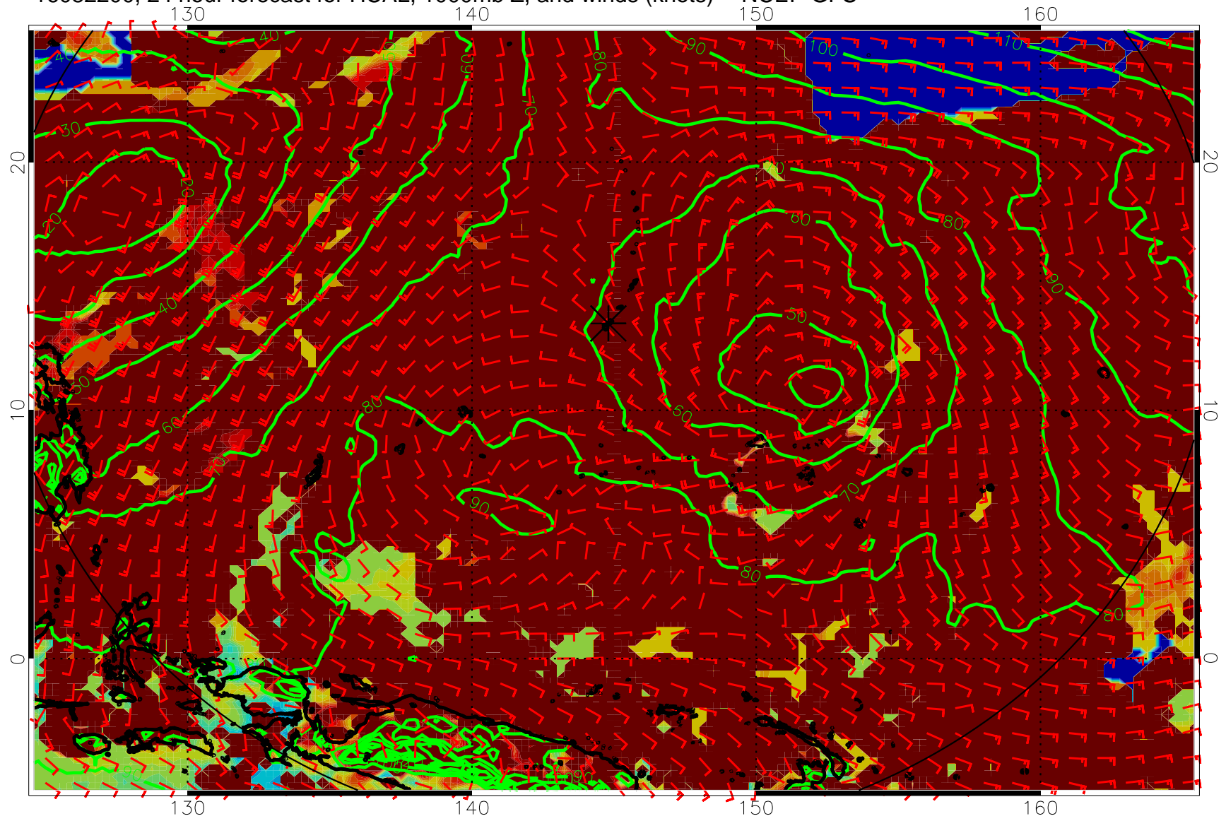
16082200, 24 hour forecast for HCAL, 1000mb Z, and winds (knots) -- NCEP GFS
