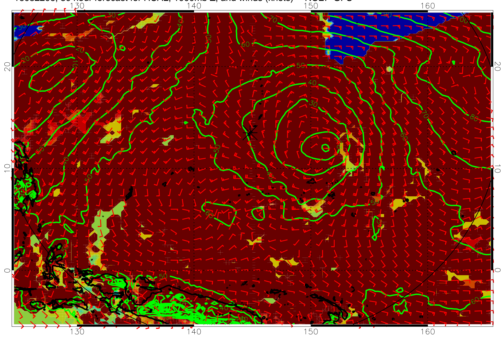
16082206, 30 hour forecast for HCAL, 1000mb Z, and winds (knots) -- NCEP GFS
