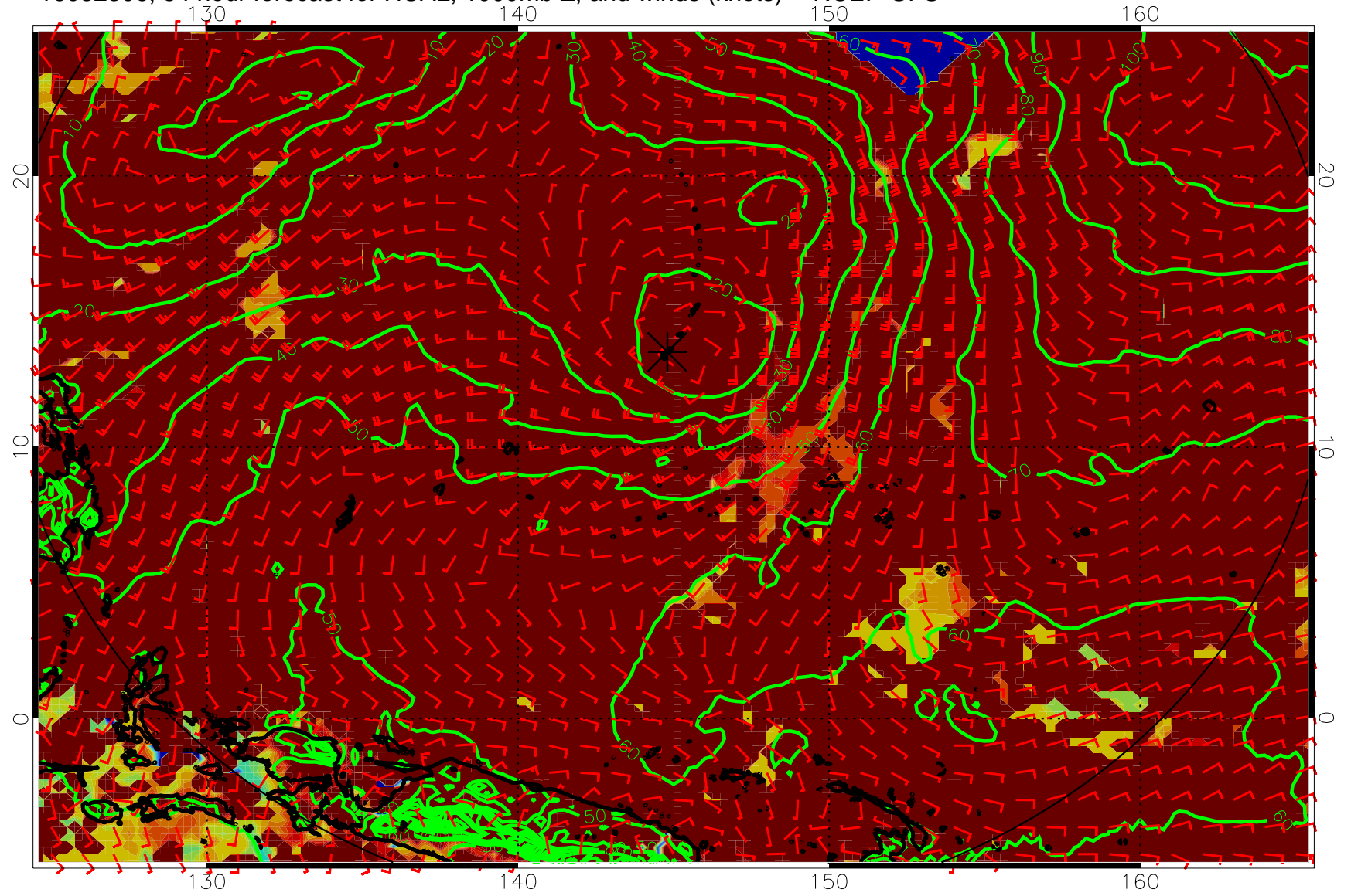
16082306, 54 hour forecast for HCAL, 1000mb Z, and winds (knots) -- NCEP GFS
