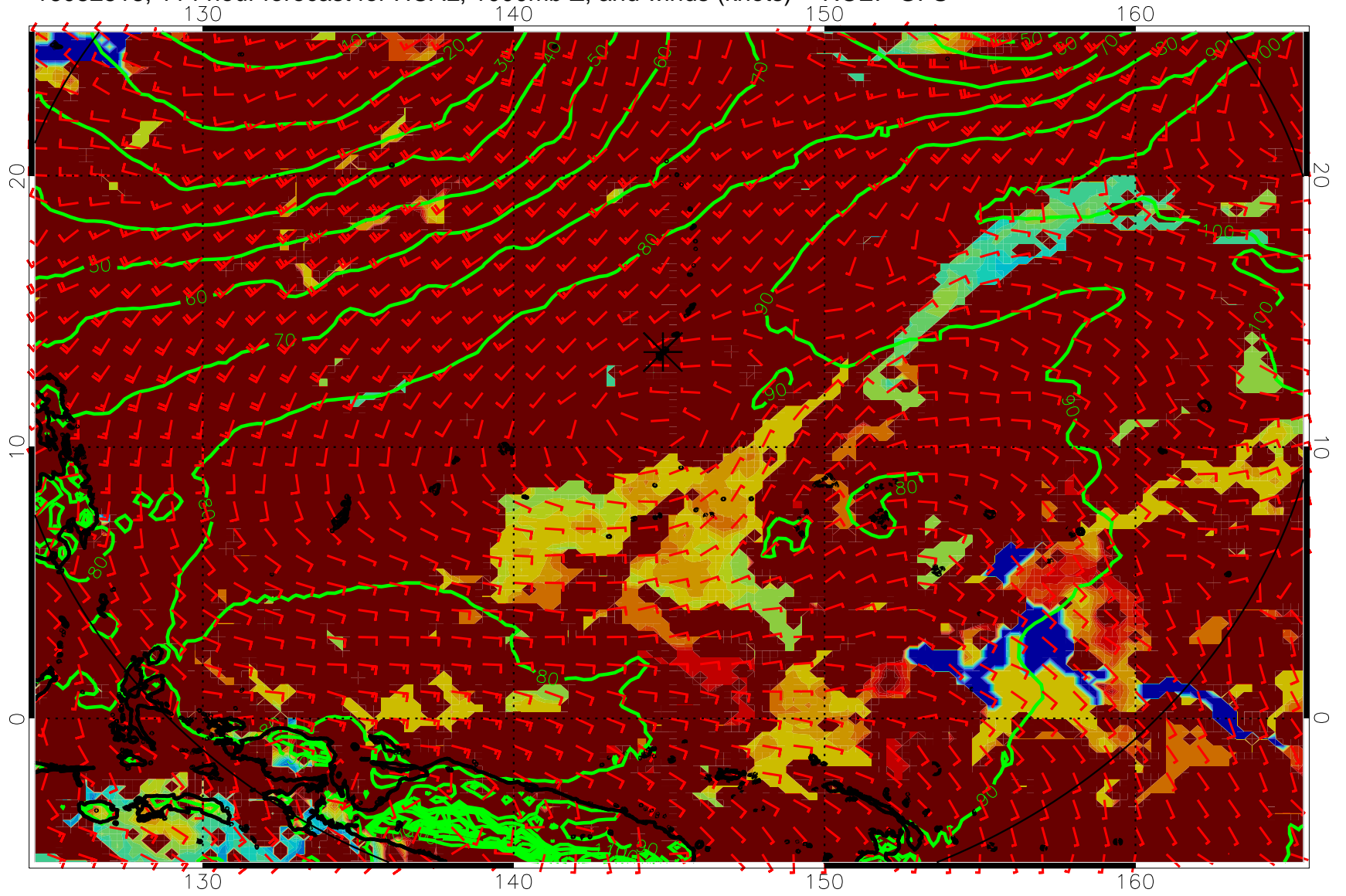
16082518, 114 hour forecast for HCAL, 1000mb Z, and winds (knots) -- NCEP GFS
