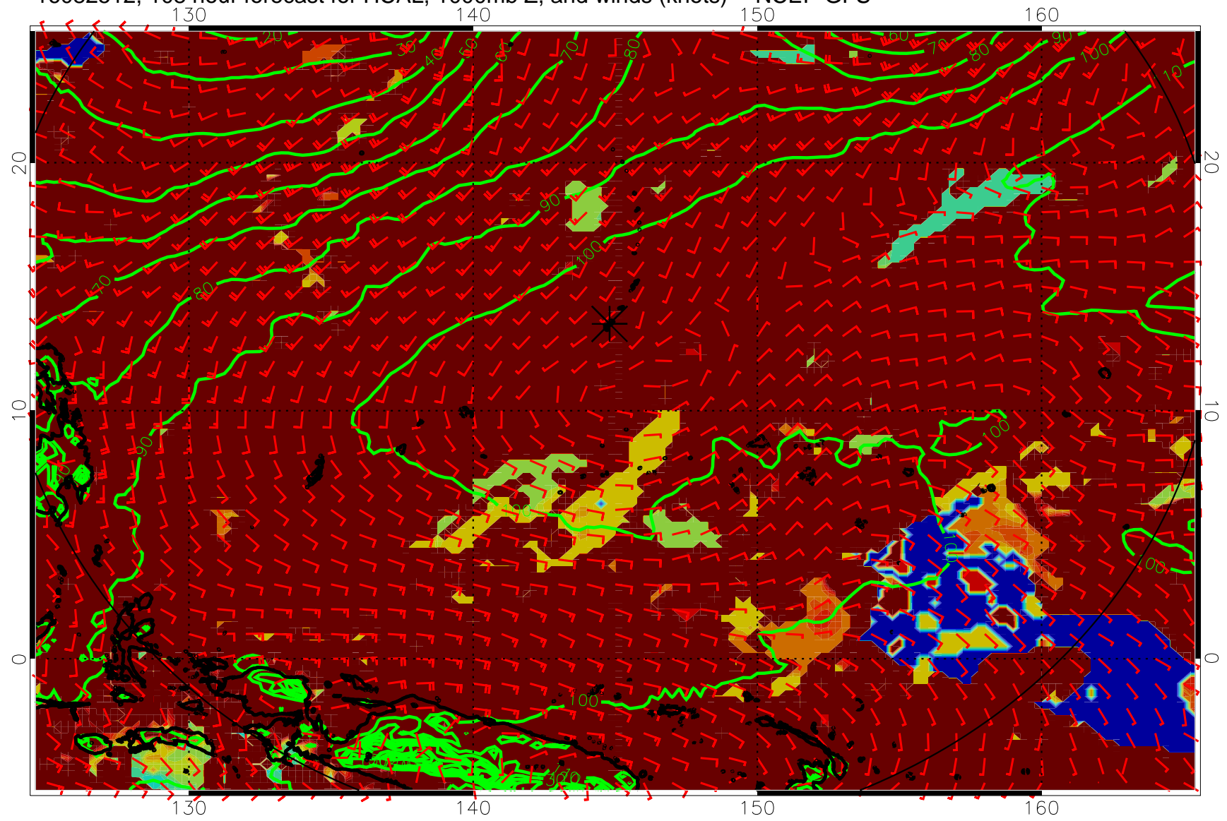
16082512, 108 hour forecast for HCAL, 1000mb Z, and winds (knots) -- NCEP GFS
