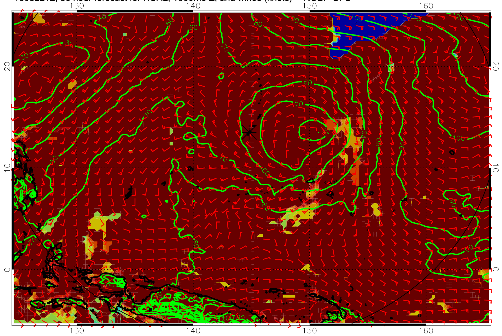
16082212, 36 hour forecast for HCAL, 1000mb Z, and winds (knots) -- NCEP GFS
