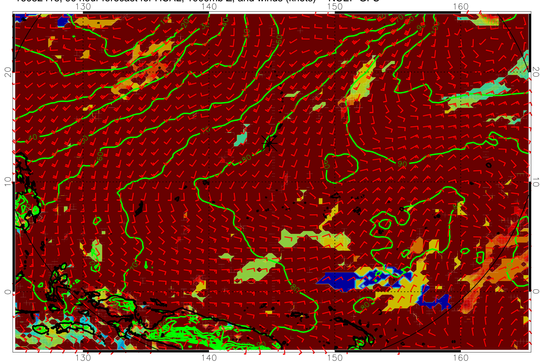
16082418, 90 hour forecast for HCAL, 1000mb Z, and winds (knots) -- NCEP GFS
