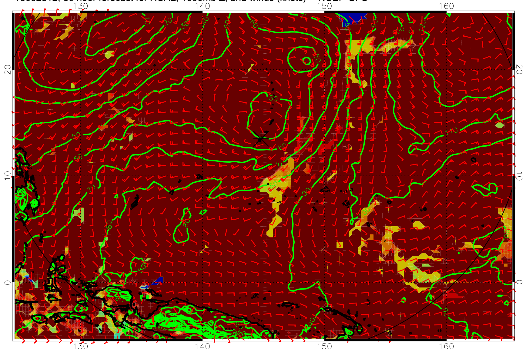
16082312, 60 hour forecast for HCAL, 1000mb Z, and winds (knots) -- NCEP GFS
