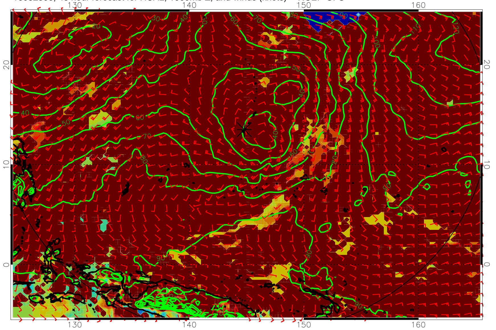
16082300, 48 hour forecast for HCAL, 1000mb Z, and winds (knots) -- NCEP GFS
