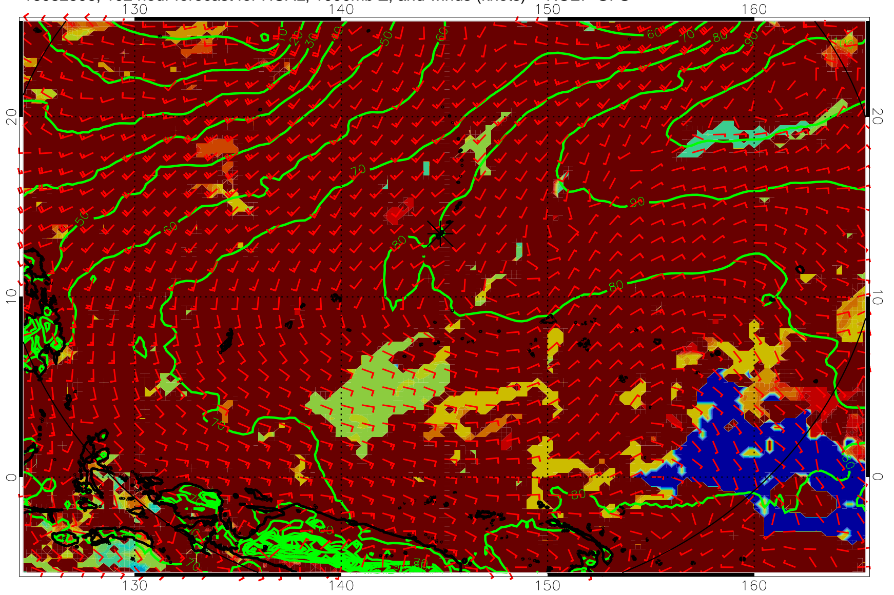
16082506, 102 hour forecast for HCAL, 1000mb Z, and winds (knots) -- NCEP GFS
