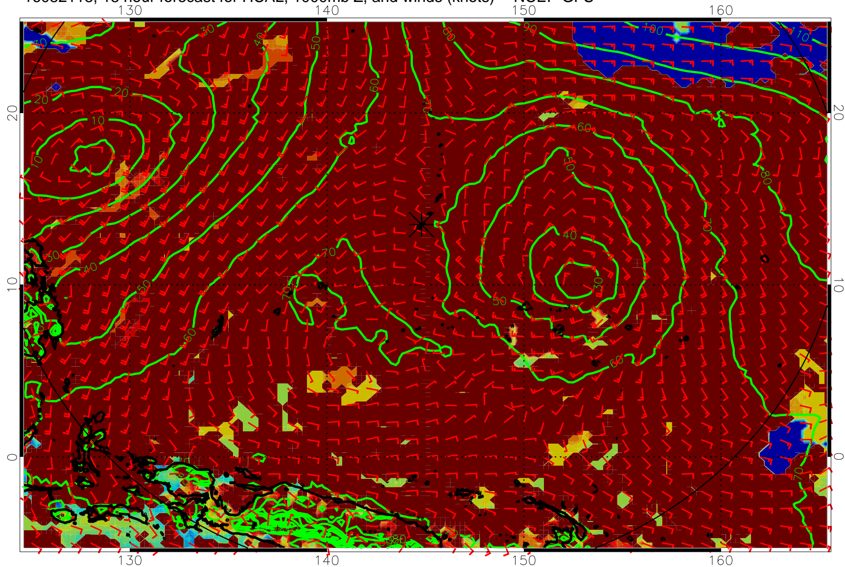
16082118, 18 hour forecast for HCAL, 1000mb Z, and winds (knots) -- NCEP GFS
