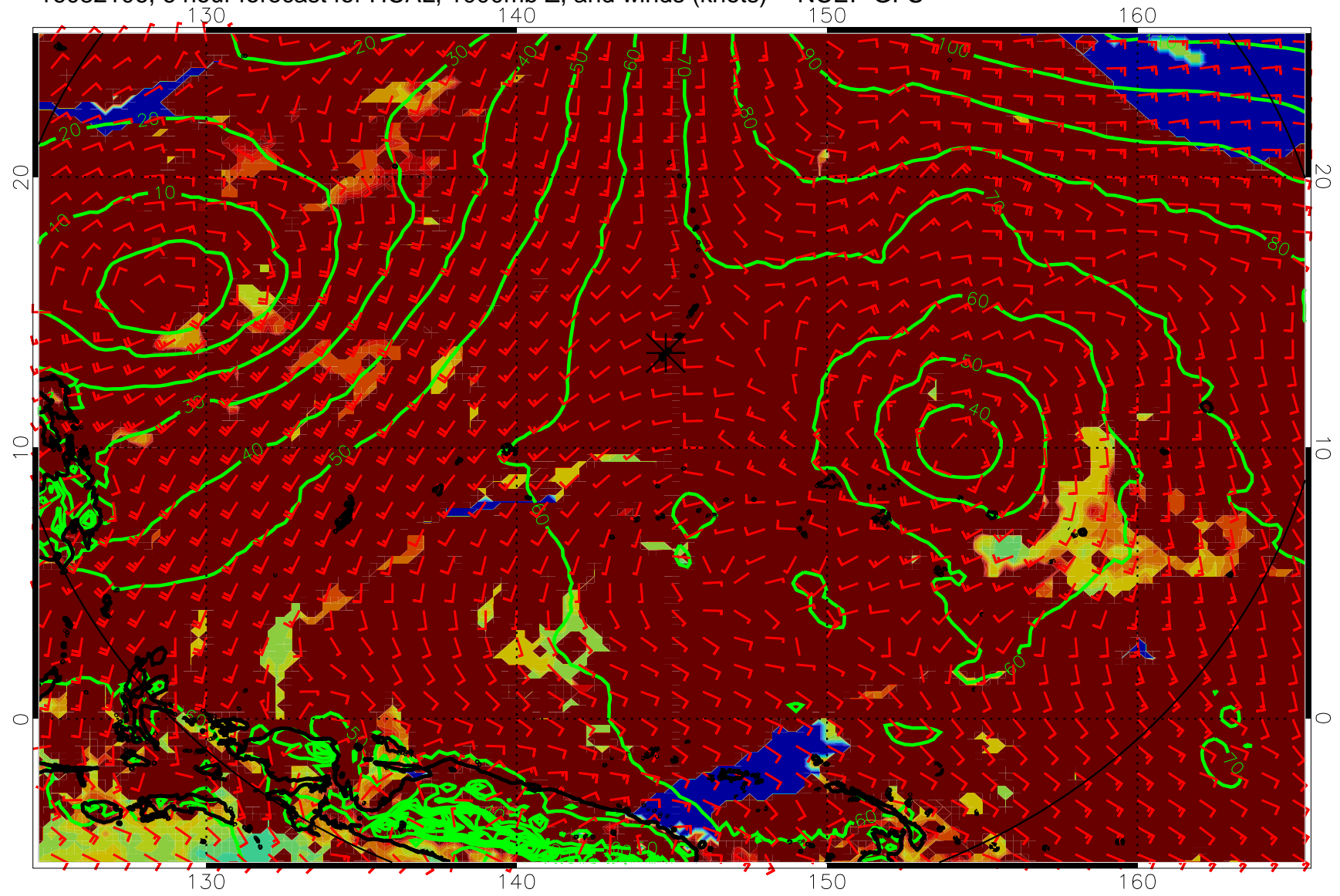
16082106, 6 hour forecast for HCAL, 1000mb Z, and winds (knots) -- NCEP GFS
