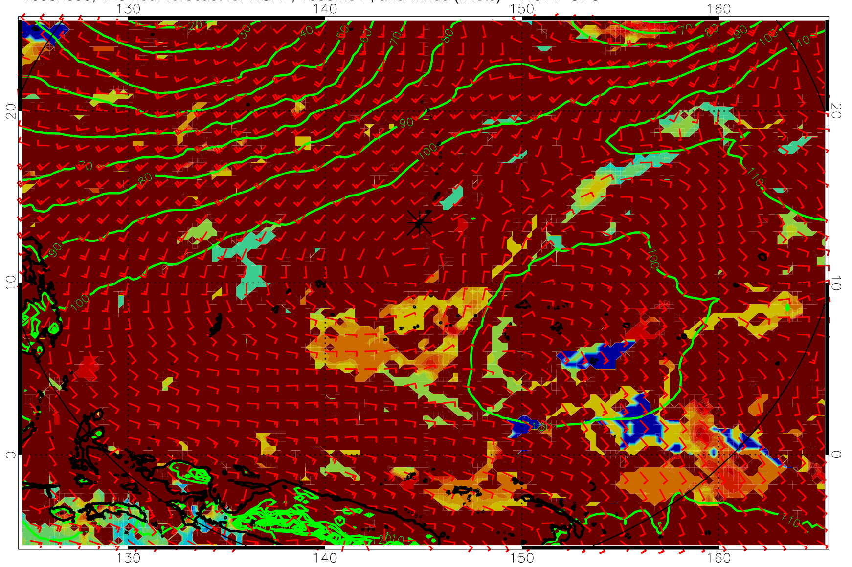
16082600, 120 hour forecast for HCAL, 1000mb Z, and winds (knots) -- NCEP GFS
