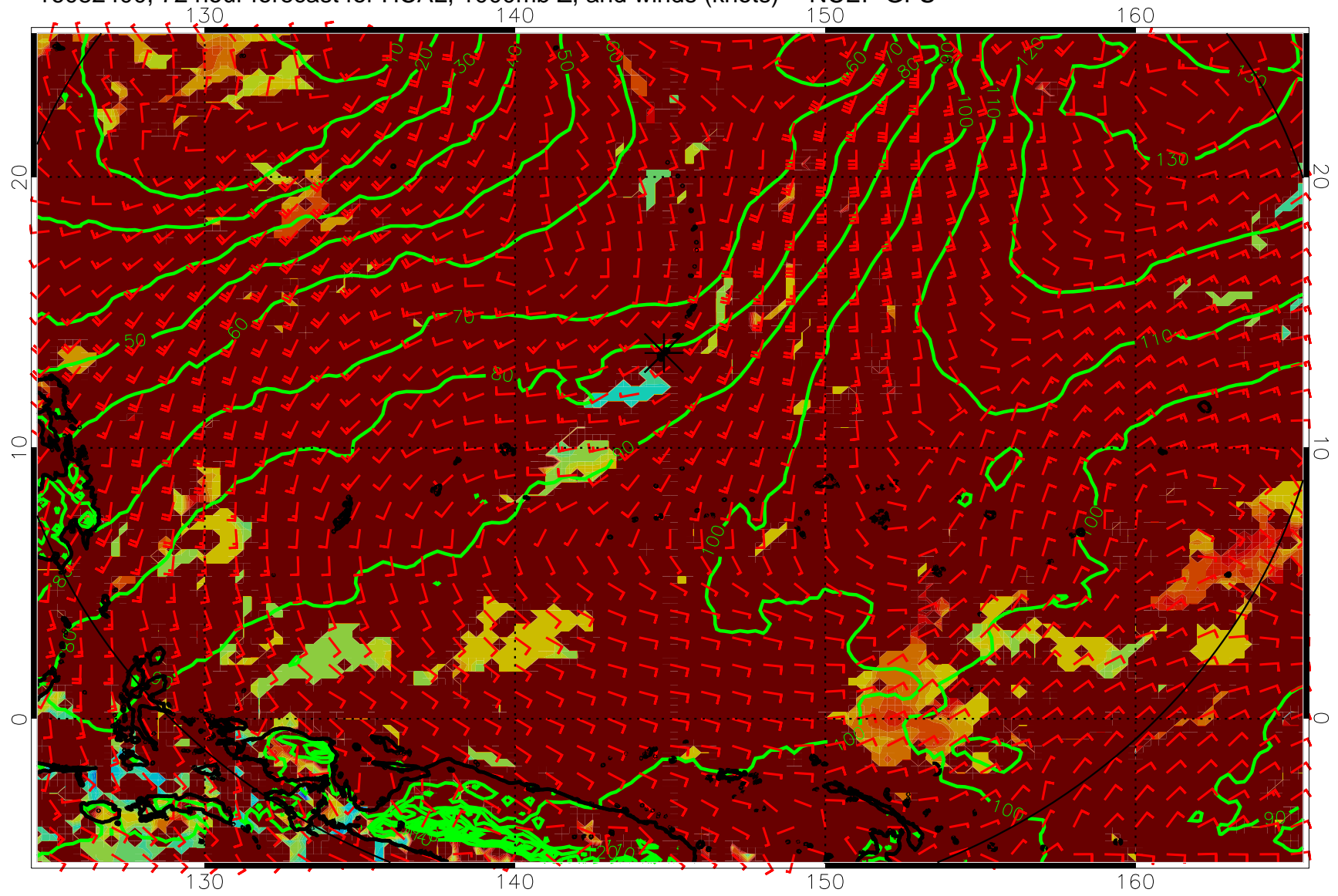
16082400, 72 hour forecast for HCAL, 1000mb Z, and winds (knots) -- NCEP GFS
