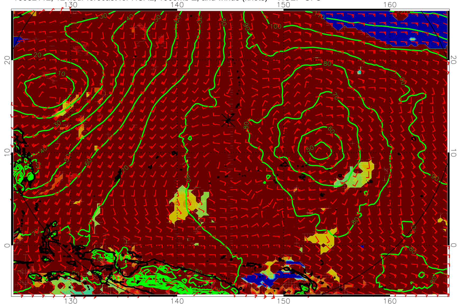
16082112, 12 hour forecast for HCAL, 1000mb Z, and winds (knots) -- NCEP GFS
