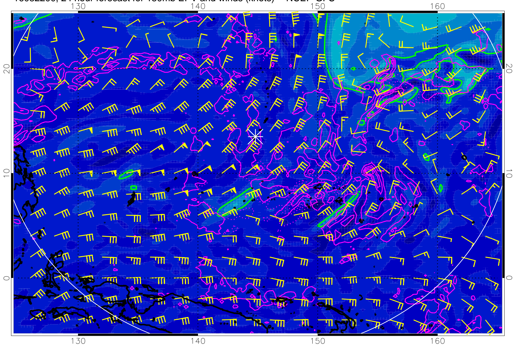
16082200, 24 hour forecast for 150mb EPV and winds (knots) -- NCEP GFS
