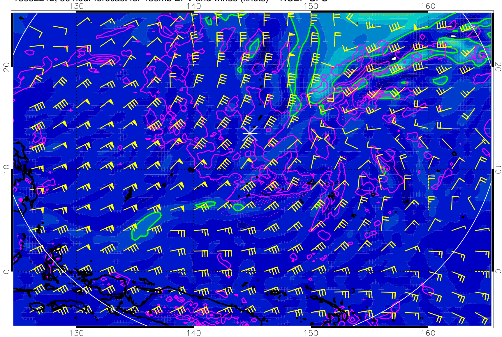
16082212, 36 hour forecast for 150mb EPV and winds (knots) -- NCEP GFS
