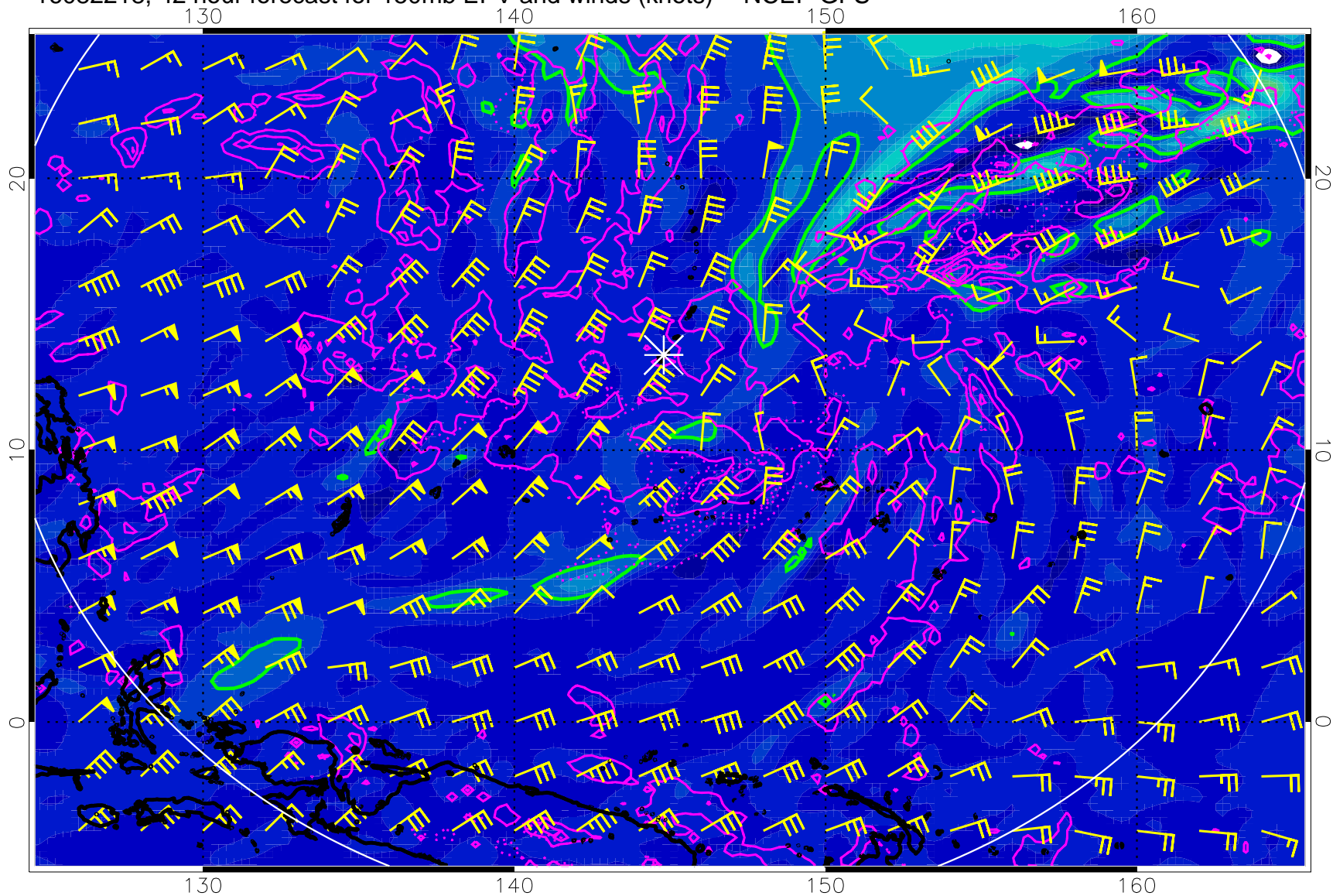
16082218, 42 hour forecast for 150mb EPV and winds (knots) -- NCEP GFS
