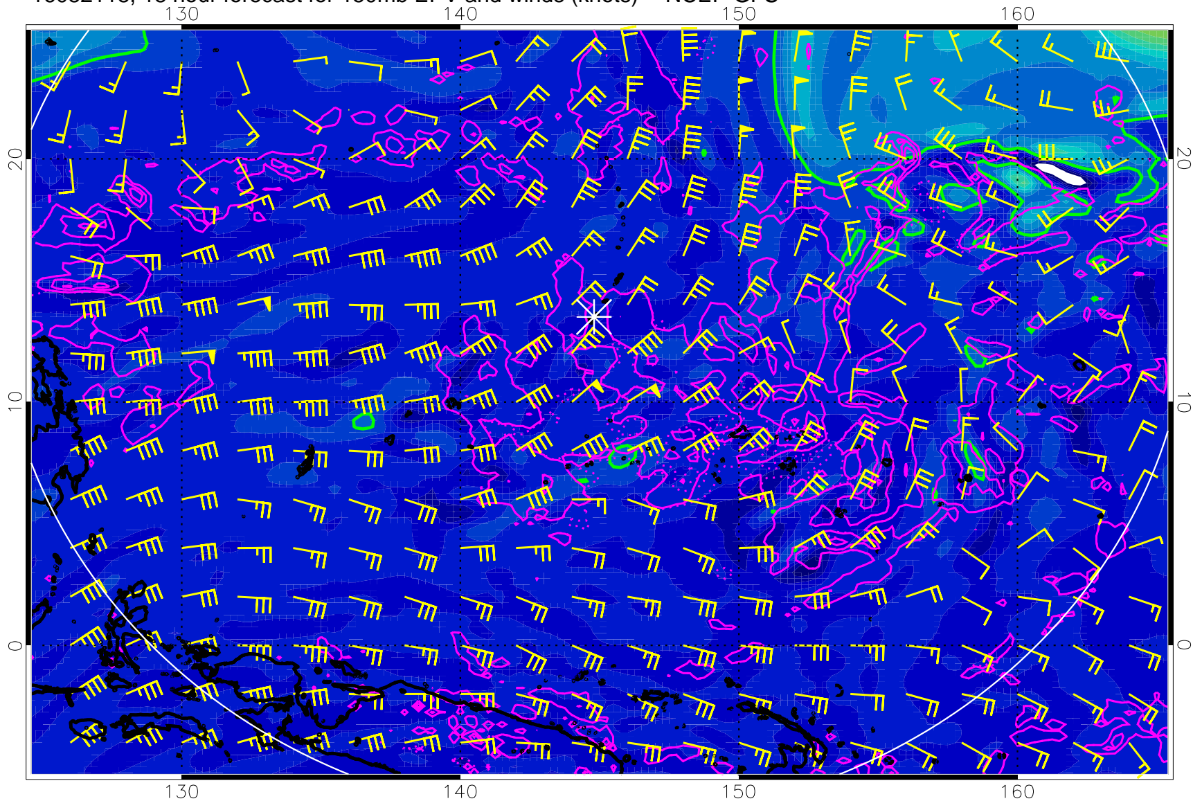
16082118, 18 hour forecast for 150mb EPV and winds (knots) -- NCEP GFS
