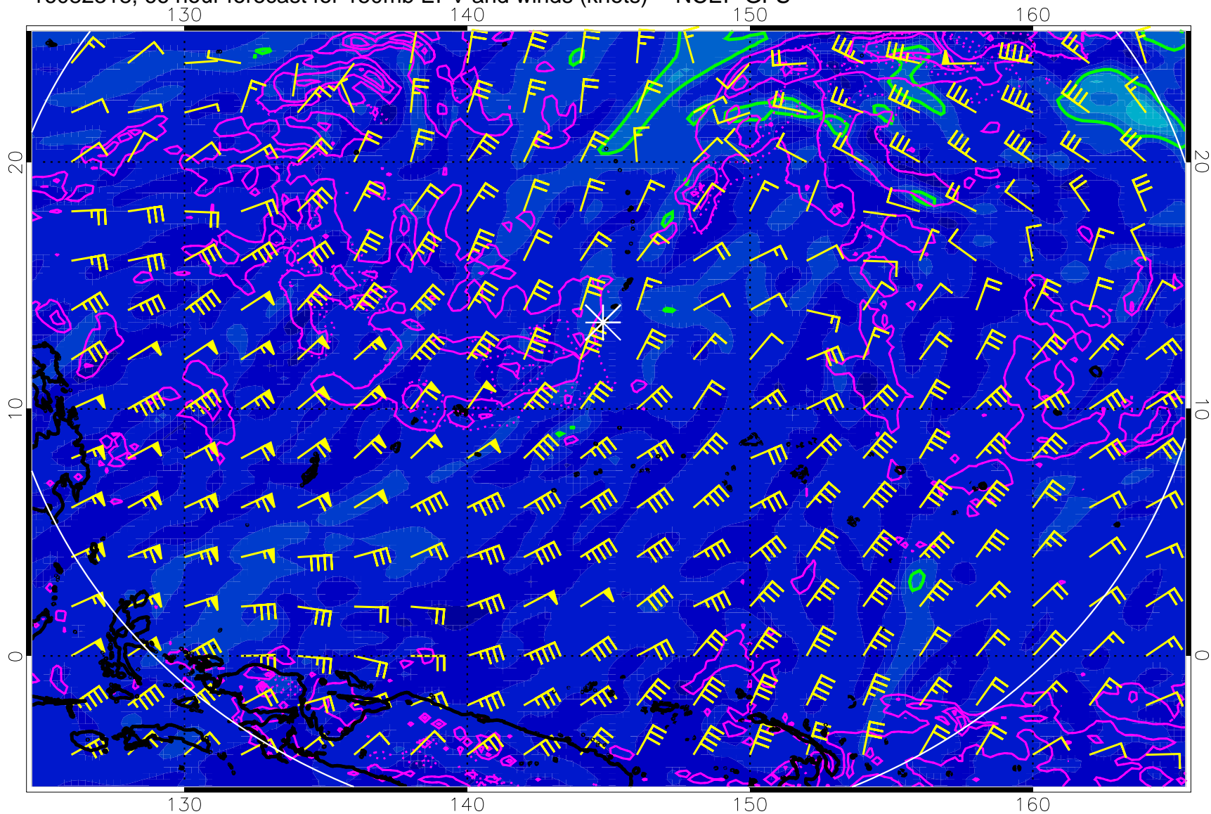
16082318, 66 hour forecast for 150mb EPV and winds (knots) -- NCEP GFS
