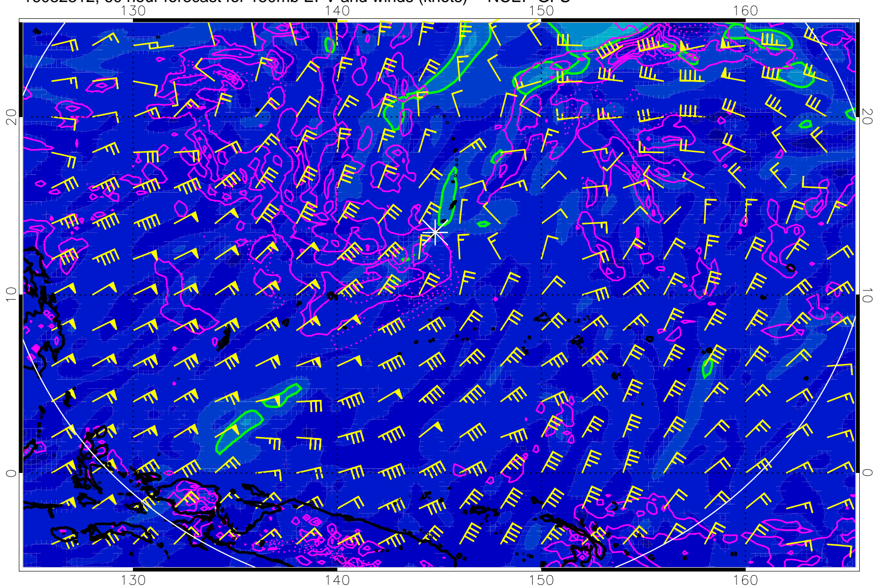
16082312, 60 hour forecast for 150mb EPV and winds (knots) -- NCEP GFS
