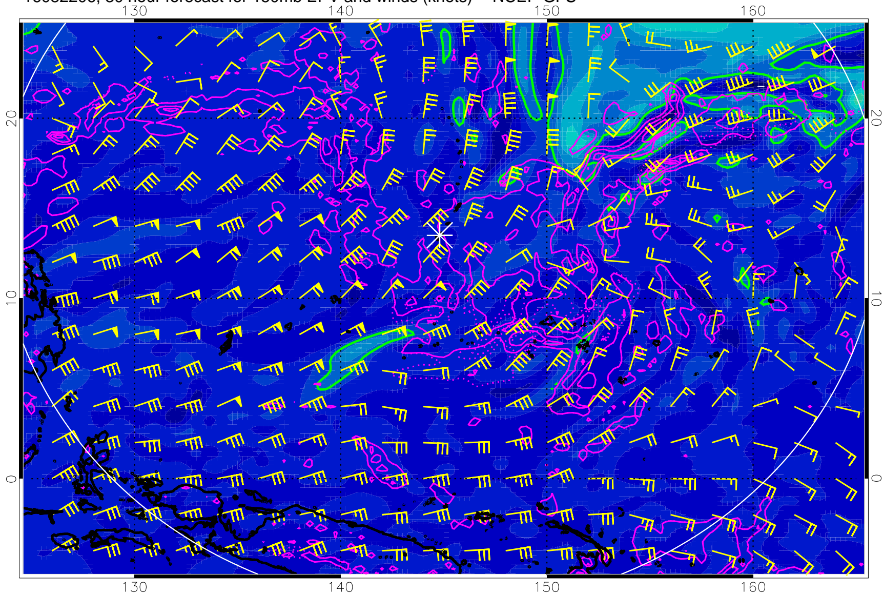
16082206, 30 hour forecast for 150mb EPV and winds (knots) -- NCEP GFS
