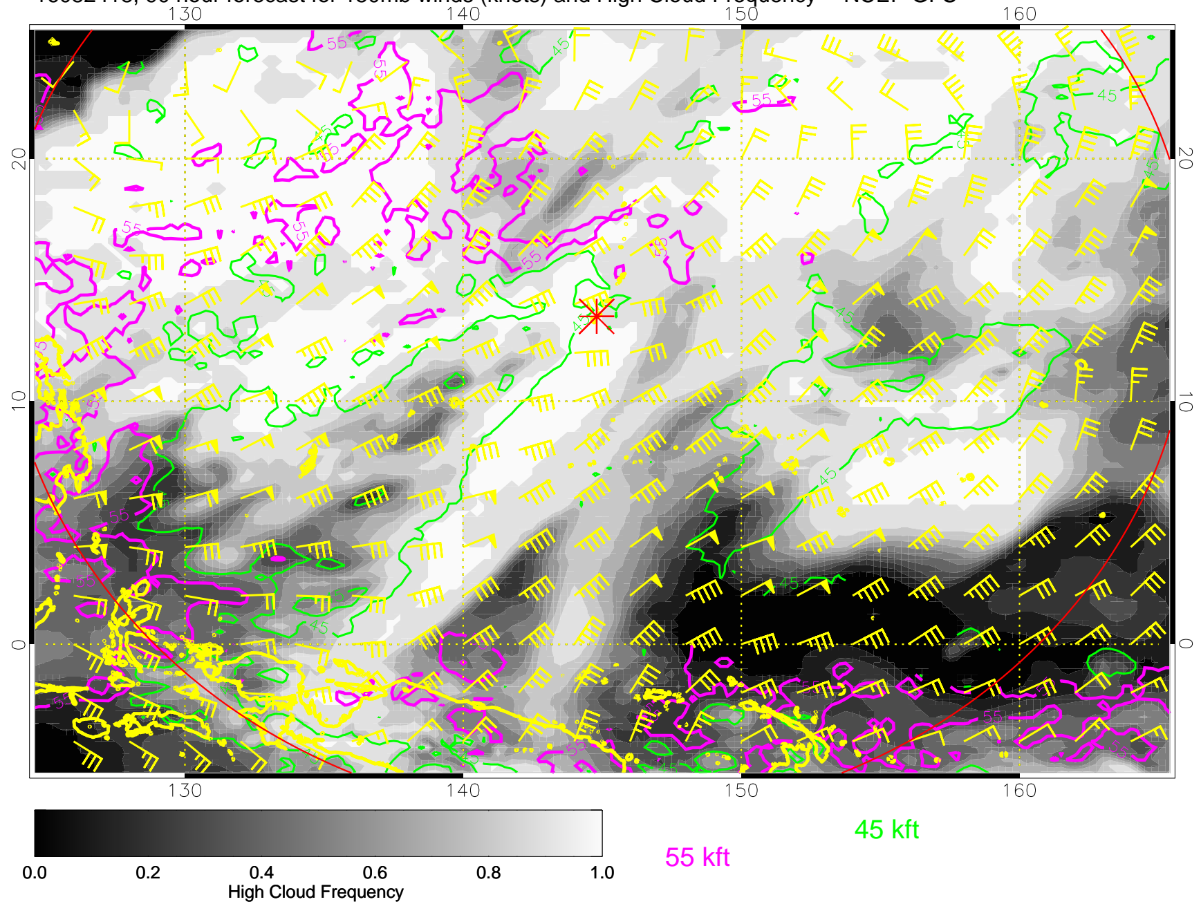
16082418, 90 hour forecast for 150mb winds (knots) and High Cloud Frequency -- NCEP GFS
