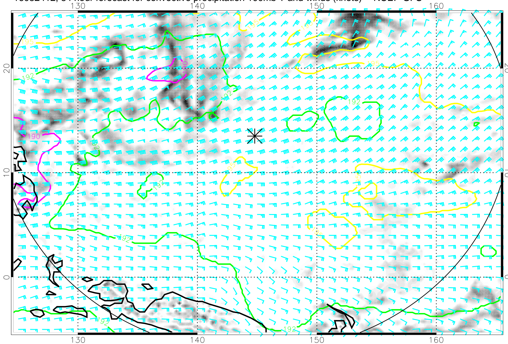
16082412, 84 hour forecast for convective precipitation 100mb T and winds (knots) -- NCEP GFS
