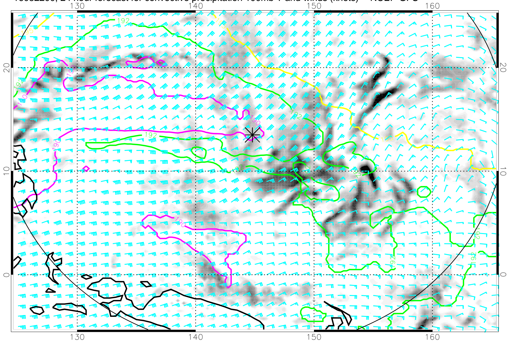
16082200, 24 hour forecast for convective precipitation 100mb T and winds (knots) -- NCEP GFS
