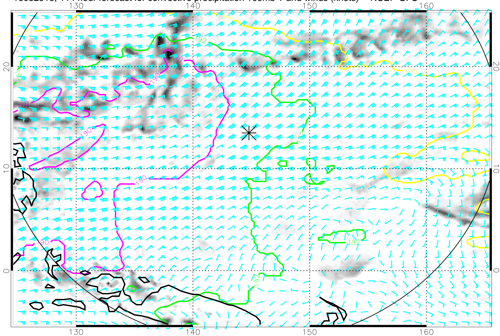
16082518, 114 hour forecast for convective precipitation 100mb T and winds (knots) -- NCEP GFS
