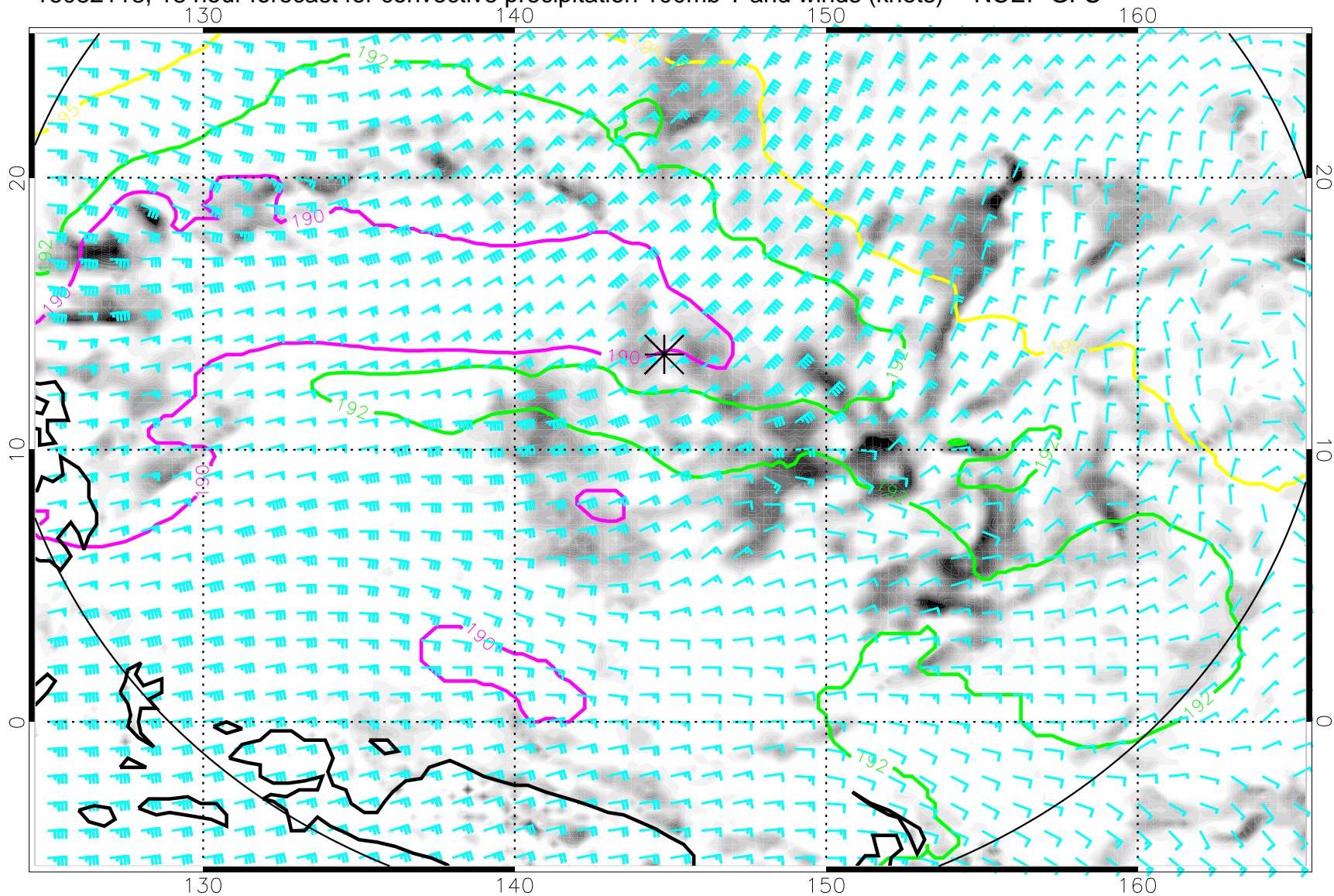
16082118, 18 hour forecast for convective precipitation 100mb T and winds (knots) -- NCEP GFS
