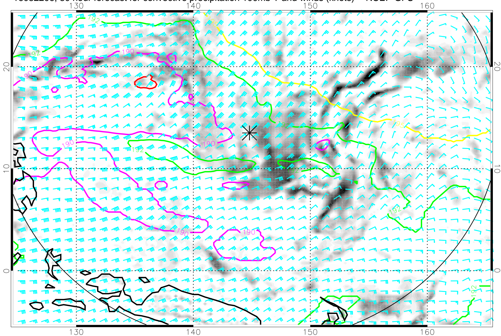
16082206, 30 hour forecast for convective precipitation 100mb T and winds (knots) -- NCEP GFS
