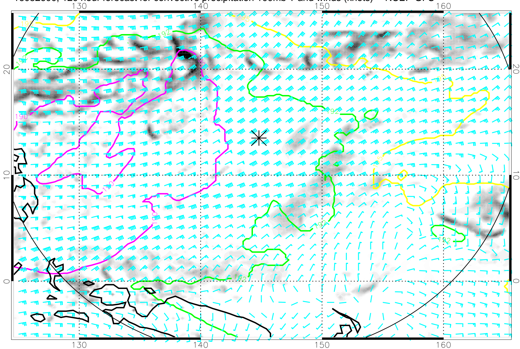
16082600, 120 hour forecast for convective precipitation 100mb T and winds (knots) -- NCEP GFS
