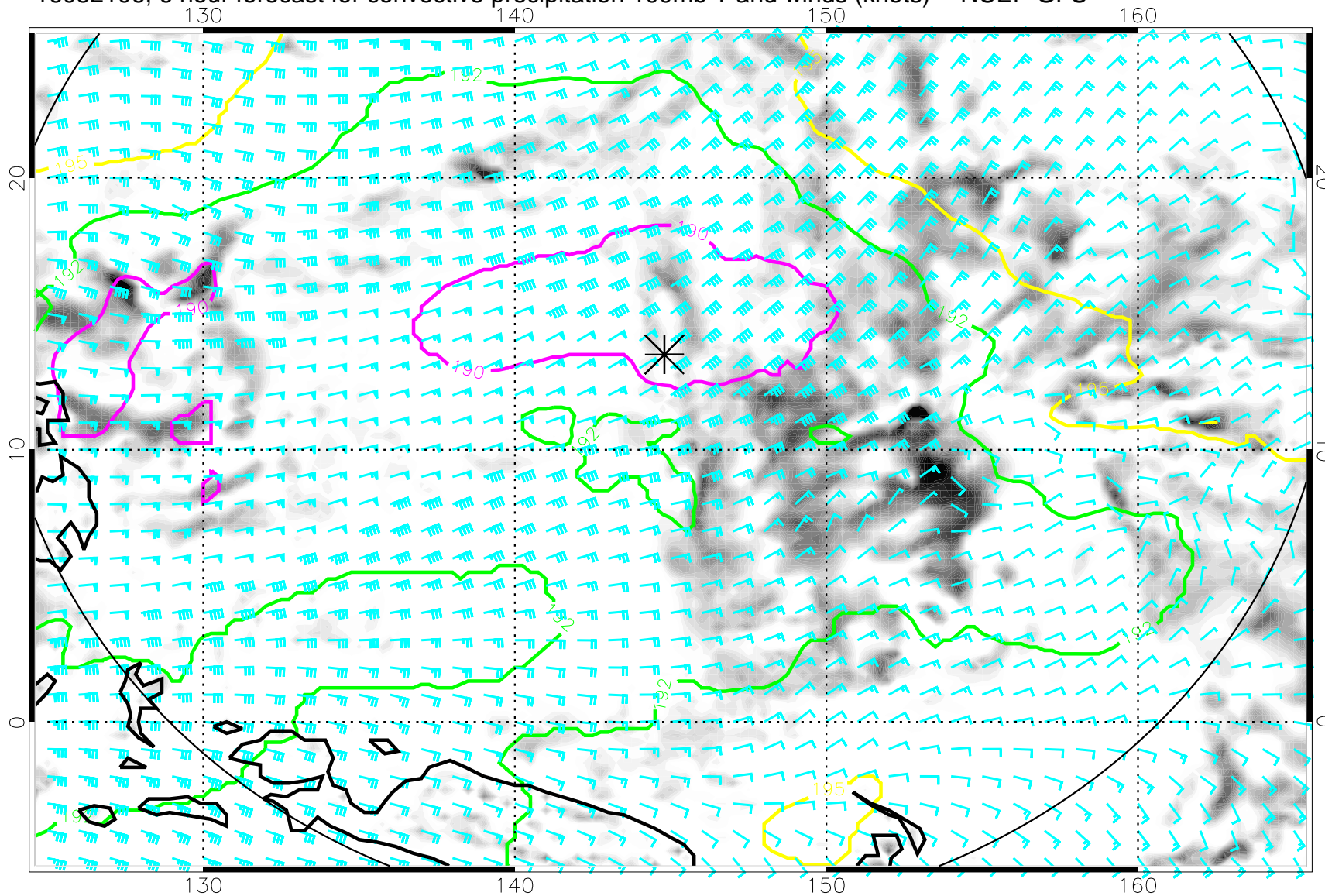
16082106, 6 hour forecast for convective precipitation 100mb T and winds (knots) -- NCEP GFS
