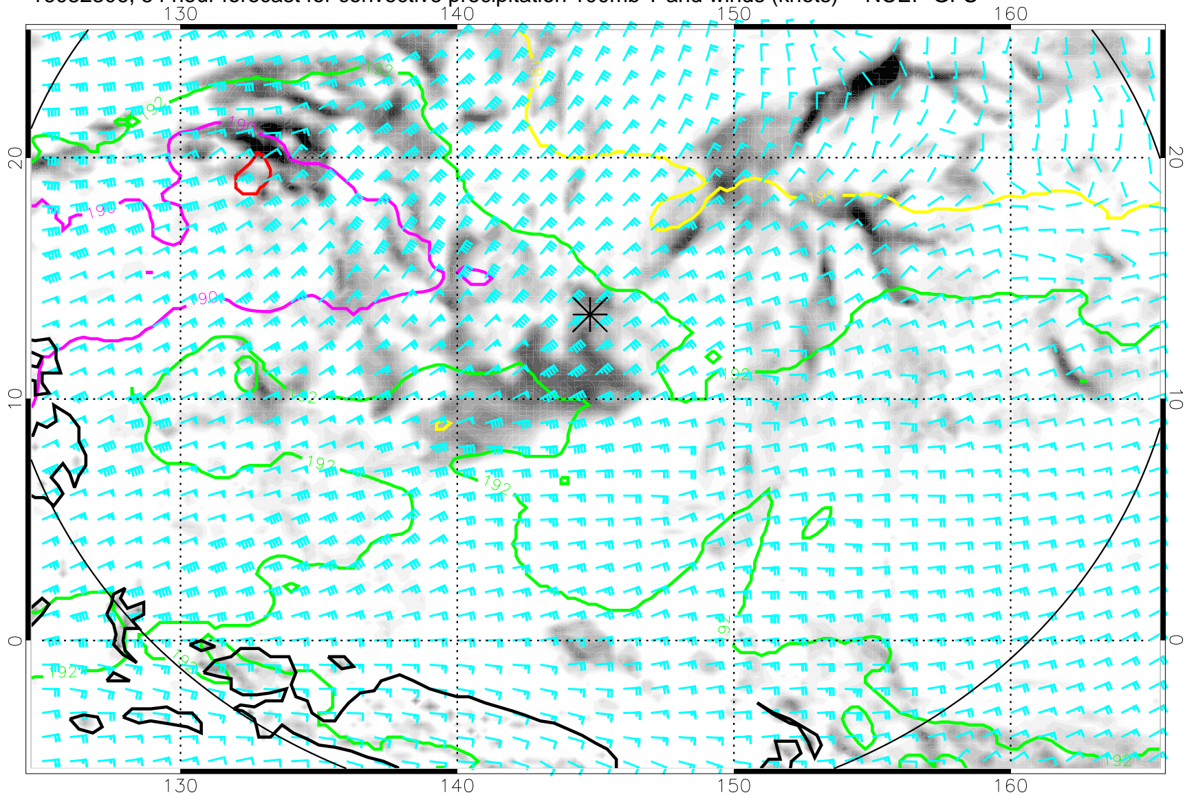
16082306, 54 hour forecast for convective precipitation 100mb T and winds (knots) -- NCEP GFS
