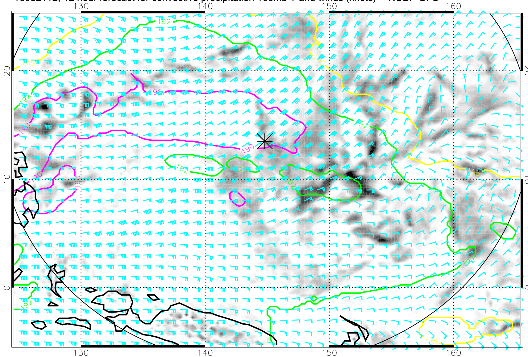
16082112, 12 hour forecast for convective precipitation 100mb T and winds (knots) -- NCEP GFS
