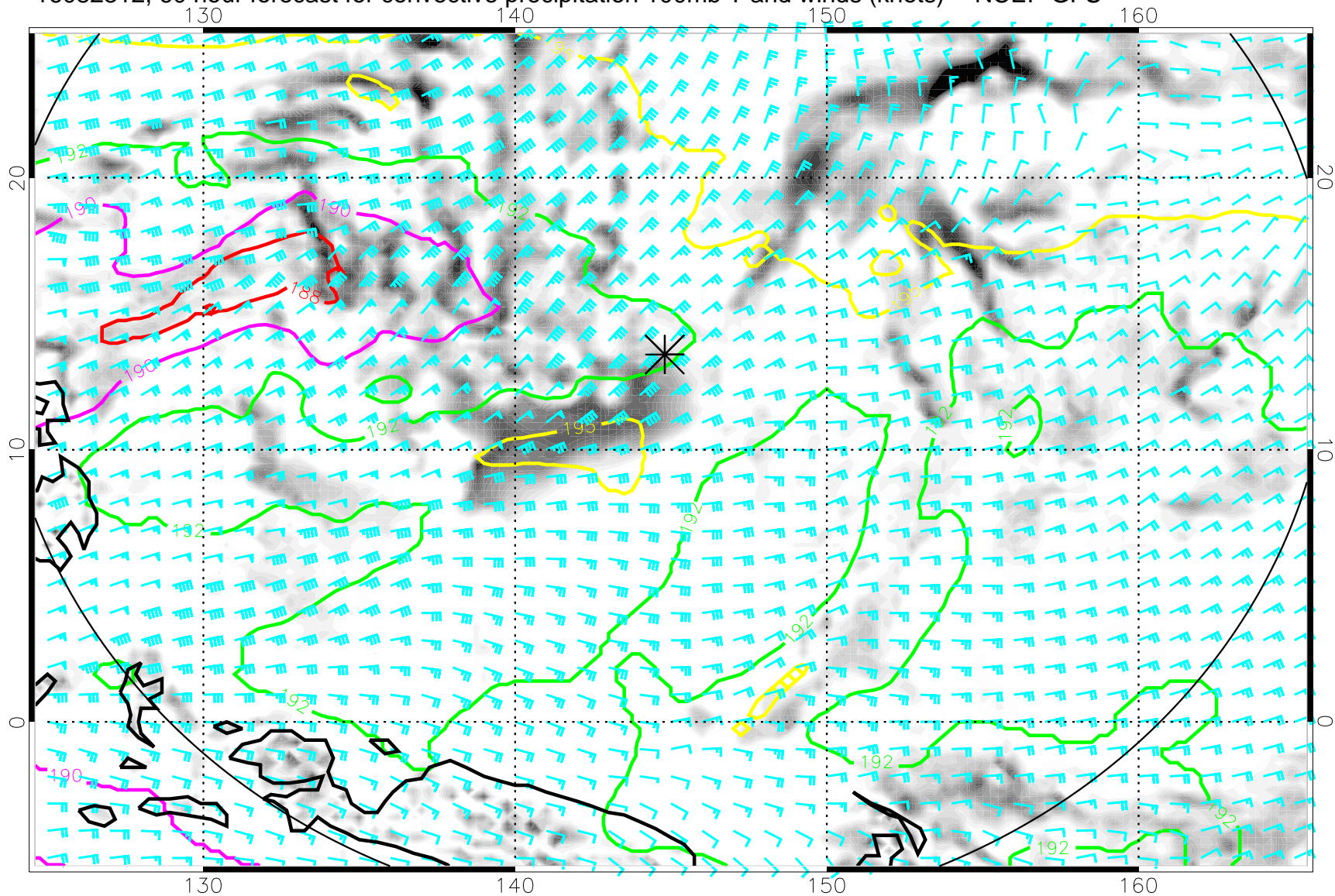
16082312, 60 hour forecast for convective precipitation 100mb T and winds (knots) -- NCEP GFS
