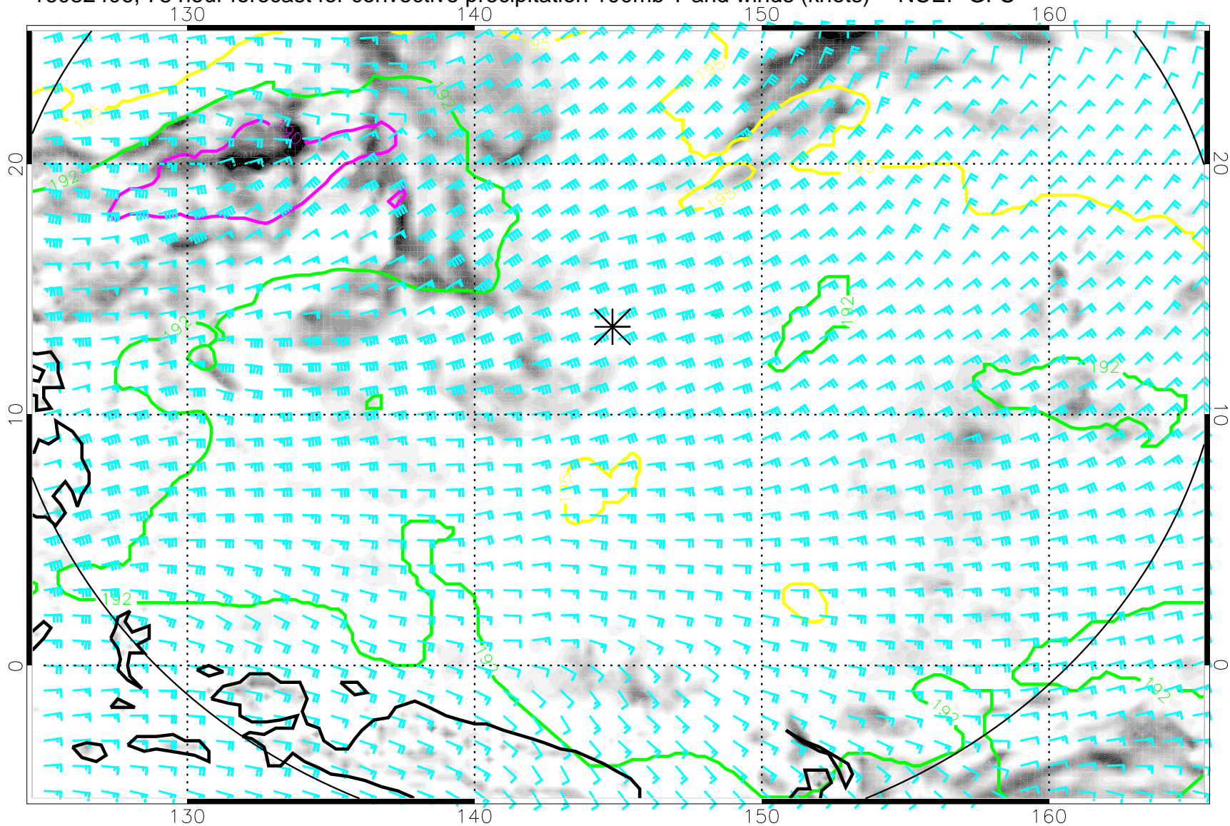
16082406, 78 hour forecast for convective precipitation 100mb T and winds (knots) -- NCEP GFS
