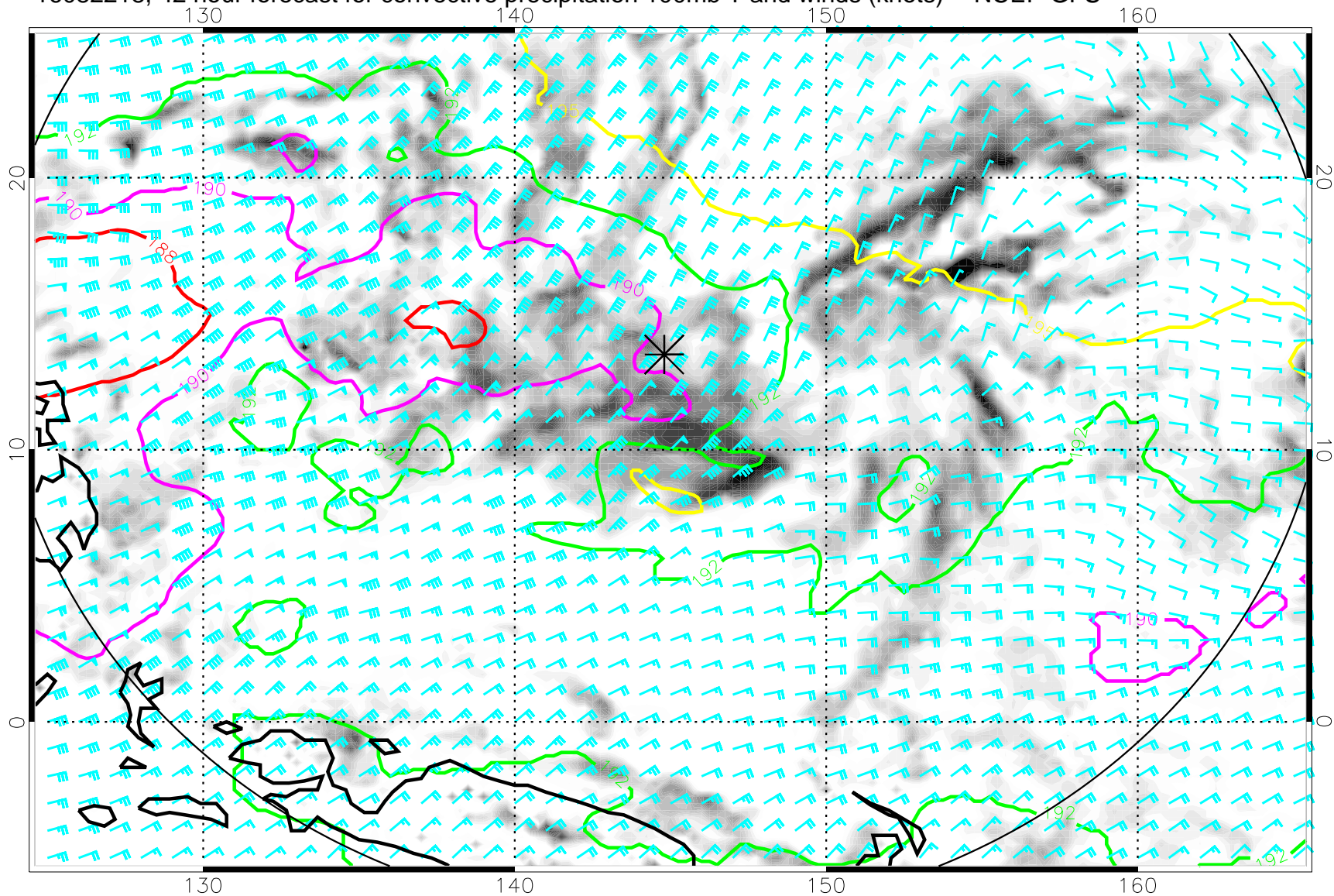
16082218, 42 hour forecast for convective precipitation 100mb T and winds (knots) -- NCEP GFS
