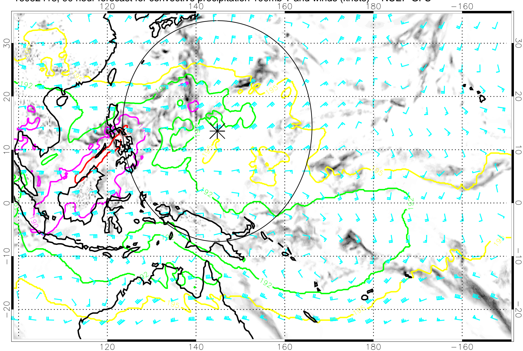
16082418, 90 hour forecast for convective precipitation 100mb T and winds (knots) -- NCEP GFS
