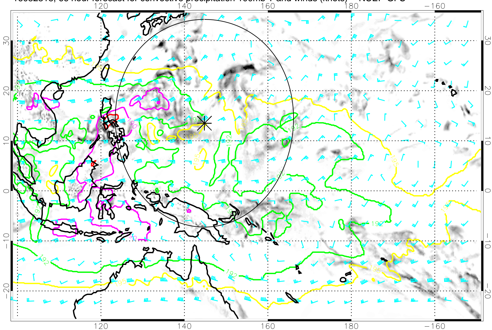
16082318, 66 hour forecast for convective precipitation 100mb T and winds (knots) -- NCEP GFS
