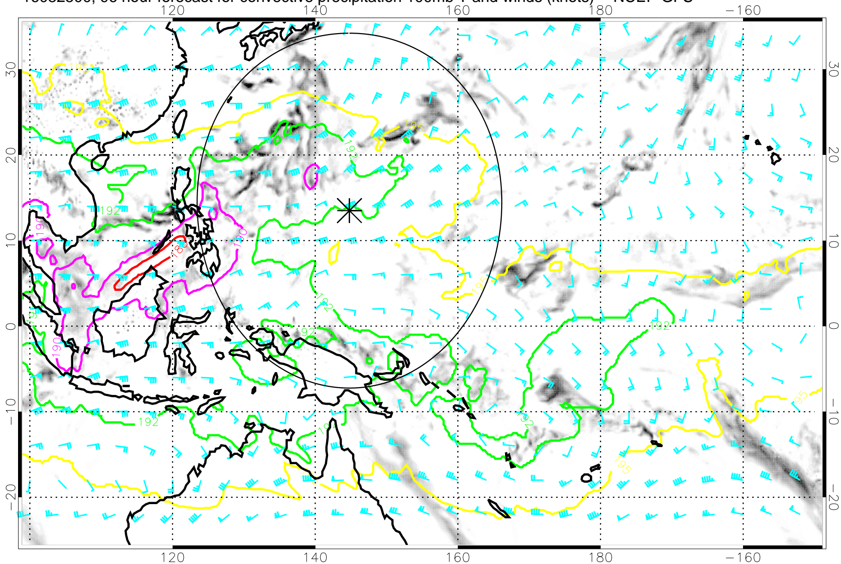
16082500, 96 hour forecast for convective precipitation 100mb T and winds (knots) -- NCEP GFS
