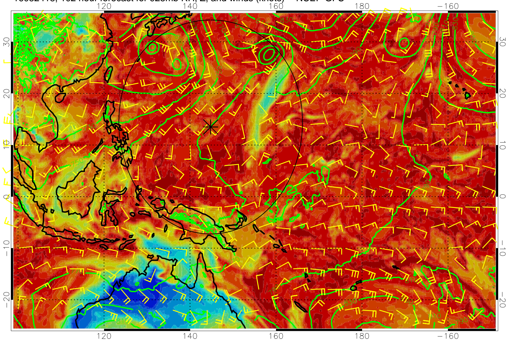
16082418, 102 hour forecast for 925mb RH, Z, and winds (knots) -- NCEP GFS
