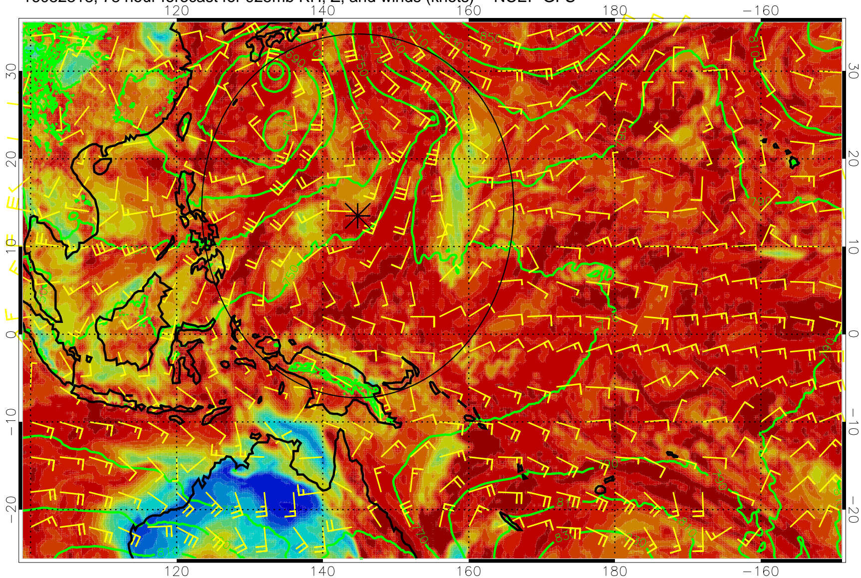
16082318, 78 hour forecast for 925mb RH, Z, and winds (knots) -- NCEP GFS
