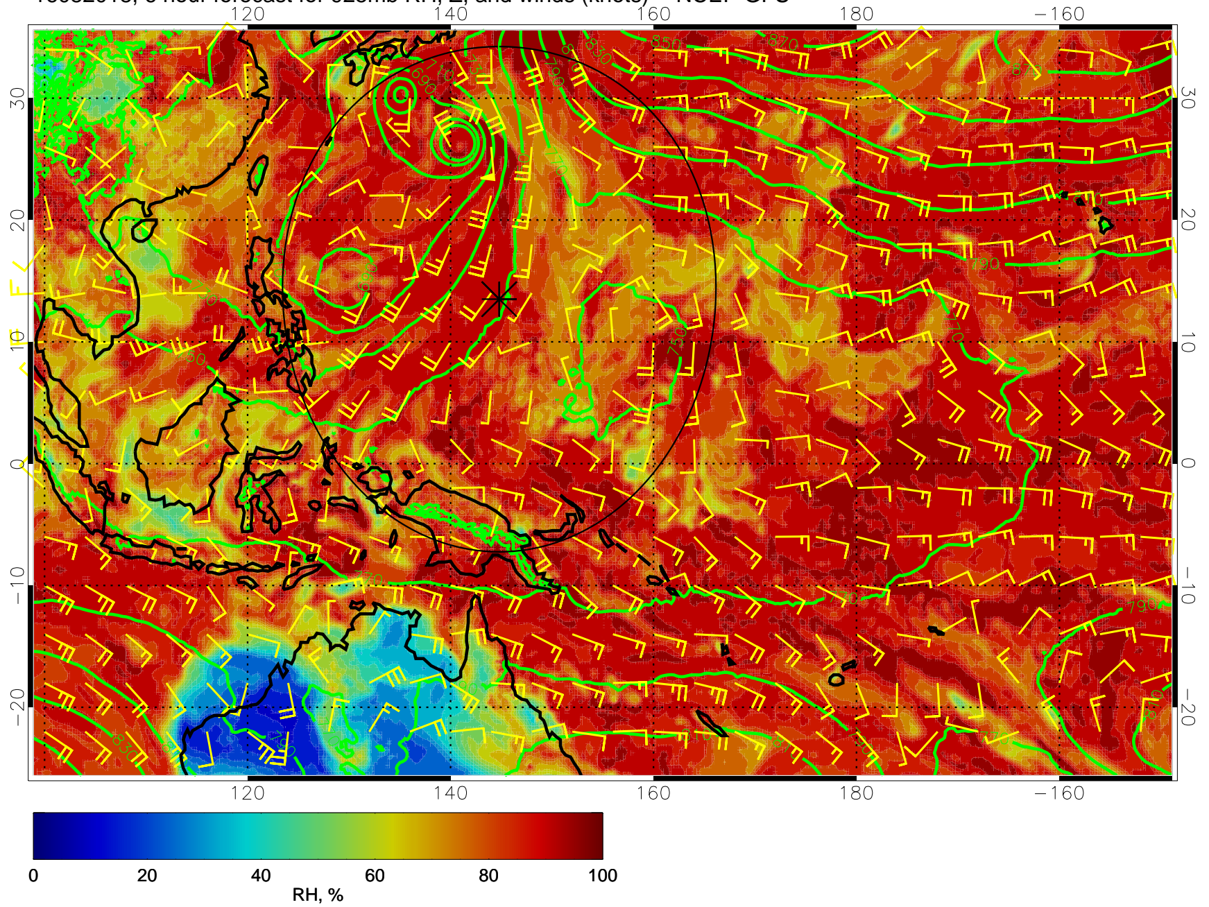
16082018, 6 hour forecast for 925mb RH, Z, and winds (knots) -- NCEP GFS
