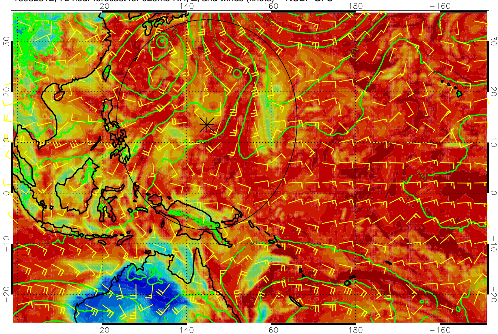
16082312, 72 hour forecast for 925mb RH, Z, and winds (knots) -- NCEP GFS
