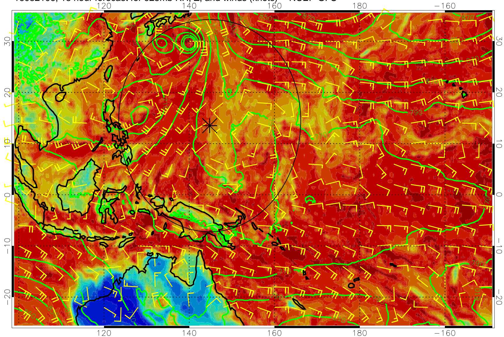
16082106, 18 hour forecast for 925mb RH, Z, and winds (knots) -- NCEP GFS
