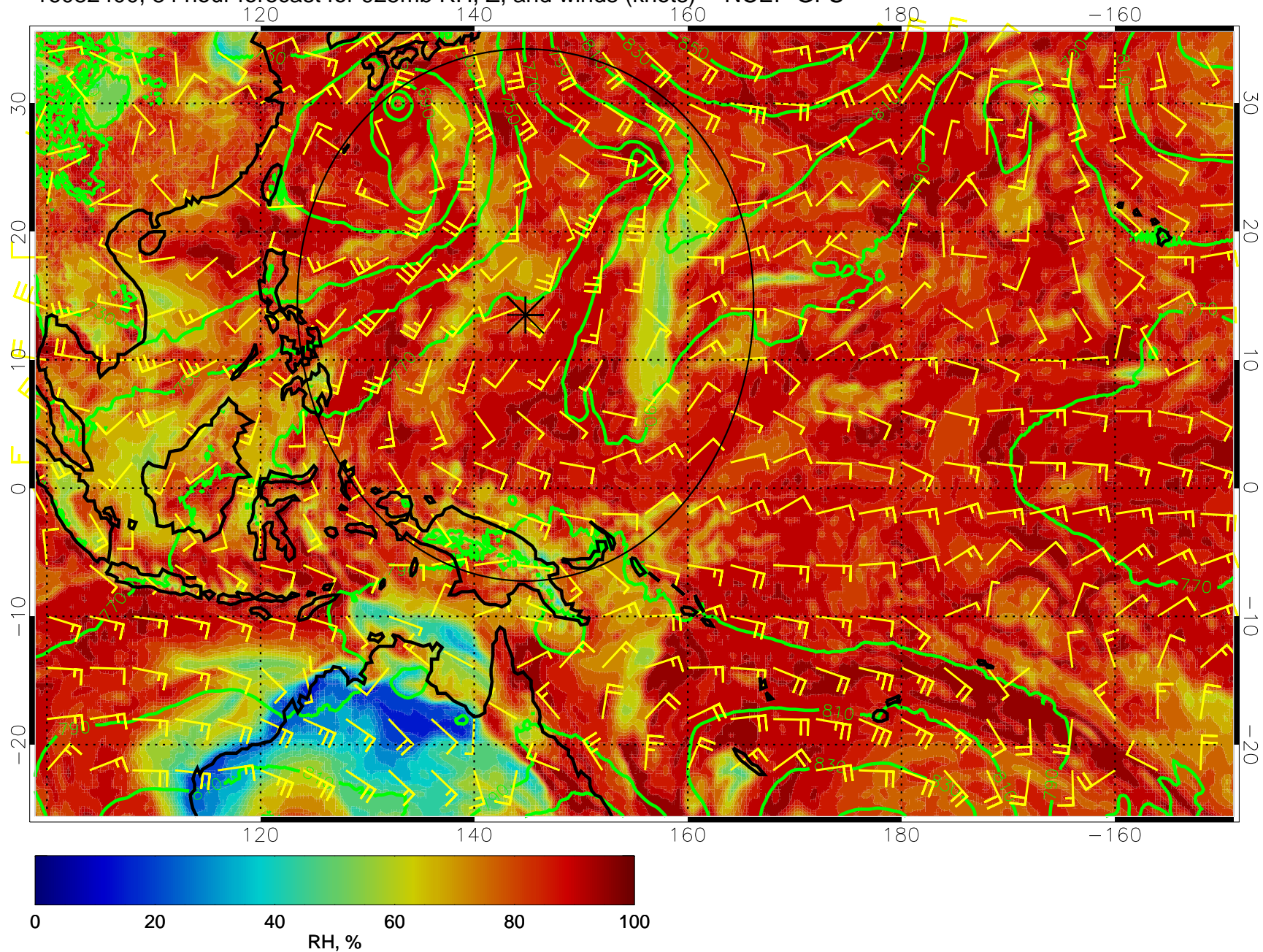
16082400, 84 hour forecast for 925mb RH, Z, and winds (knots) -- NCEP GFS
