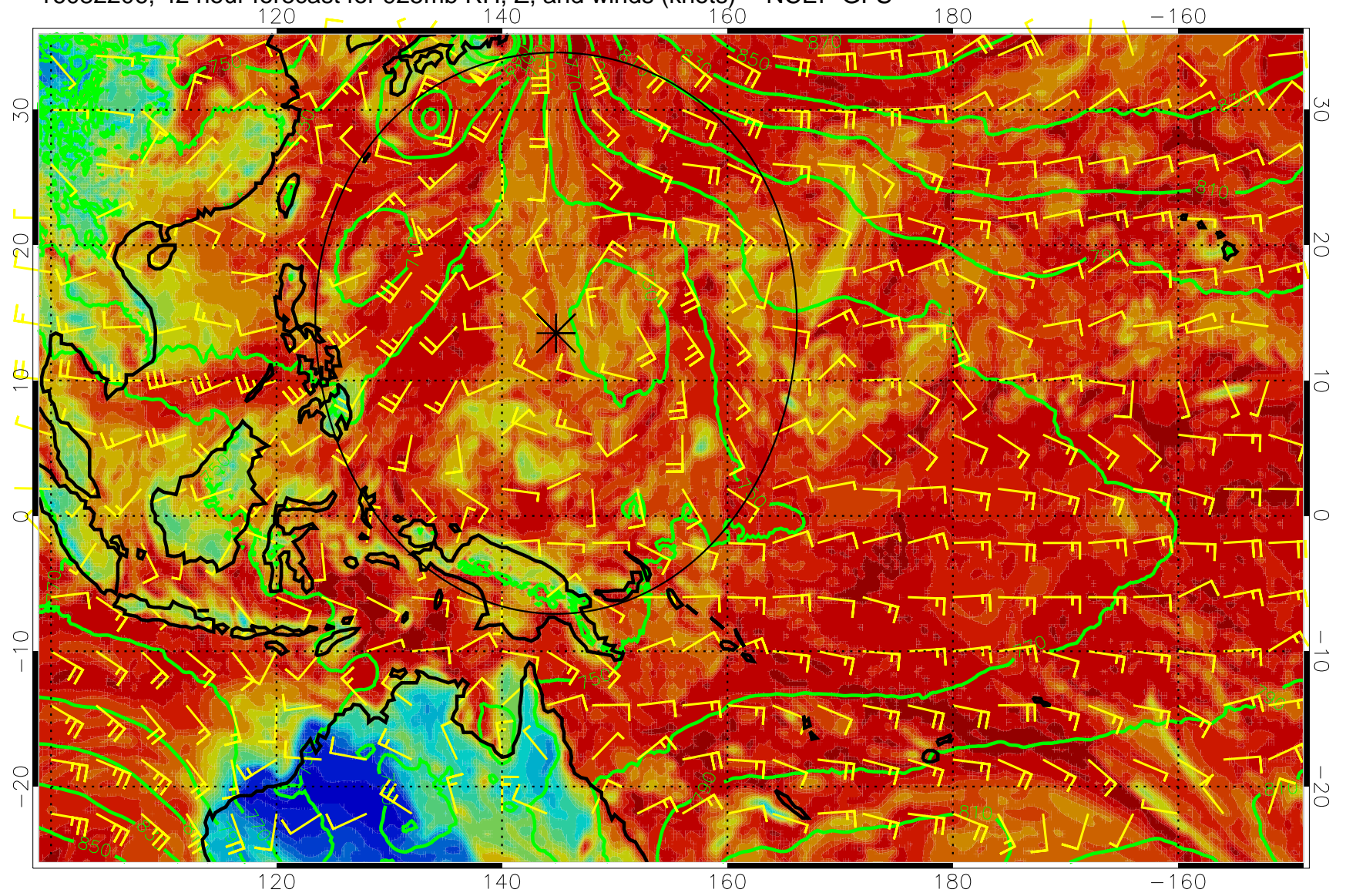
16082206, 42 hour forecast for 925mb RH, Z, and winds (knots) -- NCEP GFS
