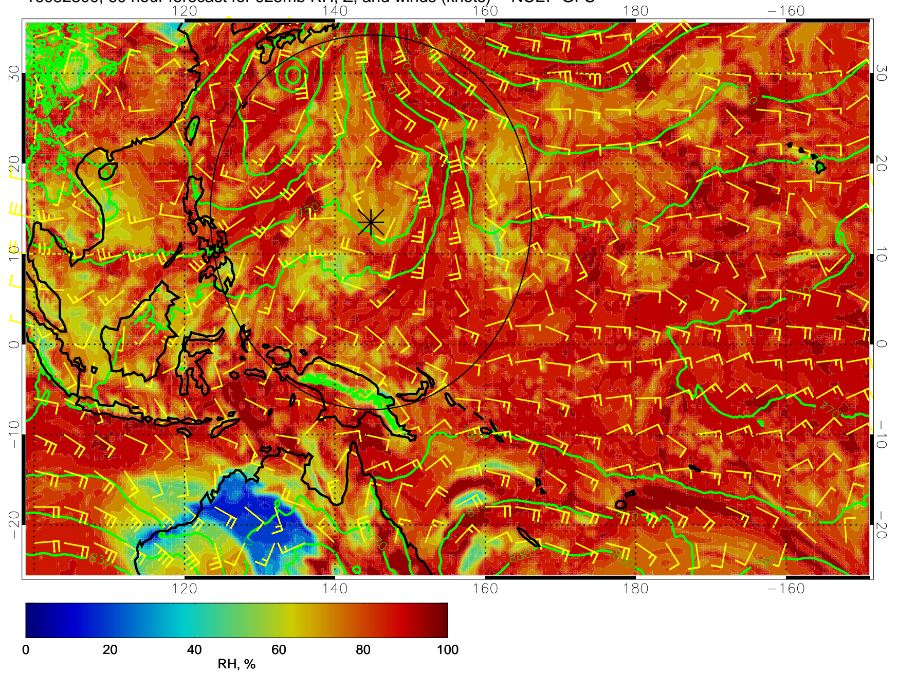
16082300, 60 hour forecast for 925mb RH, Z, and winds (knots) -- NCEP GFS
