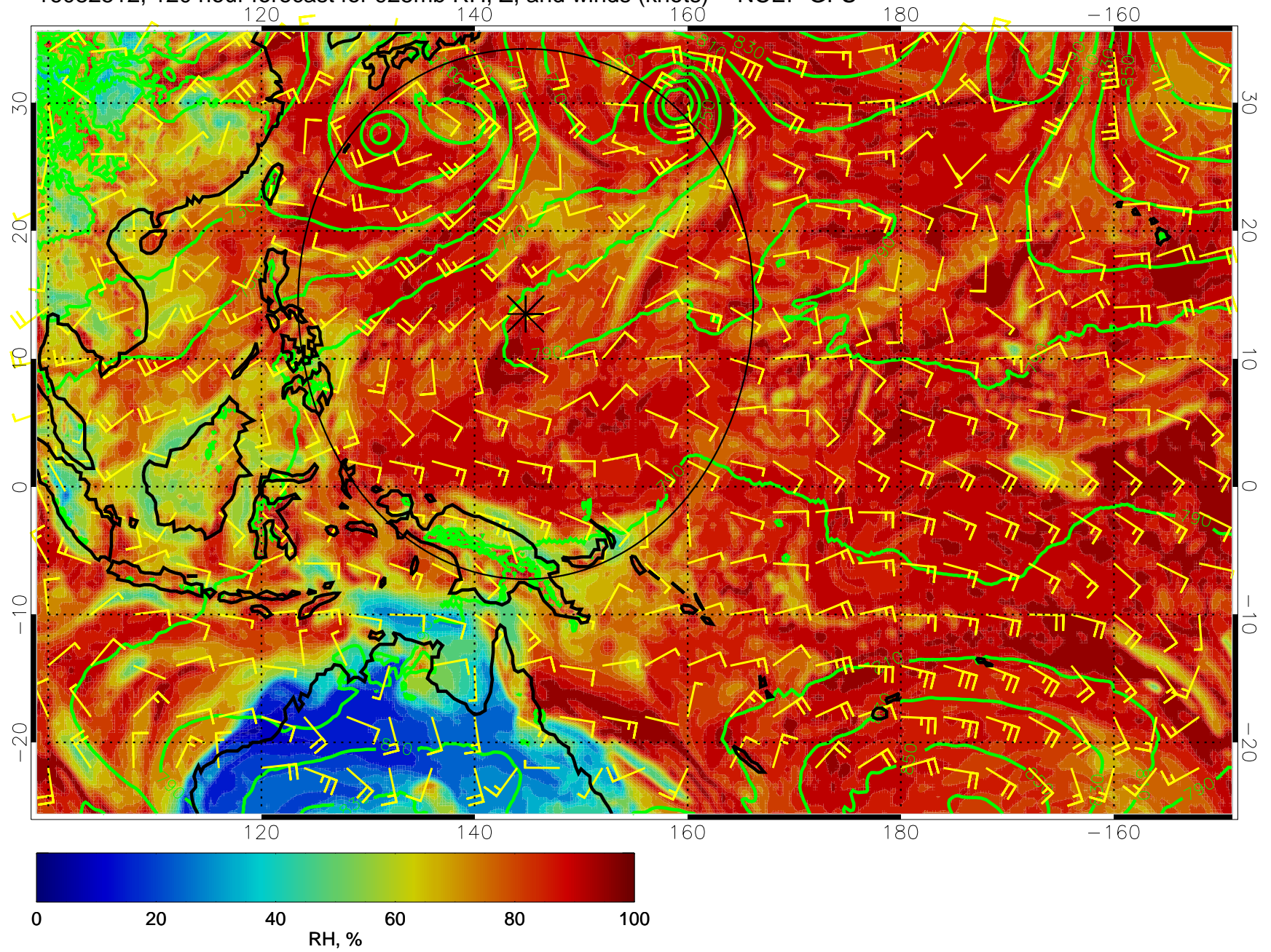
16082512, 120 hour forecast for 925mb RH, Z, and winds (knots) -- NCEP GFS
