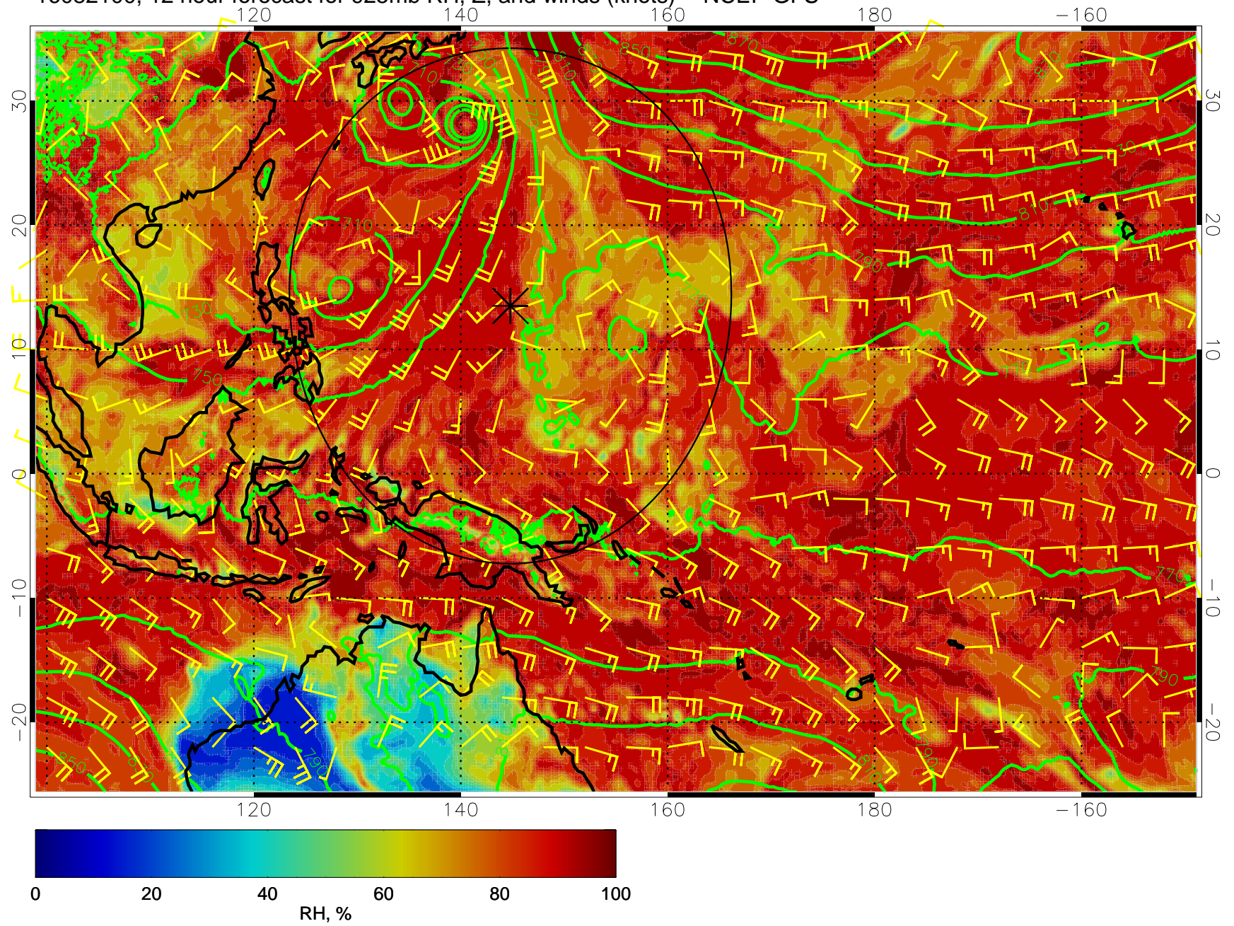
16082100, 12 hour forecast for 925mb RH, Z, and winds (knots) -- NCEP GFS
