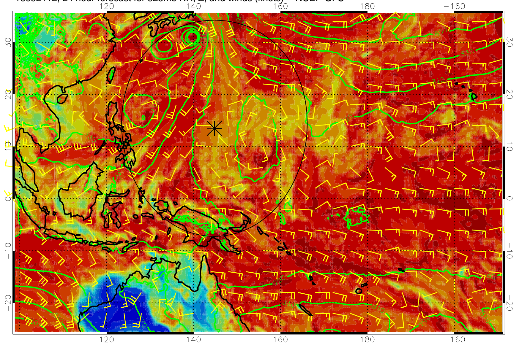
16082112, 24 hour forecast for 925mb RH, Z, and winds (knots) -- NCEP GFS
