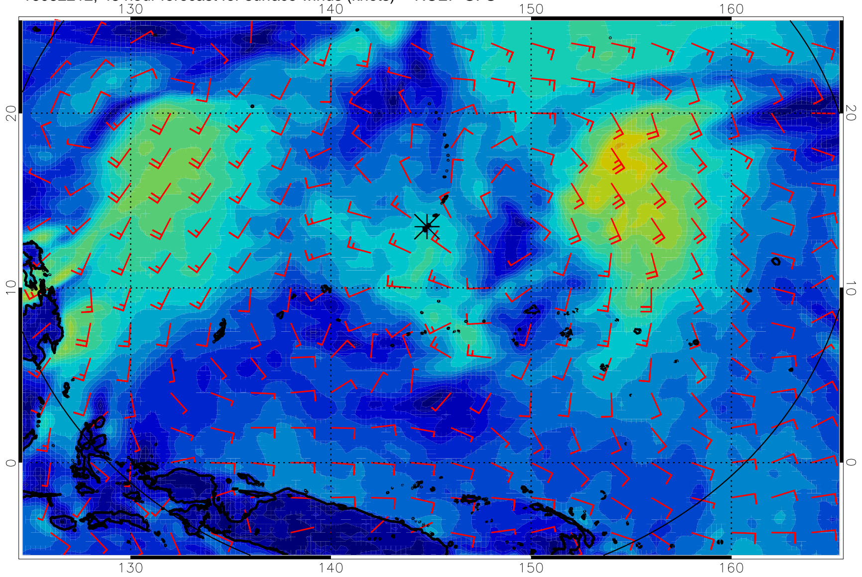
16082212, 48 hour forecast for surface winds (knots) -- NCEP GFS
