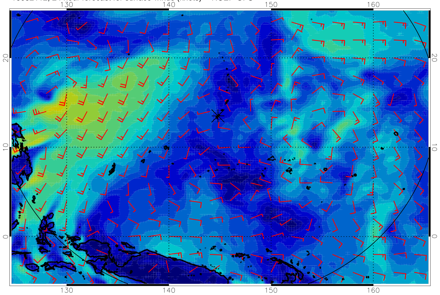
16082112, 24 hour forecast for surface winds (knots) -- NCEP GFS
