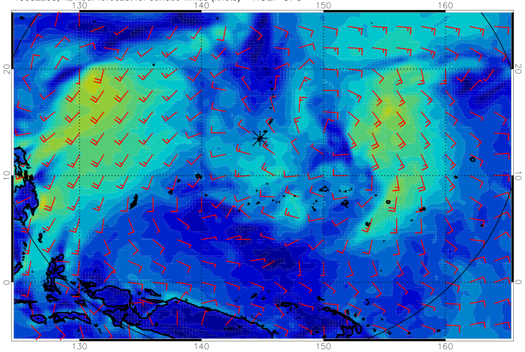
16082206, 42 hour forecast for surface winds (knots) -- NCEP GFS
