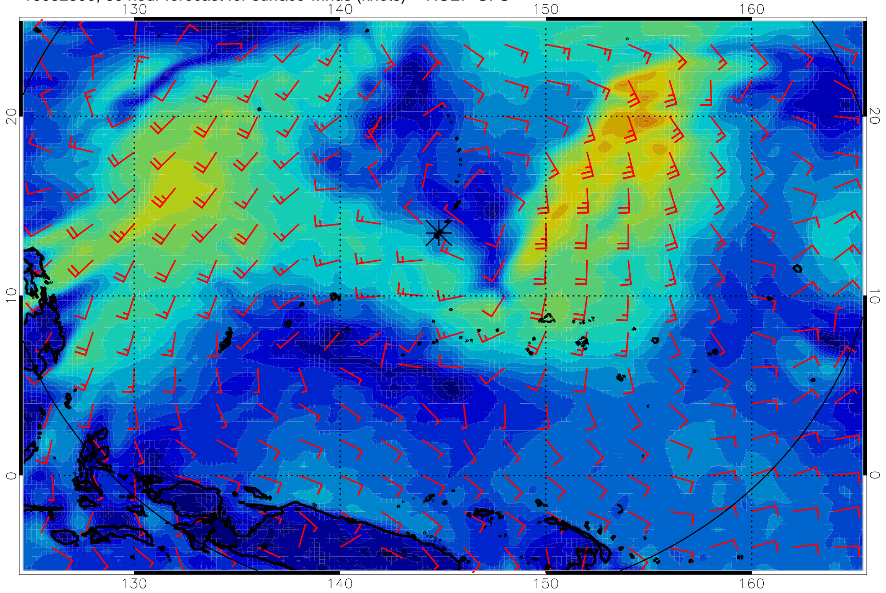
16082300, 60 hour forecast for surface winds (knots) -- NCEP GFS
