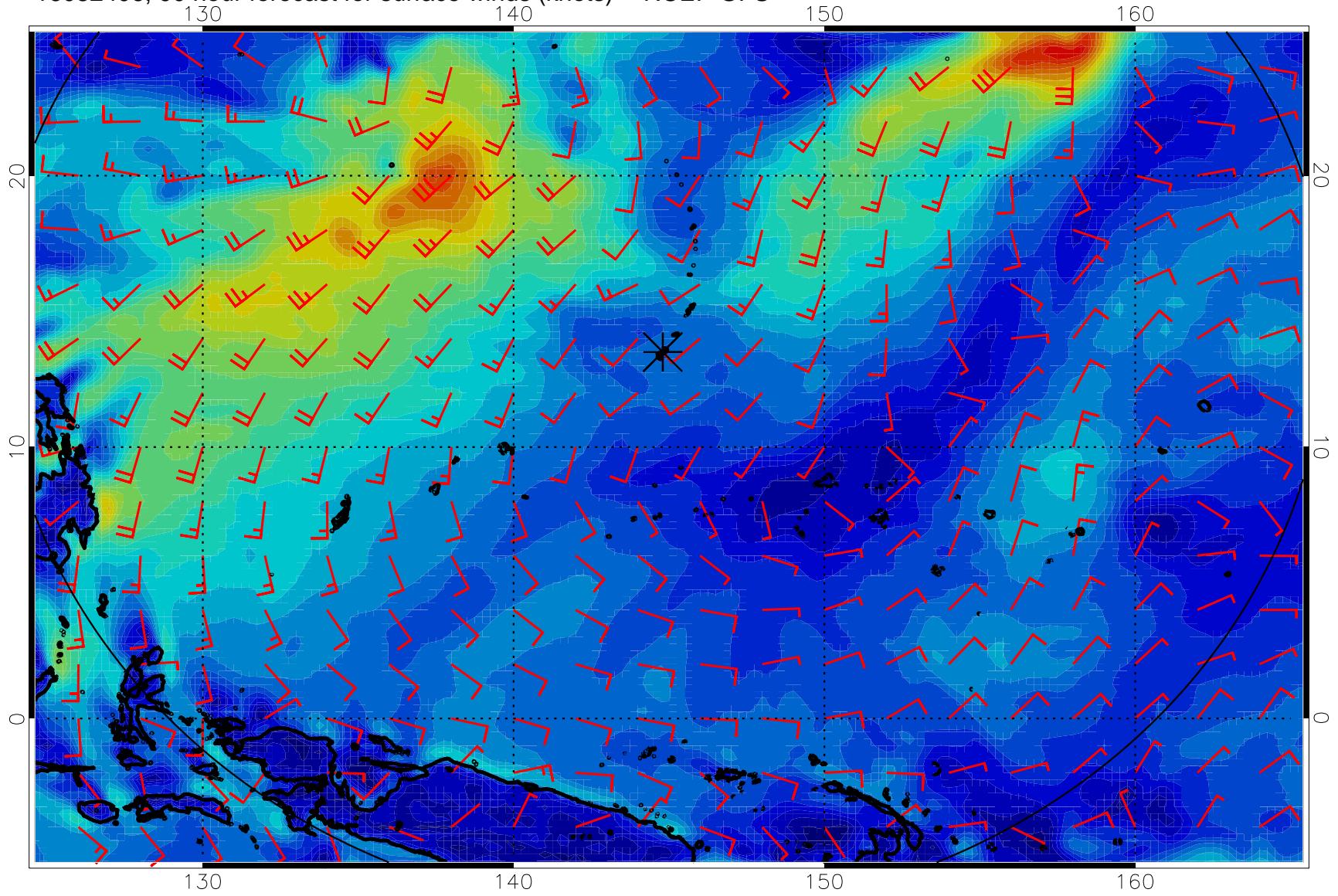
16082406, 90 hour forecast for surface winds (knots) -- NCEP GFS
