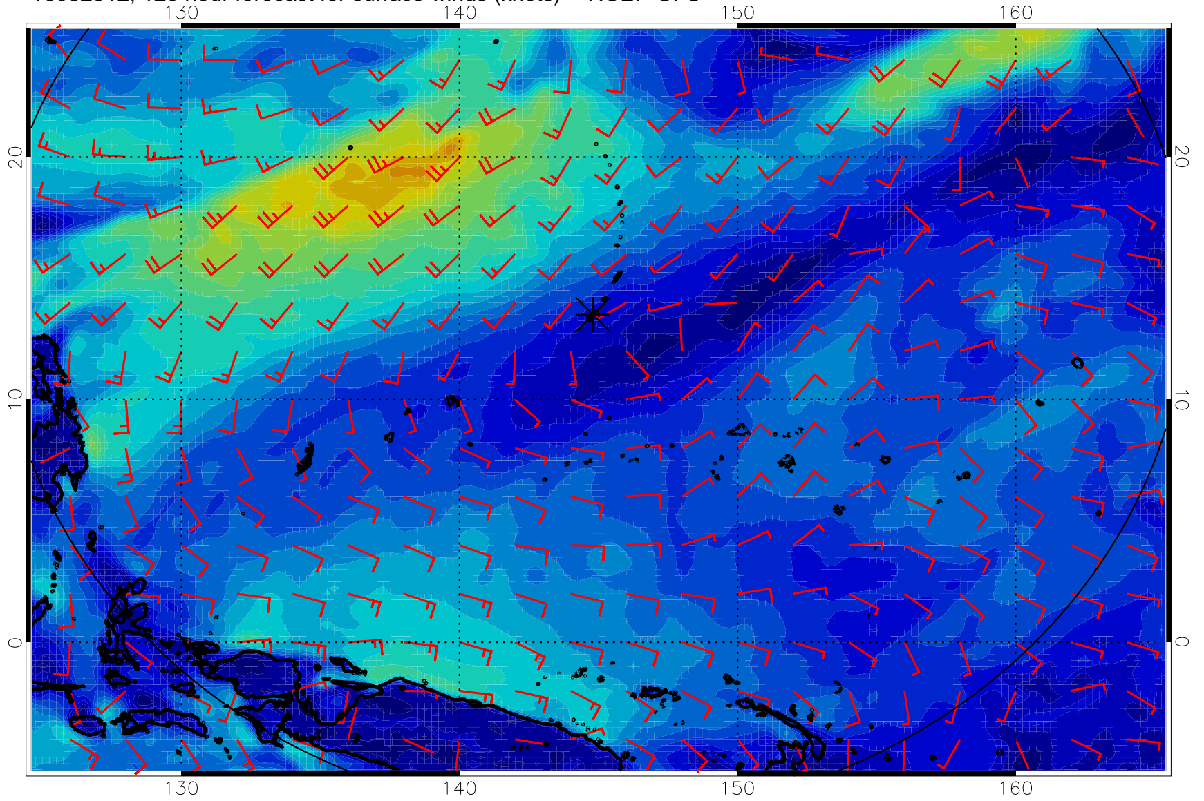
16082512, 120 hour forecast for surface winds (knots) -- NCEP GFS
