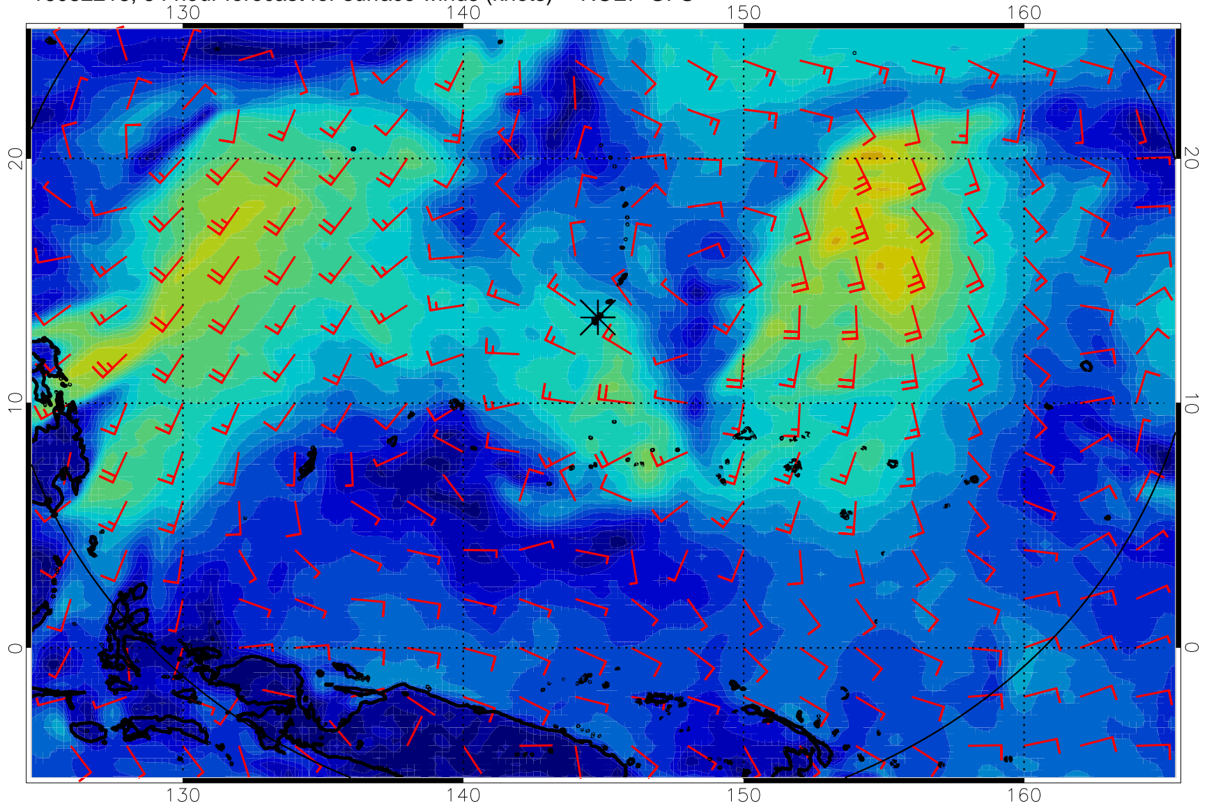
16082218, 54 hour forecast for surface winds (knots) -- NCEP GFS
