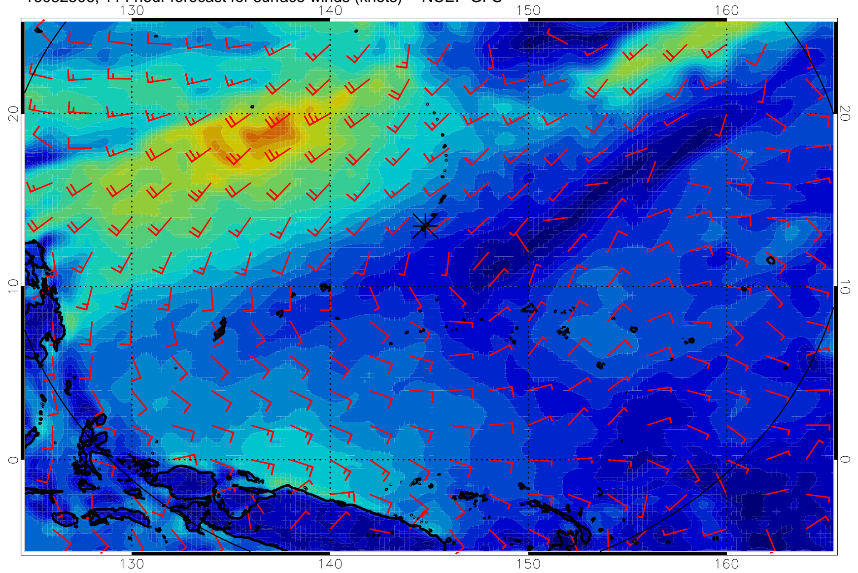
16082506, 114 hour forecast for surface winds (knots) -- NCEP GFS
