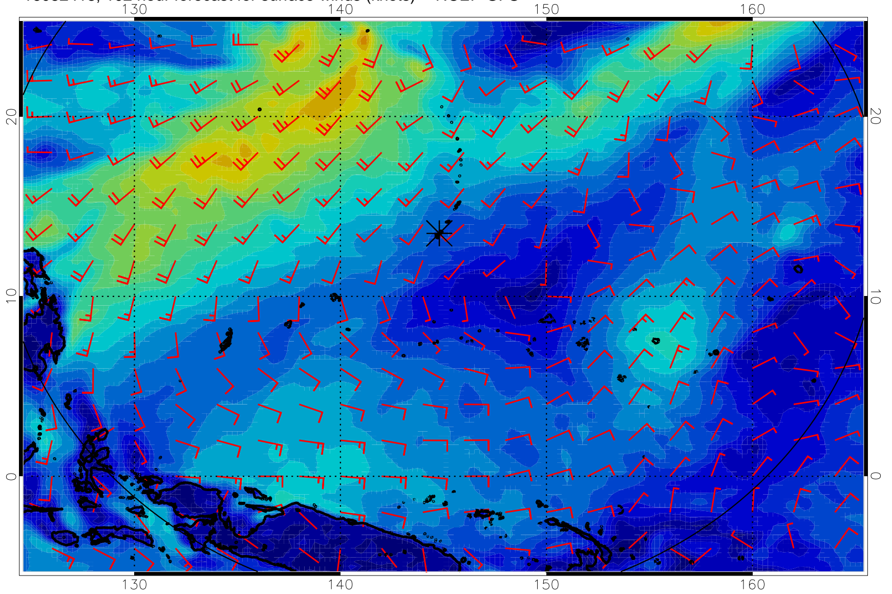
16082418, 102 hour forecast for surface winds (knots) -- NCEP GFS
