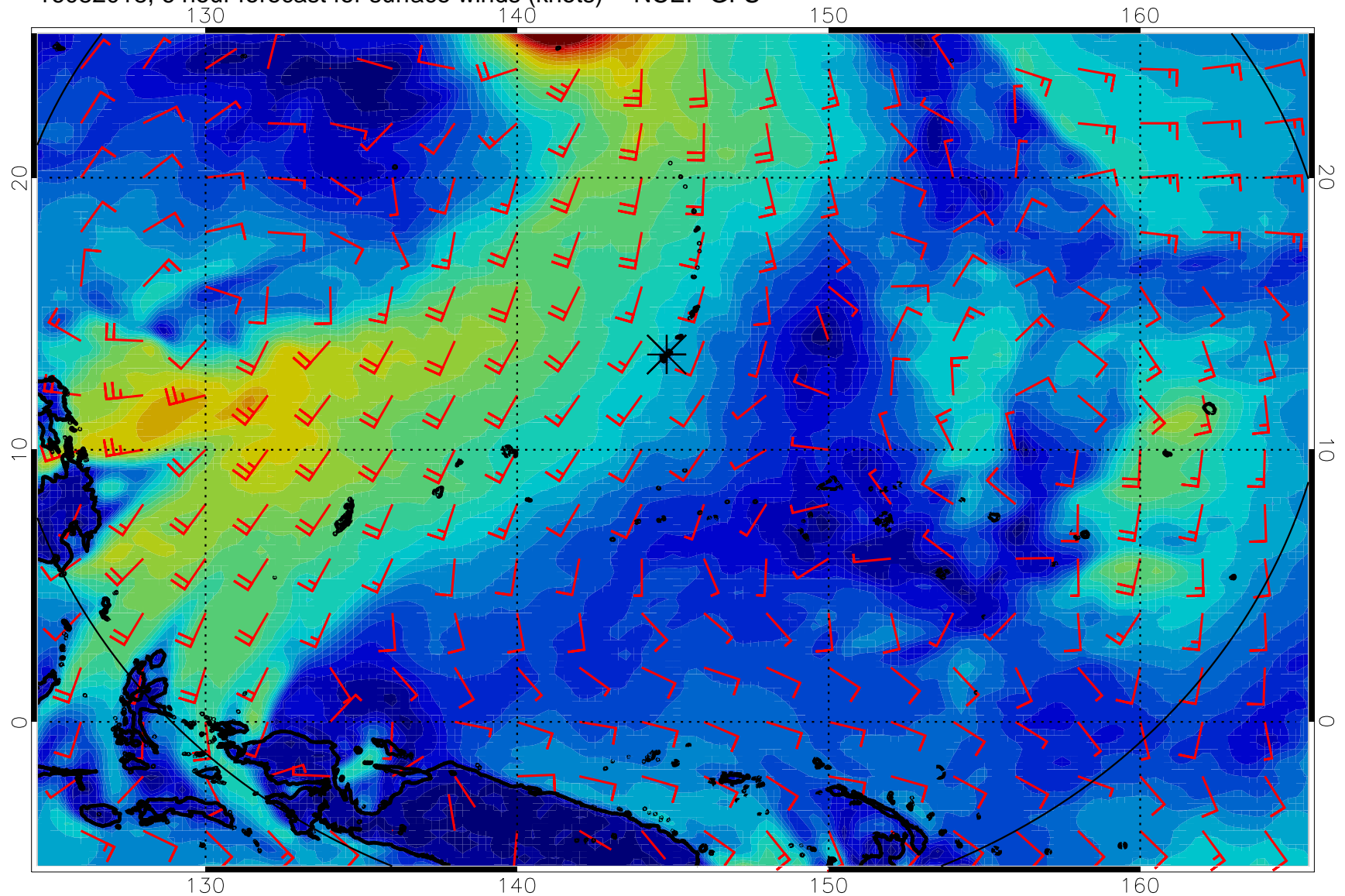
16082018, 6 hour forecast for surface winds (knots) -- NCEP GFS
