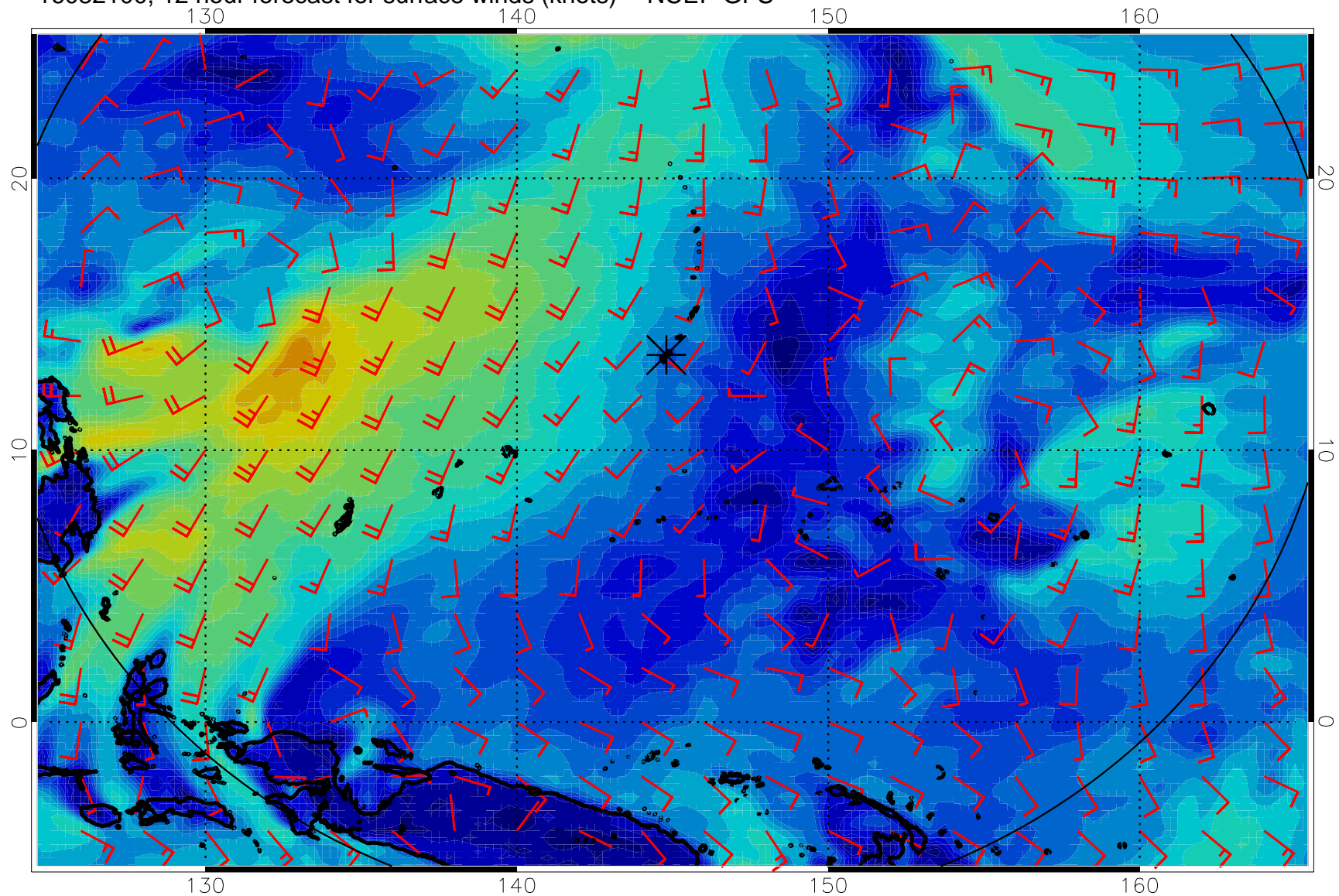
16082100, 12 hour forecast for surface winds (knots) -- NCEP GFS
