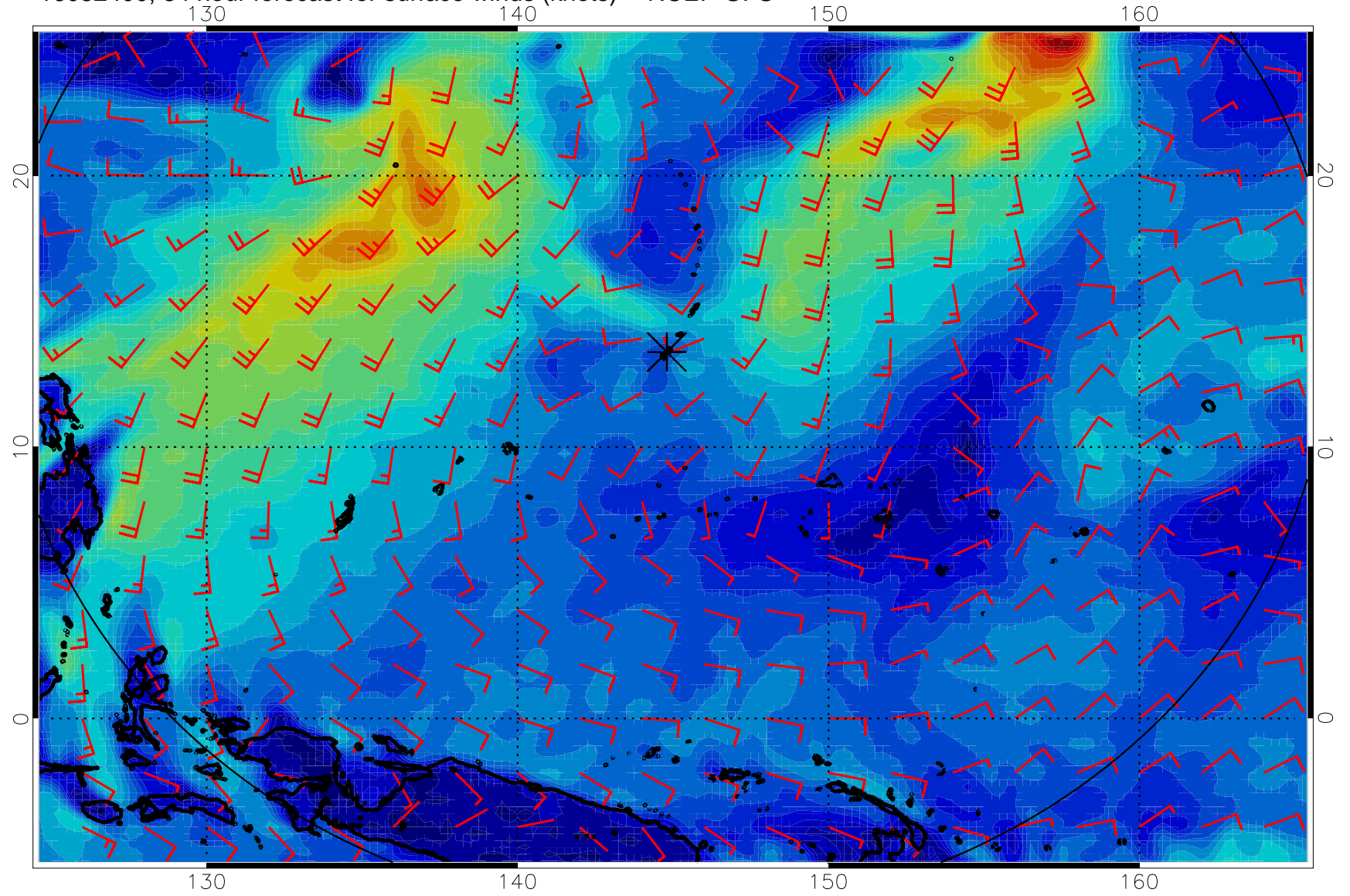
16082400, 84 hour forecast for surface winds (knots) -- NCEP GFS
