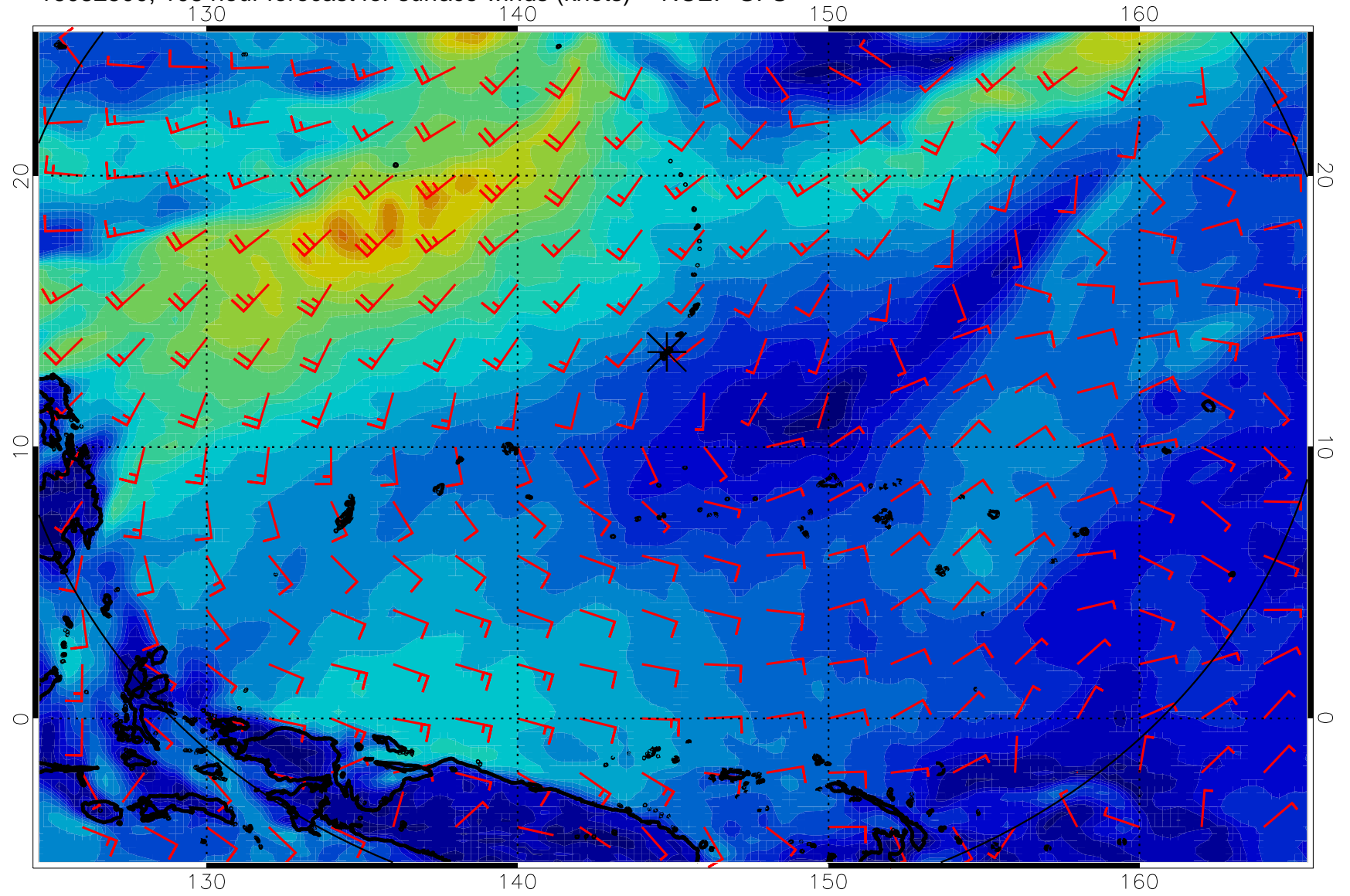
16082500, 108 hour forecast for surface winds (knots) -- NCEP GFS
