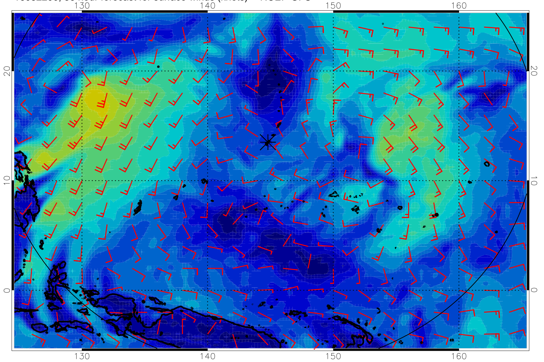
16082200, 36 hour forecast for surface winds (knots) -- NCEP GFS
