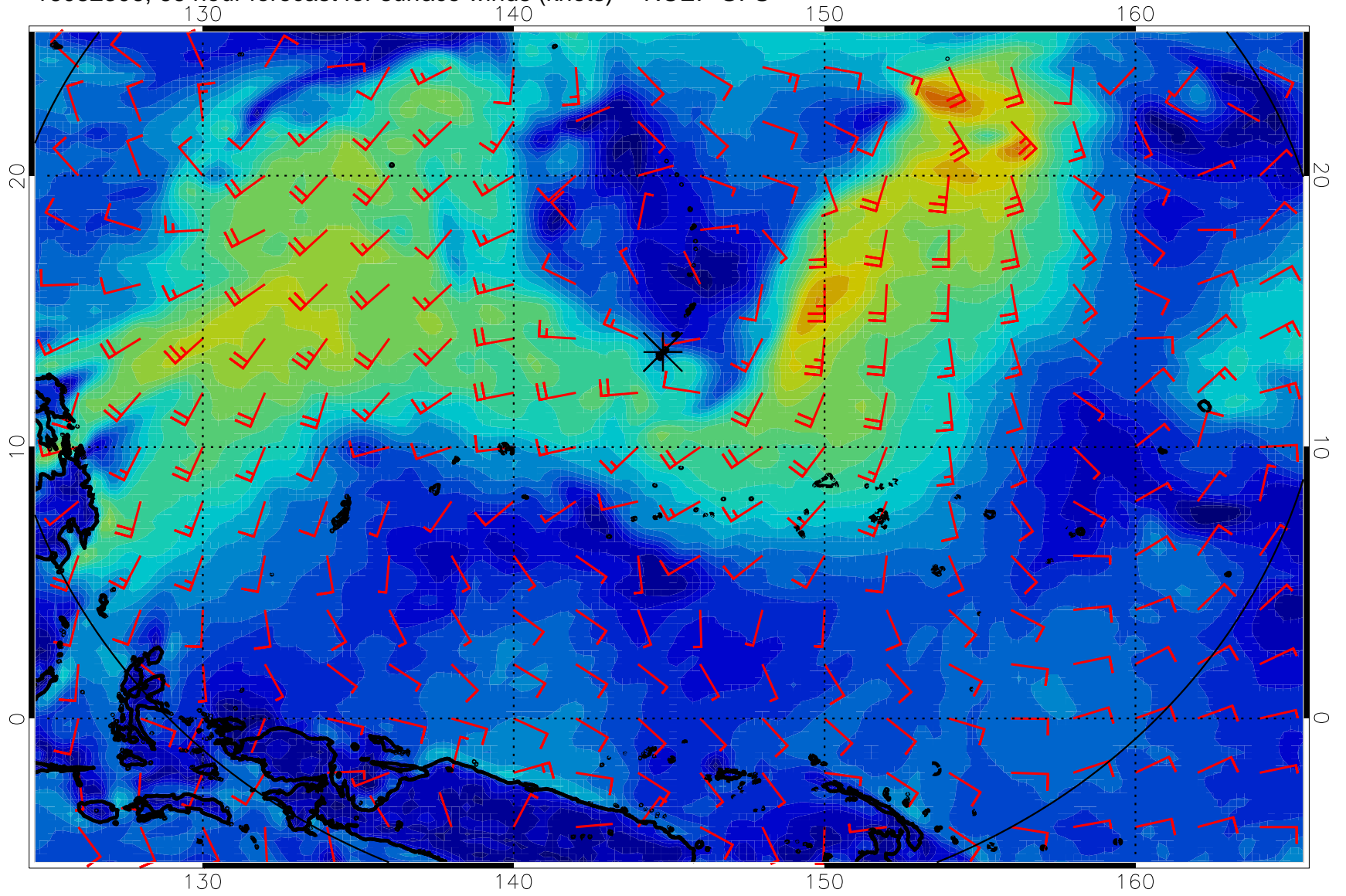
16082306, 66 hour forecast for surface winds (knots) -- NCEP GFS
