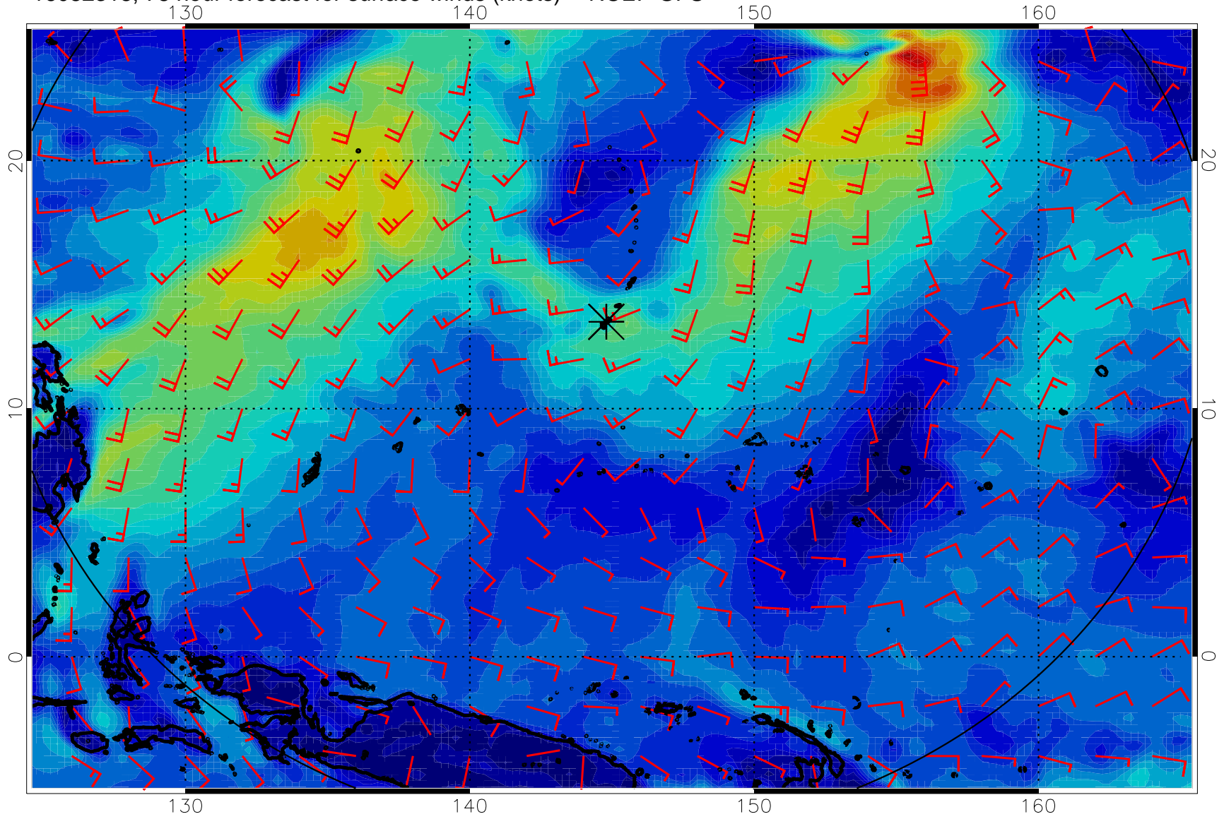
16082318, 78 hour forecast for surface winds (knots) -- NCEP GFS
