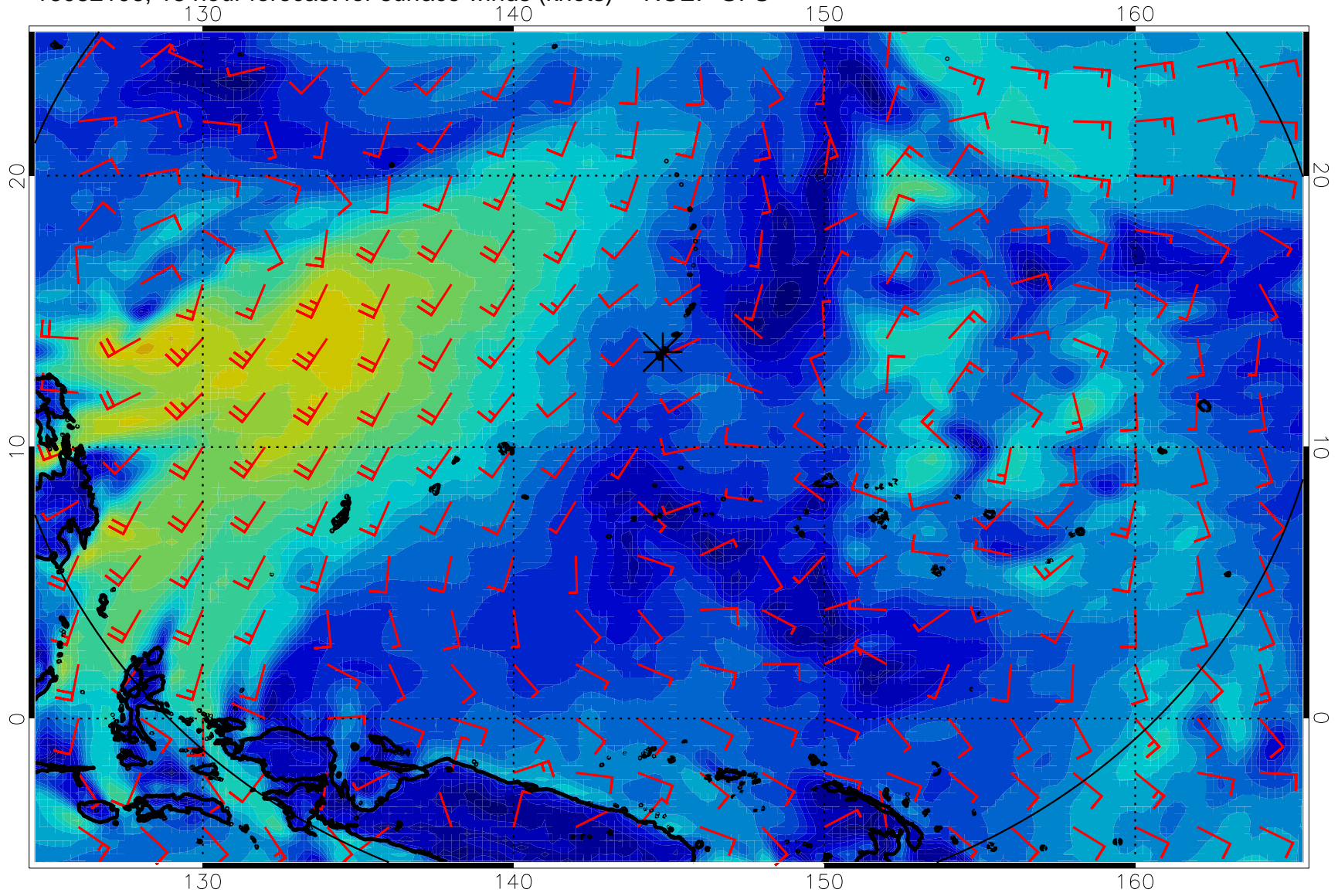
16082106, 18 hour forecast for surface winds (knots) -- NCEP GFS
