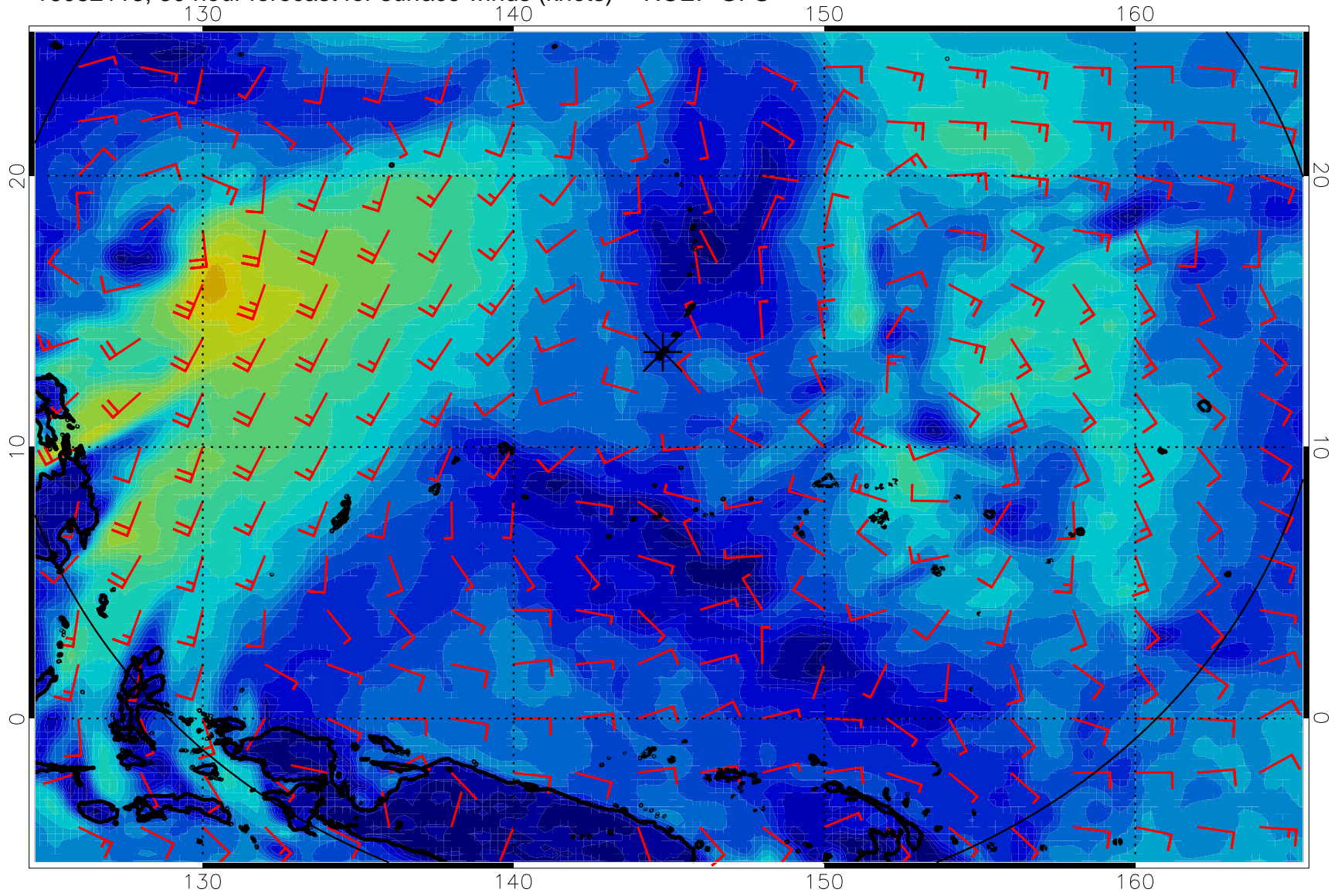
16082118, 30 hour forecast for surface winds (knots) -- NCEP GFS
