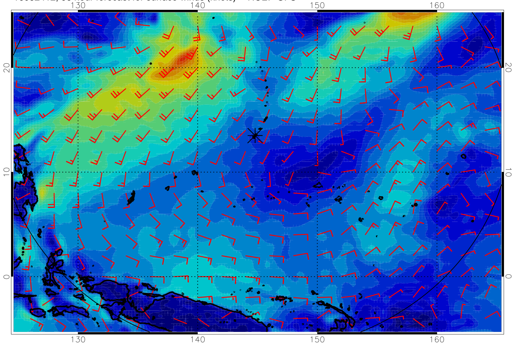
16082412, 96 hour forecast for surface winds (knots) -- NCEP GFS
