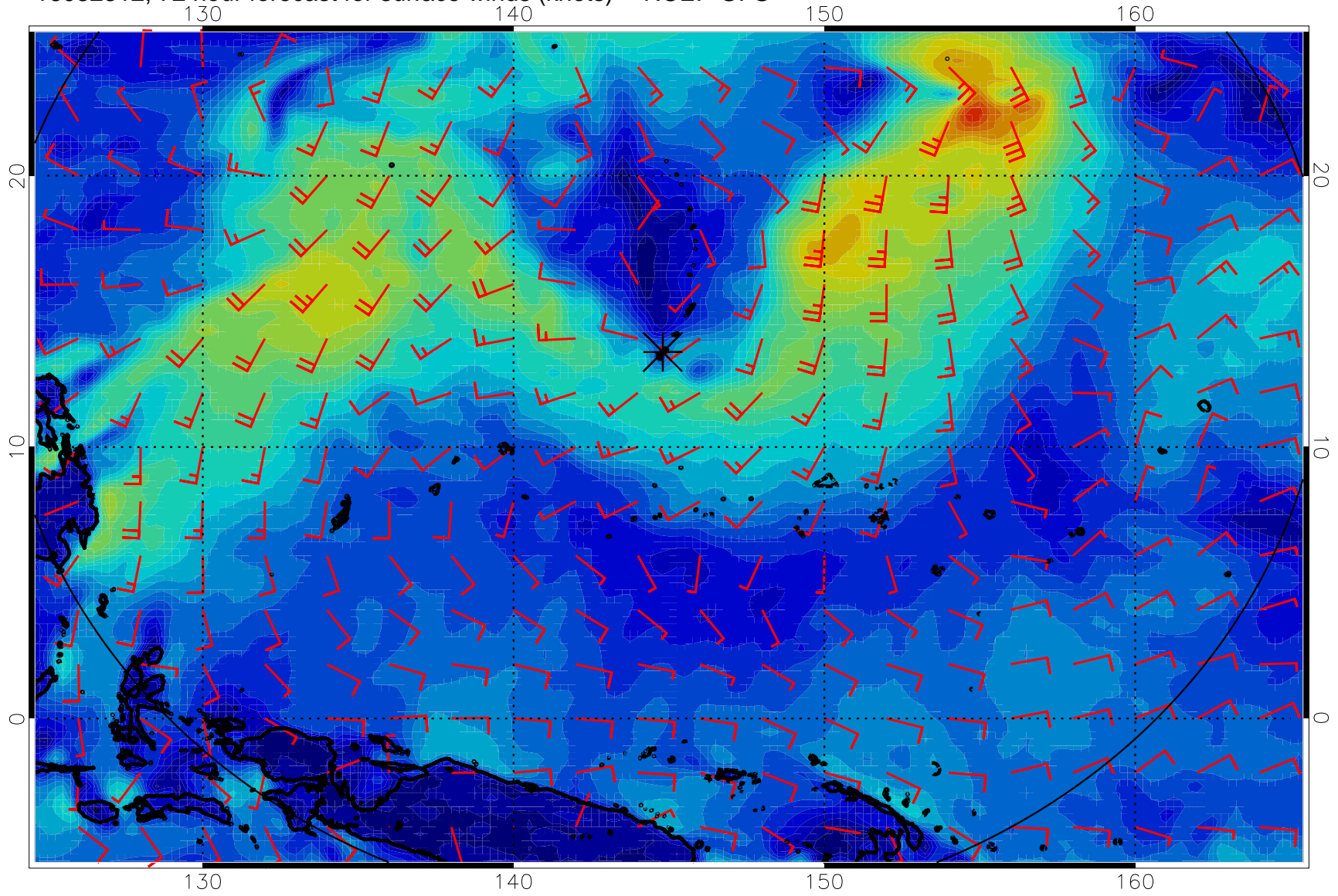
16082312, 72 hour forecast for surface winds (knots) -- NCEP GFS
