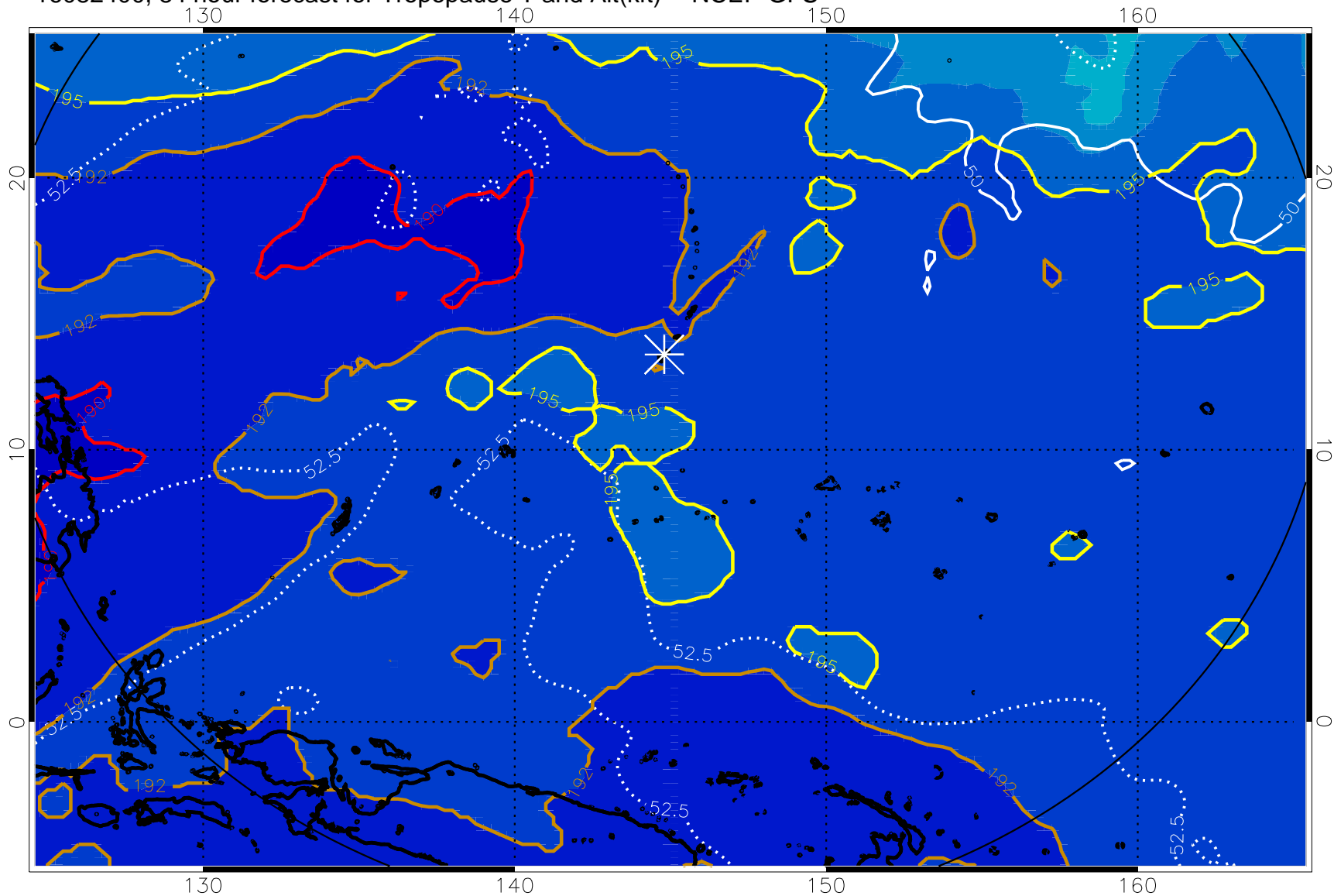
16082400, 84 hour forecast for Tropopause T and Alt(kft) -- NCEP GFS
