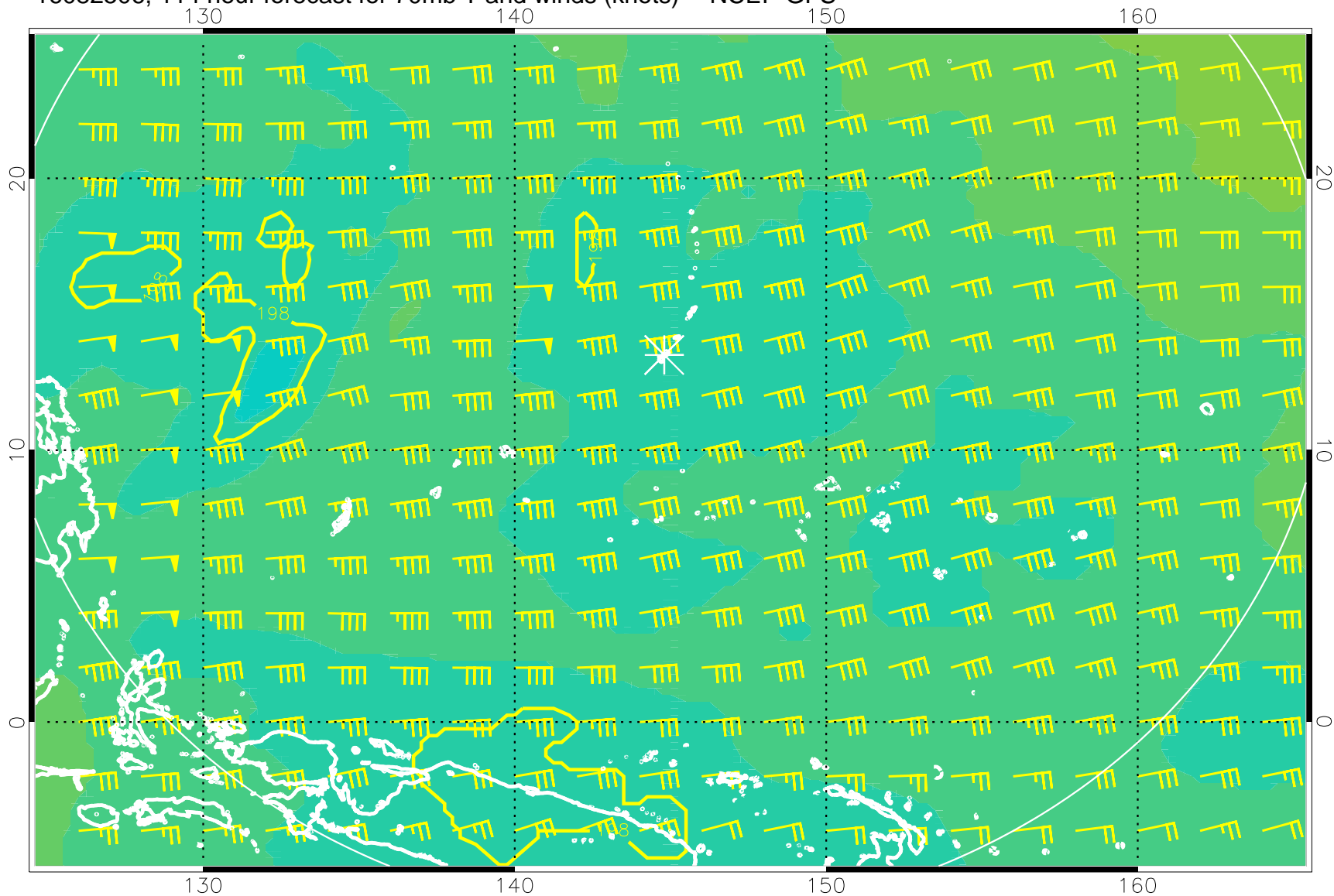
16082506, 114 hour forecast for 70mb T and winds (knots) -- NCEP GFS
