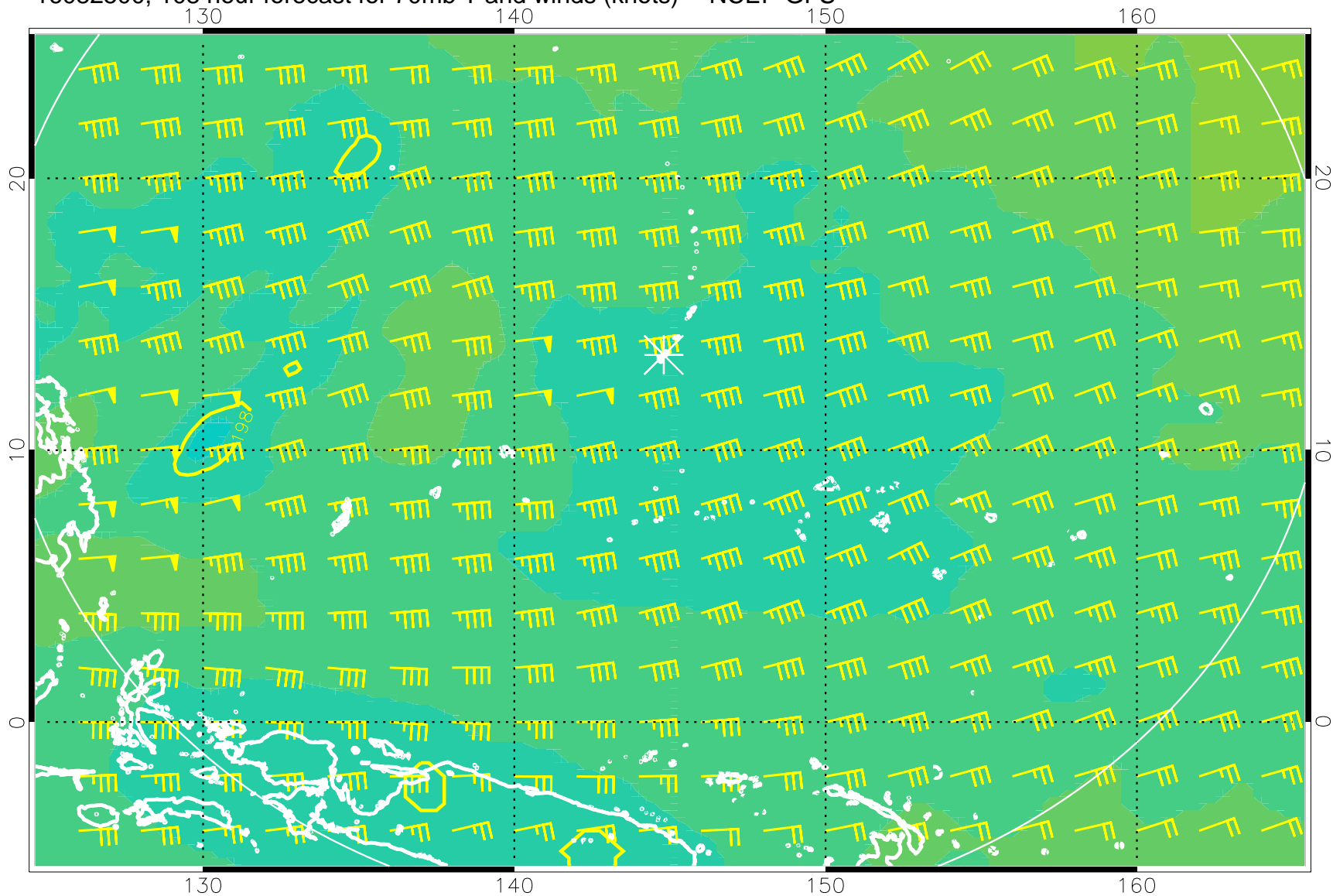
16082500, 108 hour forecast for 70mb T and winds (knots) -- NCEP GFS
