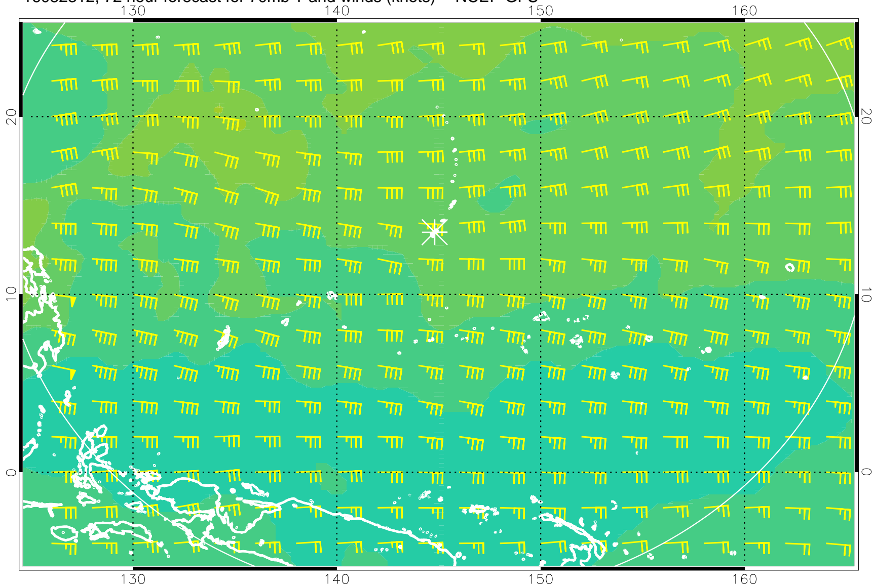
16082312, 72 hour forecast for 70mb T and winds (knots) -- NCEP GFS
