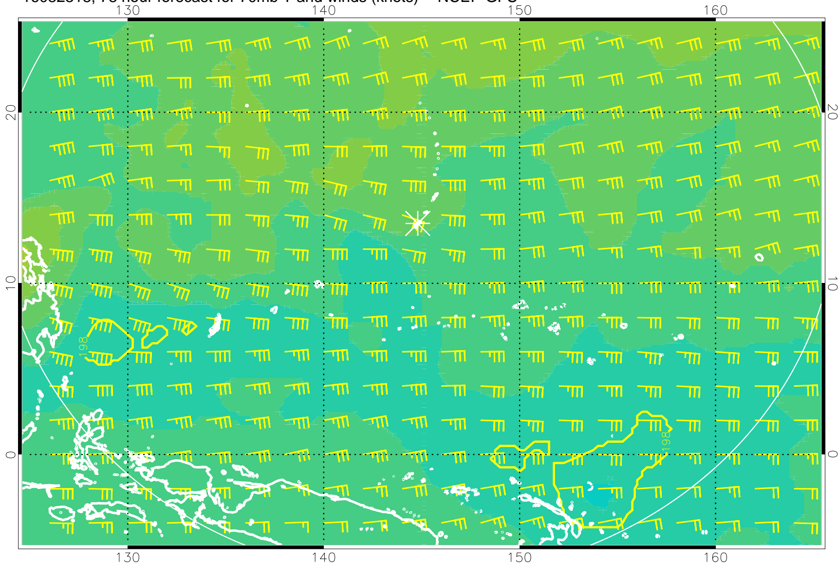
16082318, 78 hour forecast for 70mb T and winds (knots) -- NCEP GFS
