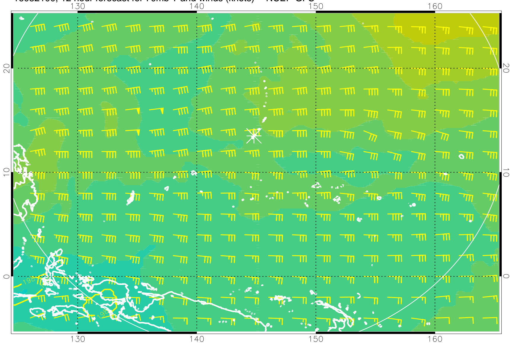
16082100, 12 hour forecast for 70mb T and winds (knots) -- NCEP GFS
