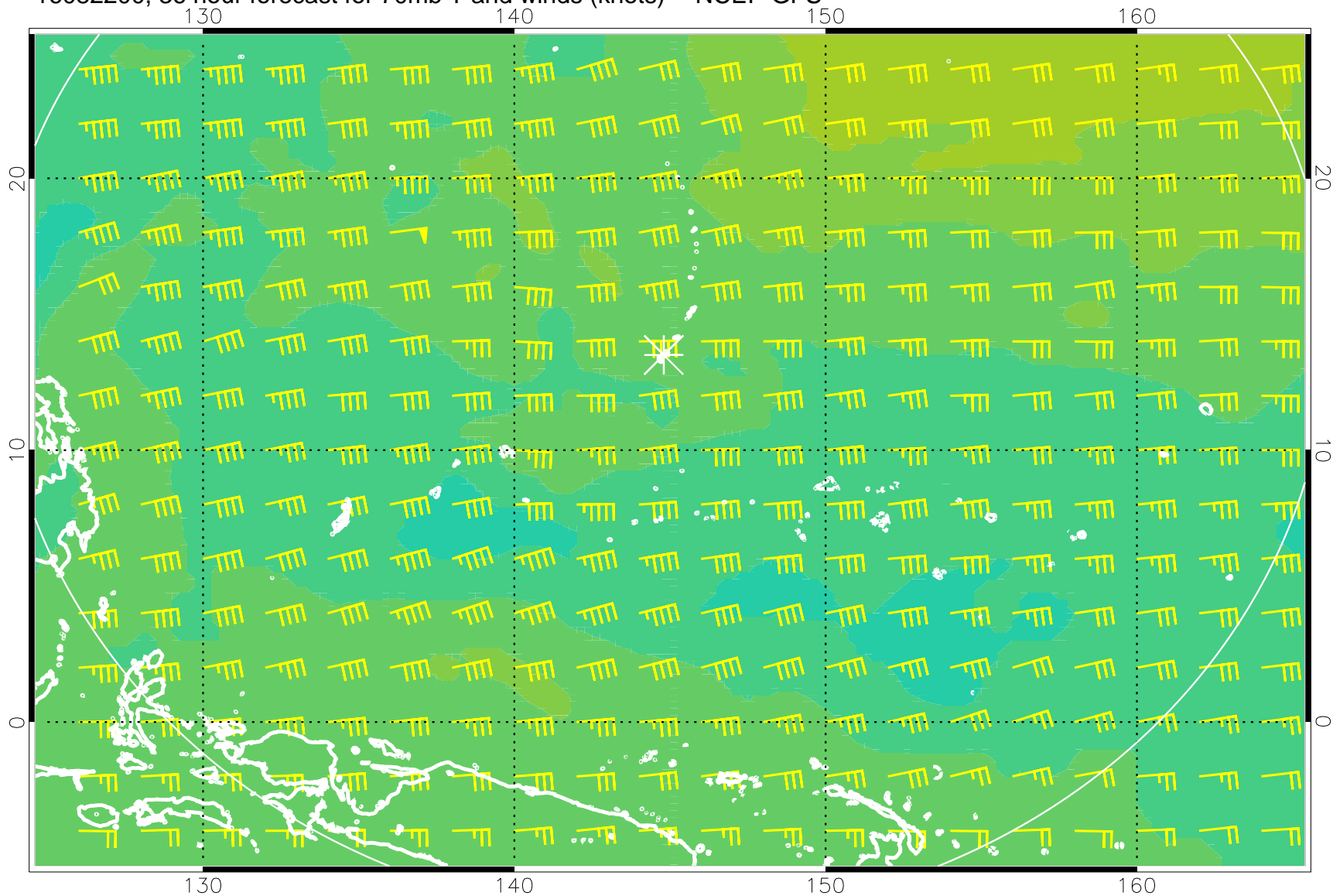
16082200, 36 hour forecast for 70mb T and winds (knots) -- NCEP GFS
