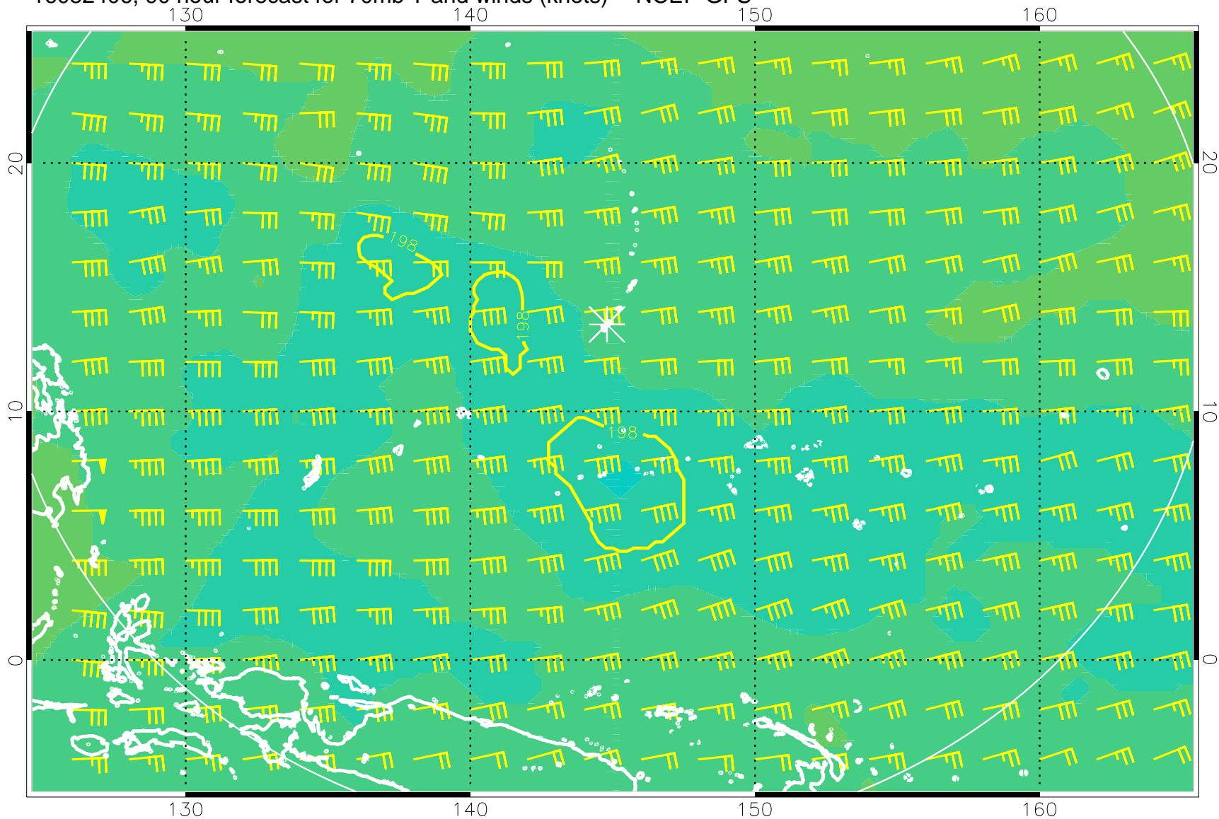
16082406, 90 hour forecast for 70mb T and winds (knots) -- NCEP GFS
