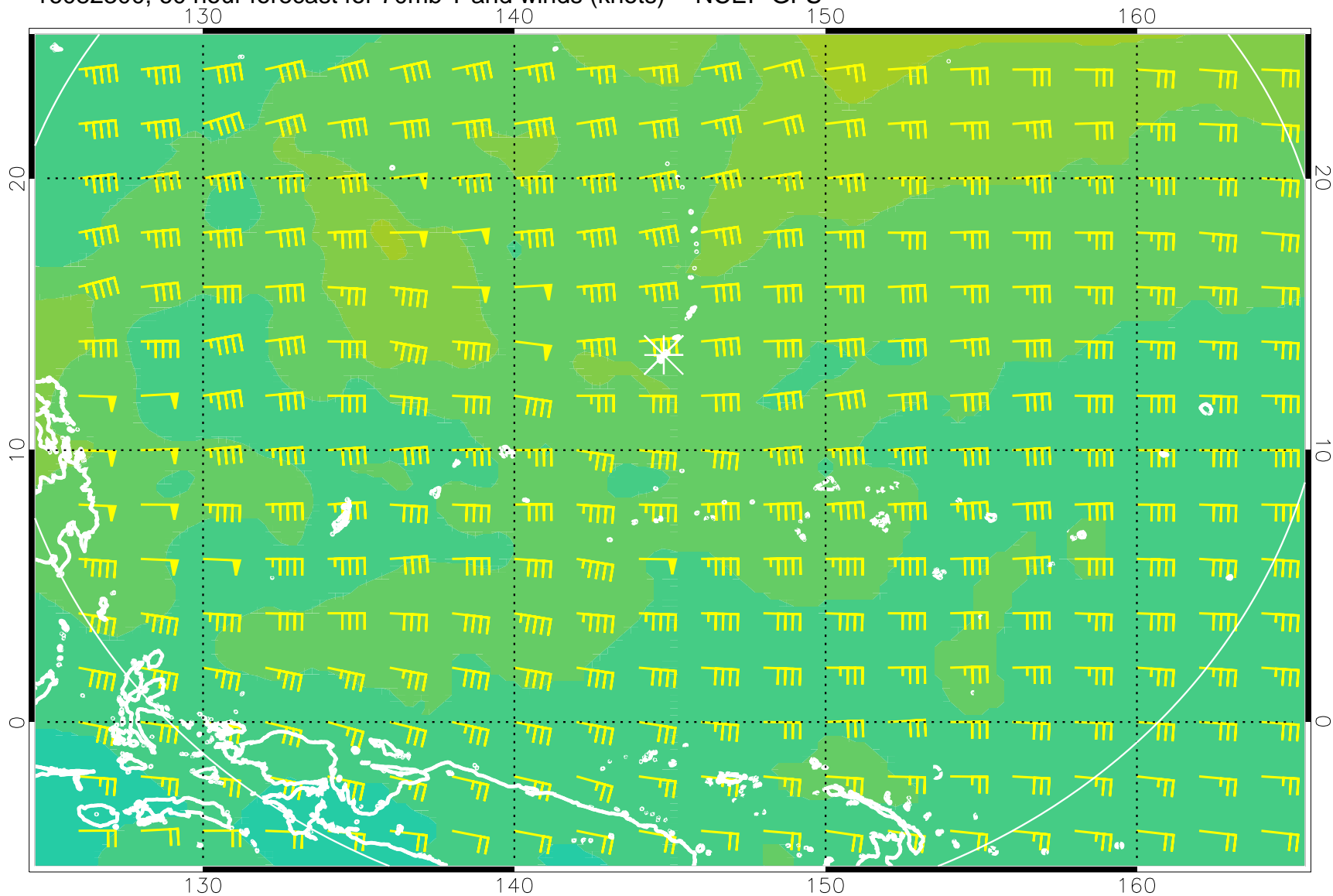
16082300, 60 hour forecast for 70mb T and winds (knots) -- NCEP GFS
