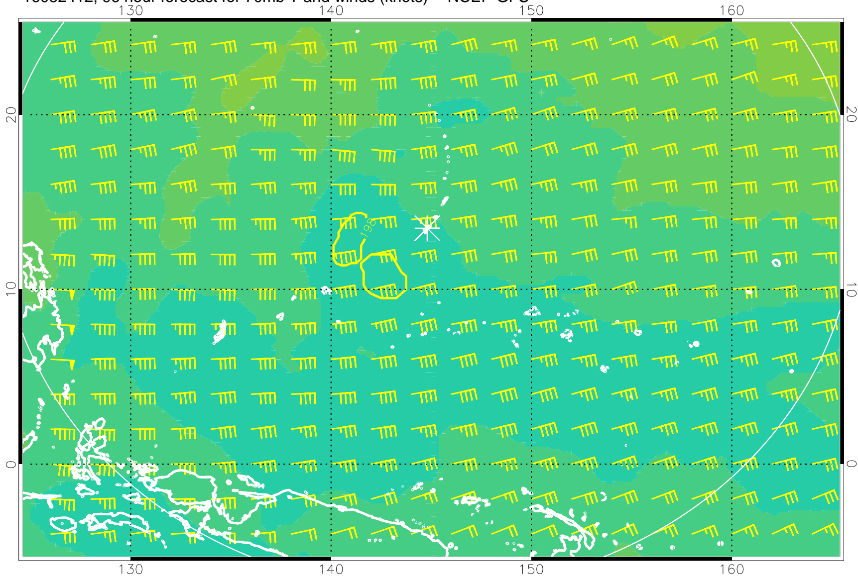
16082412, 96 hour forecast for 70mb T and winds (knots) -- NCEP GFS
