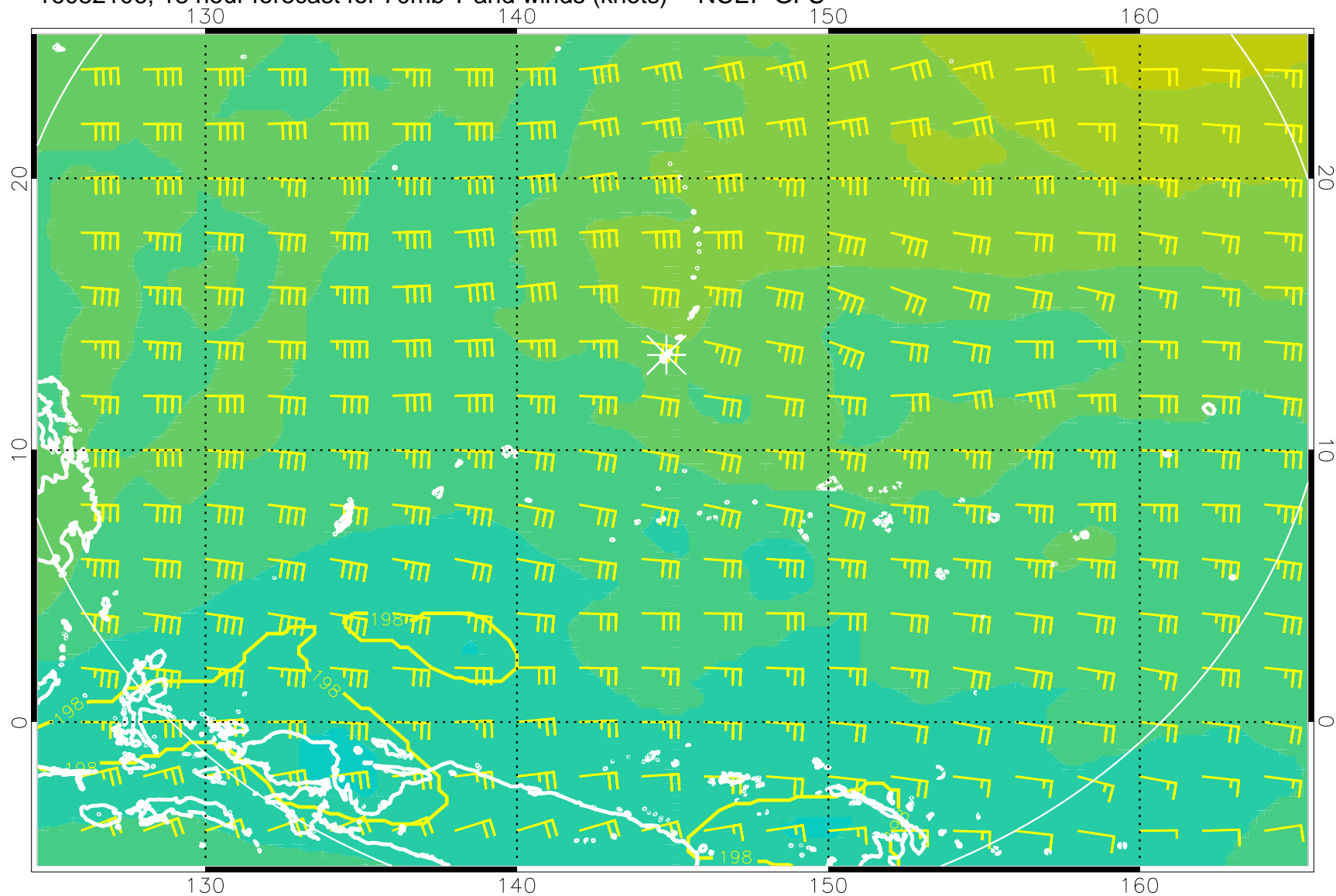
16082106, 18 hour forecast for 70mb T and winds (knots) -- NCEP GFS
