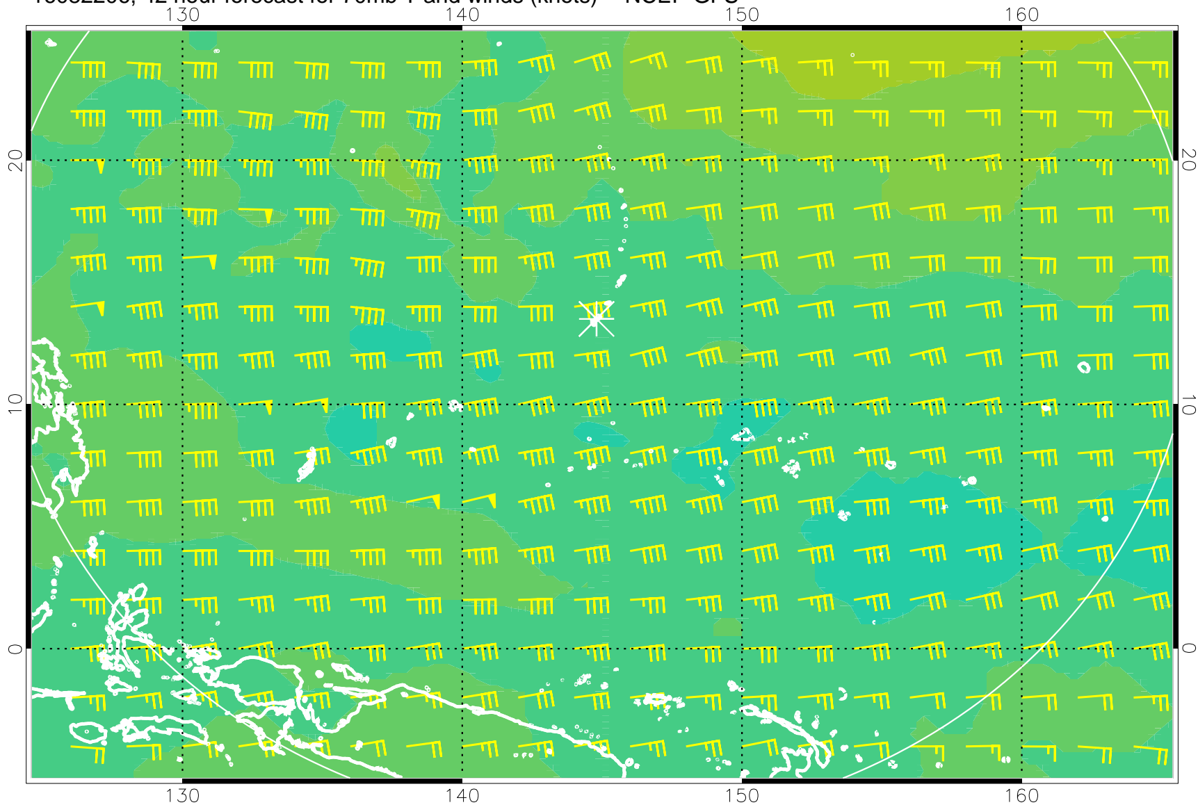
16082206, 42 hour forecast for 70mb T and winds (knots) -- NCEP GFS
