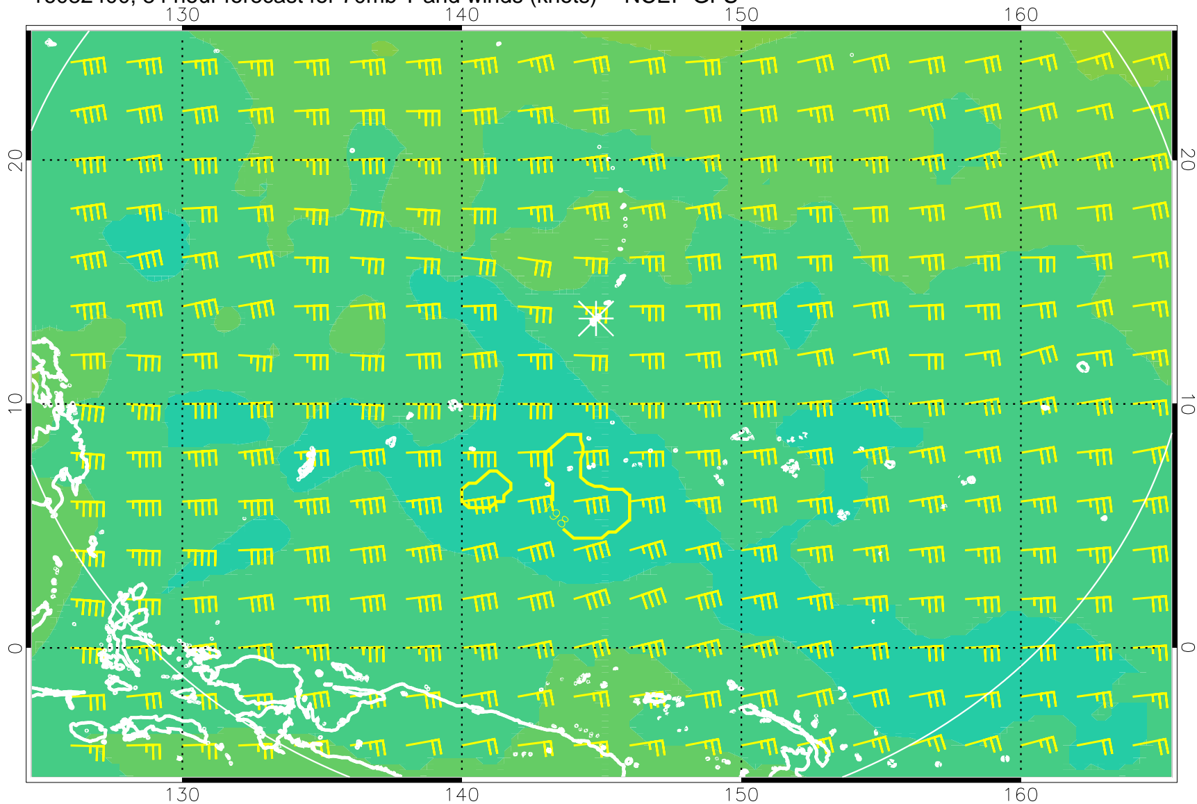
16082400, 84 hour forecast for 70mb T and winds (knots) -- NCEP GFS
