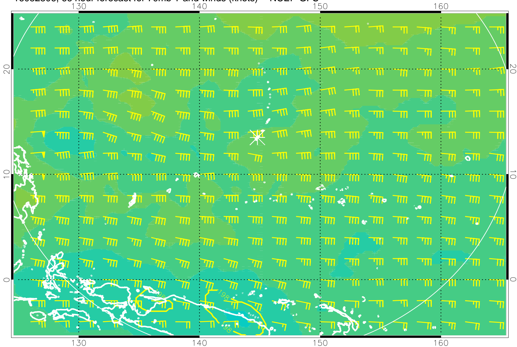
16082306, 66 hour forecast for 70mb T and winds (knots) -- NCEP GFS
