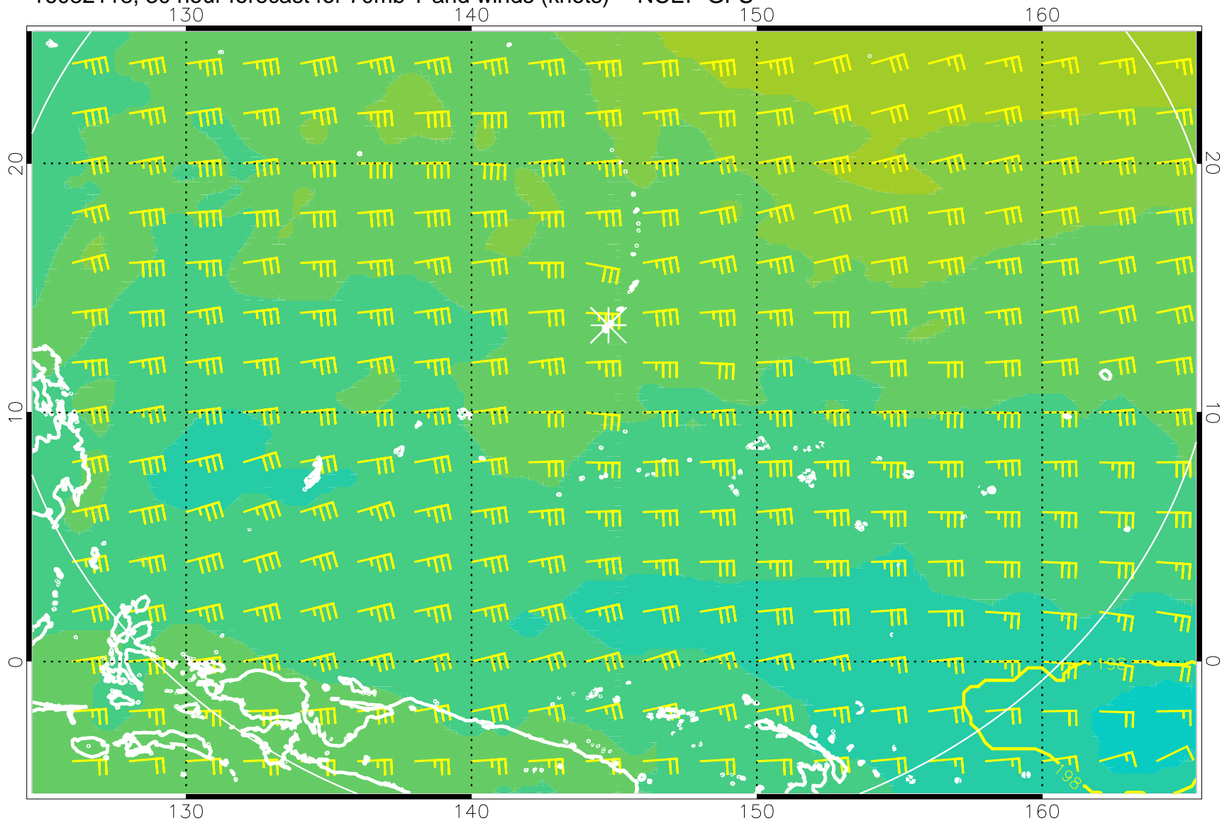
16082118, 30 hour forecast for 70mb T and winds (knots) -- NCEP GFS
