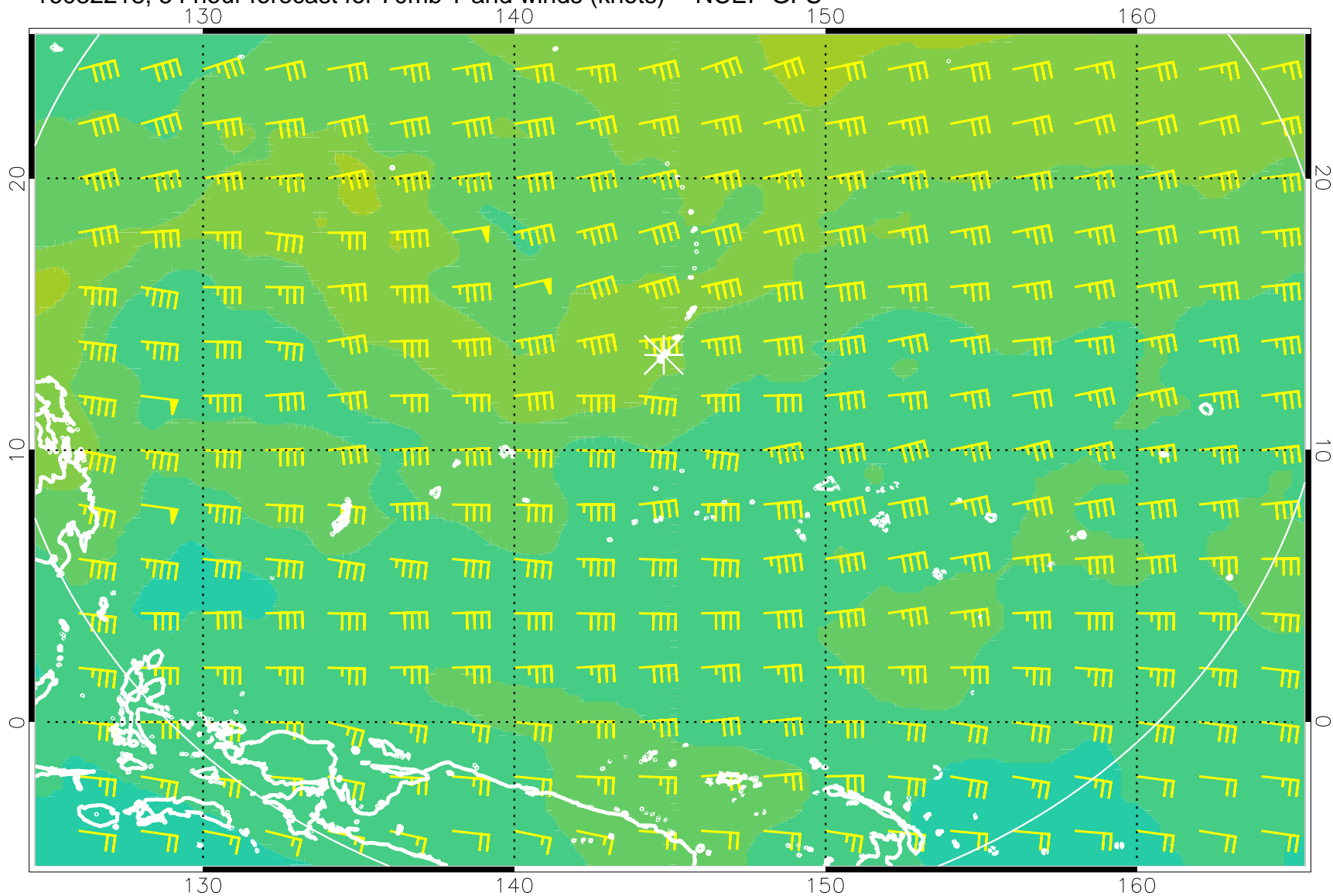
16082218, 54 hour forecast for 70mb T and winds (knots) -- NCEP GFS
