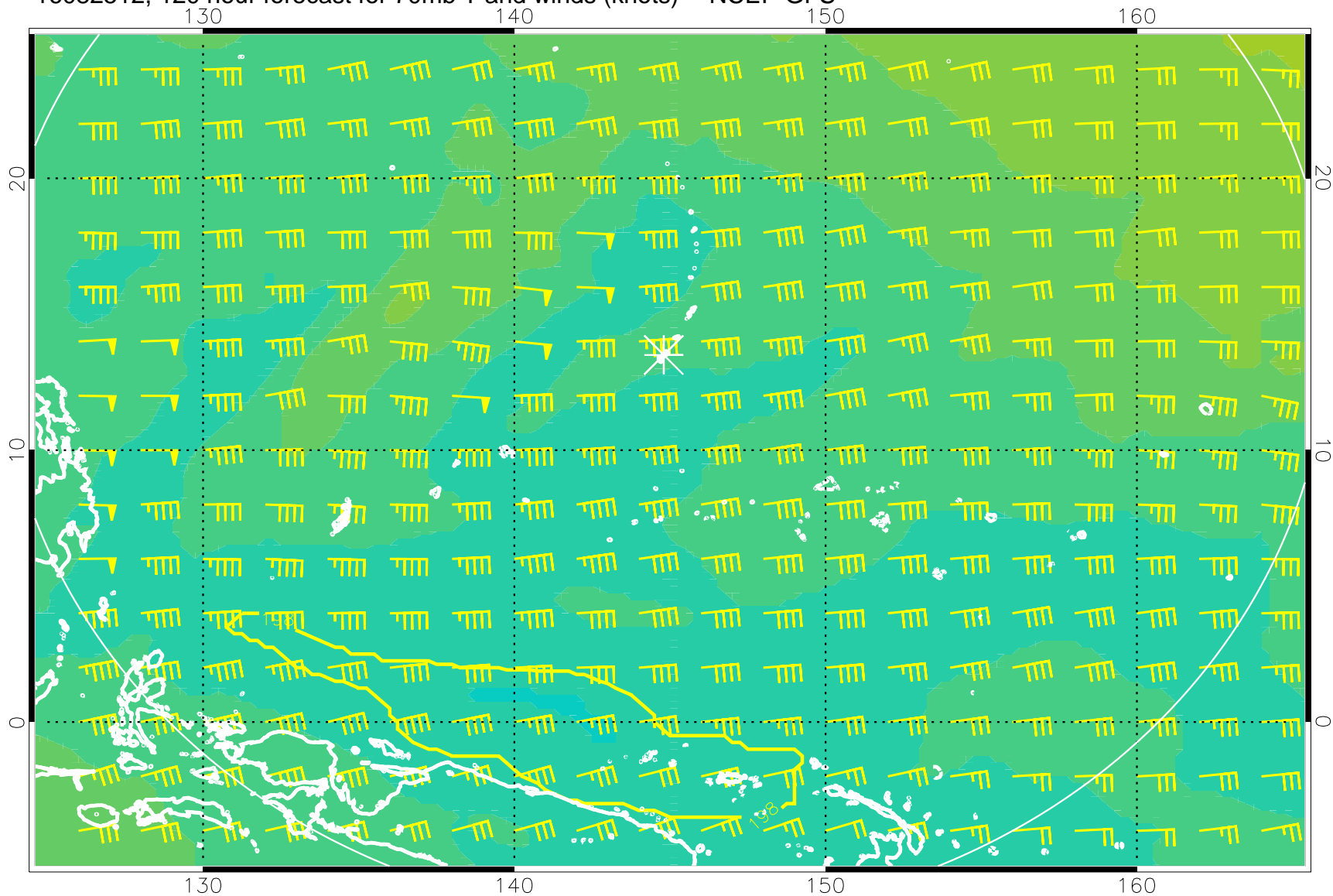
16082512, 120 hour forecast for 70mb T and winds (knots) -- NCEP GFS
