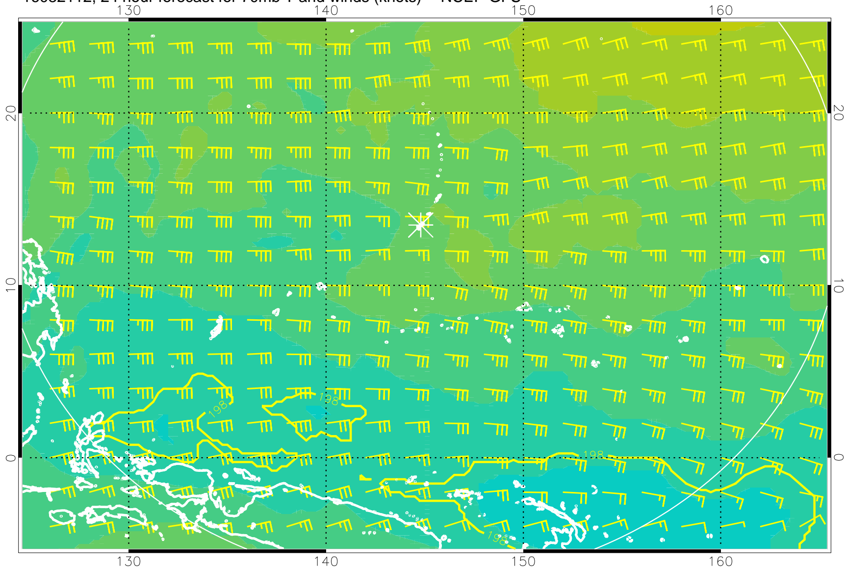
16082112, 24 hour forecast for 70mb T and winds (knots) -- NCEP GFS
