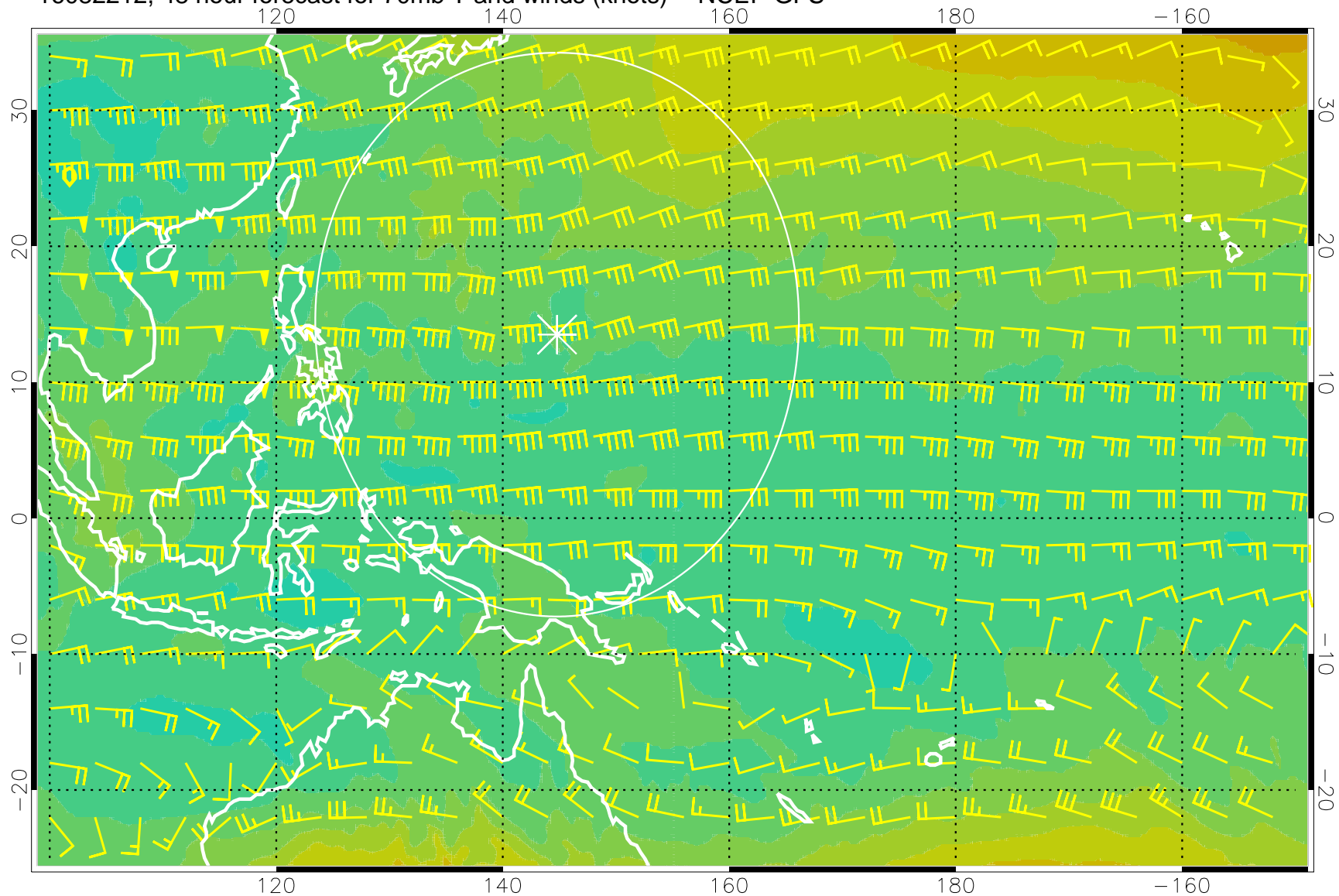
16082212, 48 hour forecast for 70mb T and winds (knots) -- NCEP GFS
