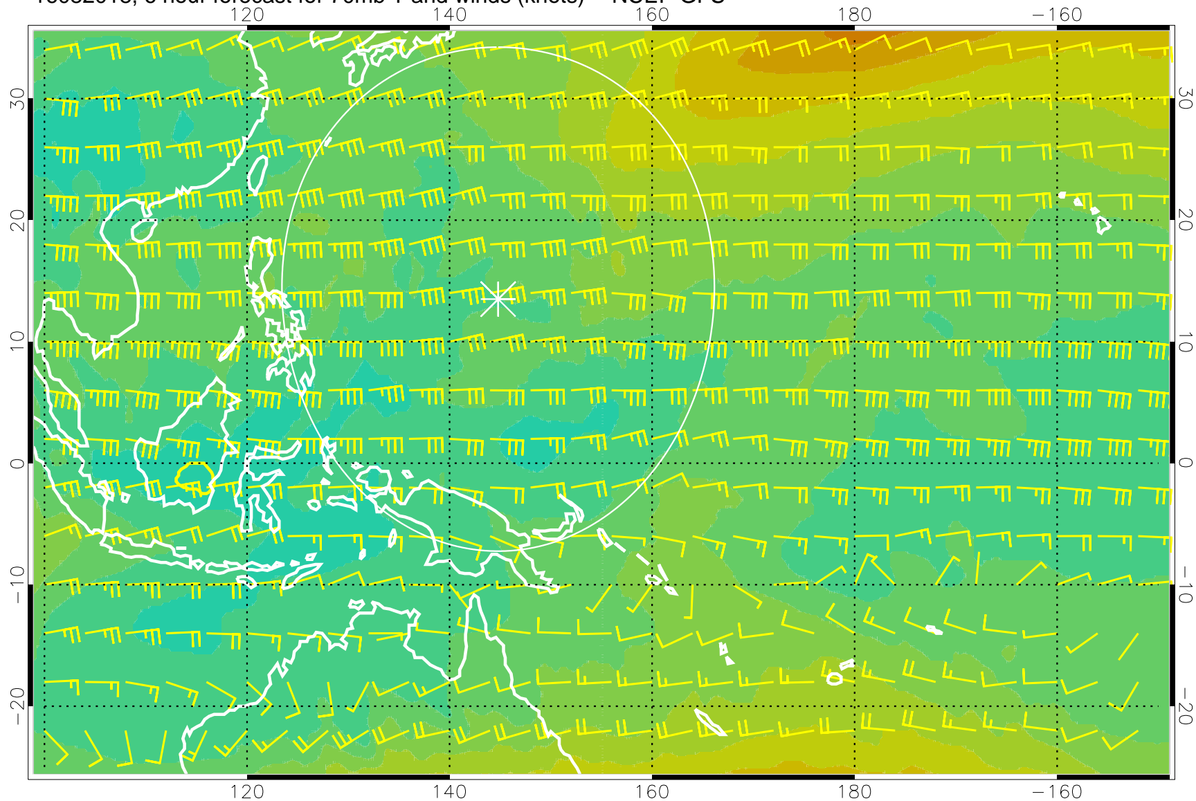
16082018, 6 hour forecast for 70mb T and winds (knots) -- NCEP GFS
