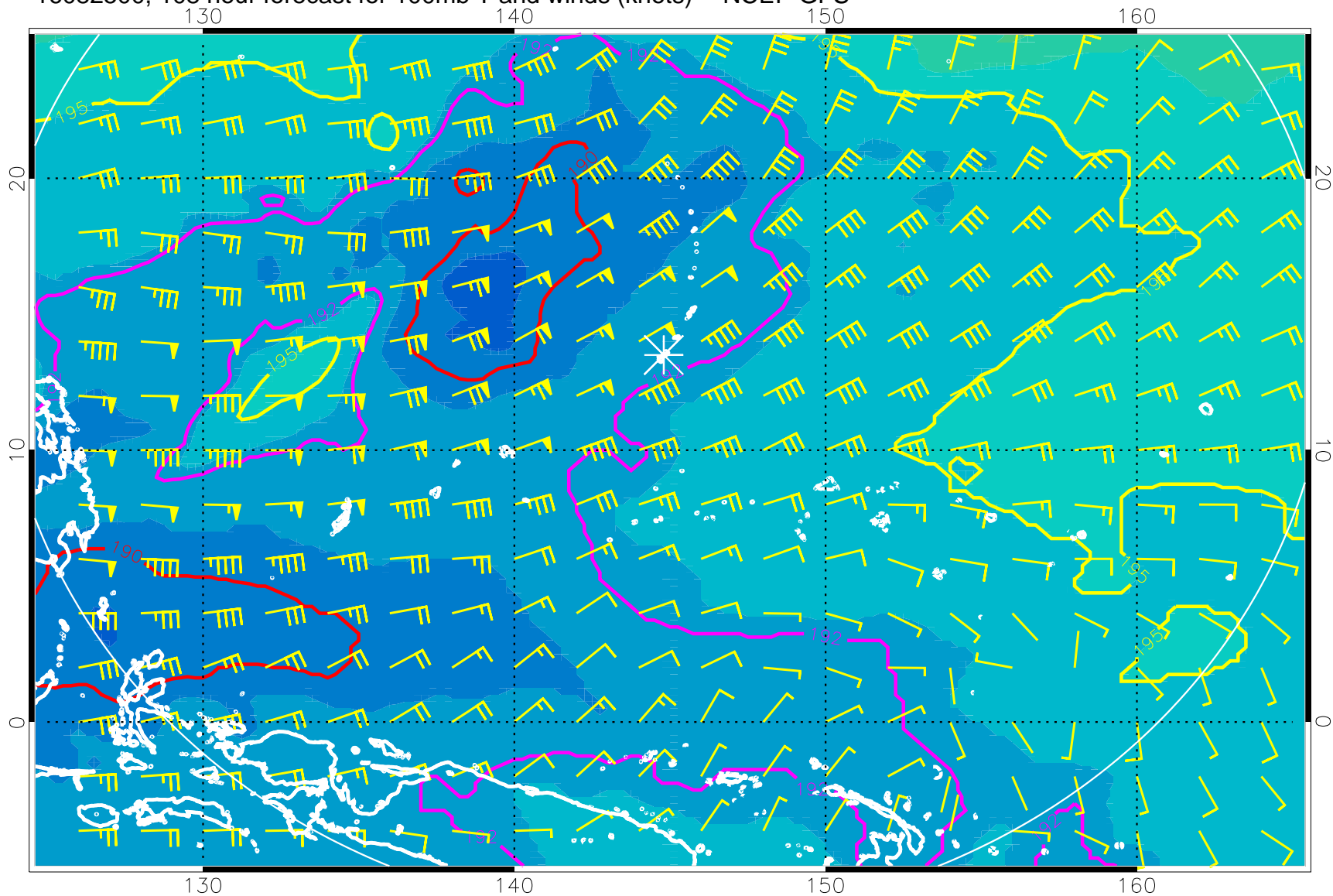
16082500, 108 hour forecast for 100mb T and winds (knots) -- NCEP GFS
