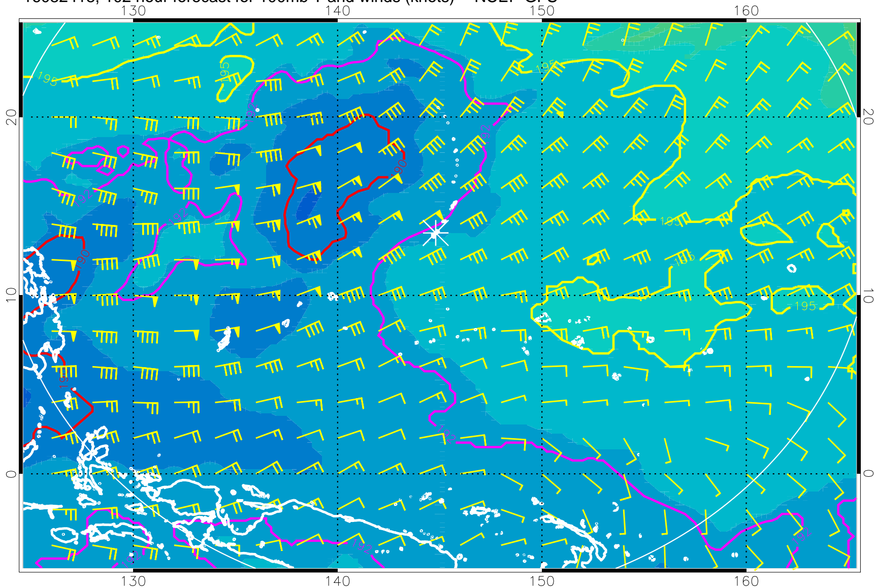
16082418, 102 hour forecast for 100mb T and winds (knots) -- NCEP GFS
