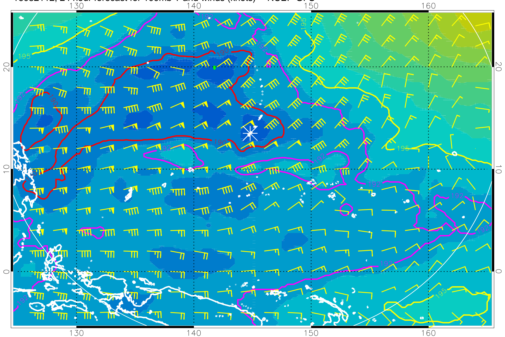
16082112, 24 hour forecast for 100mb T and winds (knots) -- NCEP GFS
