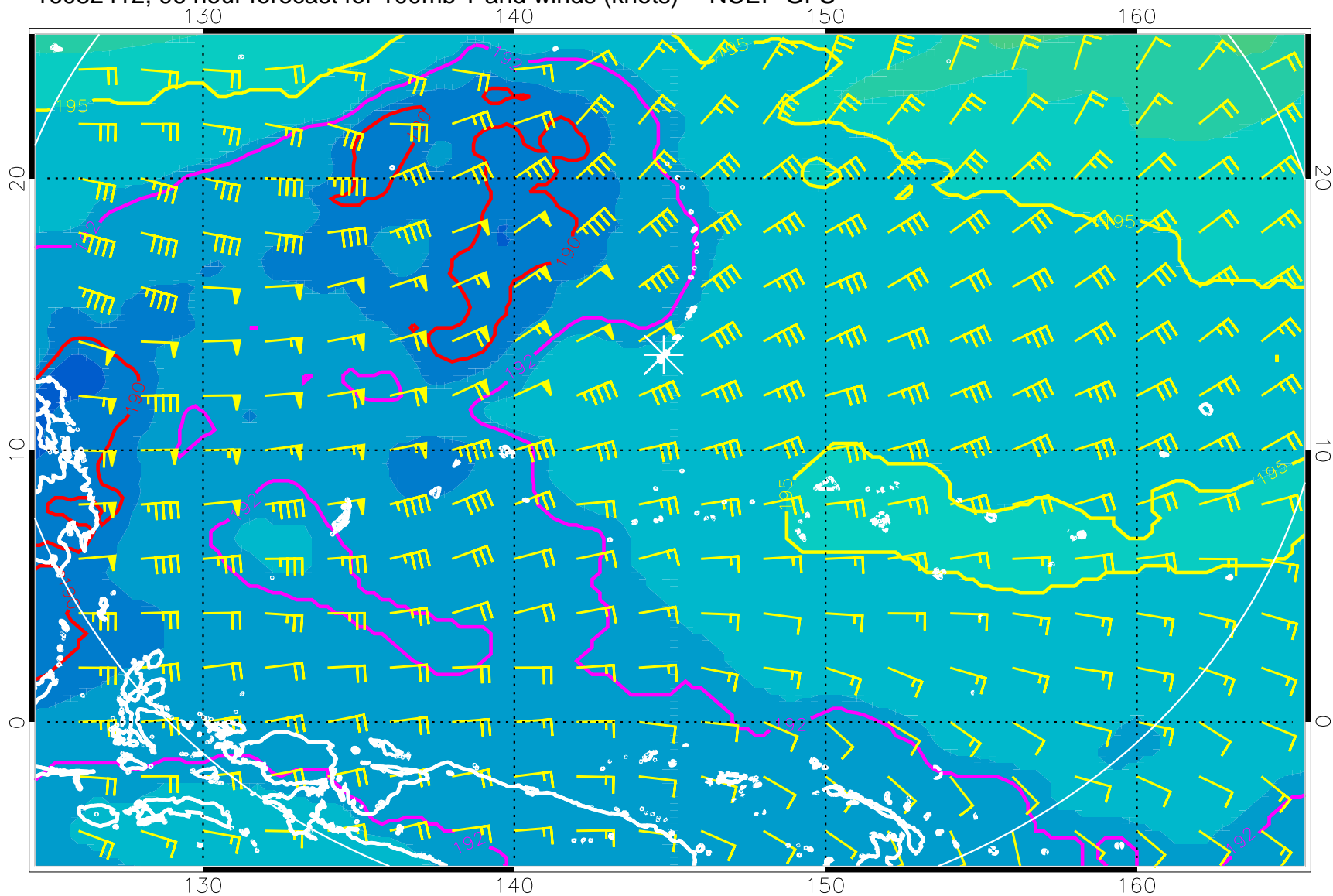
16082412, 96 hour forecast for 100mb T and winds (knots) -- NCEP GFS
