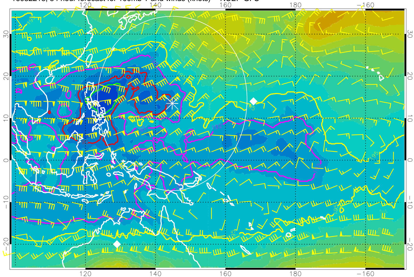
16082218, 54 hour forecast for 100mb T and winds (knots) -- NCEP GFS
