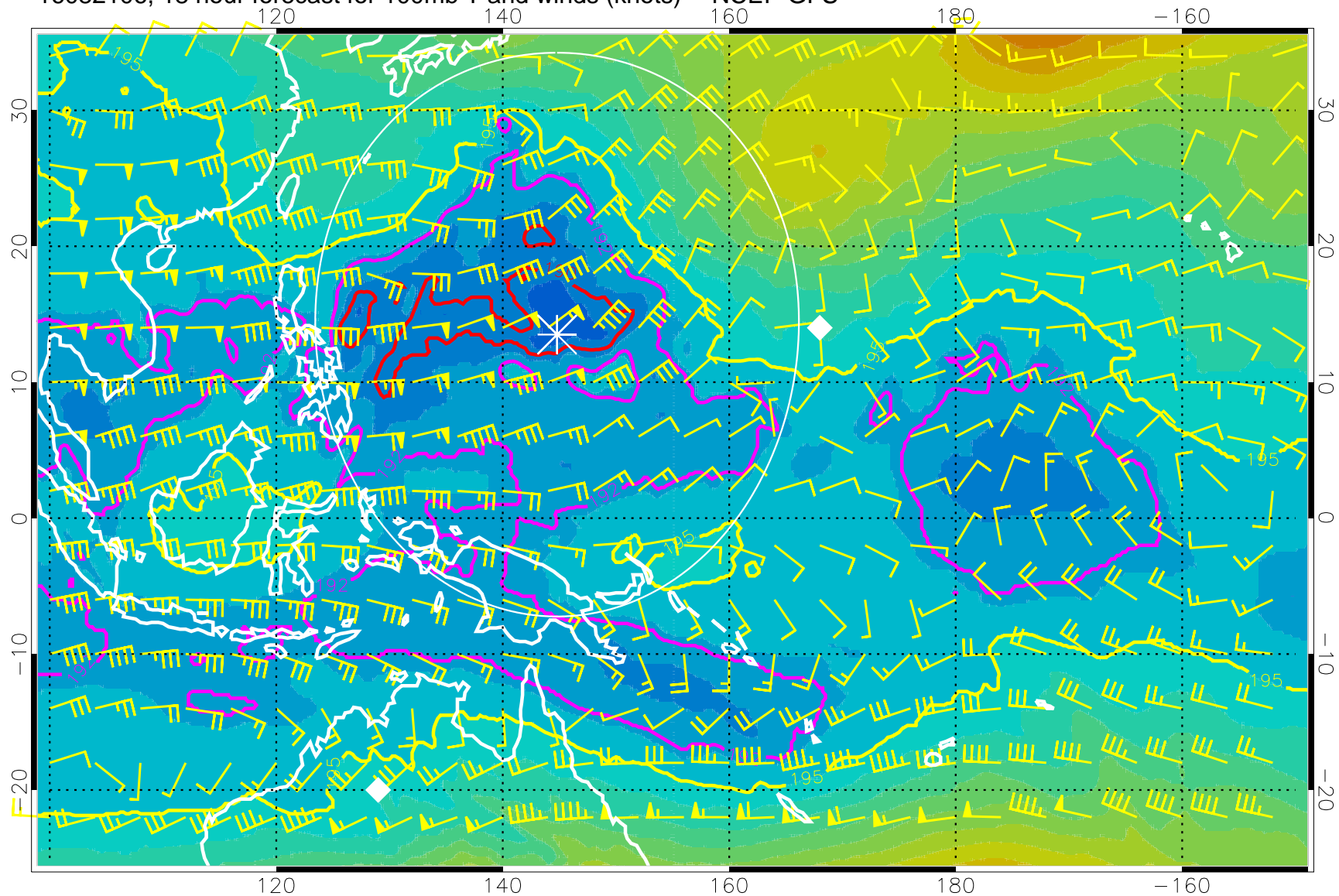
16082106, 18 hour forecast for 100mb T and winds (knots) -- NCEP GFS
