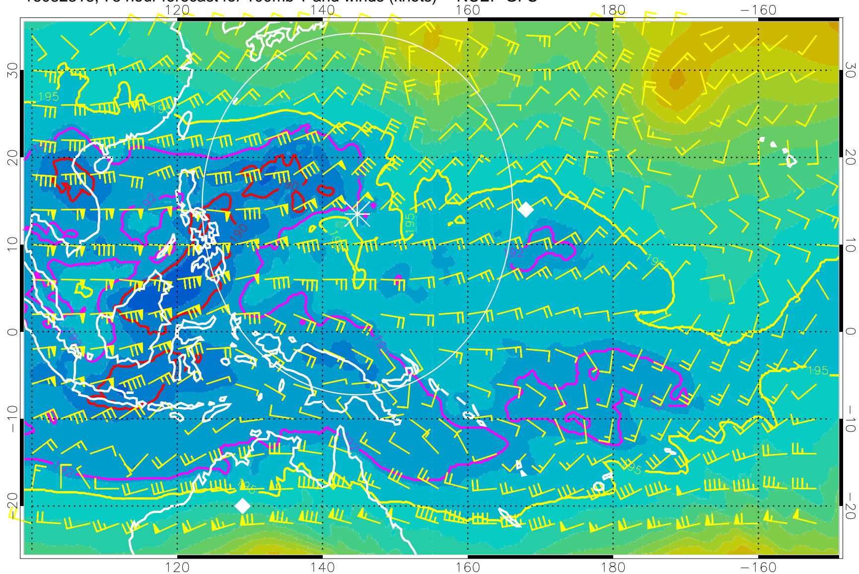
16082318, 78 hour forecast for 100mb T and winds (knots) -- NCEP GFS
