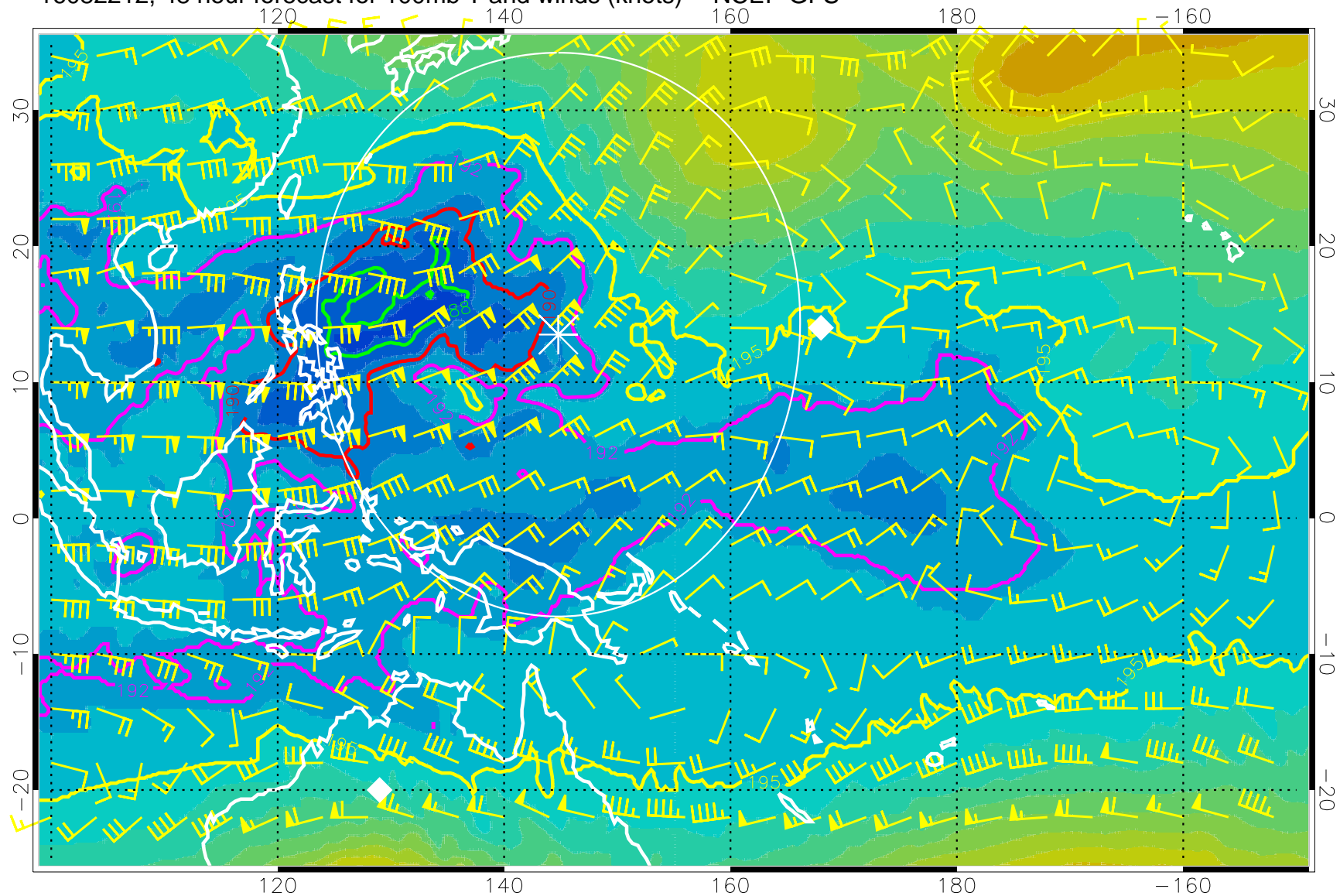
16082212, 48 hour forecast for 100mb T and winds (knots) -- NCEP GFS
