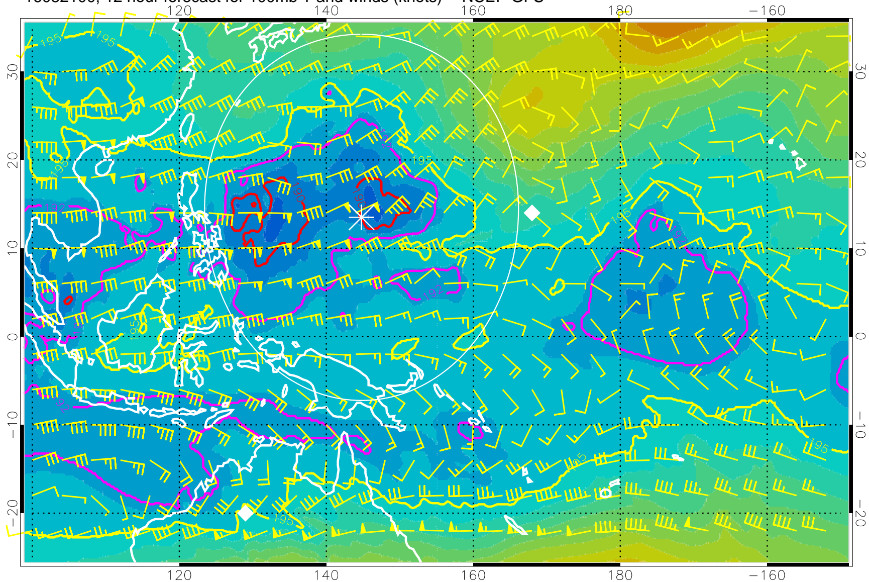
16082100, 12 hour forecast for 100mb T and winds (knots) -- NCEP GFS
