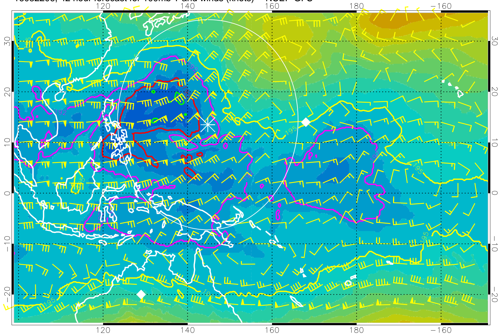
16082206, 42 hour forecast for 100mb T and winds (knots) -- NCEP GFS
