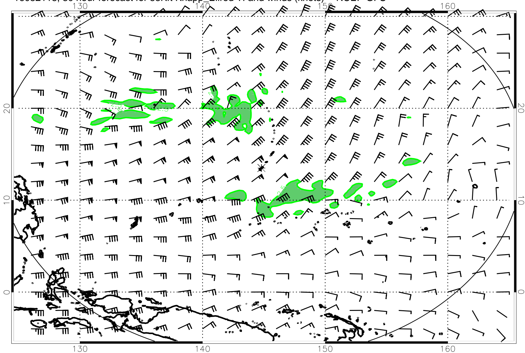
16082118, 30 hour forecast for 53Kft Knapp_Ellrod TI and winds (knots) -- NCEP GFS
