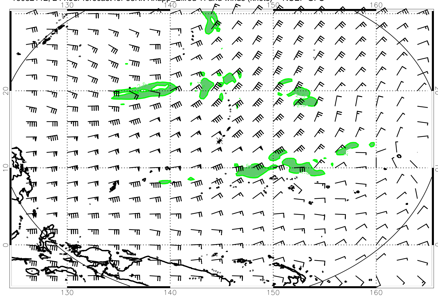
16082112, 24 hour forecast for 53Kft Knapp_Ellrod TI and winds (knots) -- NCEP GFS
