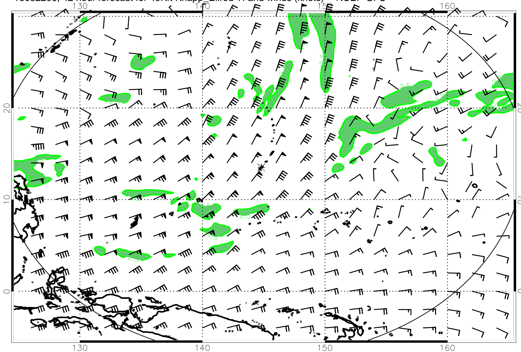
16082206, 42 hour forecast for 49Kft Knapp_Ellrod TI and winds (knots) -- NCEP GFS
