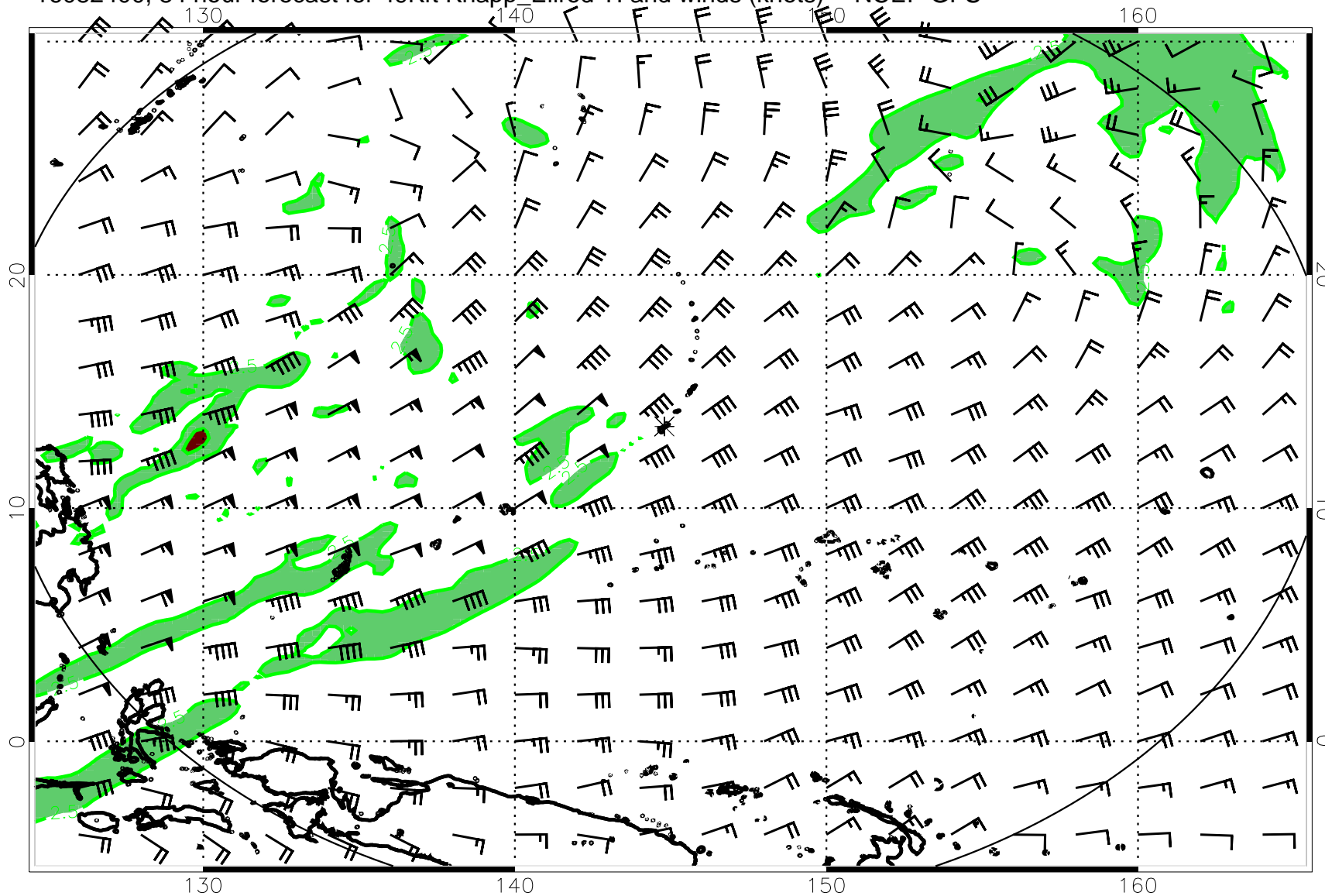
16082400, 84 hour forecast for 49Kft Knapp_Ellrod TI and winds (knots) -- NCEP GFS
