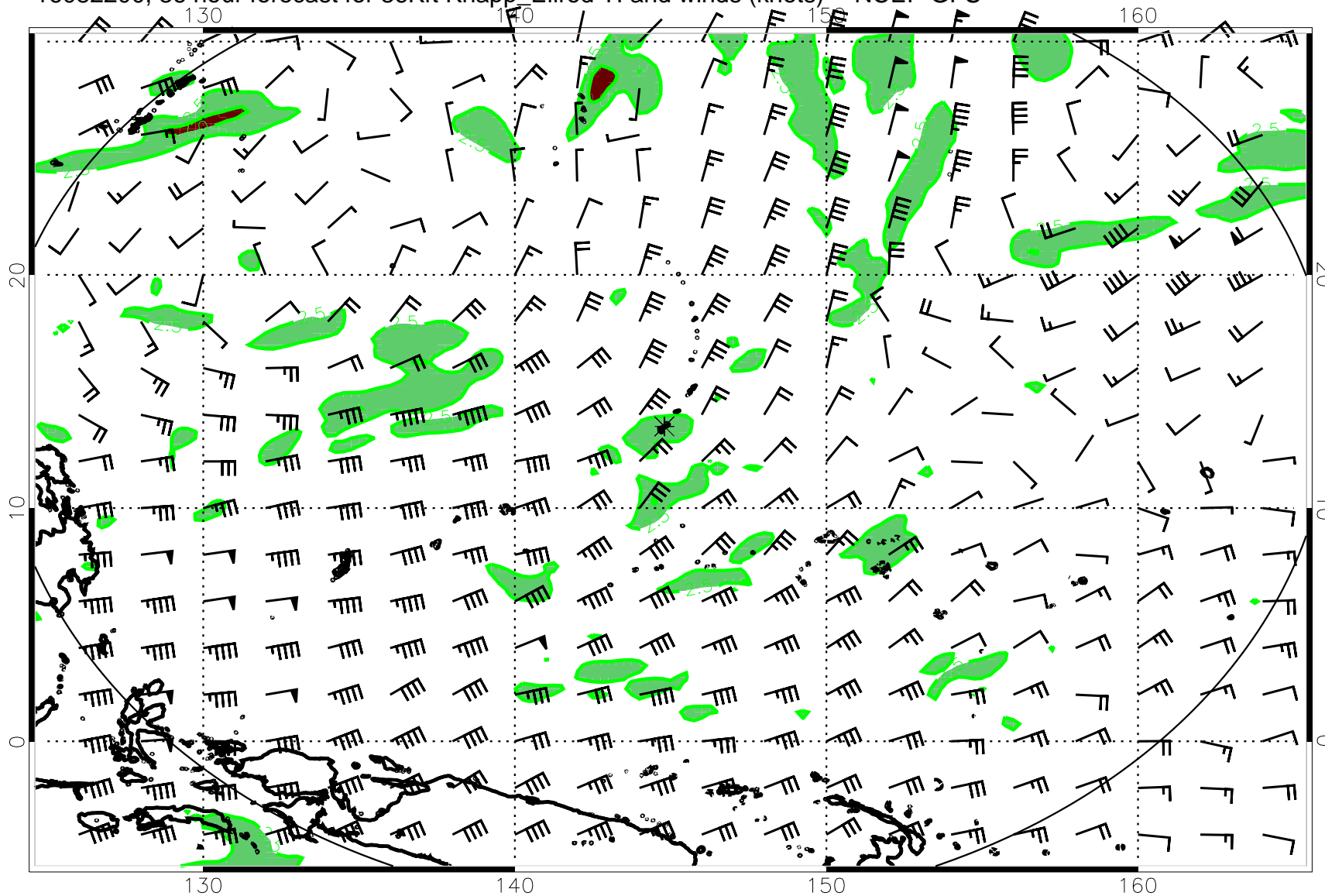
16082200, 36 hour forecast for 36Kft Knapp_Ellrod TI and winds (knots) -- NCEP GFS
