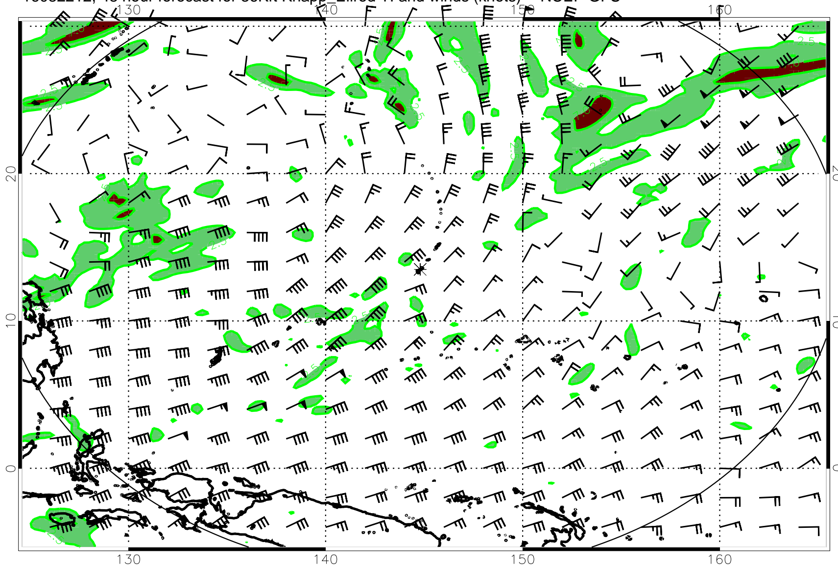
16082212, 48 hour forecast for 36Kft Knapp Ellrod TI and winds (knots) -- NCEP GFS
