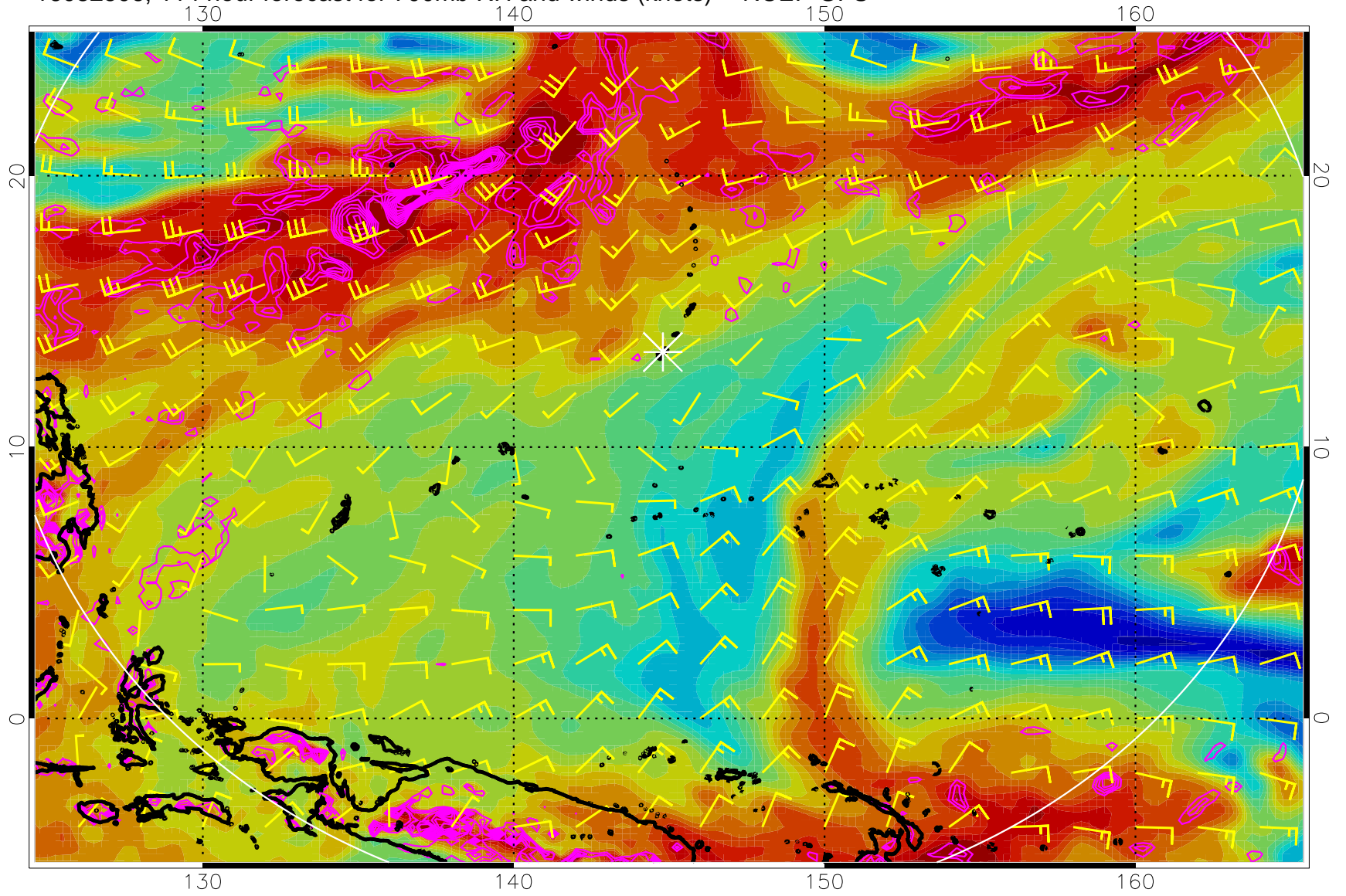
16082506, 114 hour forecast for 700mb RH and winds (knots) -- NCEP GFS
