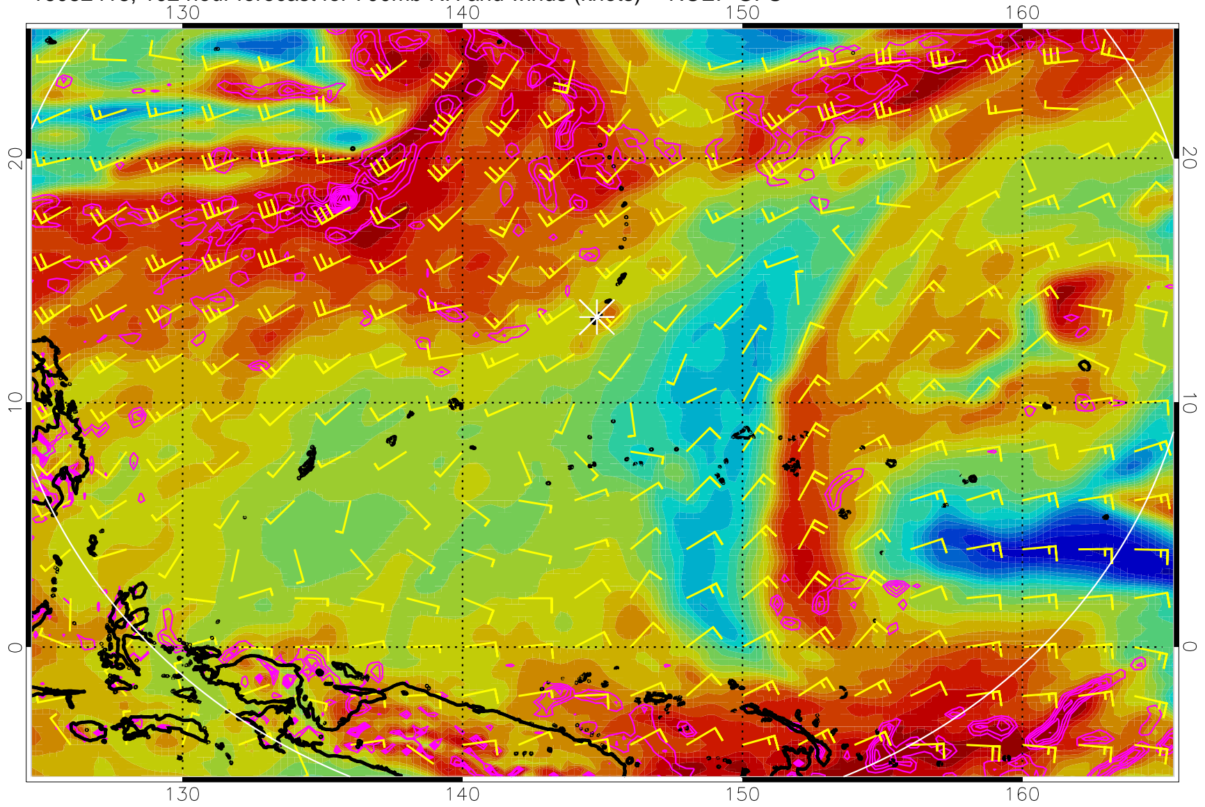
16082418, 102 hour forecast for 700mb RH and winds (knots) -- NCEP GFS
