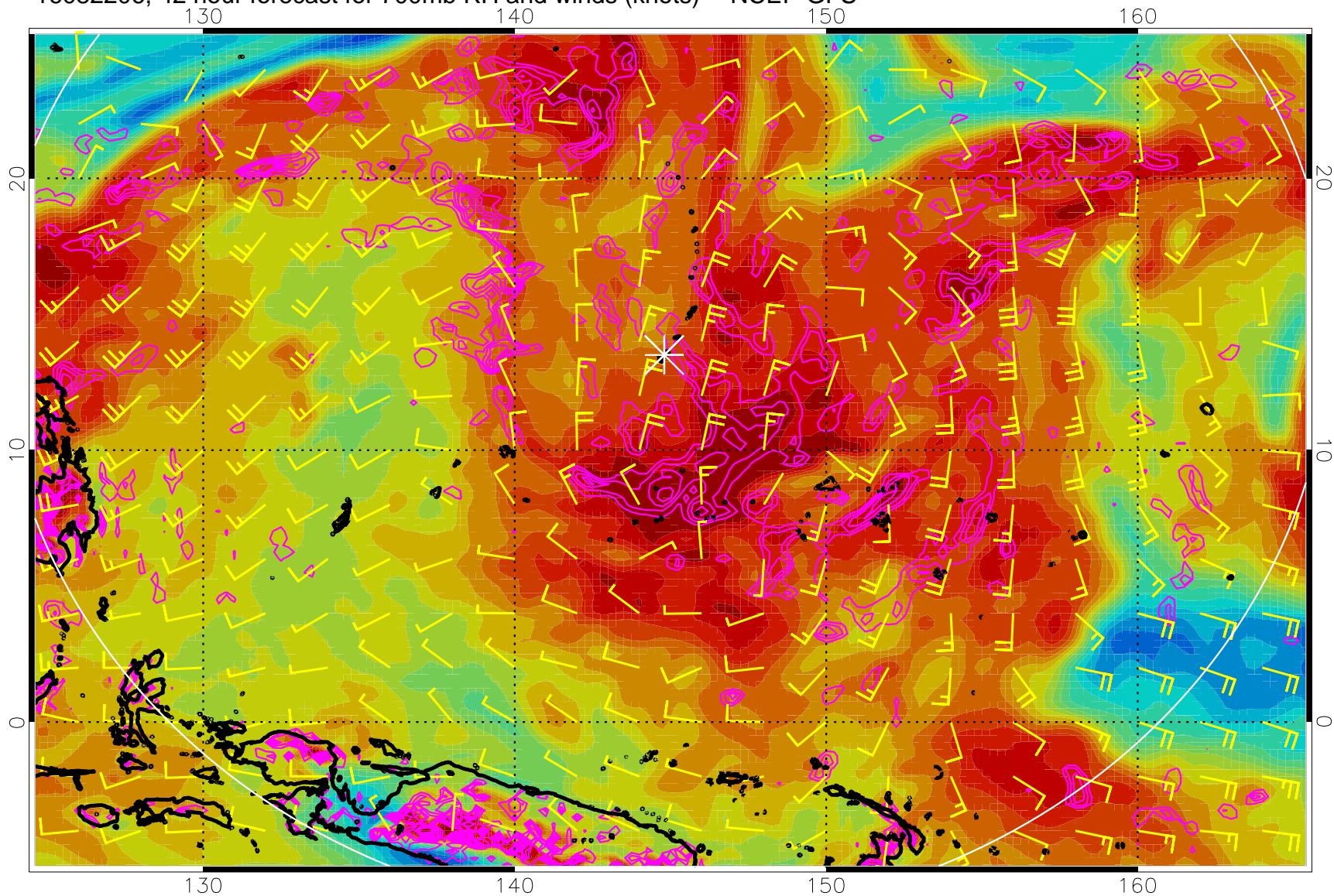
16082206, 42 hour forecast for 700mb RH and winds (knots) -- NCEP GFS
