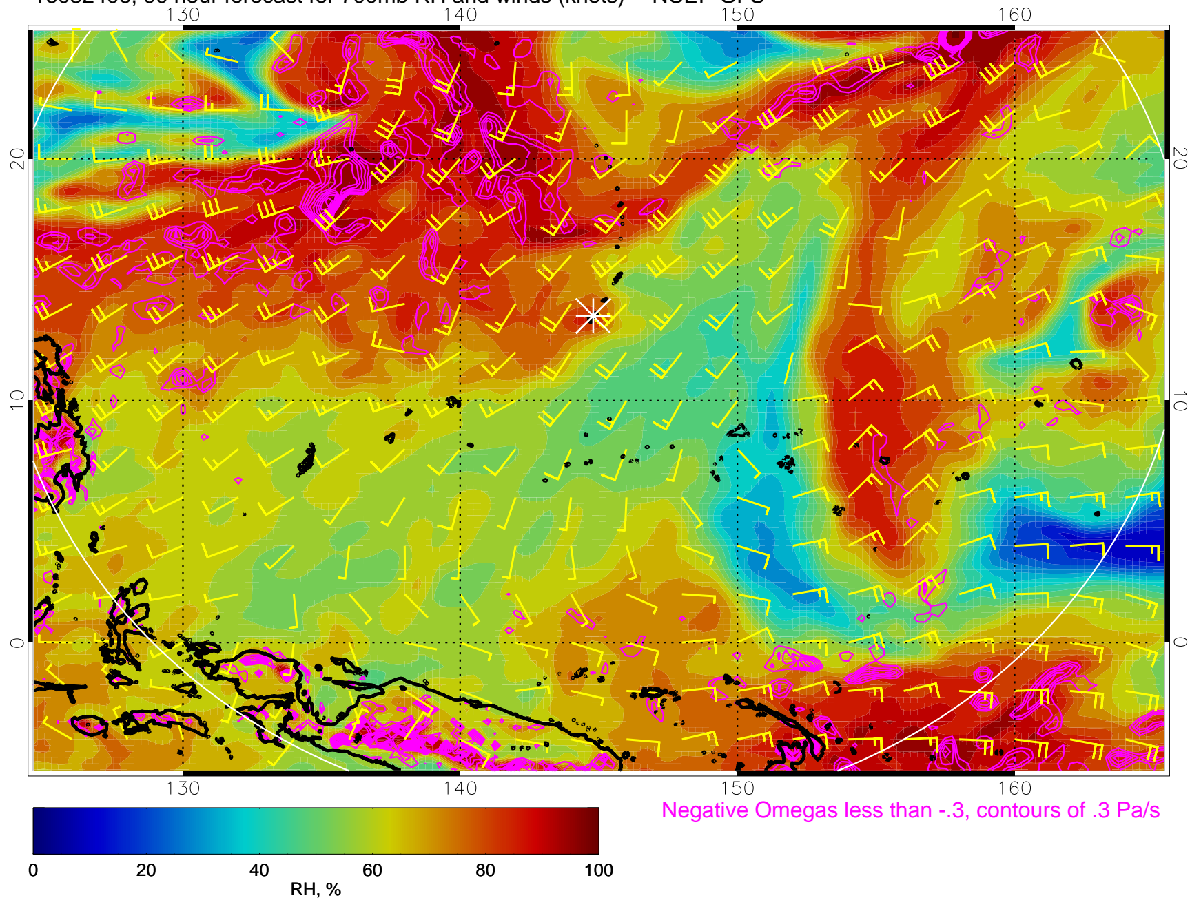
16082406, 90 hour forecast for 700mb RH and winds (knots) -- NCEP GFS
