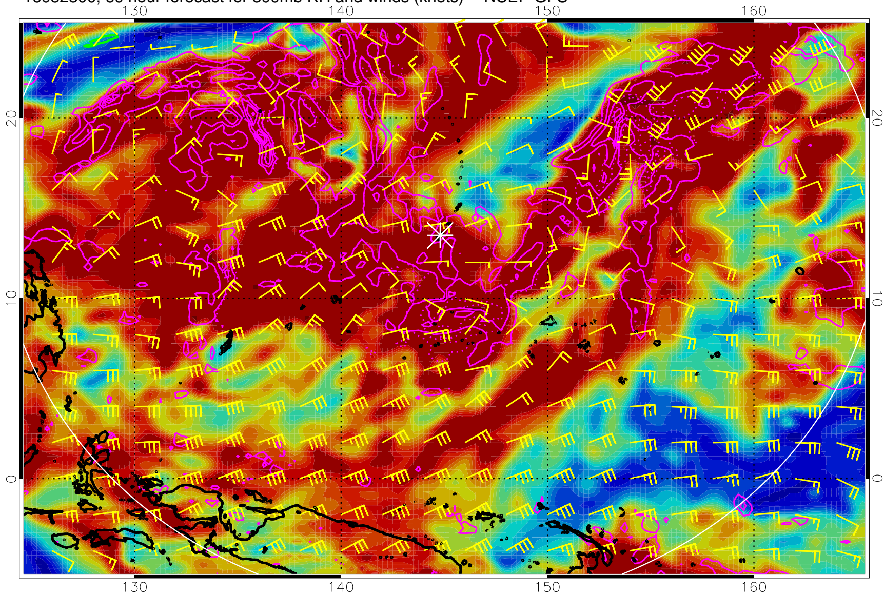
16082300, 60 hour forecast for 300mb RH and winds (knots) -- NCEP GFS
