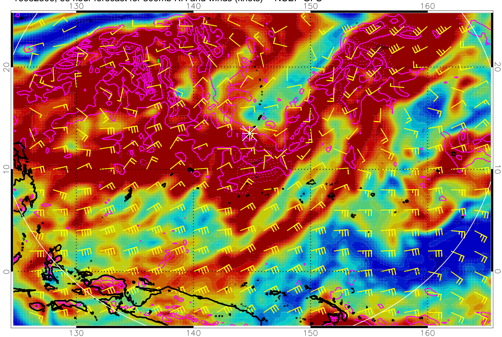
16082306, 66 hour forecast for 300mb RH and winds (knots) -- NCEP GFS
