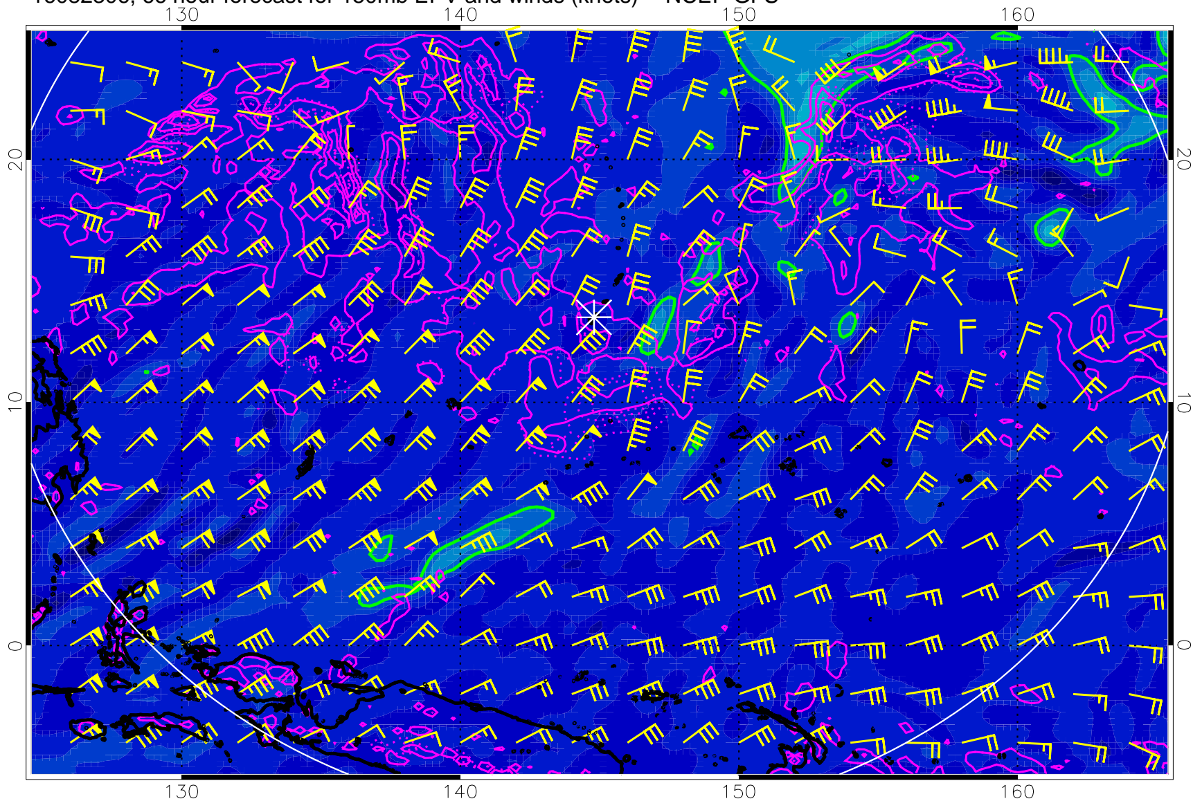
16082306, 66 hour forecast for 150mb EPV and winds (knots) -- NCEP GFS
