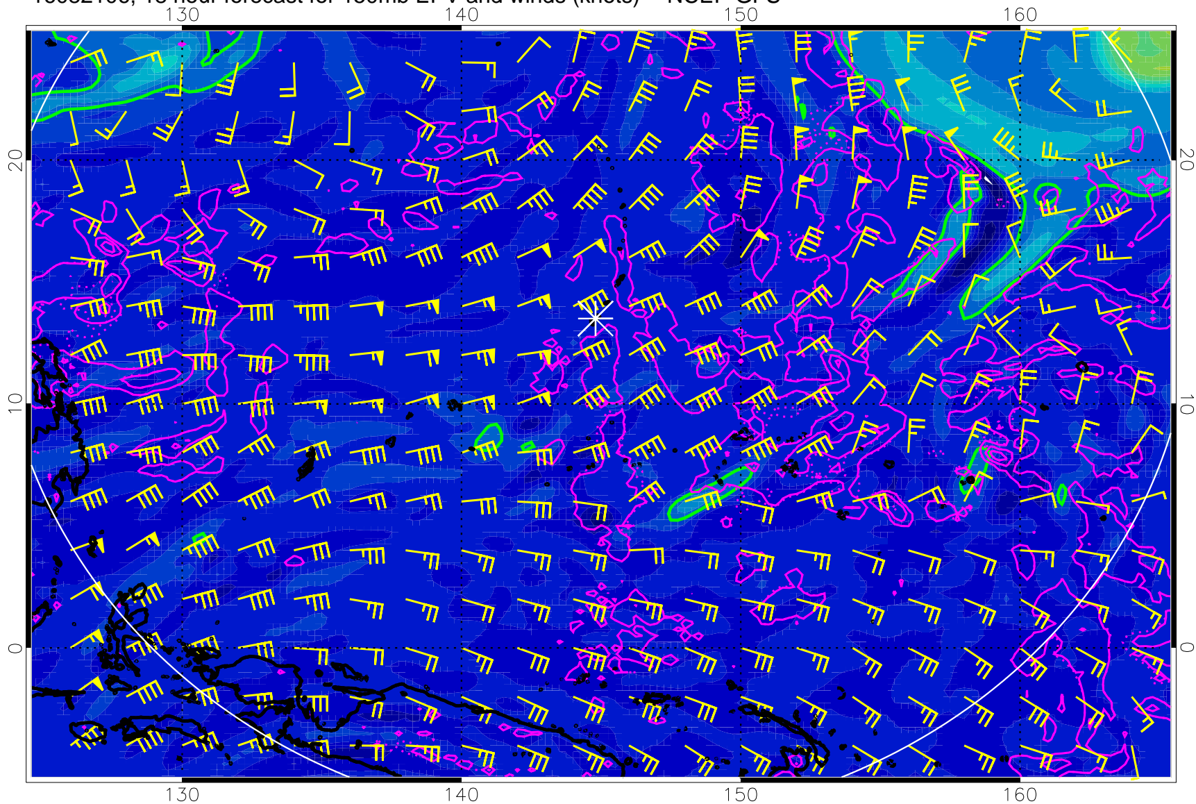
16082106, 18 hour forecast for 150mb EPV and winds (knots) -- NCEP GFS
