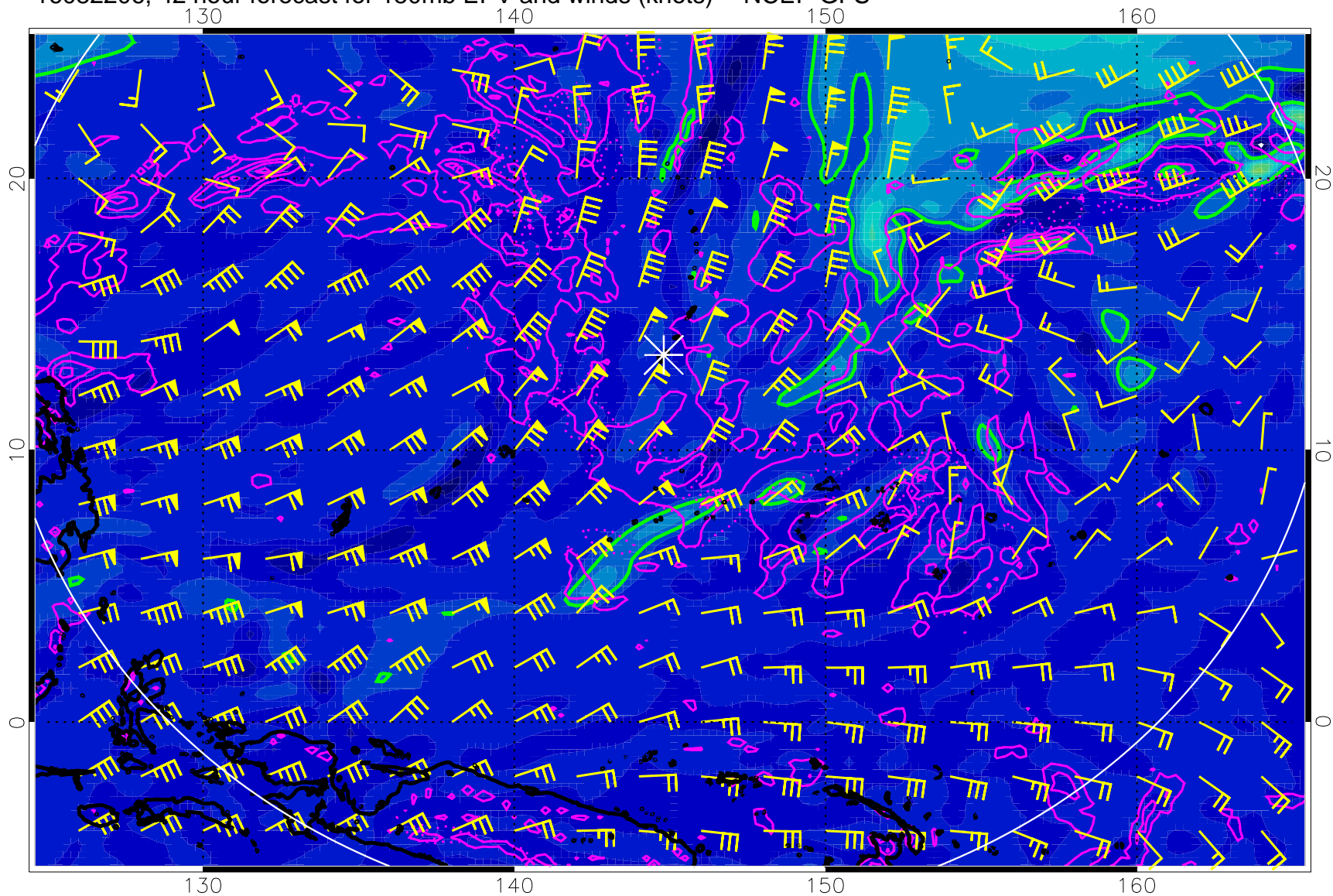
16082206, 42 hour forecast for 150mb EPV and winds (knots) -- NCEP GFS
