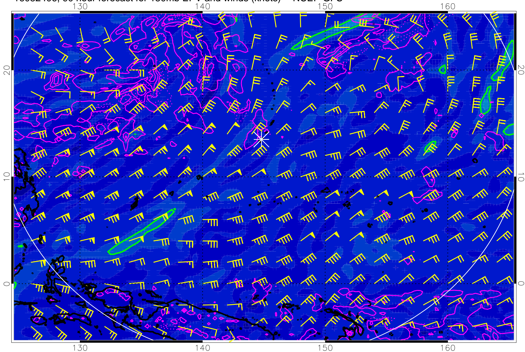
16082406, 90 hour forecast for 150mb EPV and winds (knots) -- NCEP GFS
