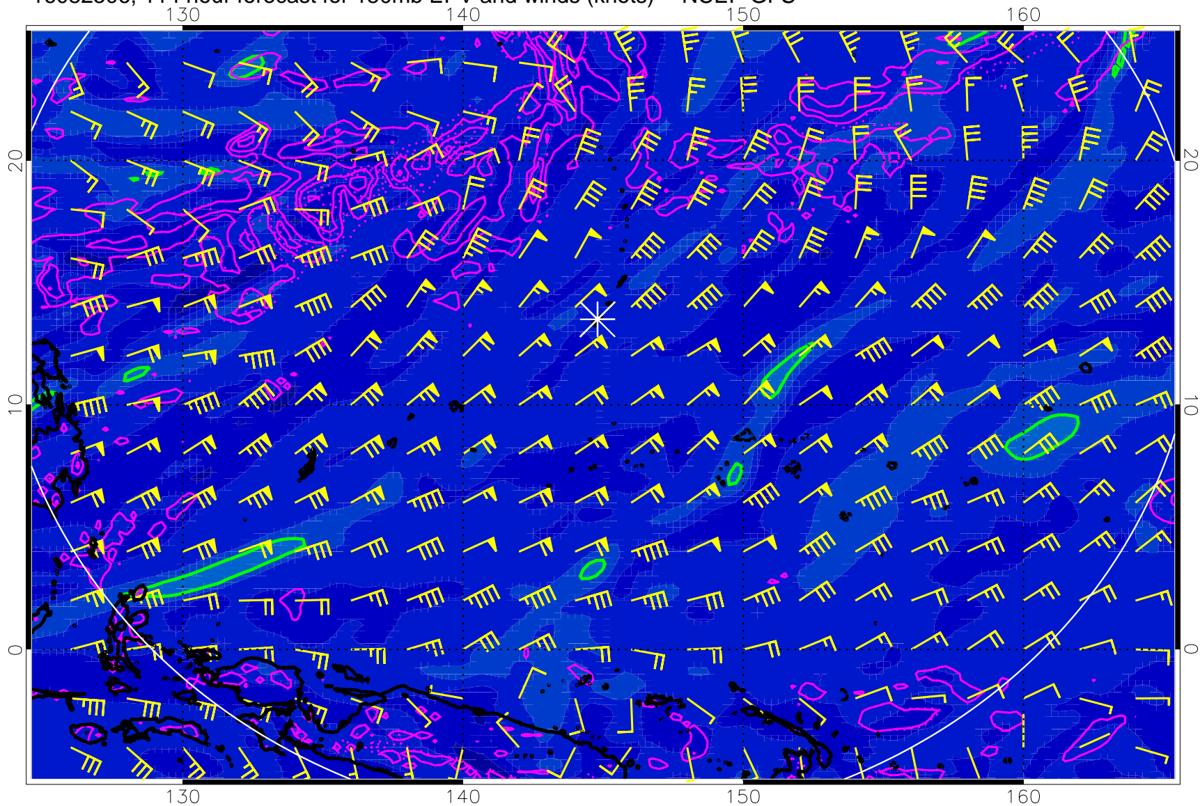
16082506, 114 hour forecast for 150mb EPV and winds (knots) -- NCEP GFS
