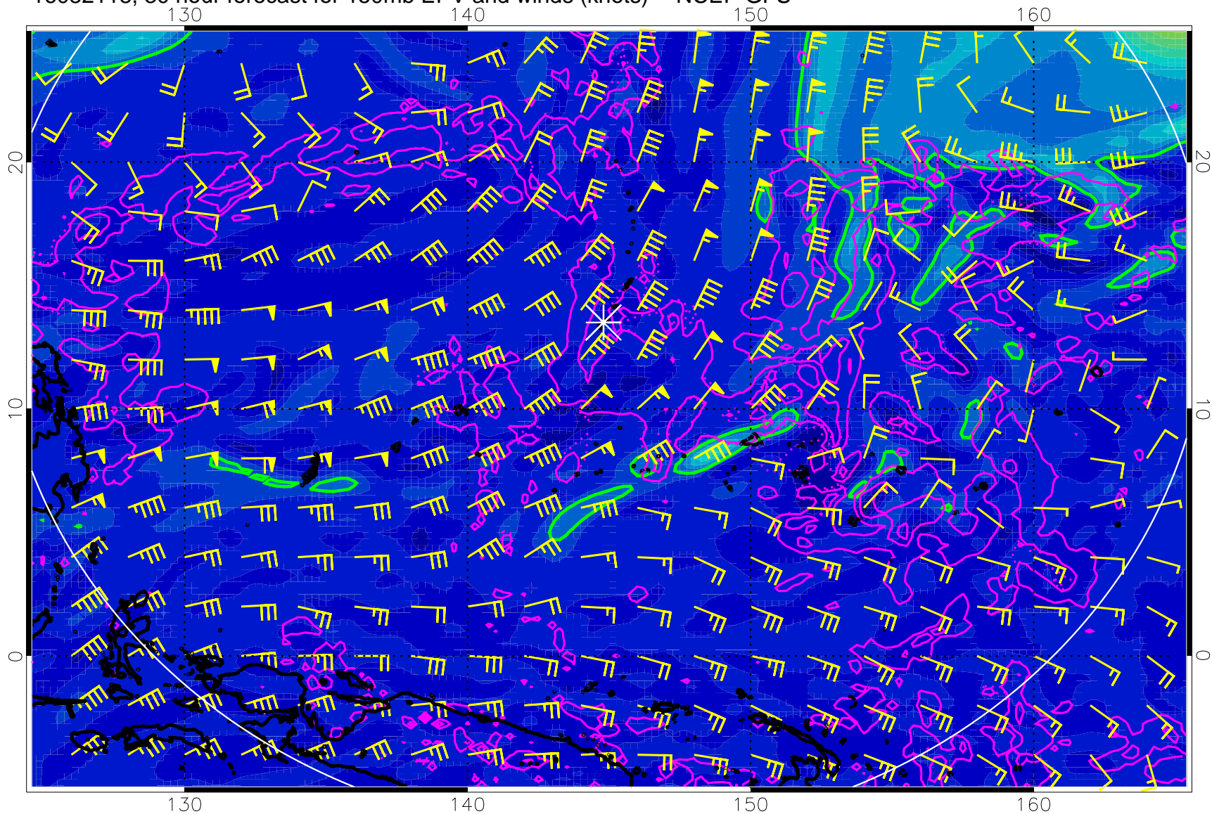
16082118, 30 hour forecast for 150mb EPV and winds (knots) -- NCEP GFS
