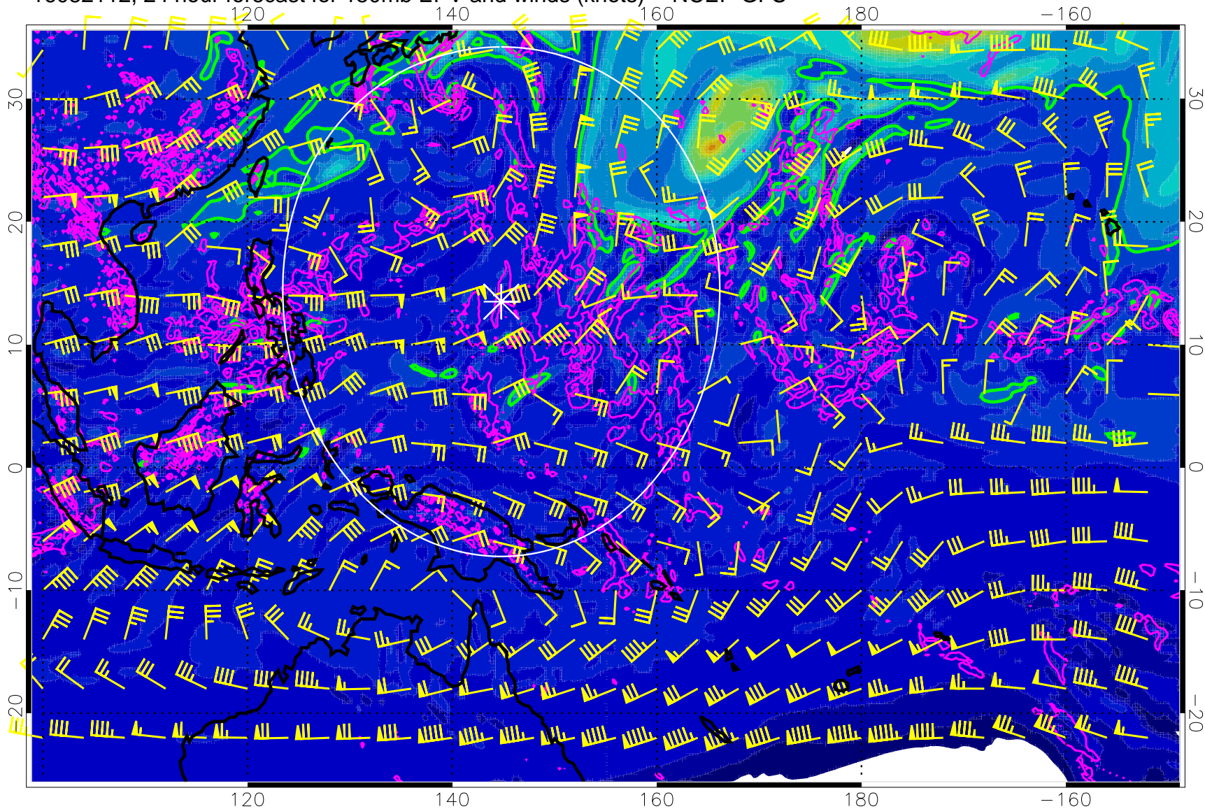
16082112, 24 hour forecast for 150mb EPV and winds (knots) -- NCEP GFS
