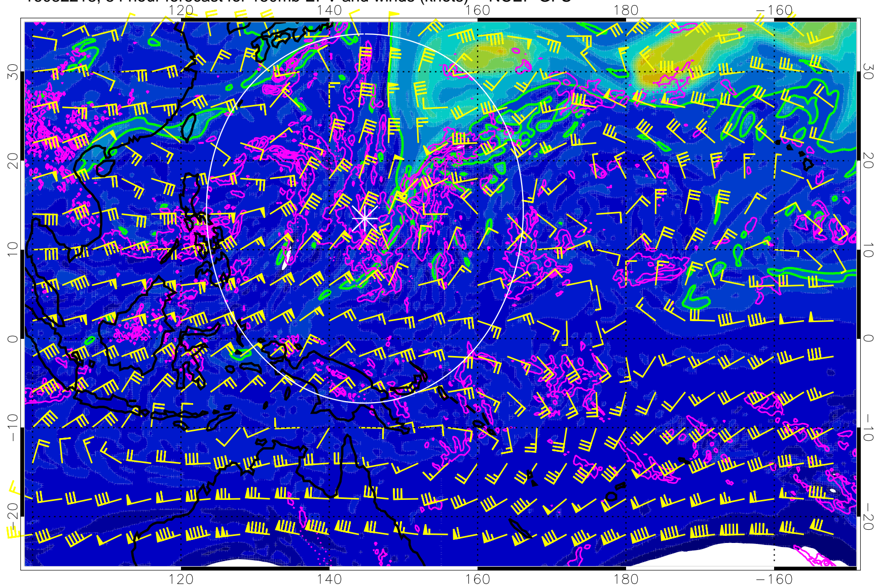
16082218, 54 hour forecast for 150mb EPV and winds (knots) -- NCEP GFS
