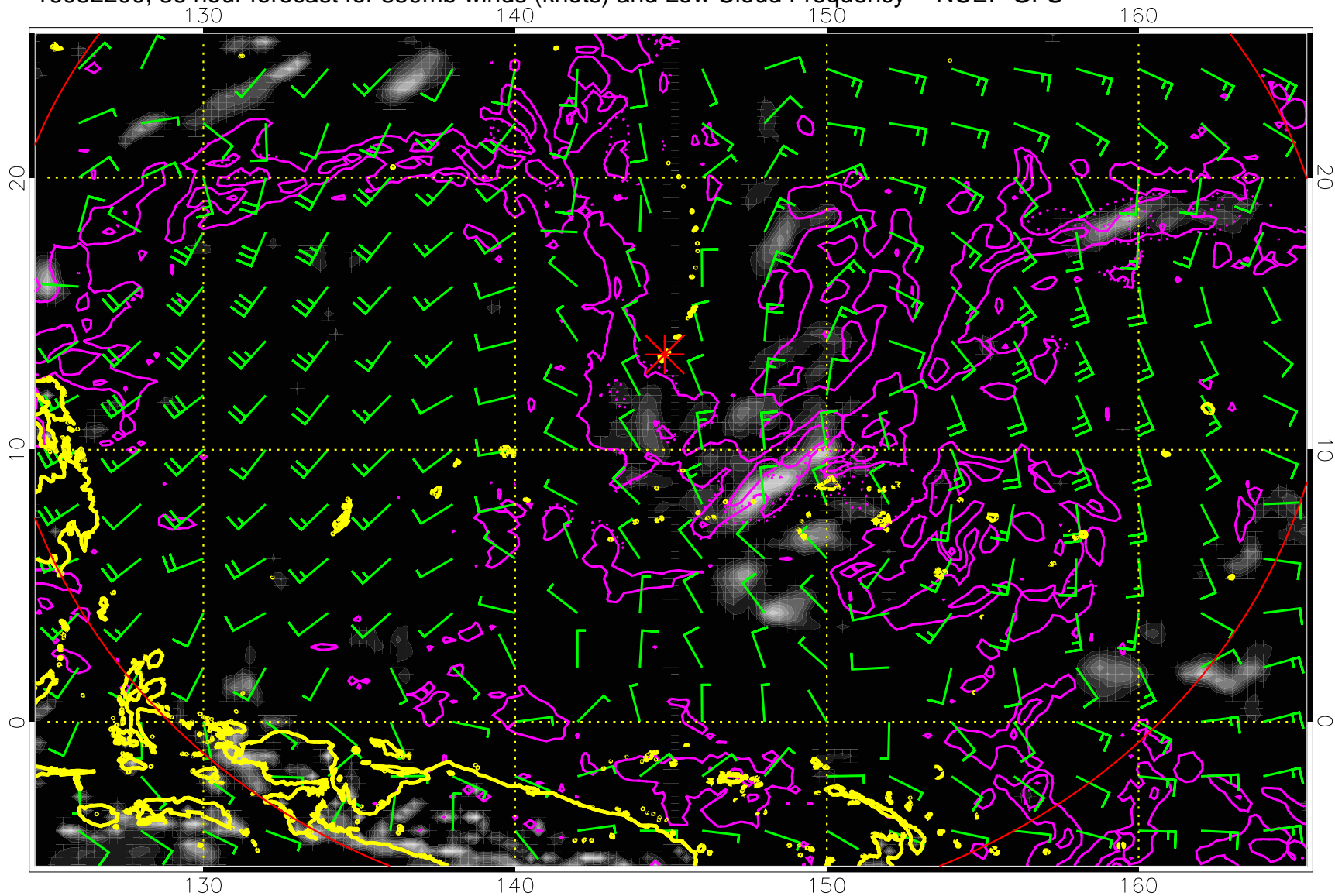
16082200, 36 hour forecast for 850mb winds (knots) and Low Cloud Frequency -- NCEP GFS
