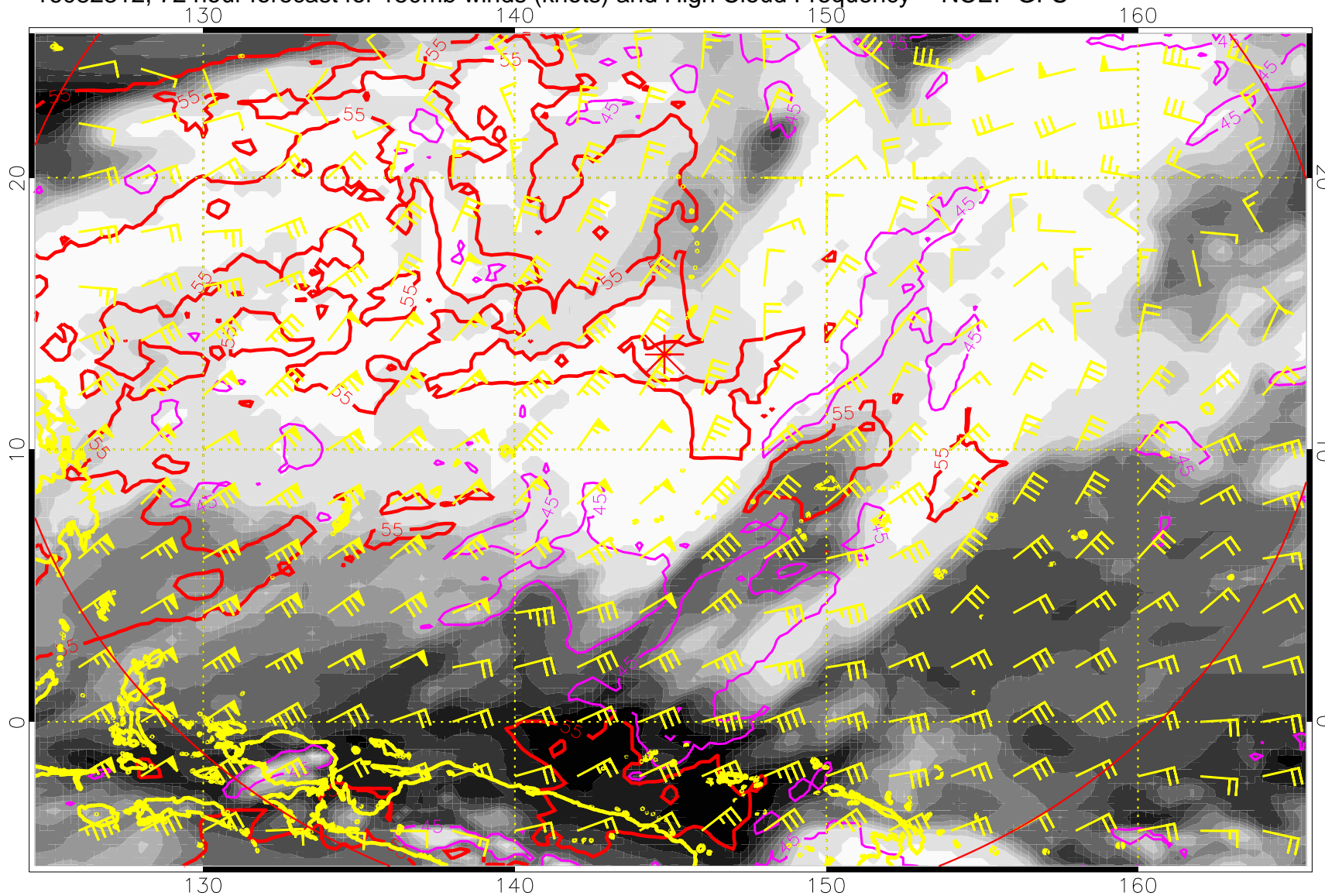
16082312, 72 hour forecast for 150mb winds (knots) and High Cloud Frequency -- NCEP GFS
