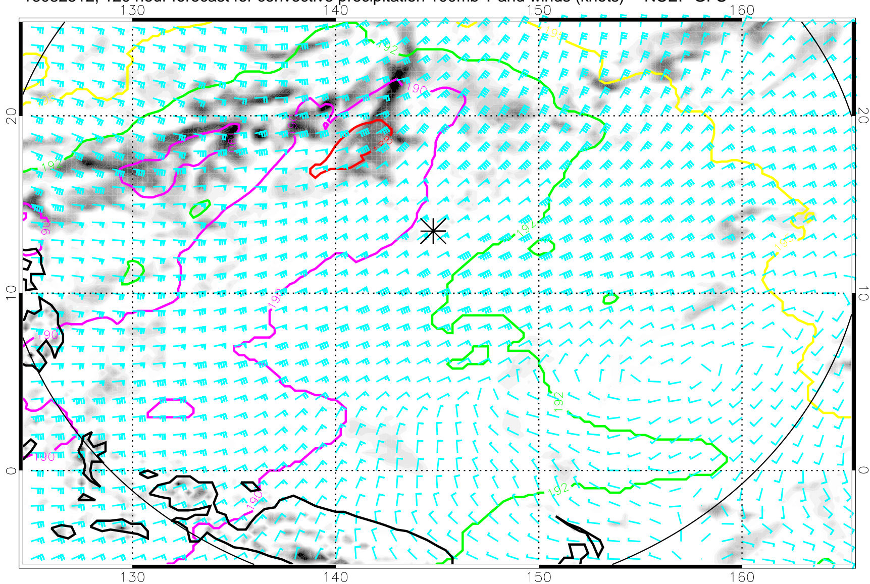
16082512, 120 hour forecast for convective precipitation 100mb T and winds (knots) -- NCEP GFS
