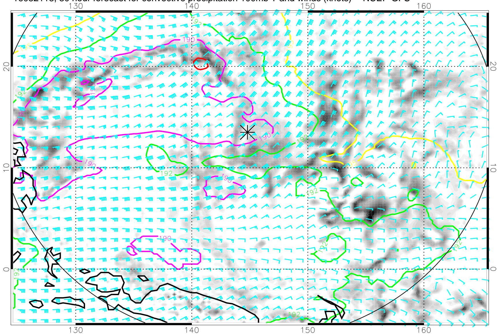
16082118, 30 hour forecast for convective precipitation 100mb T and winds (knots) -- NCEP GFS
