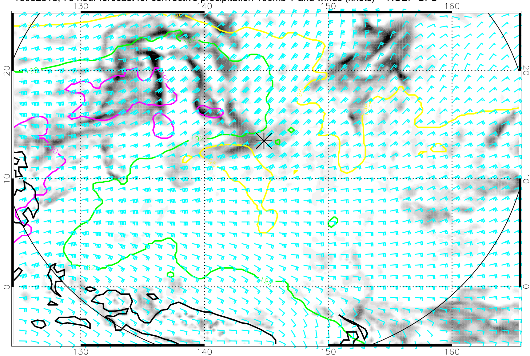
16082318, 78 hour forecast for convective precipitation 100mb T and winds (knots) -- NCEP GFS
