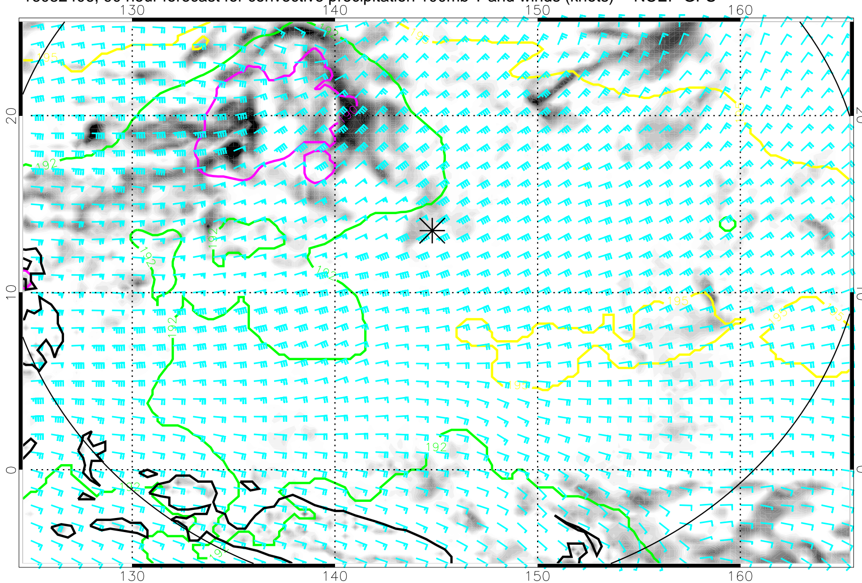
16082406, 90 hour forecast for convective precipitation 100mb T and winds (knots) -- NCEP GFS
