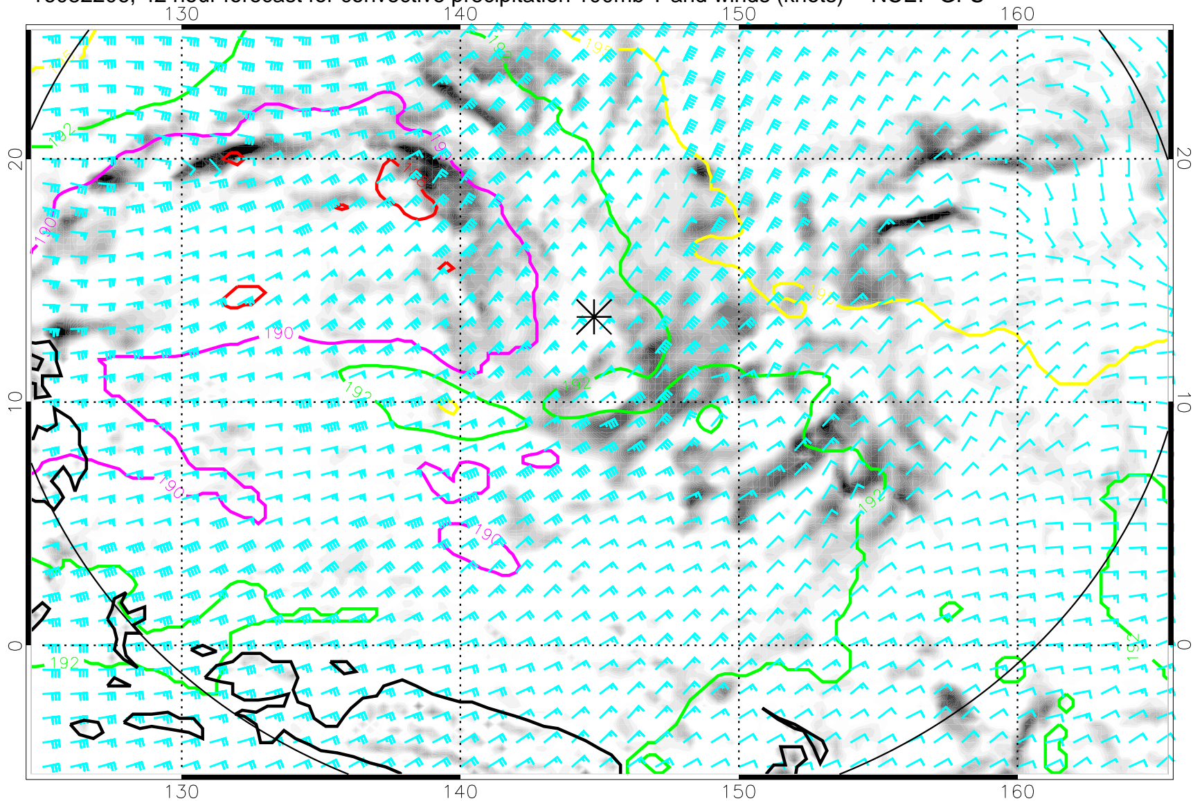
16082206, 42 hour forecast for convective precipitation 100mb T and winds (knots) -- NCEP GFS
