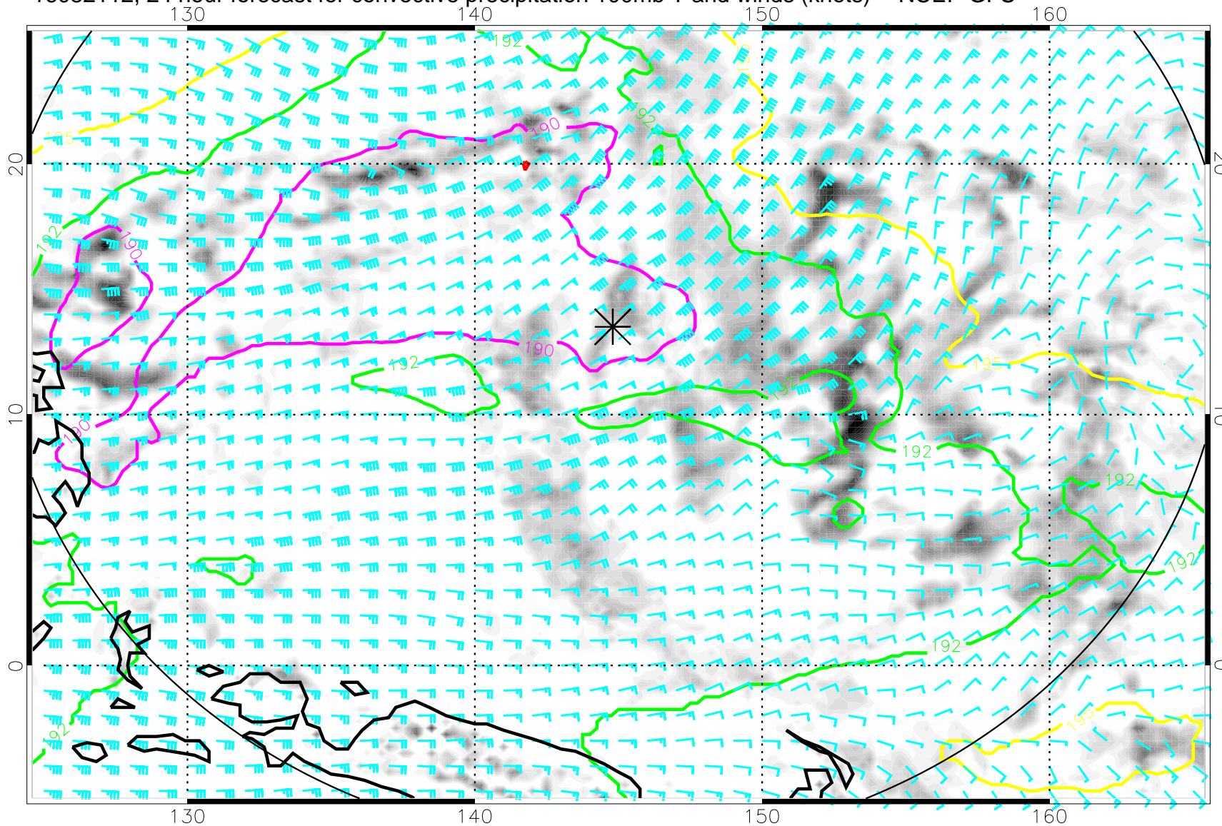
16082112, 24 hour forecast for convective precipitation 100mb T and winds (knots) -- NCEP GFS
