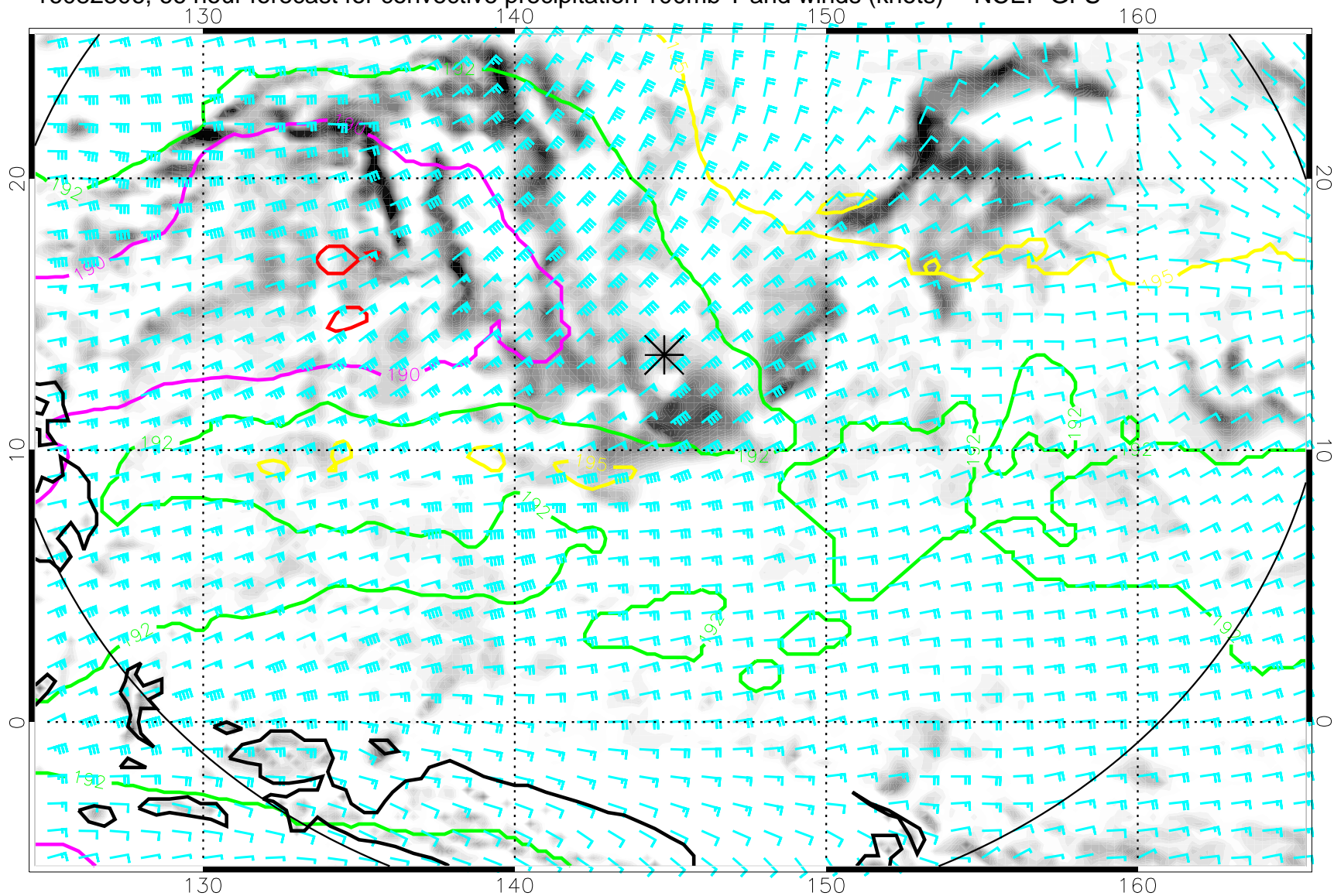
16082306, 66 hour forecast for convective precipitation 100mb T and winds (knots) -- NCEP GFS
