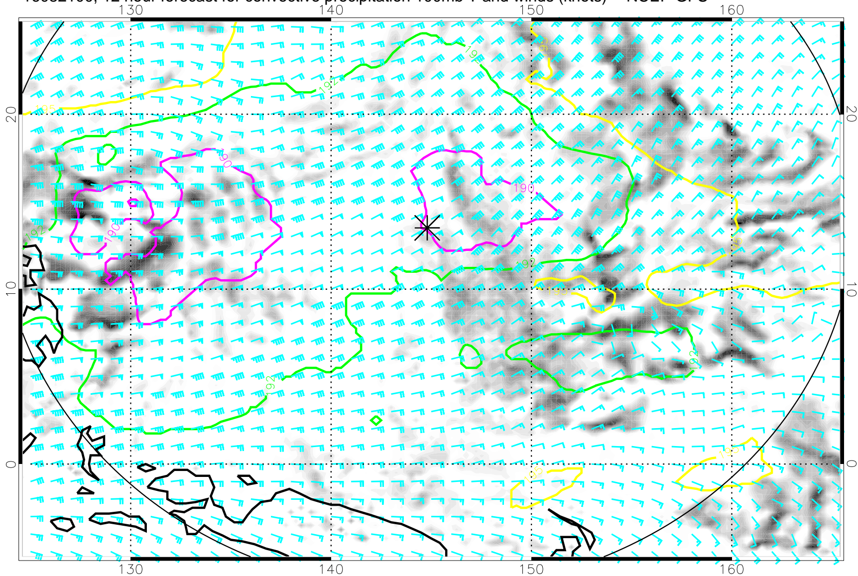
16082100, 12 hour forecast for convective precipitation 100mb T and winds (knots) -- NCEP GFS
