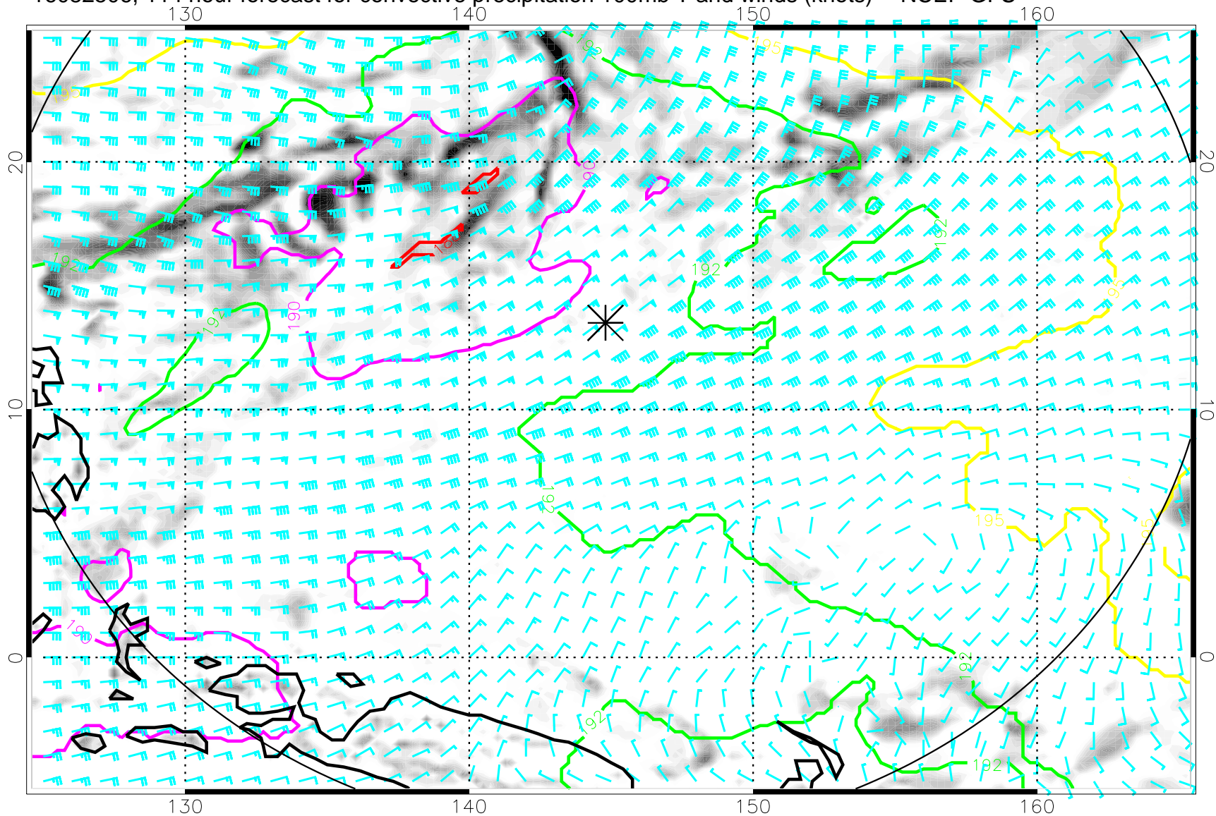
16082506, 114 hour forecast for convective precipitation 100mb T and winds (knots) -- NCEP GFS
