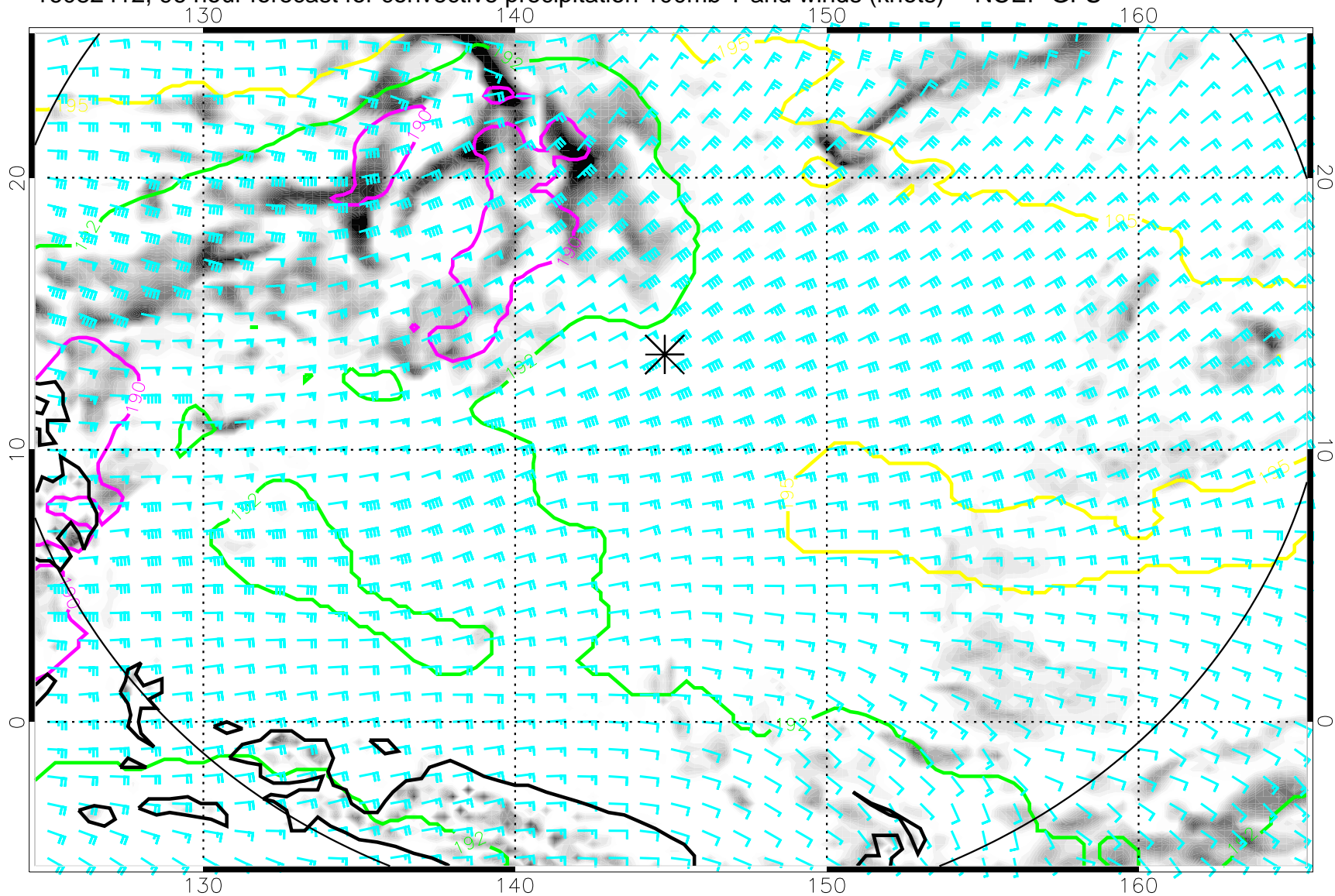
16082412, 96 hour forecast for convective precipitation 100mb T and winds (knots) -- NCEP GFS
