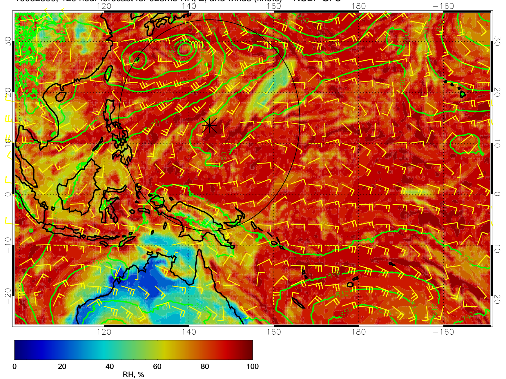
16082500, 120 hour forecast for 925mb RH, Z, and winds (knots) -- NCEP GFS
