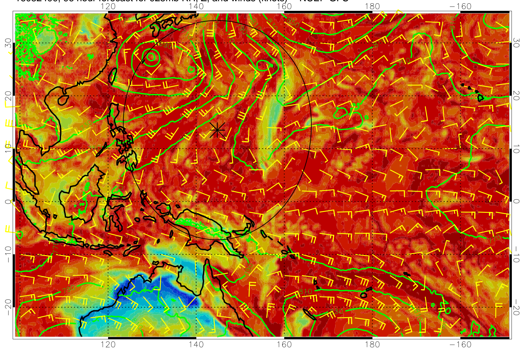
16082400, 96 hour forecast for 925mb RH, Z, and winds (knots) -- NCEP GFS
