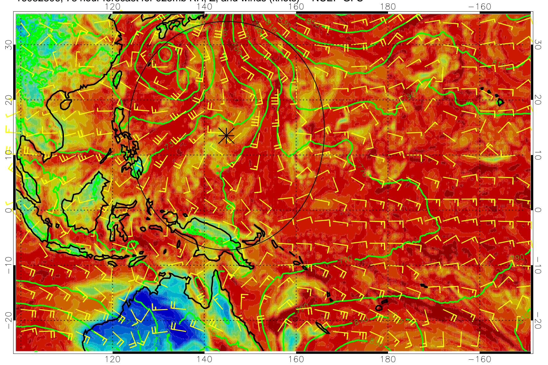
16082306, 78 hour forecast for 925mb RH, Z, and winds (knots) -- NCEP GFS
