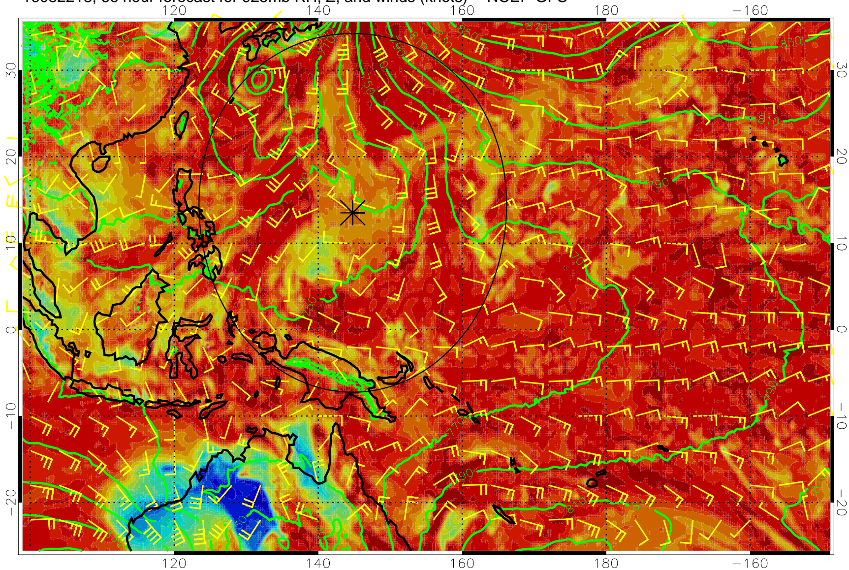
16082218, 66 hour forecast for 925mb RH, Z, and winds (knots) -- NCEP GFS
