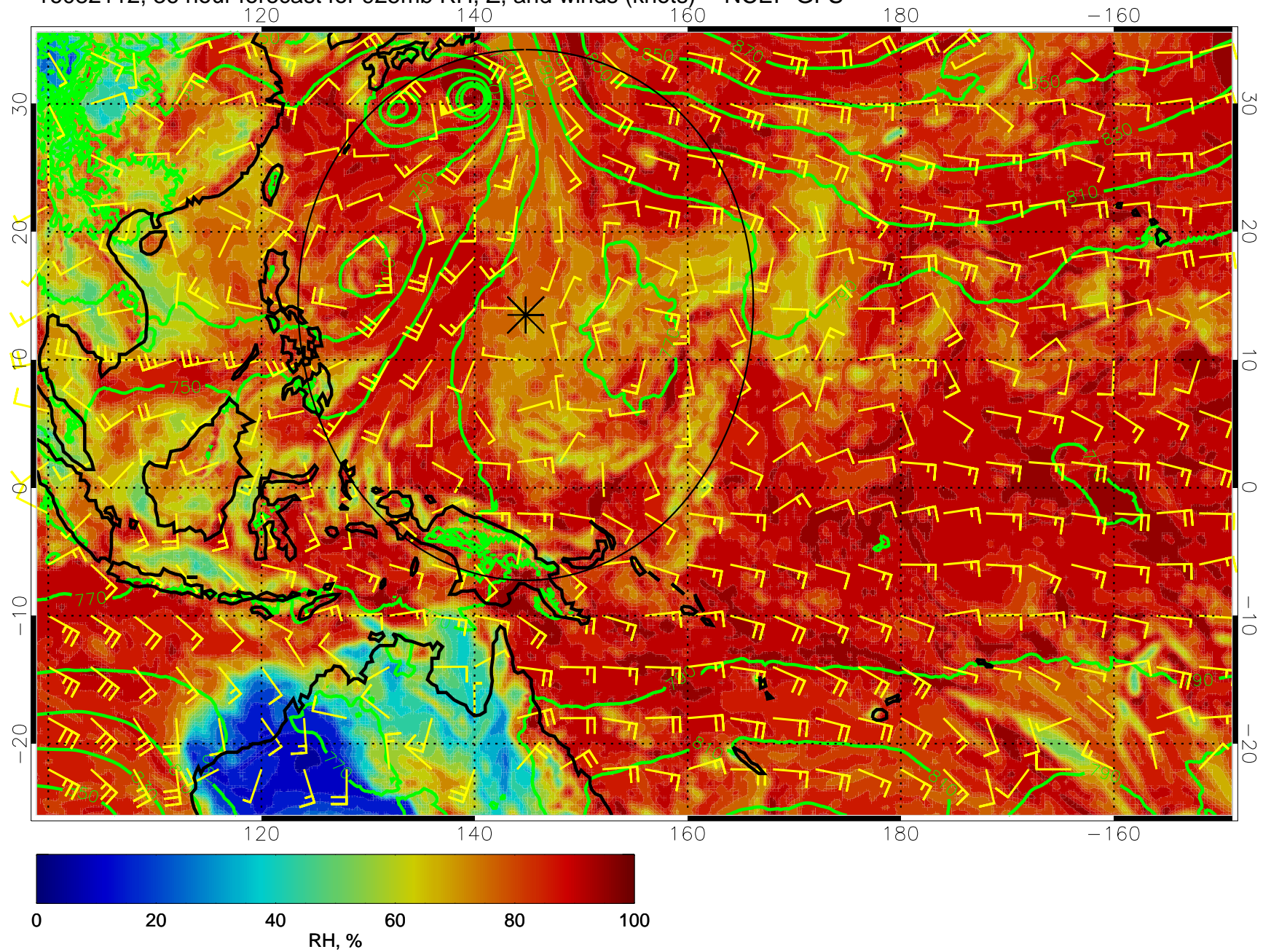
16082112, 36 hour forecast for 925mb RH, Z, and winds (knots) -- NCEP GFS
