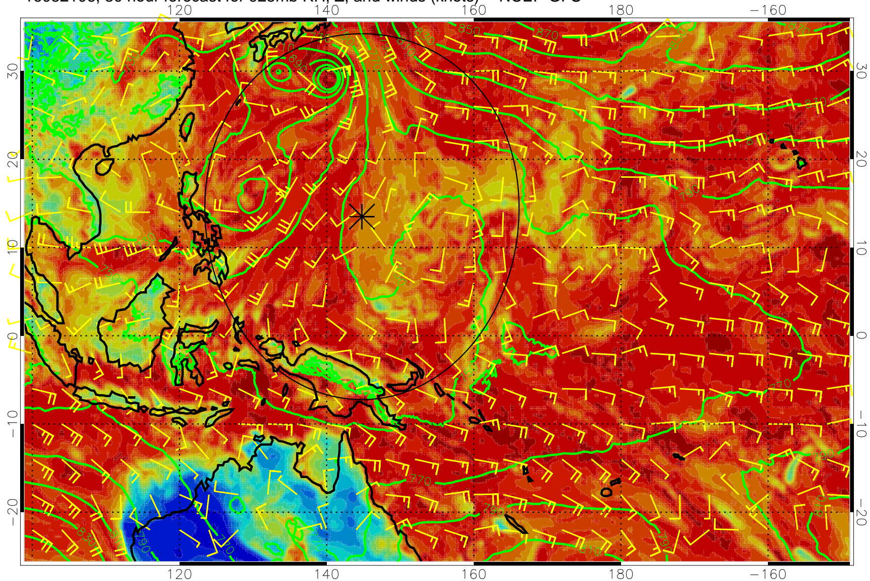
16082106, 30 hour forecast for 925mb RH, Z, and winds (knots) -- NCEP GFS
