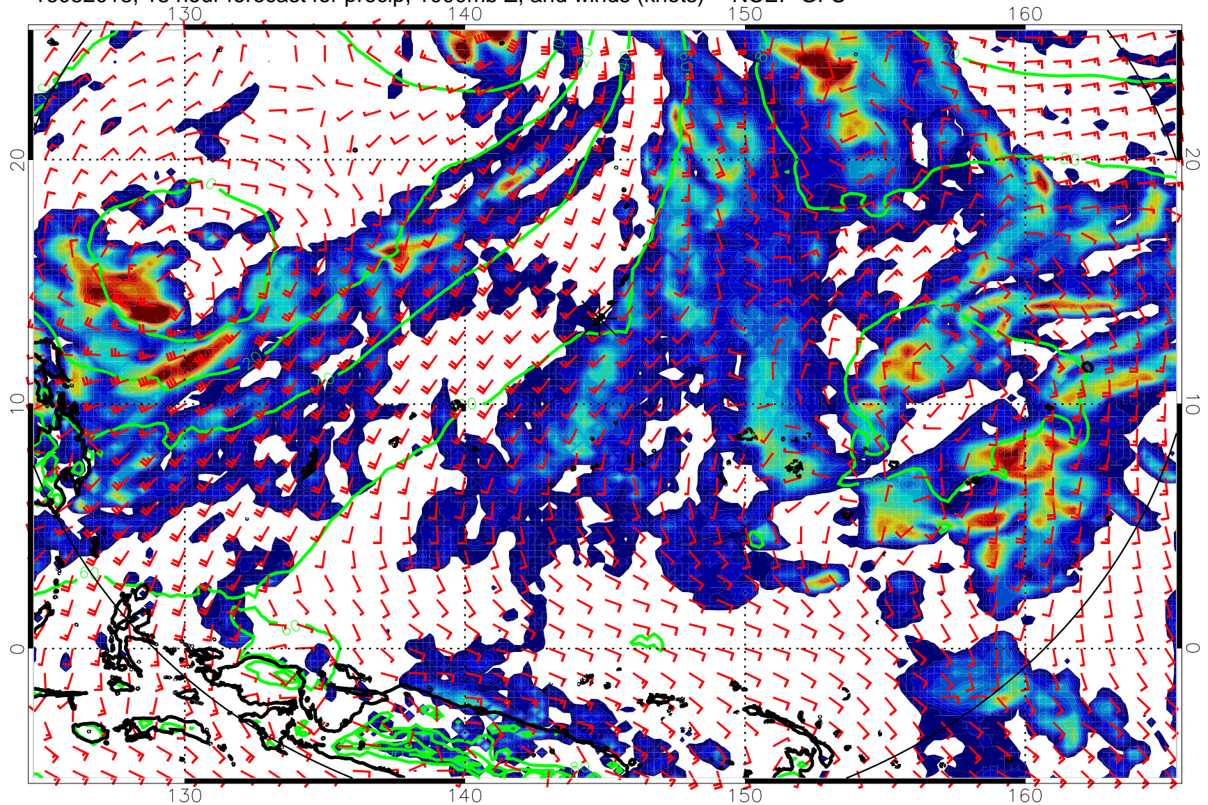
16082018, 18 hour forecast for precip, 1000mb Z, and winds (knots) -- NCEP GFS
