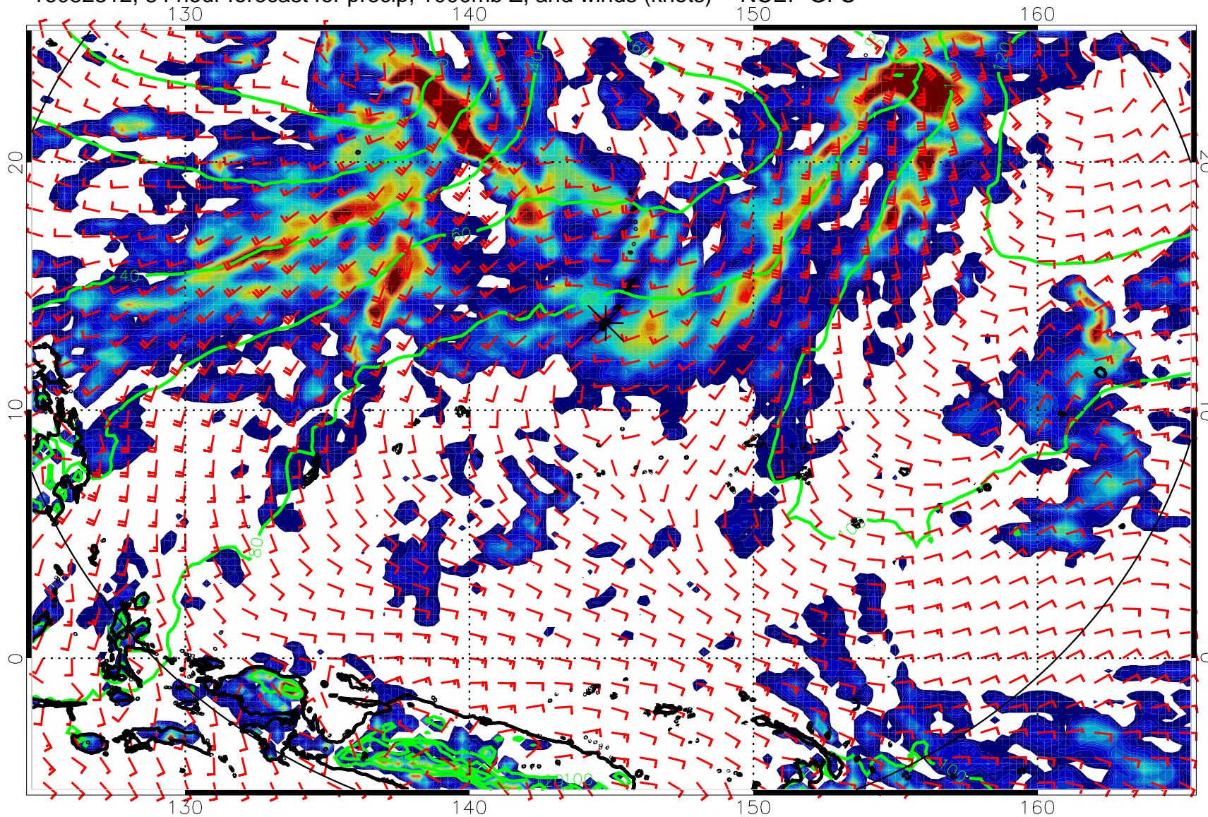
16082312, 84 hour forecast for precip, 1000mb Z, and winds (knots) -- NCEP GFS
