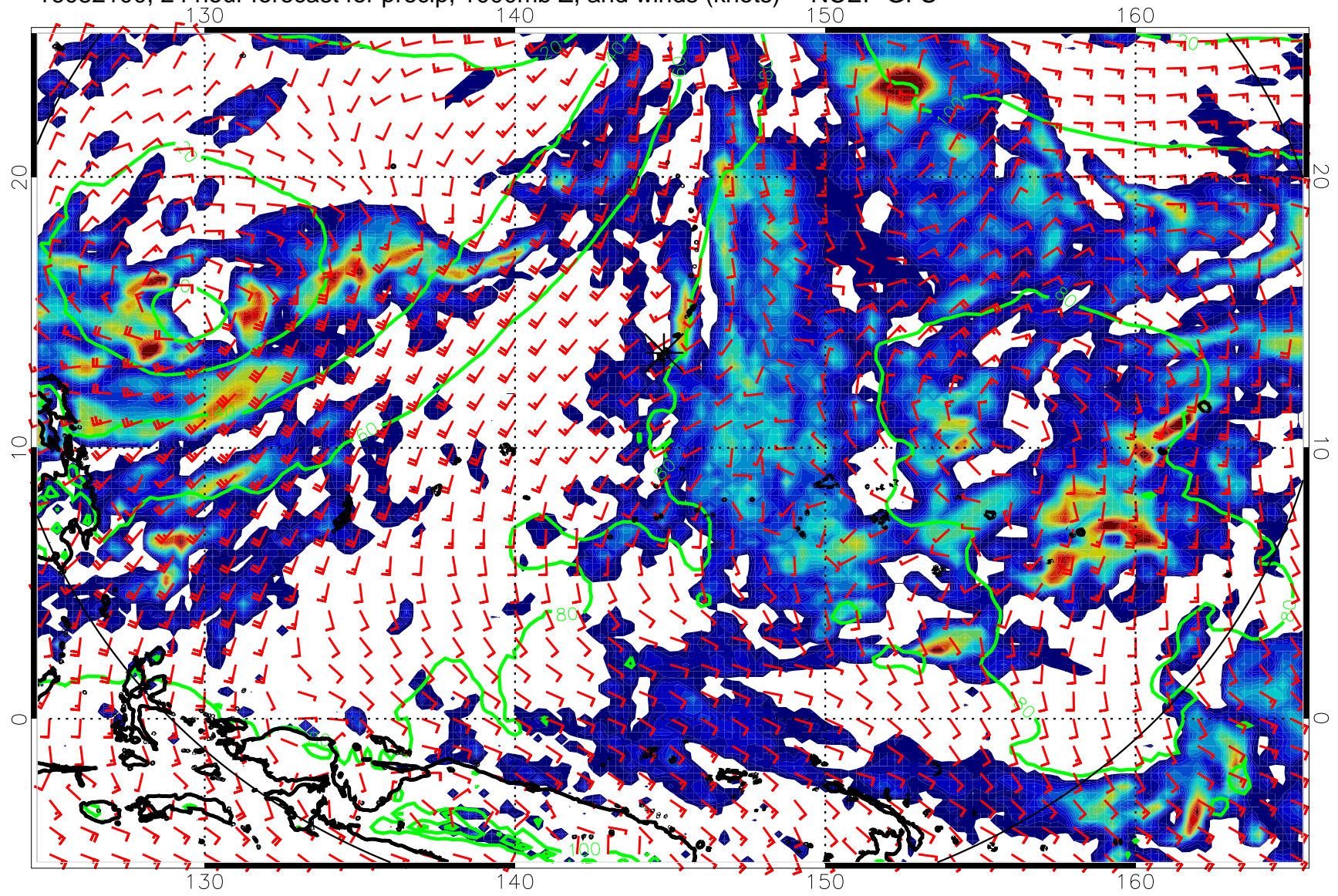
16082100, 24 hour forecast for precip, 1000mb Z, and winds (knots) -- NCEP GFS
