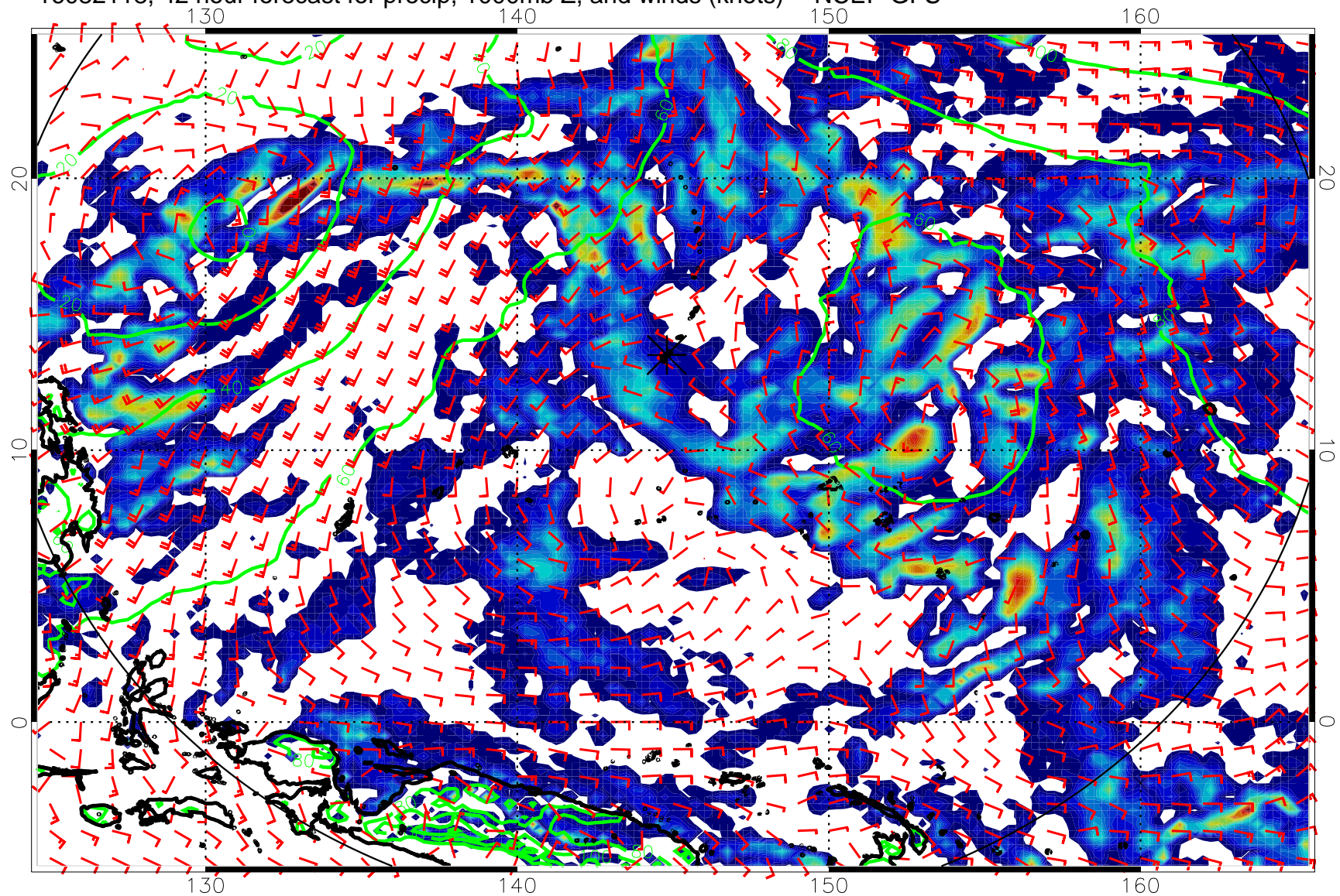
16082118, 42 hour forecast for precip, 1000mb Z, and winds (knots) -- NCEP GFS
