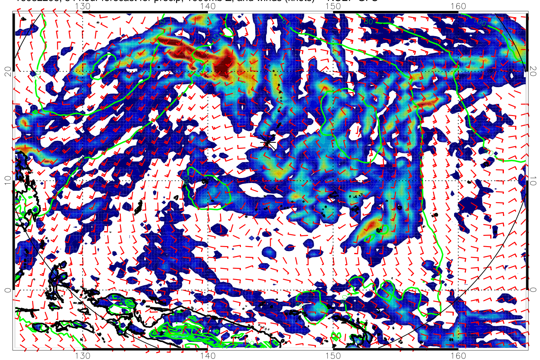
16082206, 54 hour forecast for precip, 1000mb Z, and winds (knots) -- NCEP GFS
