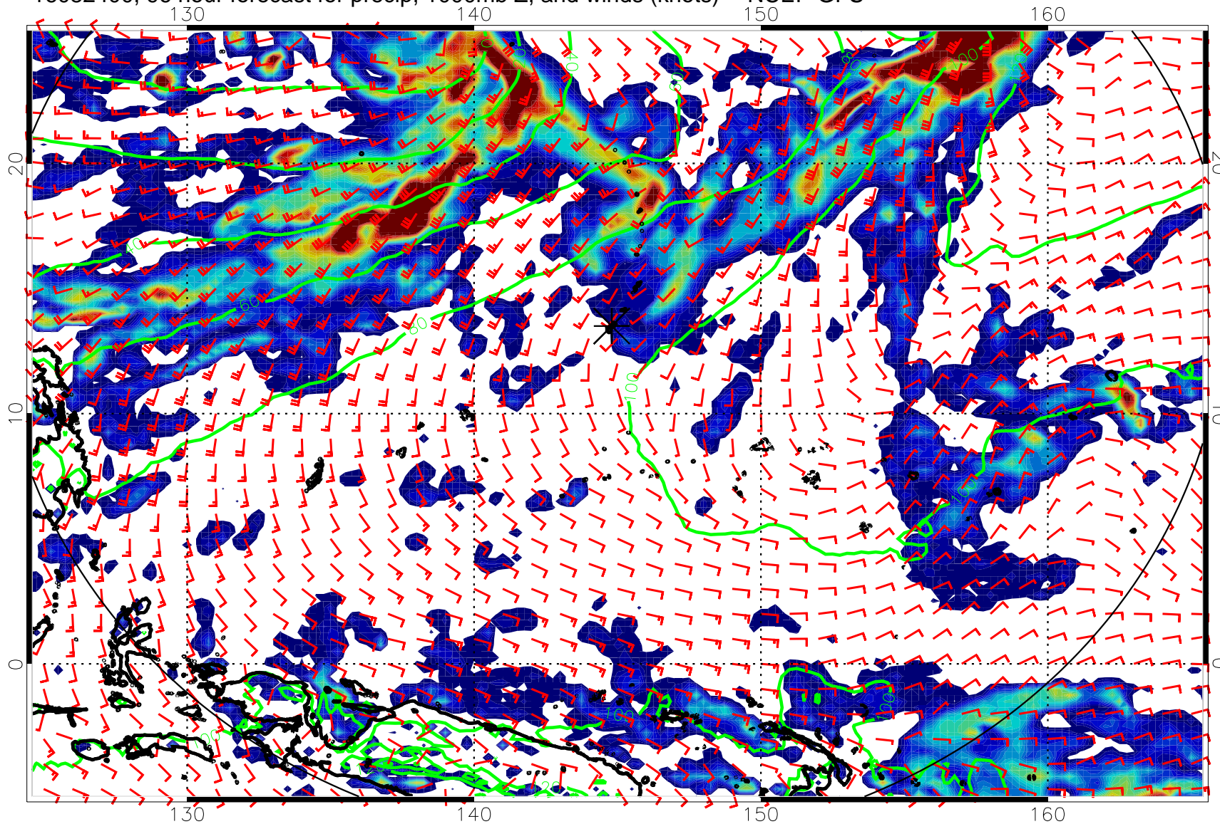
16082400, 96 hour forecast for precip, 1000mb Z, and winds (knots) -- NCEP GFS
