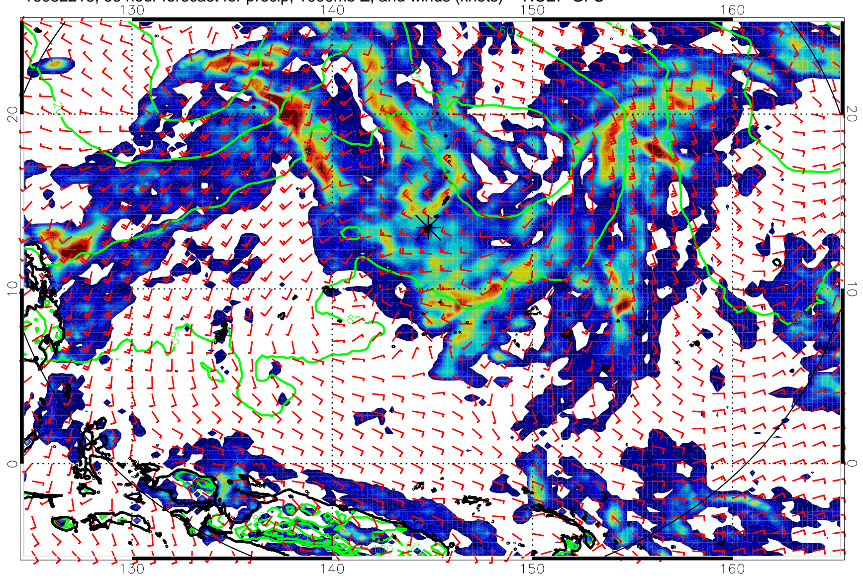
16082218, 66 hour forecast for precip, 1000mb Z, and winds (knots) -- NCEP GFS
