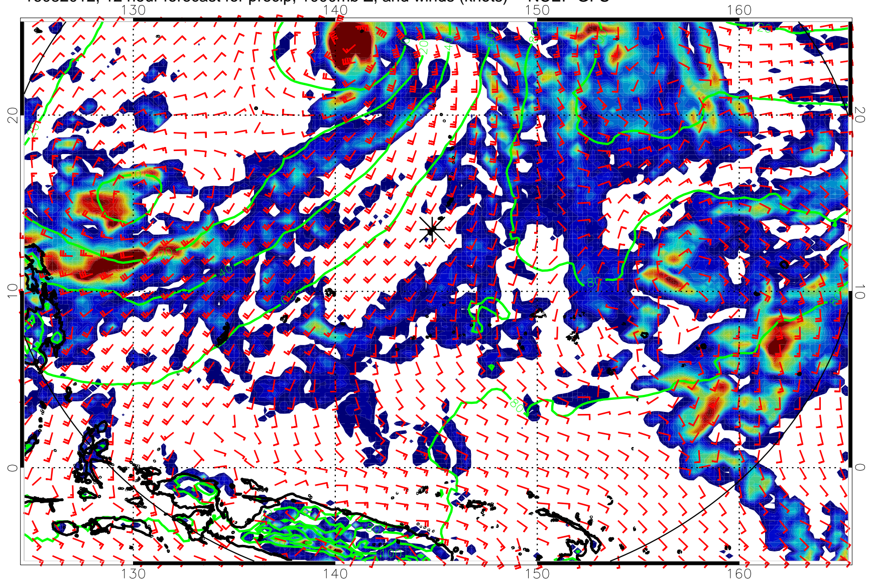
16082012, 12 hour forecast for precip, 1000mb Z, and winds (knots) -- NCEP GFS
