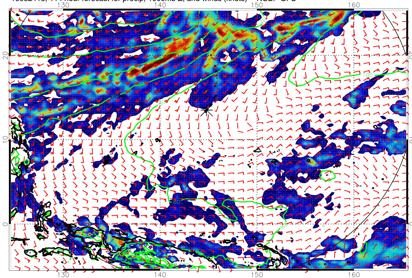
16082418, 114 hour forecast for precip, 1000mb Z, and winds (knots) -- NCEP GFS
