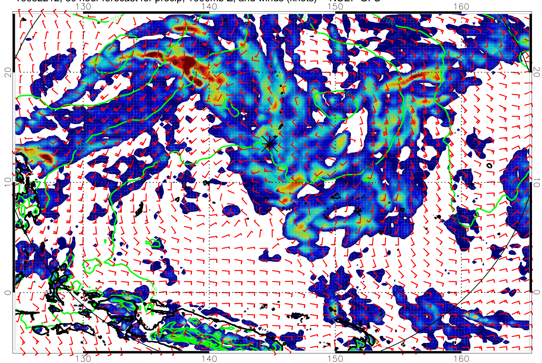
16082212, 60 hour forecast for precip, 1000mb Z, and winds (knots) -- NCEP GFS
