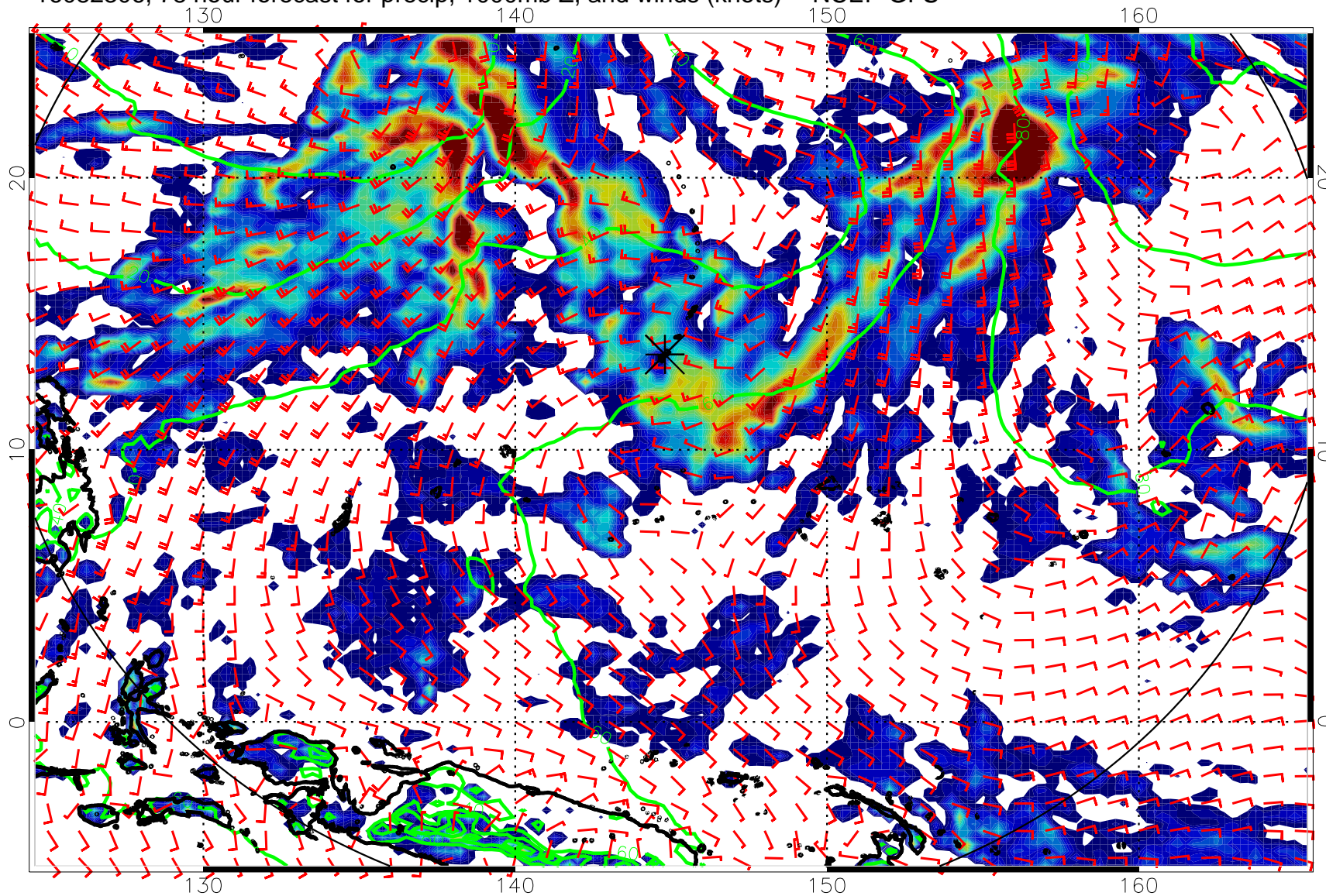
16082306, 78 hour forecast for precip, 1000mb Z, and winds (knots) -- NCEP GFS
