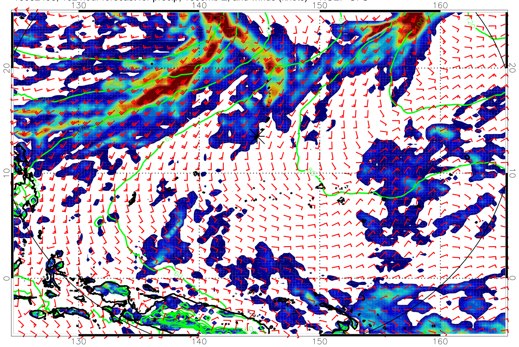
16082406, 102 hour forecast for precip, 1000mb Z, and winds (knots) -- NCEP GFS
