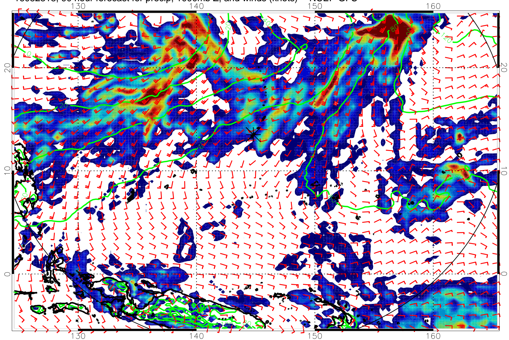
16082318, 90 hour forecast for precip, 1000mb Z, and winds (knots) -- NCEP GFS
