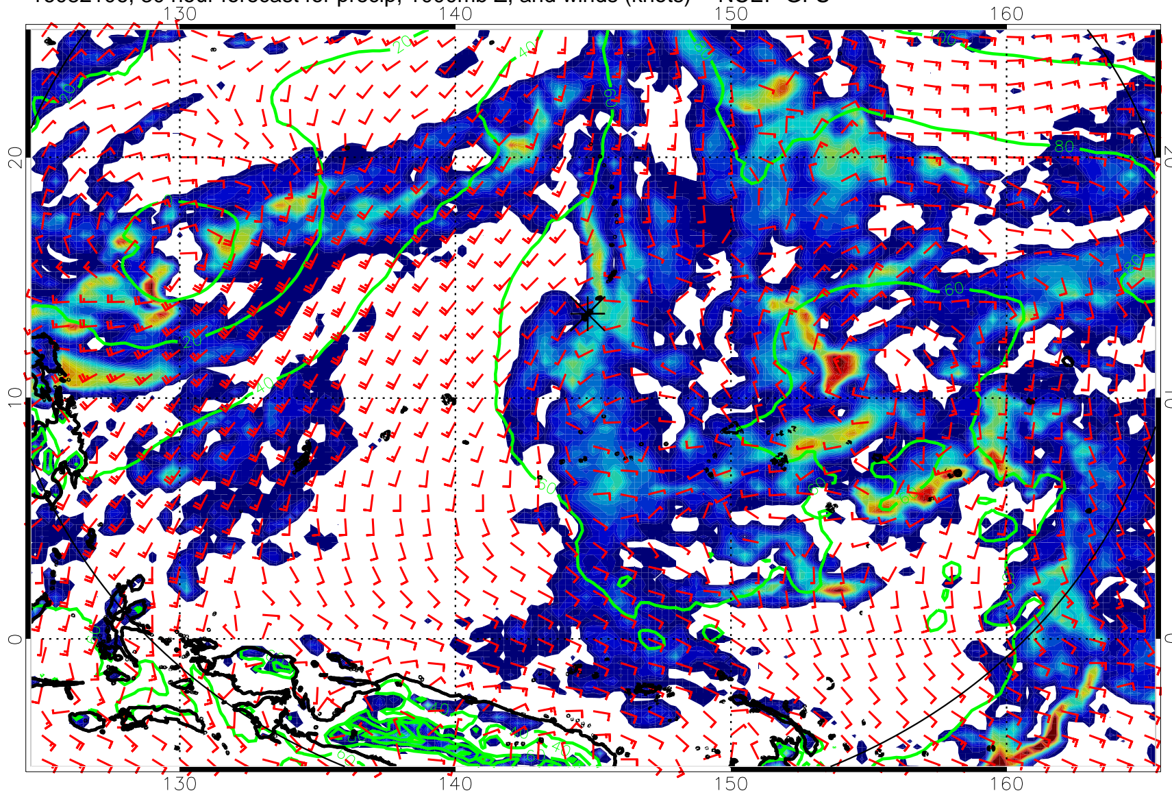
16082106, 30 hour forecast for precip, 1000mb Z, and winds (knots) -- NCEP GFS
