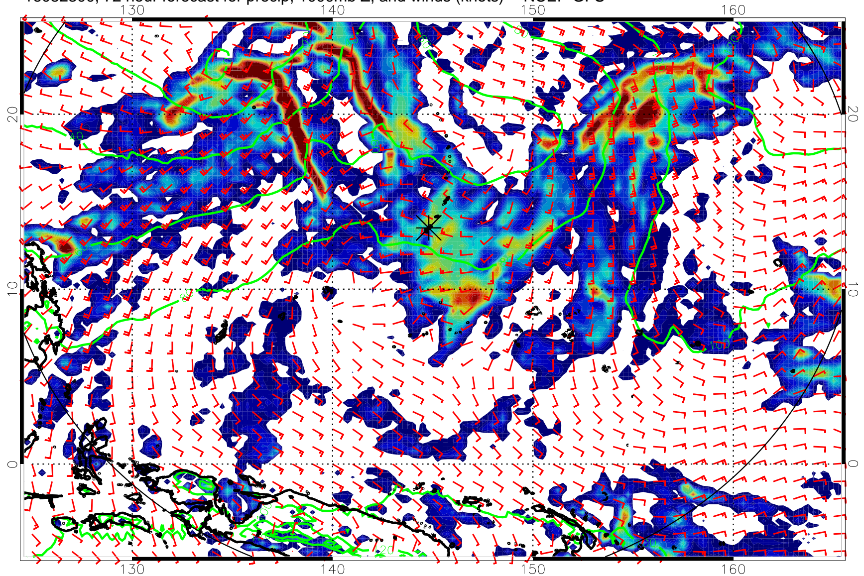
16082300, 72 hour forecast for precip, 1000mb Z, and winds (knots) -- NCEP GFS
