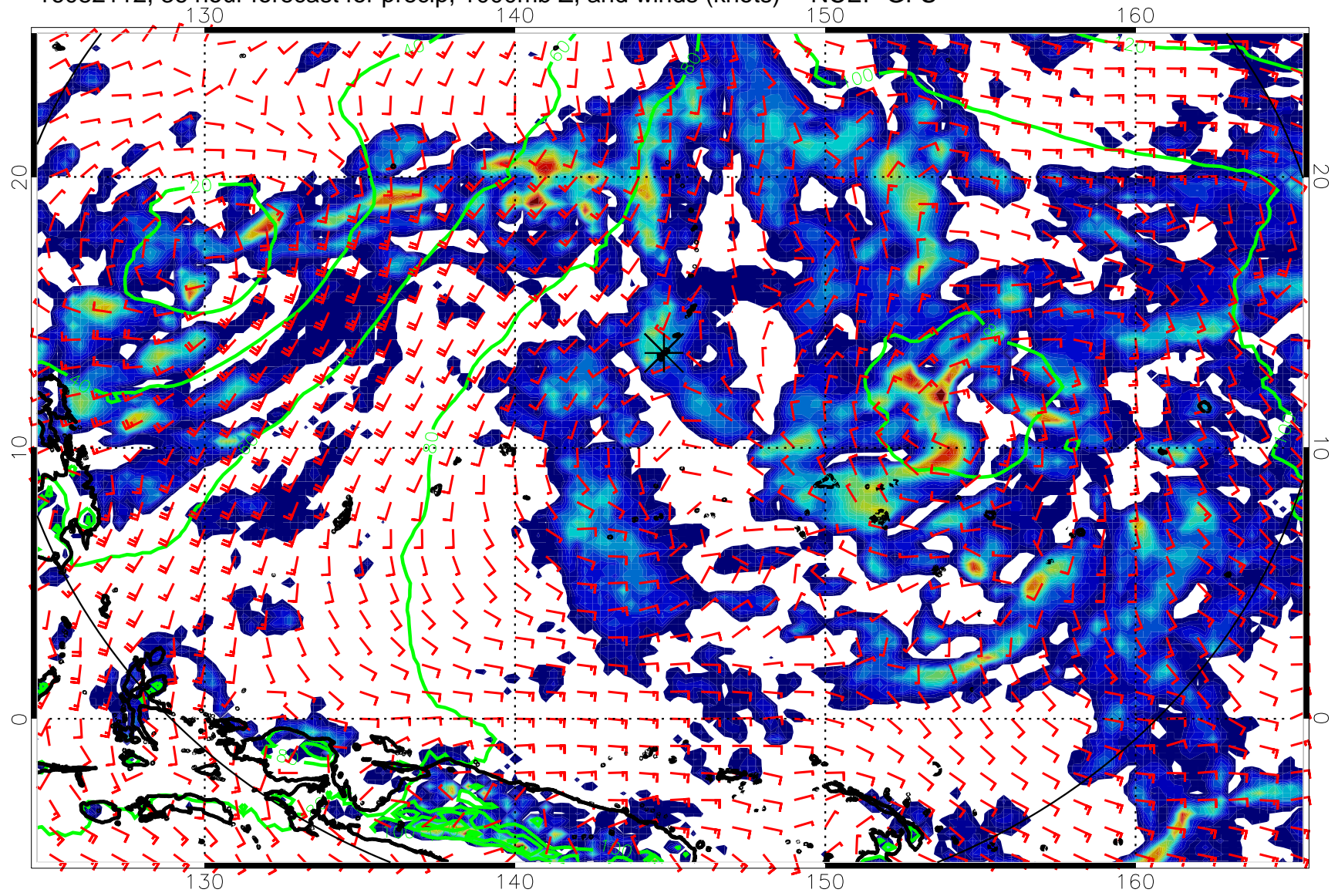
16082112, 36 hour forecast for precip, 1000mb Z, and winds (knots) -- NCEP GFS
