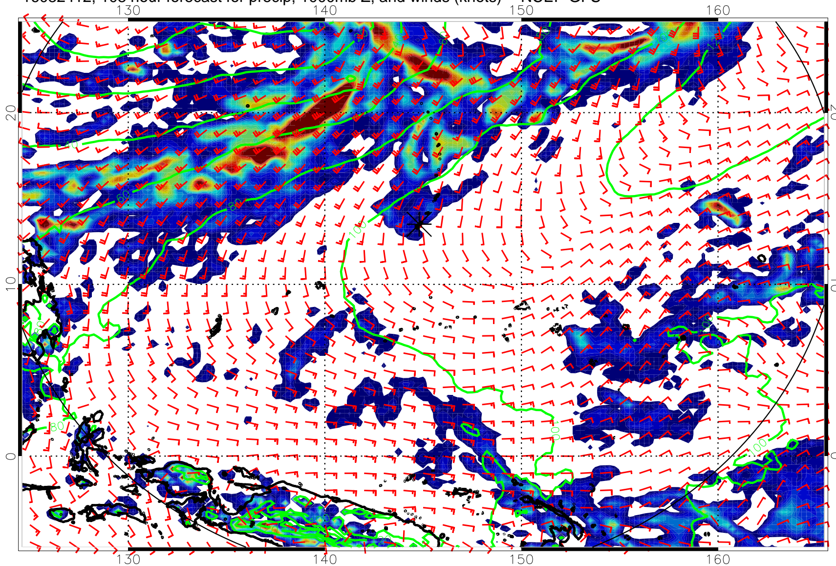
16082412, 108 hour forecast for precip, 1000mb Z, and winds (knots) -- NCEP GFS
