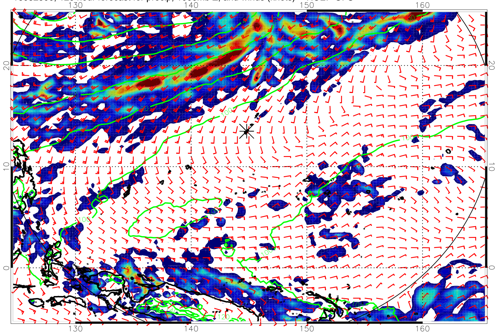
16082500, 120 hour forecast for precip, 1000mb Z, and winds (knots) -- NCEP GFS
