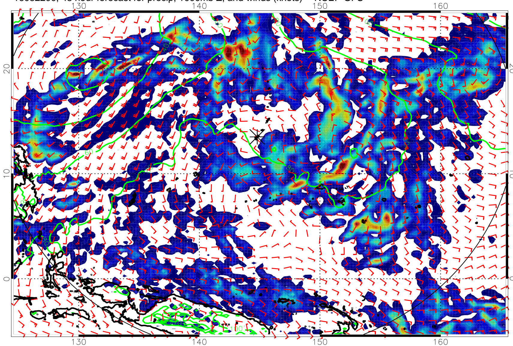
16082200, 48 hour forecast for precip, 1000mb Z, and winds (knots) -- NCEP GFS
