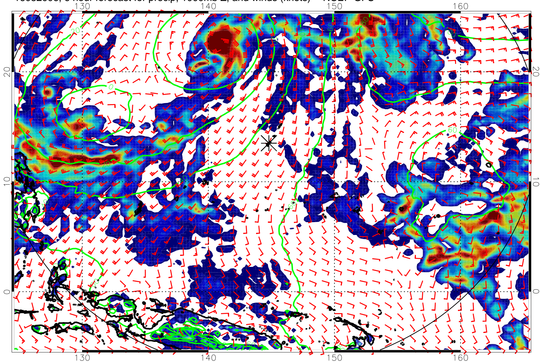
16082006, 6 hour forecast for precip, 1000mb Z, and winds (knots) -- NCEP GFS
