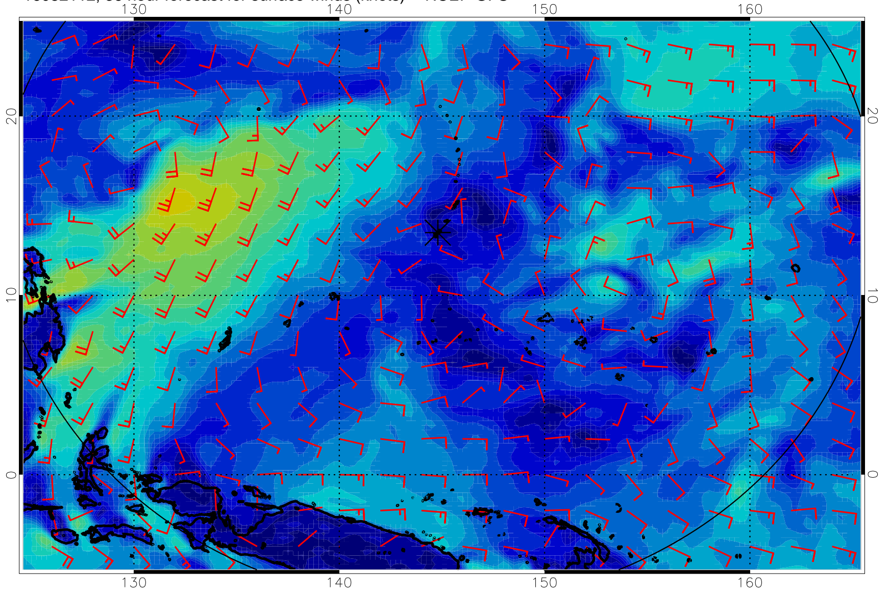
16082112, 36 hour forecast for surface winds (knots) -- NCEP GFS
