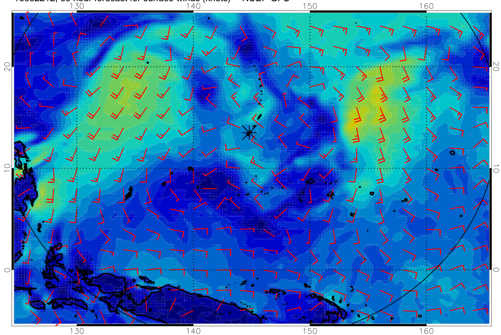
16082212, 60 hour forecast for surface winds (knots) -- NCEP GFS
