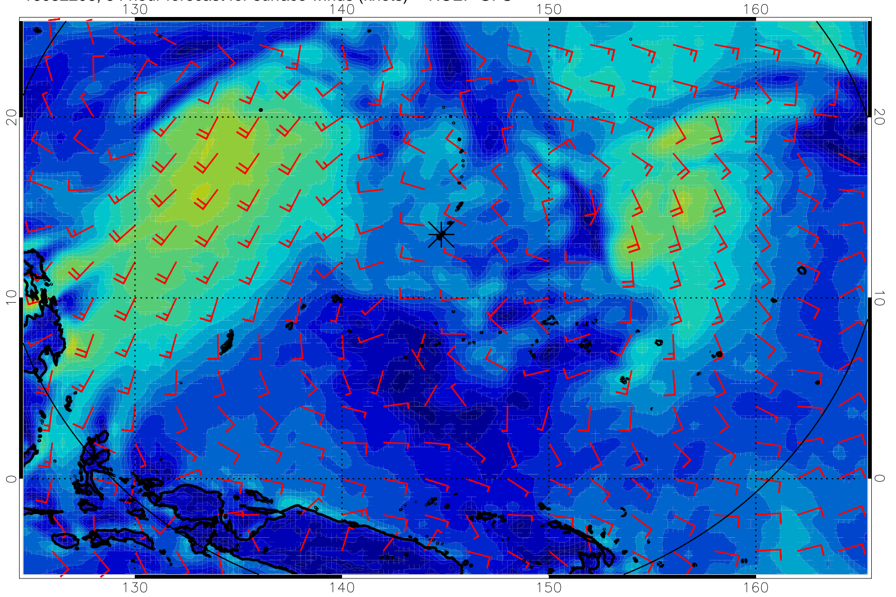
16082206, 54 hour forecast for surface winds (knots) -- NCEP GFS
