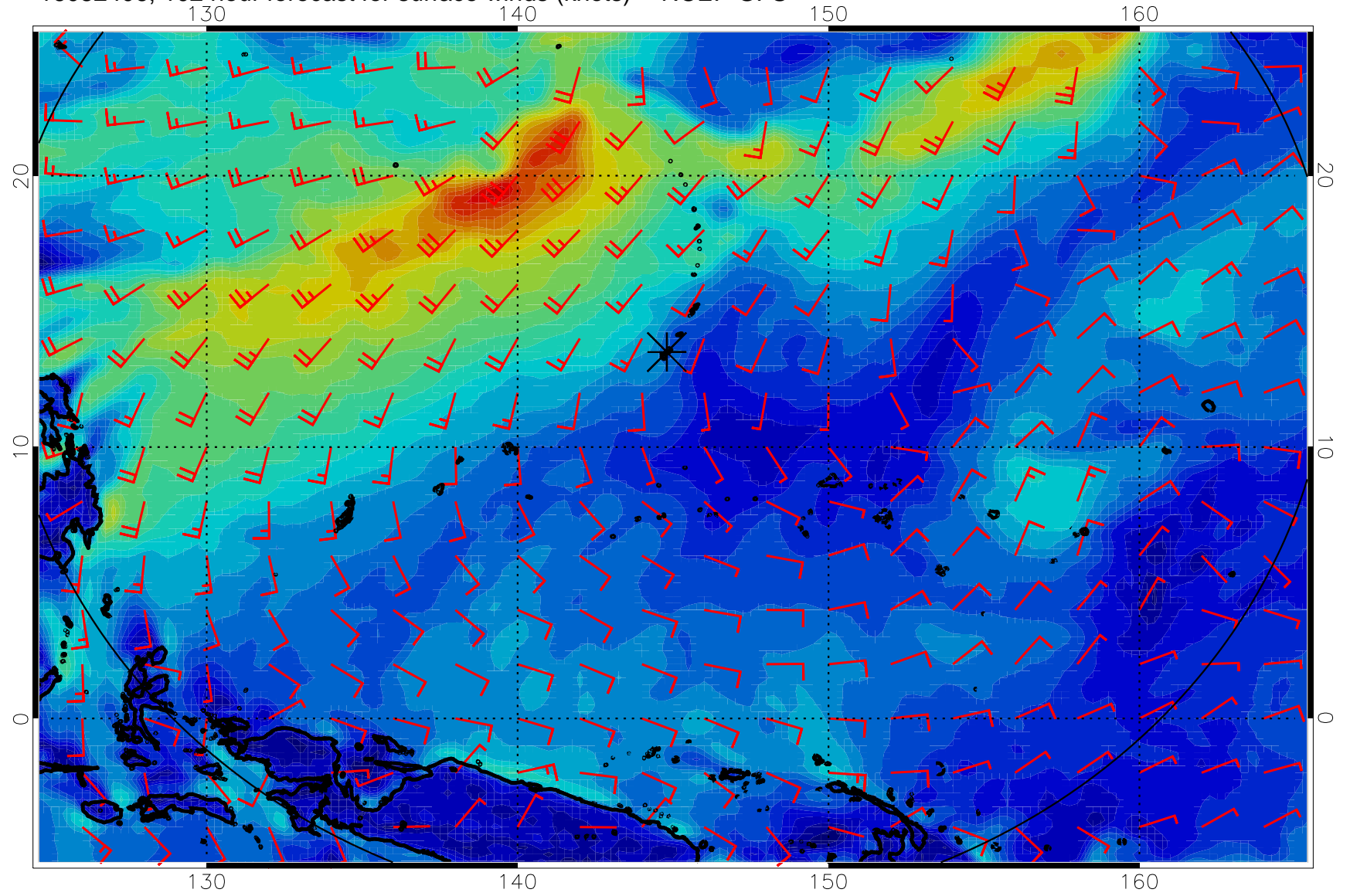
16082406, 102 hour forecast for surface winds (knots) -- NCEP GFS
