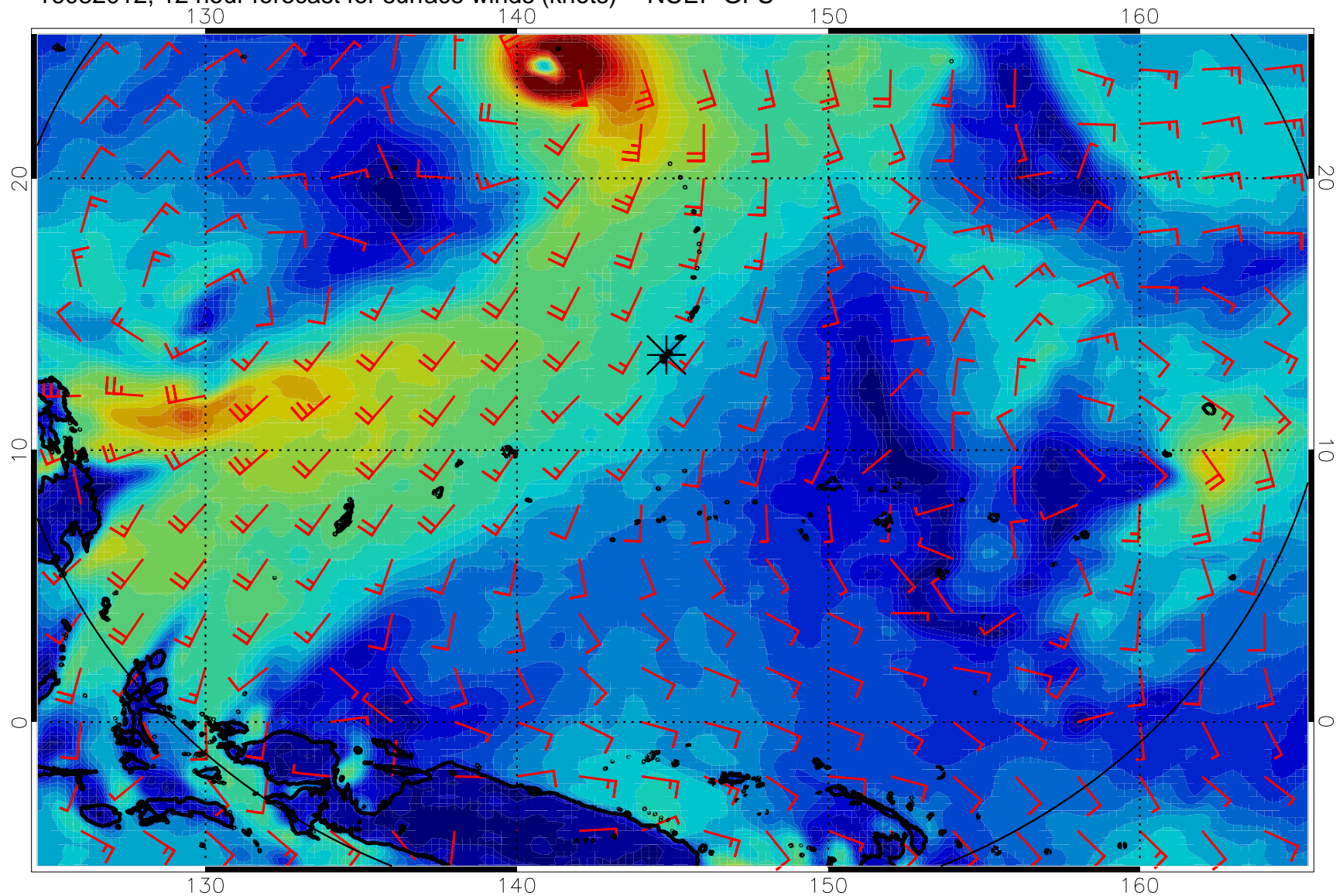
16082012, 12 hour forecast for surface winds (knots) -- NCEP GFS
