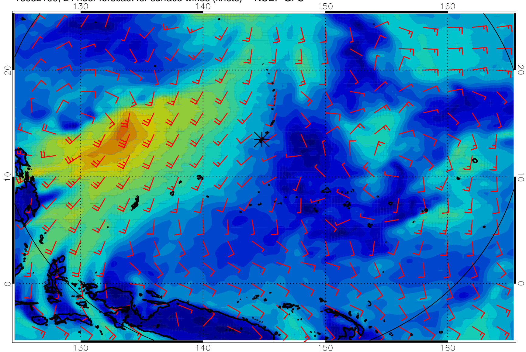
16082100, 24 hour forecast for surface winds (knots) -- NCEP GFS
