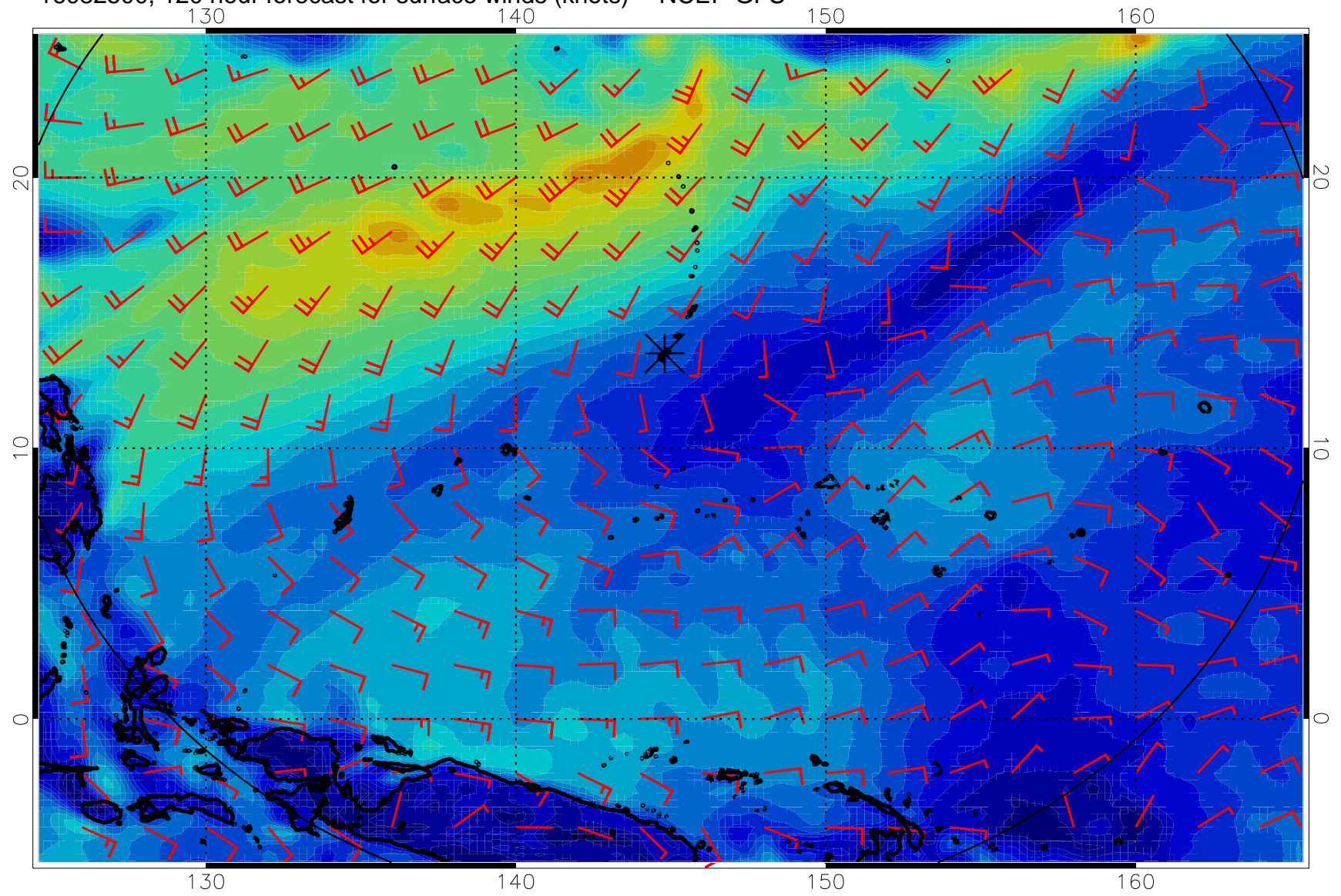
16082500, 120 hour forecast for surface winds (knots) -- NCEP GFS
