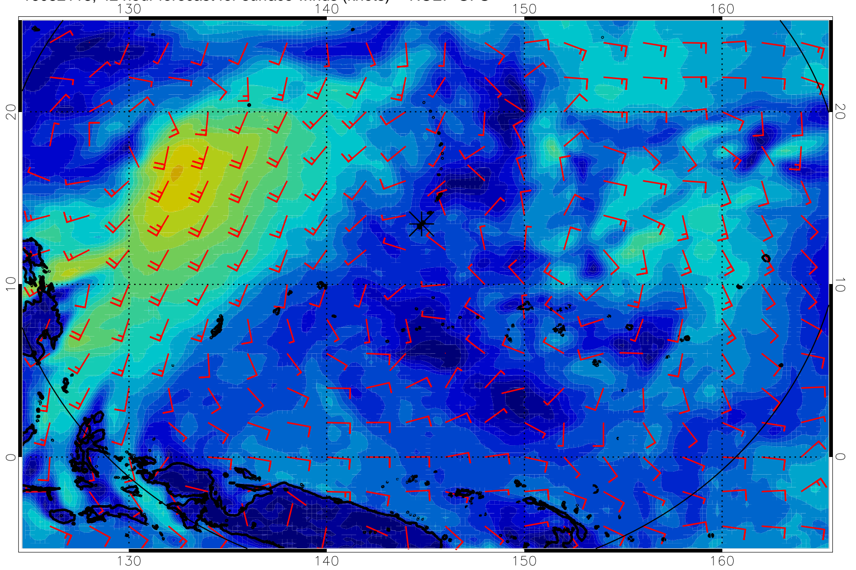
16082118, 42 hour forecast for surface winds (knots) -- NCEP GFS
