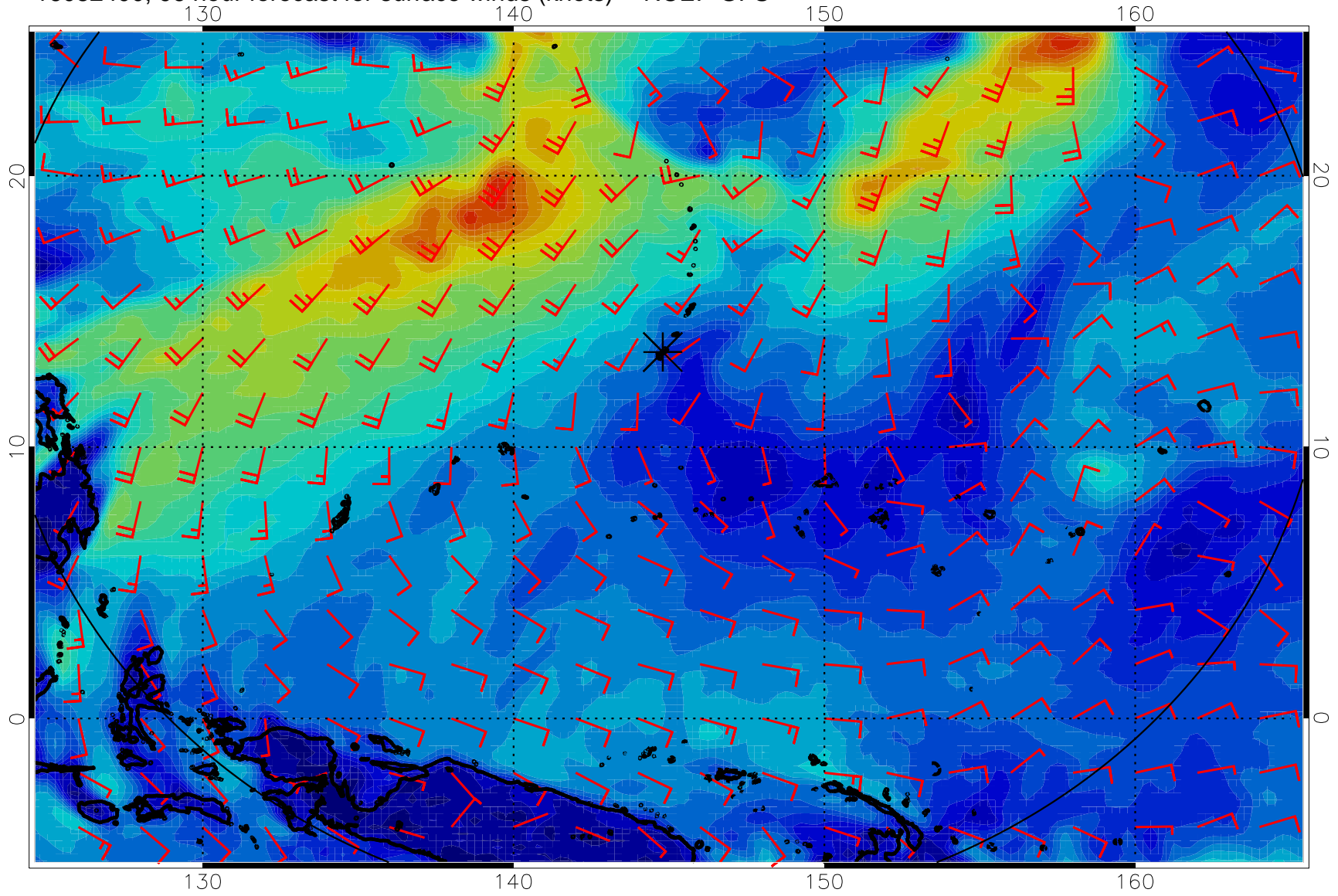
16082400, 96 hour forecast for surface winds (knots) -- NCEP GFS
