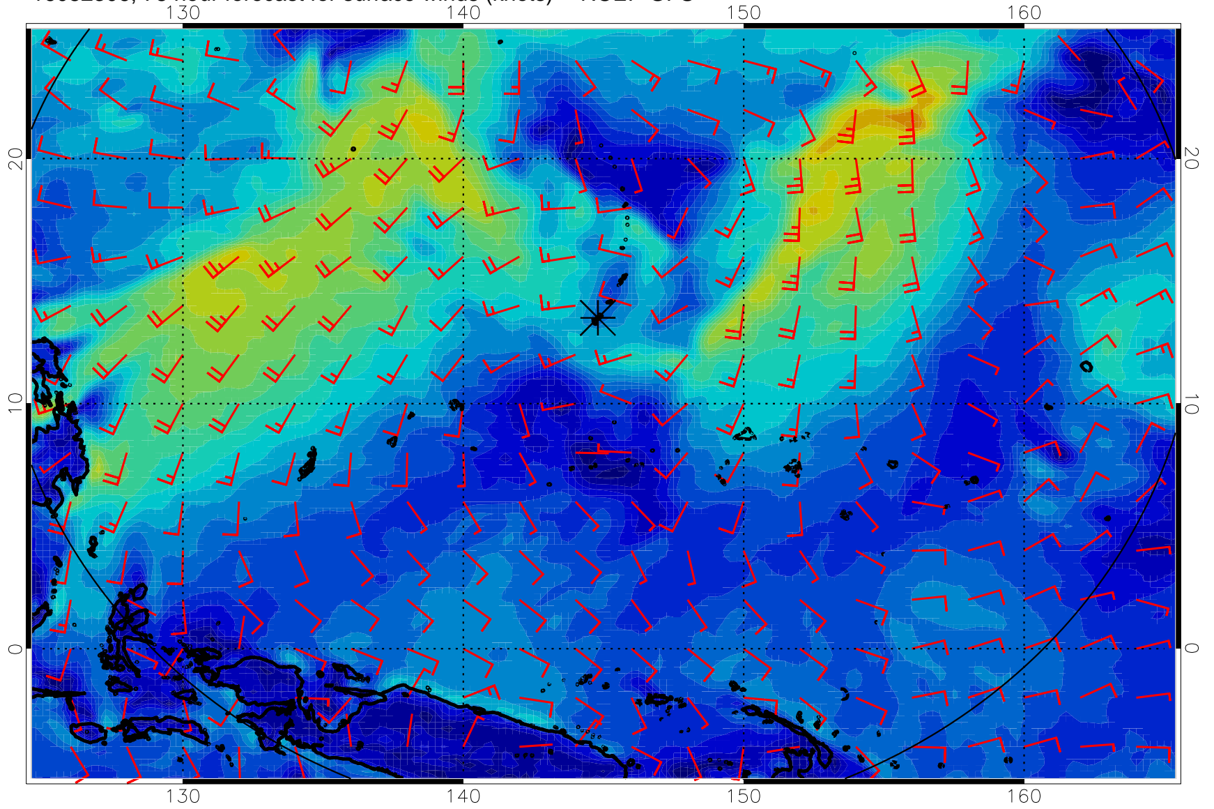
16082306, 78 hour forecast for surface winds (knots) -- NCEP GFS
