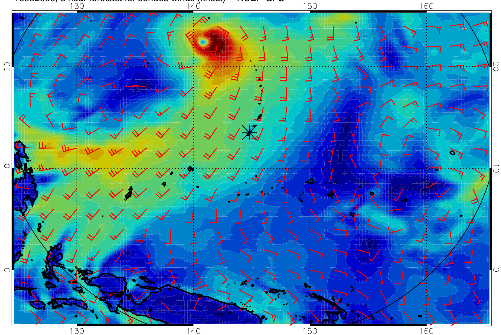
16082006, 6 hour forecast for surface winds (knots) -- NCEP GFS
