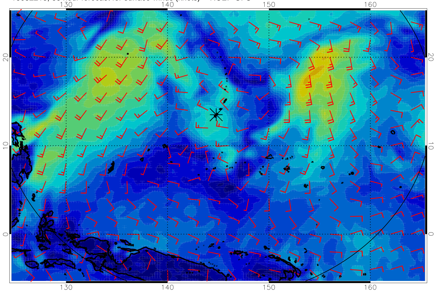
16082218, 66 hour forecast for surface winds (knots) -- NCEP GFS
