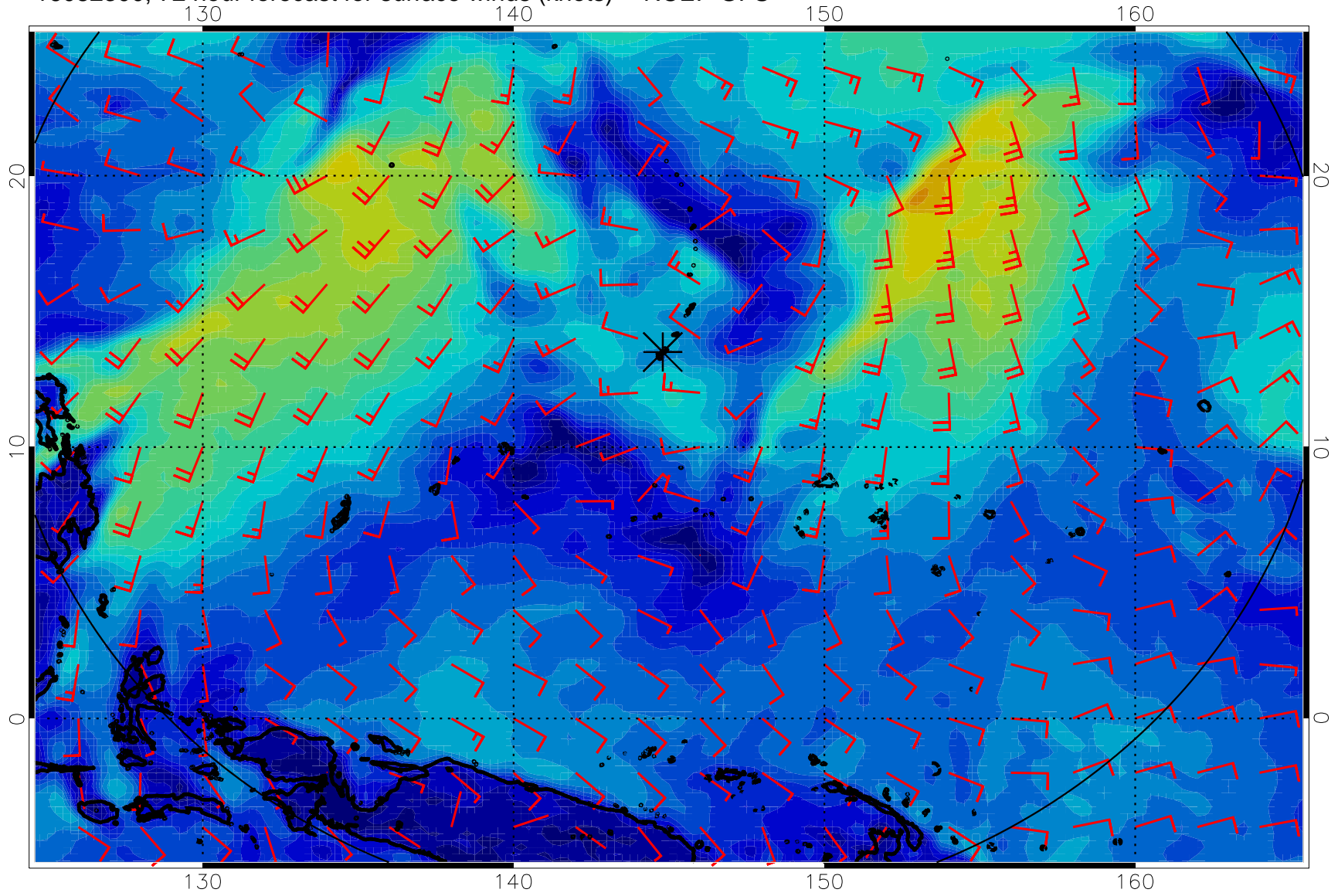
16082300, 72 hour forecast for surface winds (knots) -- NCEP GFS
