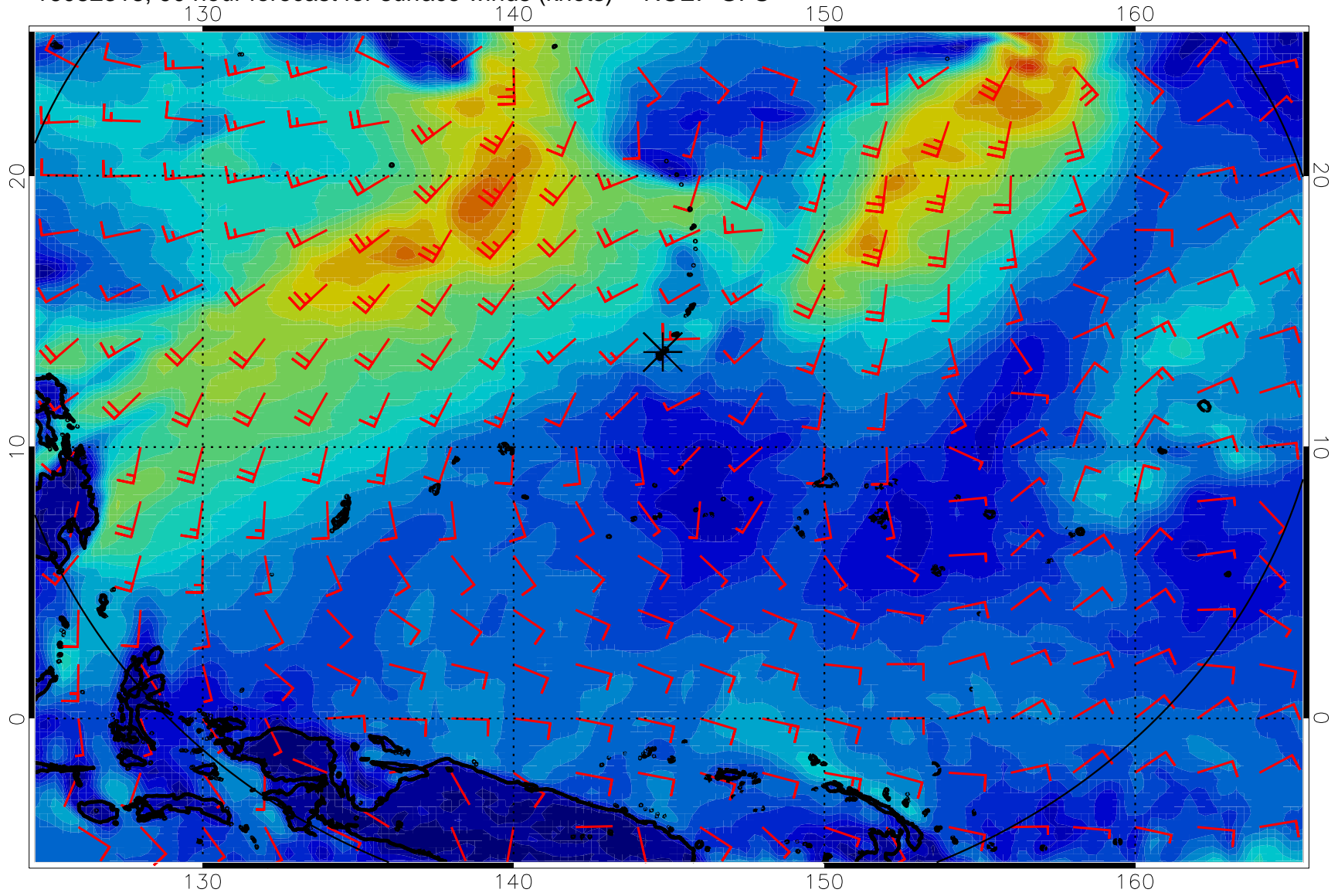
16082318, 90 hour forecast for surface winds (knots) -- NCEP GFS
