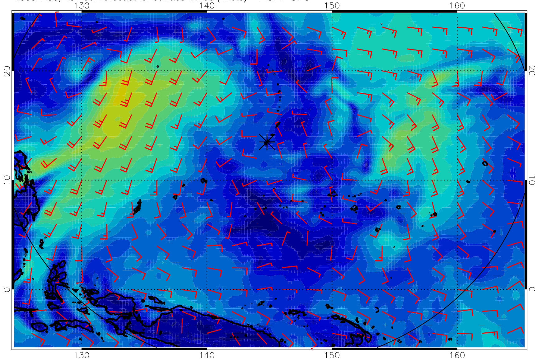
16082200, 48 hour forecast for surface winds (knots) -- NCEP GFS
