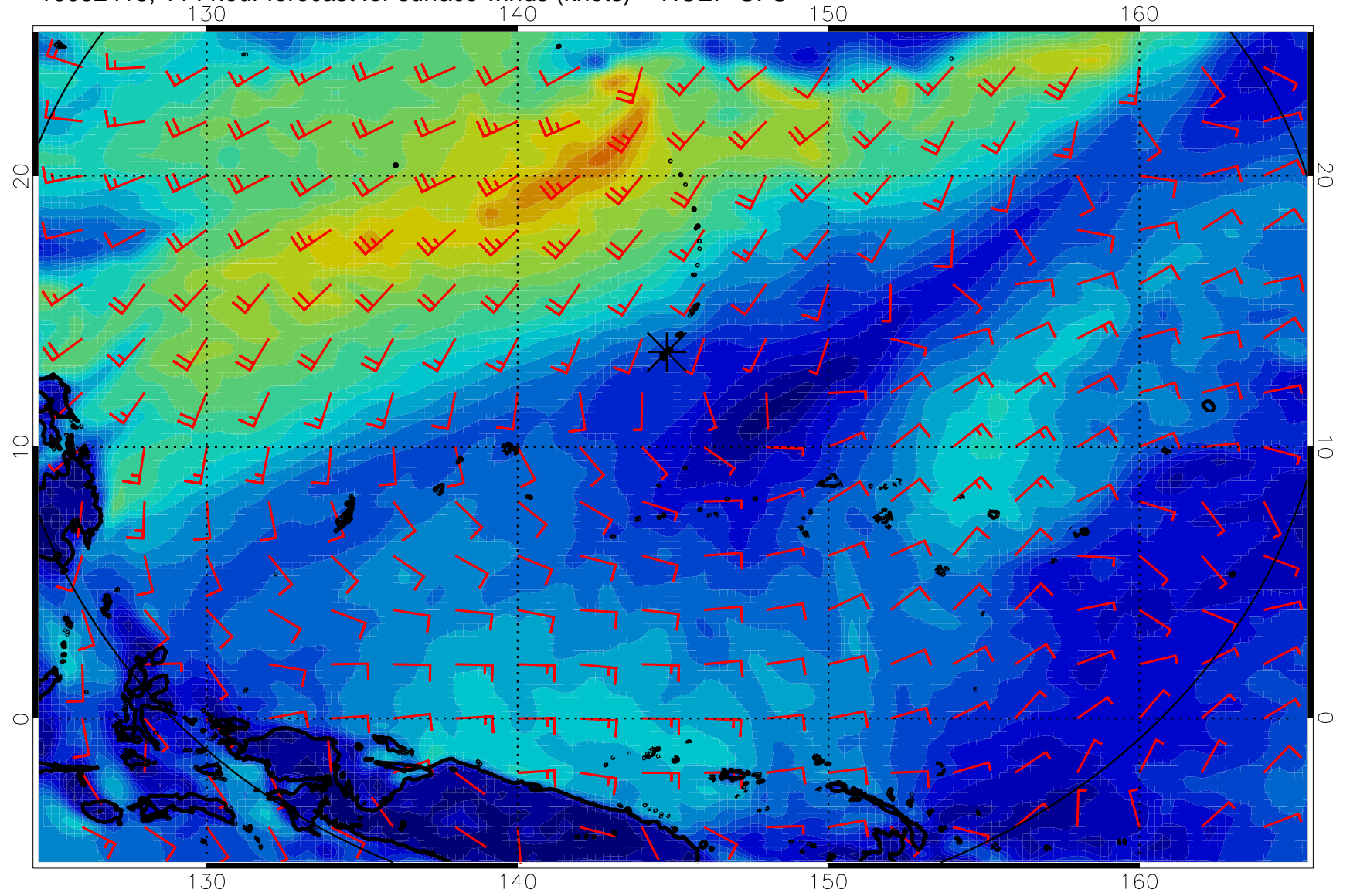
16082418, 114 hour forecast for surface winds (knots) -- NCEP GFS
