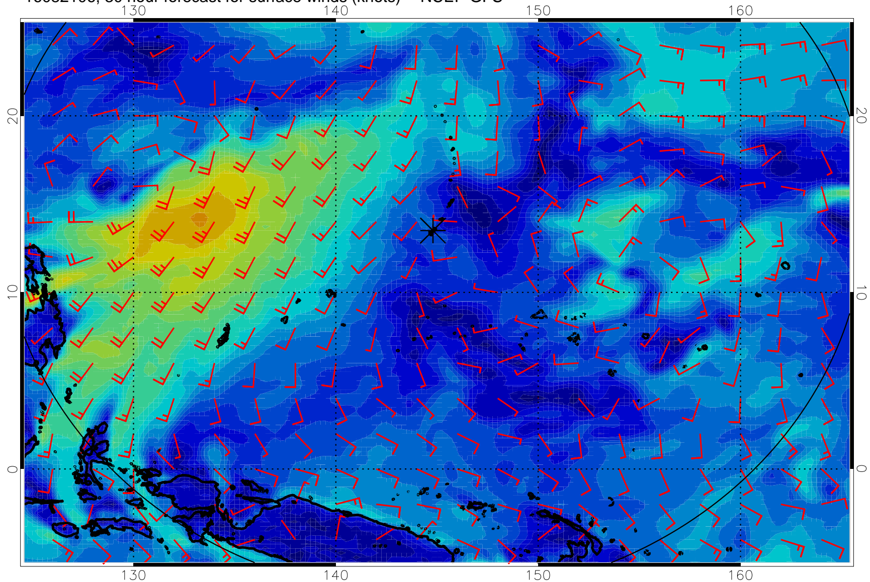
16082106, 30 hour forecast for surface winds (knots) -- NCEP GFS
