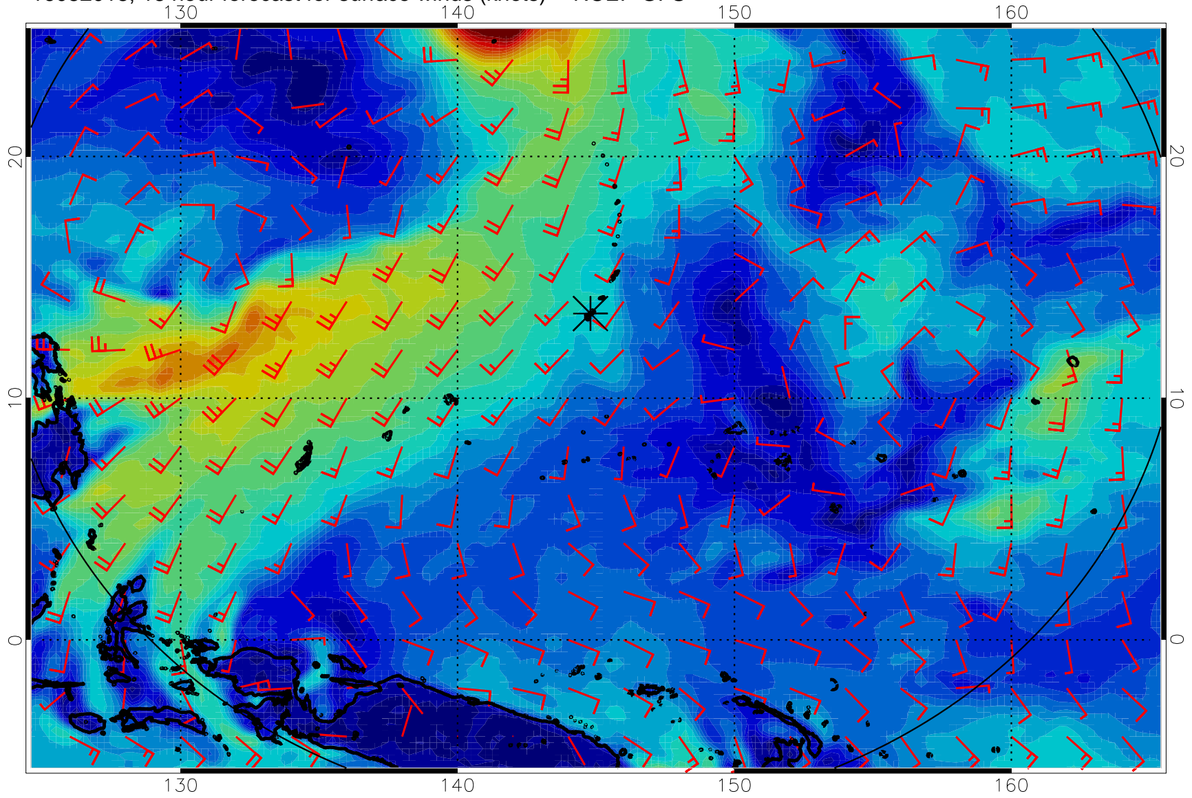
16082018, 18 hour forecast for surface winds (knots) -- NCEP GFS
