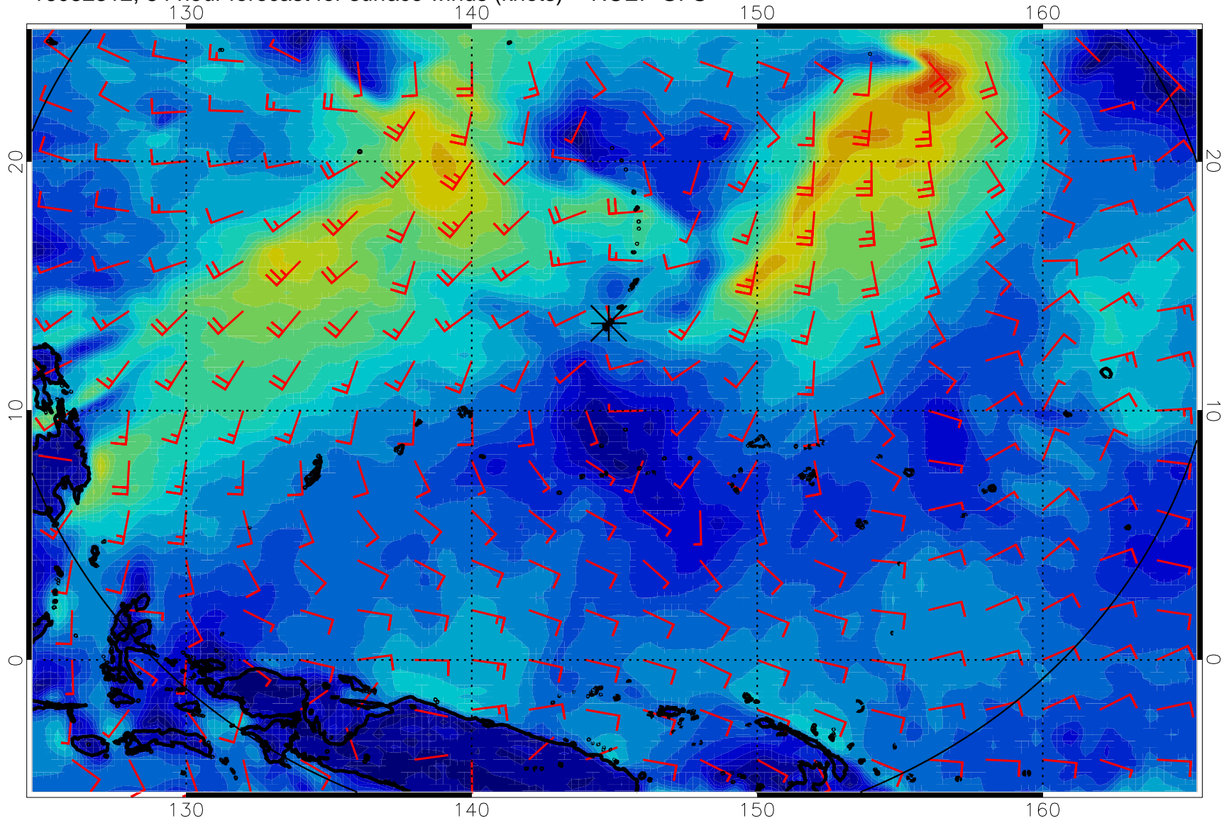
16082312, 84 hour forecast for surface winds (knots) -- NCEP GFS
