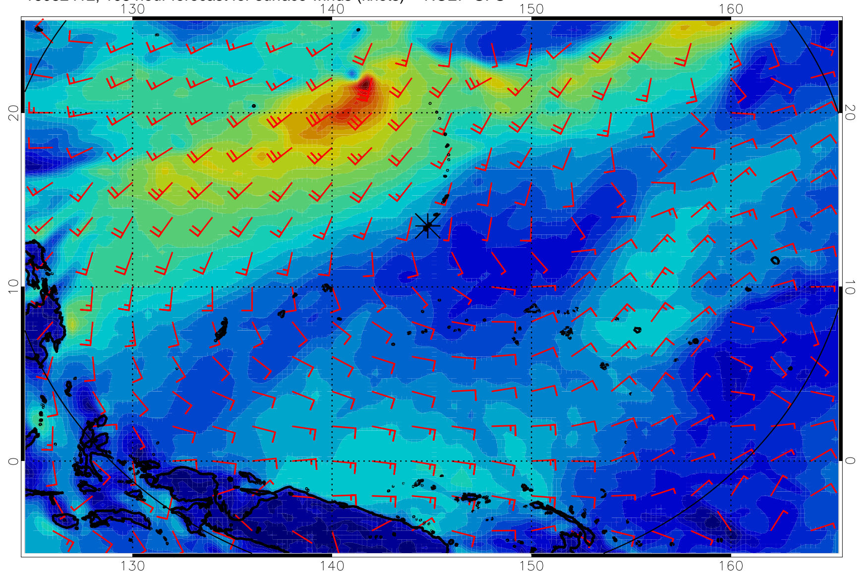
16082412, 108 hour forecast for surface winds (knots) -- NCEP GFS
