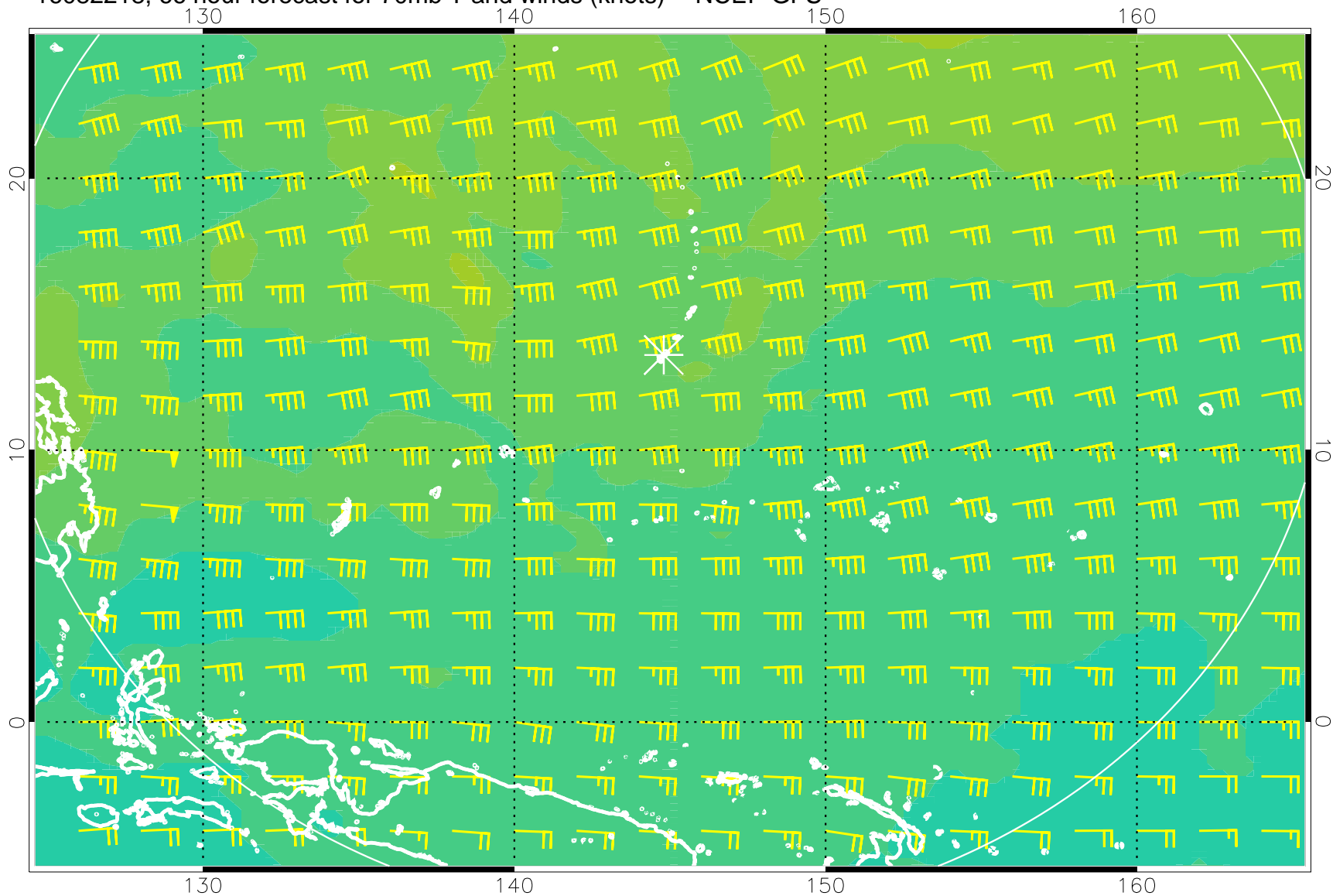
16082218, 66 hour forecast for 70mb T and winds (knots) -- NCEP GFS
