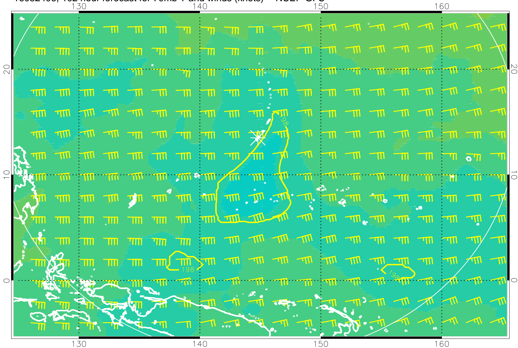
16082406, 102 hour forecast for 70mb T and winds (knots) -- NCEP GFS
