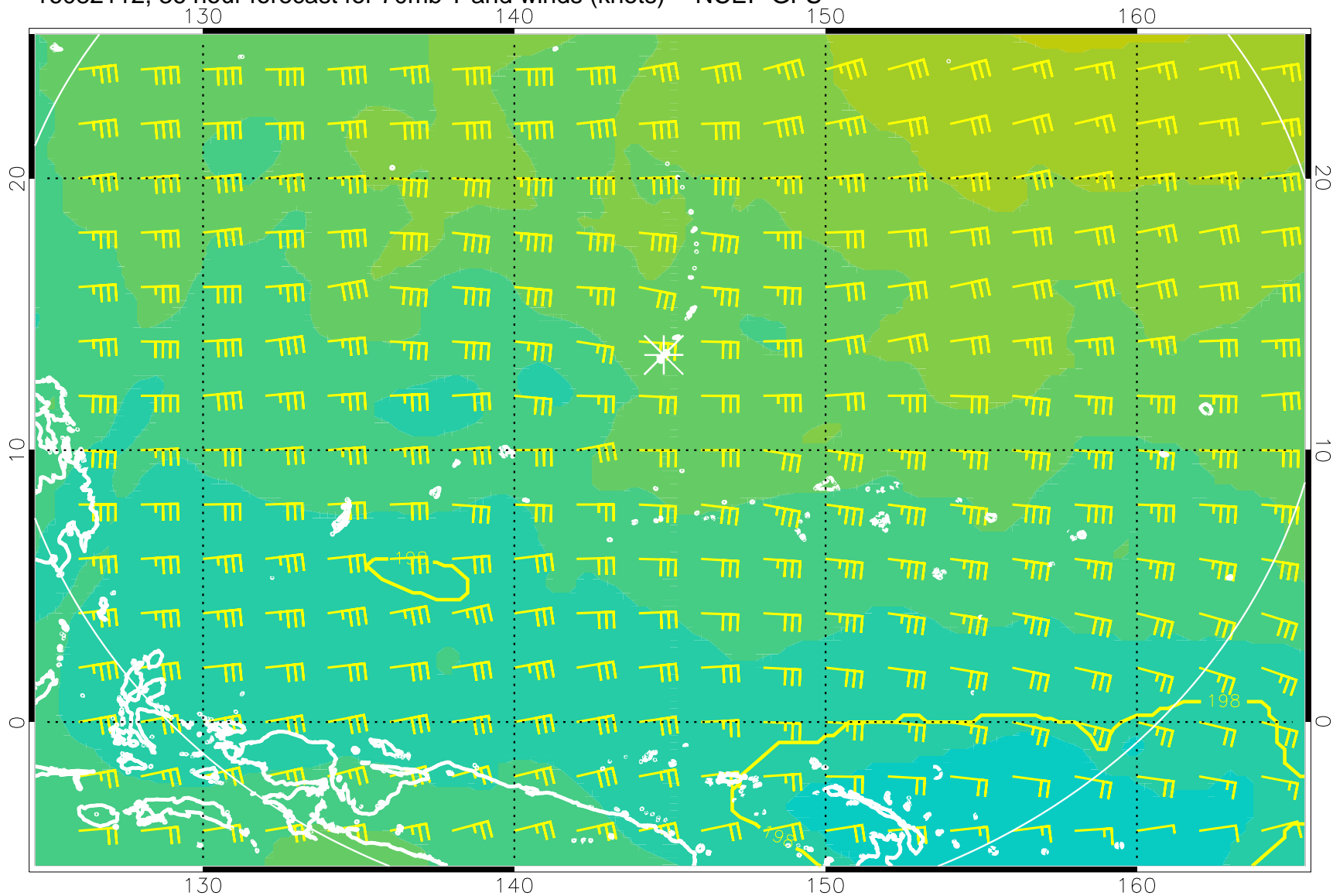
16082112, 36 hour forecast for 70mb T and winds (knots) -- NCEP GFS
