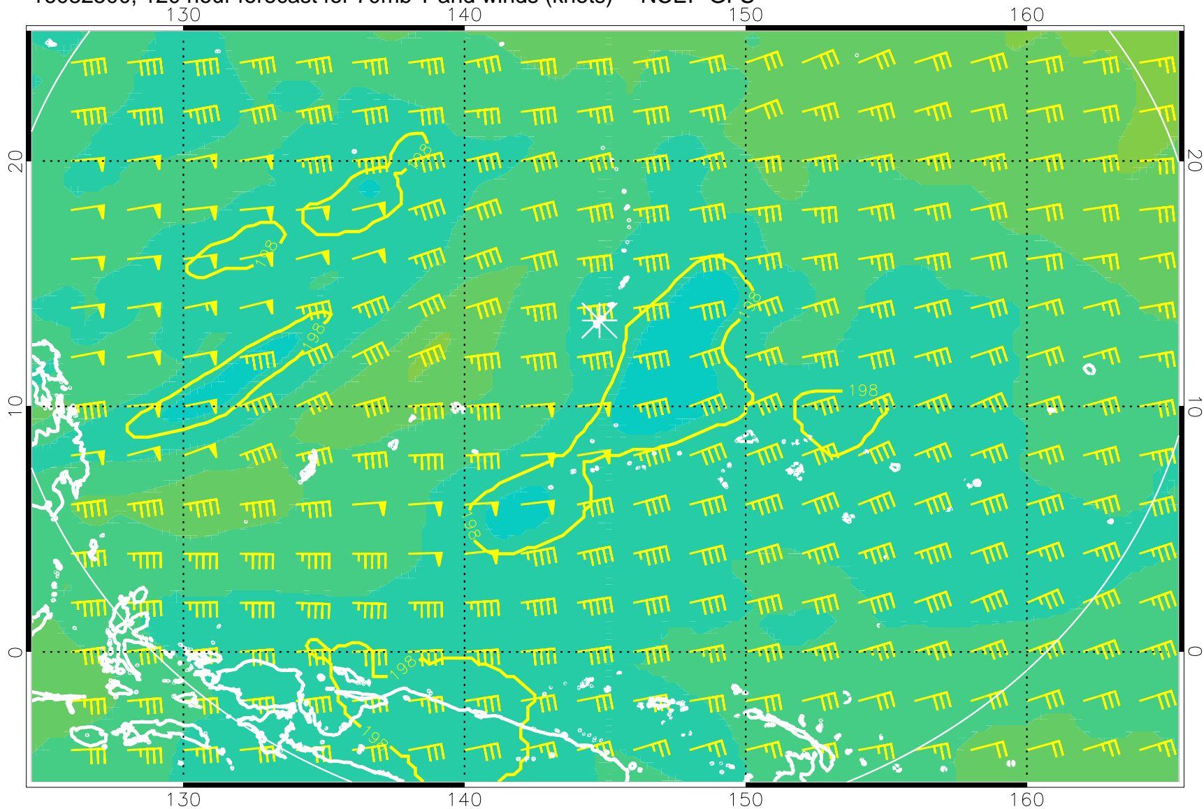
16082500, 120 hour forecast for 70mb T and winds (knots) -- NCEP GFS
