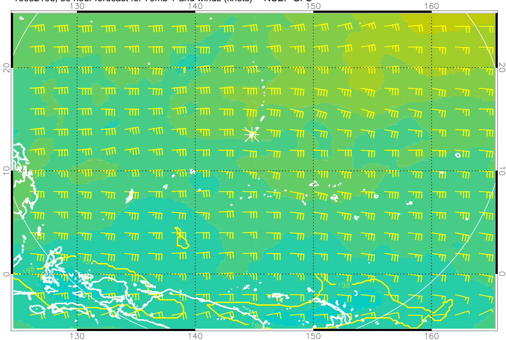
16082106, 30 hour forecast for 70mb T and winds (knots) -- NCEP GFS
