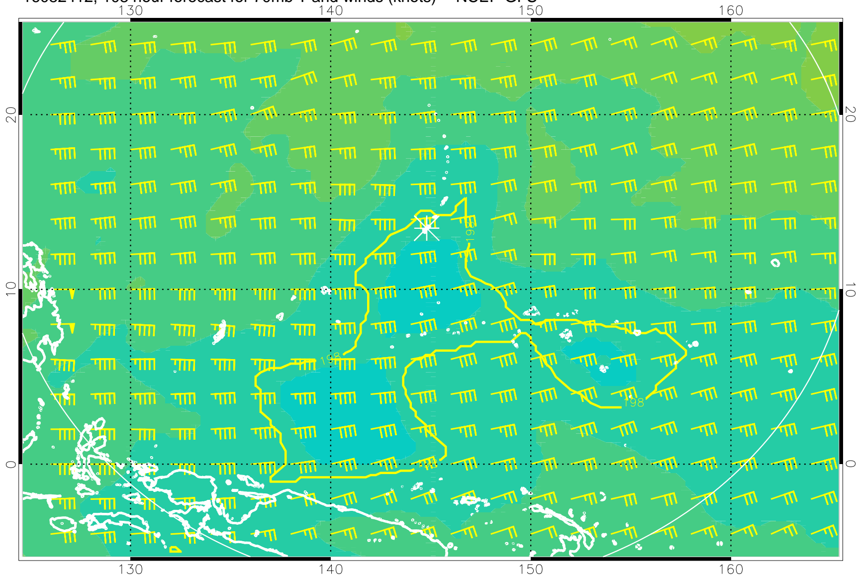
16082412, 108 hour forecast for 70mb T and winds (knots) -- NCEP GFS
