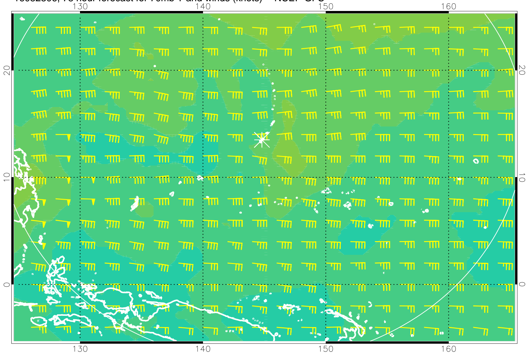
16082306, 78 hour forecast for 70mb T and winds (knots) -- NCEP GFS
