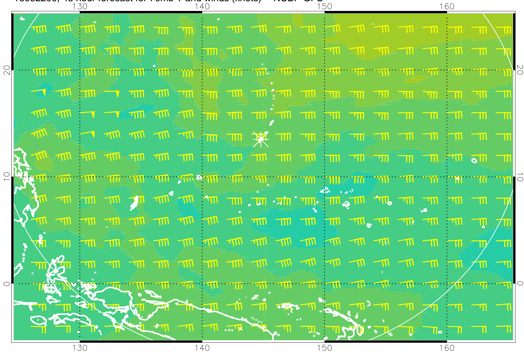
16082200, 48 hour forecast for 70mb T and winds (knots) -- NCEP GFS
