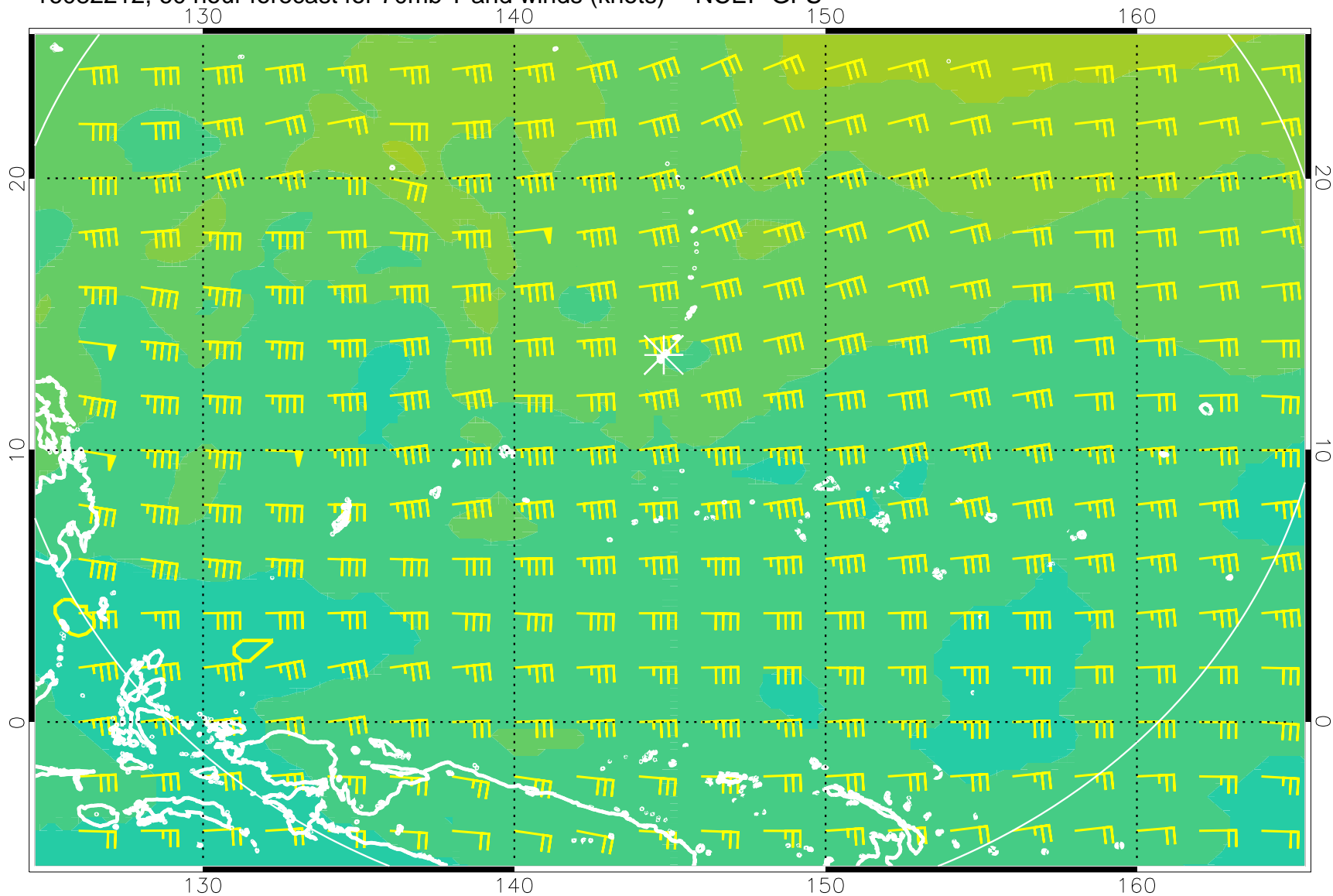
16082212, 60 hour forecast for 70mb T and winds (knots) -- NCEP GFS
