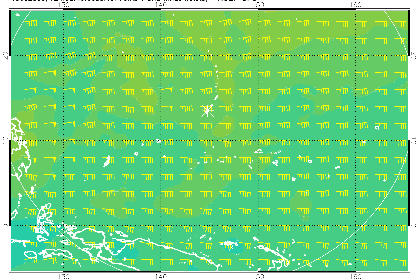
16082300, 72 hour forecast for 70mb T and winds (knots) -- NCEP GFS
