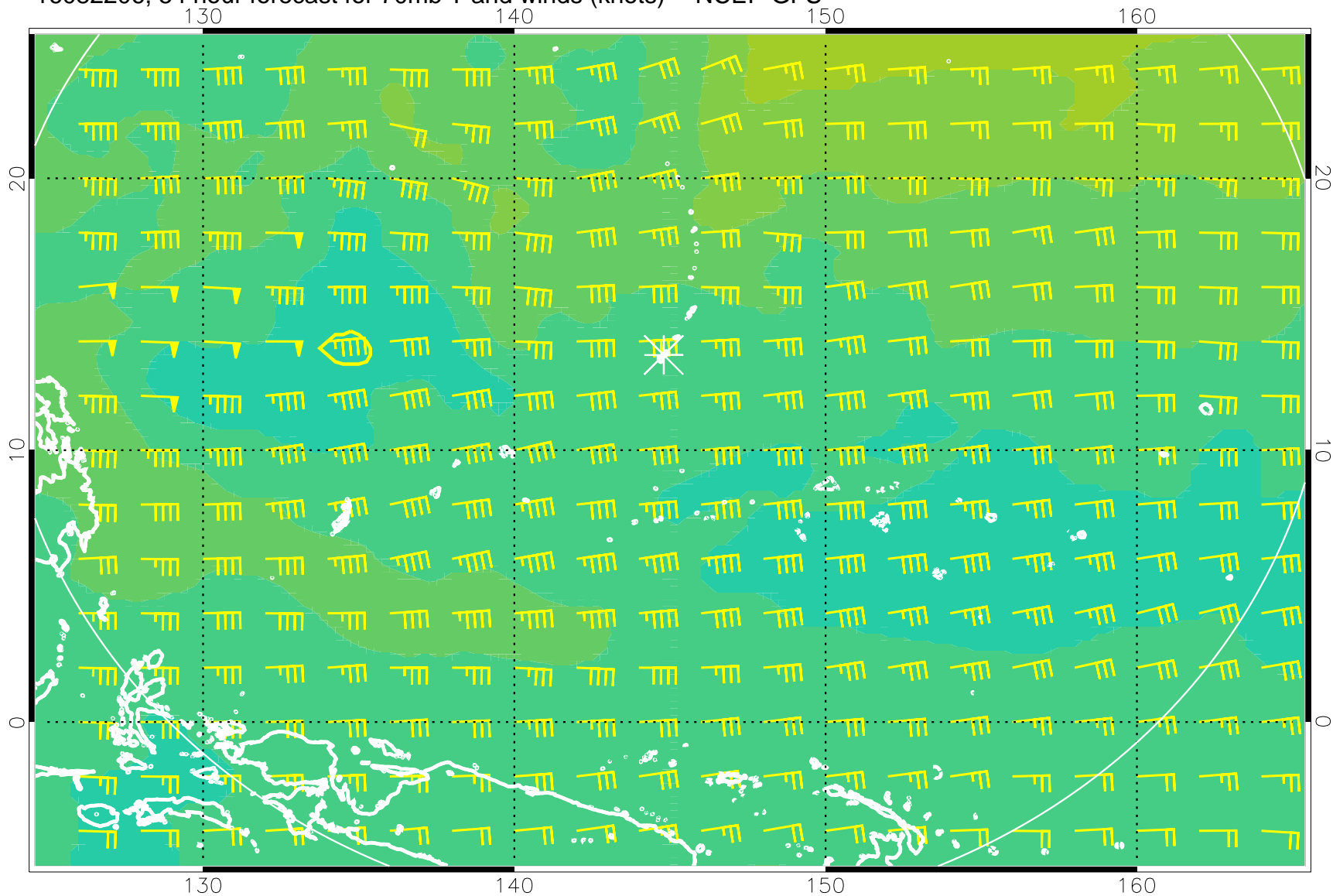
16082206, 54 hour forecast for 70mb T and winds (knots) -- NCEP GFS
