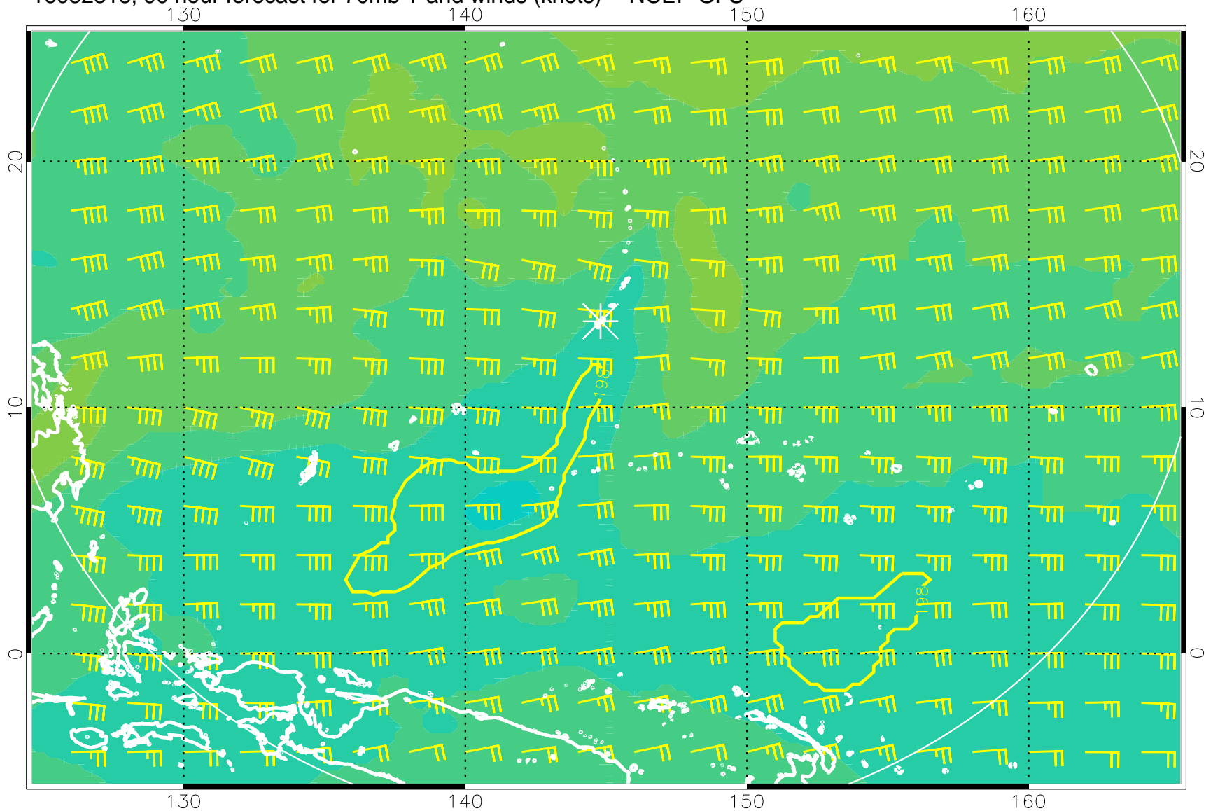
16082318, 90 hour forecast for 70mb T and winds (knots) -- NCEP GFS
