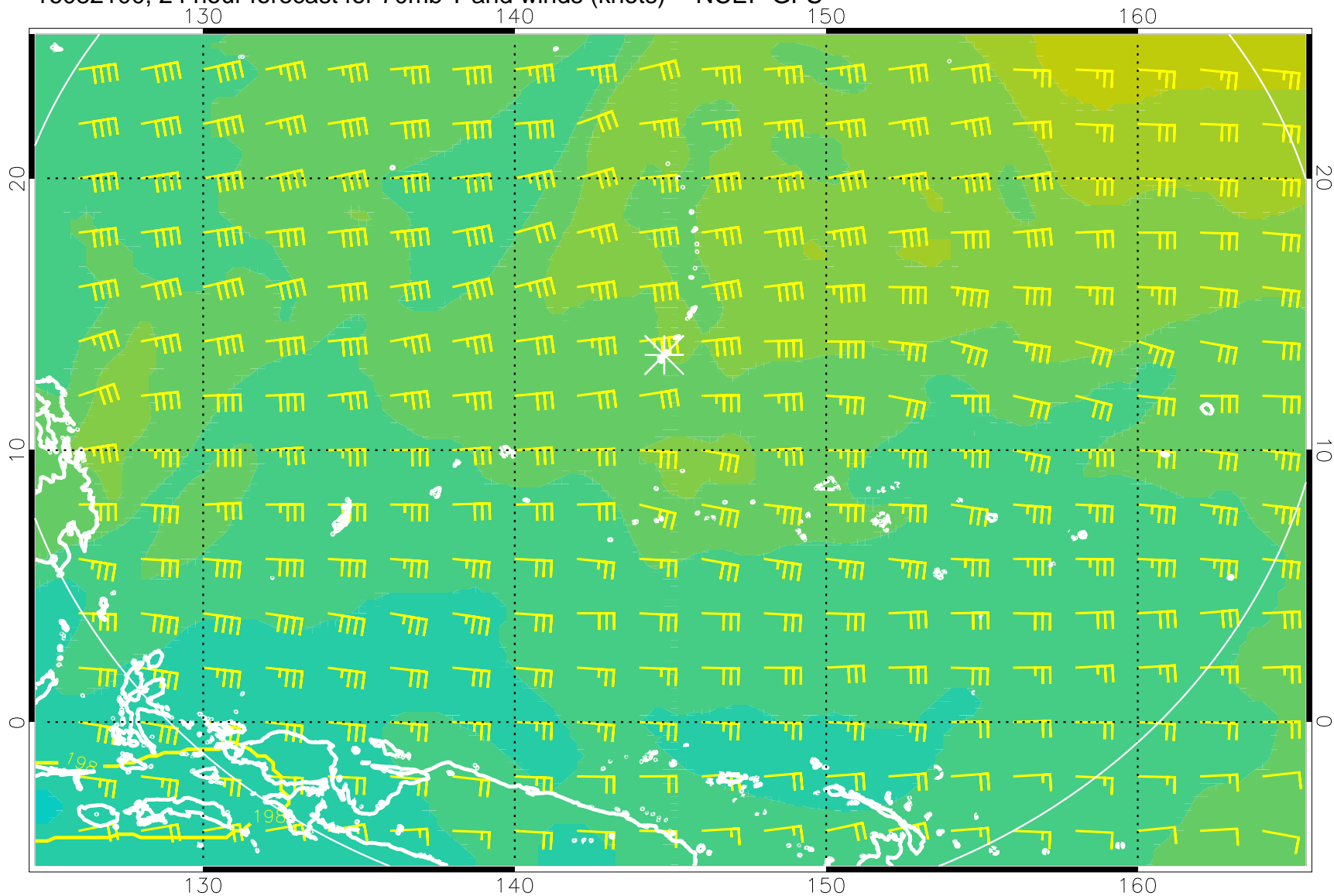
16082100, 24 hour forecast for 70mb T and winds (knots) -- NCEP GFS
