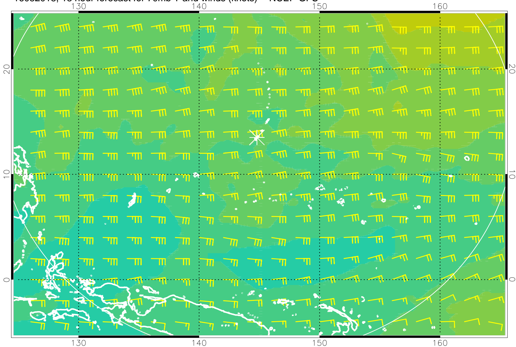
16082018, 18 hour forecast for 70mb T and winds (knots) -- NCEP GFS
