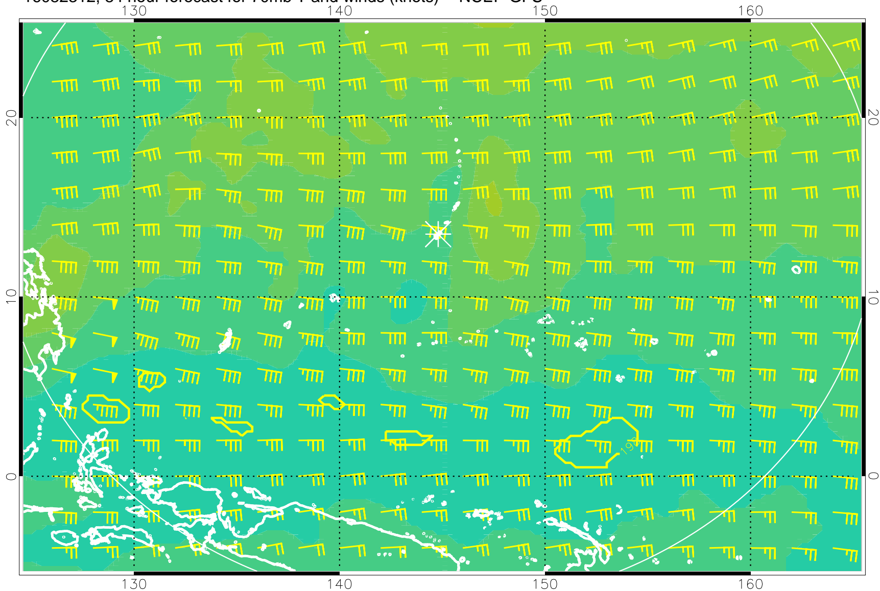
16082312, 84 hour forecast for 70mb T and winds (knots) -- NCEP GFS
