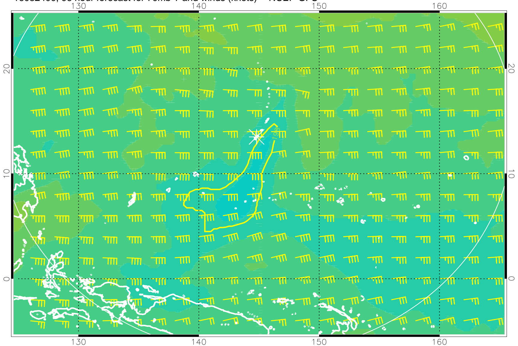
16082400, 96 hour forecast for 70mb T and winds (knots) -- NCEP GFS
